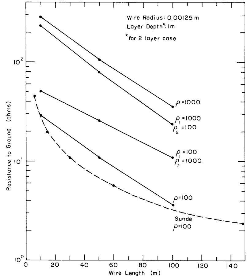
Figure 4. Resistance to ground as a function of electrode length for a horizontal wire lying on various one- and two-layer earth models.
