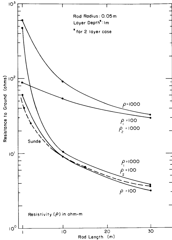
Figure 3. Resistance to ground as a function of electrode length for a vertical rod placed in various one- and two-layer earth models.
