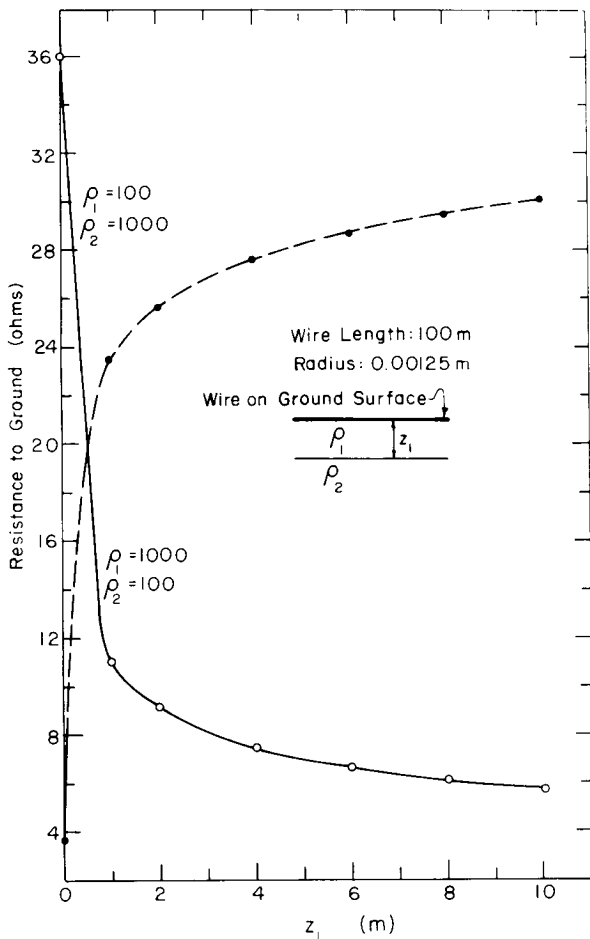
Figure 6. Resistance to ground of a horizontal wire resting on the surface as a function of first-layer thickness z_1 .
