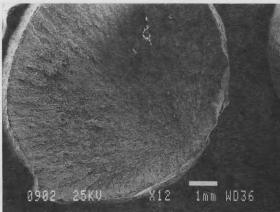
Figure B3. Beam A6, bar 1 (magnification \times 12 ).
