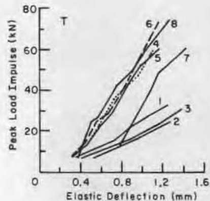
Figure 11. Elastic deflections of unreinforced beams prior to cracking of the concrete.
