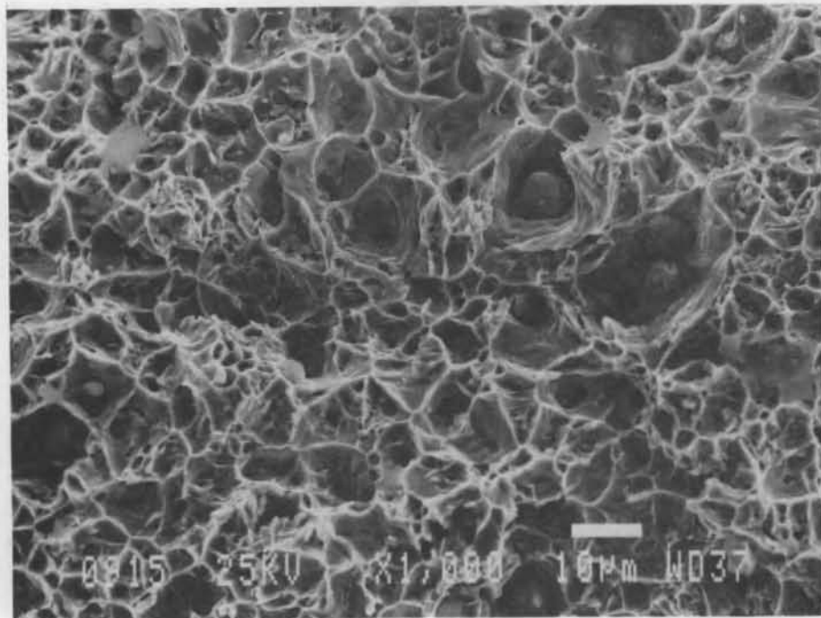
Figure B10. Beam D3 (magnification \times 1000 ).
