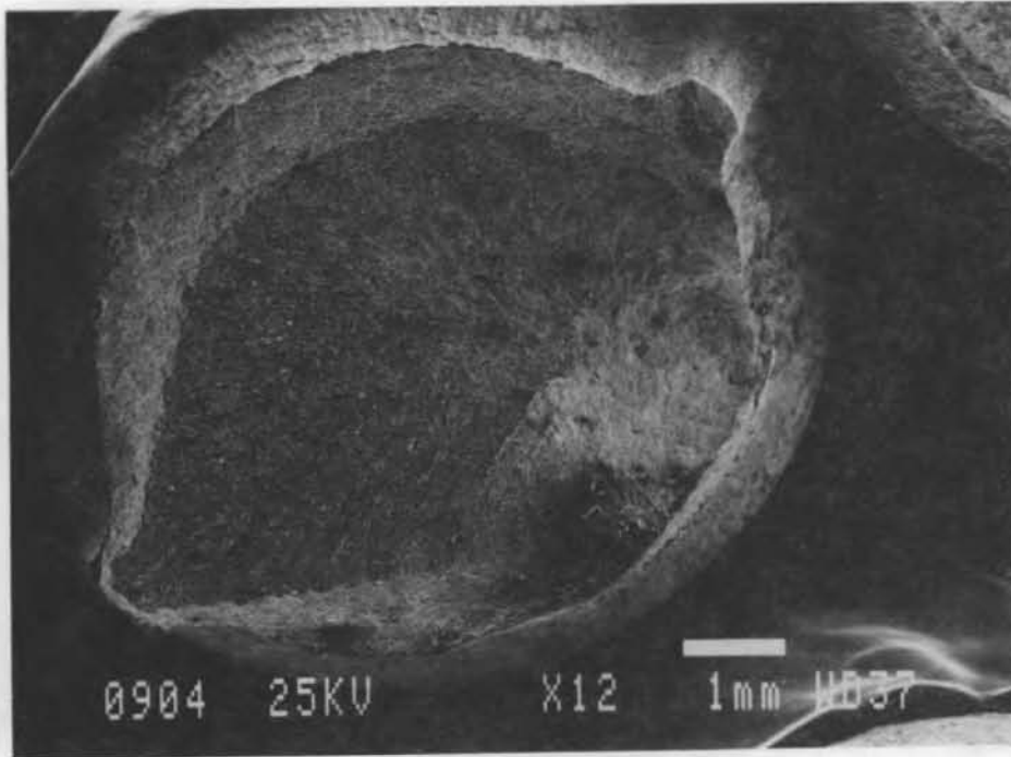
Figure B5. Beam A6, bar 2 (magnification \times 12 ).
