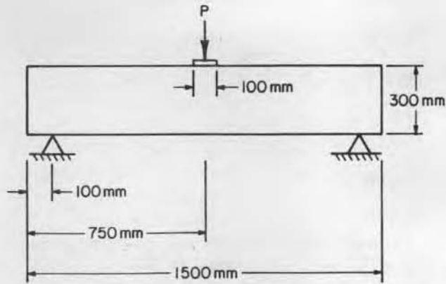
Figure 3. Beam test setup.
