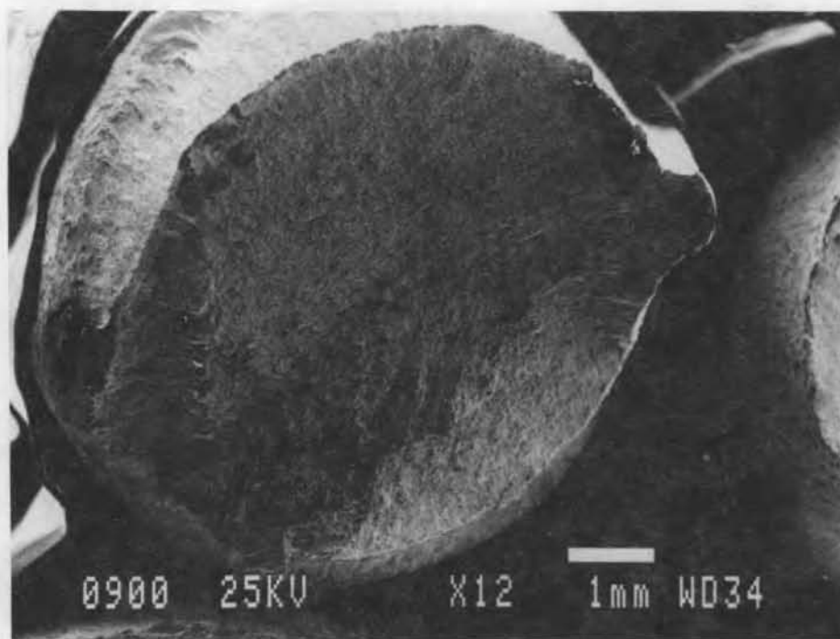
Figure B1. Beam A2 (magnification \times 12 ).
