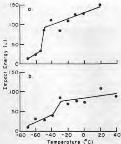
Figure 13. Relationship between failure energy and temperature for the steels in the Charpy-V test. a-cold worked smooth bar, b-hot rolled deformed bar.
