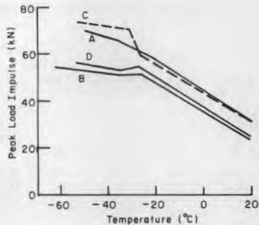
Figure 7. Loads at which reinforced beams first cracked.
