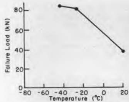
Figure 6. Impact strength of unreinforced beams.
