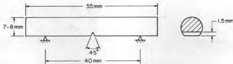
Figure 2. Rebar test specimens.
