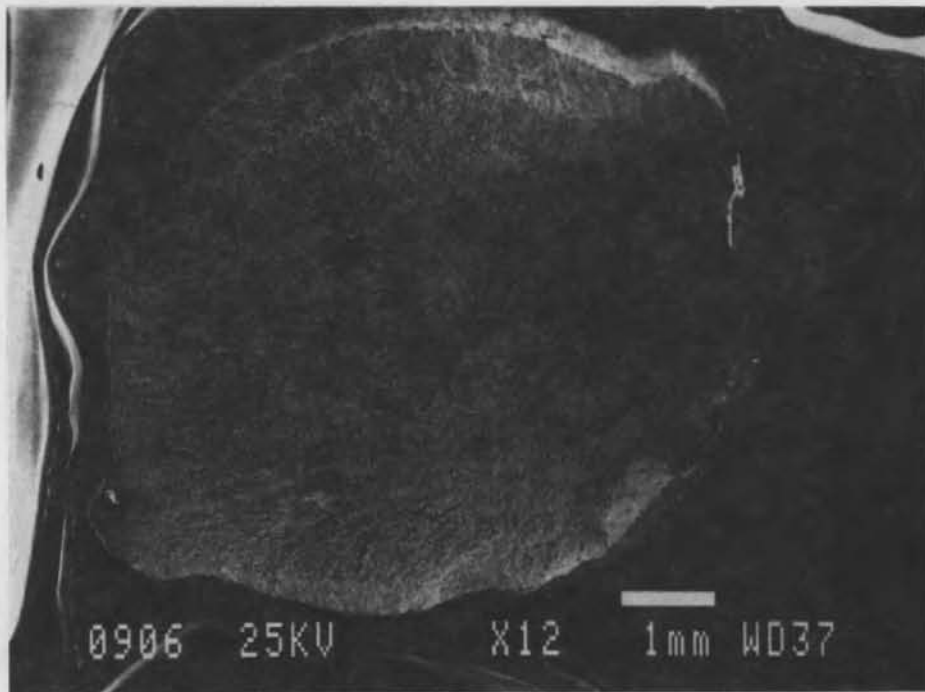
Figure B7. Beam A9 (magnification \times 12 ).
