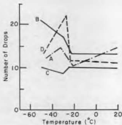
Figure 5. Drops needed to break tension reinforcement (see Table 1 for beam group designations.)
