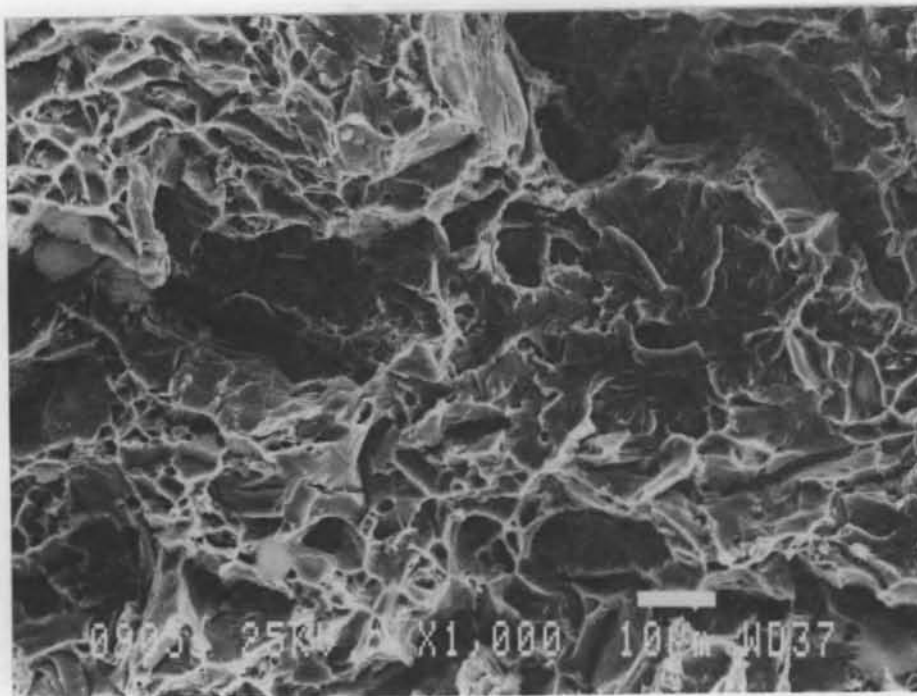
Figure B6. Beam A6, bar 2 (magnification \times 1000 ).
