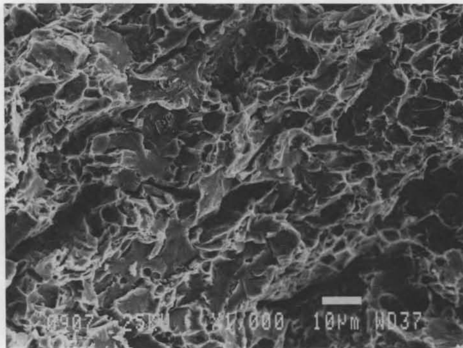
Figure B8. Beam A9 (magnification \times 1000 ).
