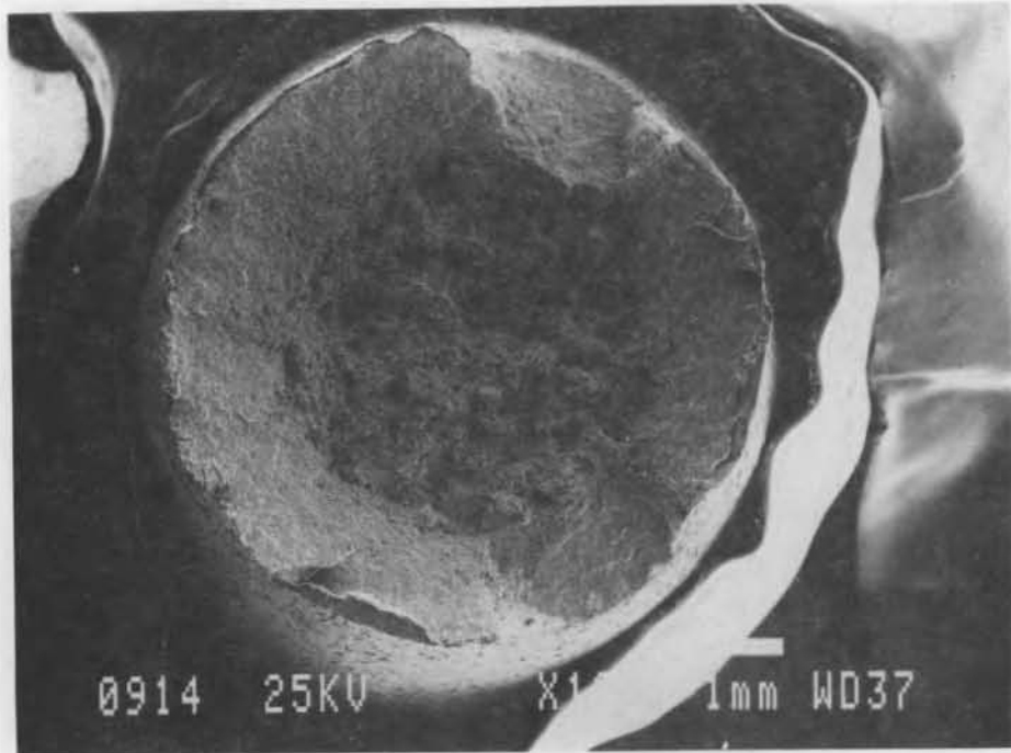
Figure B9. Beam D3 (magnification \times 12 ).
