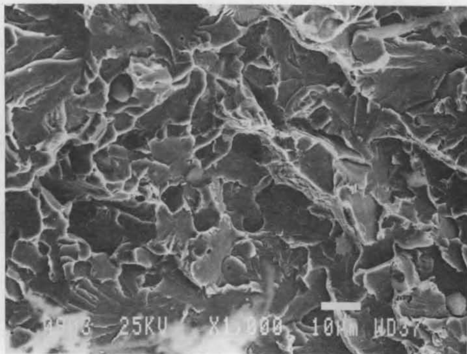
Figure B4. Beam A6, bar 1 (magnification \times 1000 ).
