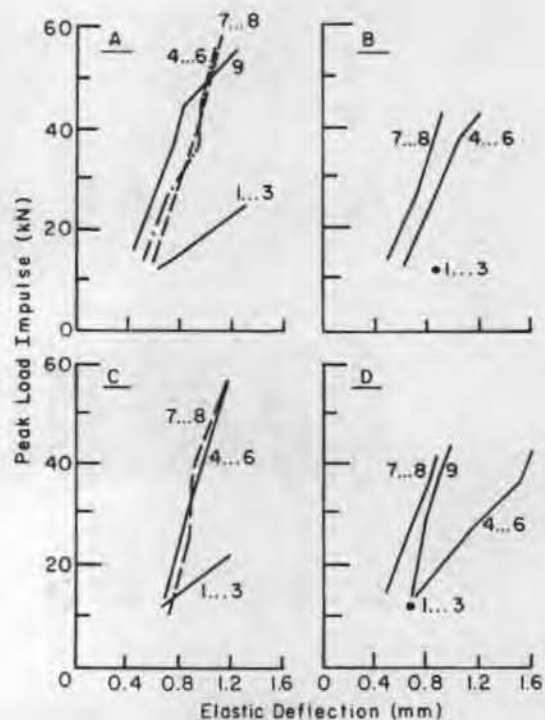
Figure 12. Elastic deflections of reinforced beams prior to cracking of the concrete. See Table 1 to identify reinforcement types for groups A, B, C and D.
