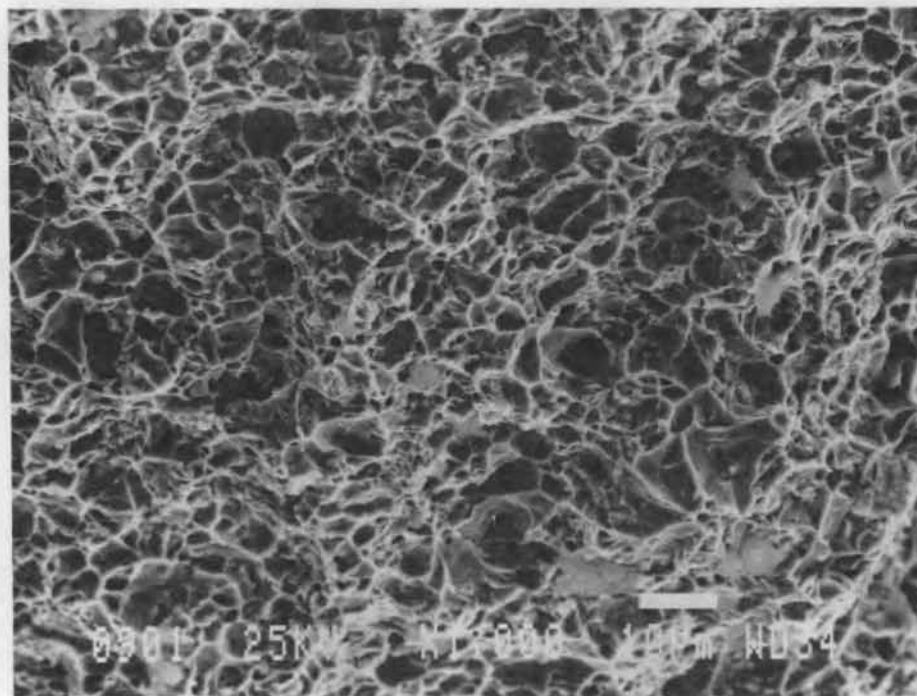
Figure B2. Beam A2 (magnification \times 1000 ).
