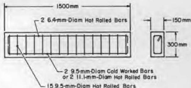
Figure 1. Beam reinforcements. Their yield/tensile strengths are 324/455 Mpa for 6.4- and 9.5-mm-diam hot rolled bars, 449/552 Mpa for 9.5-mm-diam cold worked bars, and 276/414 MPa for 11.1-mm-diam hot rolled bars.
