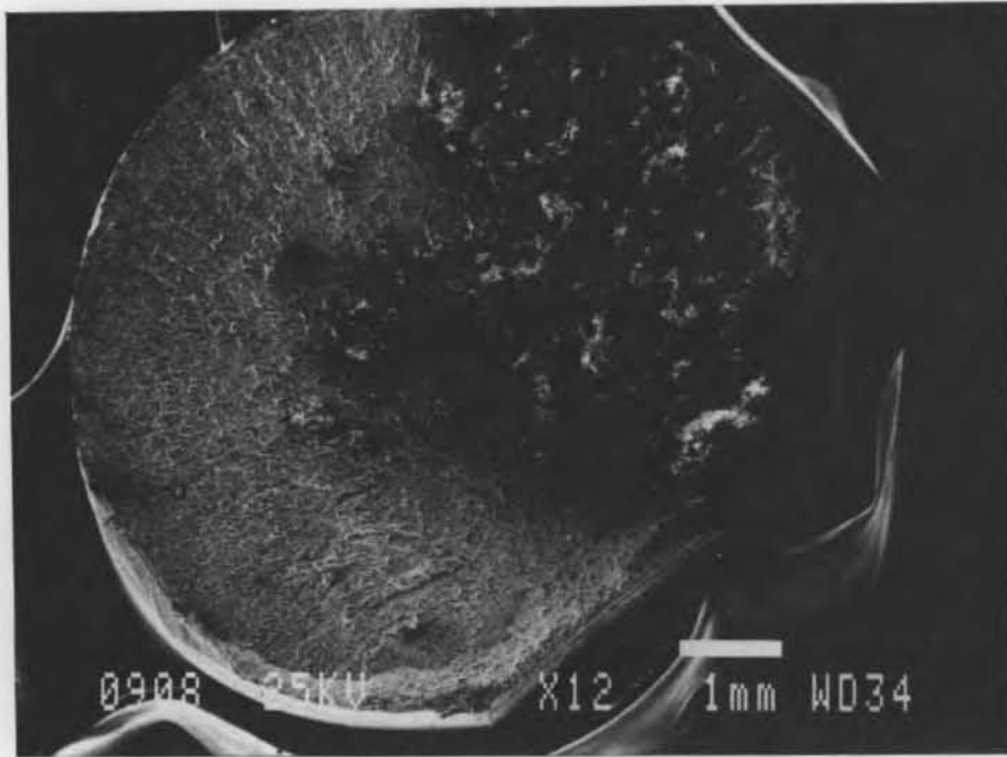
Figure B13. Beam D9, bar 1 (magnification \times 12 ).
