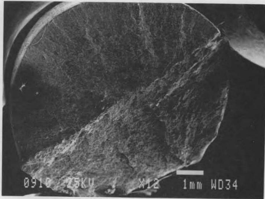
Figure B15. Beam D9, bar 2 (magnification \times 12 ).
