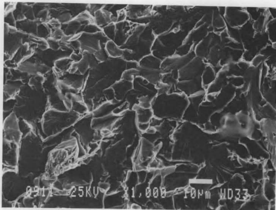
Figure B16. Beam D9, bar 2 (magnification \times 1000 ).
