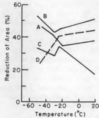
Figure 9. Reduction of area for tension steels upon breaking.
