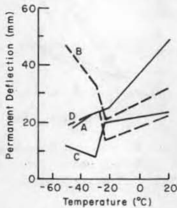
Figure 8. Permanent deflections of reinforced beams prior to breakage of the tension reinforcing steel.
