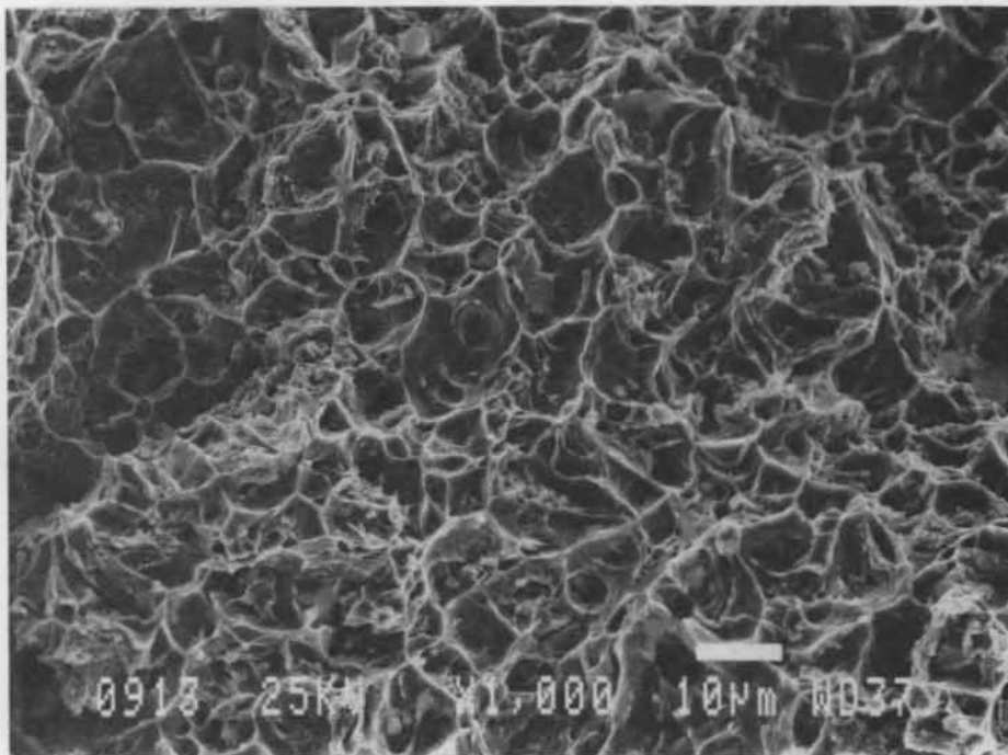
Figure B12. Beam D5 (magnification \times 1000 ).
