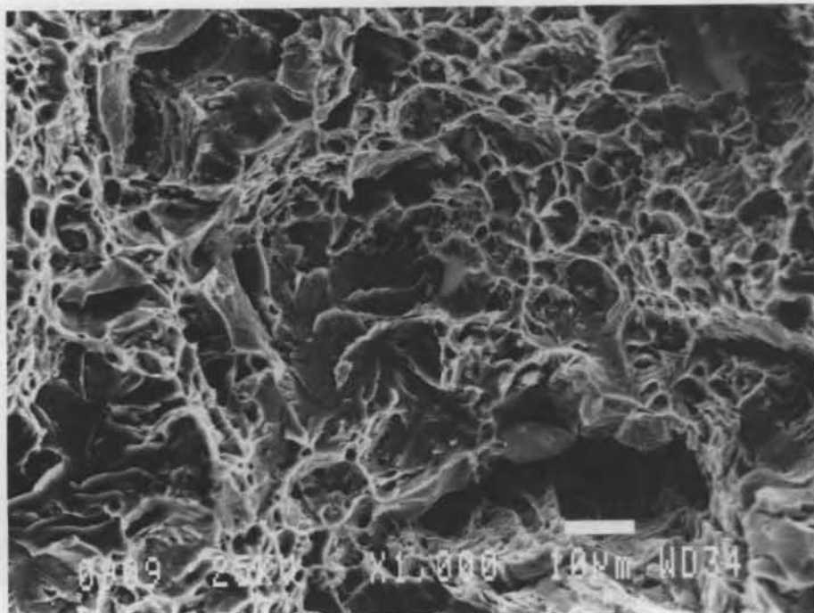
Figure B14. Beam D9, bar 1 (magnification \times 1000 ).
