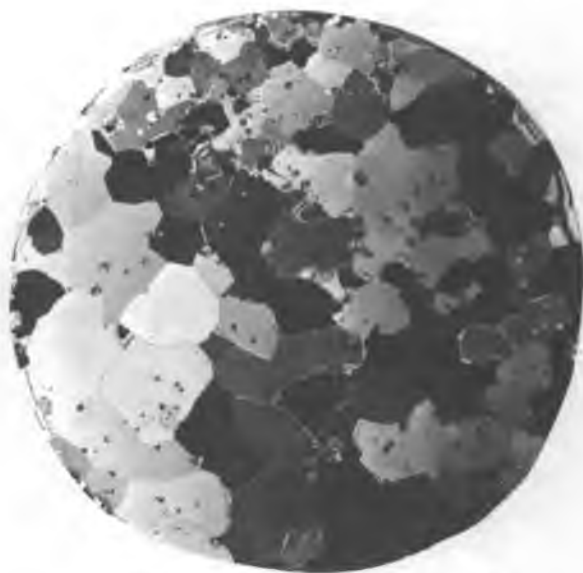
b. Thin section of ice from Ross Island.
