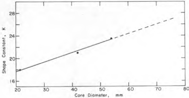
Figure 8. Shape constant vs test sample diameter.
