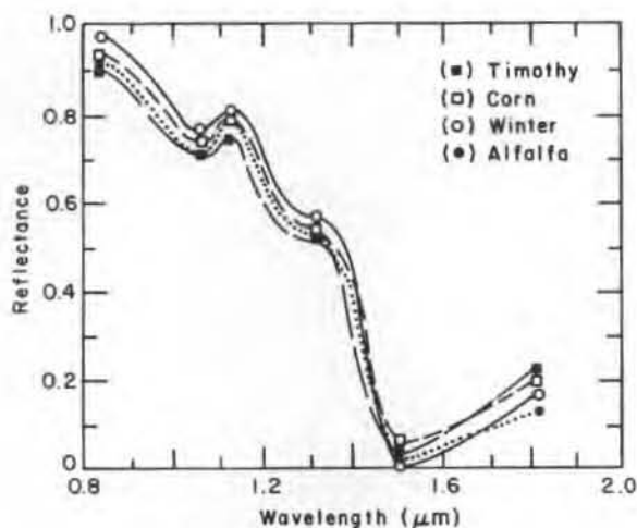
Figure 5. Reflectance of snow-covered crop grasses.
