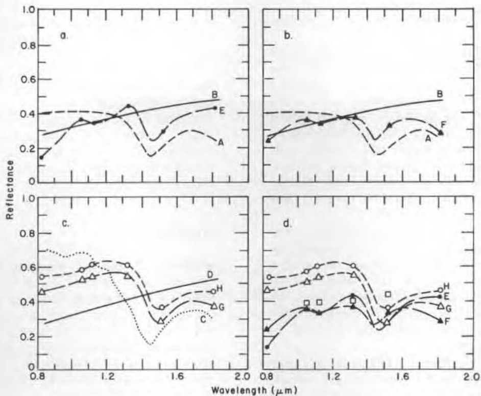
Figure 12. Reflectance from substrates.
