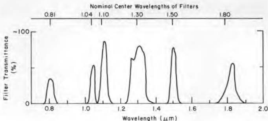
Figure 4. Transmission curves of filters used in measurements.
