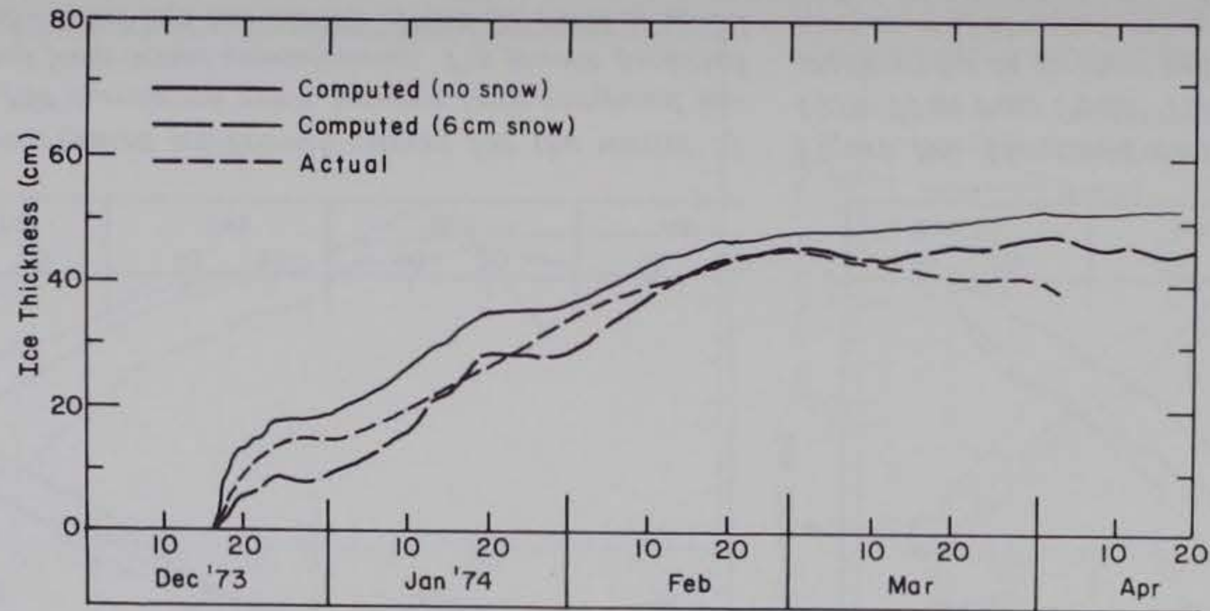
Figure B1. Measured and computed ice-growth curves for the winter of 1973-74 at Post Pond. The departure of the predicted ice growth from that actually measured is substantially decreased when the predicted curve incorporates the effect of a 6-cm snow cover. This result is in essential agreement with the snow distribution for this winter.
