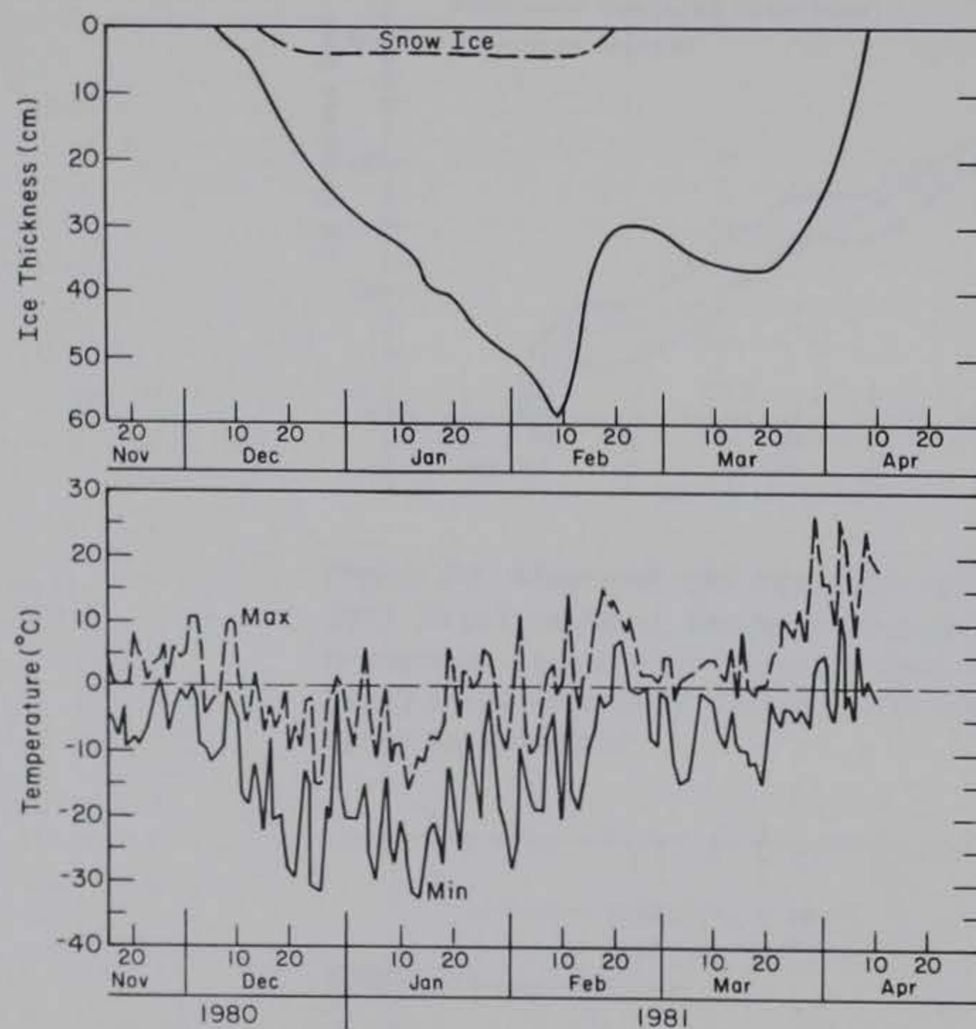
Figure A8. Ice growth on Post Pond and daily maximum and minimum surface air temperatures at CRREL for the winter of 1980-81. Freeze-up occurred on 6 December and was followed by exceptionally rapid ice growth, which averaged nearly 9 mm/day over the next 2 months. A maximum ice thickness of 59 cm, including just 4 cm of snow ice, was measured on 9 February. This was followed by unseasonably warm weather, resulting in the loss of nearly half the ice cover during the next 11 days. This in turn was followed by a renewal of ice growth that continued into the third week of March before the ice again began to melt. Ice-out occurred on 7 April.
