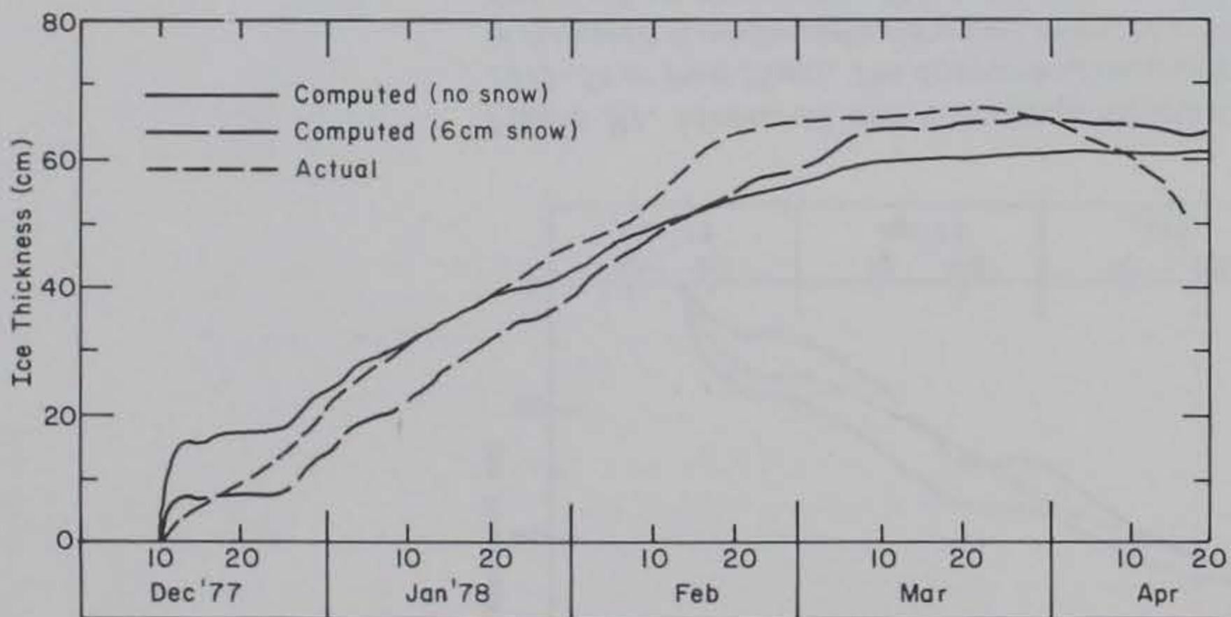
Figure B5. Measured and computed ice-growth curves for the winter of 1977-78 at Post Pond. A fair correlation exists between both computed ice-growth curves and that obtained from actual measurements. The growth predicted on the basis of a 6-cm-thick snow cover lags consistently behind the curve of actual growth, but both match closely in the region of maximum ice thickness.
