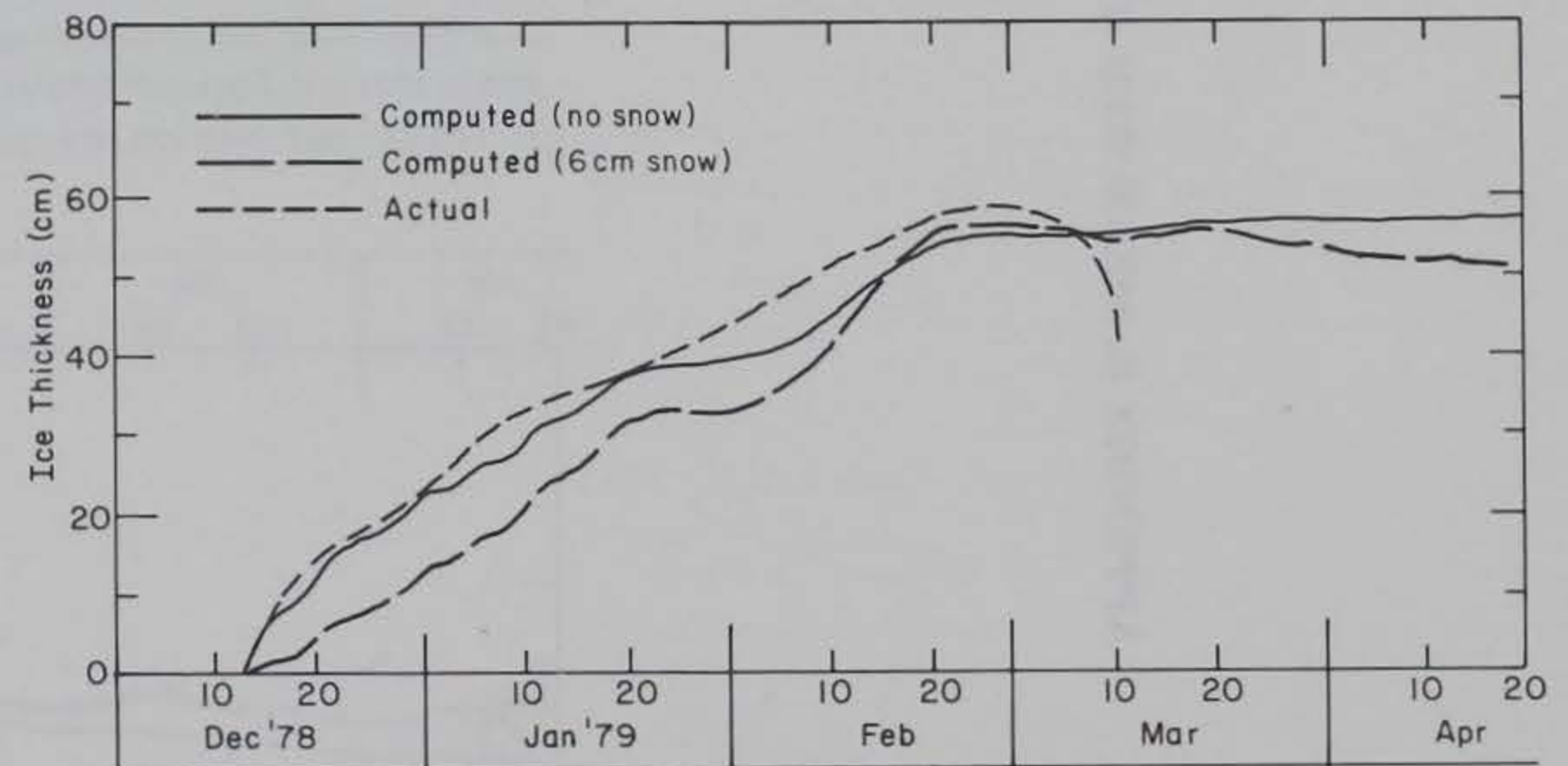
Figure B6. Measured and computed ice-growth curves for the winter of 1978-79 at Post Pond. The measured ice-growth curve agrees closely with growth predicted for an ice sheet lacking a snow cover. This result appears at odds with the formation of abundant snow ice. A possible explanation, borne out by observation, is that the insulating effect of the snow was diminished significantly by its rapid conversion to snow ice.
