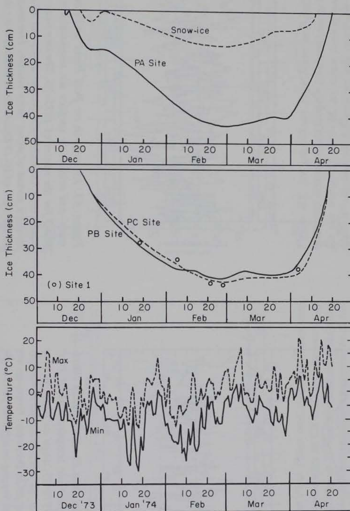
Figure A1. Ice growth on Post Pond and the daily maximum and minimum surface air temperatures at CRREL for the winter of 1973-74. (From Gow and Langston 1977.) (Thickness data from three other sites are included to demonstrate the small variability in ice thicknesses measured at various locations on Post Pond.) Initial freeze-over occurred during the night of 13-14 December. This produced a 4- to 5-cm-thick ice sheet, which melted completely during a warm period on 14 and 15 December. A steep decline in surface air temperatures followed, leading to freeze-up on 17 December. The ice cover attained its maximum thickness (45 cm) during the last week of February 1974. However, the ice sheet, composed of 13 cm of snow ice overlying 32 cm of lake ice, did not undergo any appreciable thinning until the second week of April. By 19 April the ice cover had disappeared completely.
