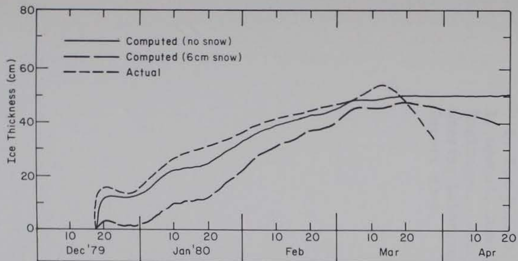
Figure B7. Measured and computed ice-growth curves for the winter of 1979-80 at Post Pond. This was the year of the "snowless" winter. Accordingly ice growth predicted on the basis of no snow cover agrees very closely with actual measurements of ice thickness.
