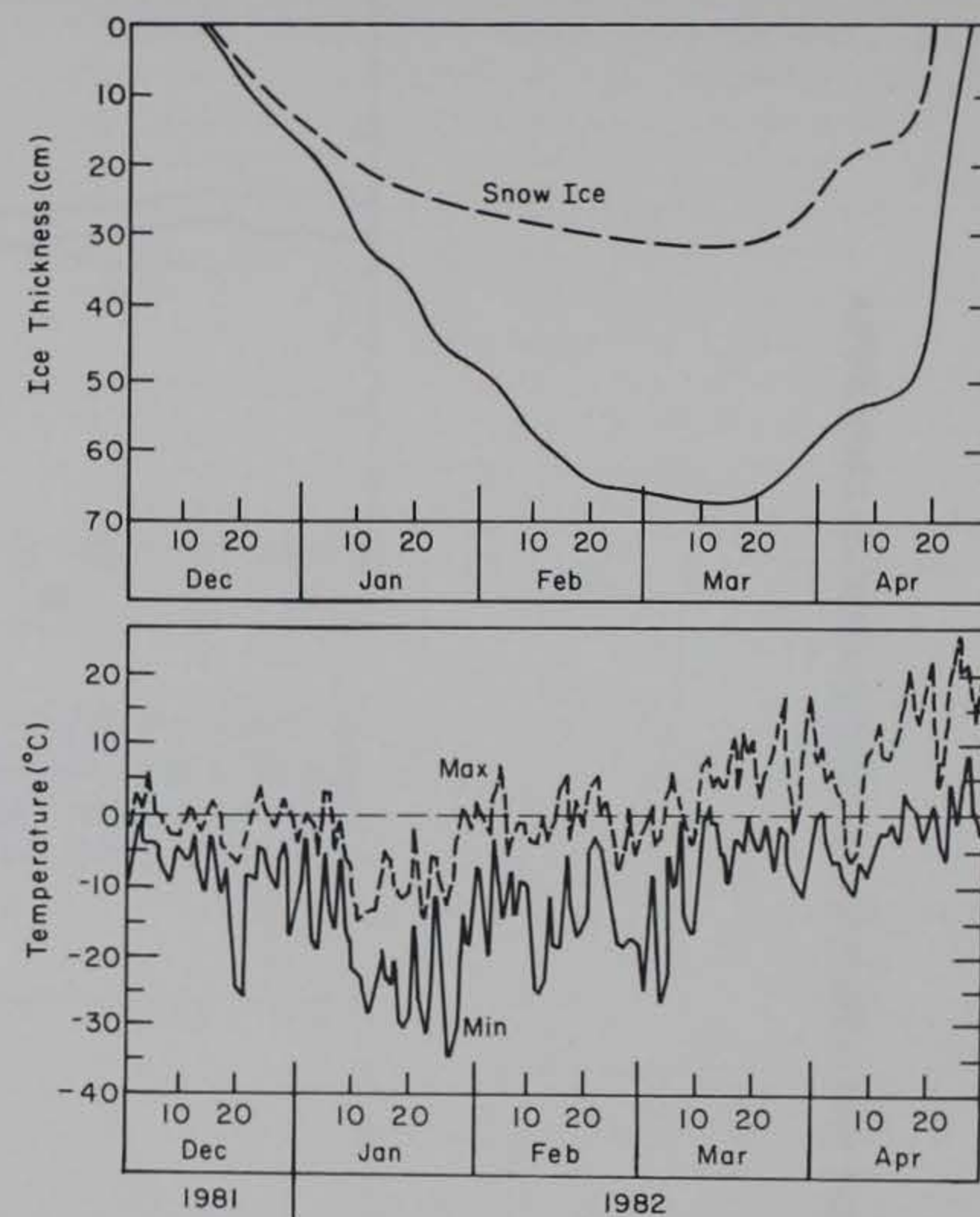
Figure A9. Ice growth on Post Pond and daily maximum and minimum surface air temperatures at CRREL for the winter of 1981-82. Freeze-up on 14 December coincided with sustained snowfall, leading to the formation of an ice sheet composed principally of snow ice in the top 20 cm. The ice sheet grew at a rate of about 9.5 mm/day until it reached a thickness of 65 cm by 20 February. A maximum ice thickness of 67 cm, including 31 cm of snow ice, was recorded on 15 March. The lake became ice-free on 27 April. Most of this loss was sustained during the two-week period beginning 14 April, when 52 cm of ice was melted, equivalent to a thinning rate of 37 mm/day.
