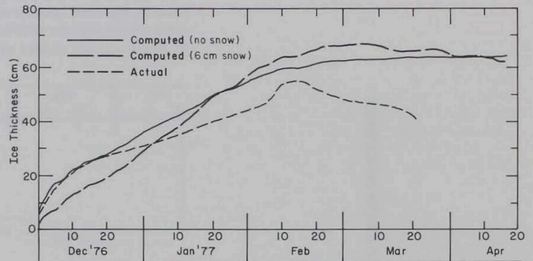
Figure B4. Measured and computed ice-growth curves for the winter of 1976-77 at Post Pond. Correlations between the computed and measured ice-growth curves were difficult because of the activities of ice fishermen during January and February. However, growth of the top 25 cm of ice, which formed before the fishermen arrived, conforms well with values predicted for the no-snow condition, a situation in accord with the lack of a snow cover during December 1976.
