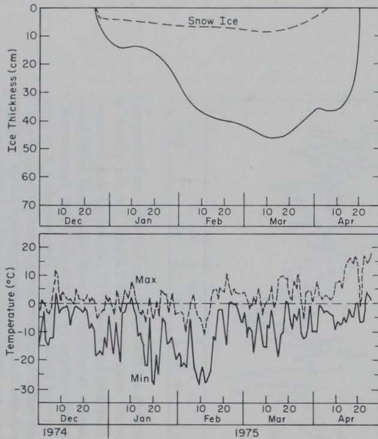
Figure A2. Ice growth on Post Pond and daily maximum and minimum surface air temperatures at Post Pond for the winter of 1974-75. Skim ice began forming towards the end of November, but the lake did not completely freeze up until the evening of 25-26 December. Freeze-up was characterized by independent freezing on different parts of the lake until it became entirely ice-covered. Maximum ice thickness (47 cm) occurred during the second week of March. The ice cover, consisting of 9 cm of snow ice and 38 cm of lake ice, began thinning two or three days later and had melted completely within one month (20 April).
