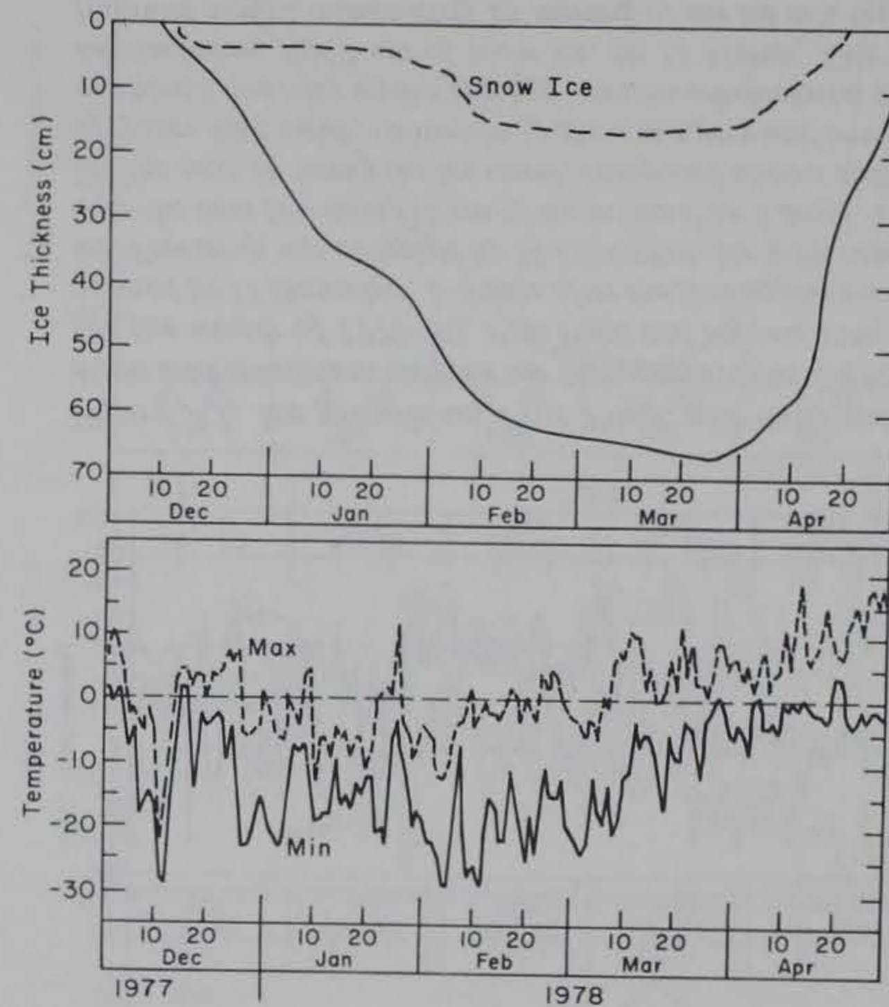
Figure A5. Ice growth on Post Pond and daily maximum and minimum surface air temperatures at CRREL for the winter of 1977-78. Ice began forming around the edges of the lake on 8 December and continued to grow towards the center of Post Pond until complete freeze-up occurred on 10 December. A maximum ice thickness of 67 cm, including 17 cm of snow ice, was recorded on 24 March 1978 and was followed by sustained melting, leading to complete dissipation by 29 April.
