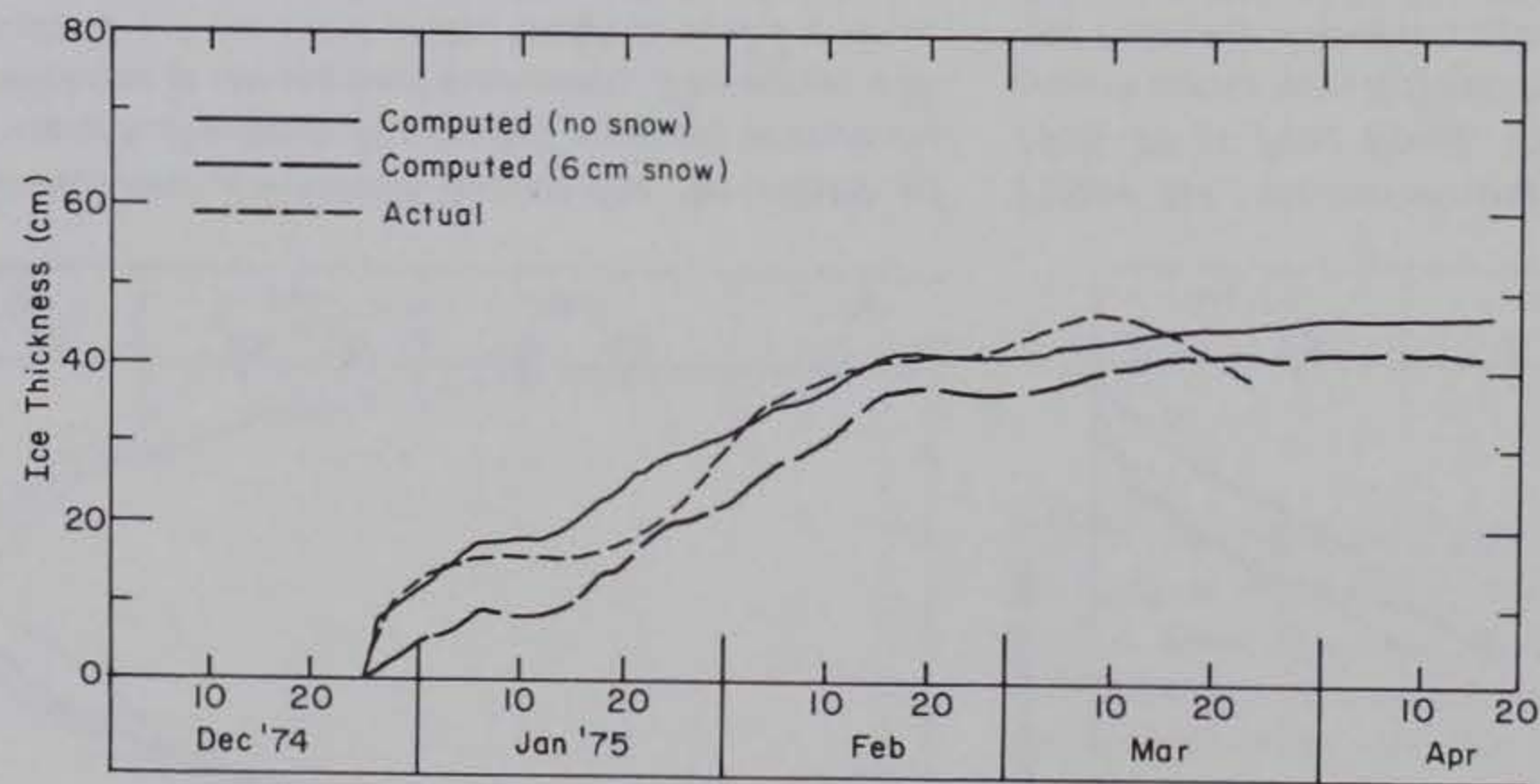
Figure B2. Measured and computed ice-growth curves for the winter of 1974-75 at Post Pond. This winter was characterized by less-than-normal snow-fall, reflected by the small amount of snow ice and the generally snow-free ice cover. The good correspondence between actual ice growth and that predicted for snow-free ice supports these observations.
