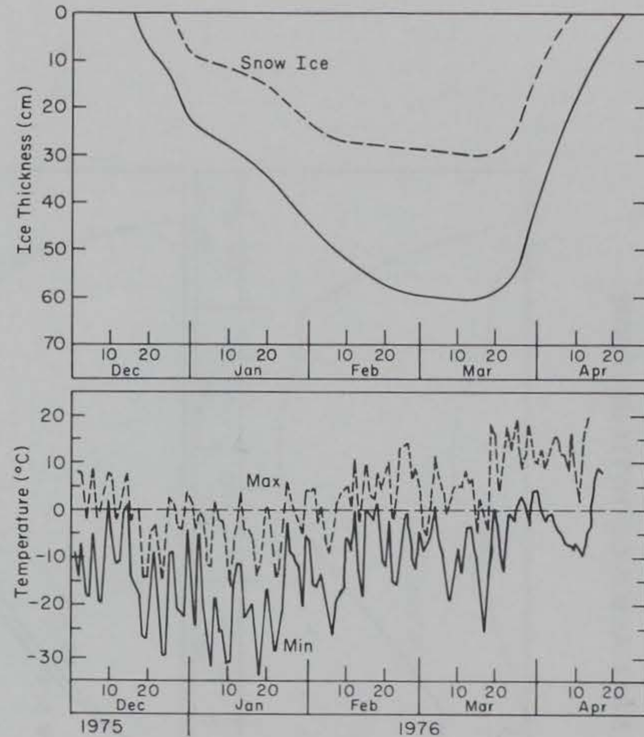
Figure A3. Ice growth on Post Pond and daily maximum and minimum surface air temperatures at Post Pond for the winter of 1975-76. The lake froze over completely on 8 December but became ice-free by 12 December during a period of warm, rainy weather. Freeze-up occurred on the night of 16-17 December. A maximum ice thickness of 60 cm, including an unusually thick, 30-cm layer of snow-ice was measured on 16 March and was followed almost immediately by thinning of the ice cover by surface melting. All ice had disappeared by 20 April.
