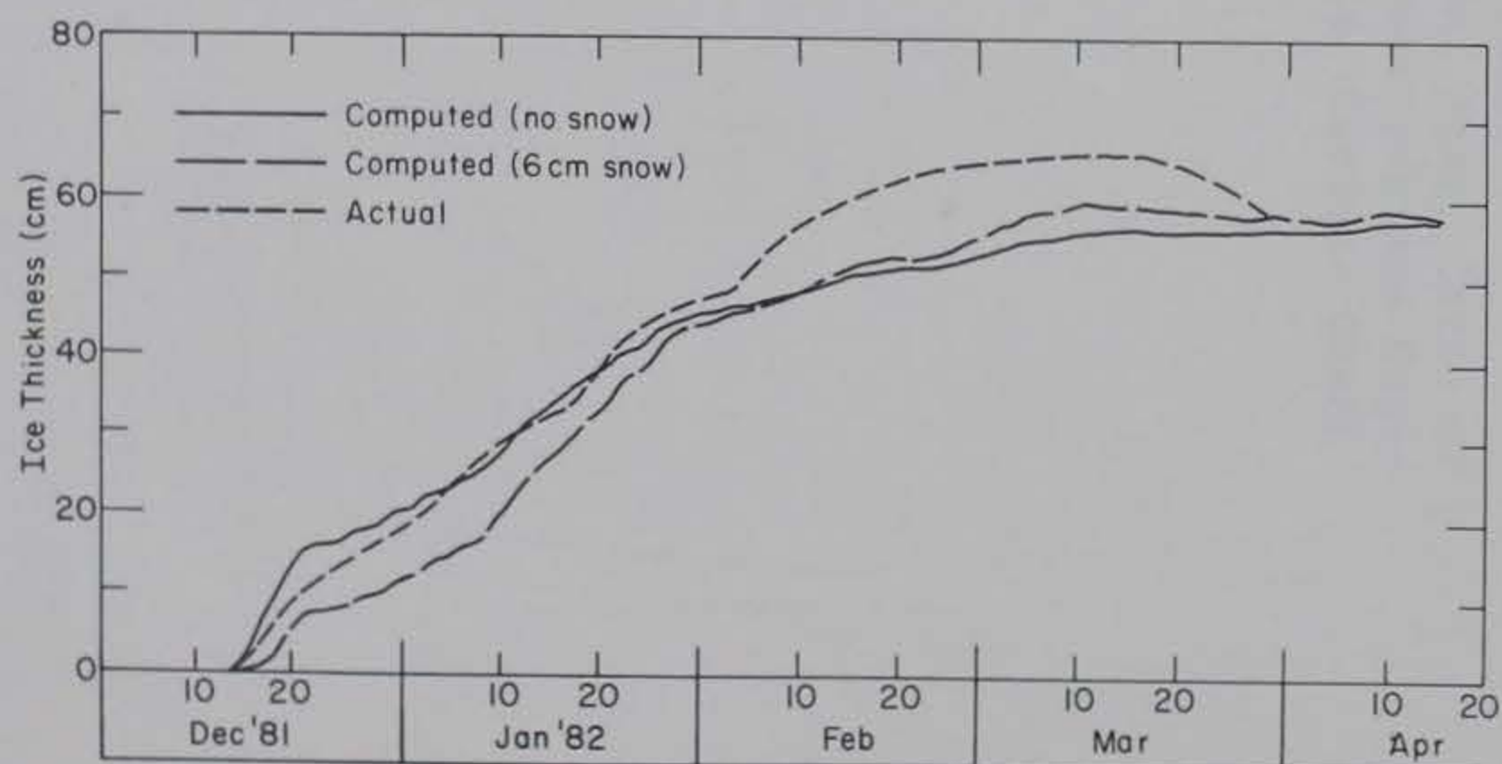
Figure B9. Measured and computed ice-growth curves for the winter of 1981-82 at Post Pond. This was a season in which substantial snowfall was recorded. Snow deposited concurrently with freeze-up led to an ice cover composed predominantly of snow ice in the top 20-25 cm. Interestingly the measured growth corresponds closer with that computed on the basis of the snow-free model than that incorporating a 6-cm snow cover. This result is probably because most of the snow was transformed to snow ice soon after it was deposited, significantly reducing its insulating effects.
