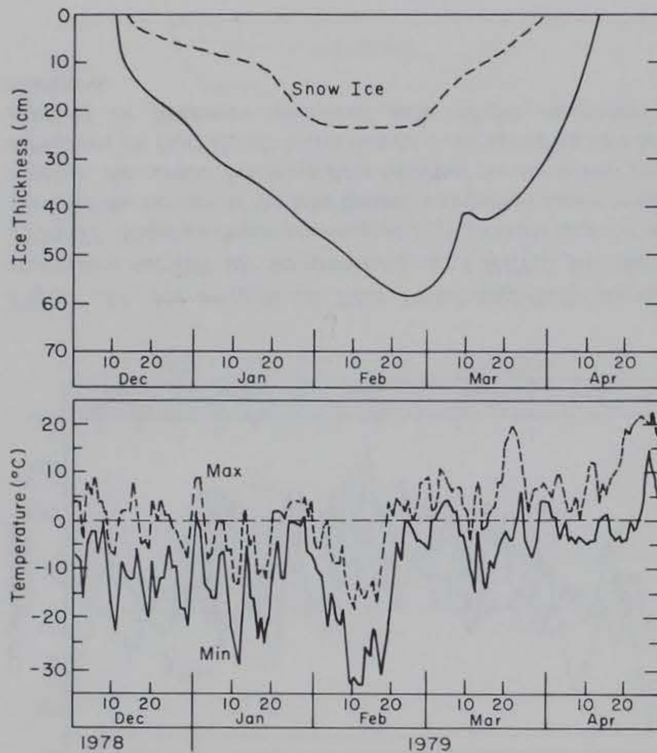
Figure A6. Ice growth on Post Pond and daily maximum and minimum surface air temperatures at CRREL for the winter of 1978-79. During the first week of December the ice grew outwards from the shore and attained a thickness of nearly 11 cm before the center of Post Pond finally froze over on 13 December. The ice cover continued to grow uniformly with time until 24 February, when it reached its maximum thickness for the season (58 cm, including 23 cm of snow ice). The lake became ice-free on 13 April.
