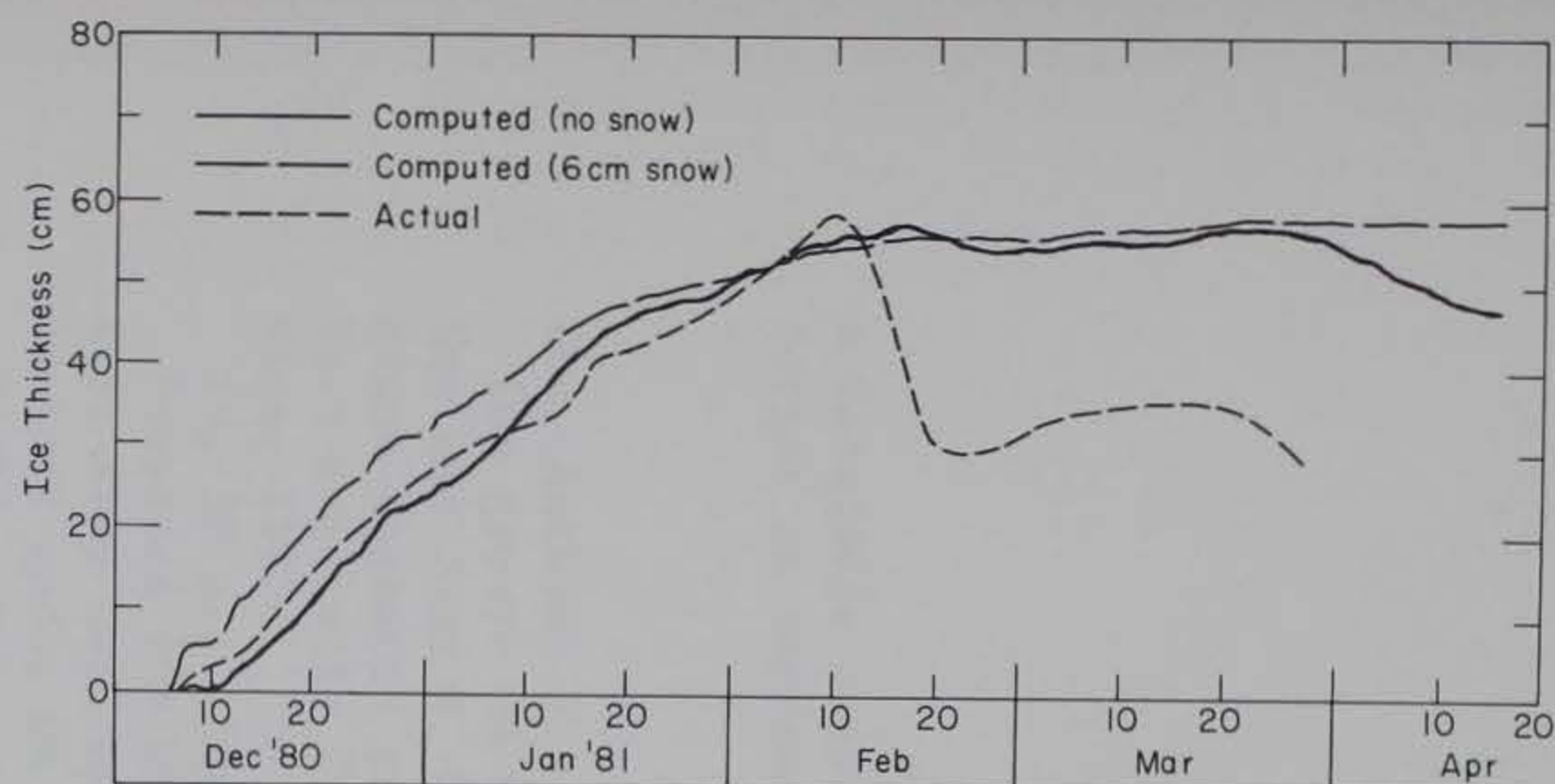
Figure B8. Measured and computed ice-growth curves for the winter of 1980-81 at Post Pond. The low snowfall of this winter is reflected in the good agreement between the measured ice growth and that predicted on the basis of no snow.
