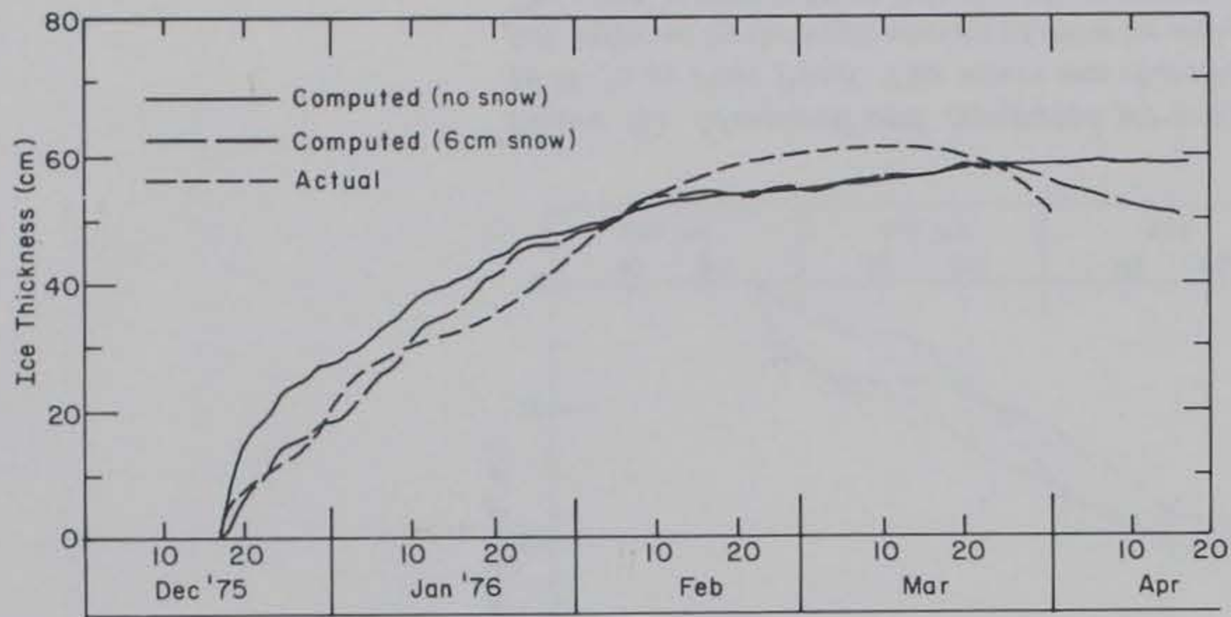
Figure B3. Measured and computed ice-growth curves for the winter of 1975-76 at Post Pond. This winter had substantial snowfall, resulting in extensive snow ice (50% of the total ice thickness at the seasonal maximum). This agrees with ice growth predicted on the basis of a 6-cm snow cover, which provides a closer match with the measured growth than the predicted curve that neglects the effect of snow.
