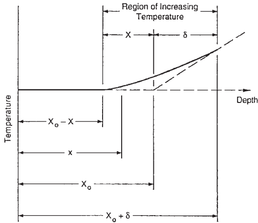
Figure 11. Bottom thaw of permafrost.
