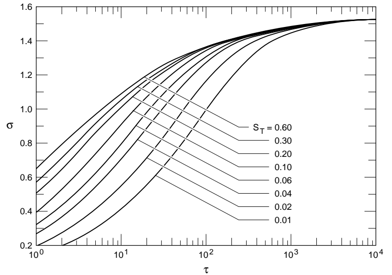
Figure 17. Formation time of permafrost, saturated mineral soils, \phi = 0 , \varepsilon = 0.3 .
