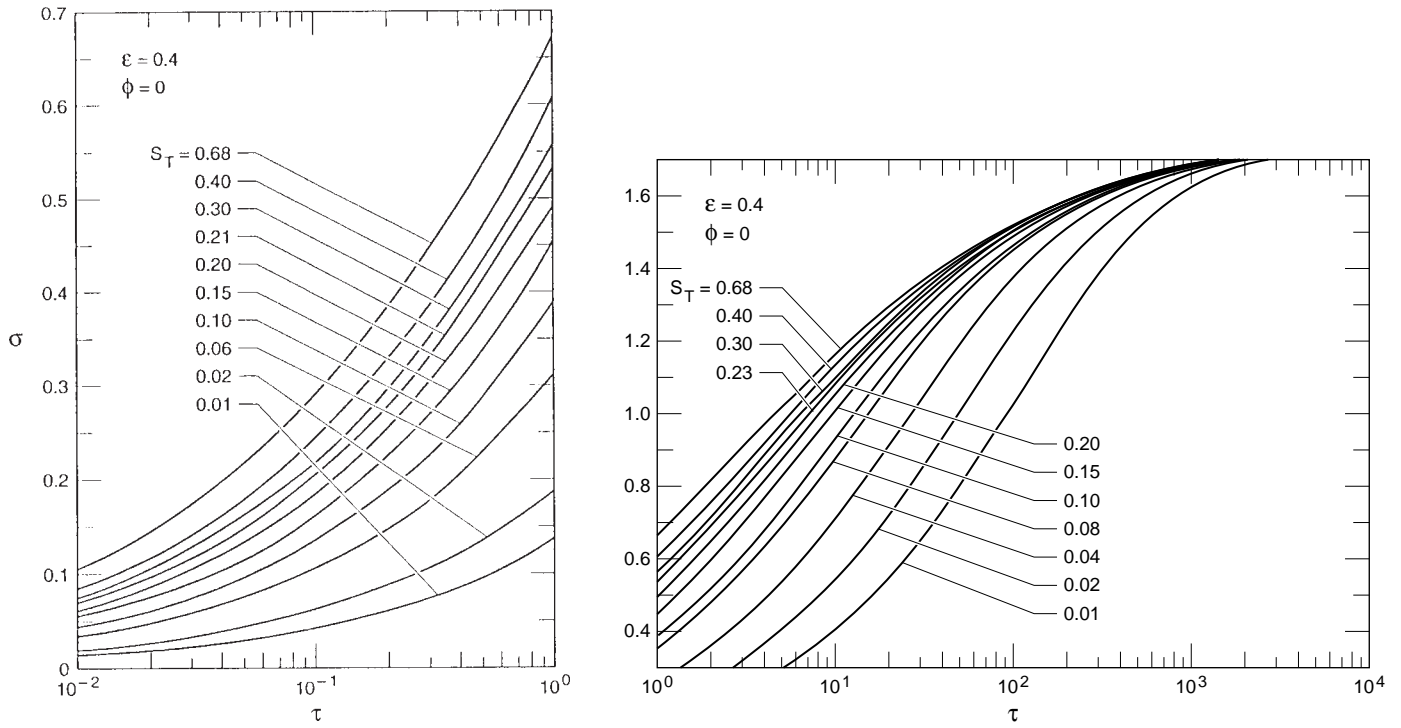
Figure 15. Formation time of permafrost, saturated mineral soils, \phi = 0 , \epsilon = 0.4 .
