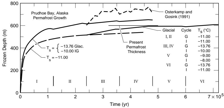
Figure 22. Growth of permafrost at Prudhoe Bay, Alaska; effect of paleotemperature scenarios.
