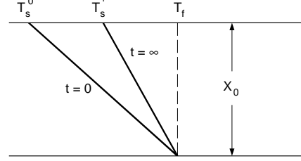
Figure D2. Permafrost equilibrium temperature profiles.
