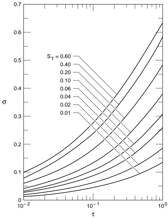
Figure 17. Formation time of permafrost, saturated mineral soils, \phi = 0 , \varepsilon = 0.3 .
