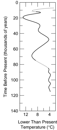
Figure 6. Reconstructed temperature for northern China during last ice age (after Sun and Li 1988).
