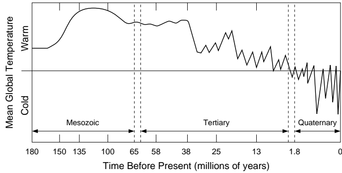
Figure 1. Paleotemperature variations (after Eddy and Bradley 1991).
