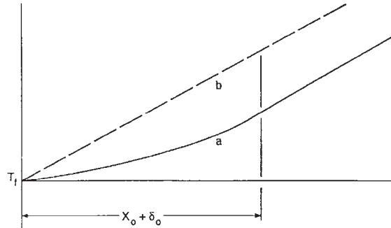
Figure 12. Thermal state at end of melting (a) and long-term equilibrium (b).
