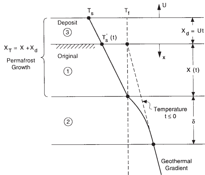
Figure 13. Geometry and coordinate system for freeze of a semi-infinite medium with moving upper surface.
