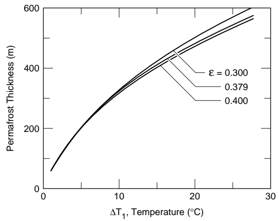
Figure 19. Effect of soil porosity on permafrost thickness after 15,000 years, saturated mineral soils, G = 0.0286^\circ\text{C}/\text{m} .
