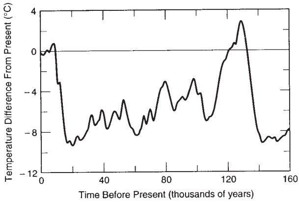
Figure 3. Vostok (Antarctica) ice core temperature inferences (after Jouzel et al. 1987)
