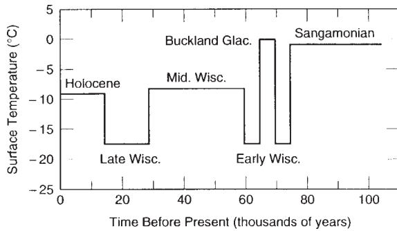
Figure 8. Paleotemperature history at Mackenzie Delta, Canada (after Allen et al. 1988).
