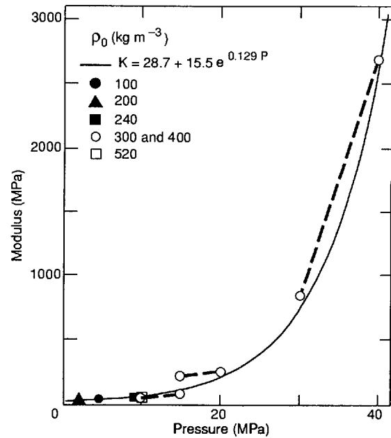
Figure 13. Release modulus for snow ( K is the initial modulus and P is the pressure at the initial release).
