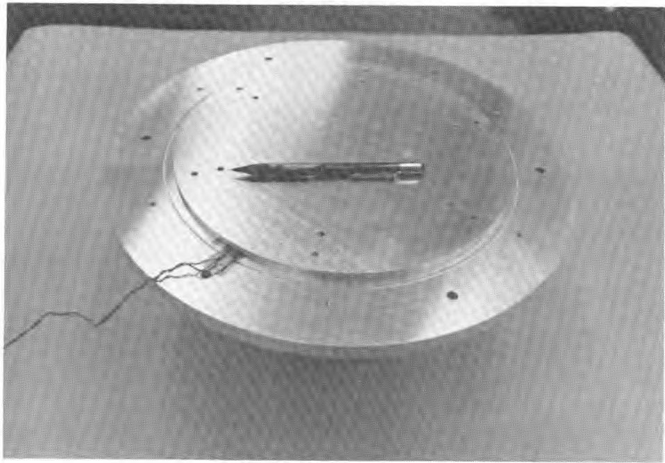
a. Front end-plate (12.7 mm thick) with epoxyed stress gauge and 6.35-mm-thick backing plate on top.
