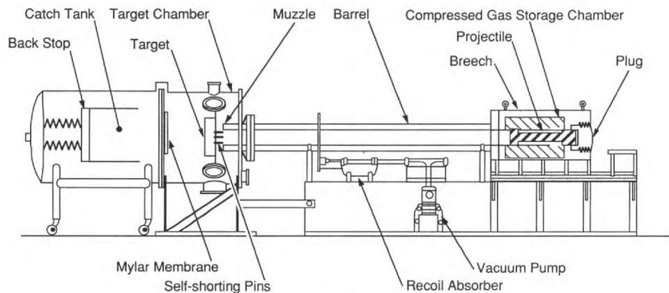
Figure 1. Gas gun assembly.
