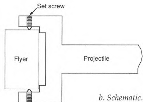
Figure 2. Projectile with mounted aluminum flyer plate.
