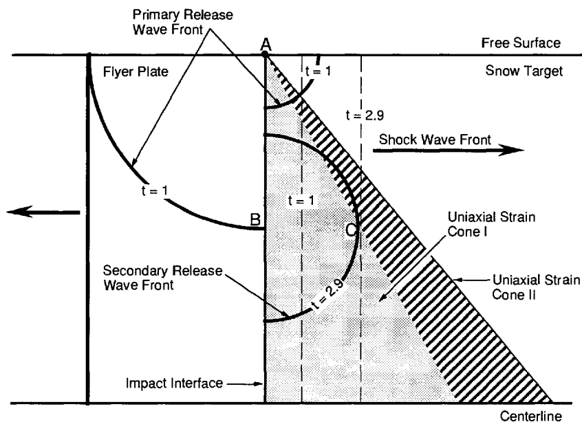
Figure 4. Uniaxial strain impact cones for a flyer and target.
