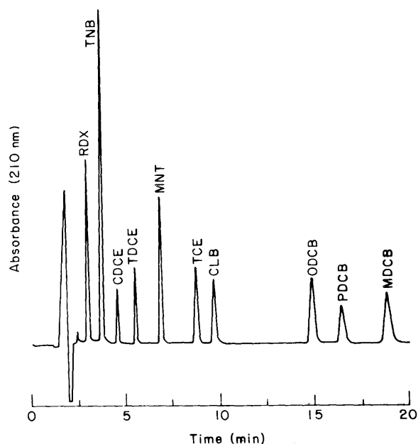
Figure 1. Chromatogram for 10 analytes.
