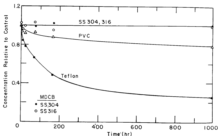
Figure 2. Sorption of MDCB by the four well casing materials.
