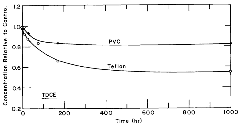
Figure 4. Sorption of TDCE by plastic casings.
