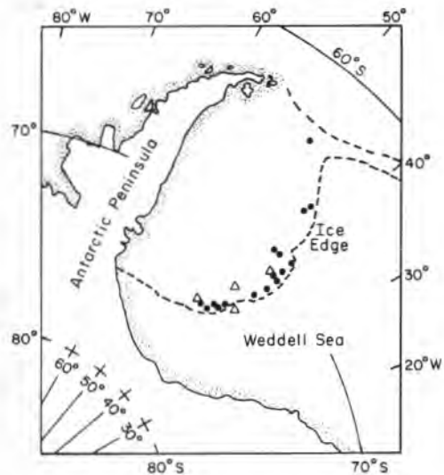
Figure 4. Locations of the primary sea ice sampling sites (circles). Data buoys used for satellite monitoring of drift and deformation of the pack ice in the Weddell Sea are indicated by triangles.
