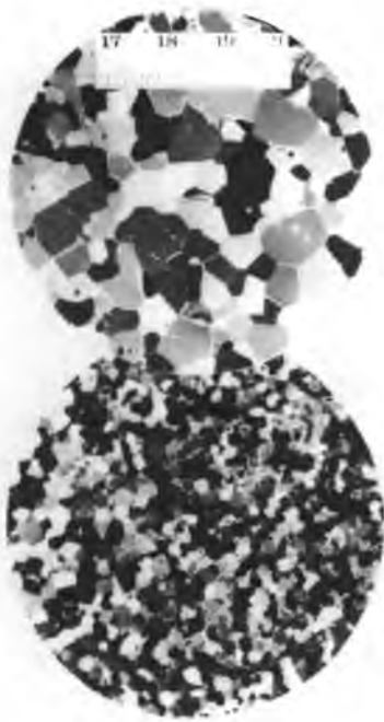
Figure 3. Examples of variable nature of grain size and texture in snow ice in Weddell Sea pack ice.
