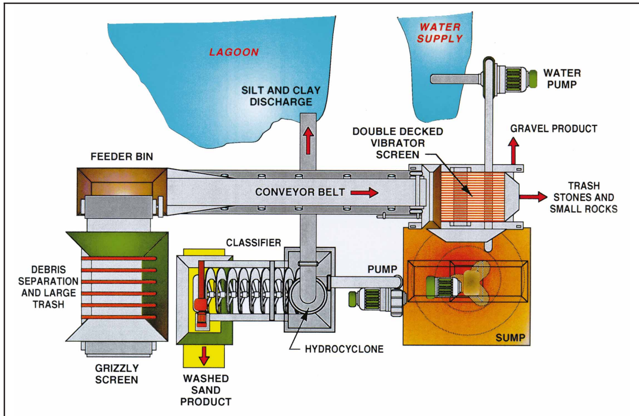
Figure 3. Proposed dredged material processing plan and equipment layout for recovering gravel and sand from the Duluth, MN, CDF
