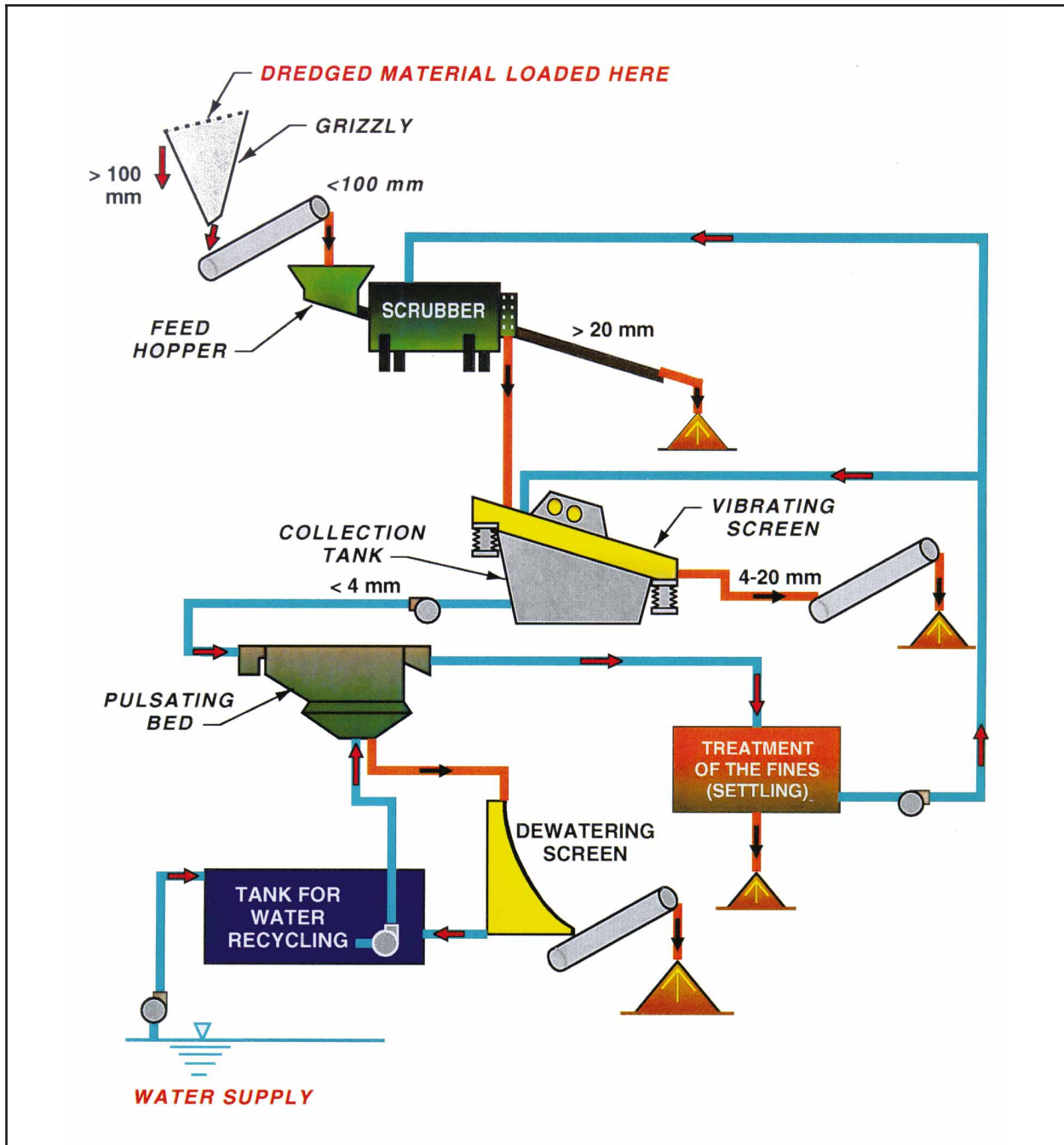
Figure 4. Dredged material processing plan and equipment layout for separating debris and trash from dredged material (adapted from de Kreuk, de Kreuk, and van Muijen 1998)
