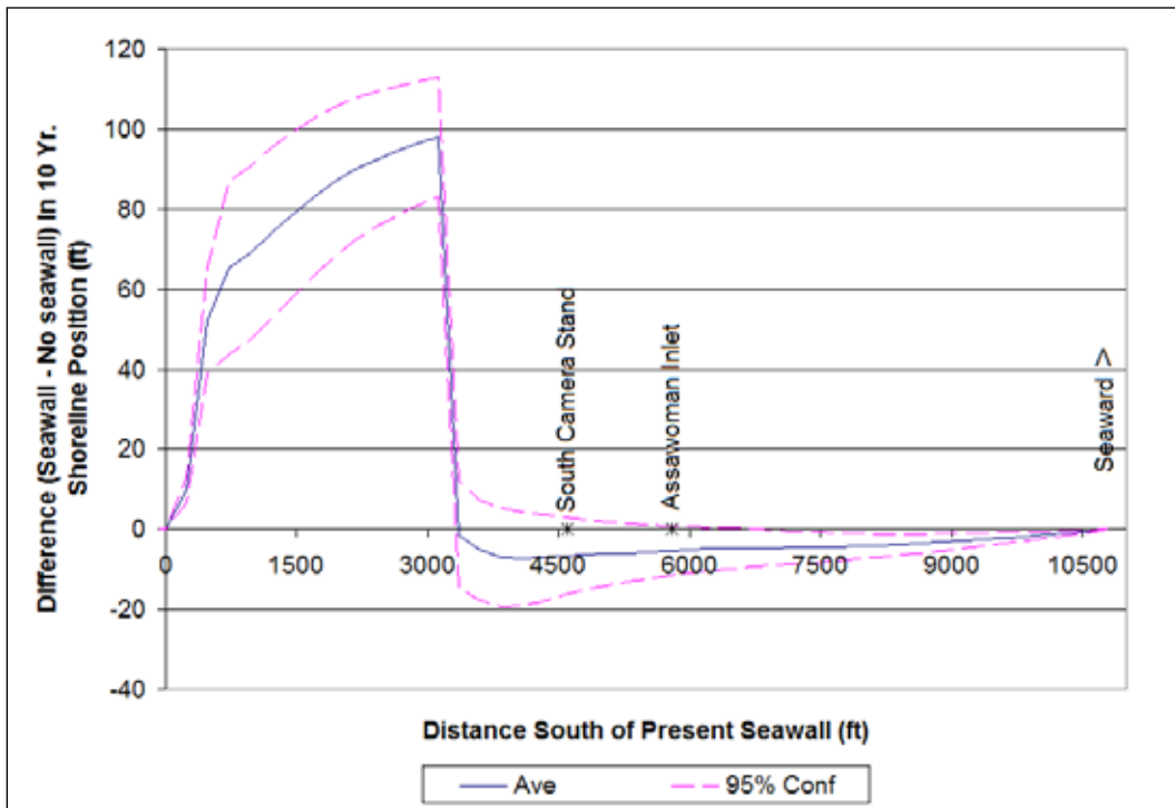
Figure F-9. Ten year shoreline difference between 3000 ft seawall extension at the shoreline and no seawall extension.
