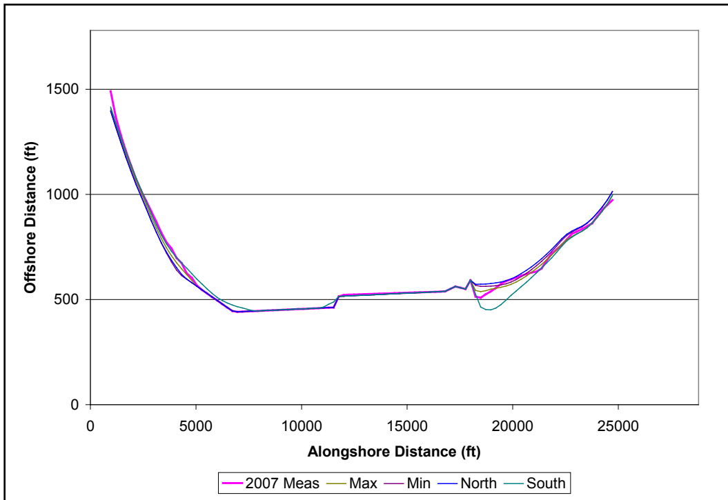
Figure 5-12. Comparison of the 2007 measured shoreline with GENESIS shorelines driven with the Max, Min, North, and South wave blocks.
