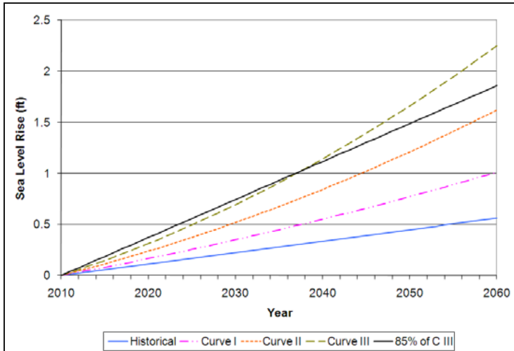
Figure 6-6. Projected Wallops Island, VA SLR, as based upon NRC (1987) curves.
