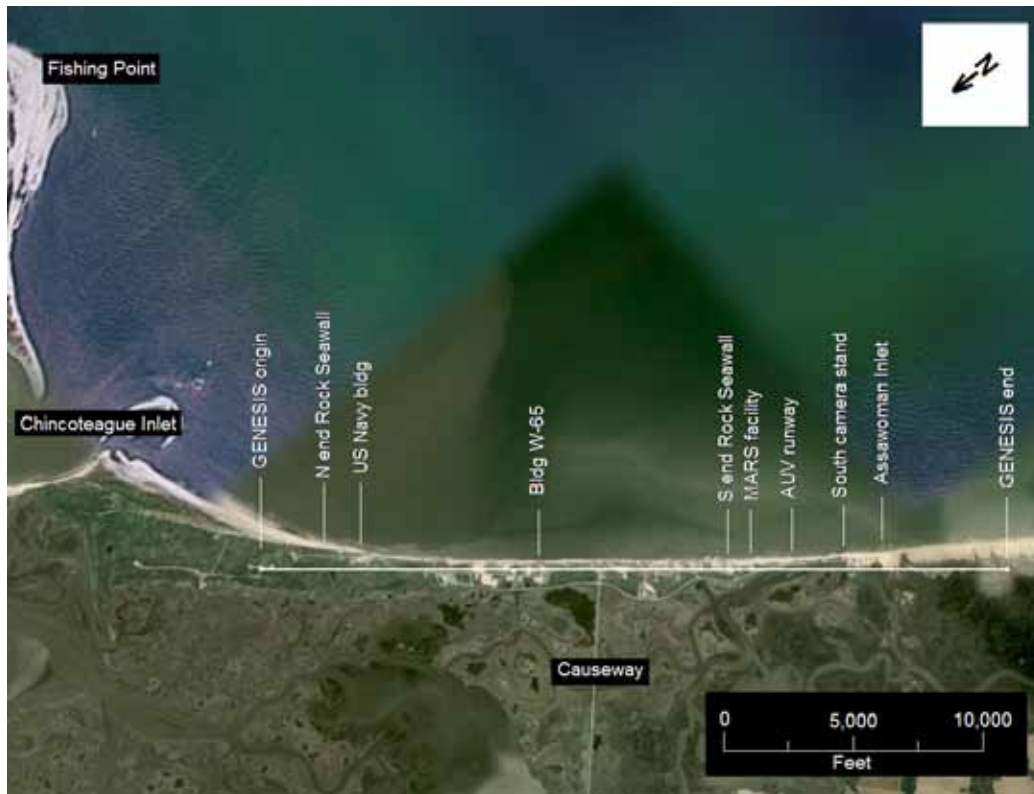
Figure 5-5. Layout of GENESIS grid.
