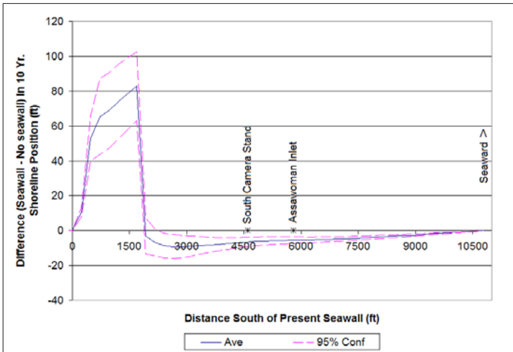
Figure F-7. Ten year shoreline difference between 1500 ft seawall extension at the shoreline and no seawall extension.
