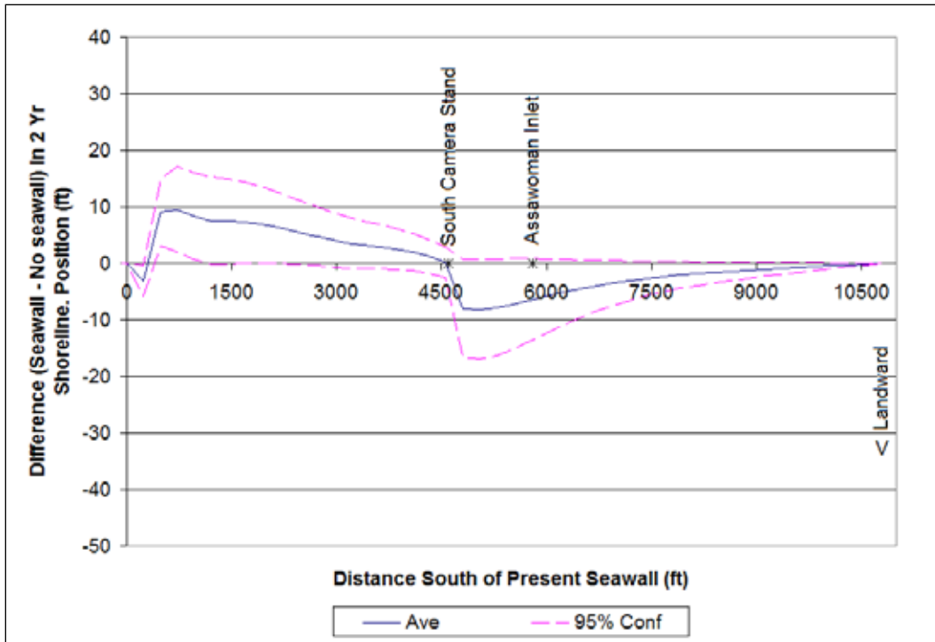
Figure F-6. Two year shoreline difference between 4600 ft seawall extension 10 yds landward and no seawall extension.
