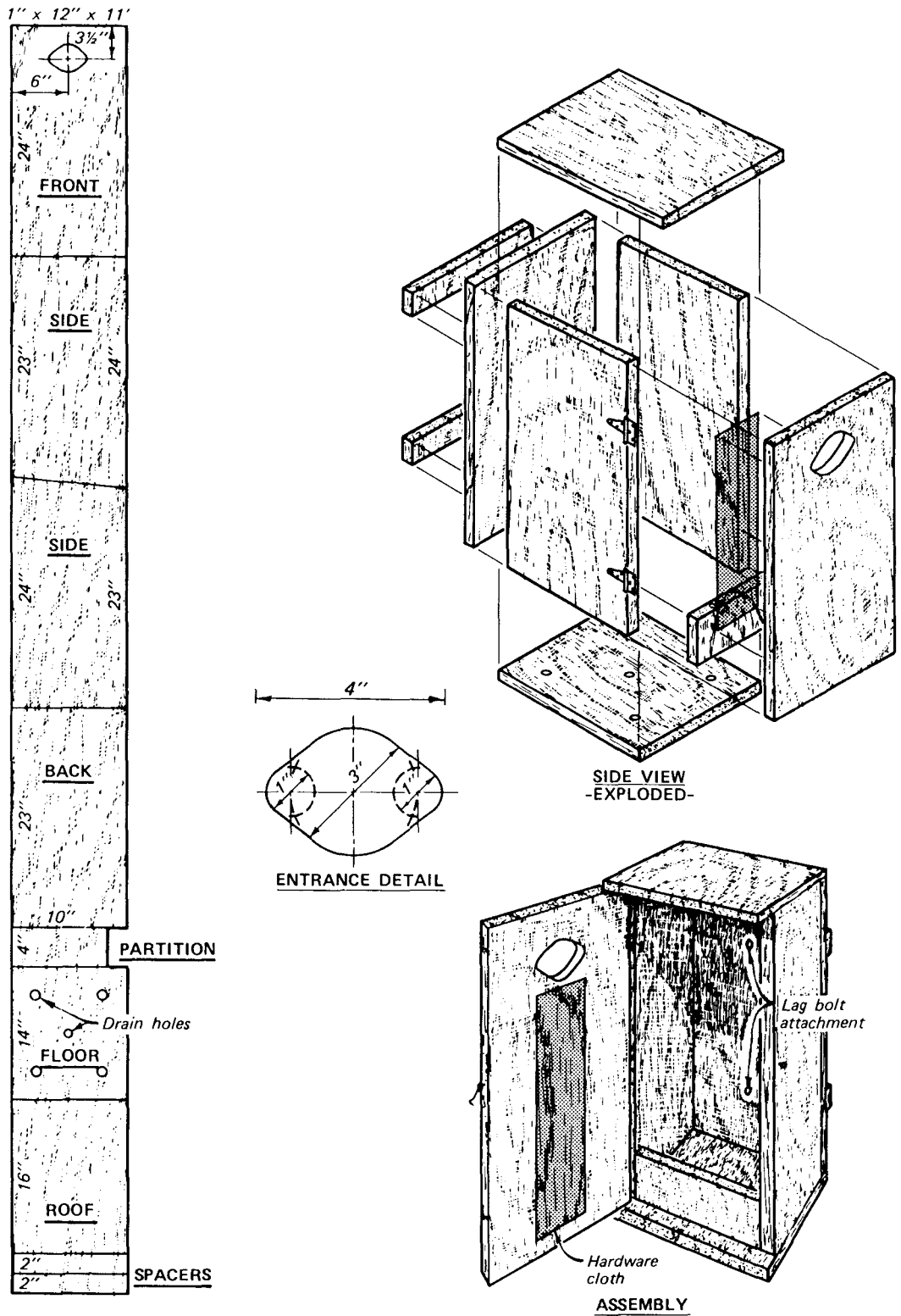
Figure 1. Construction details for a front-opening wooden nest box (entrance detail from Bellrose 1980)
