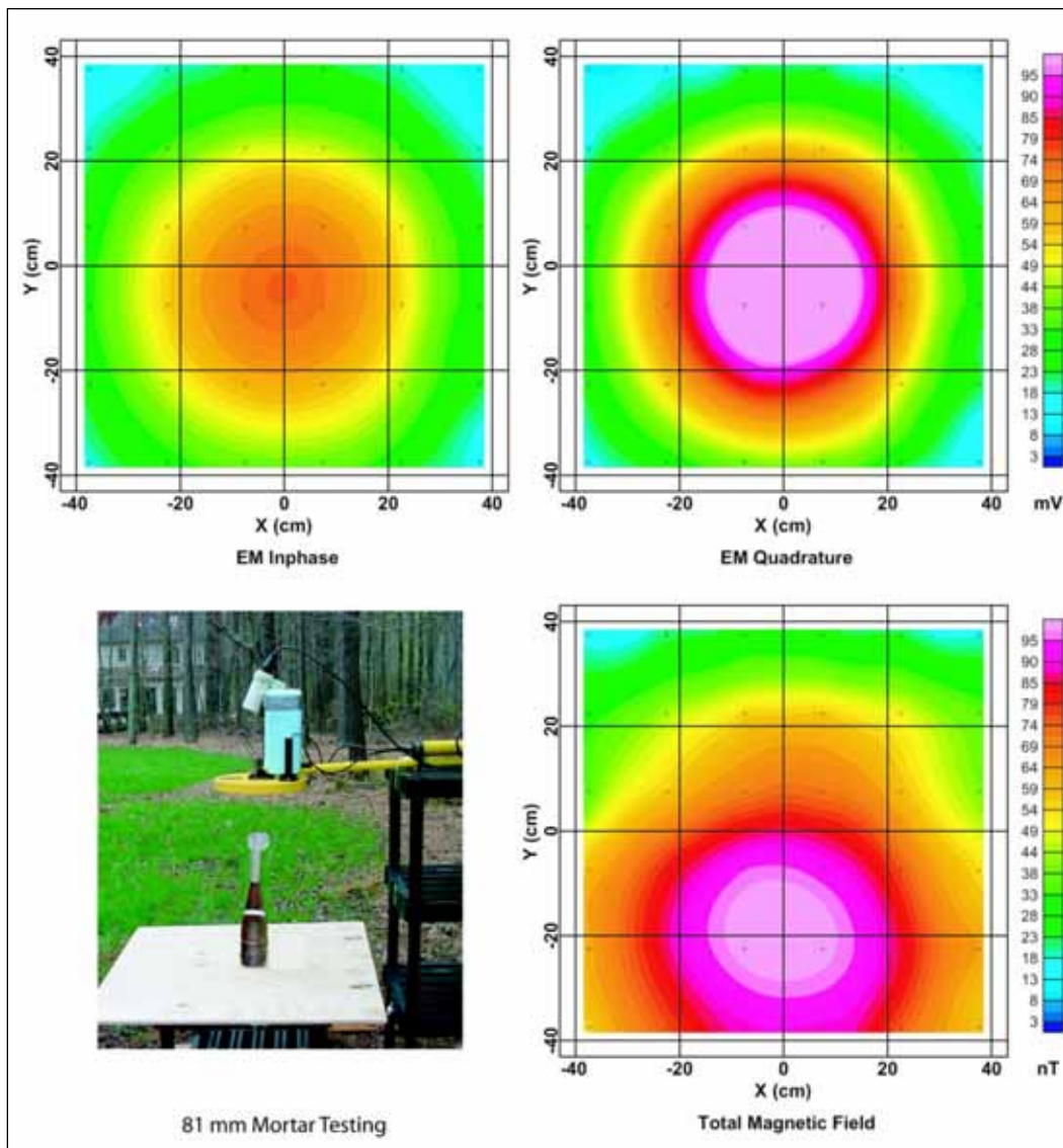
Figure 5. Simultaneously collected test stand data for an 81 mm mortar. The upper panels present the EM inphase (left) and quadrature (right) component responses in millivolts. The lower left panel shows the test set-up, and the magnetometer data (nT) are presented in the lower right panel.
