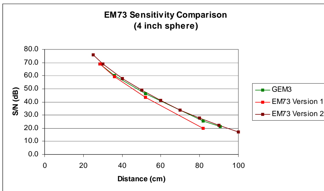
Figure 3. Sensor sensitivity test results for a 4-in.-diameter sphere placed at varying distances along the centerline of the coil axis. S/N decibels (dB) calculated as 20 \times \log(\text{signal}/\text{noise}) .
