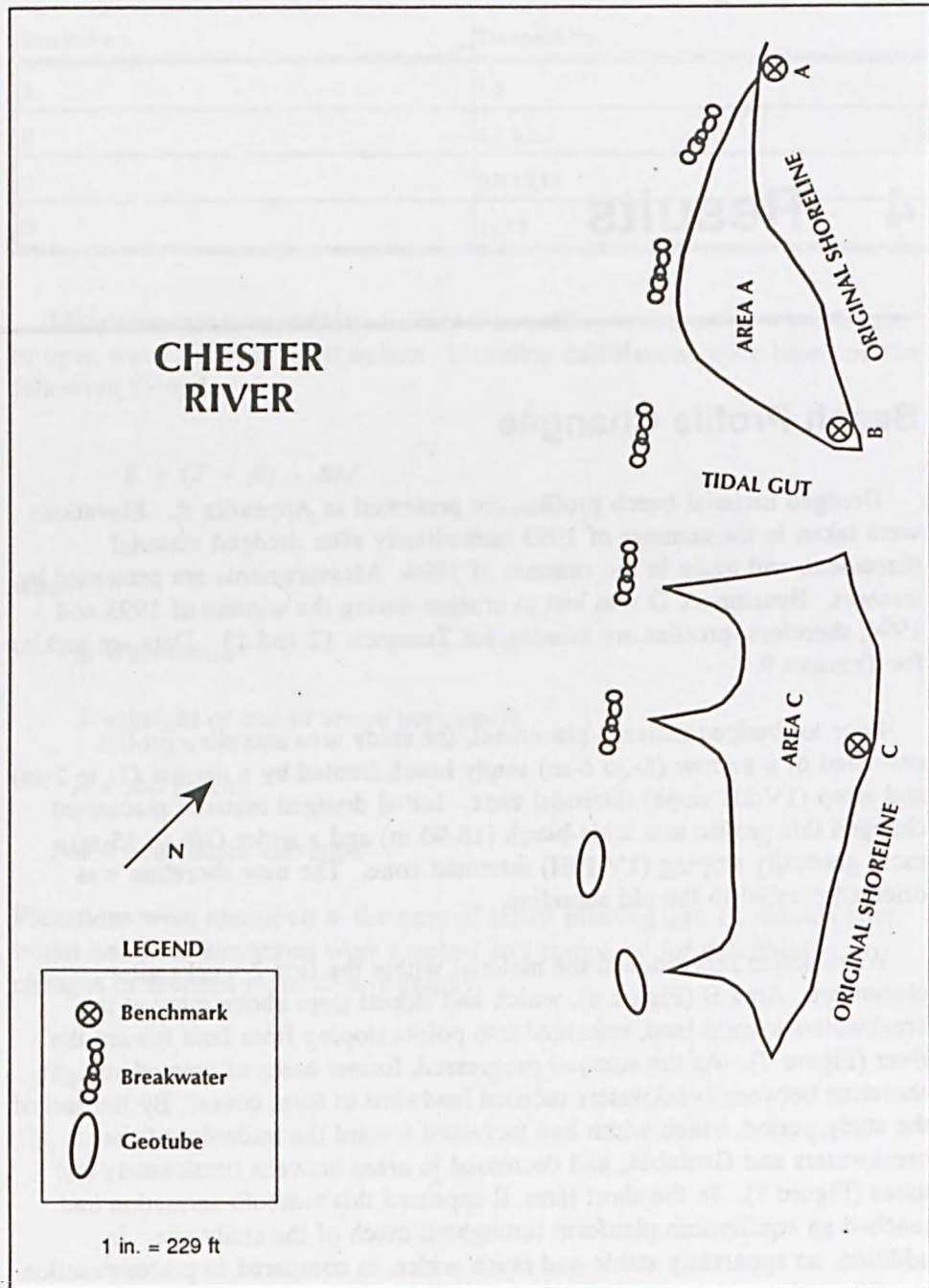
Figure 7. 1994 shoreline configuration
