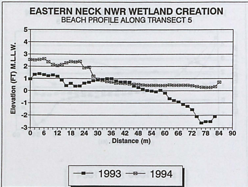
Figure A5. Beach profile along Transect 5
