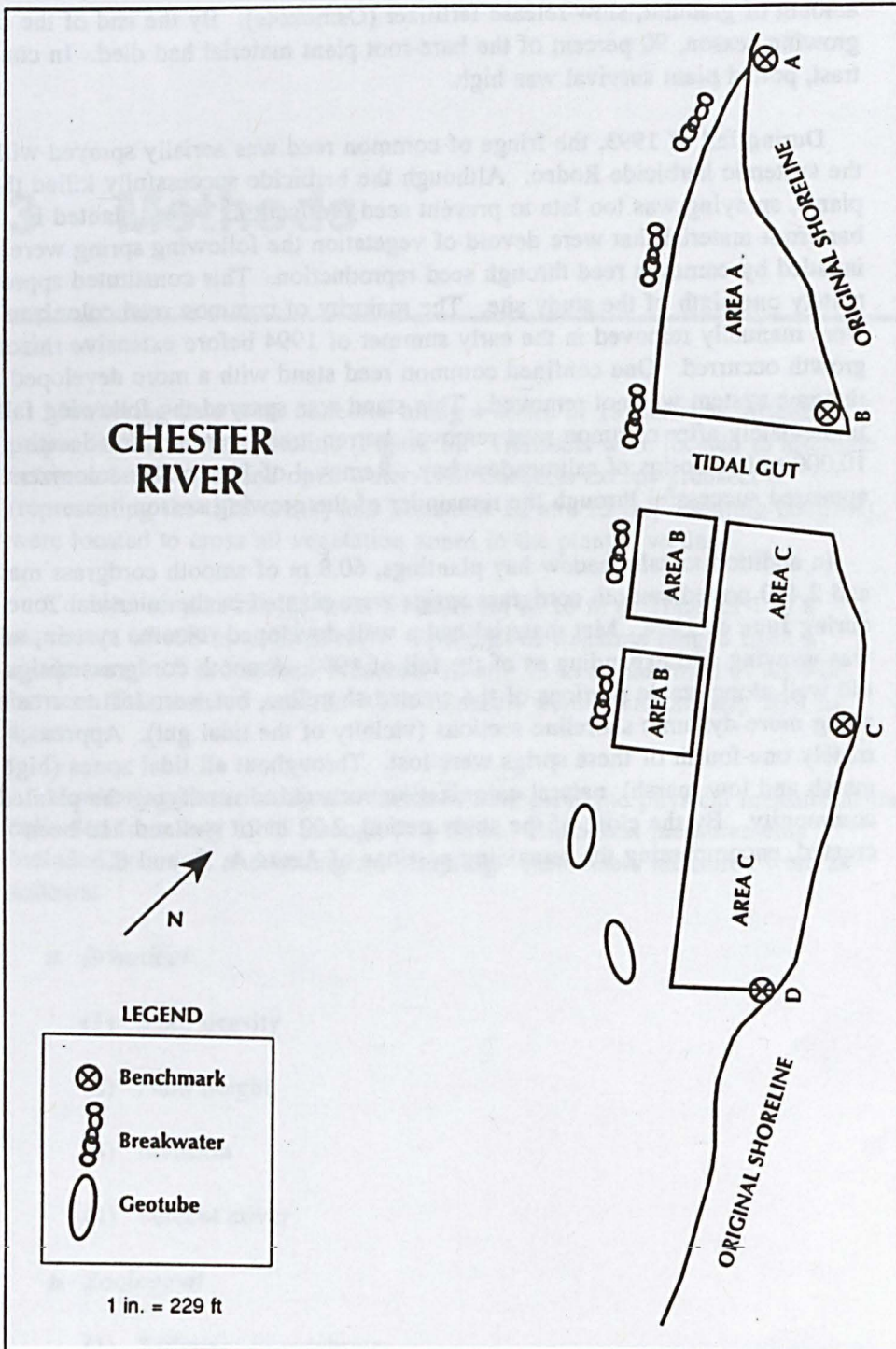
Figure 5. Dredged material deposition areas
