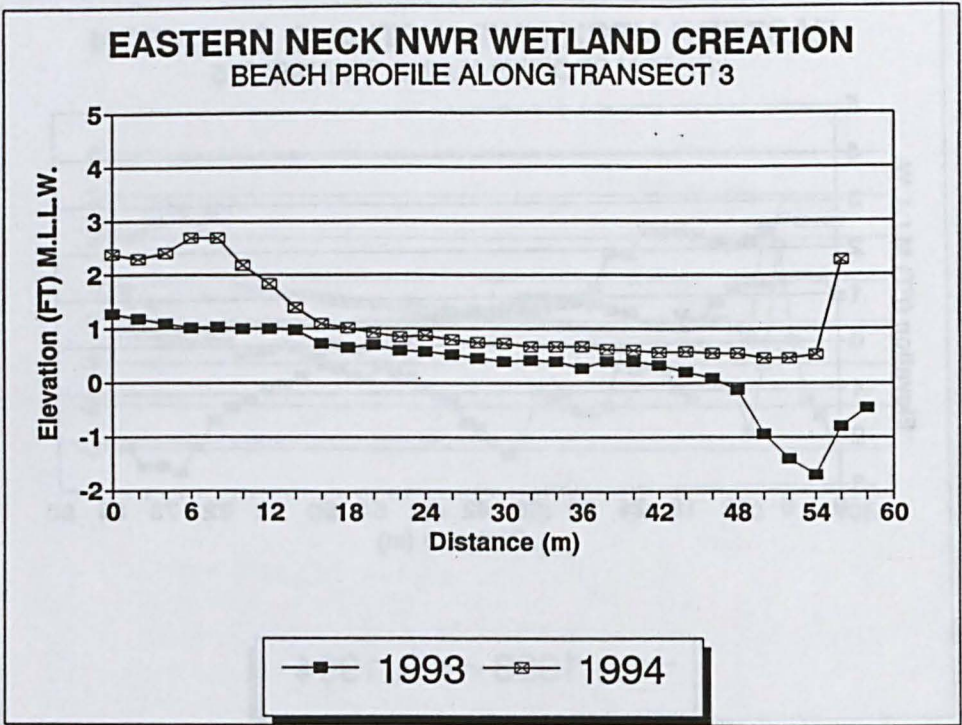
Figure A3. Beach profile along Transect 3
