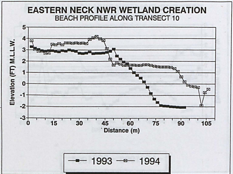
Figure A9. Beach profile along Transect 10
