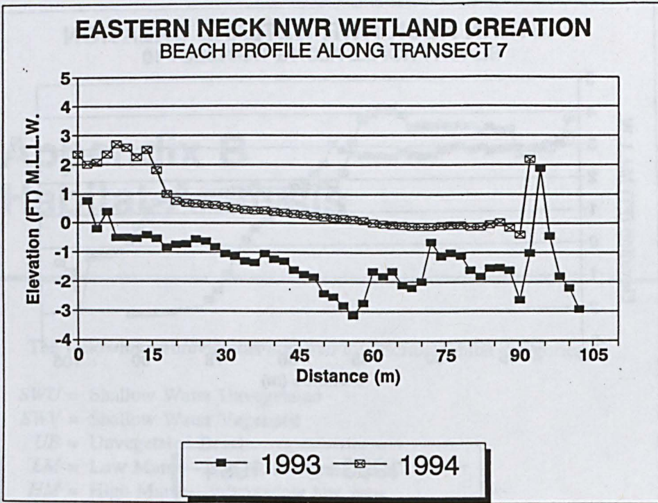
Figure A7. Beach profile along Transect 7
