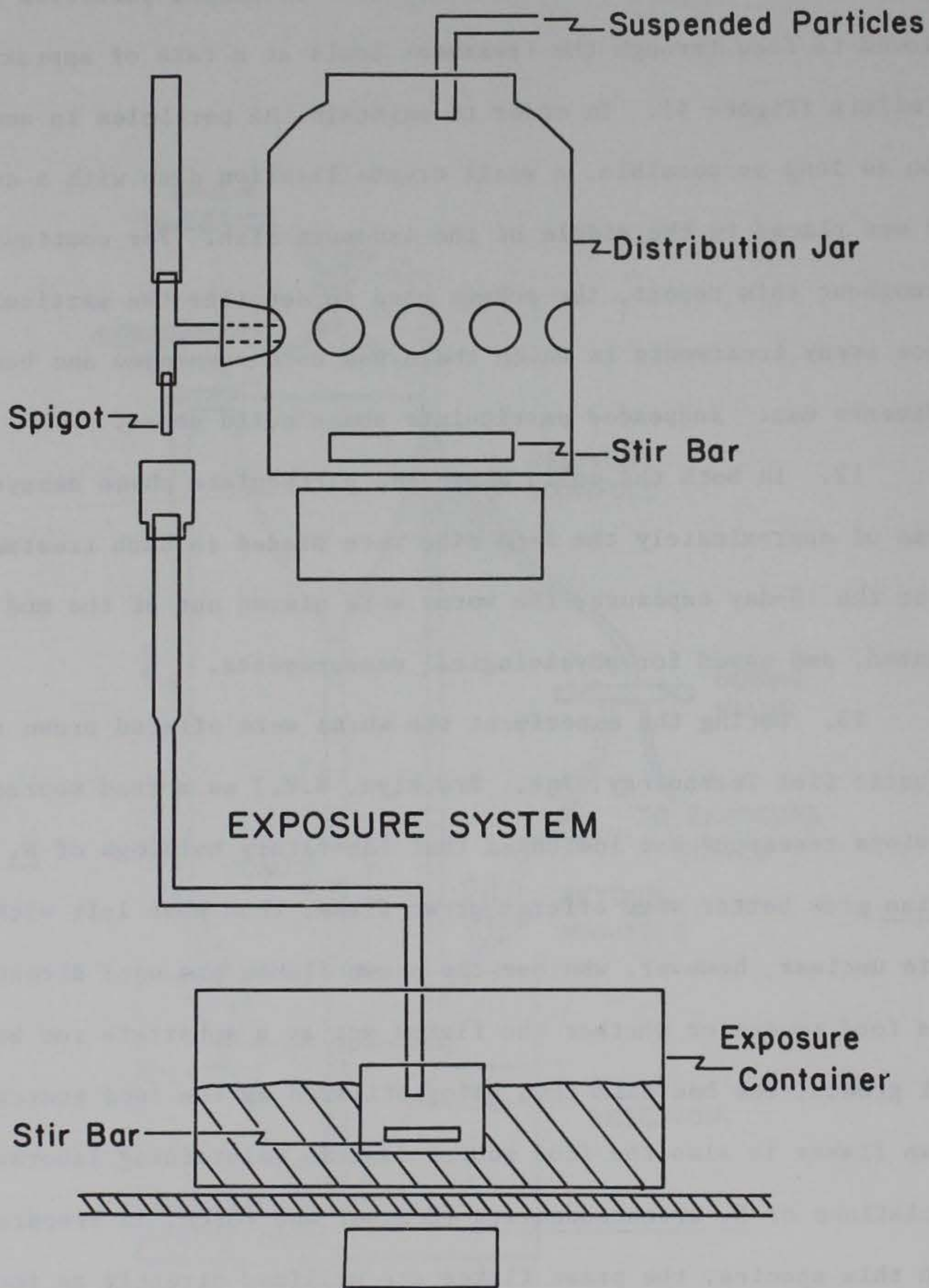
Figure 4. Schematic of the suspended distribution and dosing system used to expose juvenile N. incisa to reference and BRH sediment
