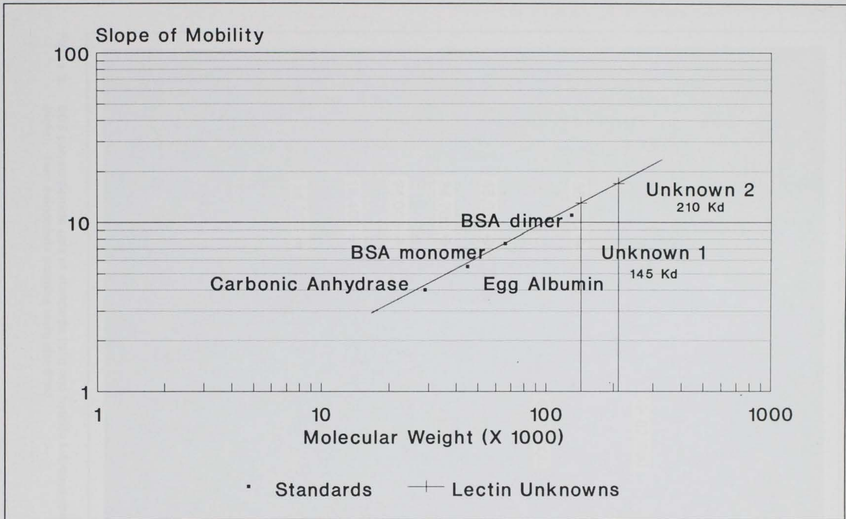
Figure 2. Graph of hydrilla lectin depicting molecular weights of standards and hydrilla L-fucose lectin. Two polymeric forms of the lectin were isolated
