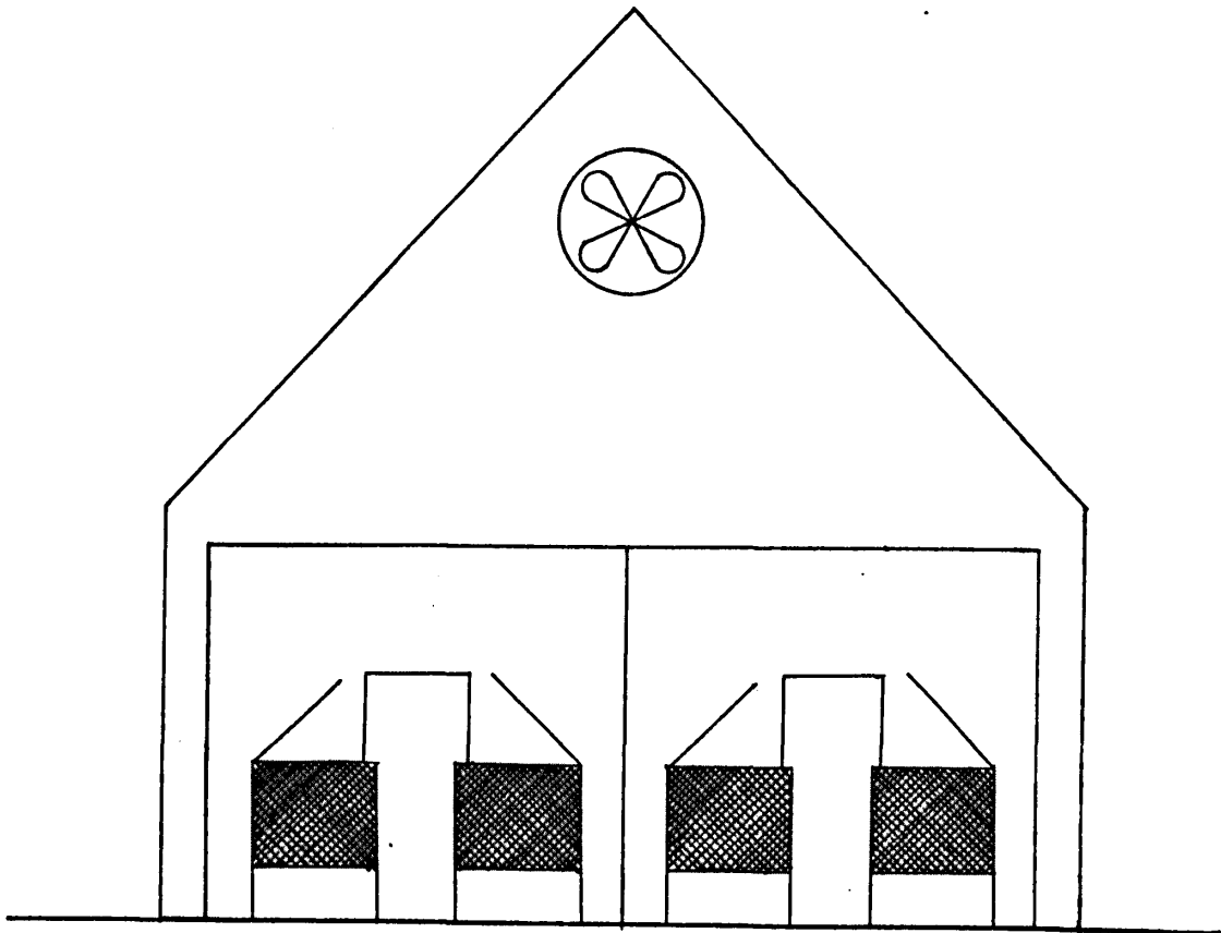
Figure 4. System of screened cages for rearing Neochetina under quarantine in San Juan, Puerto Rico
