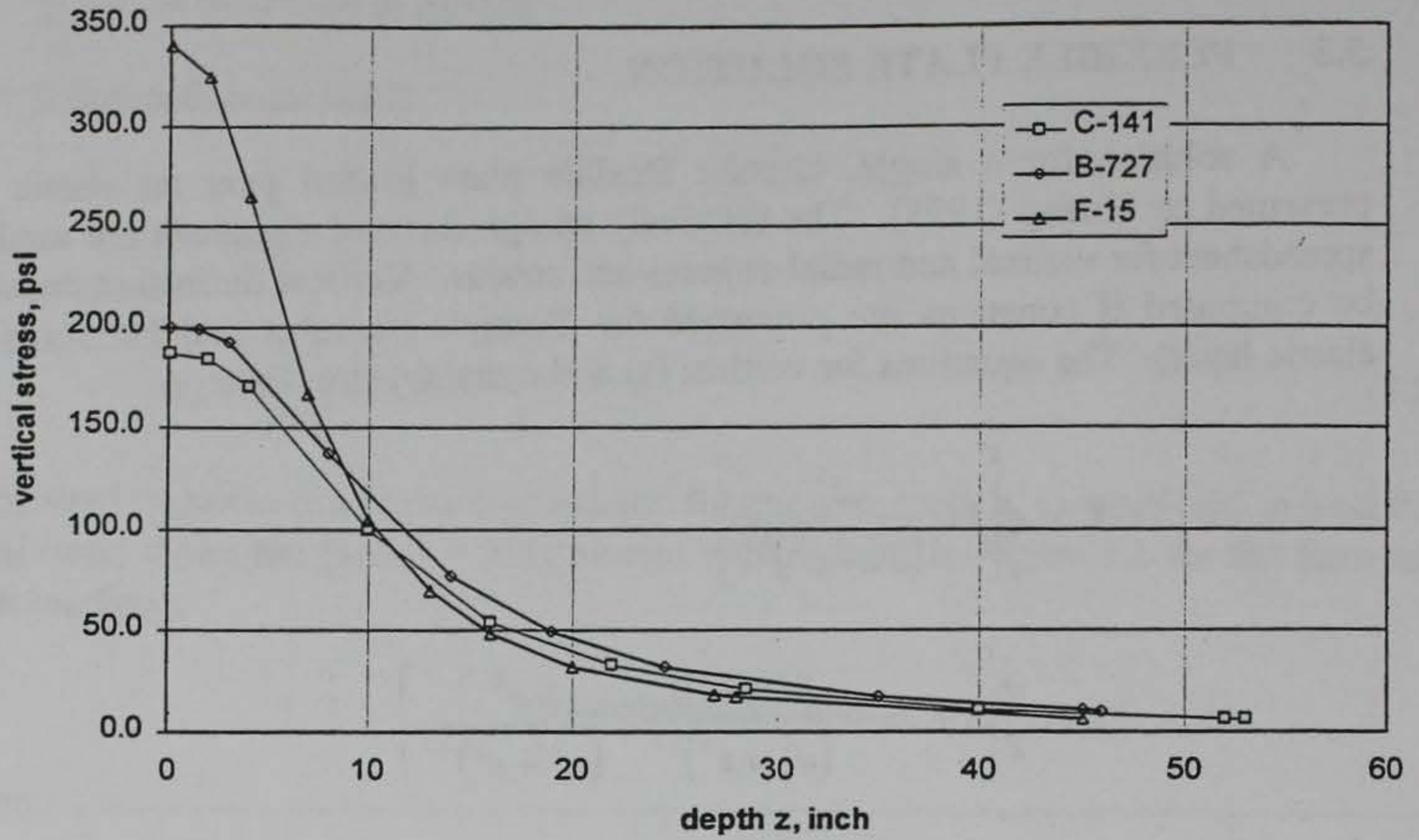
Figure 3.2. Flexible plate solution for vertical stress.
