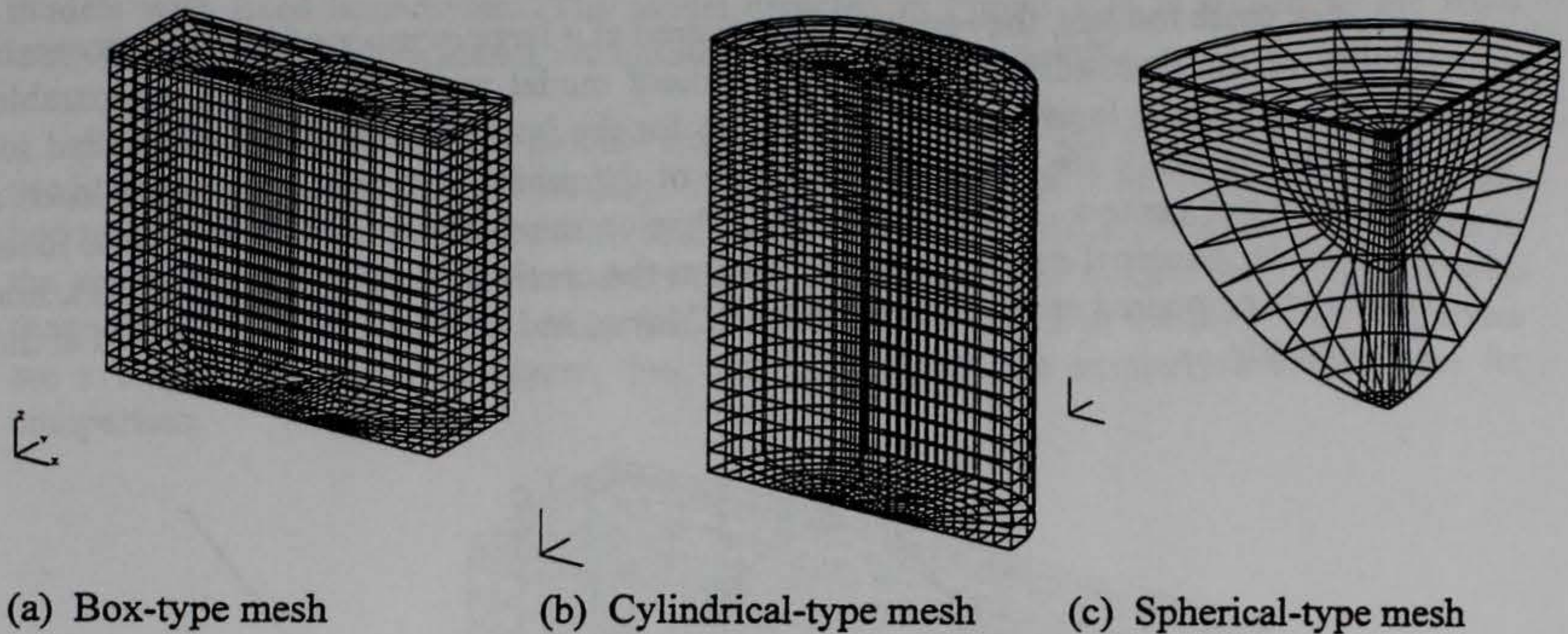
Figure 3.21. General 3-D finite element mesh types.
