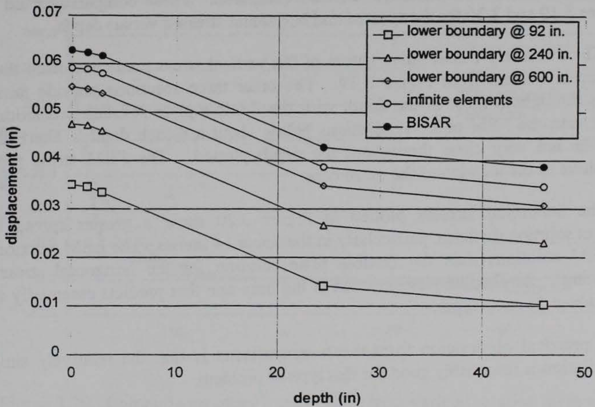
Figure 3.18. Effect on displacement of distance to lower boundary.
