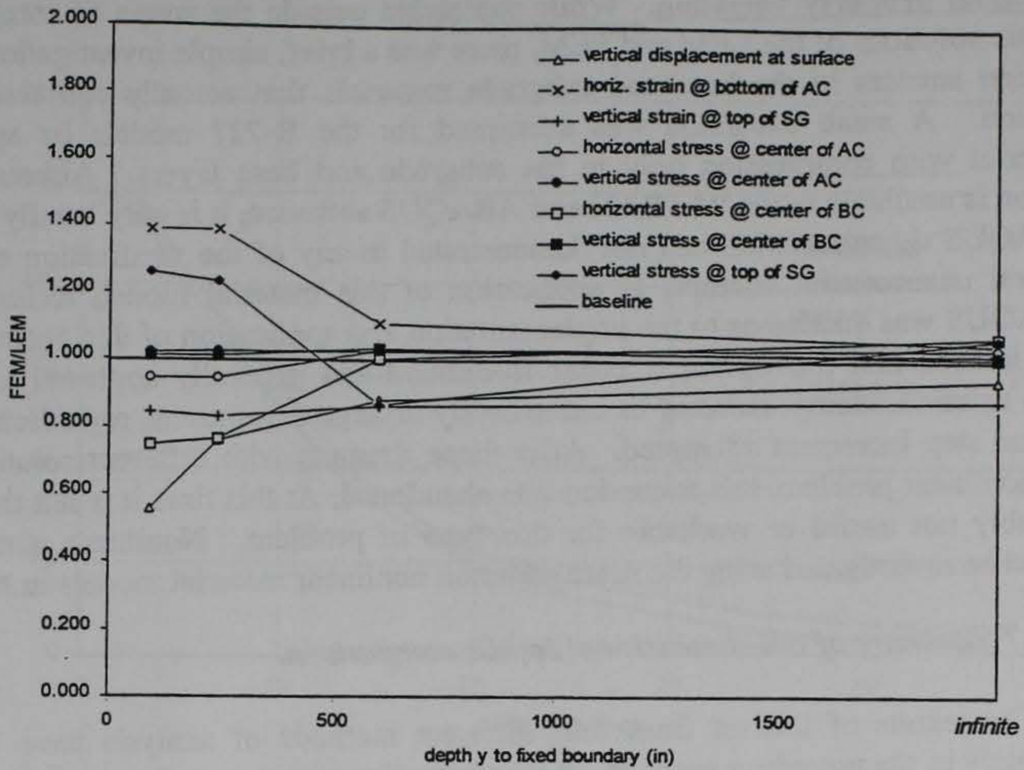
Figure 3.17. Effect on results of distance to lower boundary.
