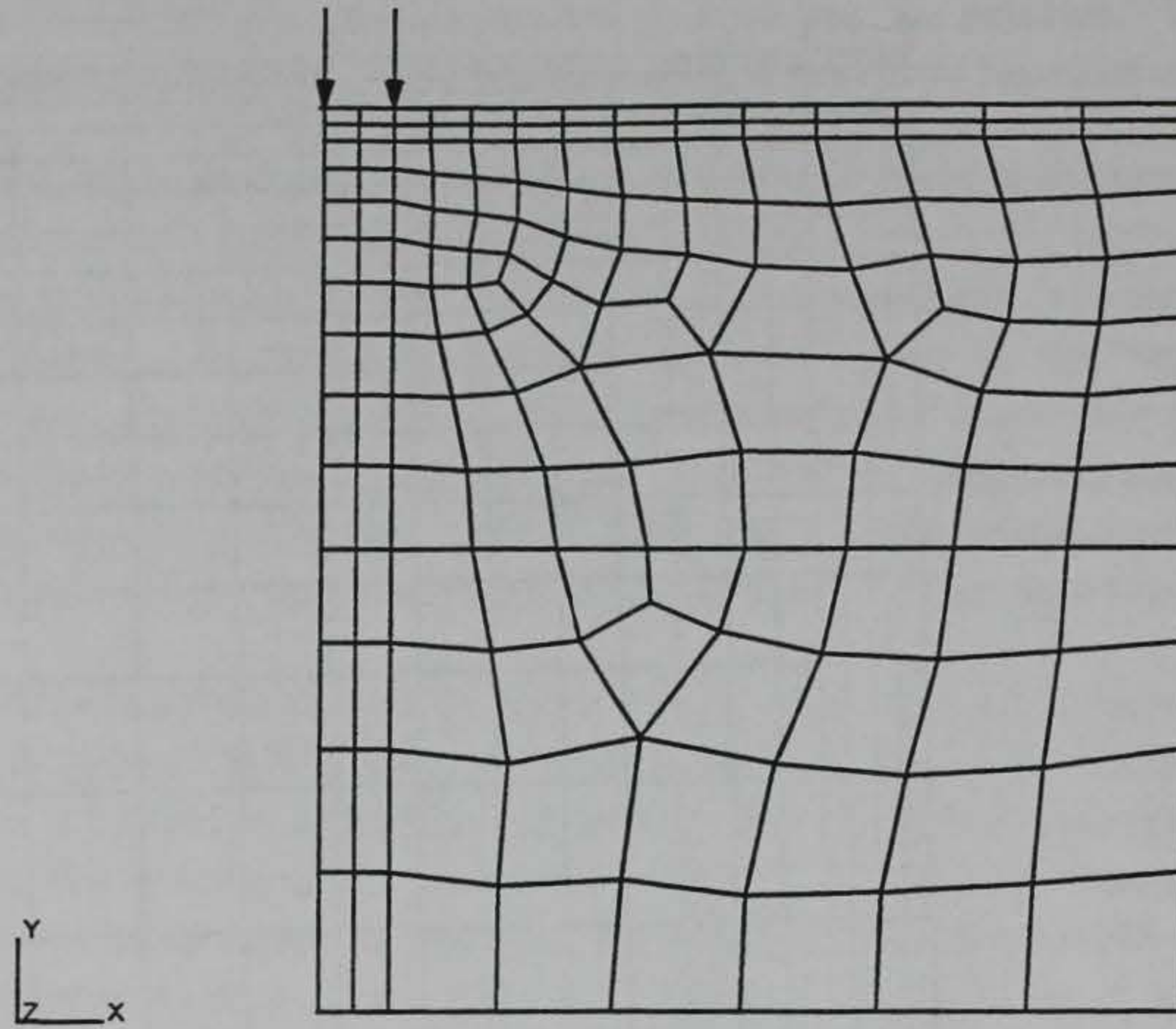
Figure 3.11. Paver-type finite element mesh for C-141 analysis.
