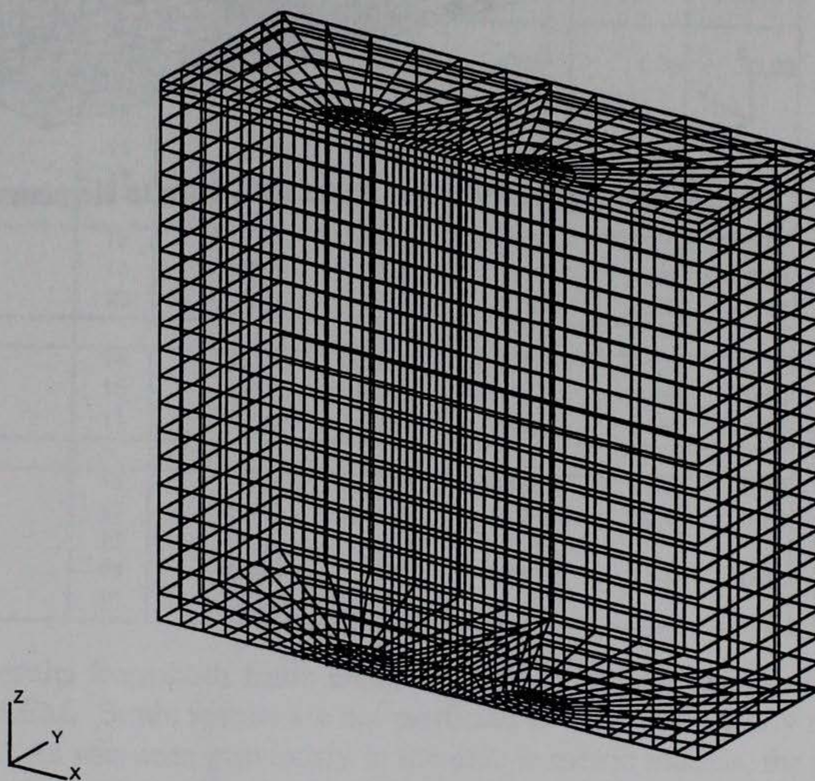
Figure 3.23. Box-type finite element mesh with fixed boundaries.
