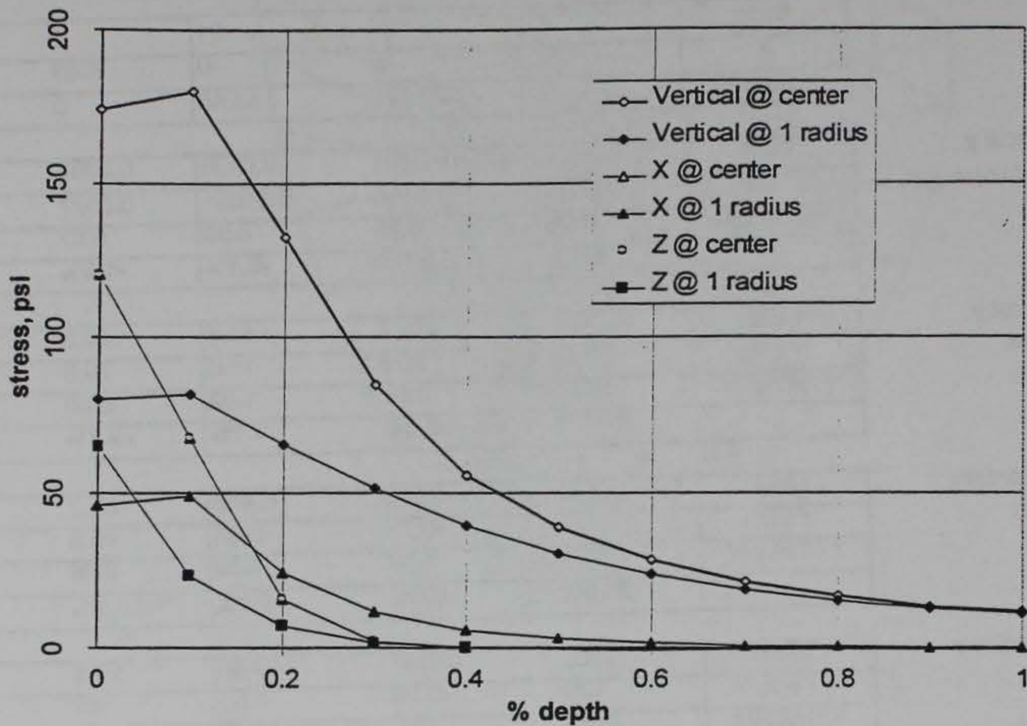
Figure 3.32. Predicted nodal stress versus depth (spherical model).
