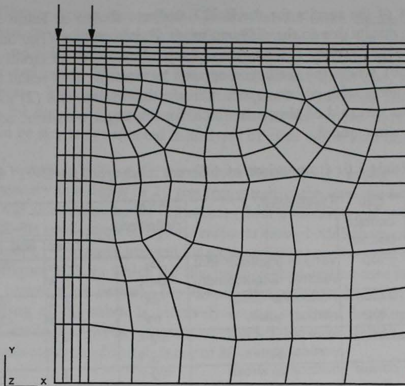
Figure 3.13. Paver-type finite element mesh for F-15 analysis.
