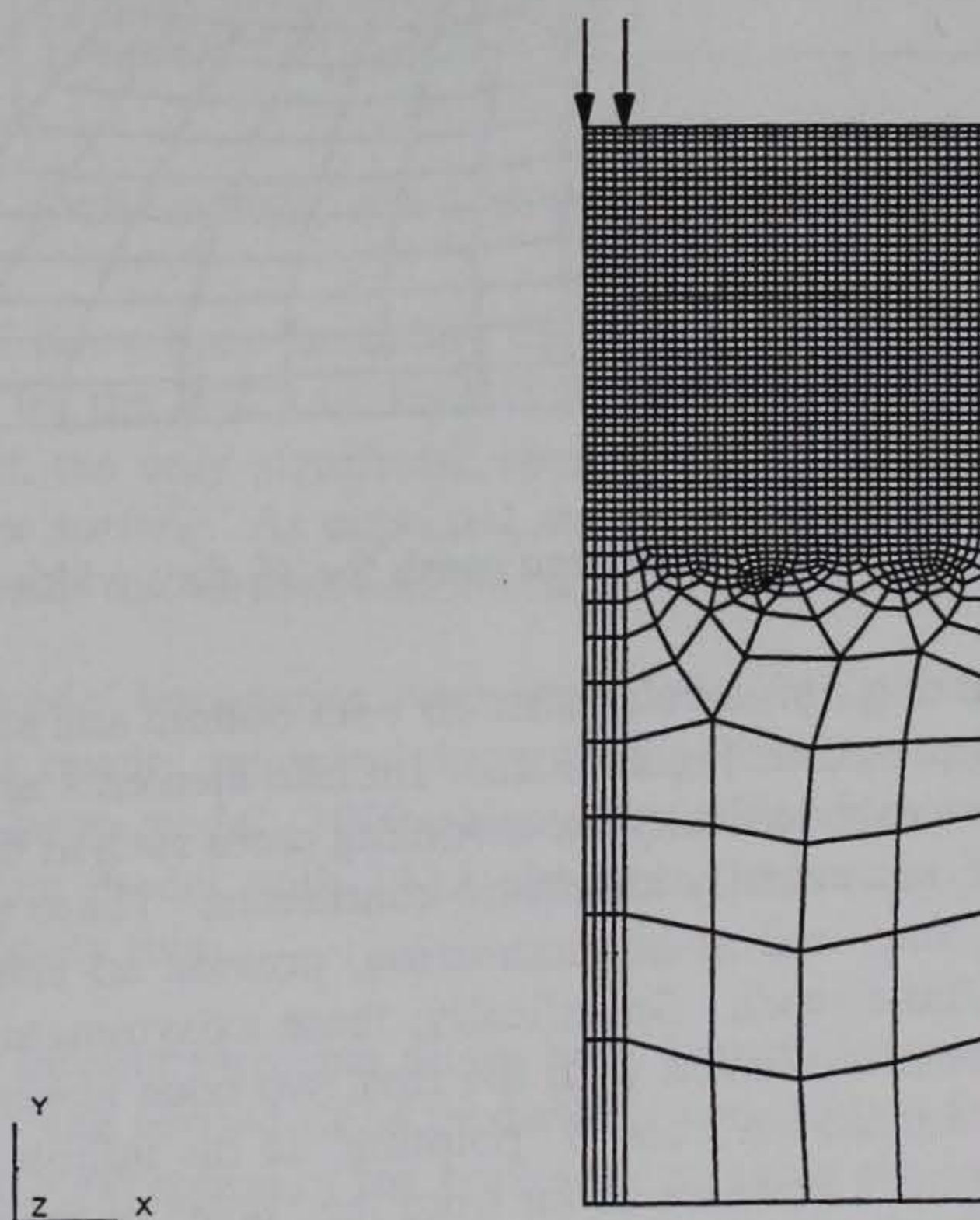
Figure 3.14. Finite element mesh for 20-foot depth.
