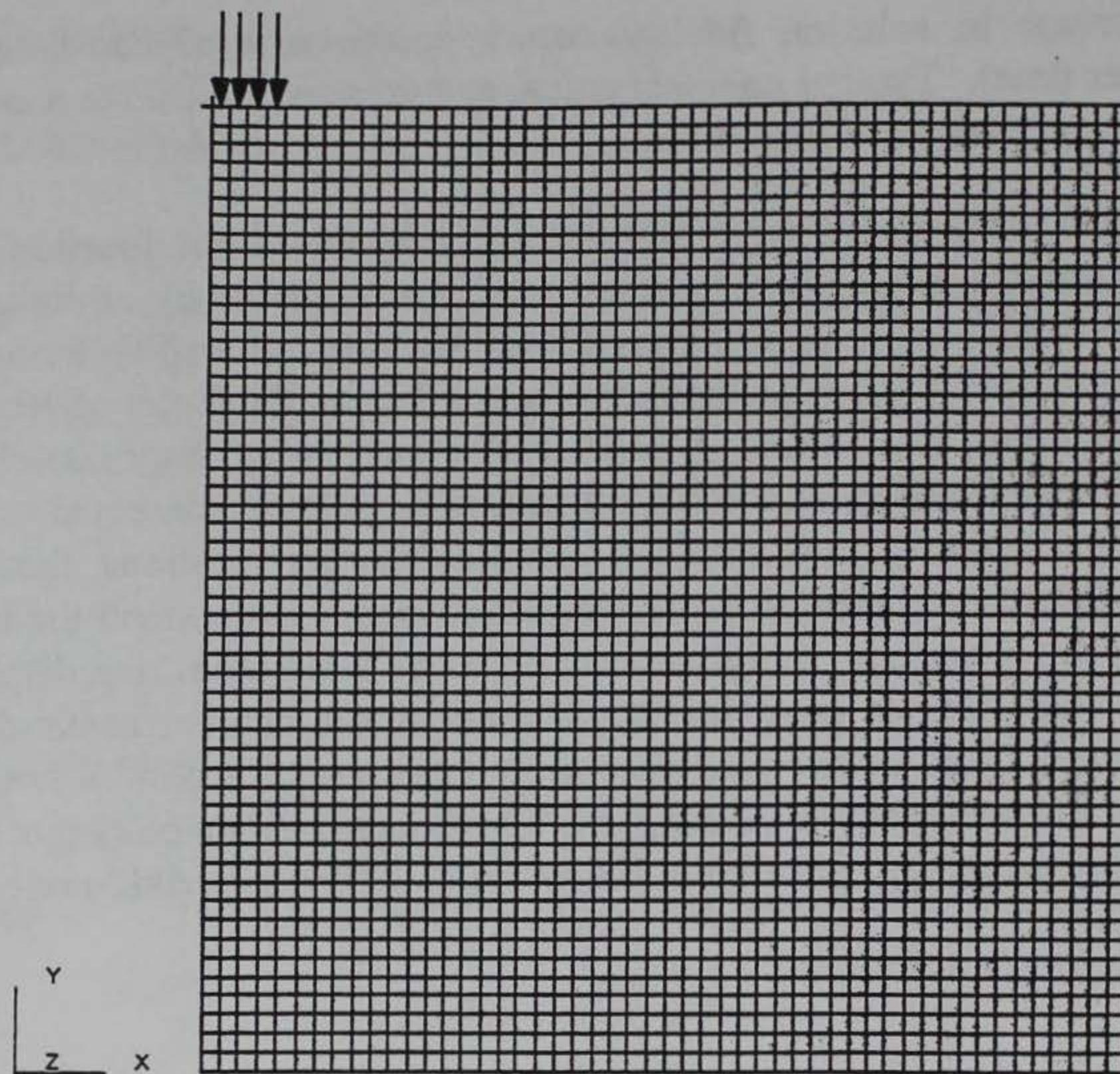
Figure 3.5. Baseline finite element mesh for C-141 analysis.
