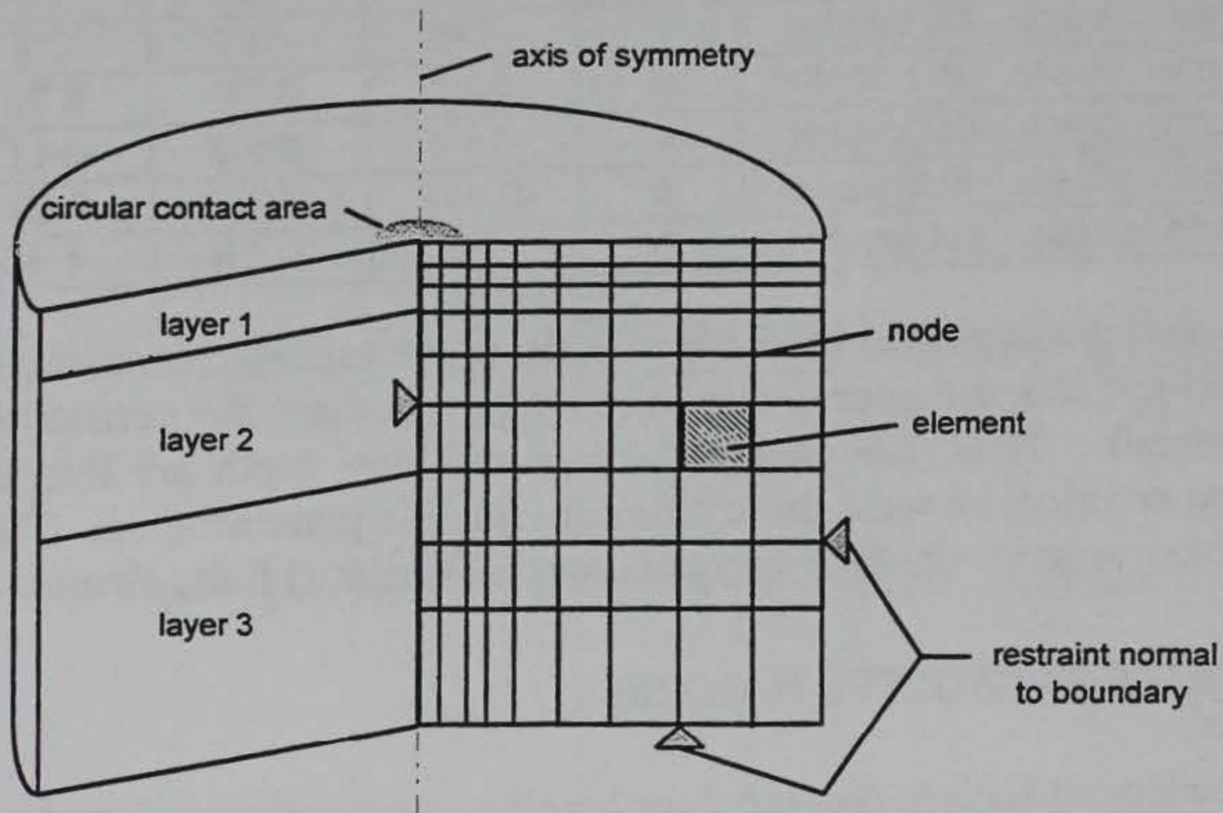
Figure 3.4. Axisymmetric model.
