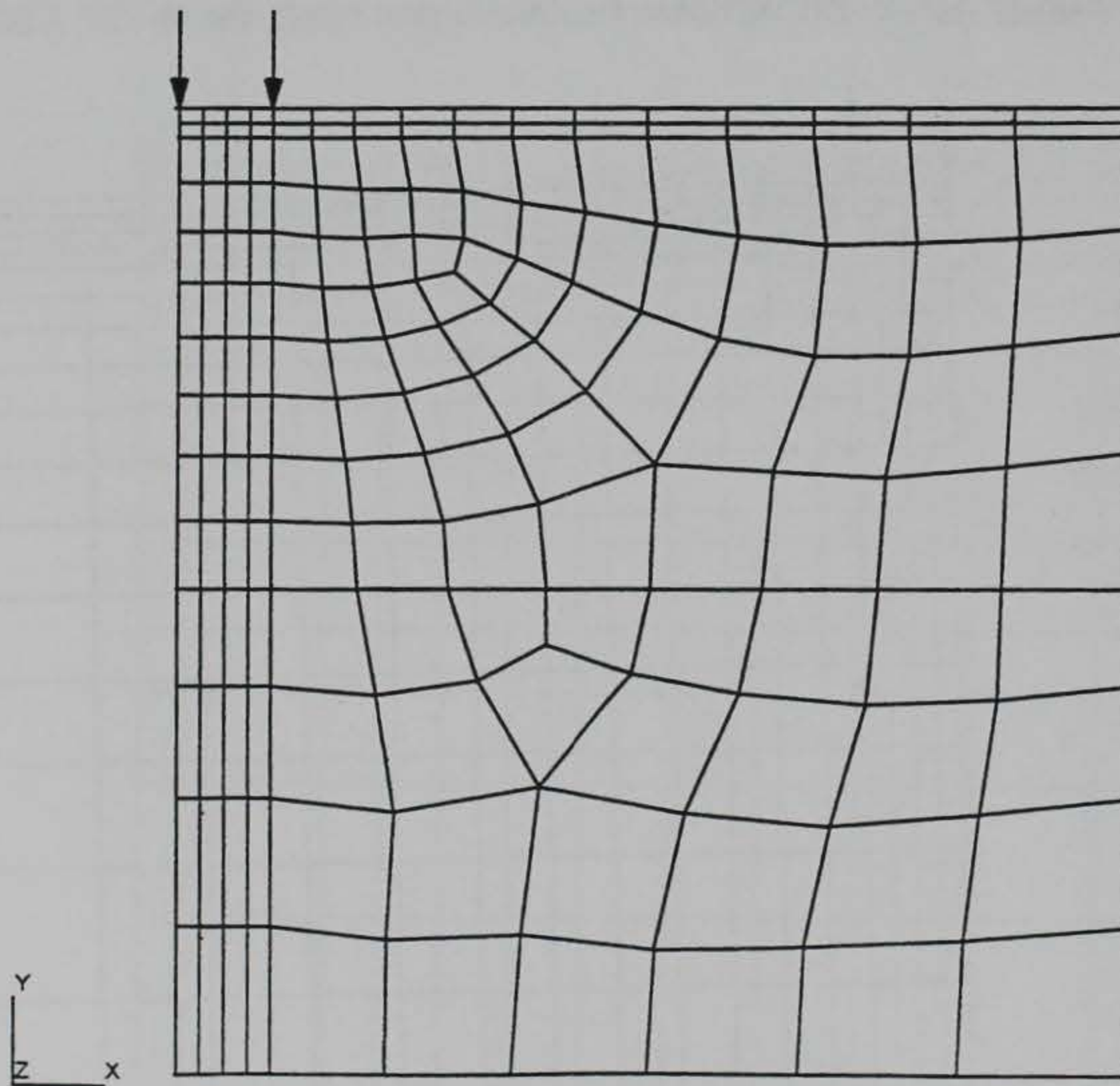
Figure 3.12. Paver-type finite element mesh for B-727 analysis.
