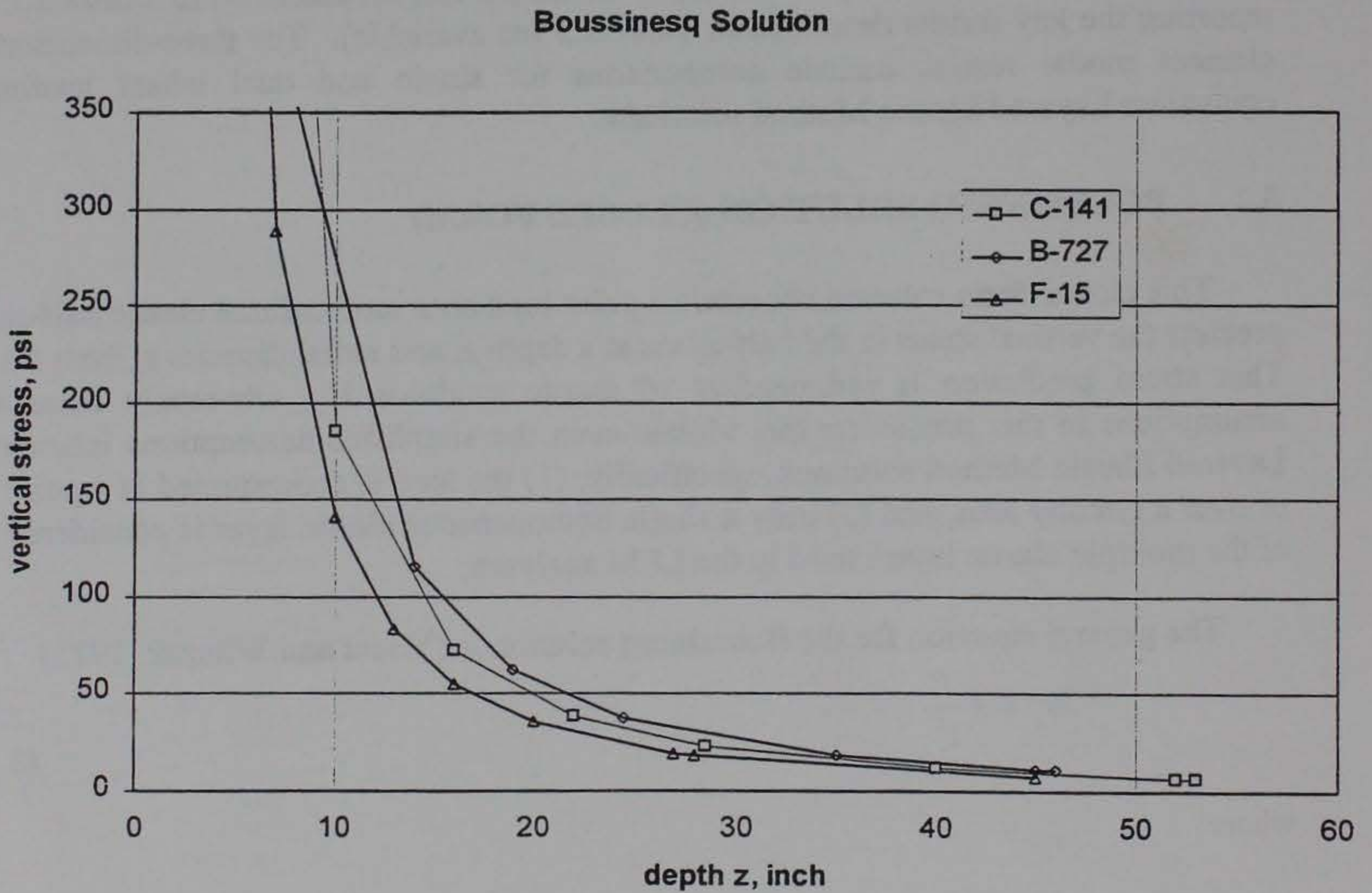
Figure 3.1. Boussinesq solution for vertical stress.
