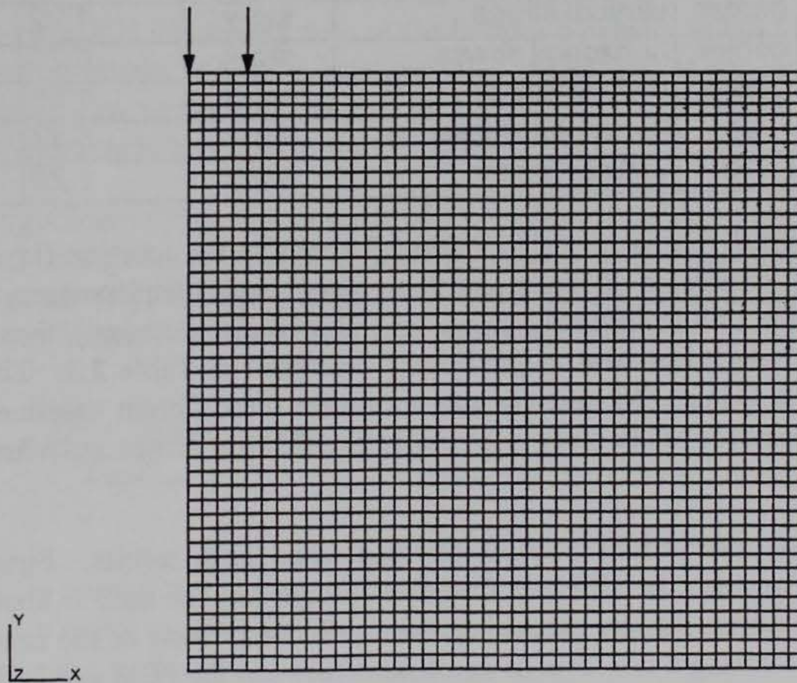
Figure 3.7. Baseline finite element mesh for F-15 analysis.
