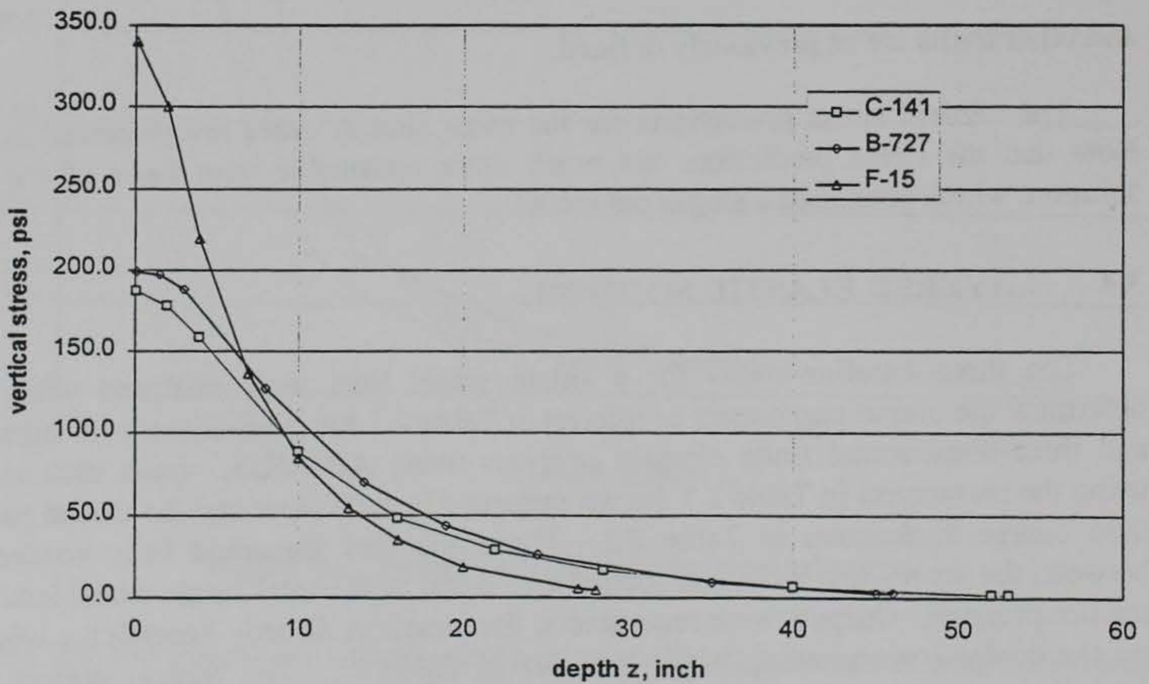
Figure 3.3. Layered elastic solution for vertical stress.
