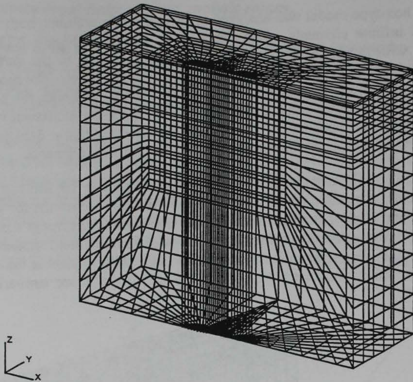
Figure 3.24. Box-type mesh with infinite elements.
