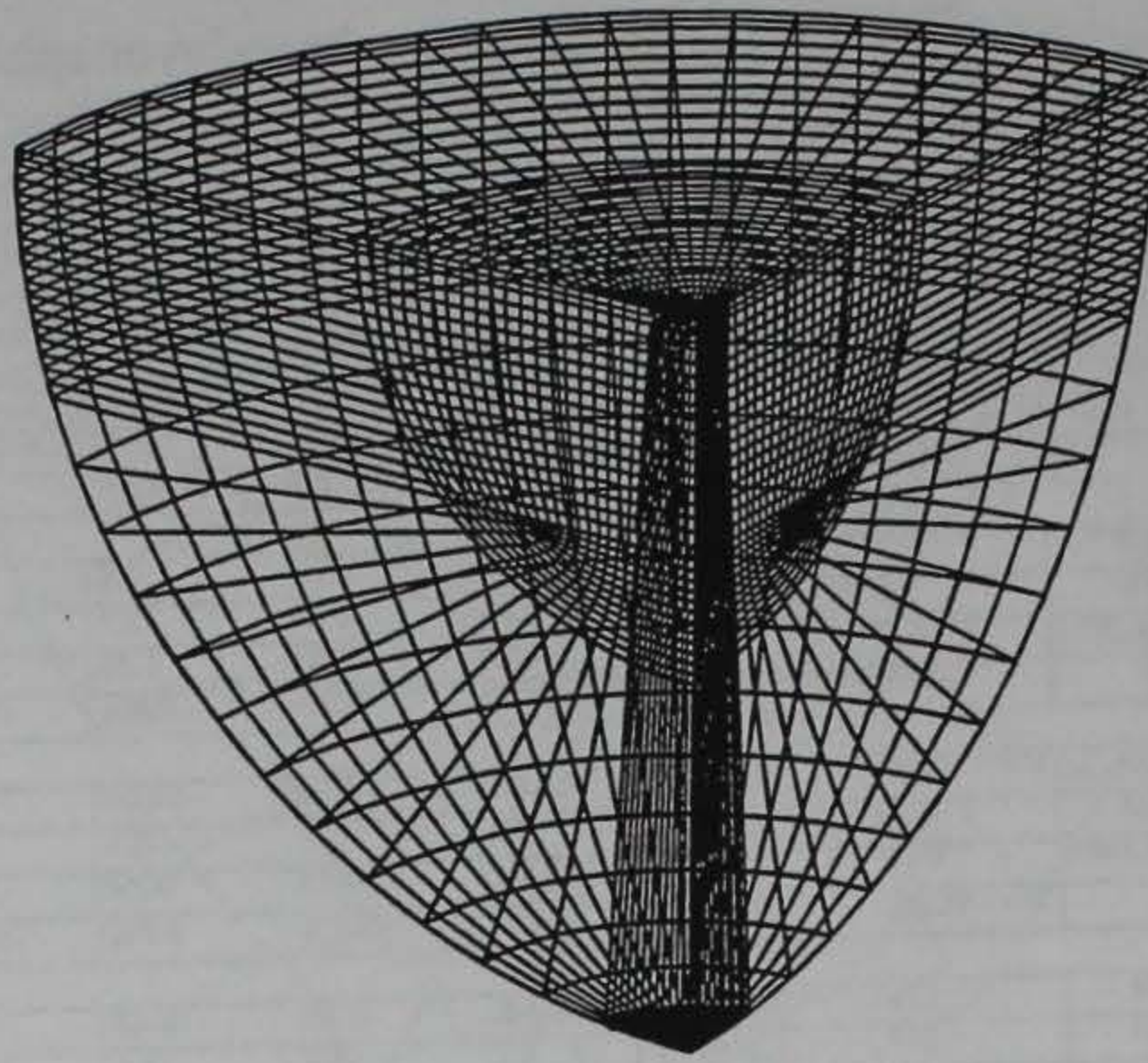
Figure 3.35. Refined three-layer spherical-type mesh with layered infinite elements.
