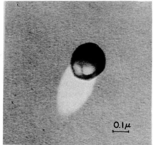
Figure 3b. Spherule (possibly extraterrestrial) in snow crystal at Site 2, Greenland.
