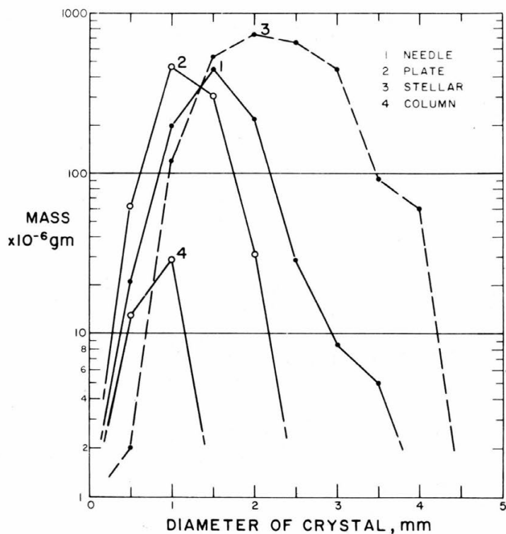
Figure 2. Mass distribution of snow crystals in summer at Site 2, Greenland.
