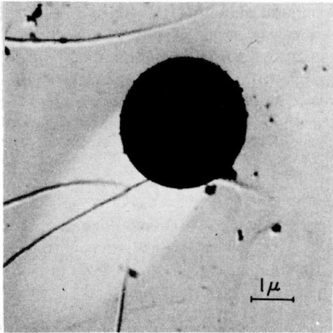
Figure 3c. Spherule (possibly fly ash) in snow crystal at Houghton, Michigan.
