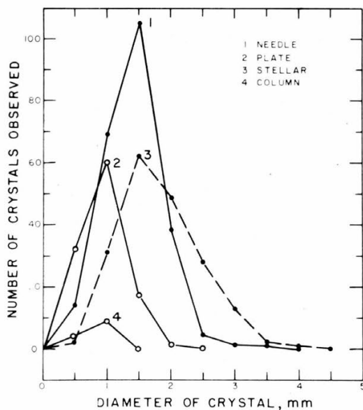
Figure 1. Size distribution of snow crystals in summer at Site 2, Greenland. The size is diameter of plate and stellar crystals and the largest dimension of needle and column-shaped crystals.
