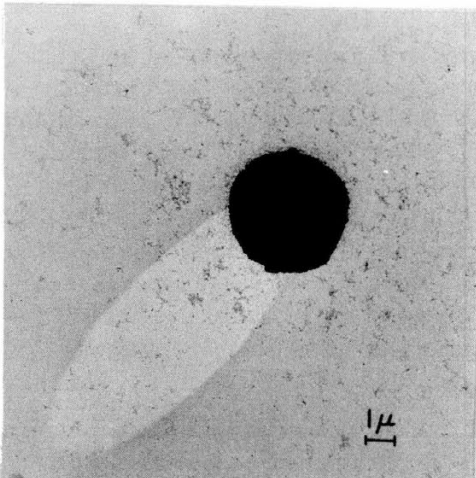
Figure 3e. Spherule found in ashes from coal furnace at Fairbanks, Alaska.
