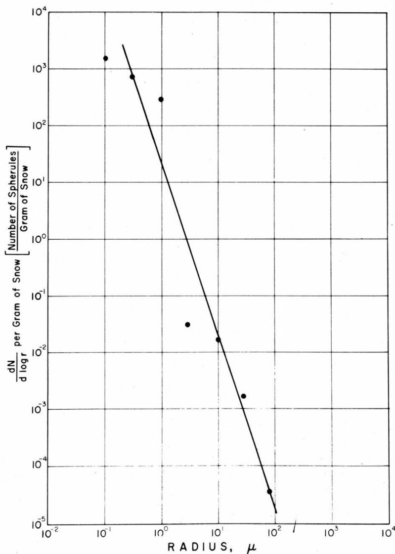
Figure 4. Size distribution of spherules per gram of snow at Site 2, Greenland.
