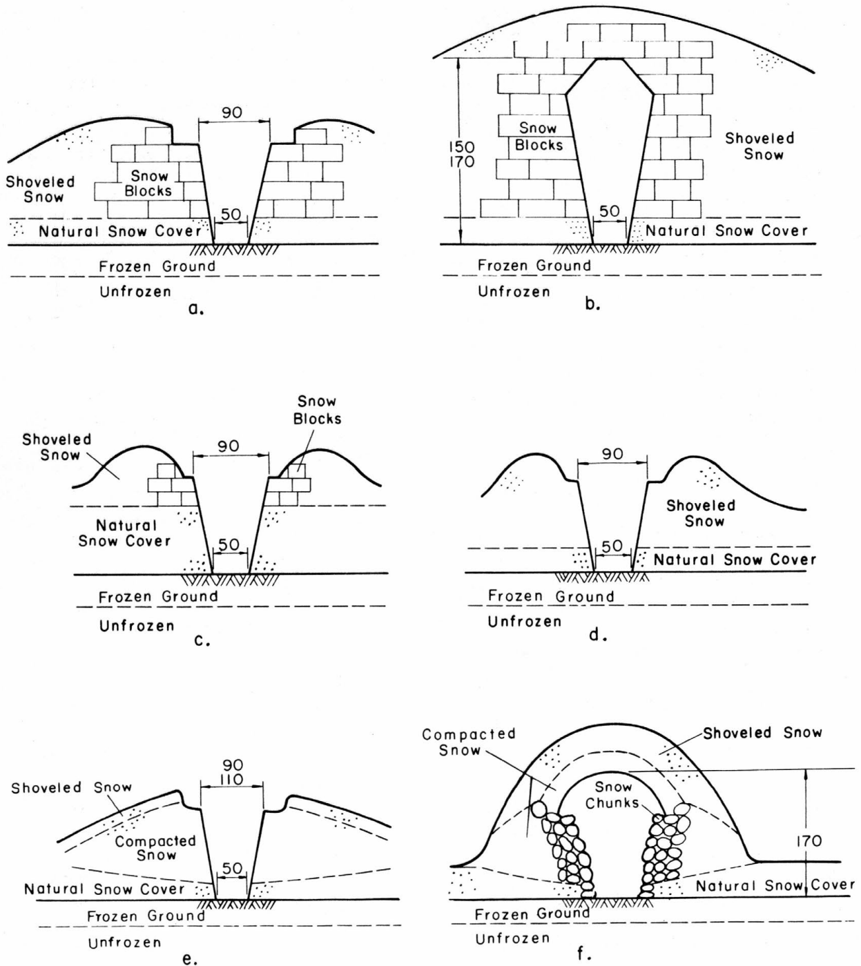
Figure 11. Types of expedient snow combat trenches. Dimensions given in centimeters (not to scale). After Shamshurov (1969). a) Uncovered trench in a snowdrift using cut blocks. b) Covered trench in a deep snowdrift. c) Hasty trench in medium snow. d) Hasty trench in shallow snow. e) Open trench in compacted, reworked snow. f) Covered trench in compacted snow using snowballs and chunks.
