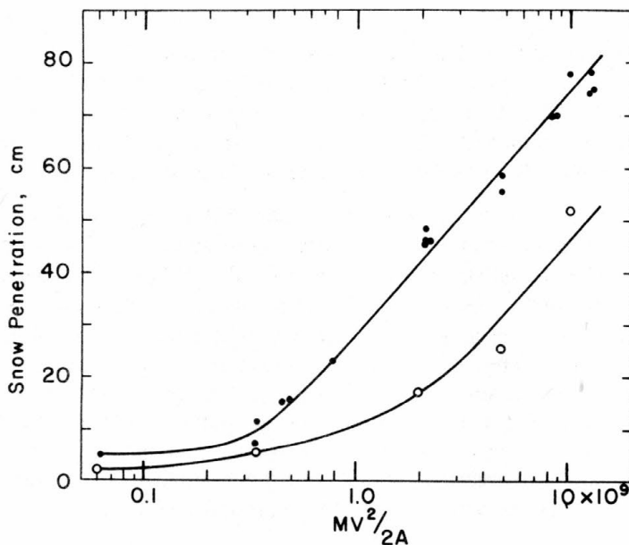
Figure 7. Snow penetration as a function of energy, 8.3 g spherical projectile. Dots: snow density 0.4 g/cm 3 . Circles: snow density 0.6 g/cm 3 .
