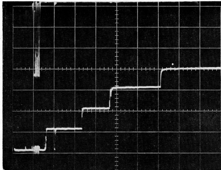
Figure 2. Example of an oscilloscope record obtained by the set-up shown in Figure 1. Snow density 0.37 \text{ g/cm}^3 , terminal velocity 19,677 \text{ cm/sec} , maximum penetration 91 \text{ cm} , projectile mass 12.5 \text{ grams} .
