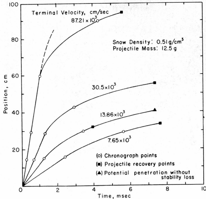
Figure 4. Loss of projectile stability in snow.
