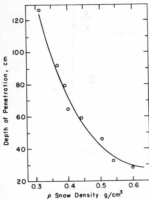
Figure 10. Dependence of snow penetration by .30-caliber projectile upon snow density at impact energy E_n = 5 \times 10^9 \text{ g cm}^2/\text{sec}^2 \text{ cm}^2 .
