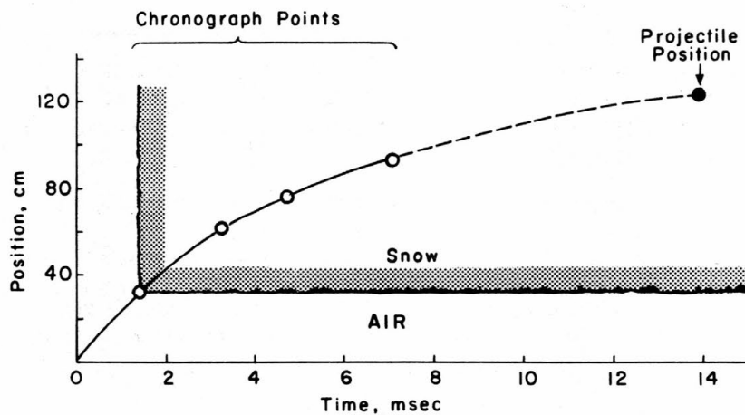
Figure 3. Projectile penetration into snow. Data from Figure 2.
