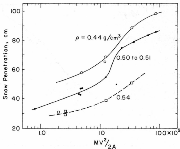
Figure 6. Snow penetration as a function of energy, .30-caliber projectile.
