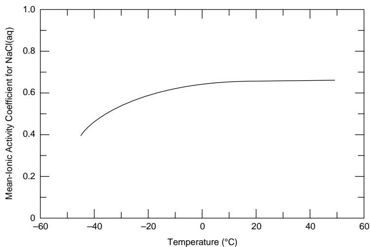
Figure 9. Mean-ionic activity coefficient of NaCl(aq) ( p = 0.1 \text{ MPa} , m = 1.0 \text{ mol kg}^{-1} ) as function of temperature.
