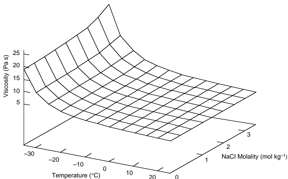
Figure 5. Predicted viscosity of aqueous NaCl solutions as affected by temperature and solution concentration.
