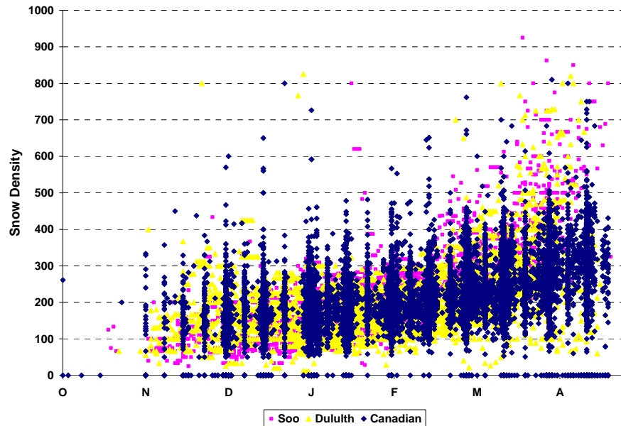
Figure 7. Snow density ( \text{kg/m}^3 ) by day of year at Sault Ste Marie (Soo), Duluth, and in the Lake Superior watershed and vicinity in Ontario, Canada.
