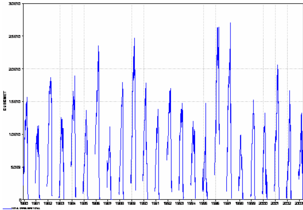
Figure 11. Daily SWE volume for the entire Lake Superior watershed.
