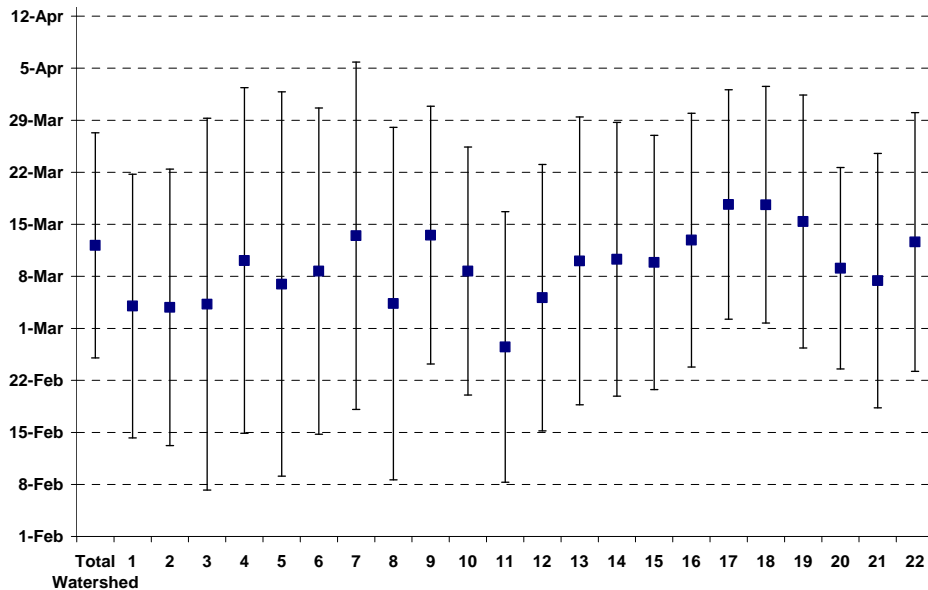
Figure 19. Average day of year and standard deviation of the maximum volume of SWE for the total Lake Superior watershed and the 22 sub-basins.
