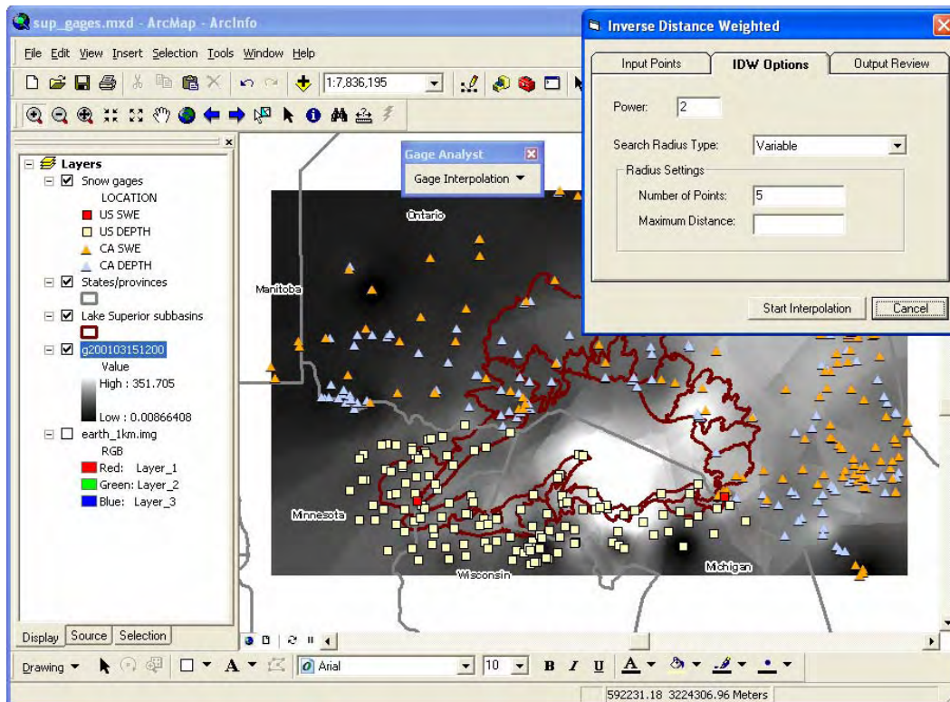
Figure 9. ArcMap and the Gage Analyst extension were used to interpolate the March 15, 2001 SWE grid displayed in a grey-scale color ramp.
