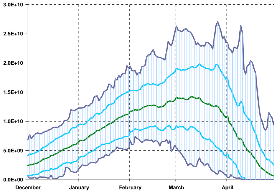
Figure 12. Daily SWE statistics for the entire Lake Superior watershed. Shown are the daily average (green), daily average plus and minus one standard deviation (blue), and the daily historical maximums and minimums.
