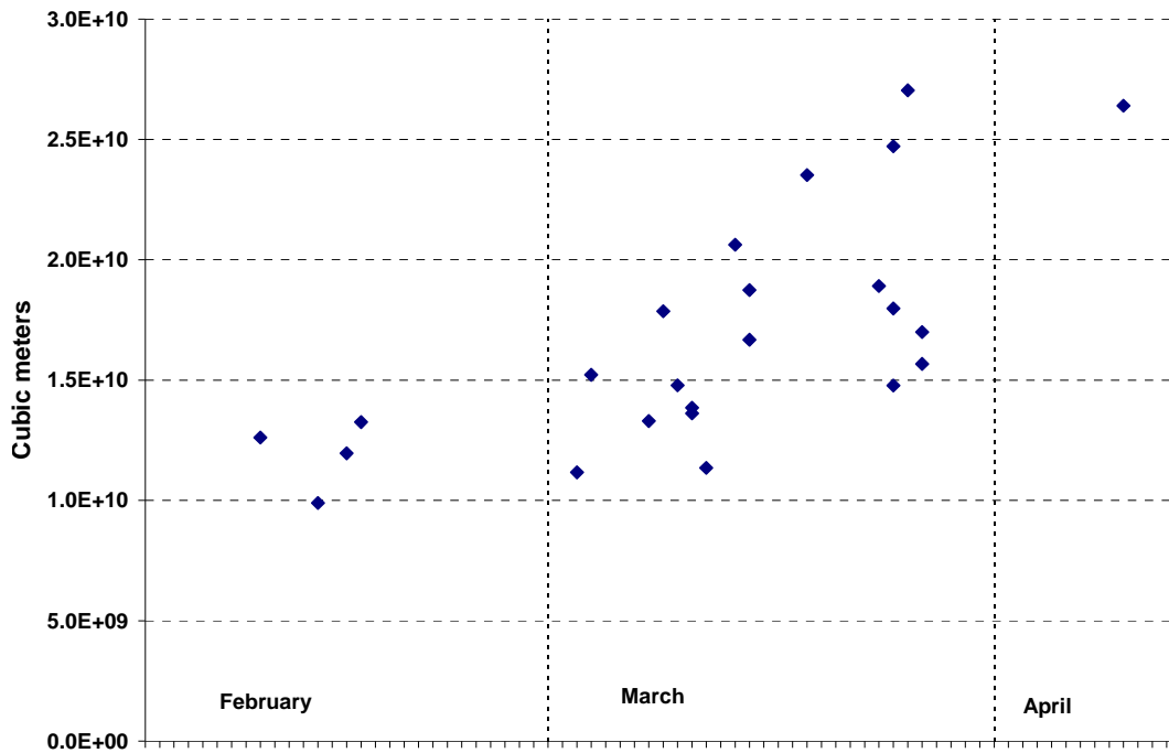
Figure 13. Maximum volume of SWE for the total Lake Superior watershed and the day of year when the maximum occurred.
