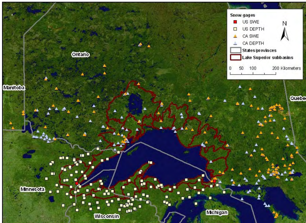
Figure 3. Stations providing snow information in the Lake Superior watershed.
