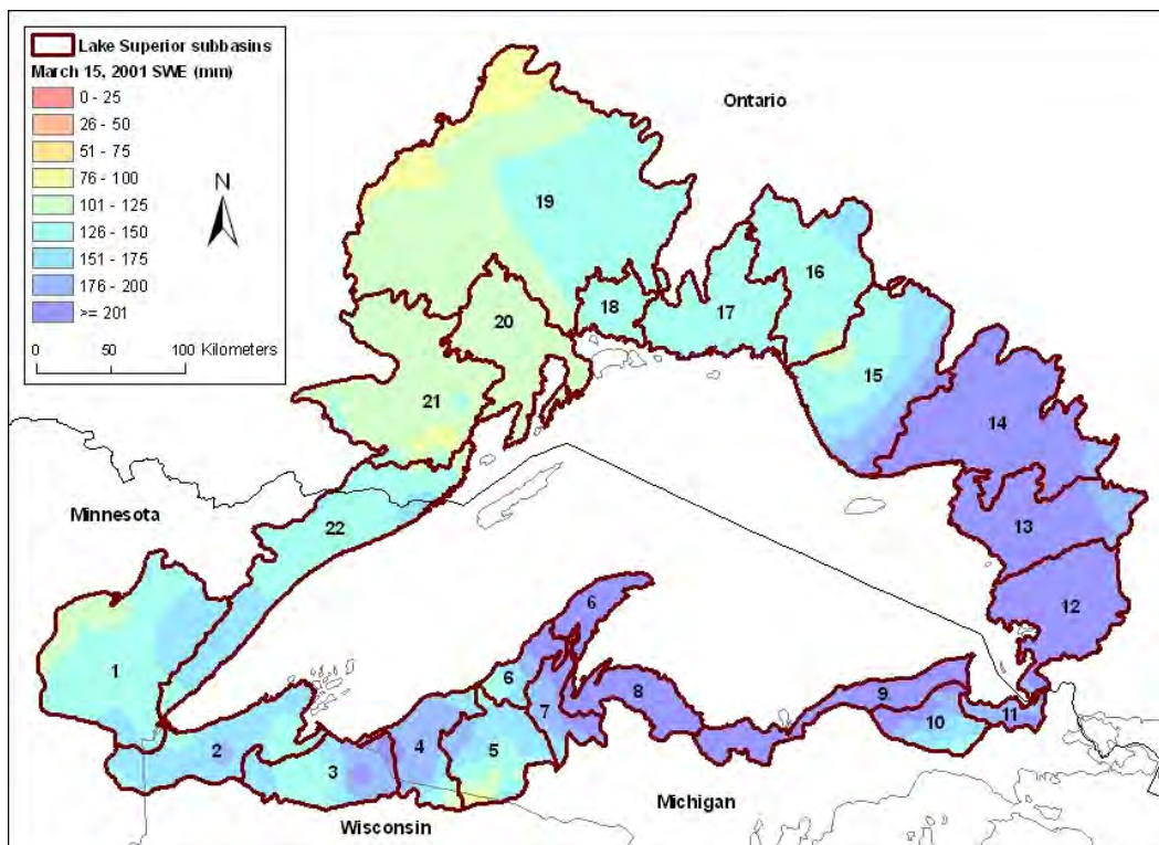
Figure 10. Map showing SWE grid that is clipped to the Lake Superior watershed for 15 March 2001.
