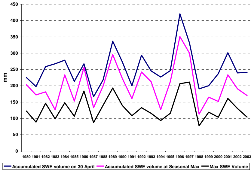
Figure 15. Maximum SWE volume, accumulated SWE volume on the day of the maximum SWE volume, and accumulated SWE volume on 30 April.
