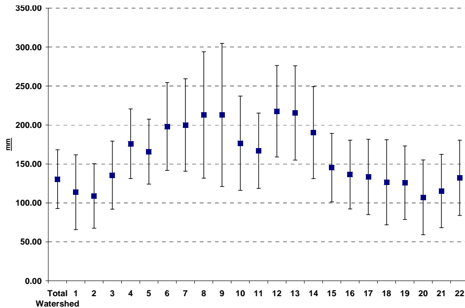
Figure 18. Average and standard deviation of the maximum volume of SWE for the total Lake Superior watershed and the 22 sub-basins.
