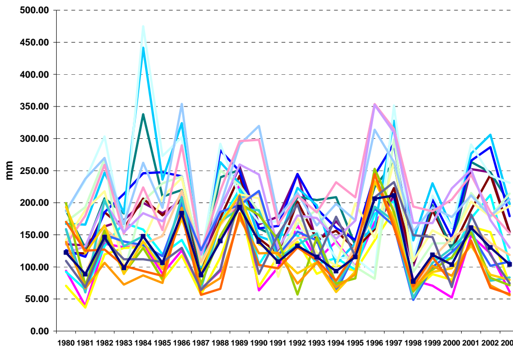
Figure 17. Maximum SWE volume in mm for all 22 Lake Superior sub-basins. The line with rectangular markers is for the entire Lake Superior watershed.
