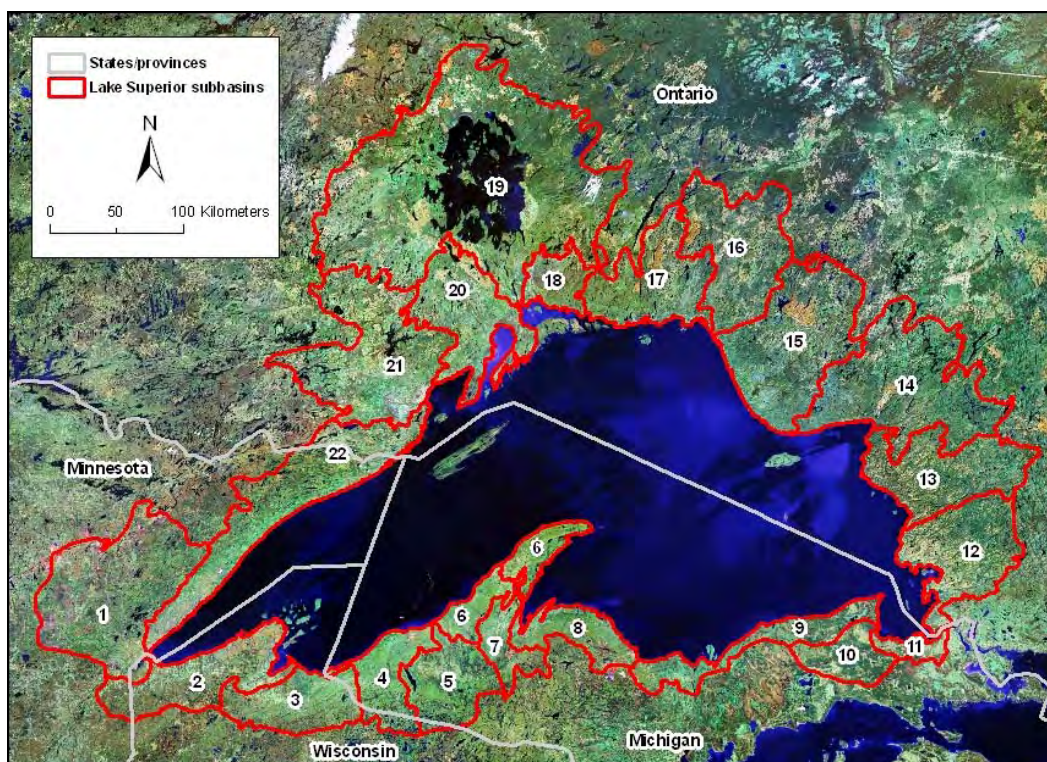
Figure 1. Lake Superior watershed.
