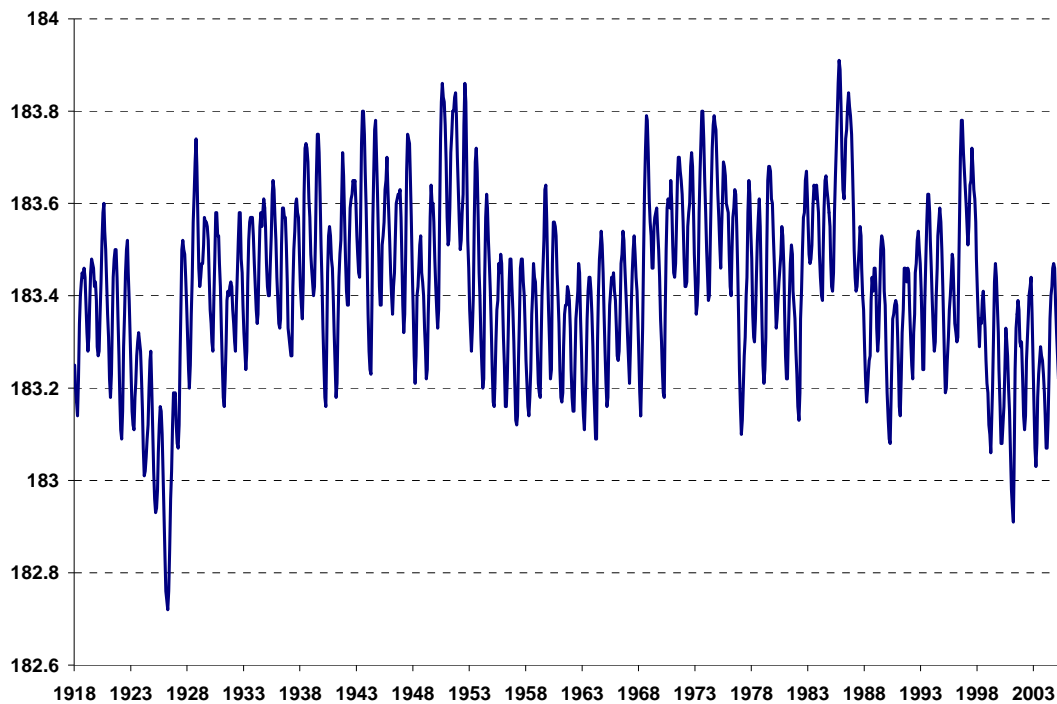
Figure 2. Lake Superior monthly water levels in meters from 1918 to 2005 (International Great Lakes Datum 1985).
