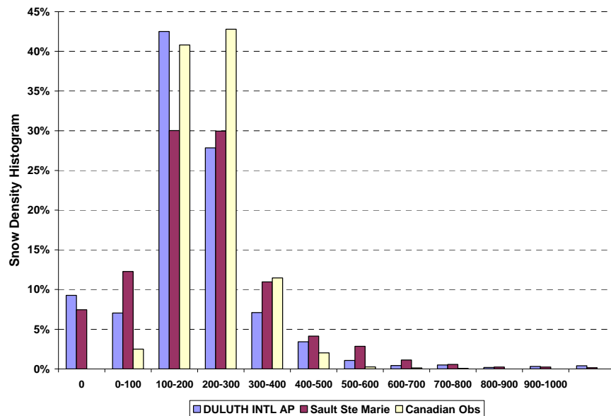
Figure 8. Snow density histogram ( \text{kg/m}^3 ) for Sault Ste Marie (Soo), MI; Duluth, MN; and in the Lake Superior watershed and vicinity in Ontario, Canada.
