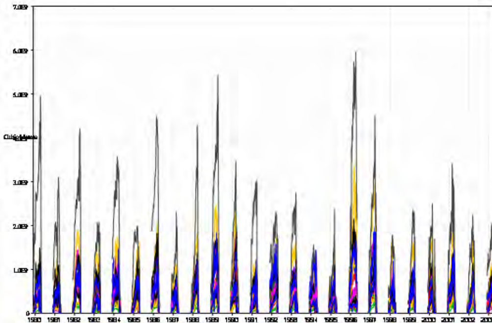
Figure 16. Daily SWE volume for the Lake Superior sub-basins.
