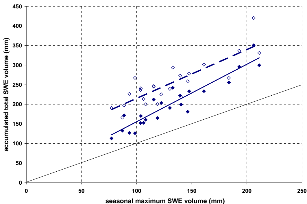
Figure 14. Accumulated SWE volume on the day of the maximum SWE volume (solid diamonds), and accumulated SWE volume on 30 April (open diamonds) plotted against the seasonal maximum SWE volume for each year.
