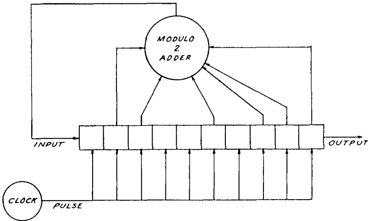
Figure 6. 10-Stage Shift Register with Feed Back Network
