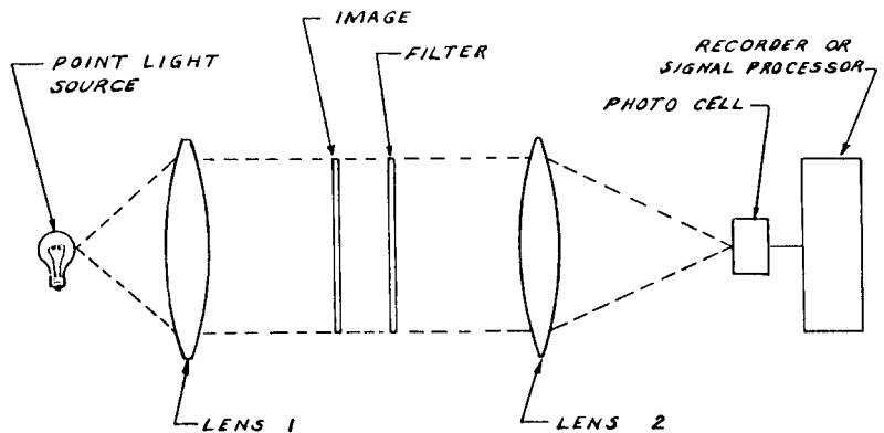
Figure 7. Optical Configuration of Spatial Spectral Image Analyzer.
