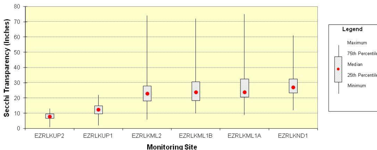
Figure 2-3. Box plot of Secchi depth transparencies measured in Zorinsky Lake during the 5-year period 2006 through 2010. (Note: monitoring sites are oriented on the x-axis in an upstream to downstream direction.)
