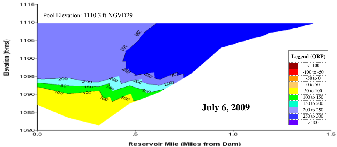
Plate 12. Longitudinal oxidation-reduction potential (ORP) contour plots of Zorinsky Lake based on depth-profile ORP levels (mV) measured from May to September 2009.
