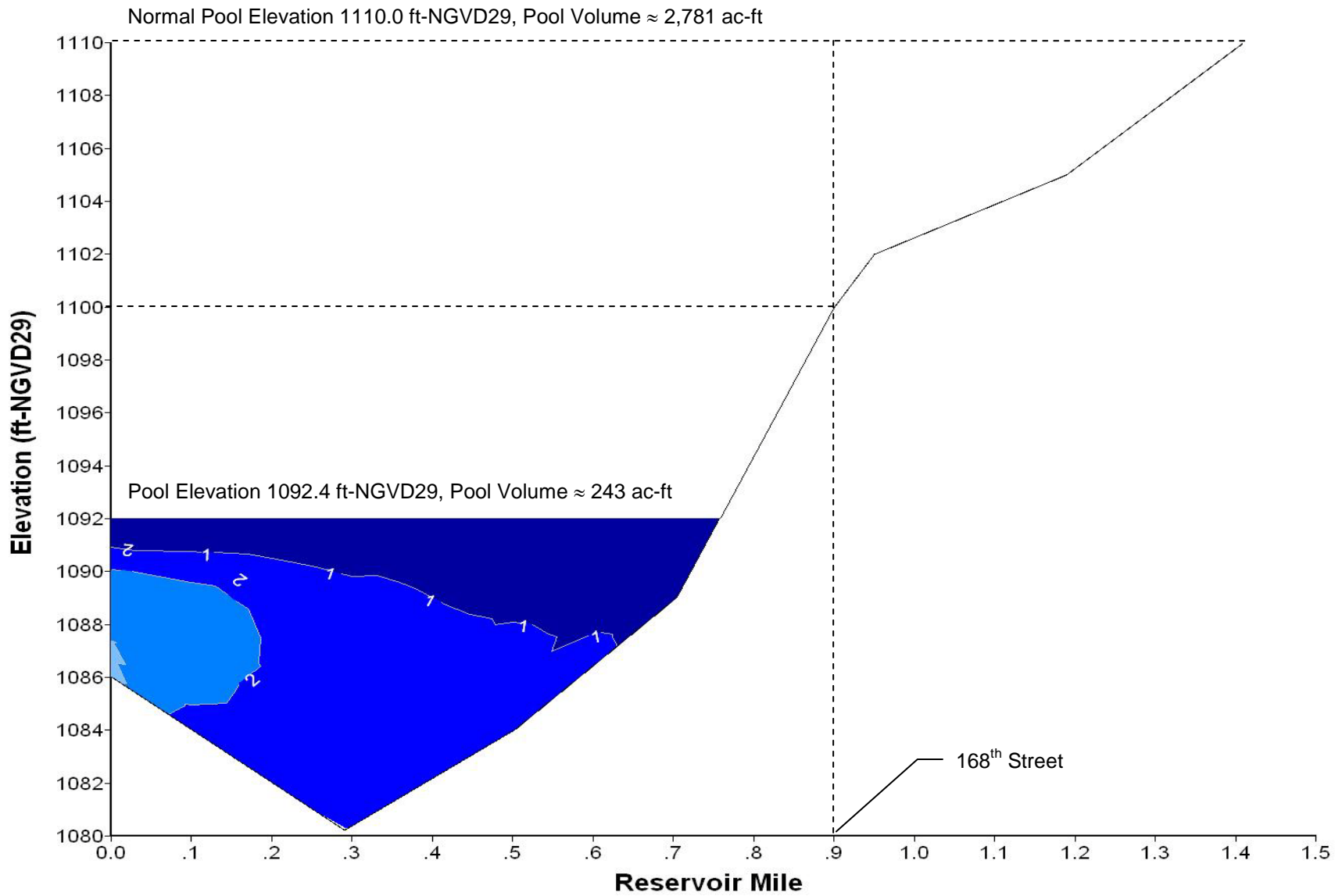
Plate 25. Longitudinal temperature (°C) contour plot of Zorinsky Lake based on depth profiles measured on 4-February 2011.
