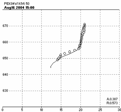
Plate 21. 2004 measured and simulated water temperature profiles at L4 (50 km from the dam) in the Missouri River arm.
