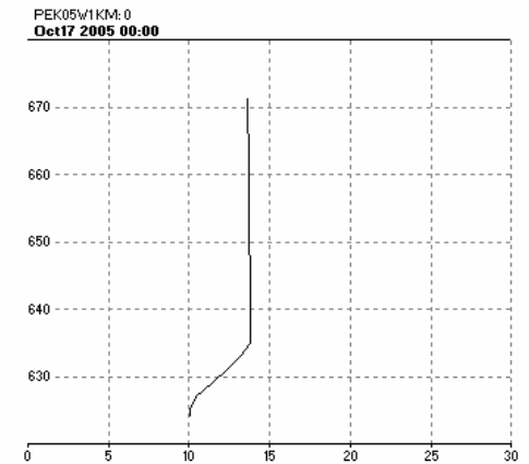
Plate 24. 2005 measured and simulated water temperature profiles at L1 (0 km from the dam) in the Missouri River arm.
