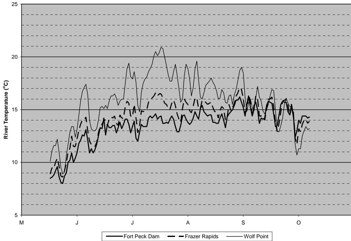
Figure 8. 2004 USGS measured temperature increases in the Missouri River from Fort Peck Dam to Wolf Point.
