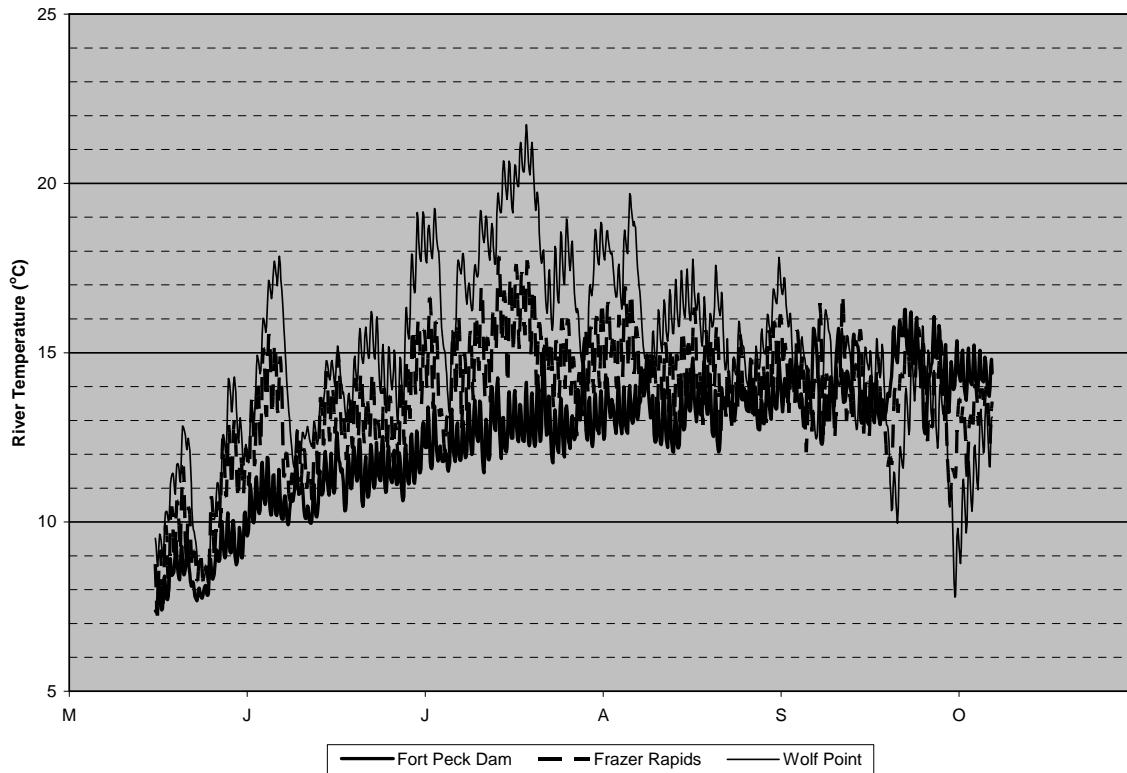
Figure 9. 2004 simulated temperature increases in the Missouri River from Fort Peck Dam to Wolf Point.
