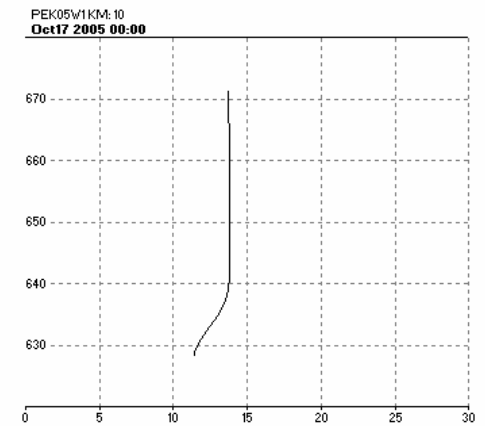
Plate 25. 2005 measured and simulated water temperature profiles at L2 (10 km from the dam) in the Missouri River arm.
