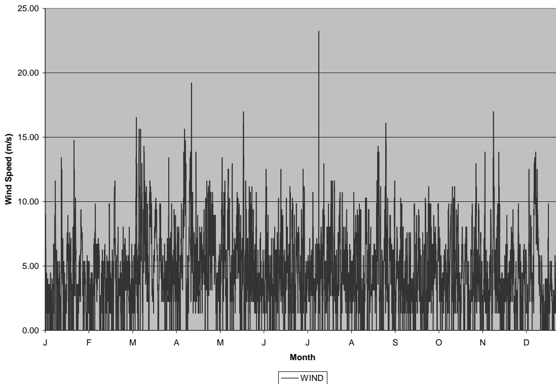
Plate 4. 2005 Glasgow International Airport (KGGW) hourly wind speed (m/s).
