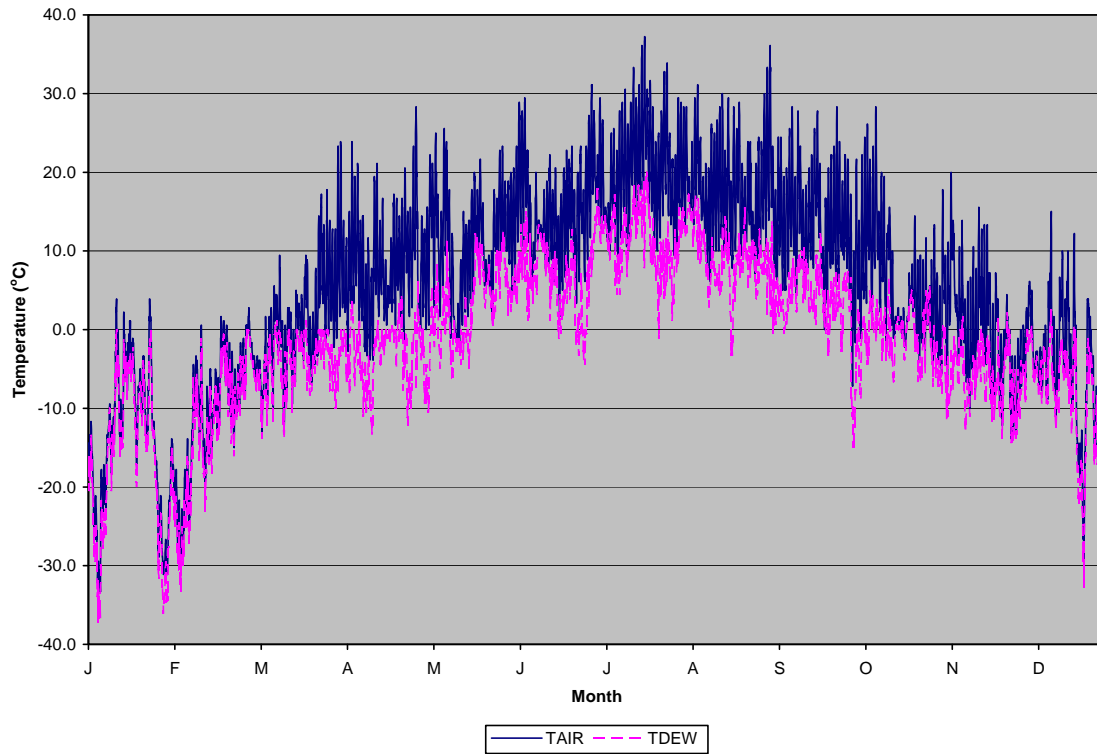
Plate 1. 2004 Glasgow International Airport (KGGW) hourly air and dew point temperature Celsius.
