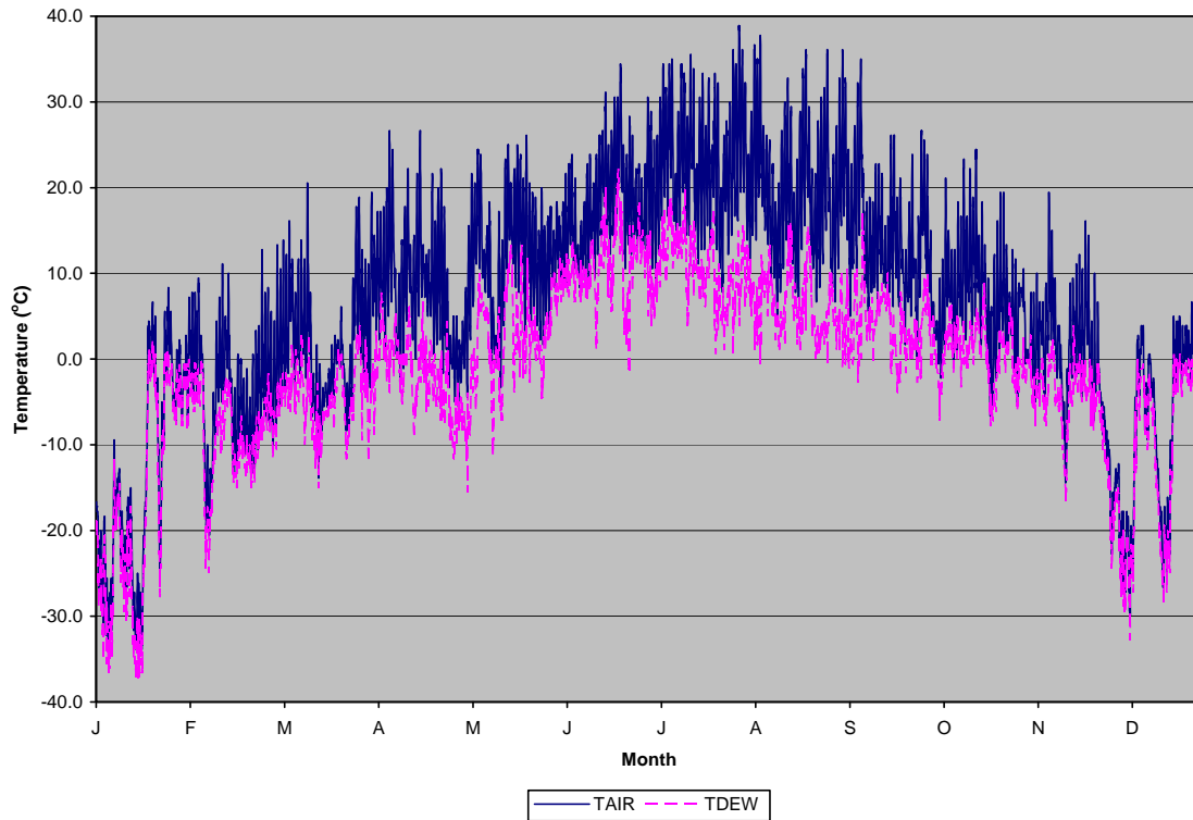
Plate 3. 2005 Glasgow International Airport (KGGW) hourly air and dew point temperature.
