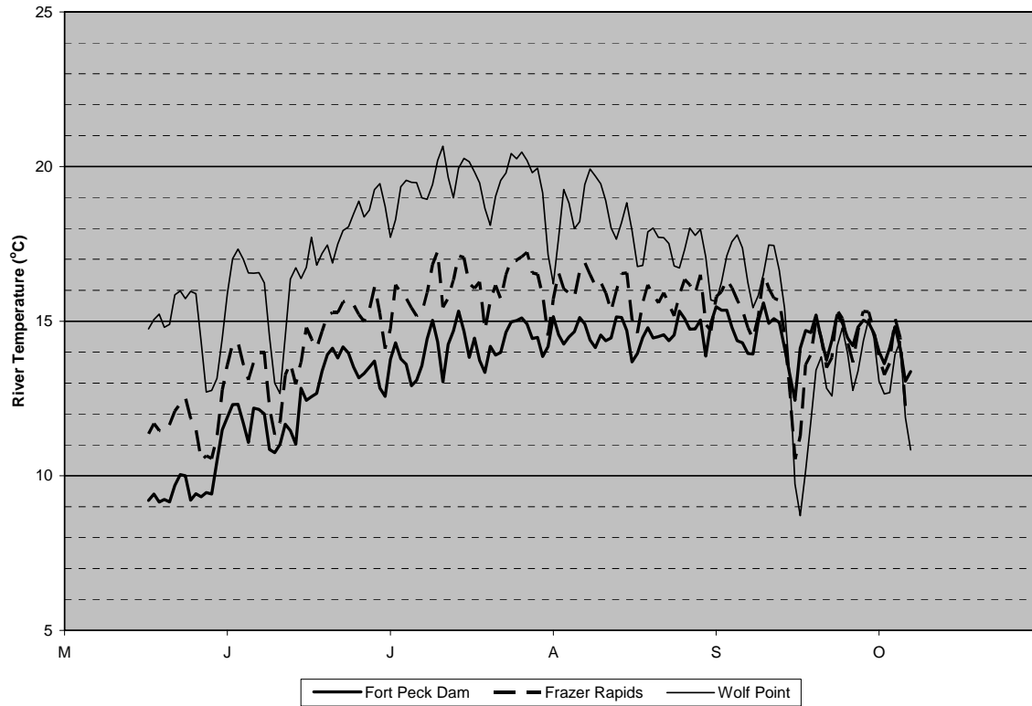
Figure 12. 2006 USGS measured temperature increases in the Missouri River from Fort Peck Dam to Wolf Point.
