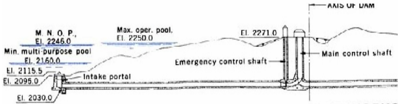
Figure 5. Fort Peck Lake outlet works schematic.
