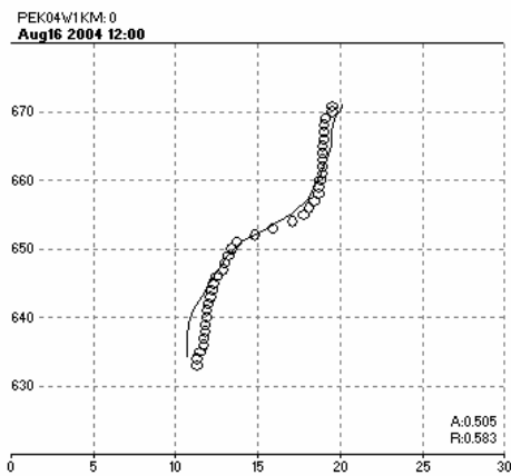
Plate 22. 2004 measured and simulated water temperature profiles at L5 in the Big Dry arm.
