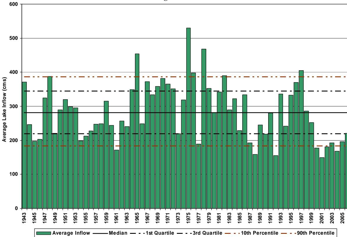
Plate 46. Fort Peck Lake average annual lake inflow and statistics.
