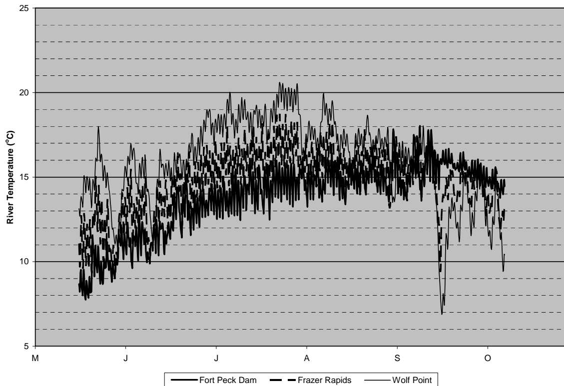
Figure 13. 2006 simulated temperature increases in the Missouri River from Fort Peck Dam to Wolf Point.
