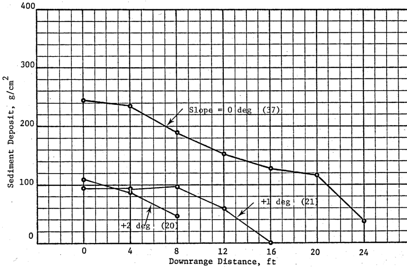
Figure B6. Sediment deposit profiles for positive slopes, 15-pcs slurry
