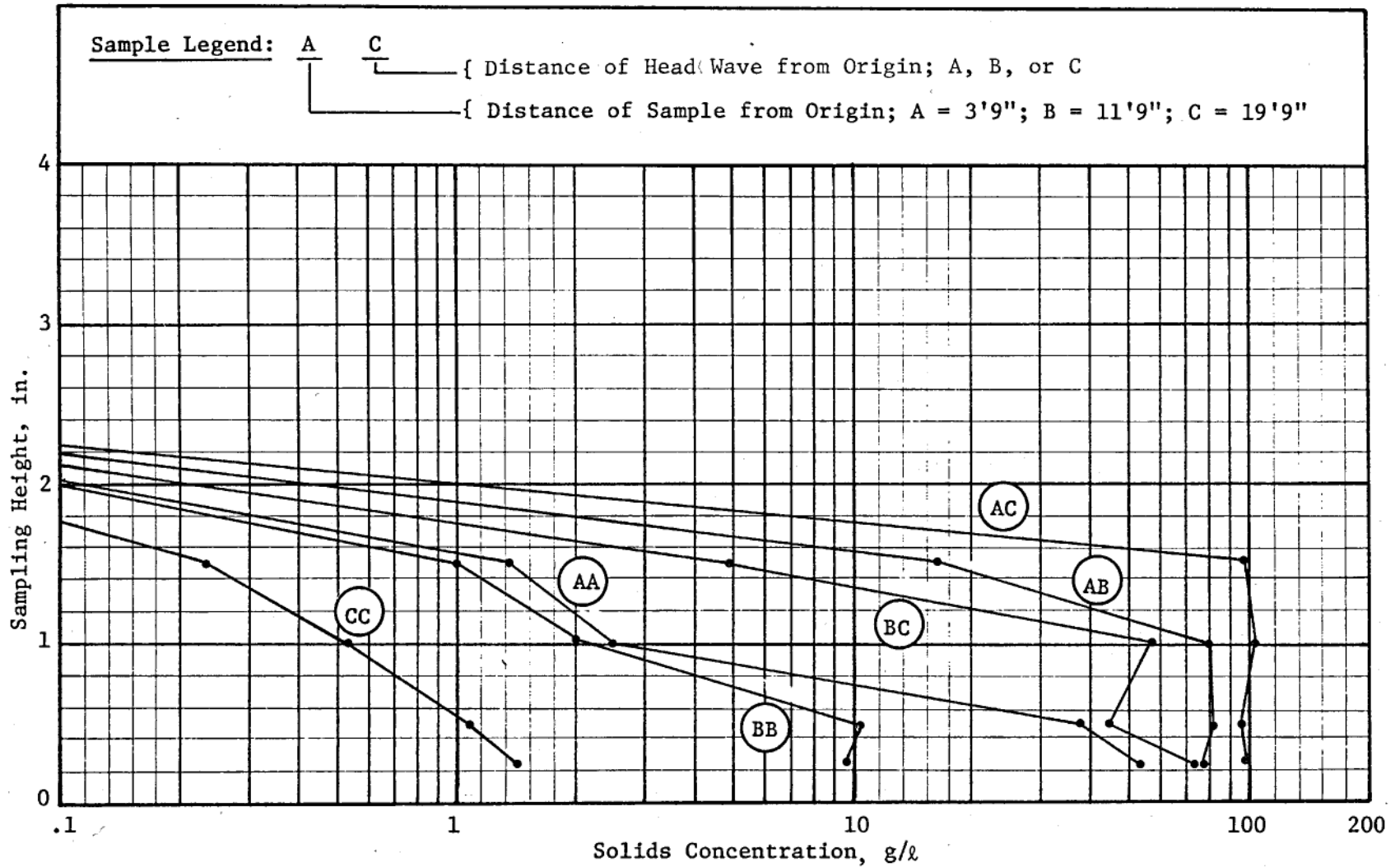
Figure C27. Concentration profiles for no waves, test 37
