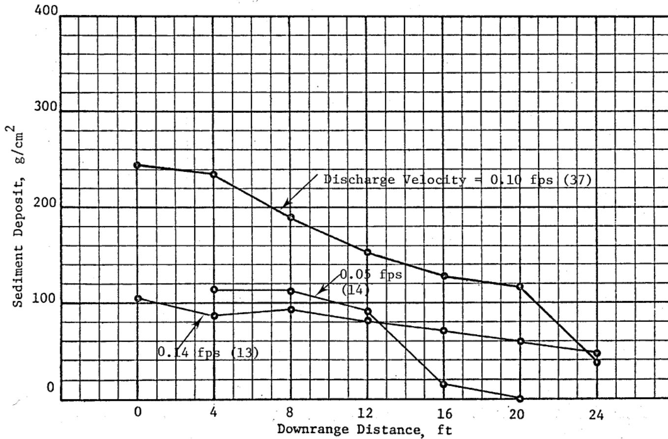
Figure B2. Sediment deposit profiles for discharge velocity tests
