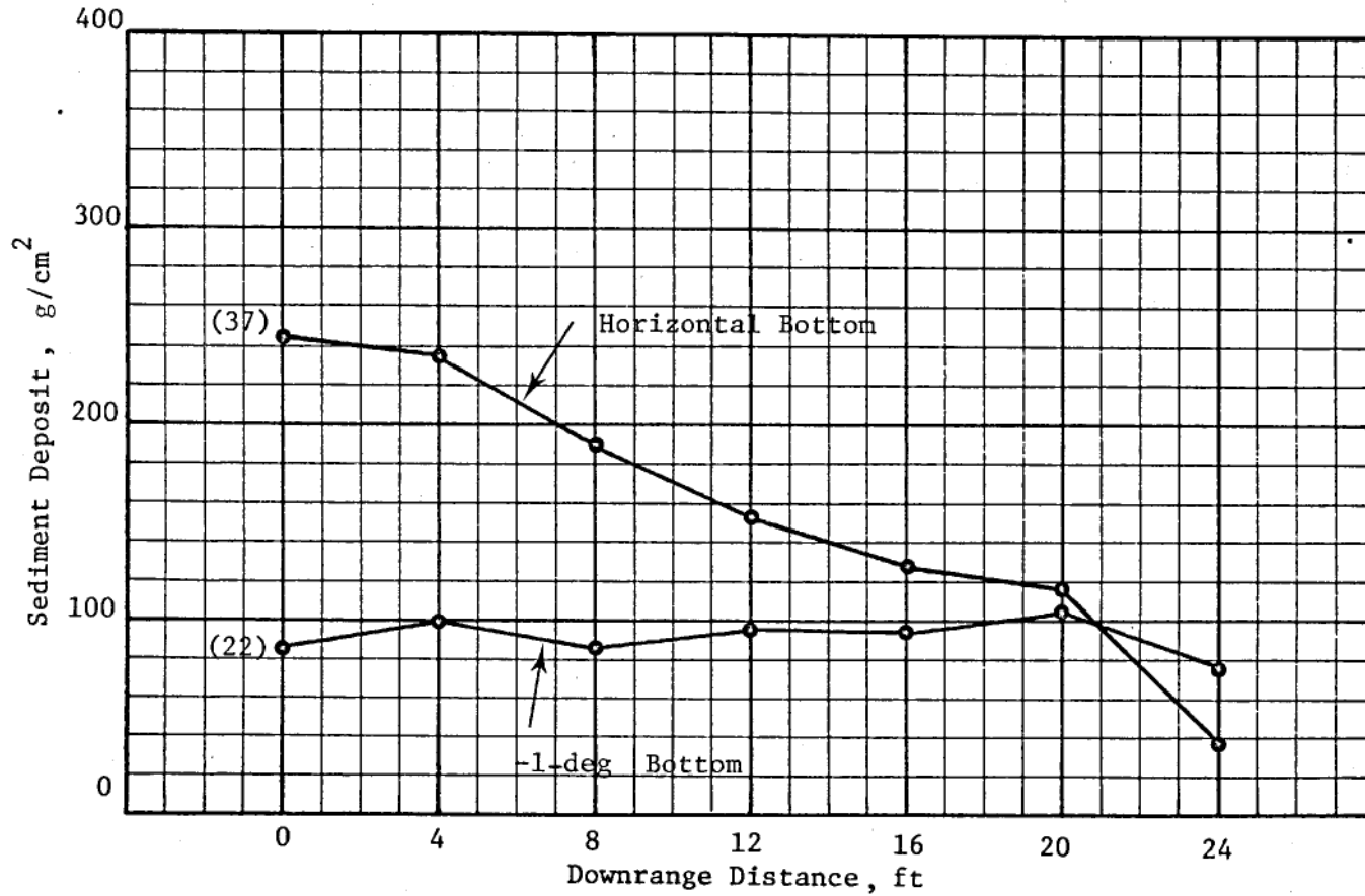
Figure 25. Sediment deposit profiles, tests 22 and 37
