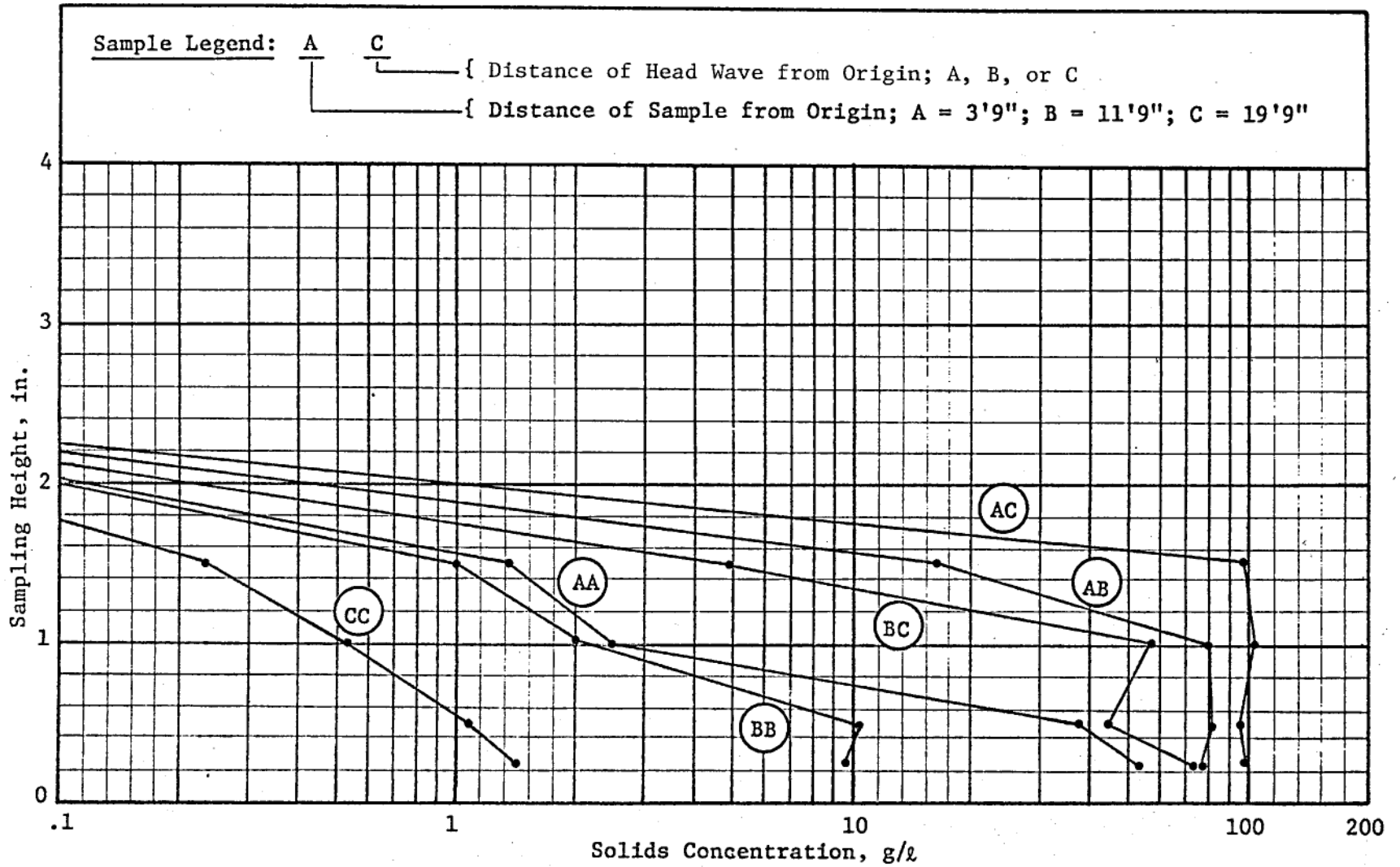
Figure C8. Concentration profiles for salt water, test 37
