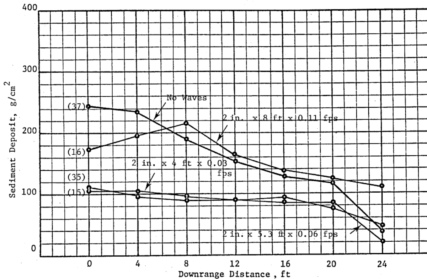
Figure B11. Sediment deposit profiles for wave conditions
