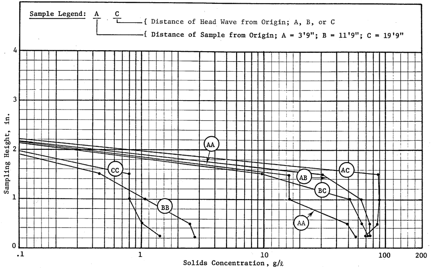
Figure C28. Concentration profiles for 2-in.-high by 4-ft-long waves, test 15
