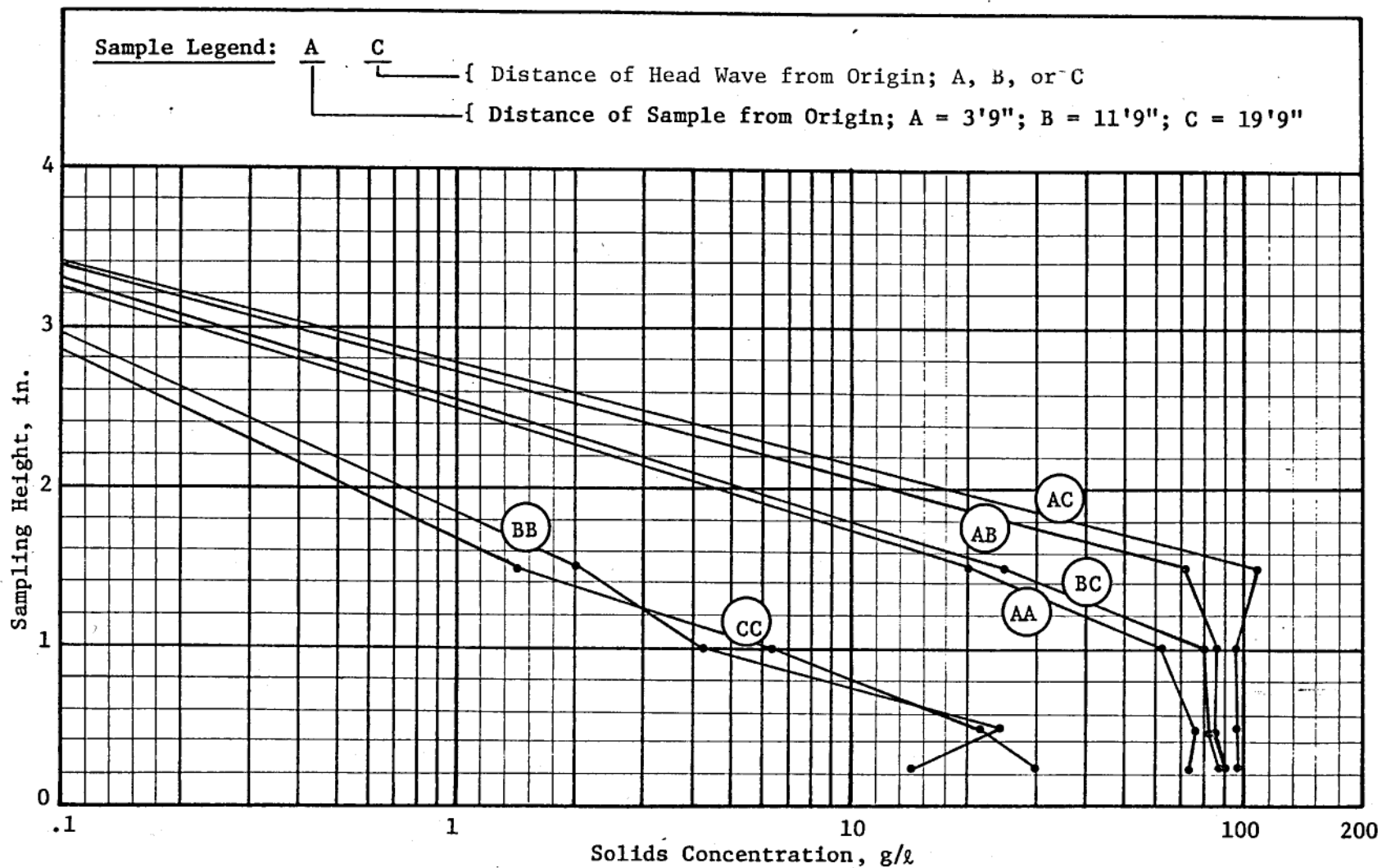
Figure C30. Concentration profiles for 2-in.-high by 8-ft-long waves, test 16
