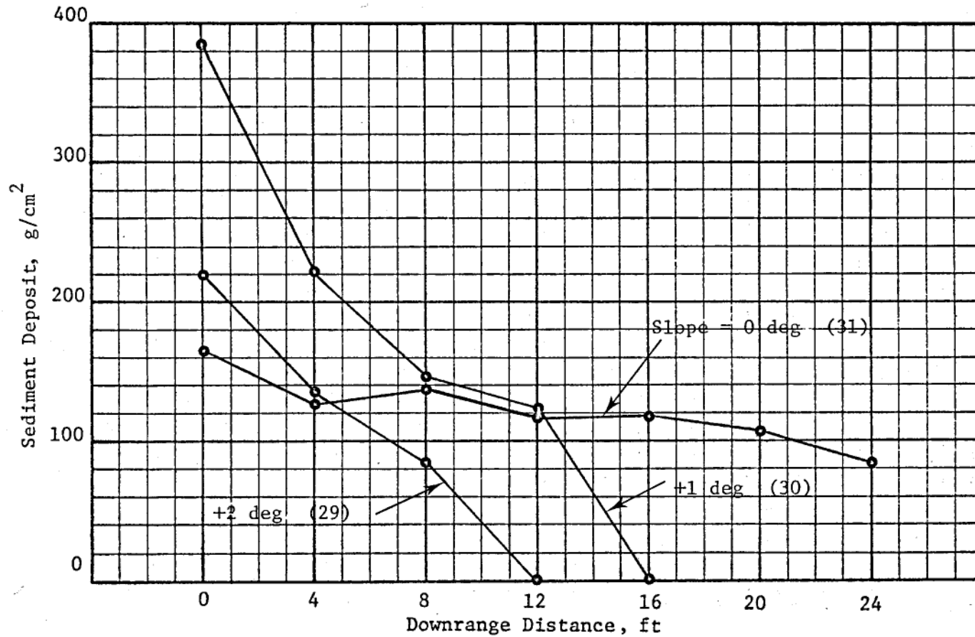
Figure B4. Sediment deposit profiles for positive slopes, 10-pcs slurry
