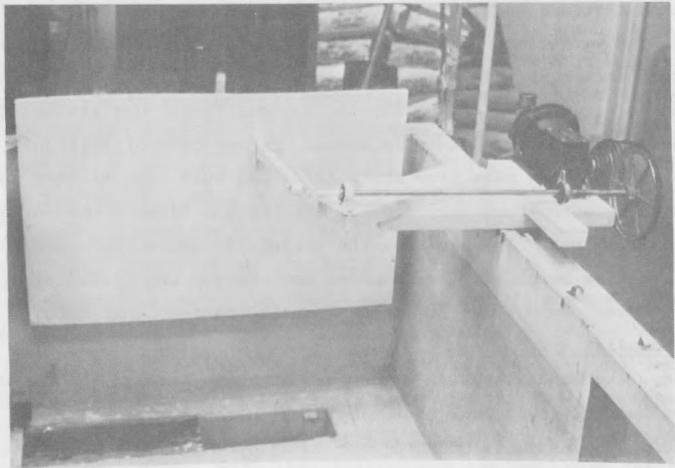
Figure 15. Wave machine
