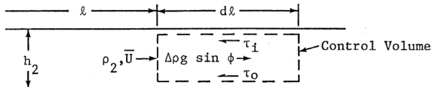
Figure 21. Control volume around bottom layer
