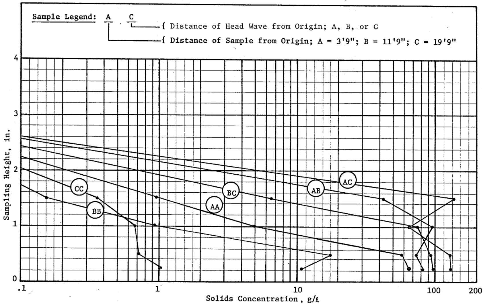
Figure C21. Concentration profiles for 20-pcs slurry, 0-deg slope, test 37
