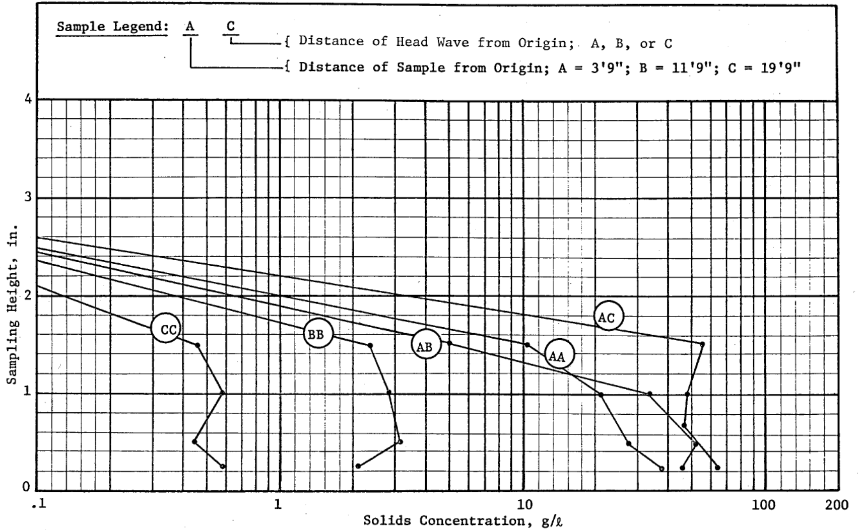
Figure C4. Concentration profiles for .05-fps discharge velocity, test 14
