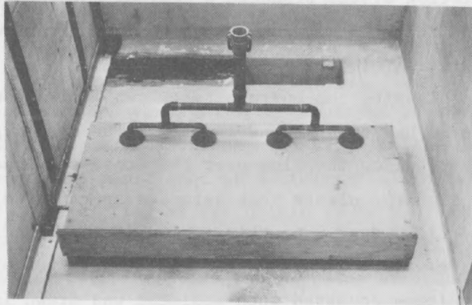
Figure 13. Mud flow generator box
