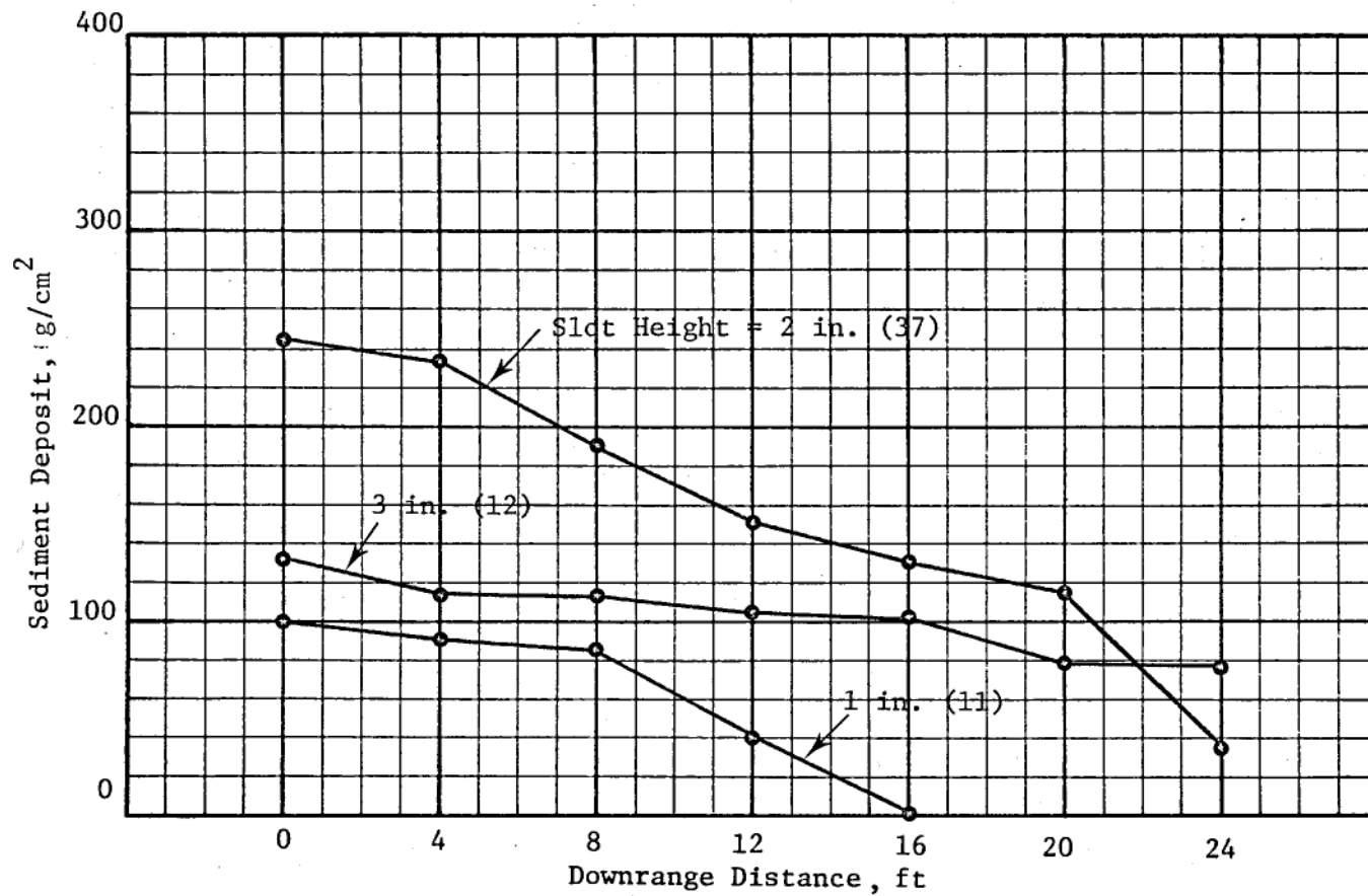
Figure B1. Sediment deposit profiles for slot height tests
