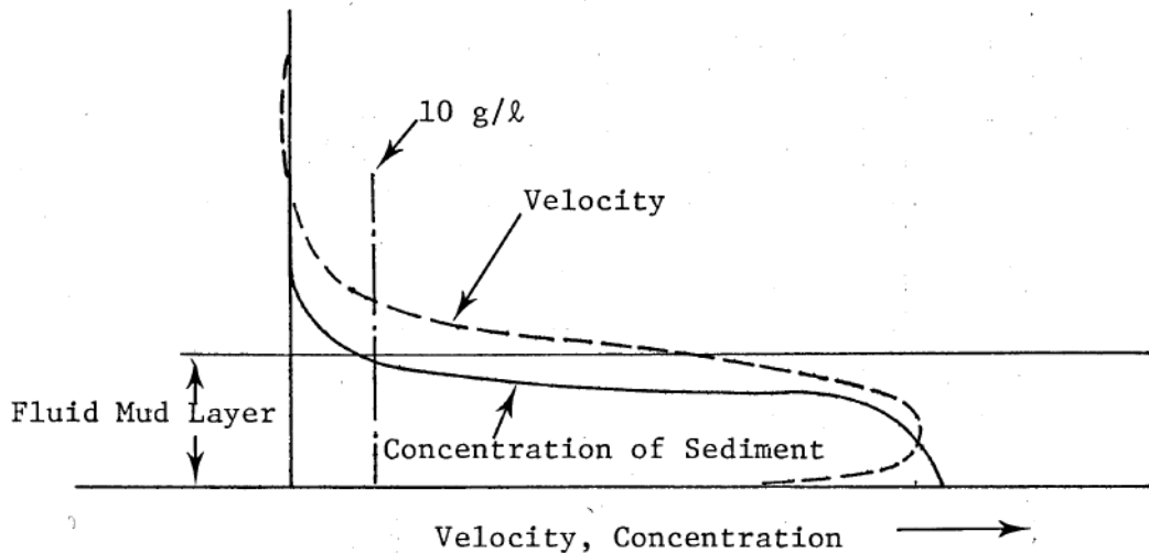
Figure 26. Generalized concentration and velocity profiles
