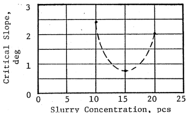
Figure 42. Critical slope versus slurry concentration
