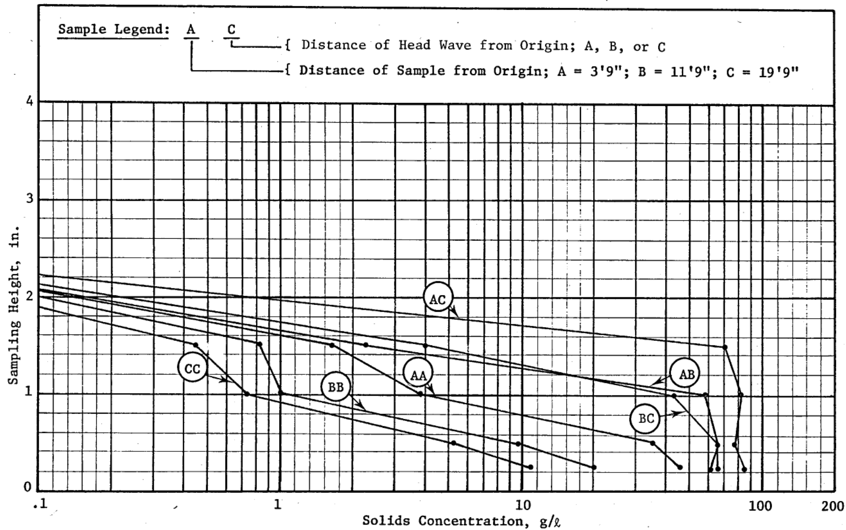
Figure C29. Concentration profiles for 2-in.-high by 5.3-ft-long waves, test 35
