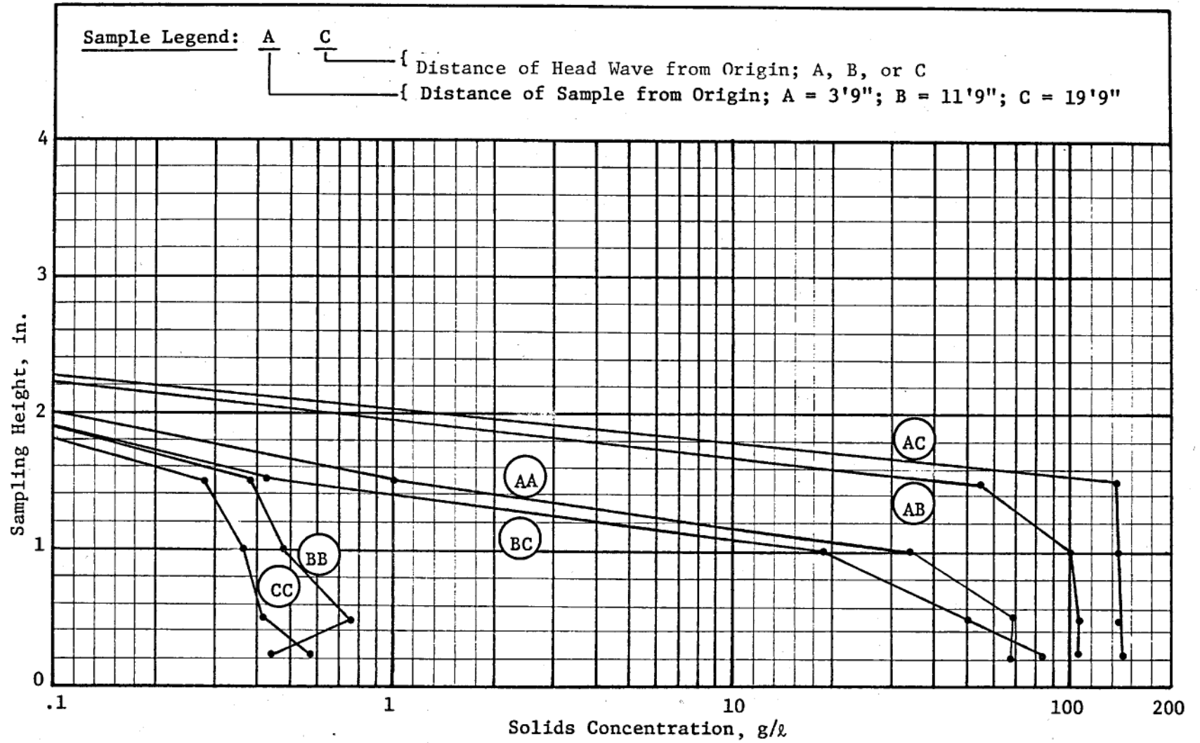
Figure C20. Concentration profiles for 20-pcs slurry, +1-deg slope, test 25
