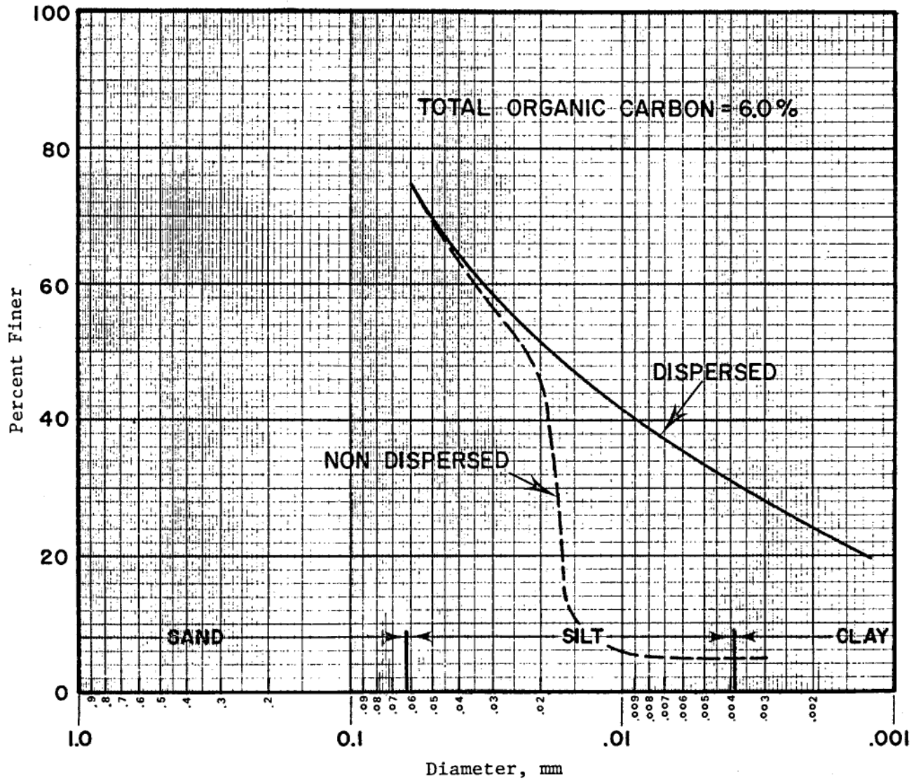
Figure 10. Grain-size distribution for saltwater (Boston Harbor) sediment
