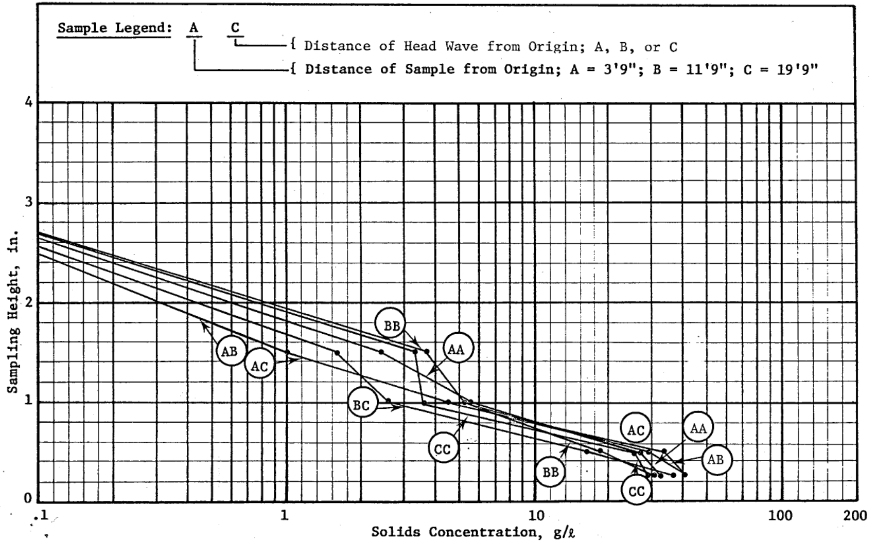
Figure C13. Concentration profiles for 10-pcs slurry, -2-deg slope, test 33
