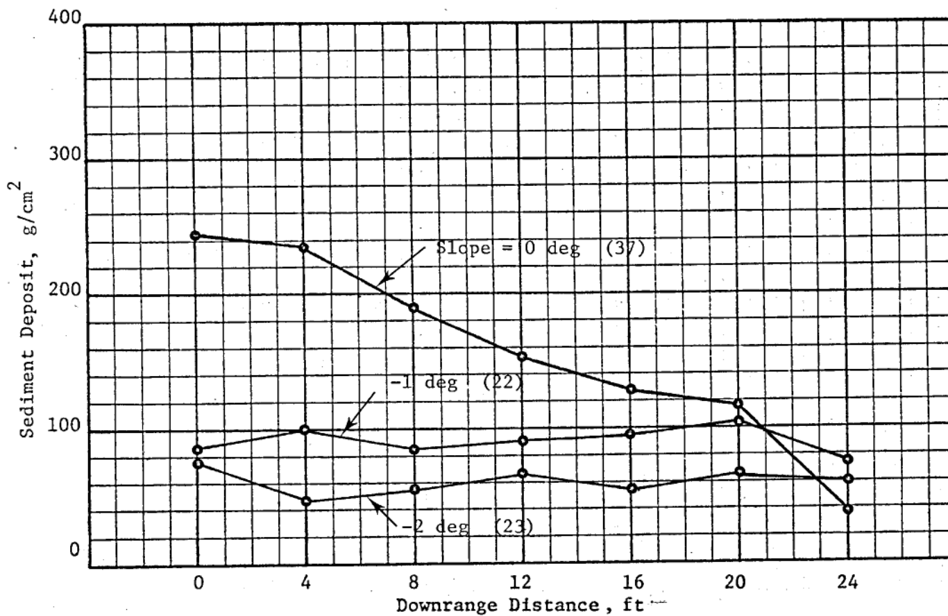
Figure B7. Sediment deposit profiles for negative slopes, 15-pcs slurry
