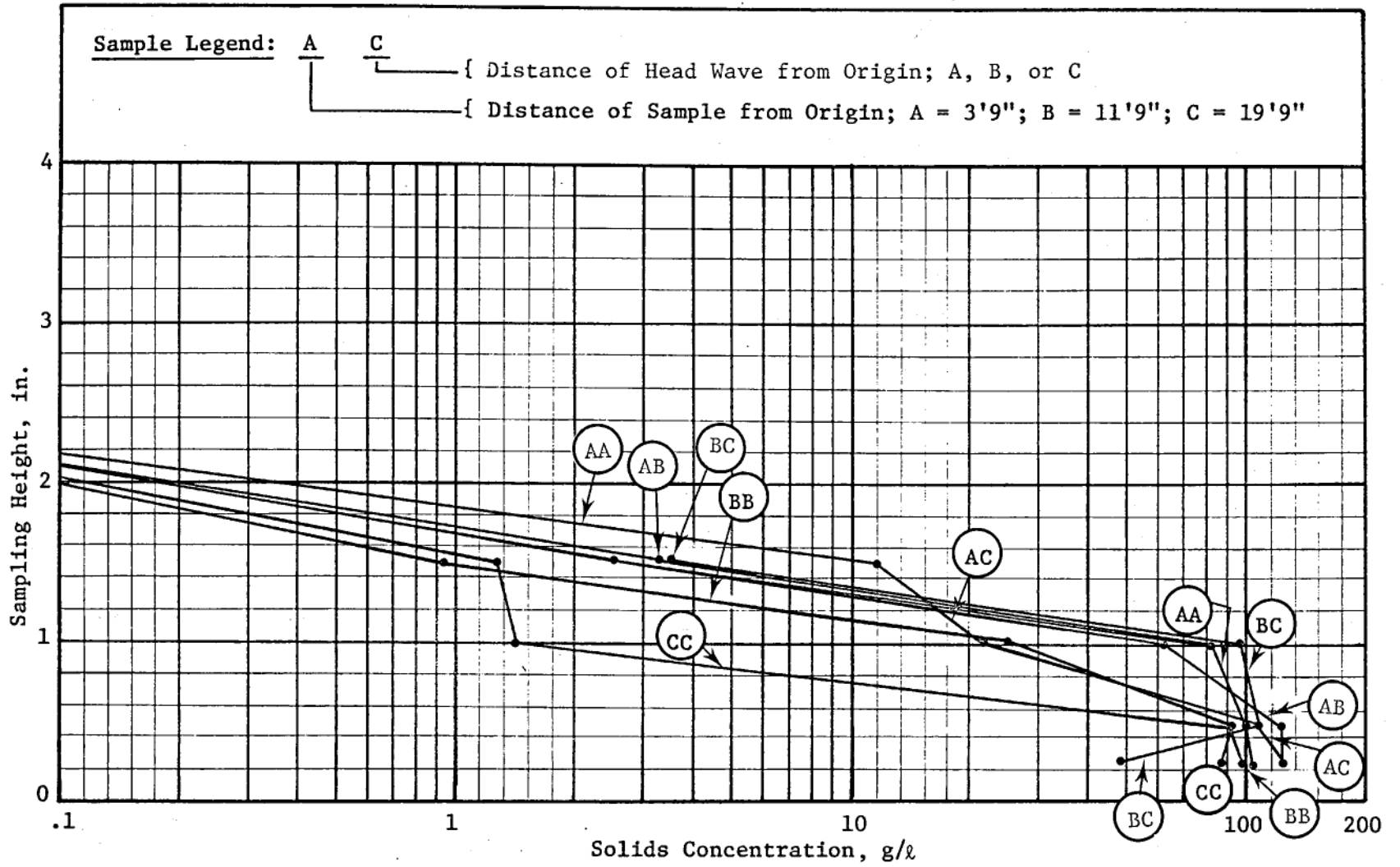
Figure C22. Concentration profiles for 20-pcs slurry, -1-deg slope, test 27
