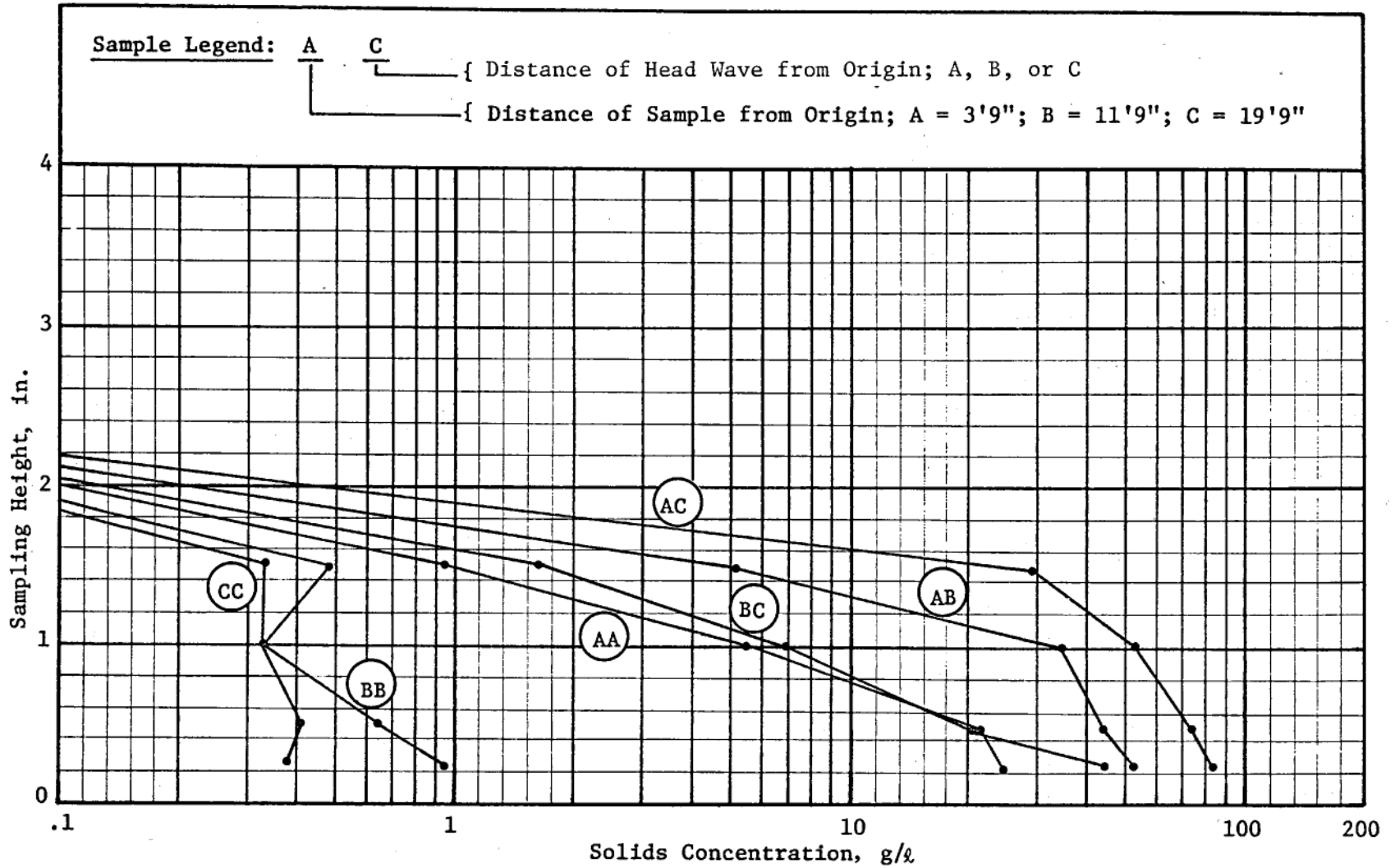
Figure C10. Concentration profiles for 10-pcs slurry, +1-deg slope, test 30
