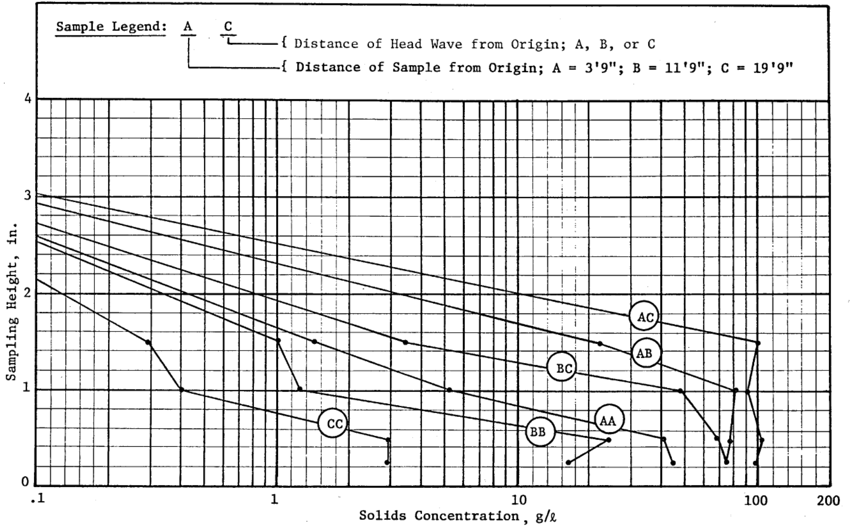
Figure C6. Concentration profiles for .14-fps discharge velocity, test 13
