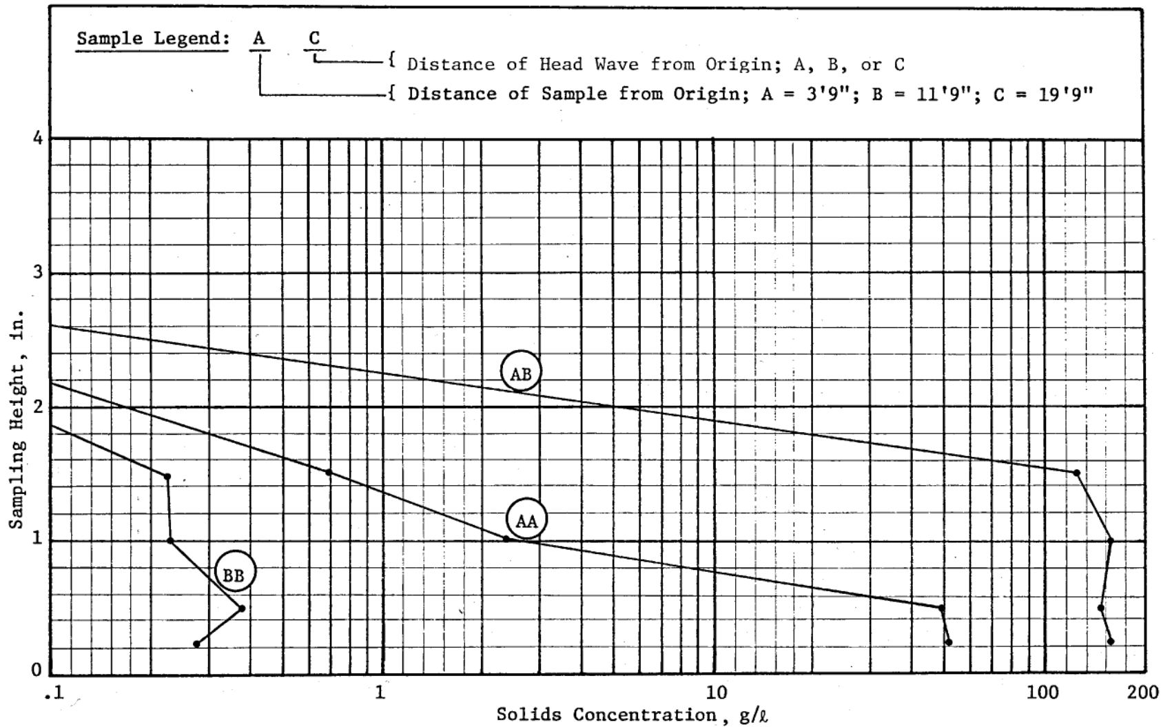
Figure C19. Concentration profiles for 20-pcs slurry, +2-deg slope, test 24
