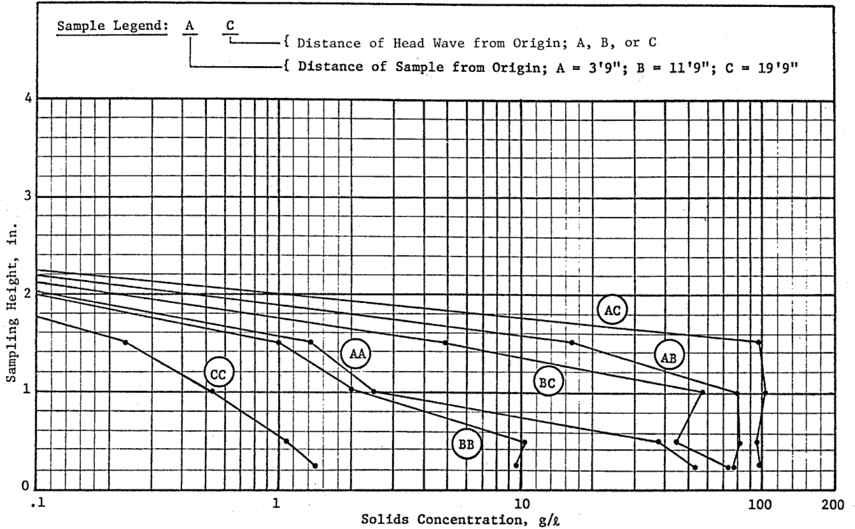
Figure C2. Concentration profiles for 2-in. slot height, test 37
