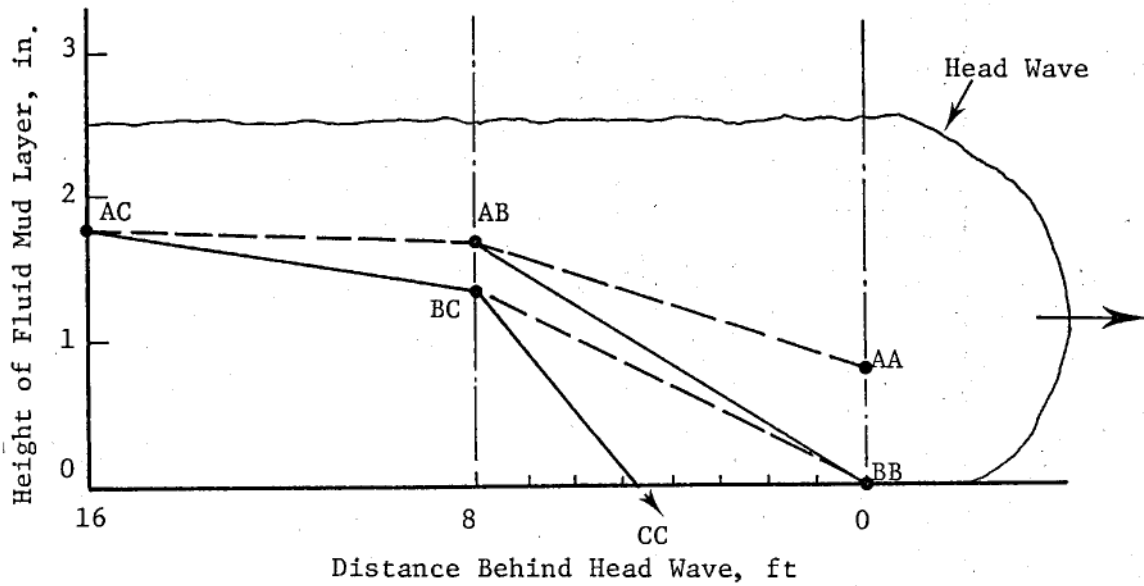
Figure 23. Fluid mud layer profiles, test 37
