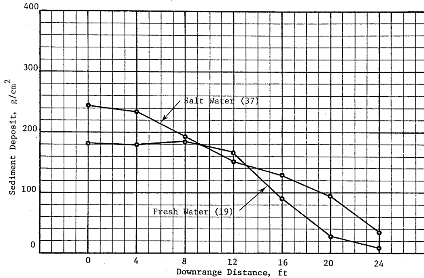
Figure B3. Sediment deposit profiles for sediment system tests
