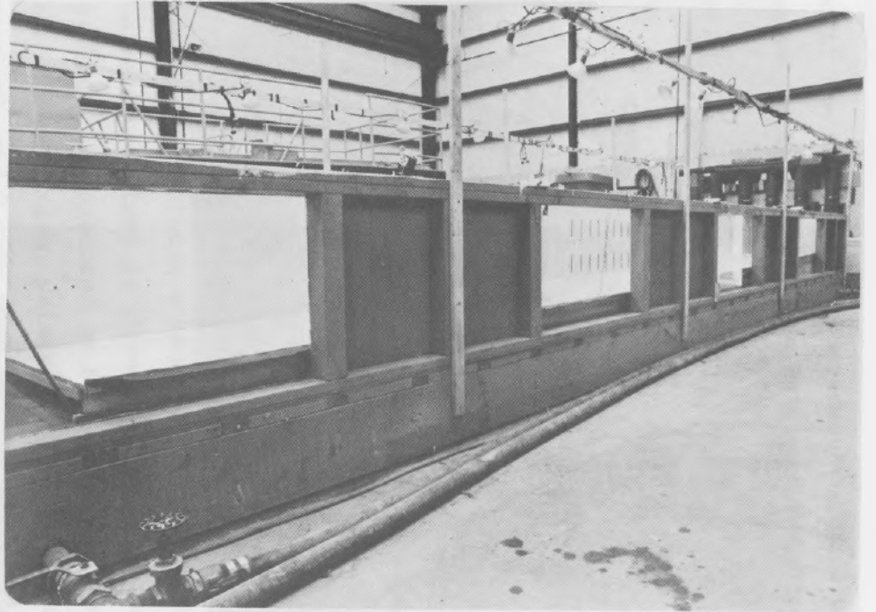
Figure 4. Test tank with sloped bottom
