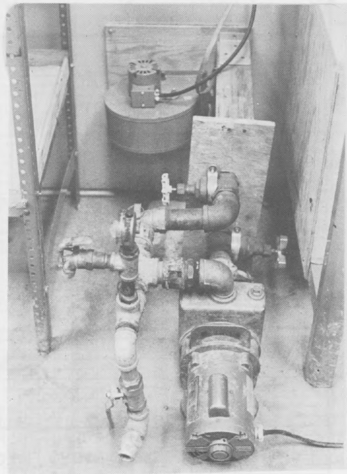
Figure 9. Slurry transfer pump and flow controls
