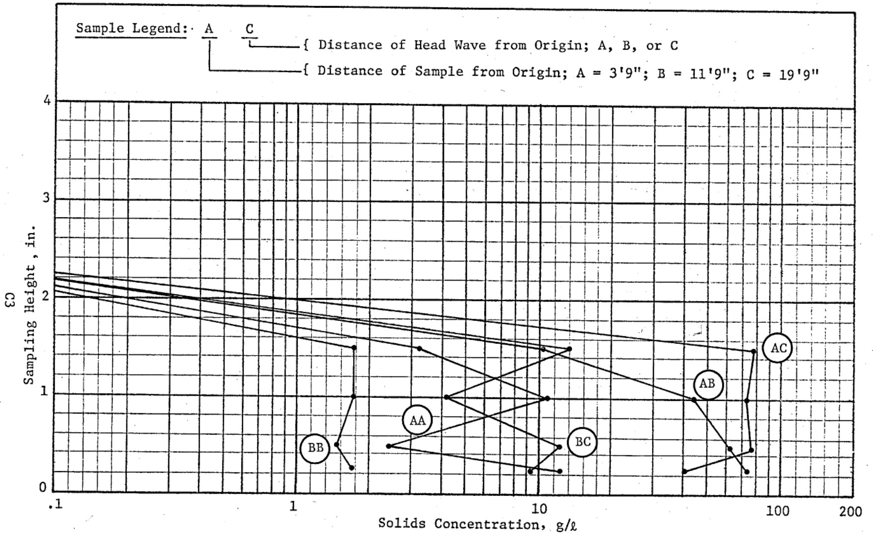
Figure C1. Concentration profiles for 1-in. slot height, test 11
