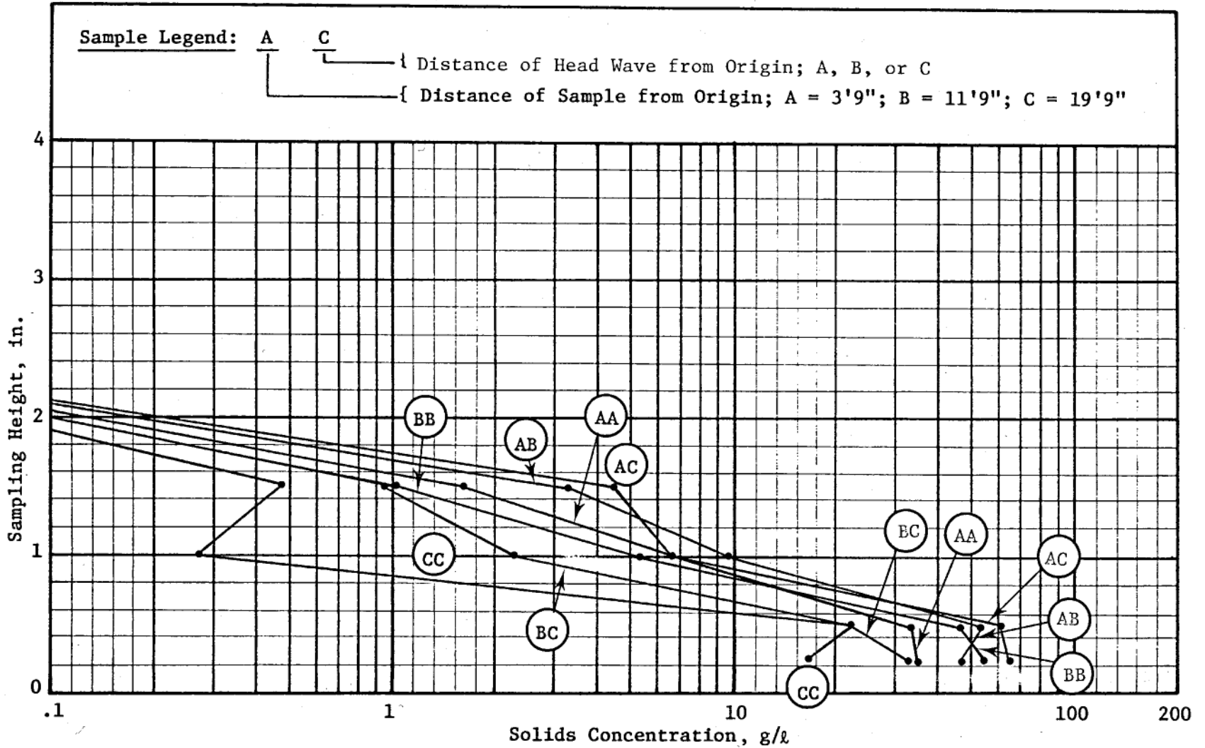
Figure C11. Concentration profiles for 10-pcs slurry, 0-deg slope, test 31
