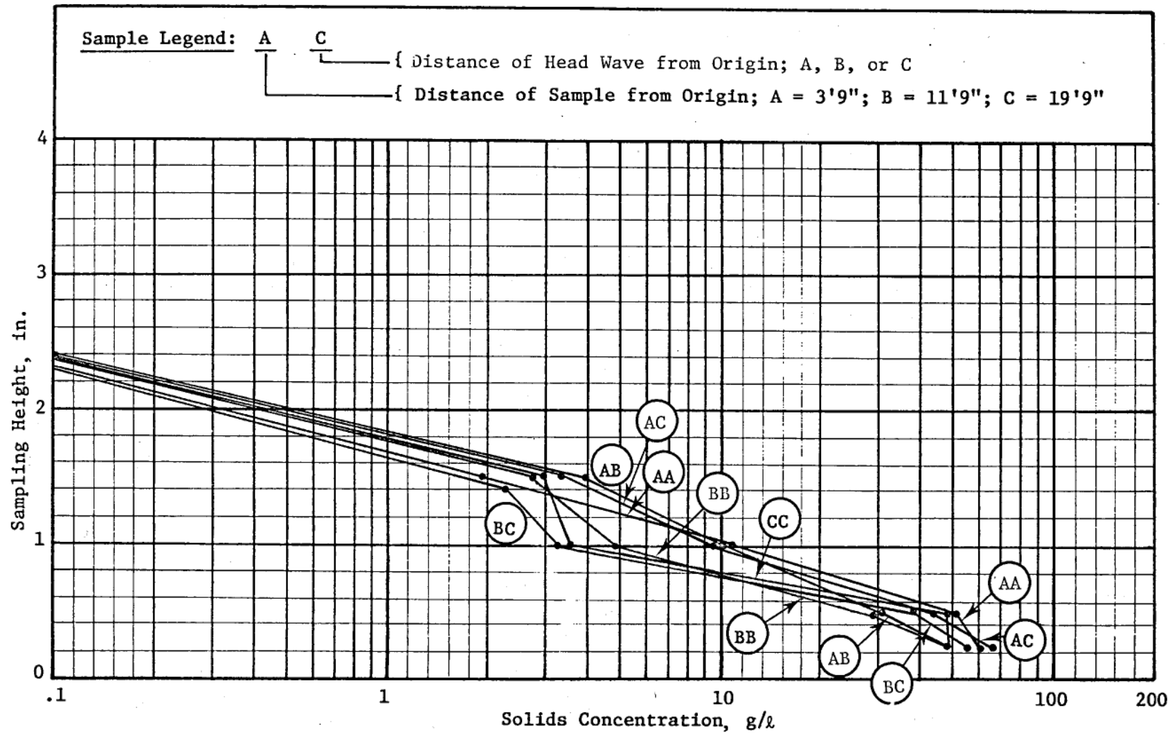
Figure C18. Concentration profiles for 15-pcs slurry, -2-deg slope, test 23
