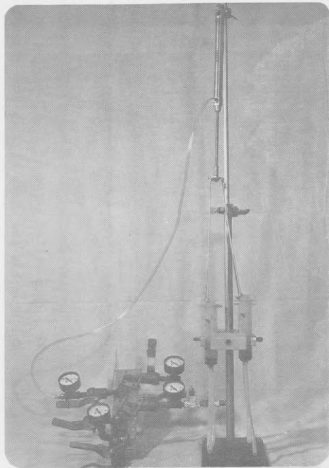
Figure 17. Water sampler assembly
