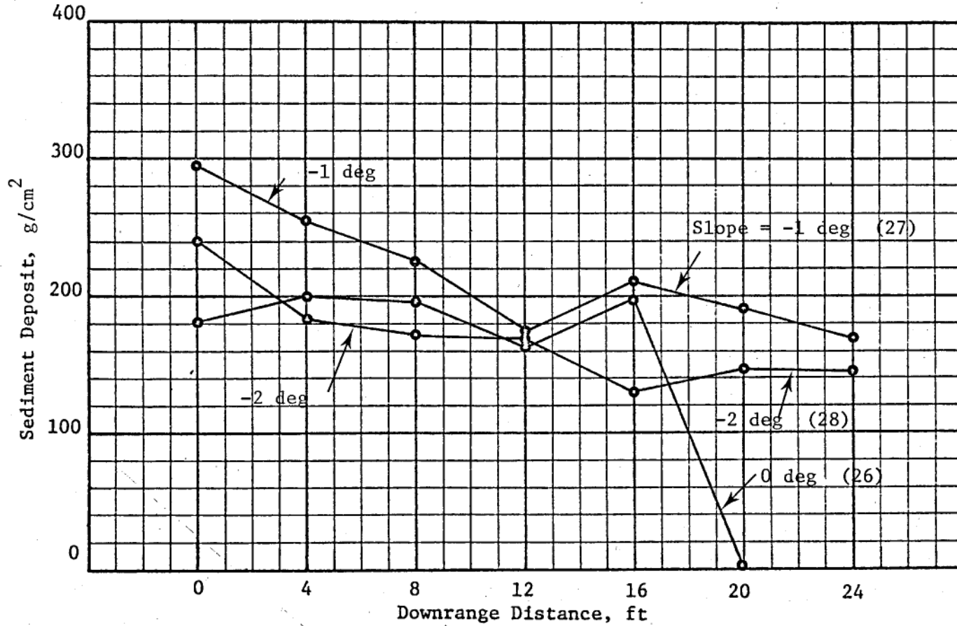
Figure B9. Sediment deposit profiles for negative slopes, 20-pcs slurry
