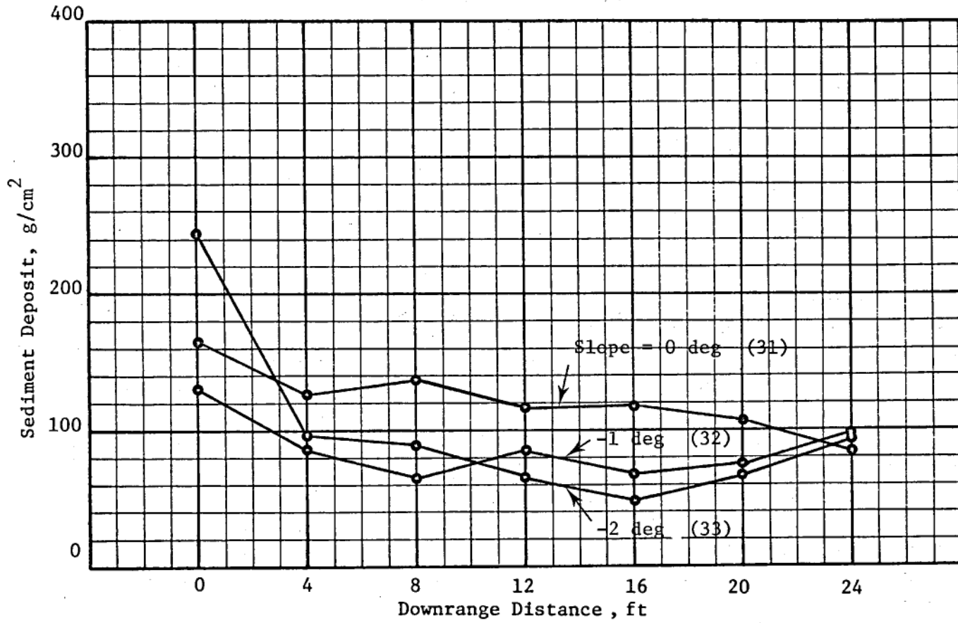
Figure B5. Sediment deposit profiles for negative slopes, 10-pcs slurry
