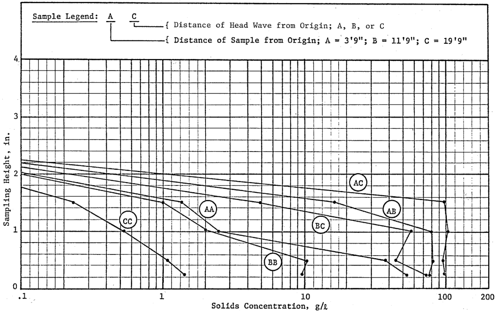
Figure C5. Concentration profiles for .10-fps discharge velocity, test 37
