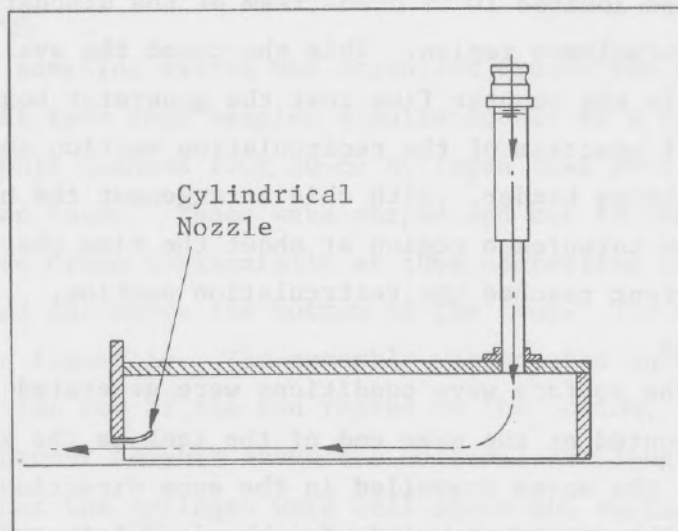
Figure 14. Section of mud flow generator box
