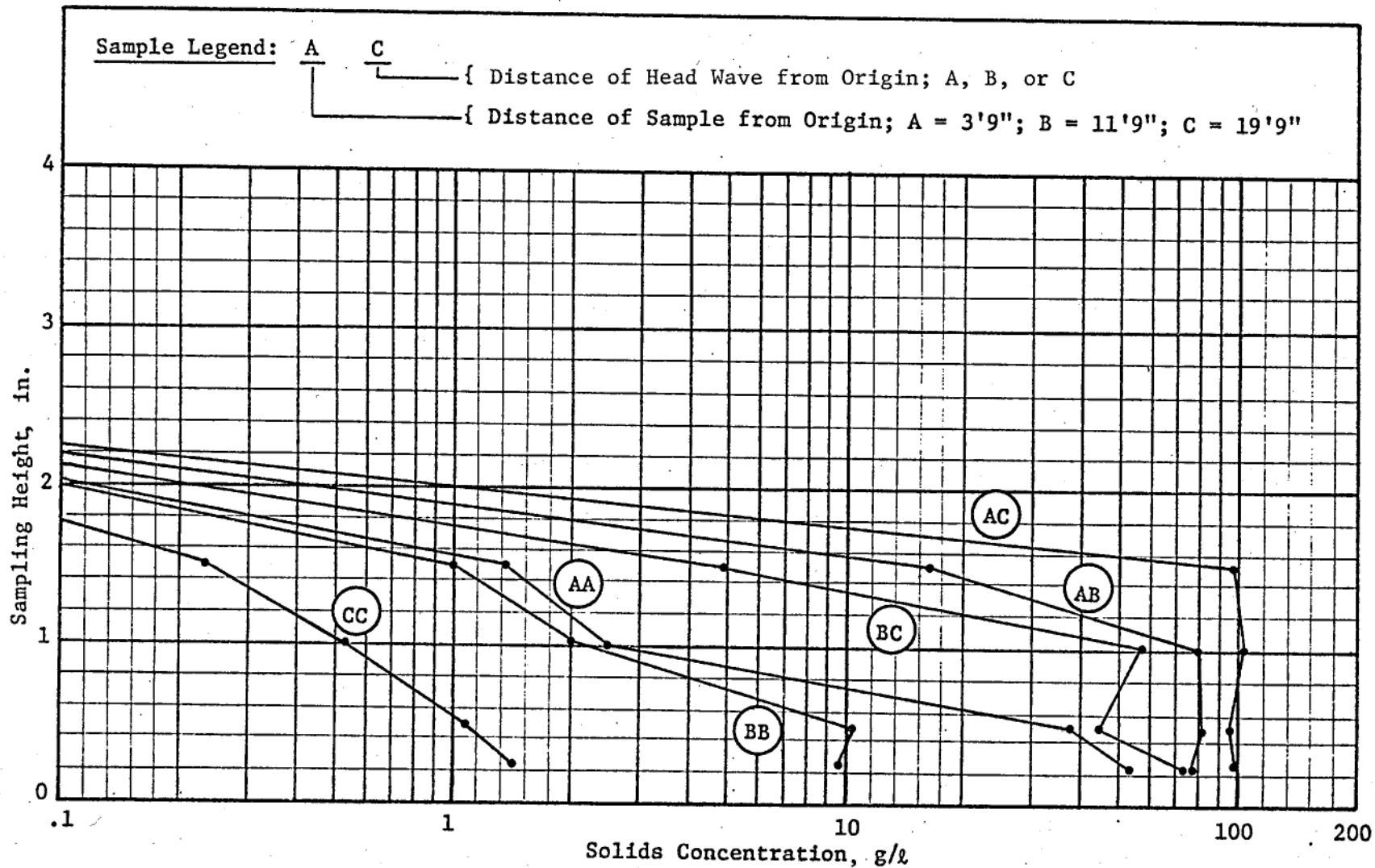
Figure C25. Concentration profiles for zero current, test 37
