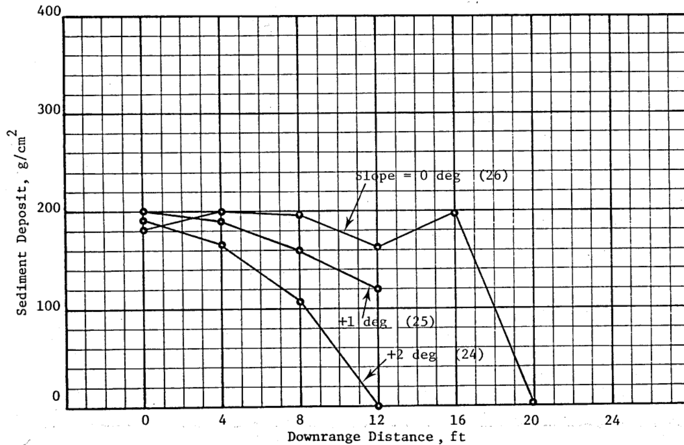
Figure B8. Sediment deposit profiles for positive slopes, 20-pcs slurry
