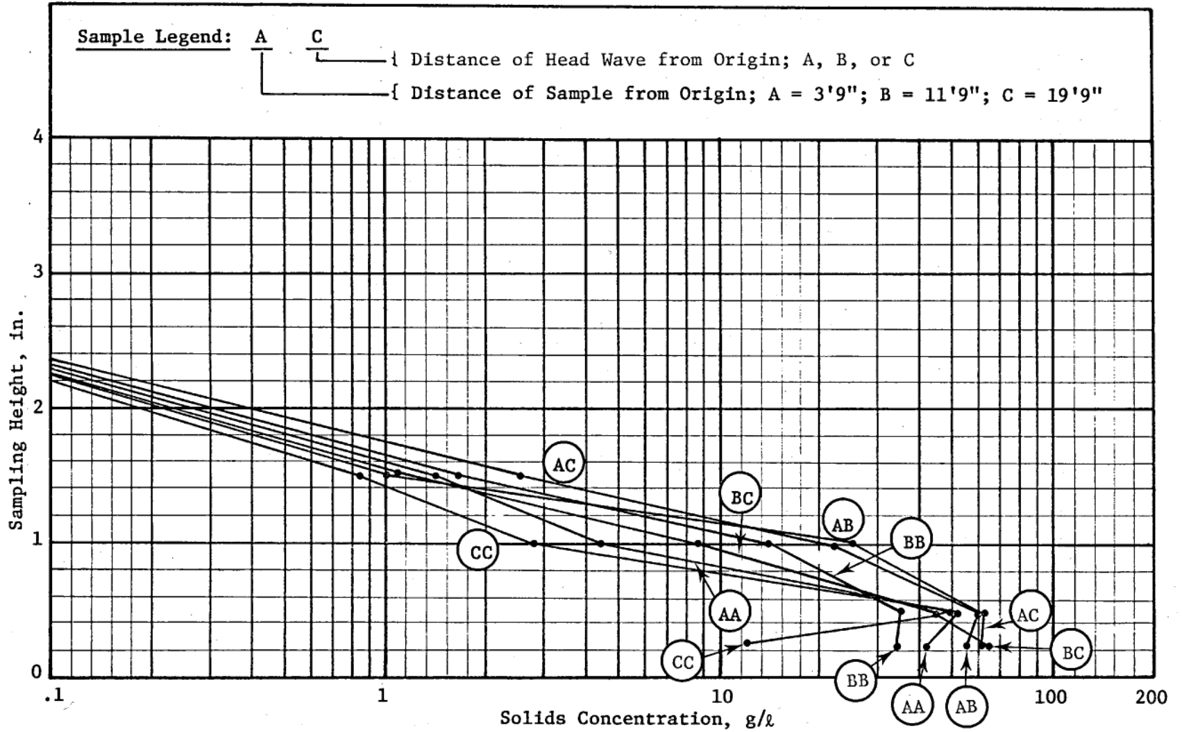
Figure C17. Concentration profiles for 15-pcs slurry, -1-deg slope, test 22
