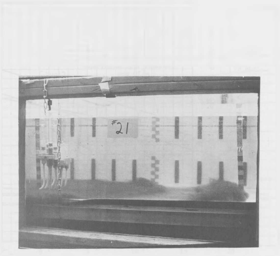
Figure 39. Separated head wave, +1-degree slope, test 21
