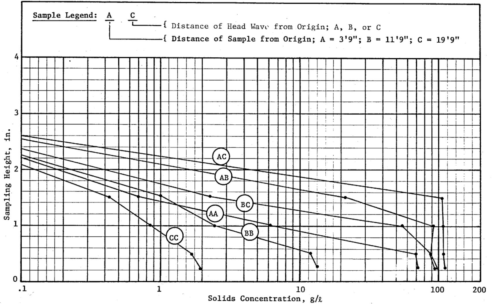
Figure C7. Concentration profiles for fresh water, test 19
