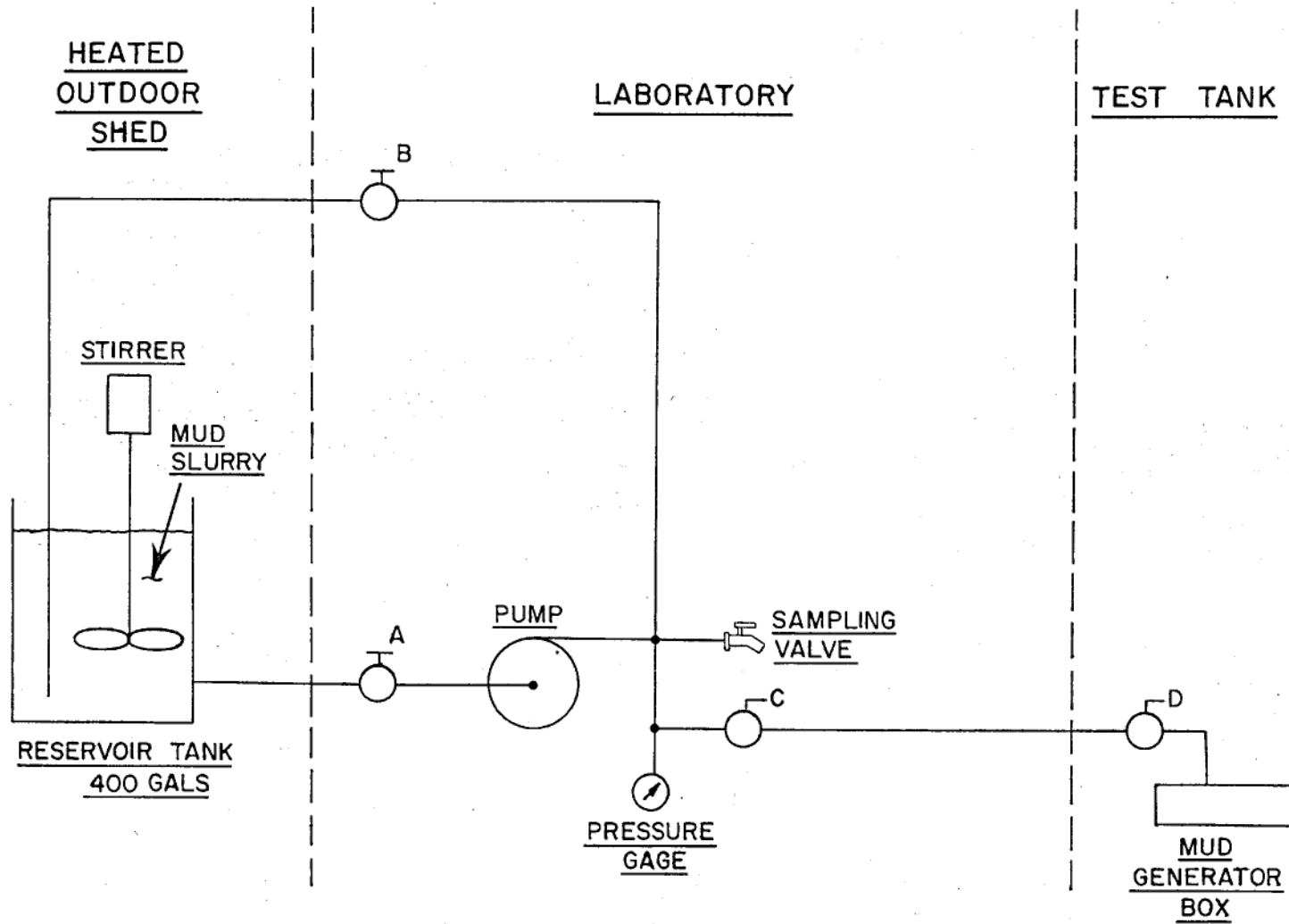
Figure 7. Plumbing schematic, mud supply system
