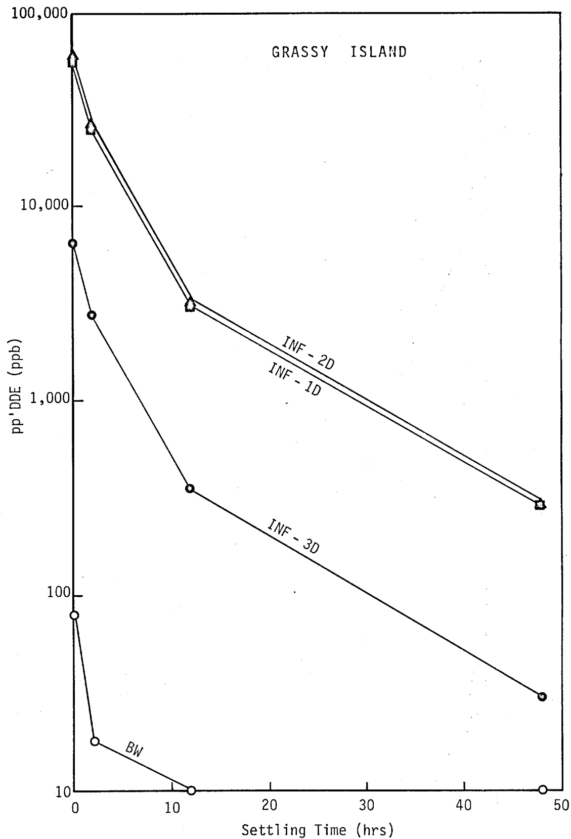
Figure 22. Supernatant Concentration of pp'DDE vs. Settling Time.
