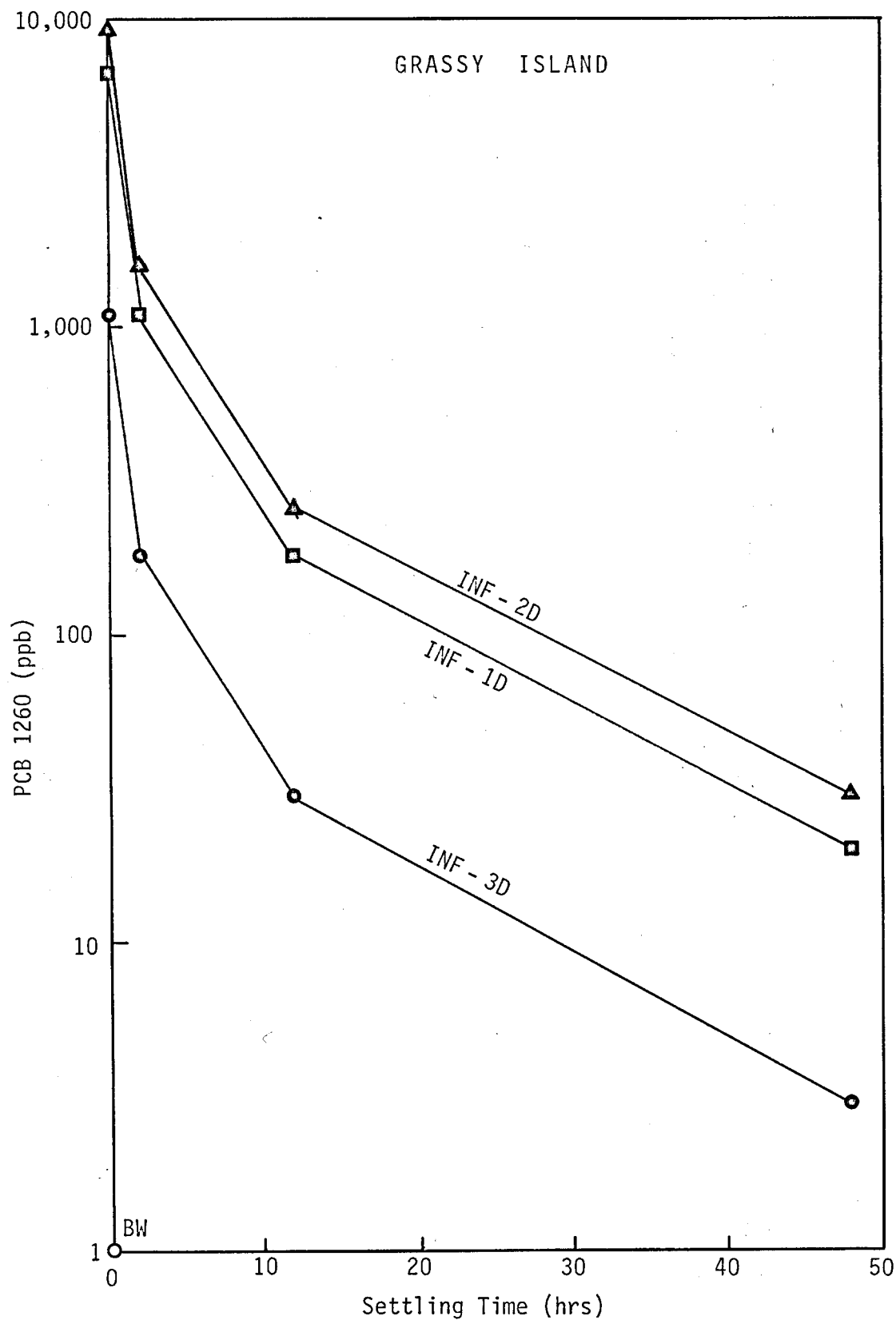
Figure 28. Supernatant Concentration of PCB 1260 vs. Settling Time.
