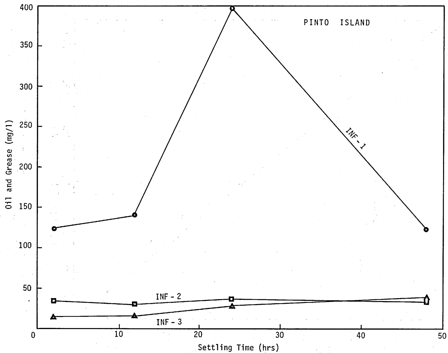
Figure 4. Influent Oil and Grease Concentration vs. Settling Time.
