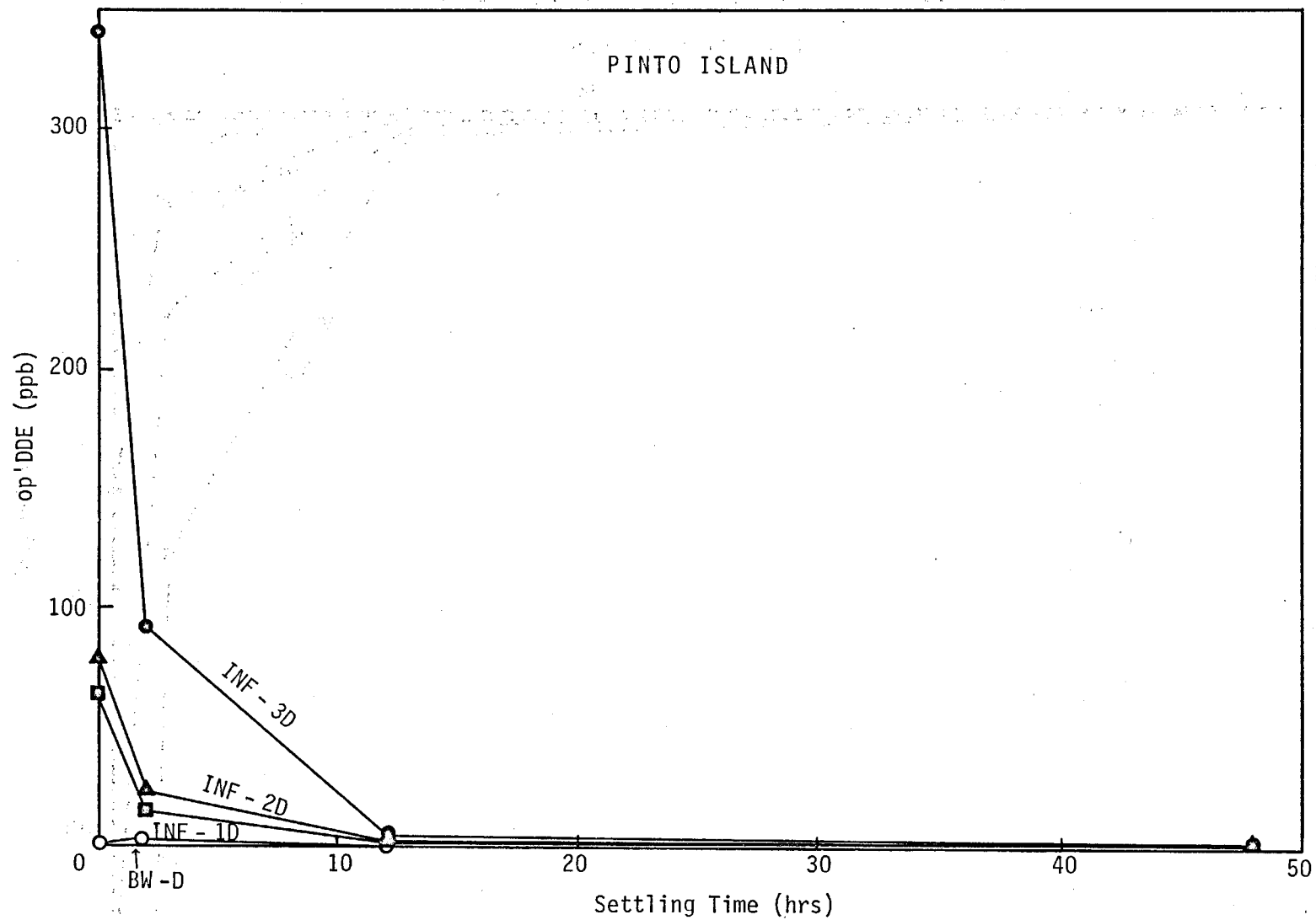
Figure 10. Supernatant Concentration of op'DDE vs. Settling Time.
