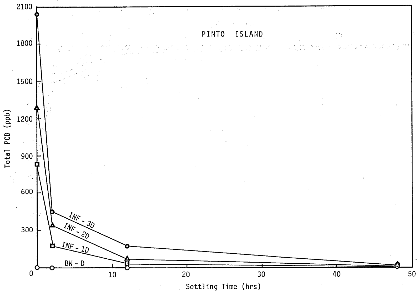
Figure 18. Supernatant Concentration of Total PCB vs. Settling Time.
