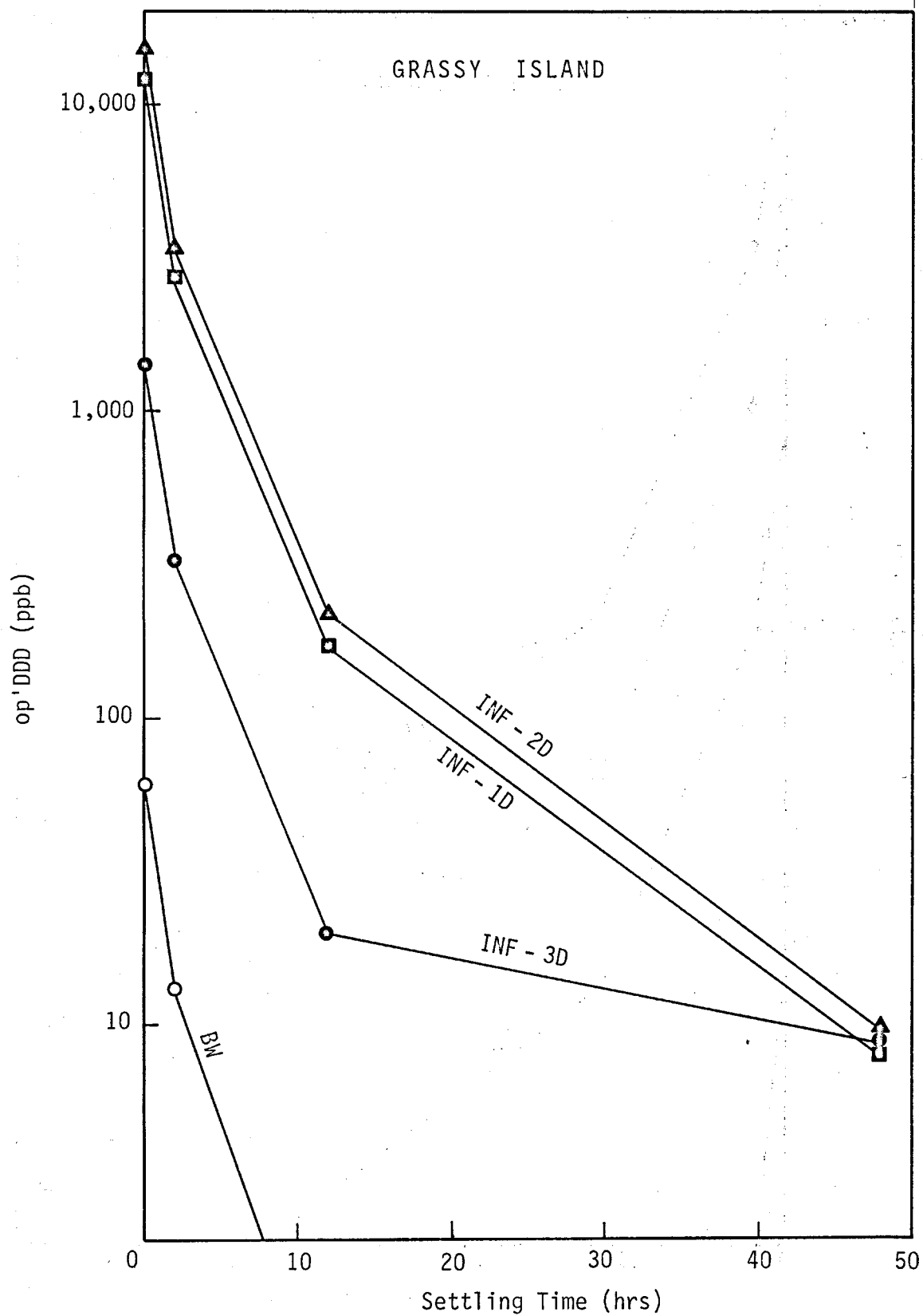
Figure 19. Supernatant Concentration of op'DDD vs. Settling Time.
