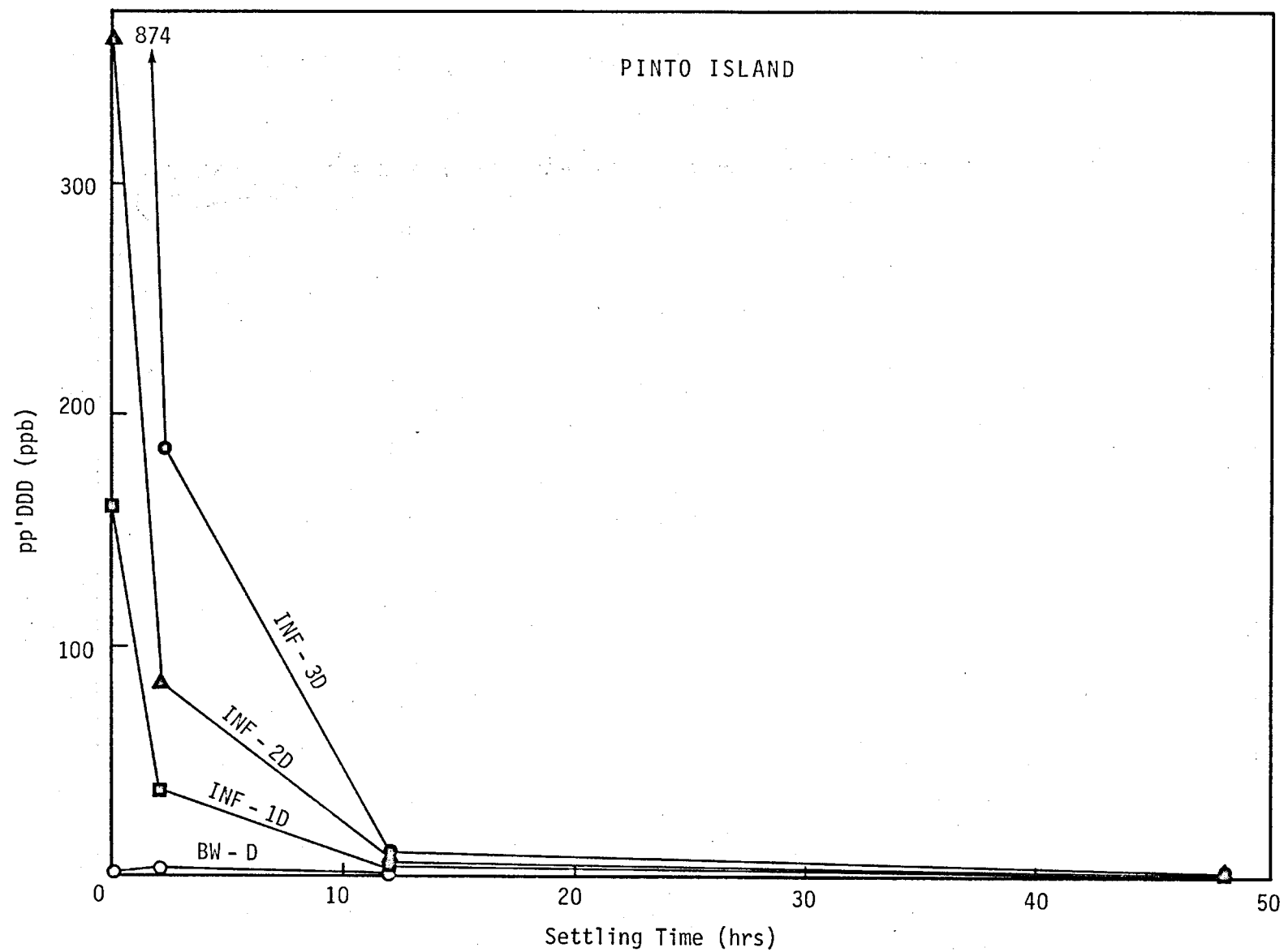
Figure 9. Supernatant Concentration of pp'DDD vs. Settling Time.
