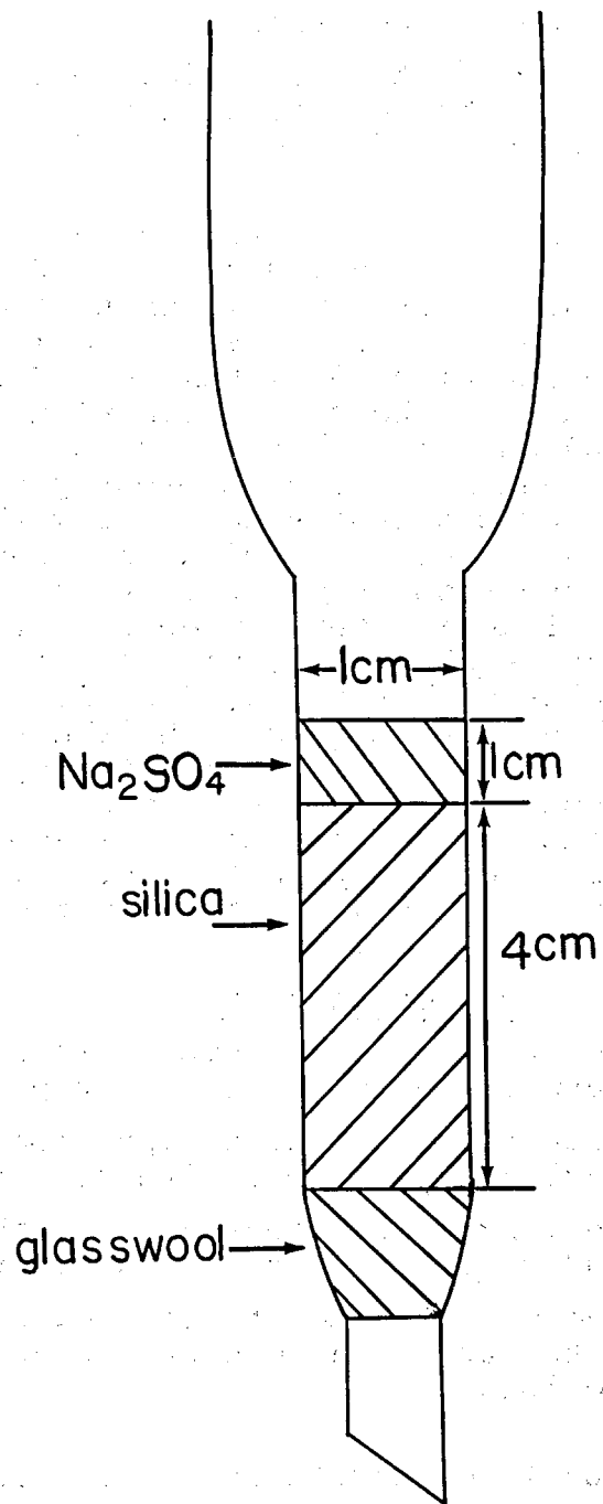
Figure B1. Silica Gel Column.
