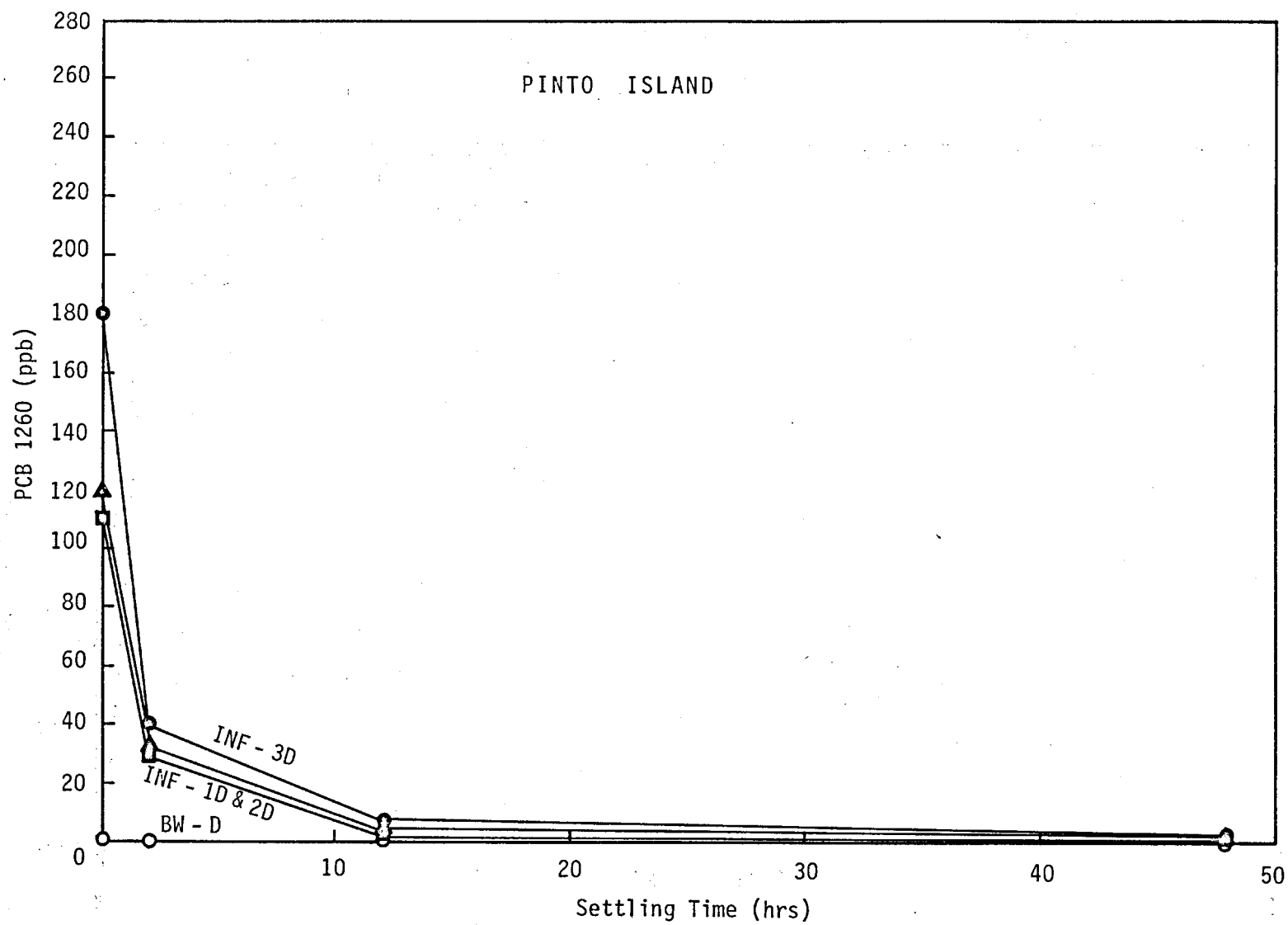
Figure 17. Supernatant Concentration of PCB 1260 vs. Settling Time.
