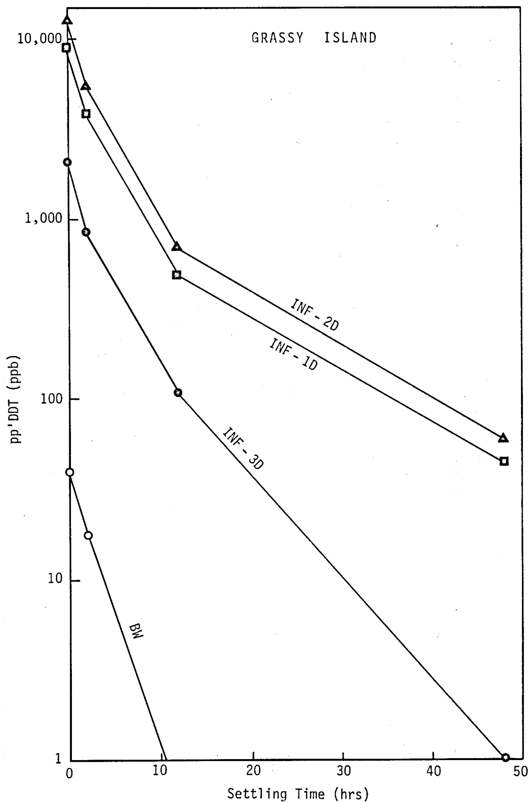
Figure 24. Supernatant Concentration of pp'DDT vs. Settling Time.
