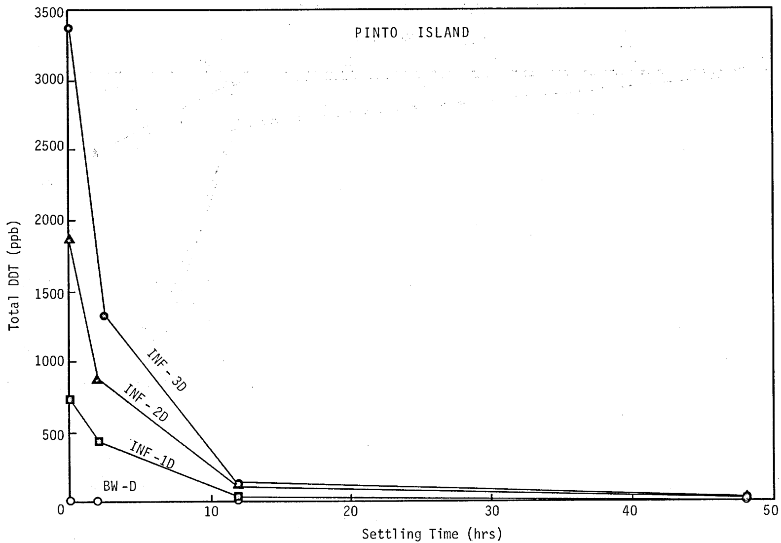
Figure 14. Supernatant Concentration of Total DDT vs. Settling Time.
