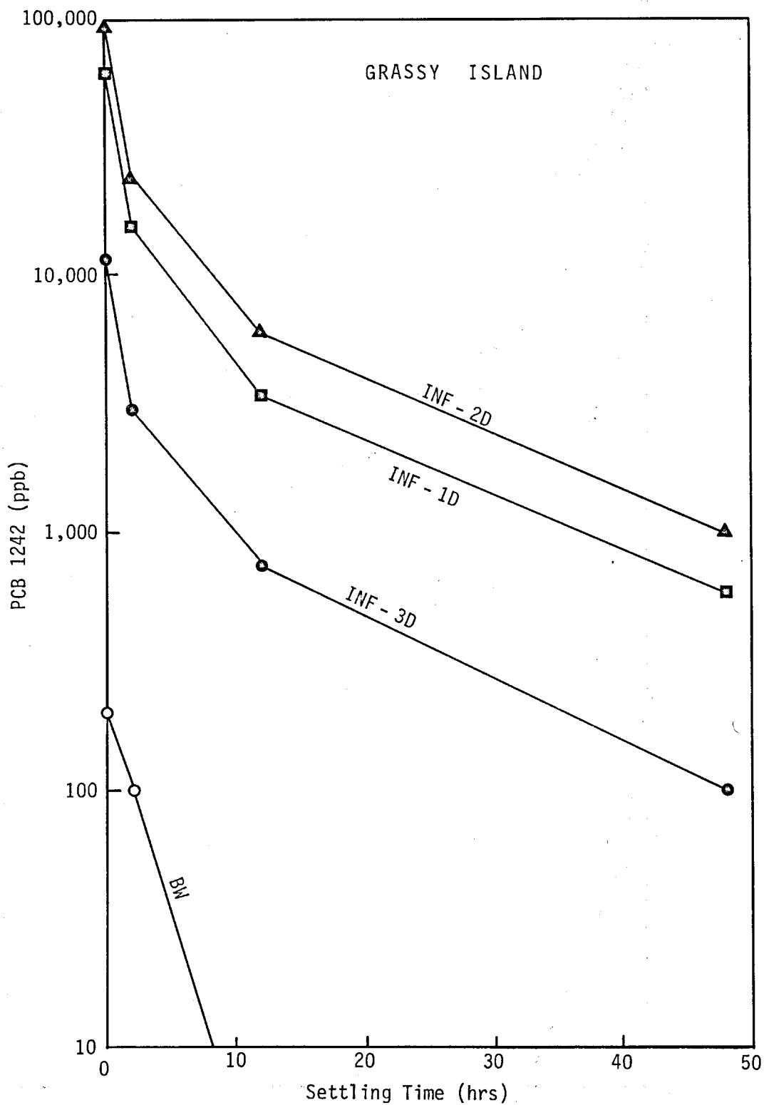
Figure 26. Supernatant Concentration of PCB 1242 vs. Settling Time.
