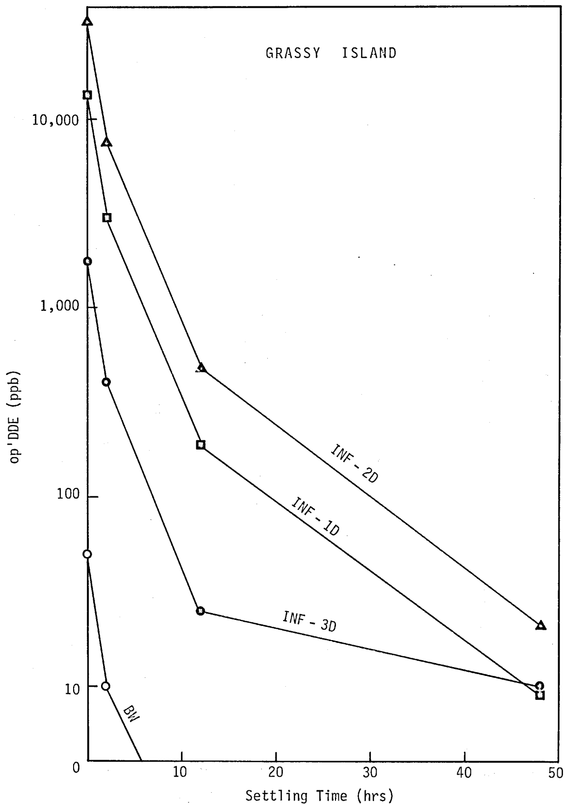
Figure 21. Supernatant Concentration of op'DDE vs. Settling Time.
