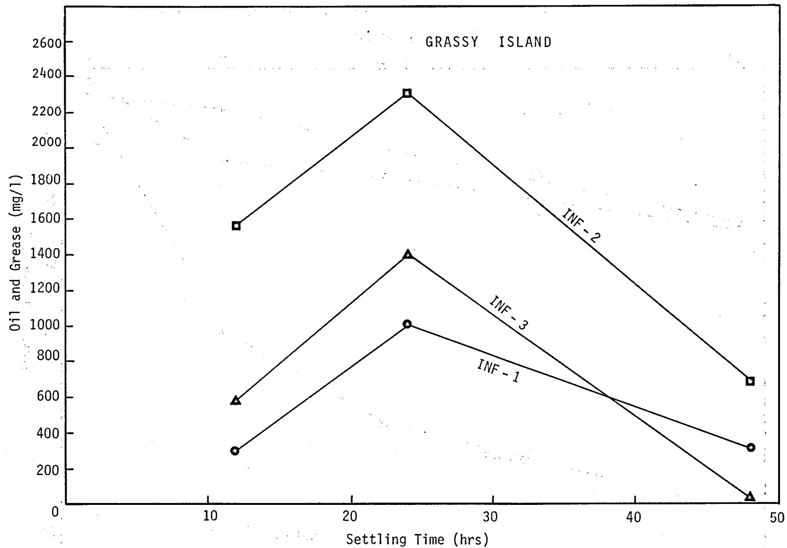
Figure 6. Influent Oil and Grease Concentration vs. Settling Time.
