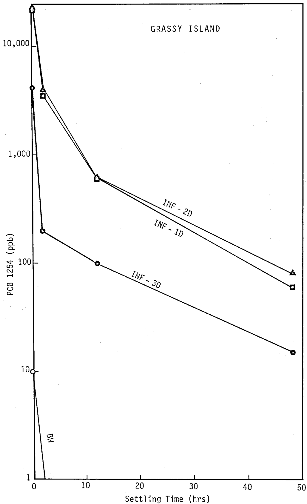
Figure 27. Supernatant Concentration of PCB 1254 vs. Settling Time.
