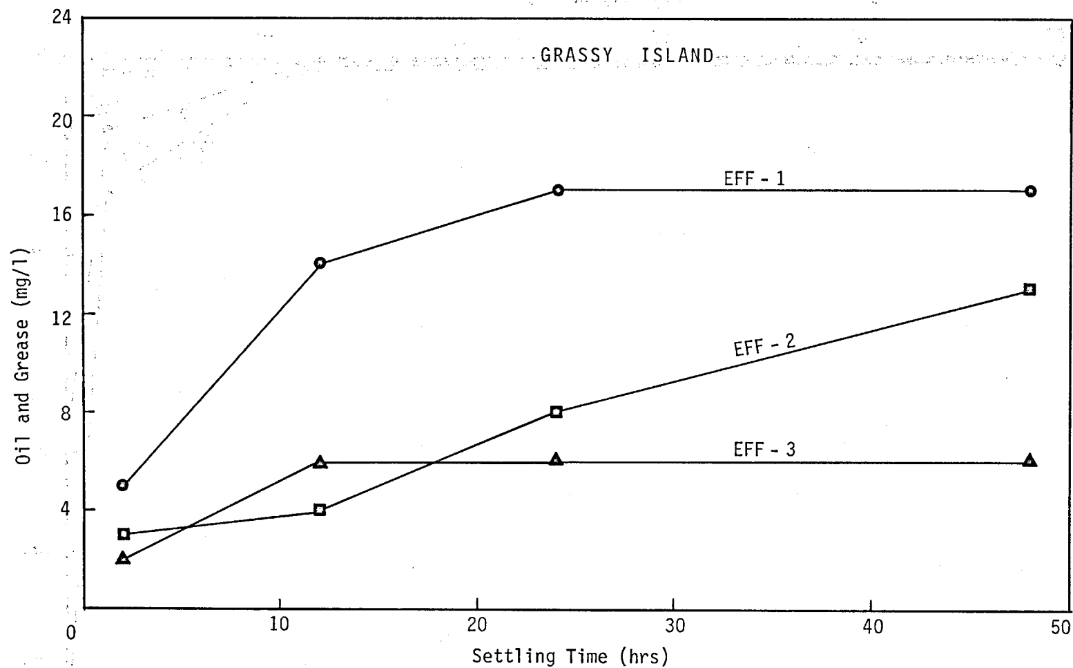
Figure 7. Effluent Oil and Grease Concentration vs. Settling Time.
