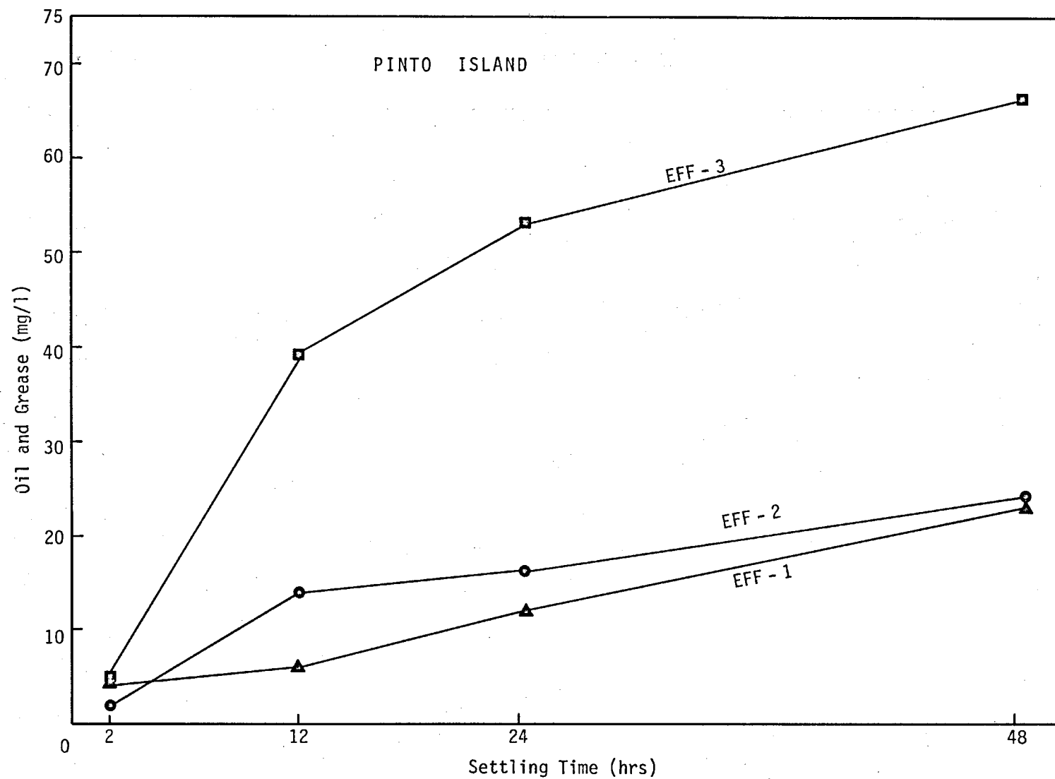
Figure 5. Effluent Oil and Grease Concentration vs Settling Time.
