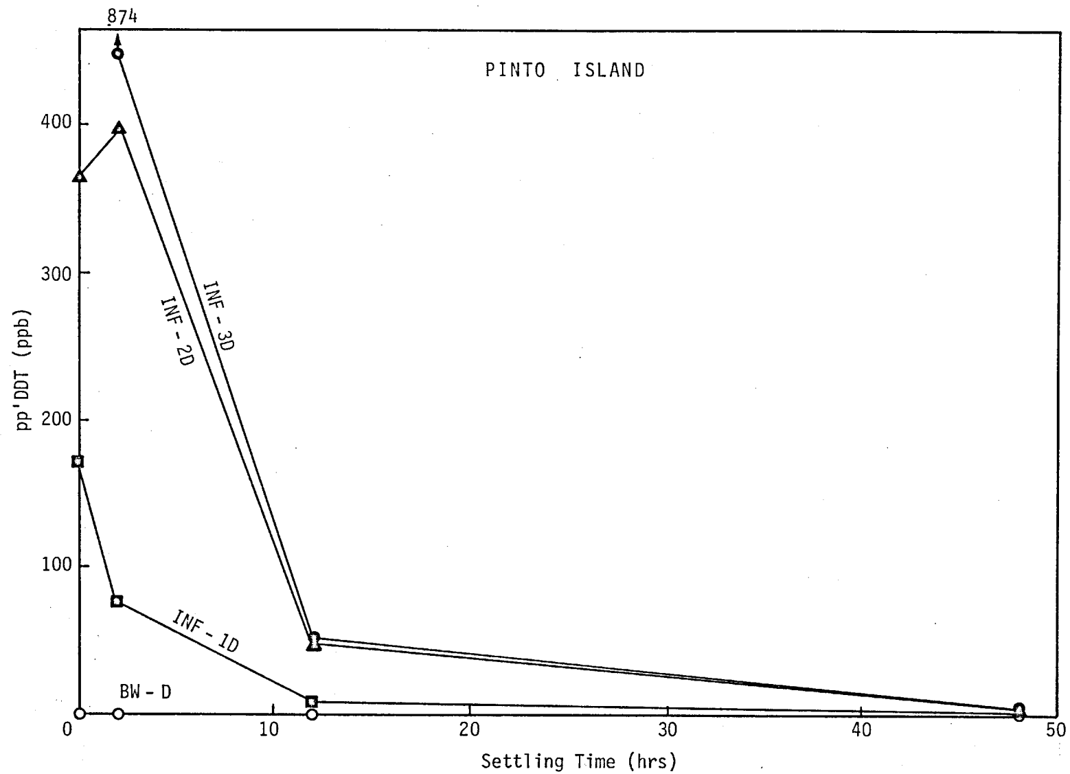
Figure 13. Supernatant Concentration of pp'DDT vs. Settling Time.
