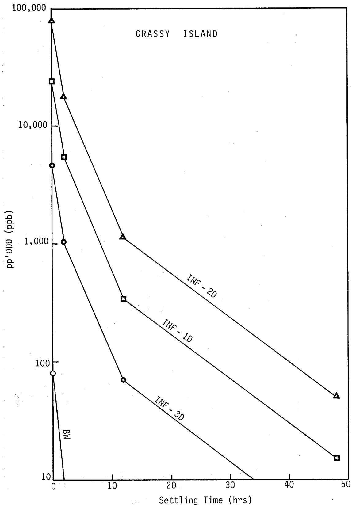
Figure 20. Supernatant Concentration of pp'DDD vs. Settling Time.
