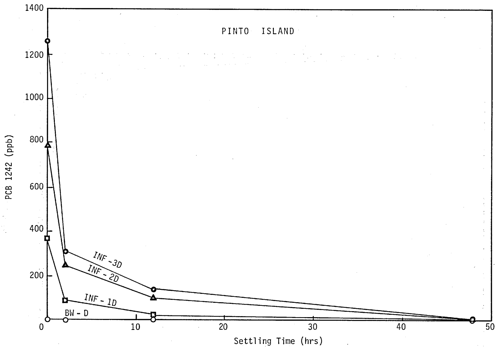
Figure 15. Supernatant Concentration of PCB 1242 vs. Settling Time.
