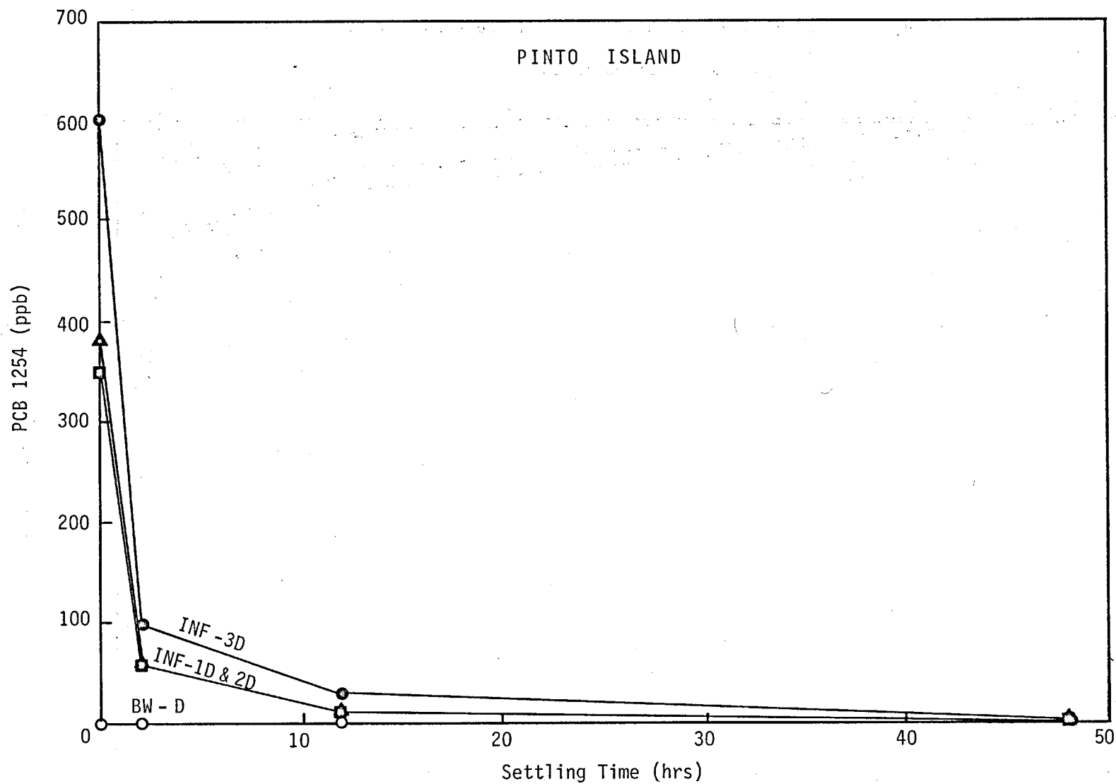
Figure 16. Supernatant Concentration of PCB 1254 vs. Settling Time.
