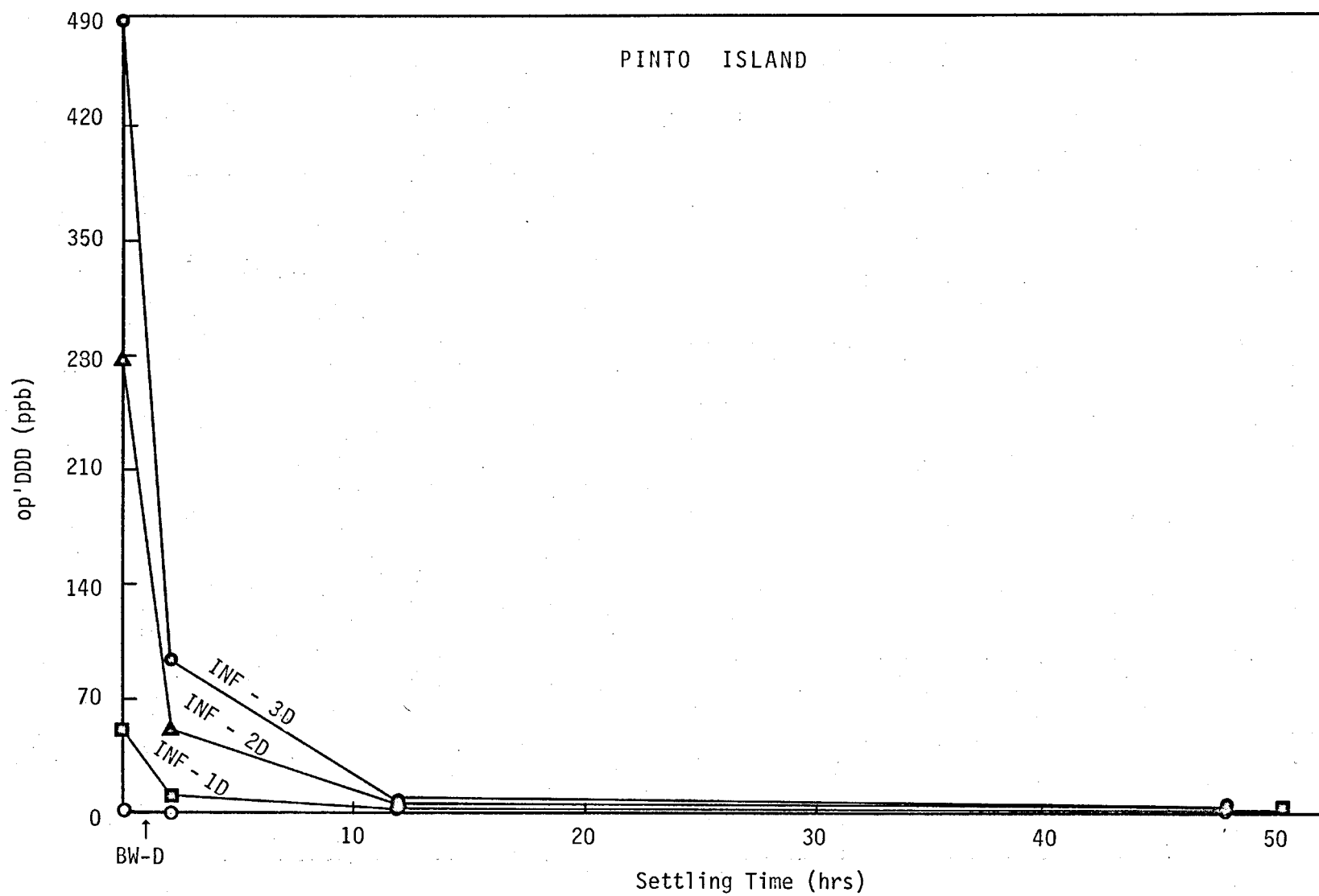
Figure 8. Supernatant Concentration of op'DDD vs. Settling Time.
