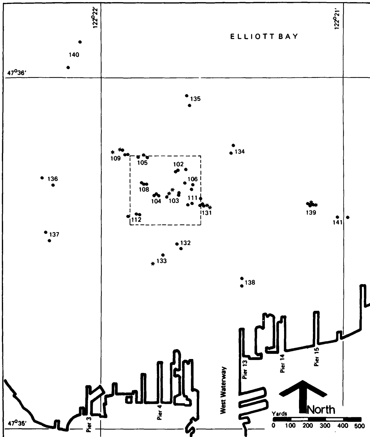
Figure 7. Station Locations (May 1979 Cruise), Gravity Cores for Grain Size • and Interstitial Water Analysis *
