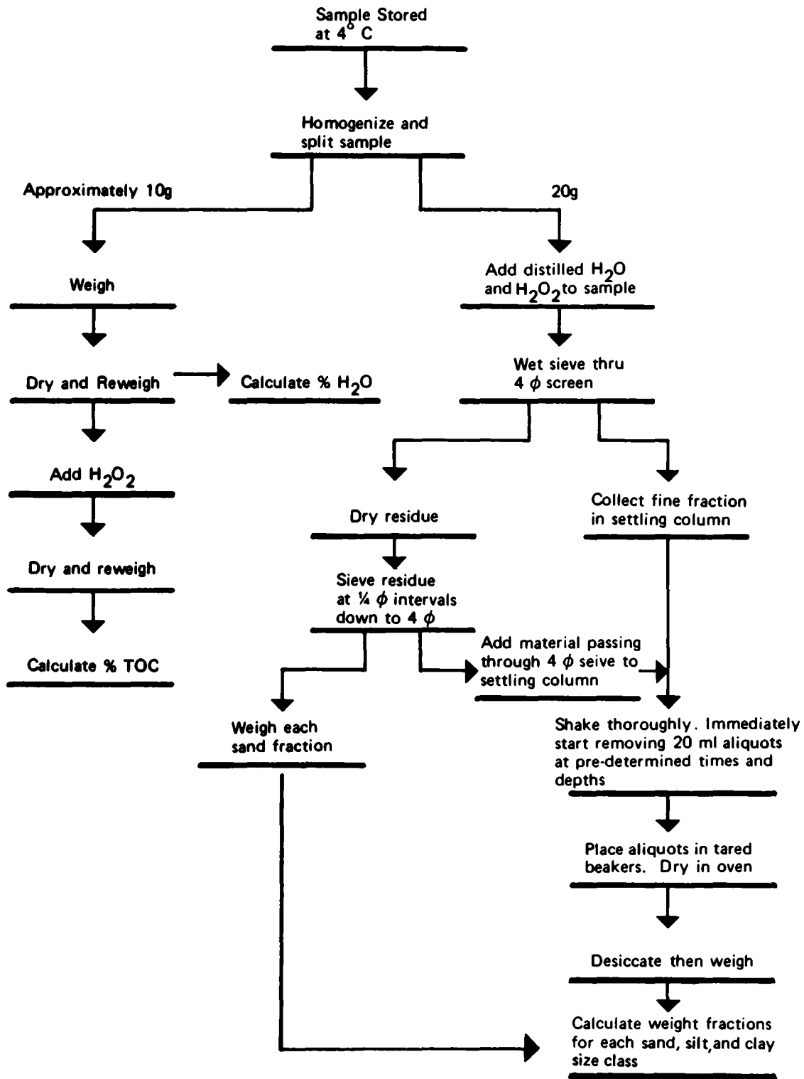
Figure 21. Flow Diagram for Sediment Texture Analysis
