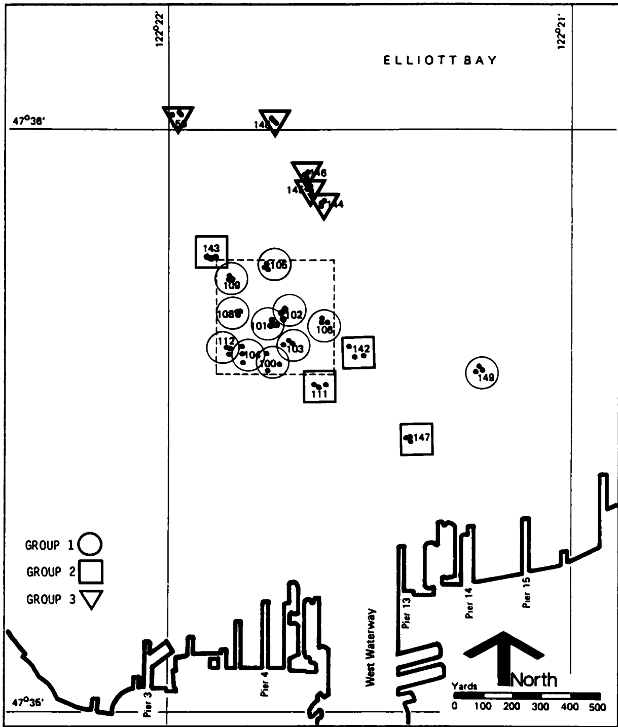
Figure 48c. Cluster Analysis Groupings for Station Medians of October 1979 Macrofauna Biomasses, Code C3MDW
