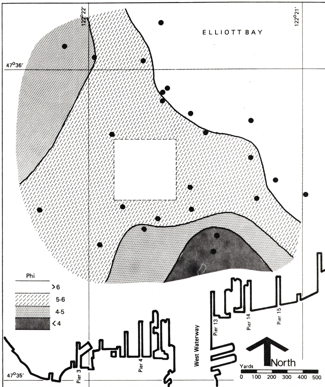
Figure 35. Distribution of Mean Phi for stations Outside the Grid Area. Station means for Cruises 2, 3, and 4 are plotted
