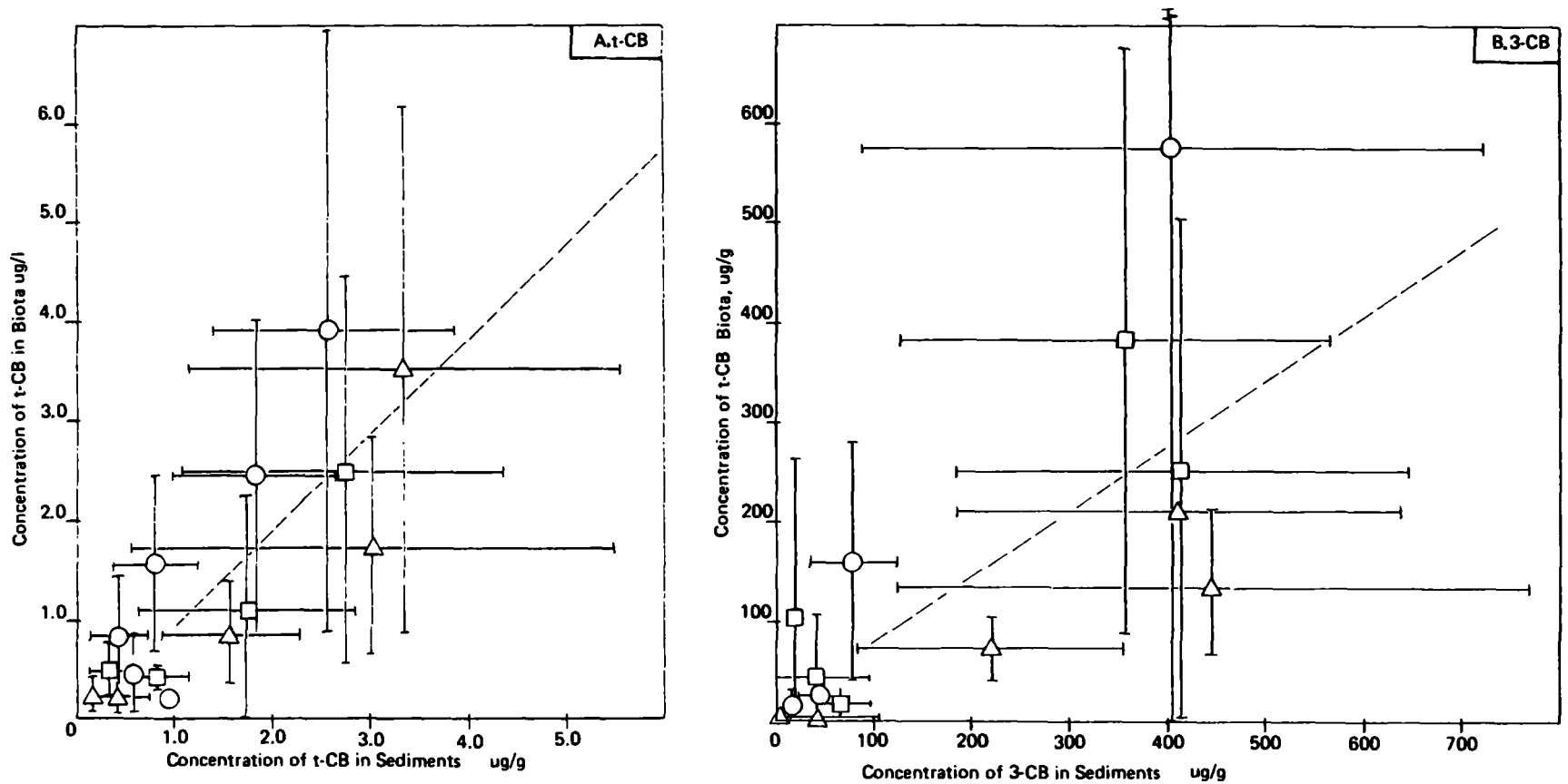
Figure 72. Mean Concentration in the Benthic Macrofauna versus the Mean Concentration in the Surface Sediments from each Sampling Station for a) t-CB and b) 3-CB. Vertical and horizontal lines represent the limits of one standard deviation for the biota and sediments, respectively. Dotted line represents the linear regression evaluation for all data. Data from Cruise 2, May 1979, ○ ; Cruise 3, October 1979, △ ; Cruise 4, May 1980, □
