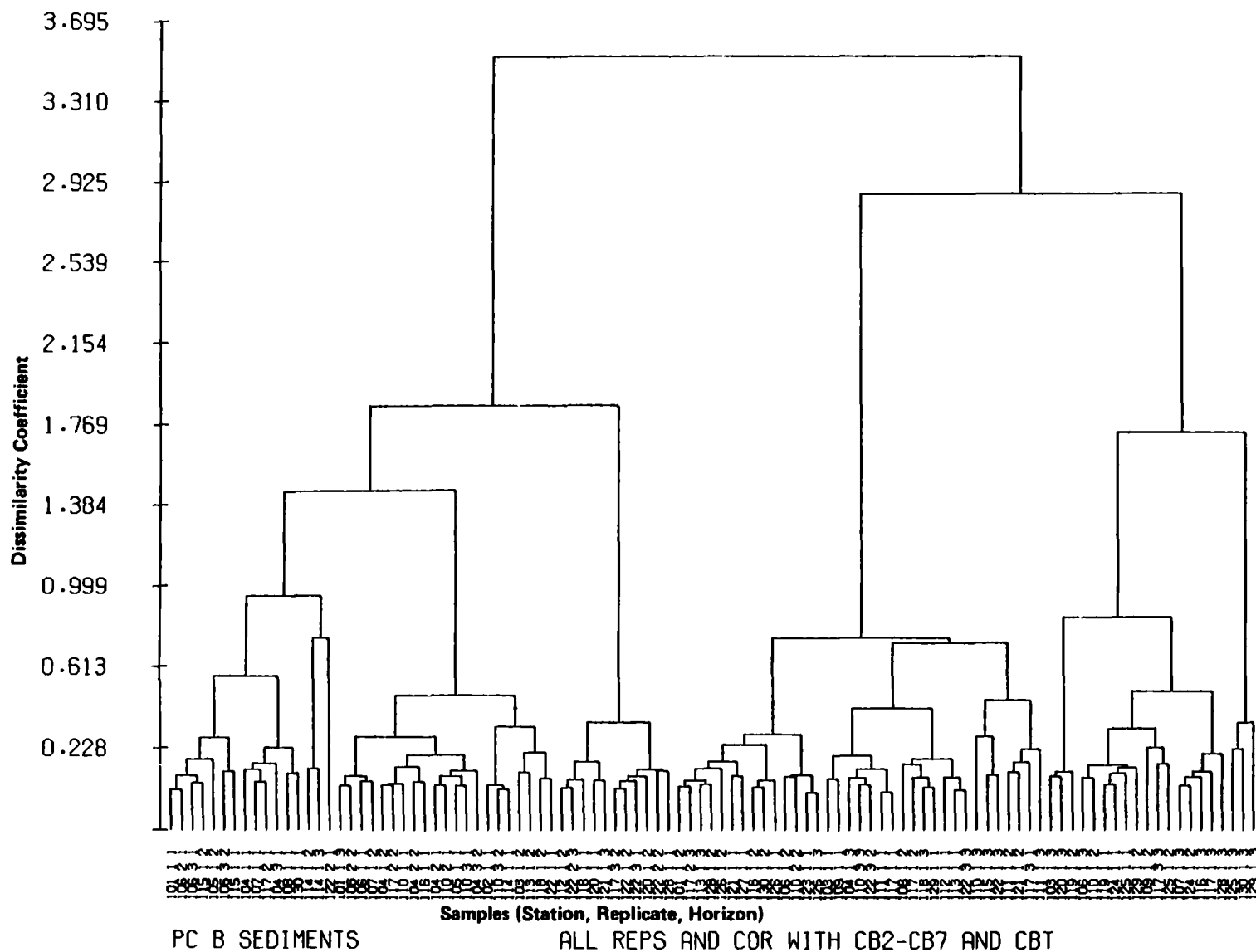
Figure 56. Dendrogram of Sediment Clustering of February 1979 PCB Data
