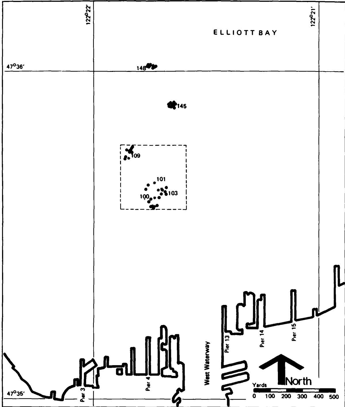
Figure 13. Station Locations (October 1979 Cruise), Samples for PCB Content of Sediments* and Interstitial Water•
