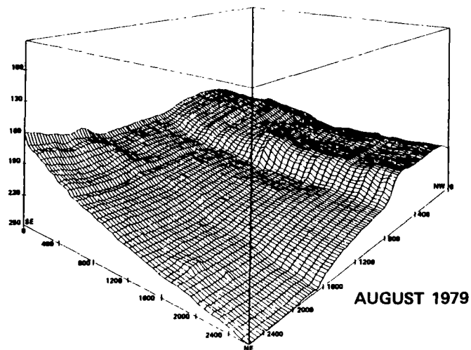
Figure 32. Three-Dimensional Representation of the Bottom Topography of the Study Area: a) February 1976, b) December 1978, c) August 1979.
