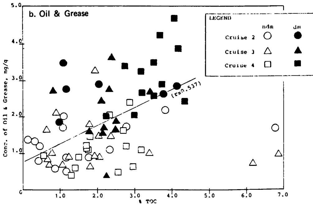
Figure 66. Plots of the Concentrations of t-CB and O&G Versus the Percent TOC of the Sediments. The solid line depicts the linear regression correlation for the dredged material, excluding the outliers indicated by the dashed lines
