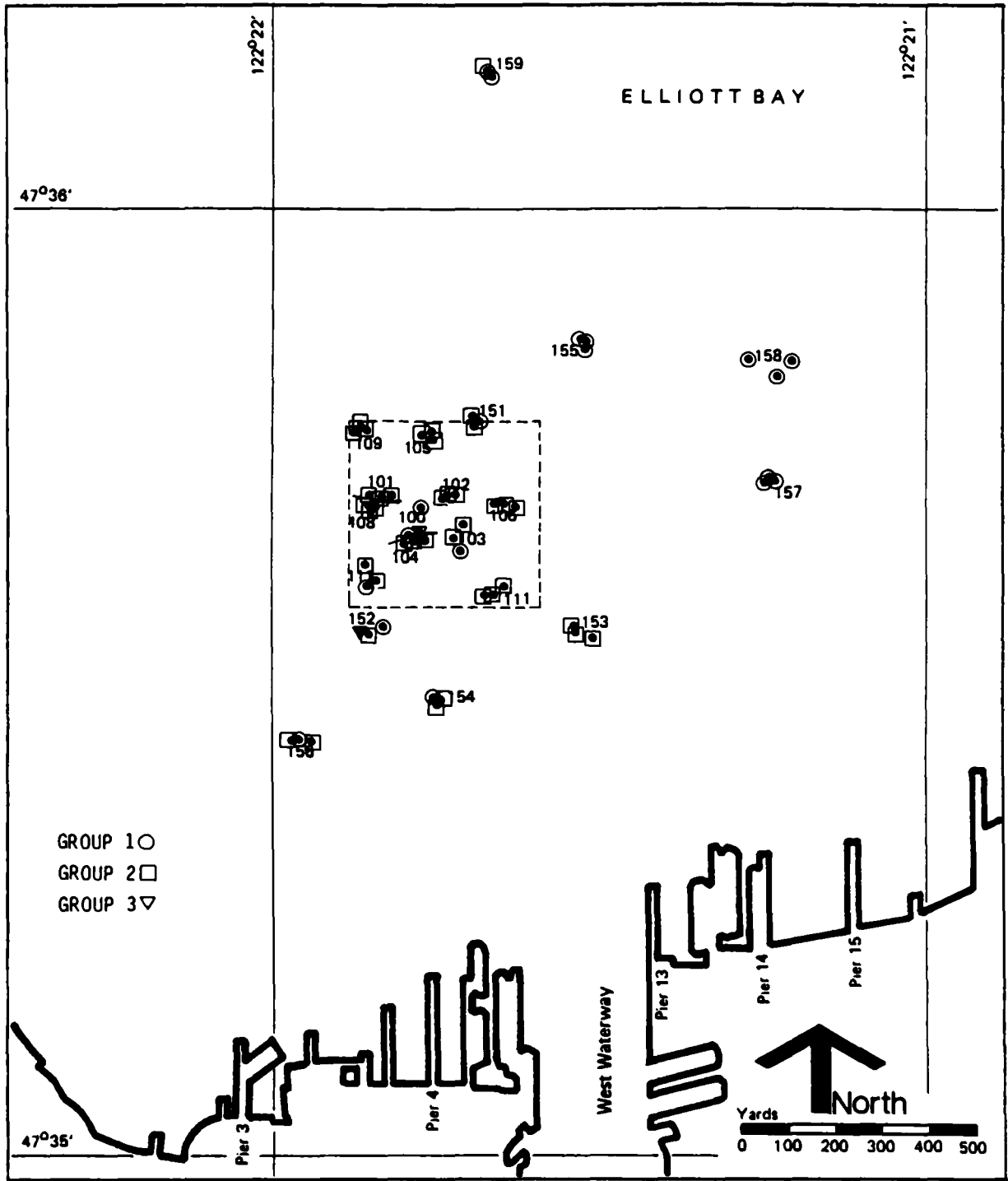
Figure 50a. Cluster Analysis Groupings for Sample (Station Replicates) of May 1980 Macrofauna Biomasses, Code C4W1
