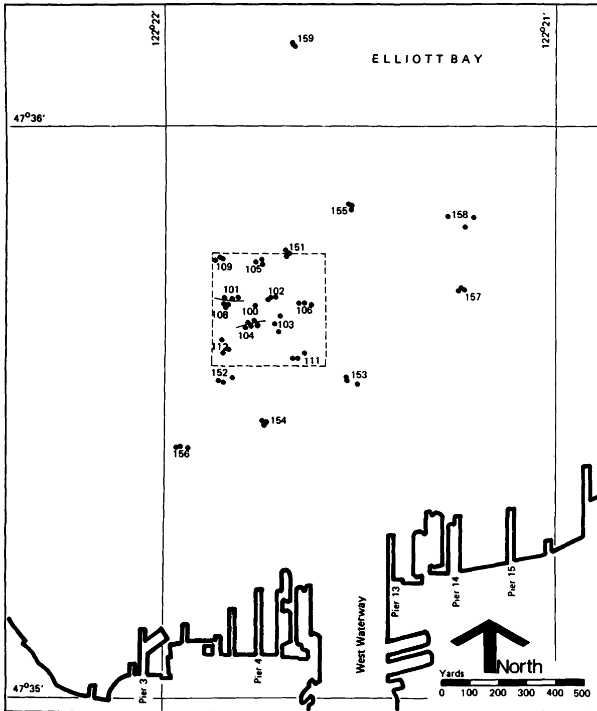
Figure 16. Station Locations (May 1980 Cruise), Grab Samples for Benthic Fauna Characterization
