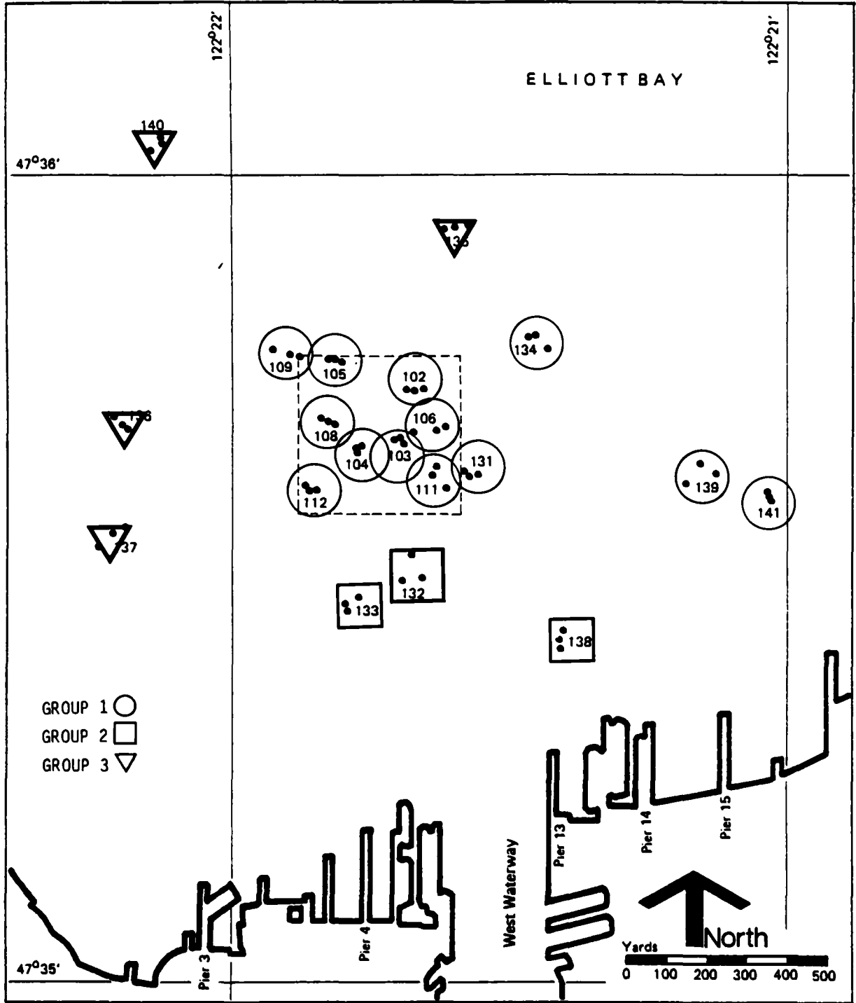
Figure 46b. Cluster Analysis Groupings for Station Means and Medians of May 1979 Macrofauna Biomasses, Codes C2MW and C2MDW
