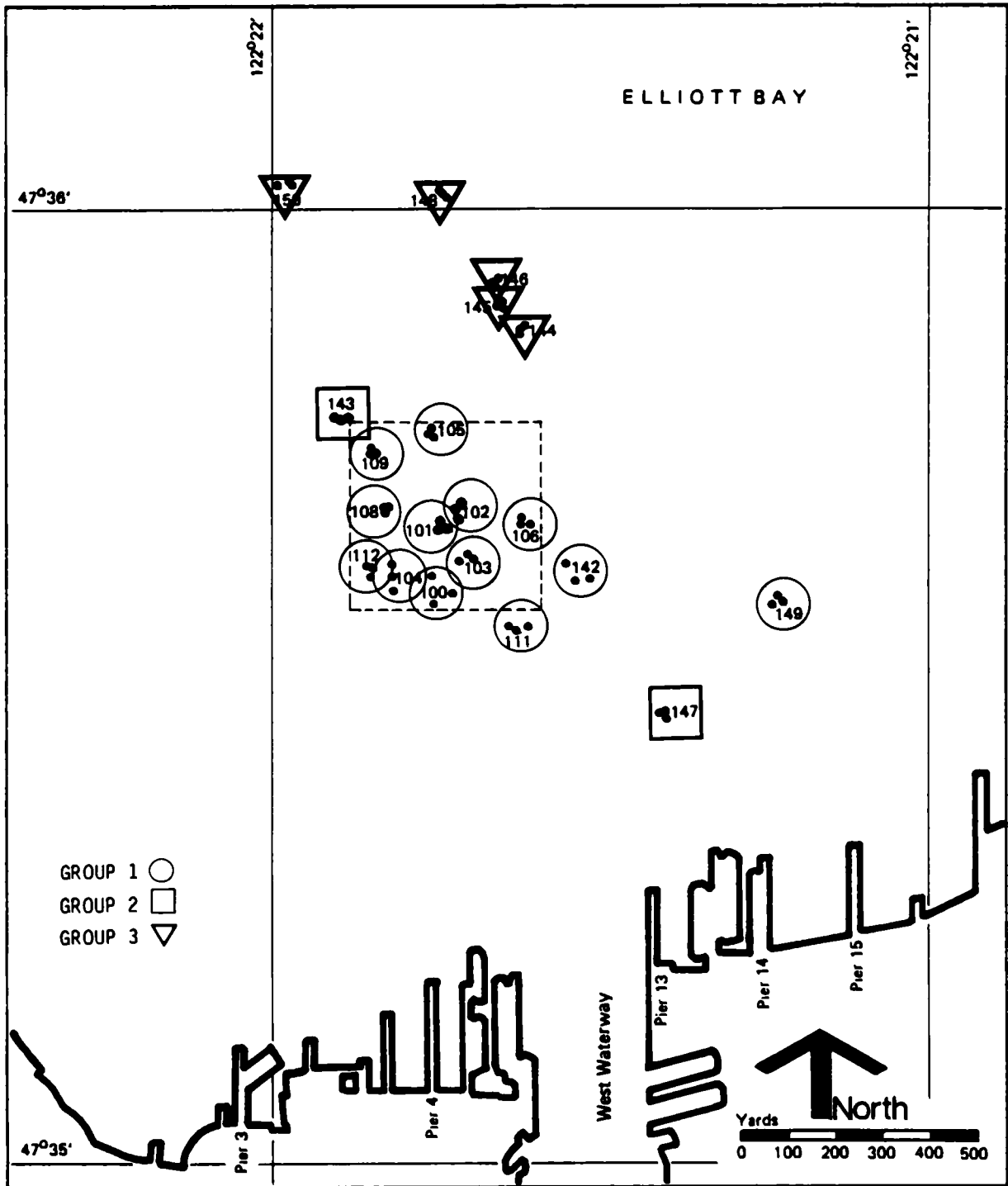
Figure 48b. Cluster Analysis Groupings for Station Means of October 1979 Macrofauna Biomasses, Code C3MW
