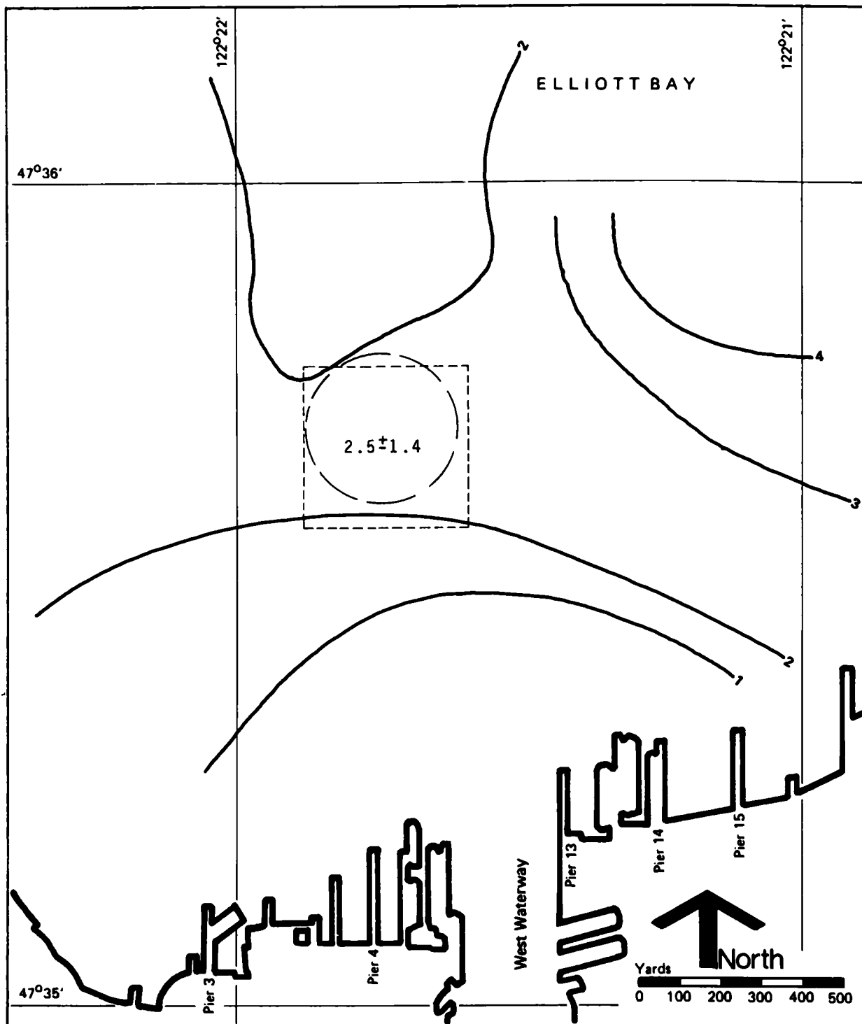
Figure 61. Contours of the Approximate Percent TOC of the Surface Sediments, Cruises 2, 3, and 4
