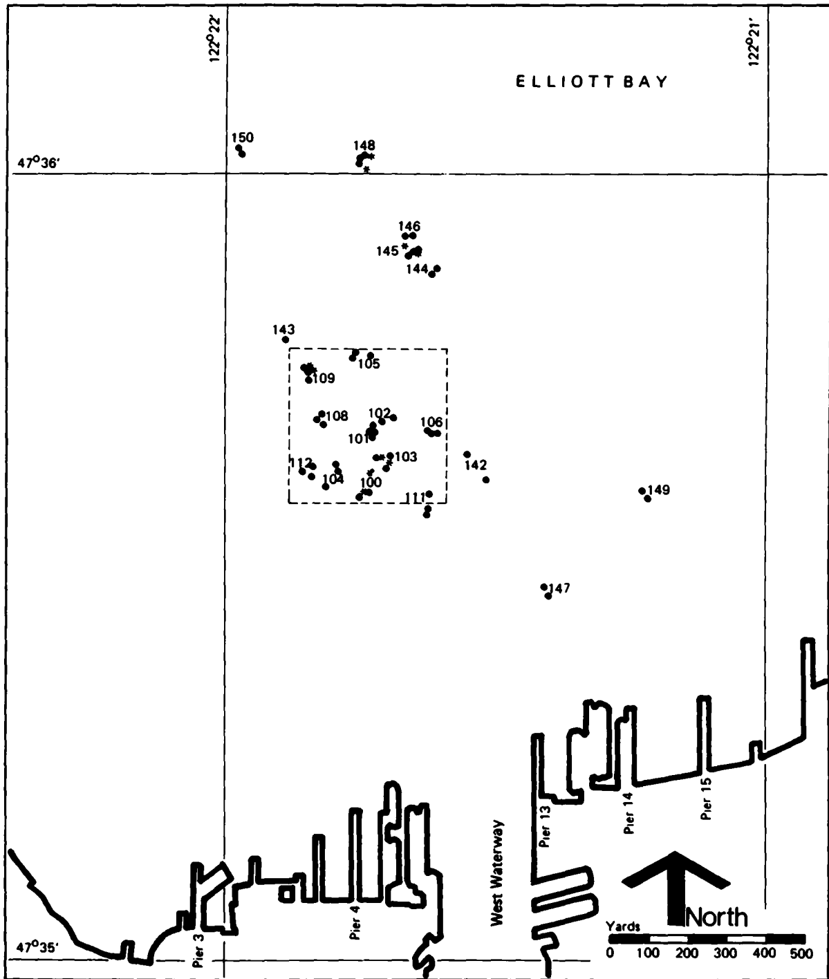
Figure 12. Station Locations (October 1979 Cruise), Gravity Cores for Grain Size * and Interstitial Water Analysis •
