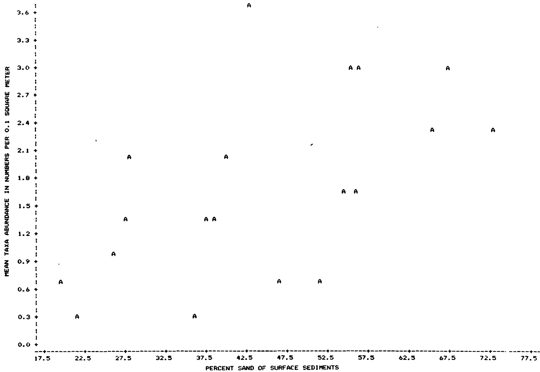
Figure 51. Scatter Plot of Praxilella gracilis versus Percent Sand, May 1979
