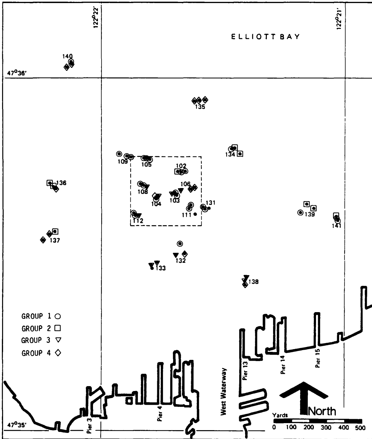
Figure 46a. Cluster Analysis Groupings for Samples (Station Replicates) of May 1979 Macrofauna Biomasses, Code C2W1
