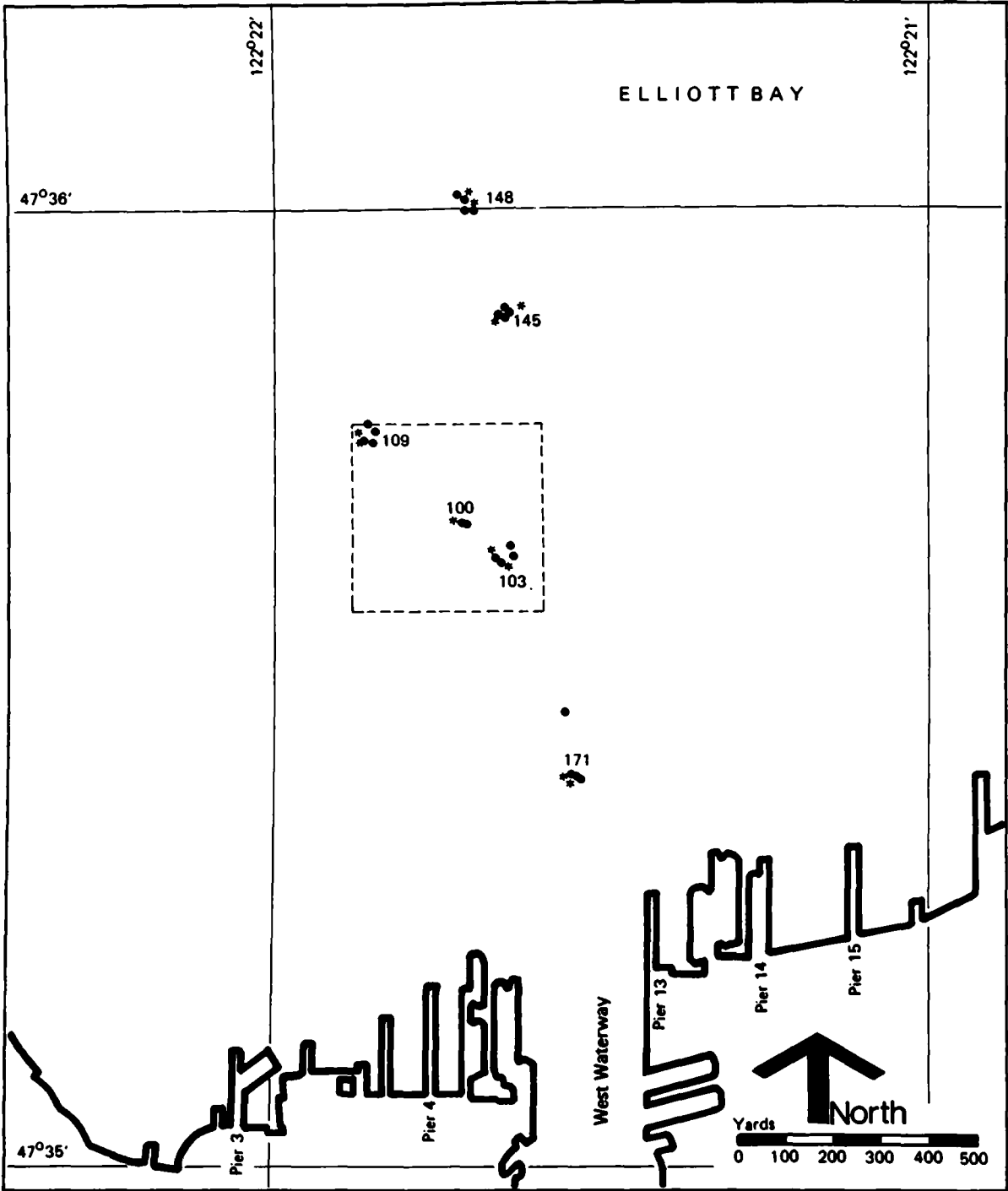
Figure 15. Station Locations (October 1979 Cruise), Water Samples for PCB Content of Water • and Suspended Particulate Matter and Hydrocasts*
