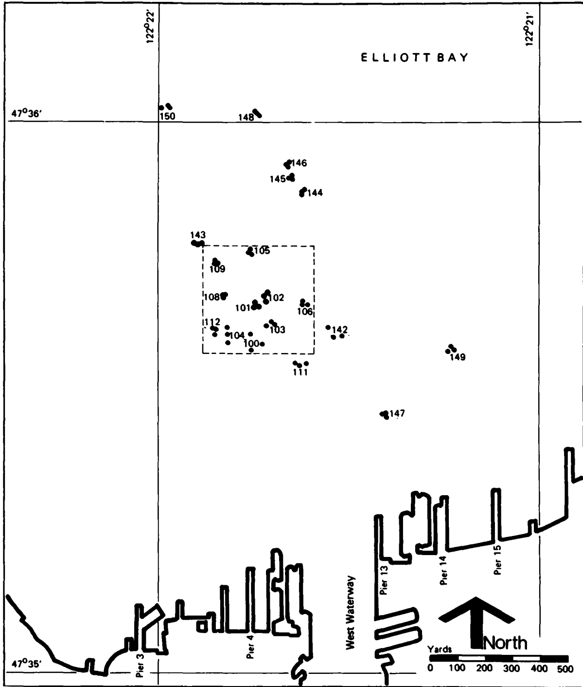
Figure 11. Station Locations (October 1979 Cruise), Grab Samples for Benthic Fauna Characterization
