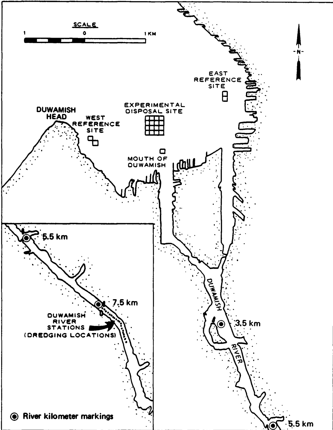
Figure 2. Original Station Grid
