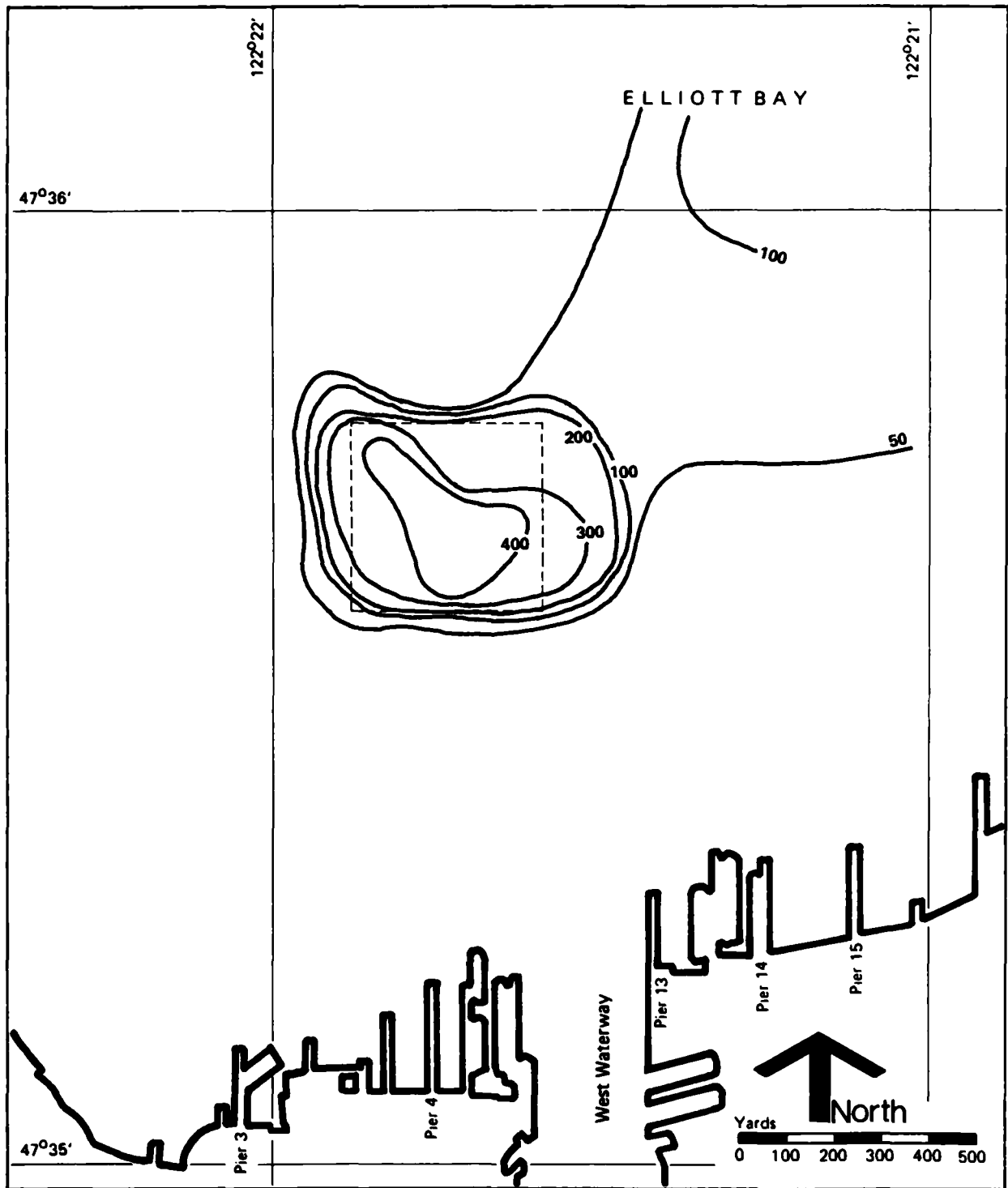
Figure 55. Concentration Contours of the Approximate Distribution of 3-CB in the Surface Sediments, Cruises 1, 2, 3, and 4. Concentrations in units of ng/g
