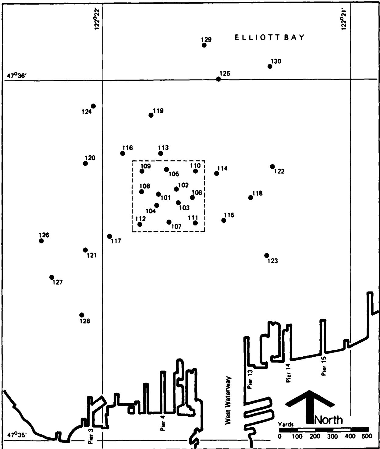
Figure 5. Station Locations - Reconnaissance Cruise, February 1979
