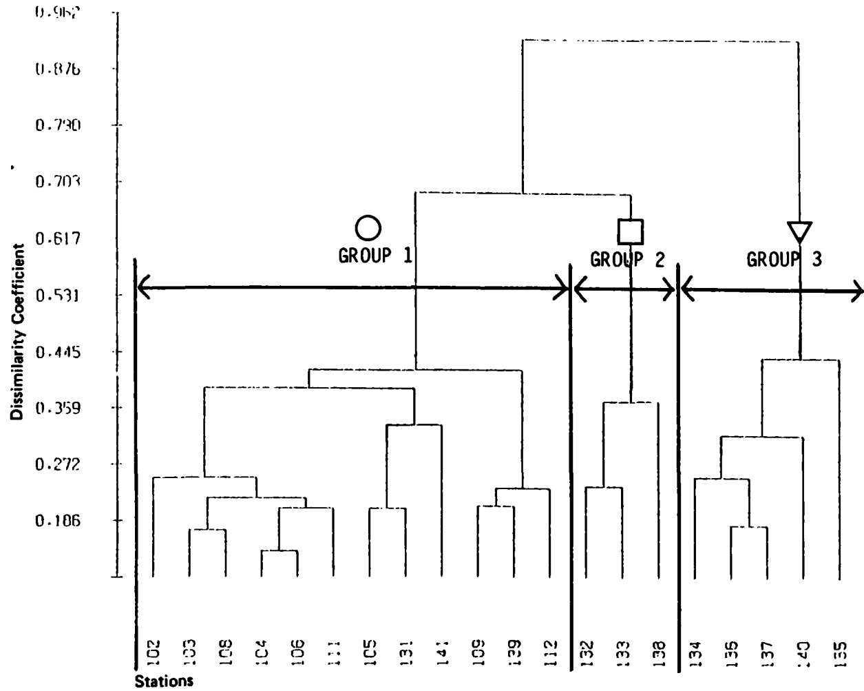
Figure 44b. Cluster Analysis Dendrogram for Station Means of May 1979 Macrofauna Abundances, Code C2MC
