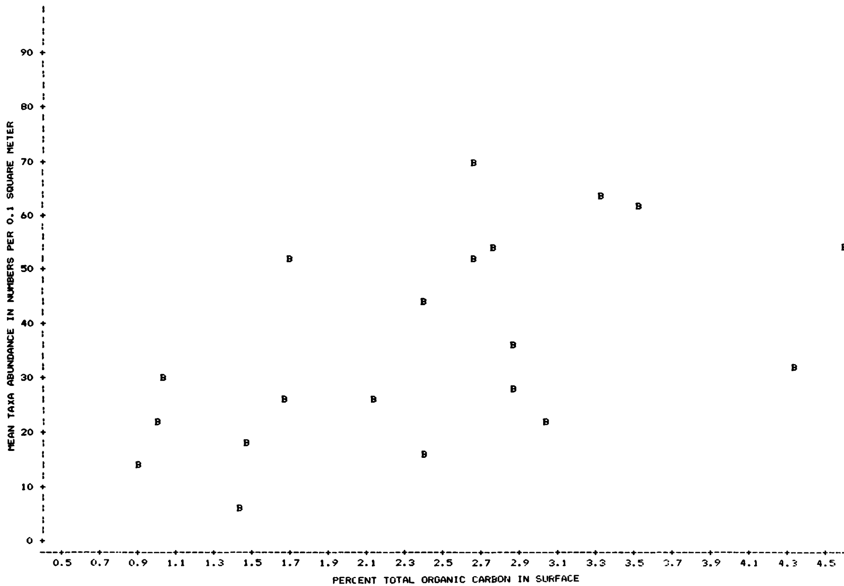
Figure 52. Scatter Plot of Paraonella spinifera versus Percent TOC, May 1979
