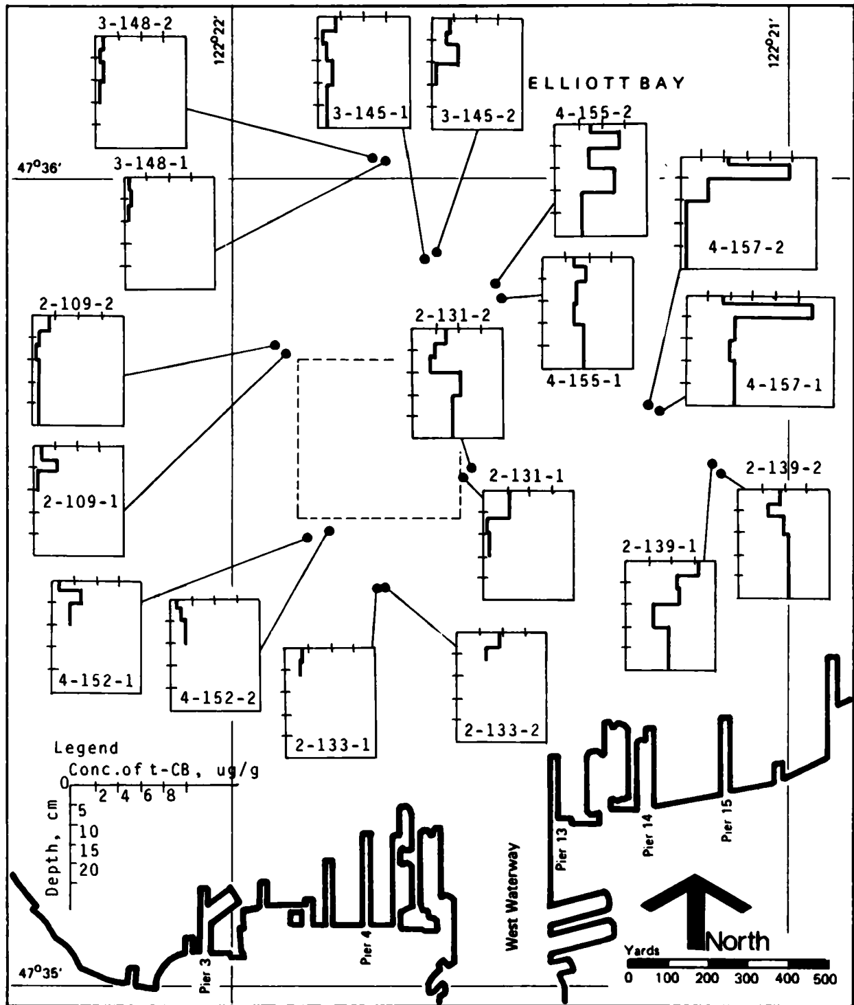
Figure 60. Depth Profiles of the t-CB Concentrations in the Non-Dredged Material Cores
