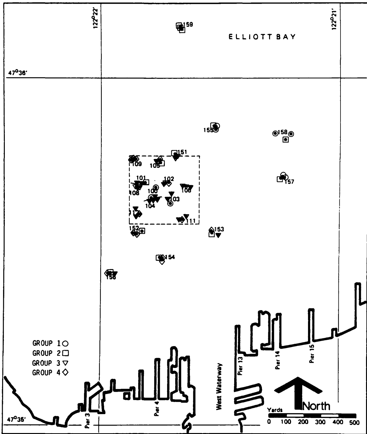
Figure 49a. Cluster Analysis Groupings for Sample (Station Replicates) of May 1980 Macrofauna Abundances, Code C4C1
