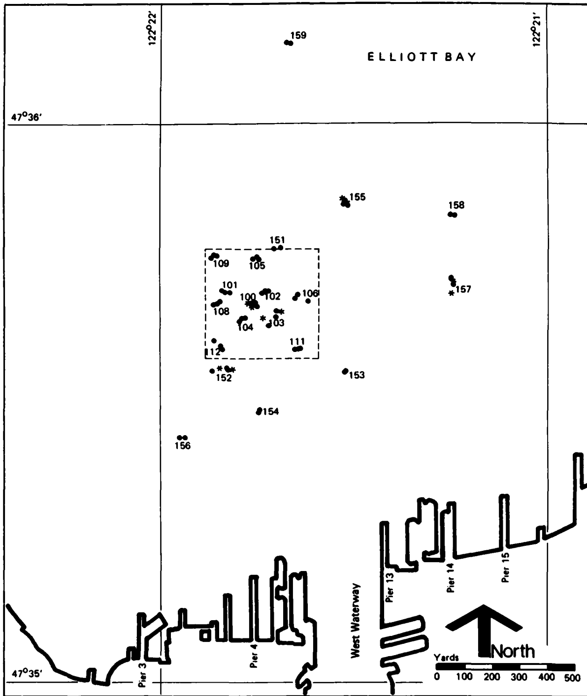
Figure 17. Station Locations (May 1980 Cruise), Gravity Cores for Grain Size • and Interstitial Water Analysis *
