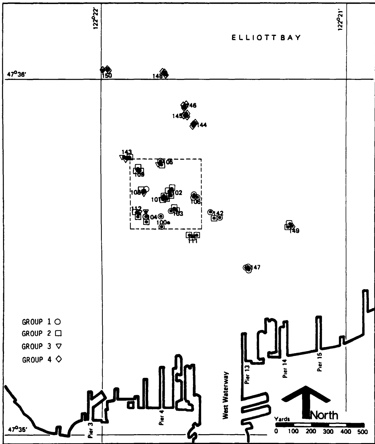
Figure 47a. Cluster Analysis Groupings for Samples (Station Replicates) of October 1979 Macrofauna Abundances, Code C3C1
