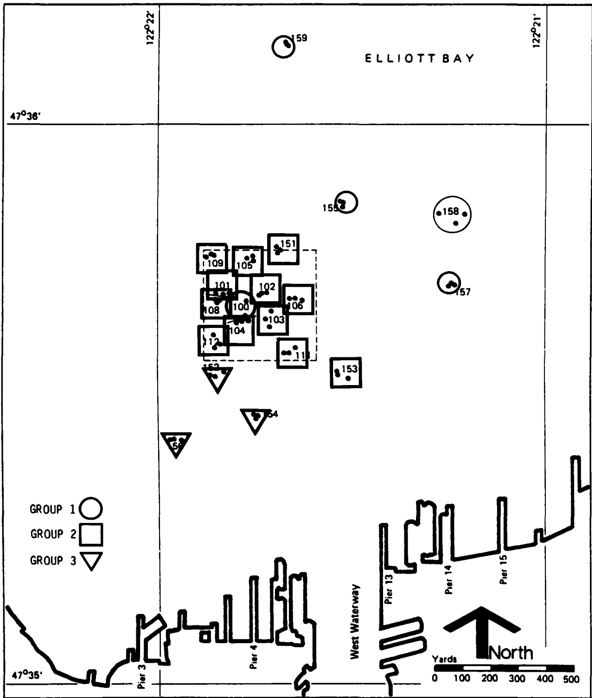
Figure 49b. Cluster Analysis Groupings for Station Medians of May 1980 Macrofauna Abundances, Code C4MDC
