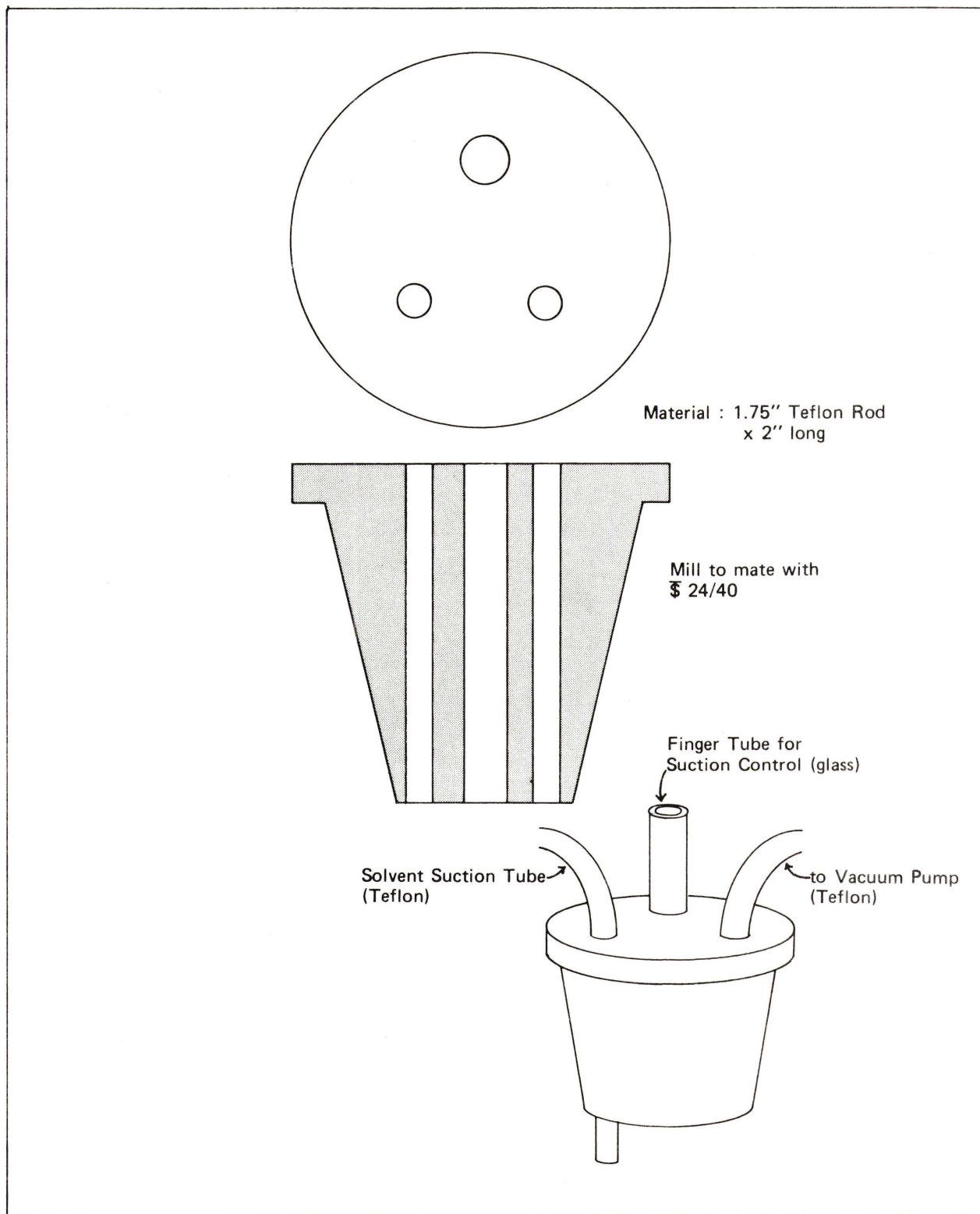
Figure 24. Projection and Perspective Drawings of the Teflon-Stopper Solvent Extractor Apparatus
