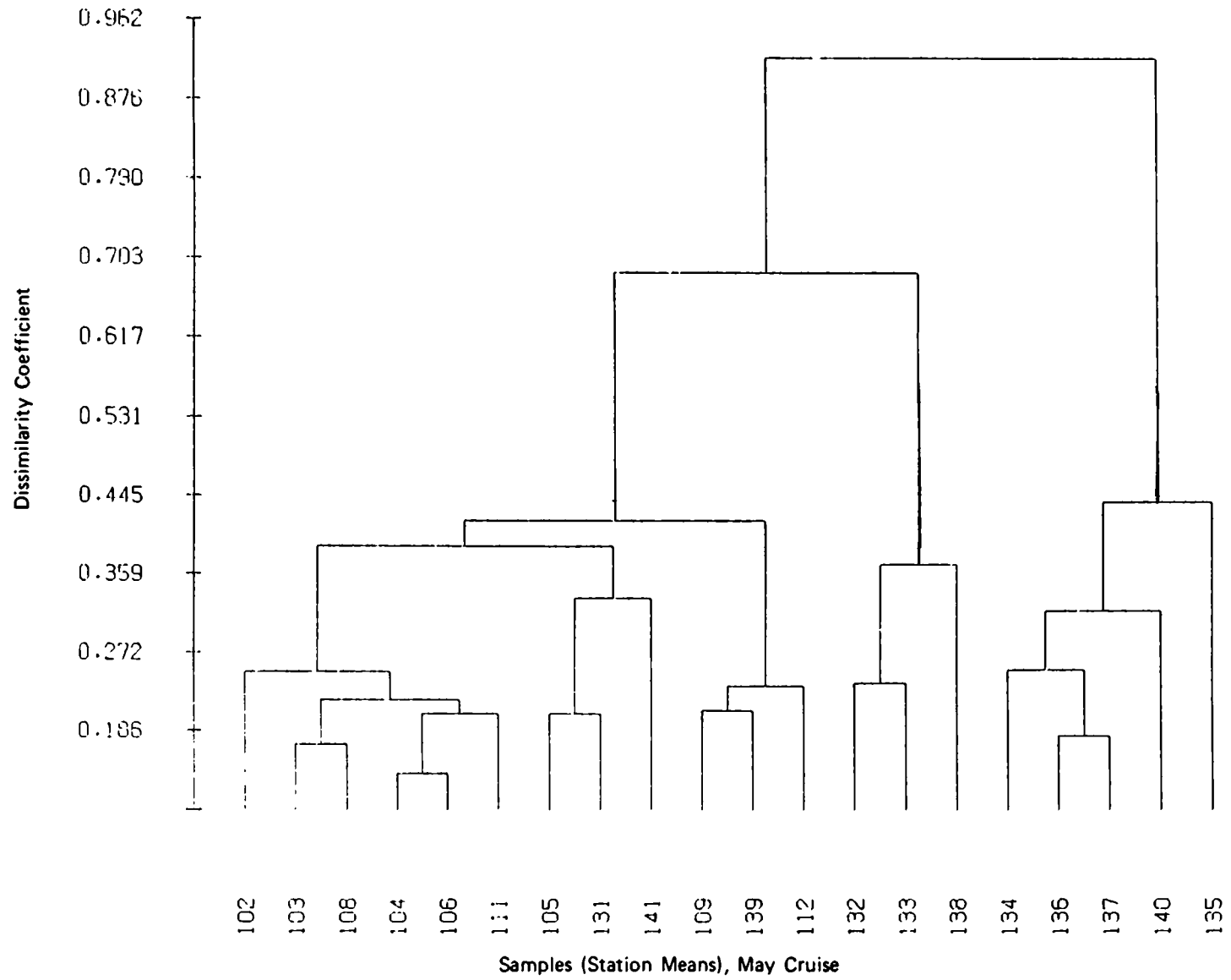
Figure 29. Typical Dendrogram Resulting from Cluster Analysis
