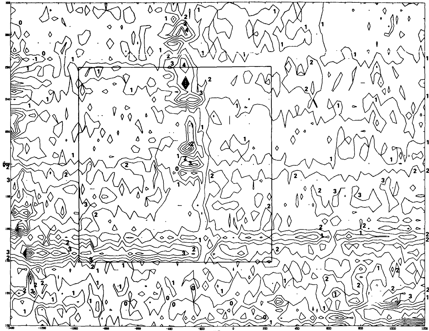
Figure 33. The Difference in Depth (in feet) Between the August 1979 and December 1978 Surveys. Original grid denoted by square
