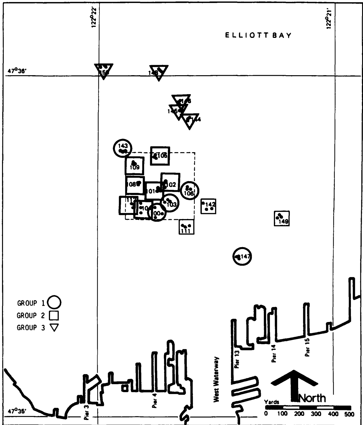
Figure 47b. Cluster Analysis Groupings for Station Means of October 1979 Macrofauna Abundances, Code C3MC
