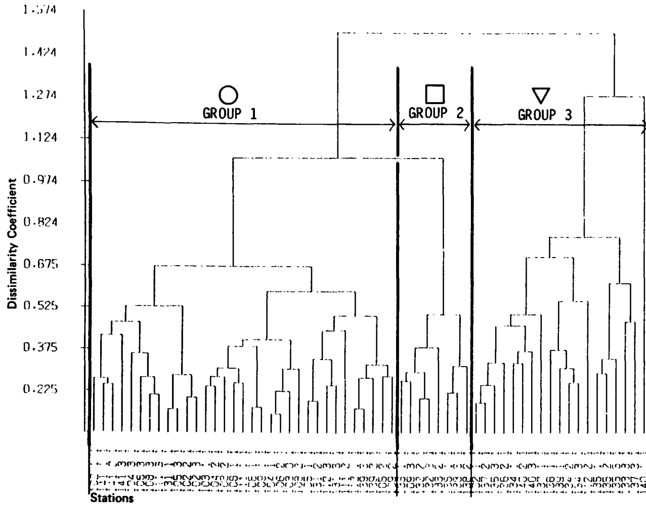
Figure 44a. Cluster Analysis Dendrogram for Samples (station replicates) of May 1979 Macrofauna Abundances, Code C2C1
