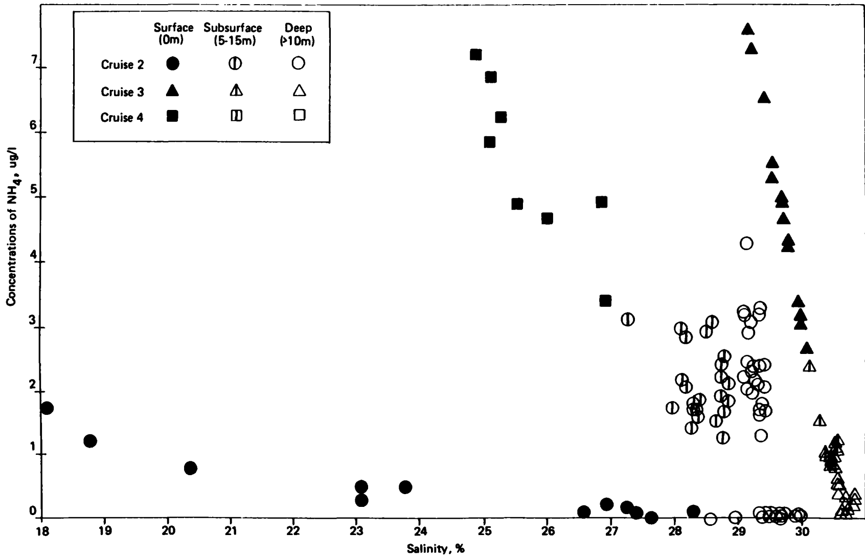
Figure 70. Concentrations of NH 4 in the Water Column as a Function of Salinity, Cruises 2, 3, and 4
