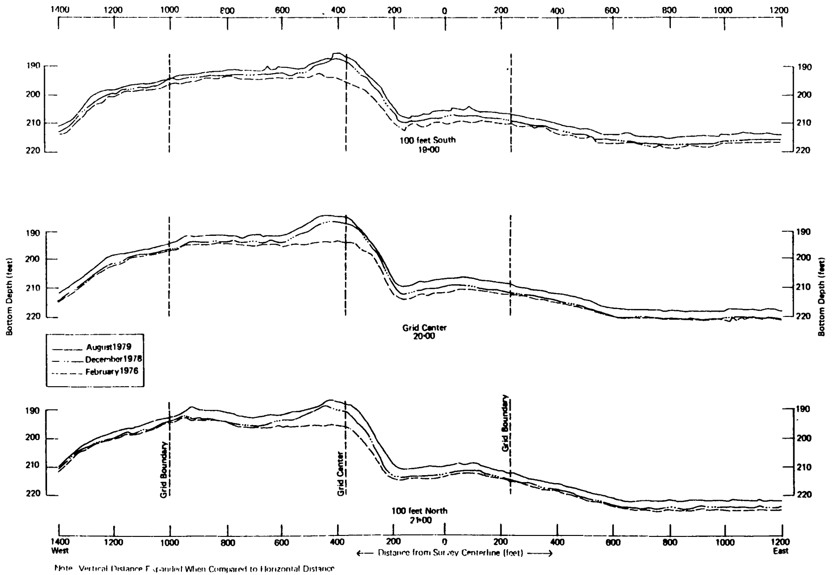
Figure 34. East-West Transects Through the Disposal Site
