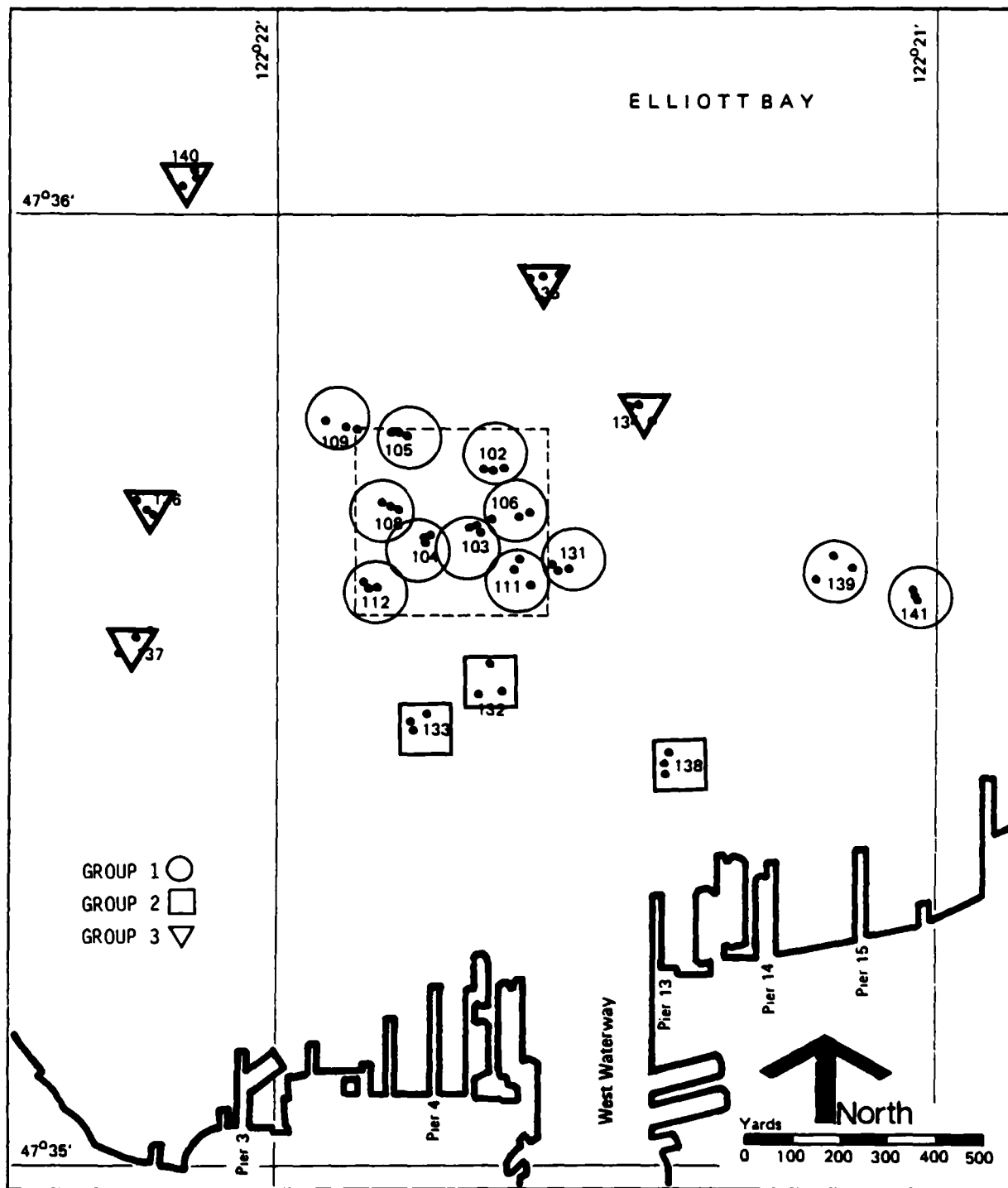
Figure 45b. Cluster Analysis Groupings for Station Means and Medians of May 1979 Macrofauna Abundances, Code C2MC
