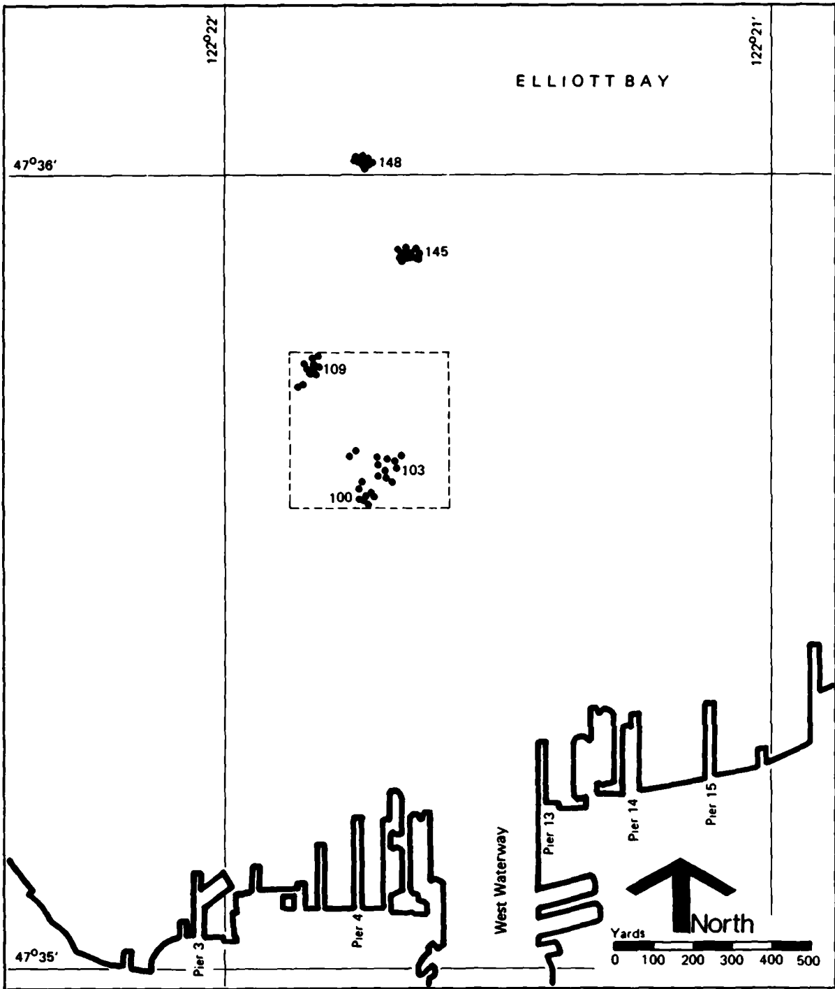
Figure 14. Station Locations (October 1979 Cruise), Grab Samples for PCB Content of Biota
