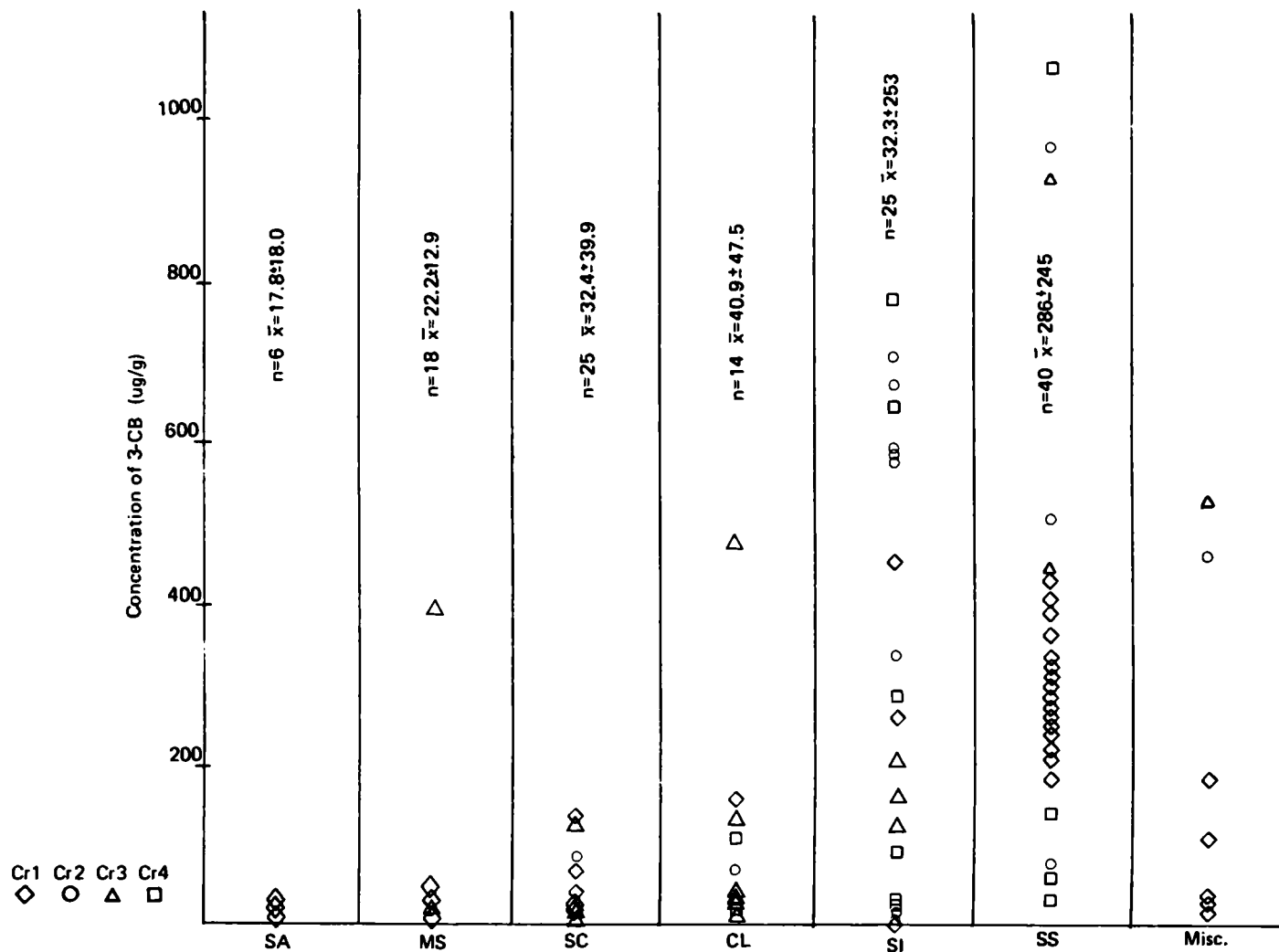
Figure 57. Histogram Showing Relationship of 3-CB Concentration to Sediment Type. Sediment types are defined in Table 1. Mean 3-CB concentrations and numbers of samples (n) are also included for each sediment type. Data are from the reconnaissance cruise \diamond ; May 1979, \circ ; October 1979, \triangle ; and May 1980, \square
