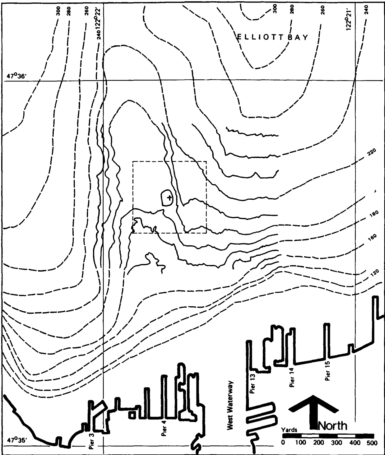
Figure 30. Bathymetric Map of the General Disposal Area. Central section denoted by solid lines was drawn from the detailed survey of December 1970; dashed lines represent extrapolation of data from standard National Ocean Survey nautical chart. Original sampling grid is denoted by dashed square near the middle of the figure
