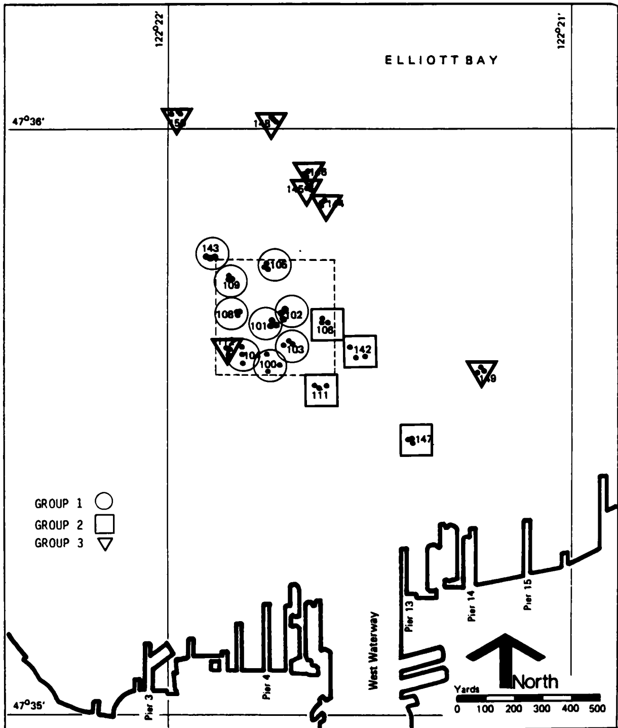
Figure 47c. Cluster Analysis Groupings for Station Medians of October 1979 Macrofauna Abundances, Code C3MDC
