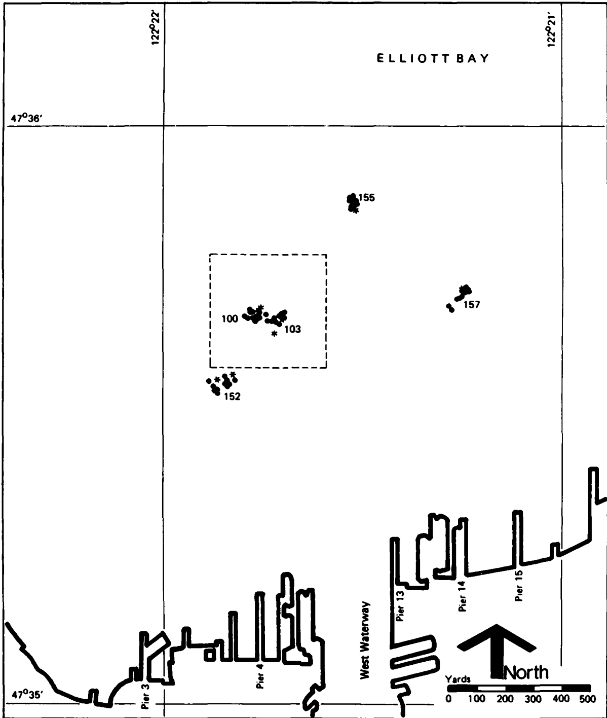
Figure 18. Station Locations (May 1980 Cruise), Samples for PCB Content of Sediments * and Interstitial Water•
