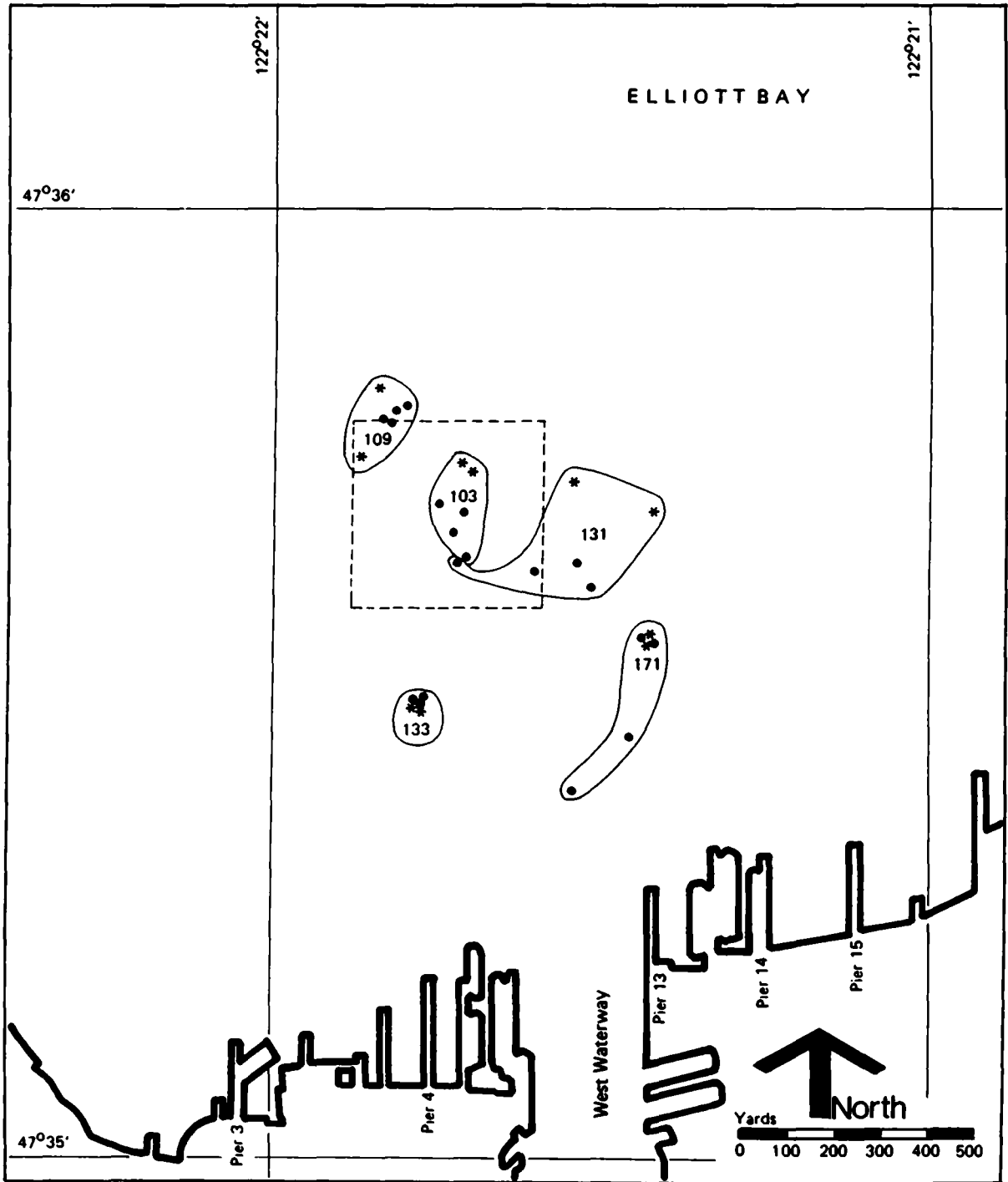
Figure 10. Station Locations (May 1979 Cruise), Water Samples for PCB Content of Water • and Suspended Particulate Matter and Hydrocasts*
