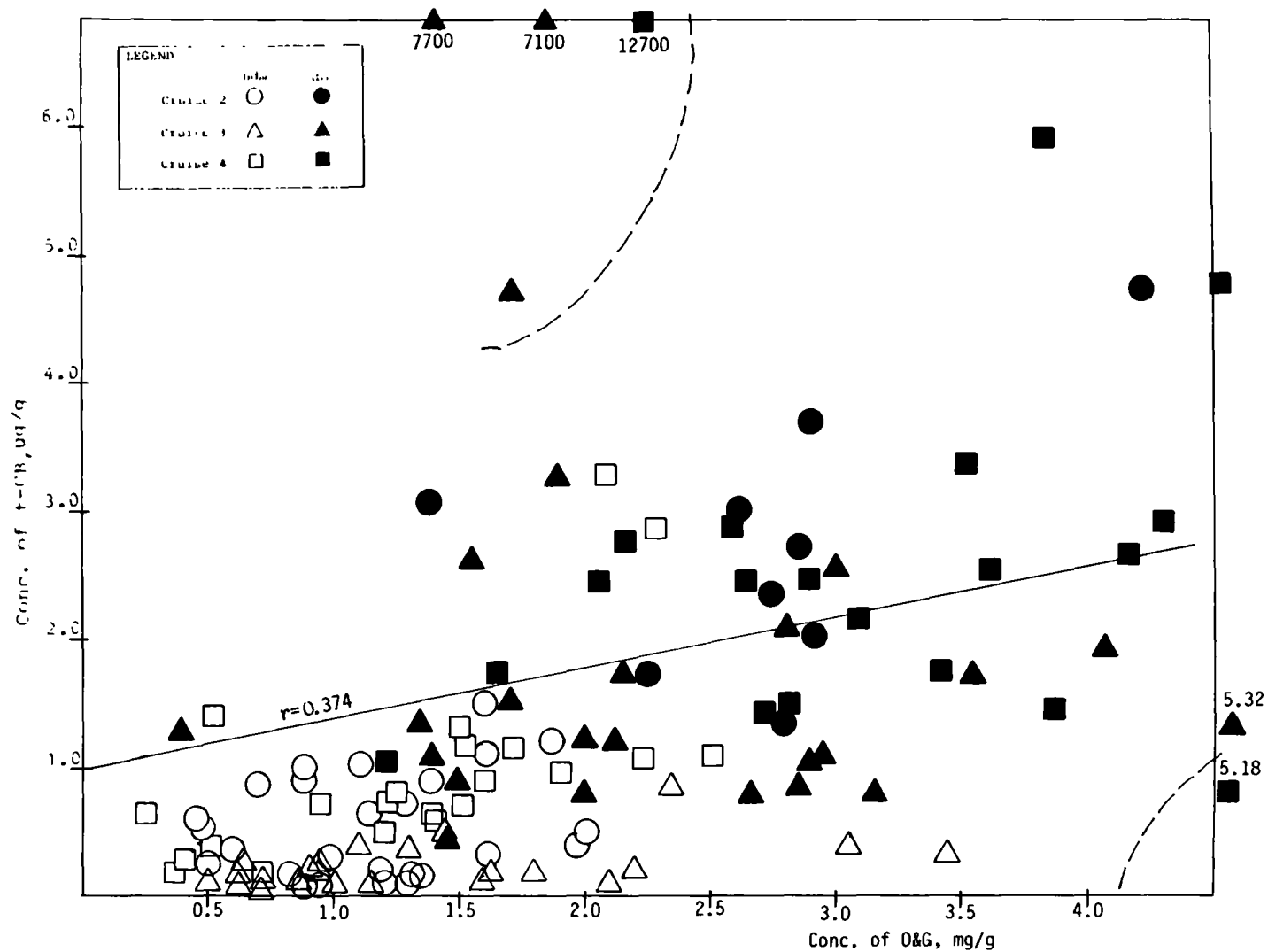
Figure 67. Plot of the Concentrations of t-CB Versus the Concentrations of O&G in the Sediments. The solid line represents the linear correlation line for the dredged material samples, excluding the outliers separated by the dashed lines
