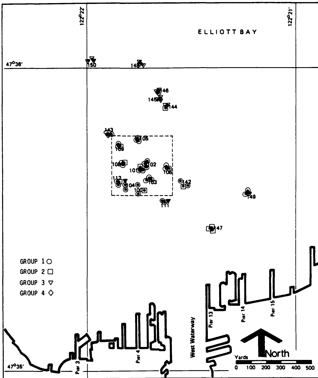
Figure 48a. Cluster Analysis Groupings for Samples (Station Replicates) of October 1979 Macrofauna Biomasses, Code C3W1
