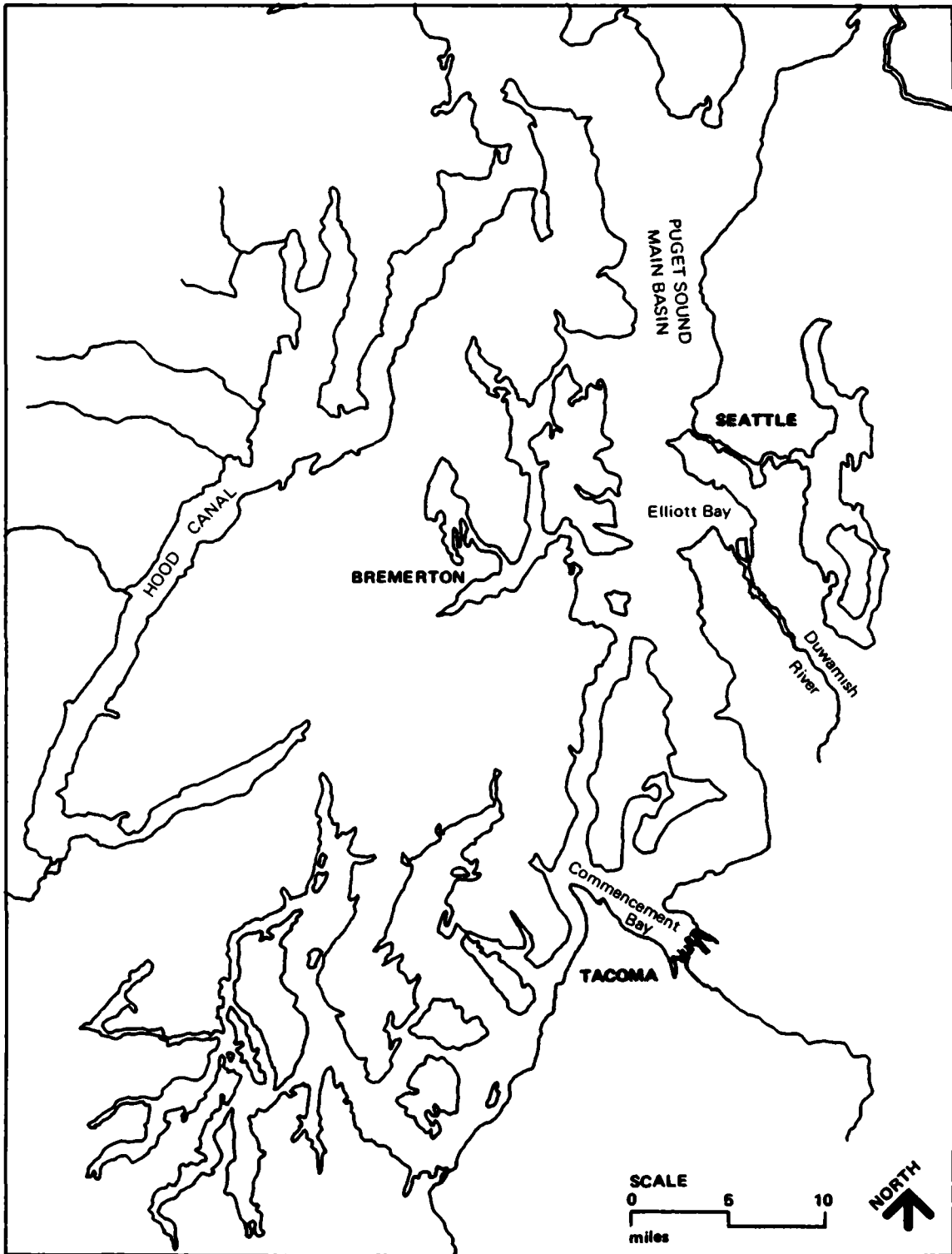
Figure 1. Elliott Bay Location Map
