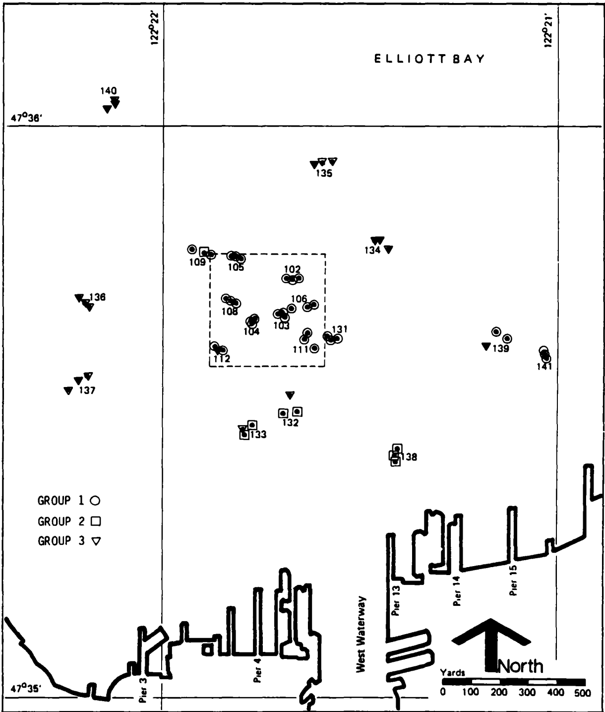
Figure 45a. Cluster Analysis Groupings for Samples (Station Replicates) of May 1979 Macrofauna Abundances, Code C2C1
