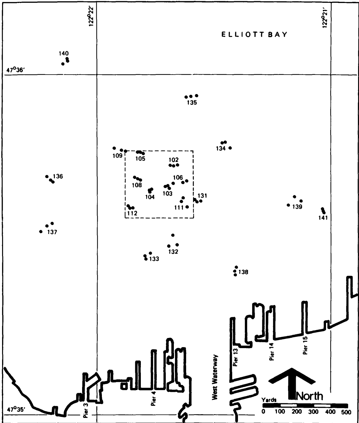
Figure 6. Station Locations (May 1979 Cruise), Grab Samples for Benthic Fauna Characterization
