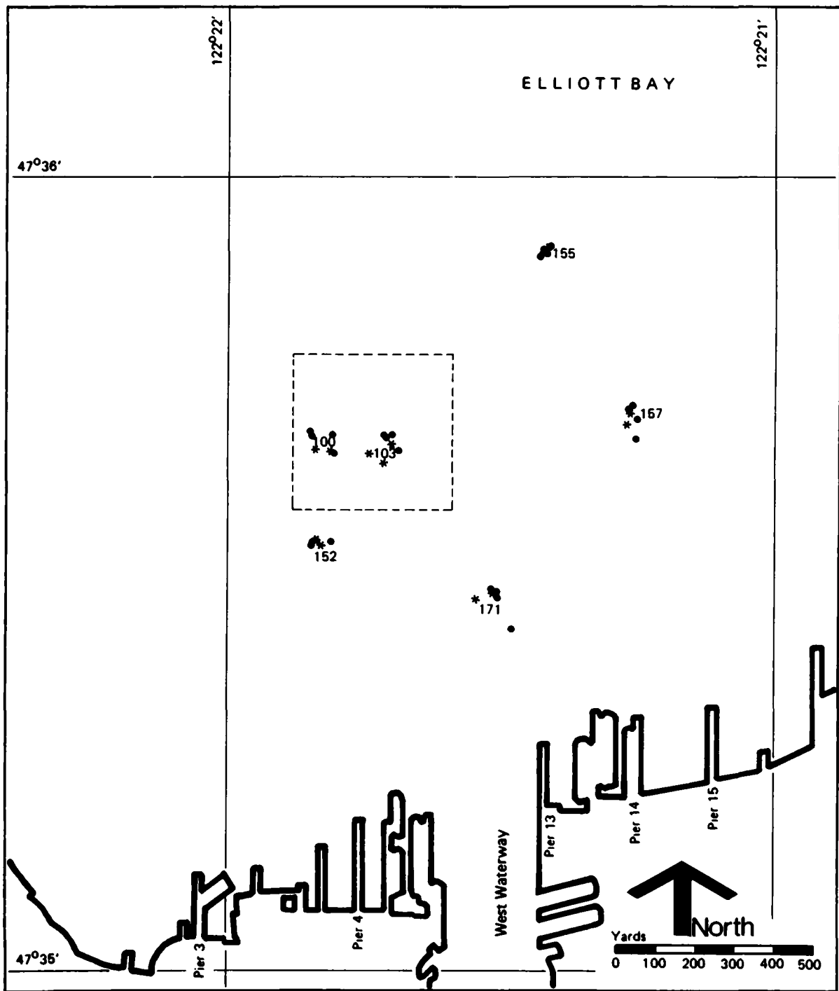
Figure 20. Station Locations (May 1980 Cruise), Water Samples for PCB Content of Water • and Suspended Particulate Matter and Hydrocasts *
