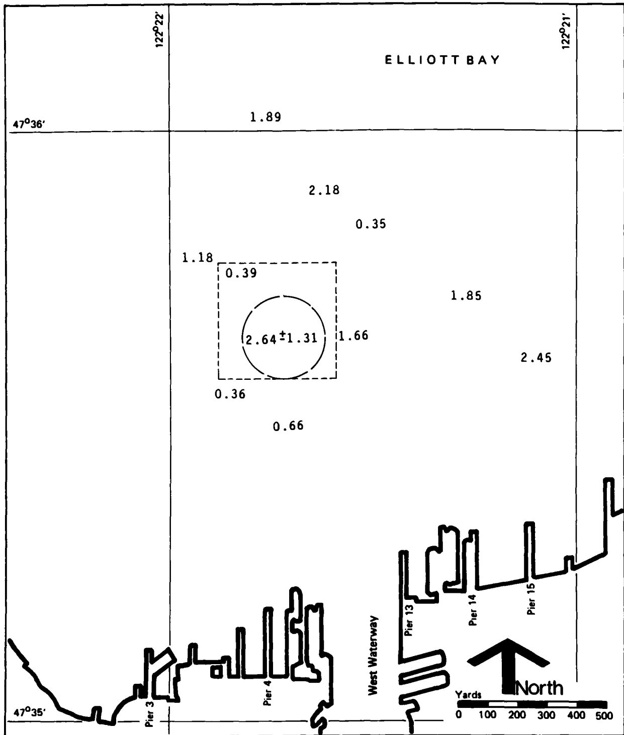
Figure 62. Spatial Distribution of O&G in the Surface Sediments. O&G values represent station averages for non-dredged material stations and as mean of disposal site sediments, units: mg O&G/g dry sediment
