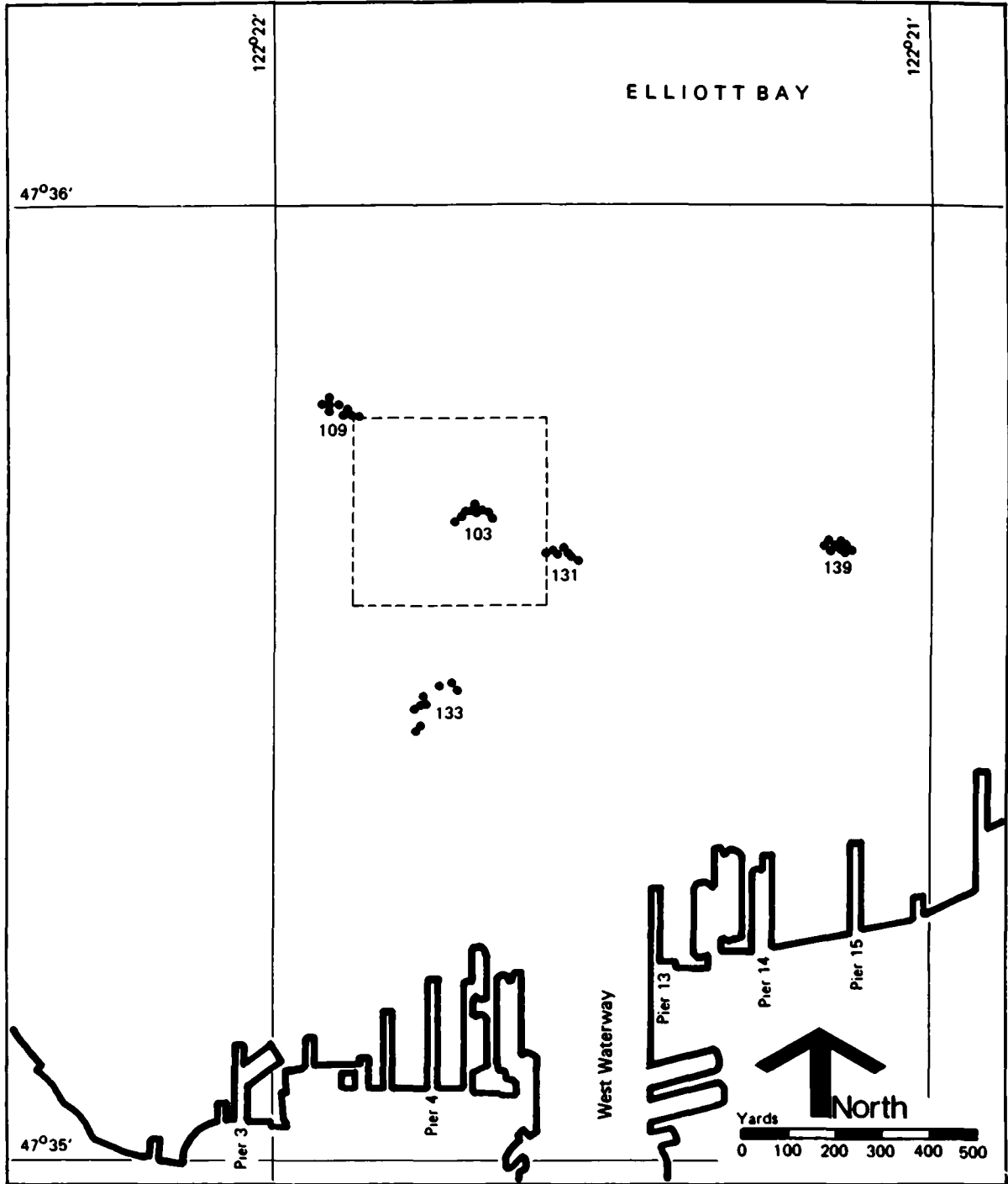
Figure 9. Station Locations (May 1979 Cruise), Grab Samples for PCB Content of Biota
