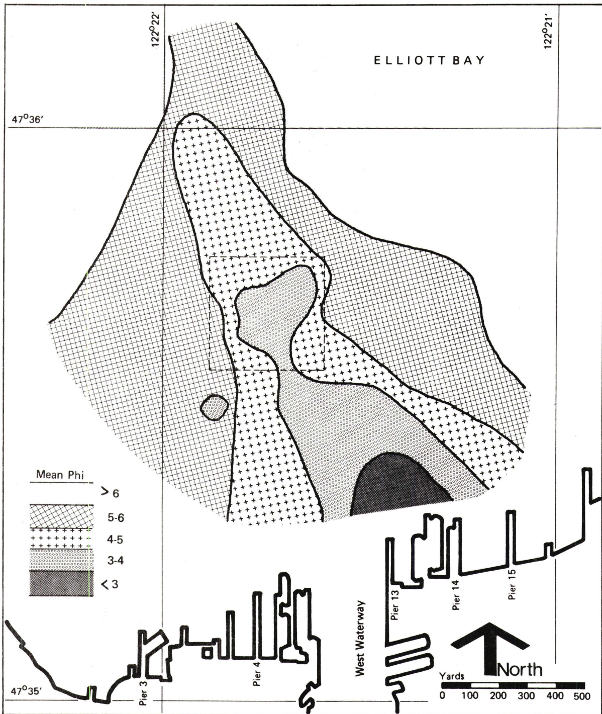
Figure 38. Distribution of the Mean Phi of the Predisposal Surface Layer. Based on the MS Subsurface Horizon
