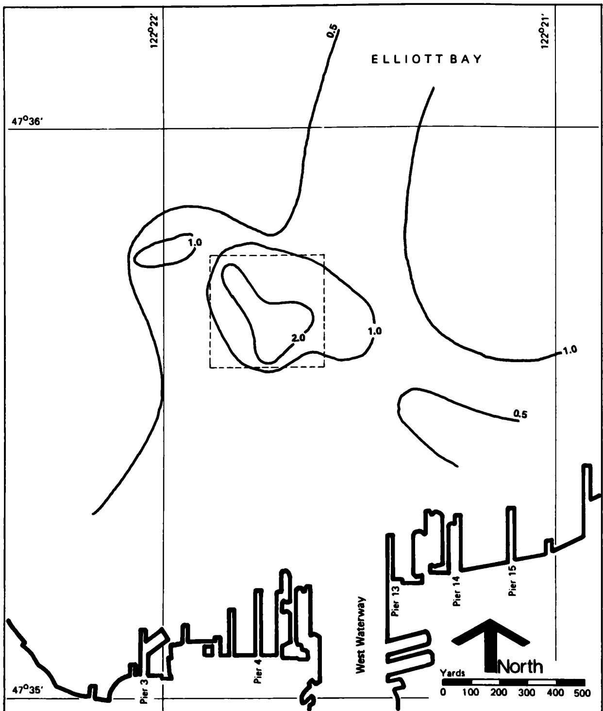
Figure 54. Concentration Contours of the Approximate Distribution of t-CB in the Surface Sediments. Concentrations in units of ug/g
