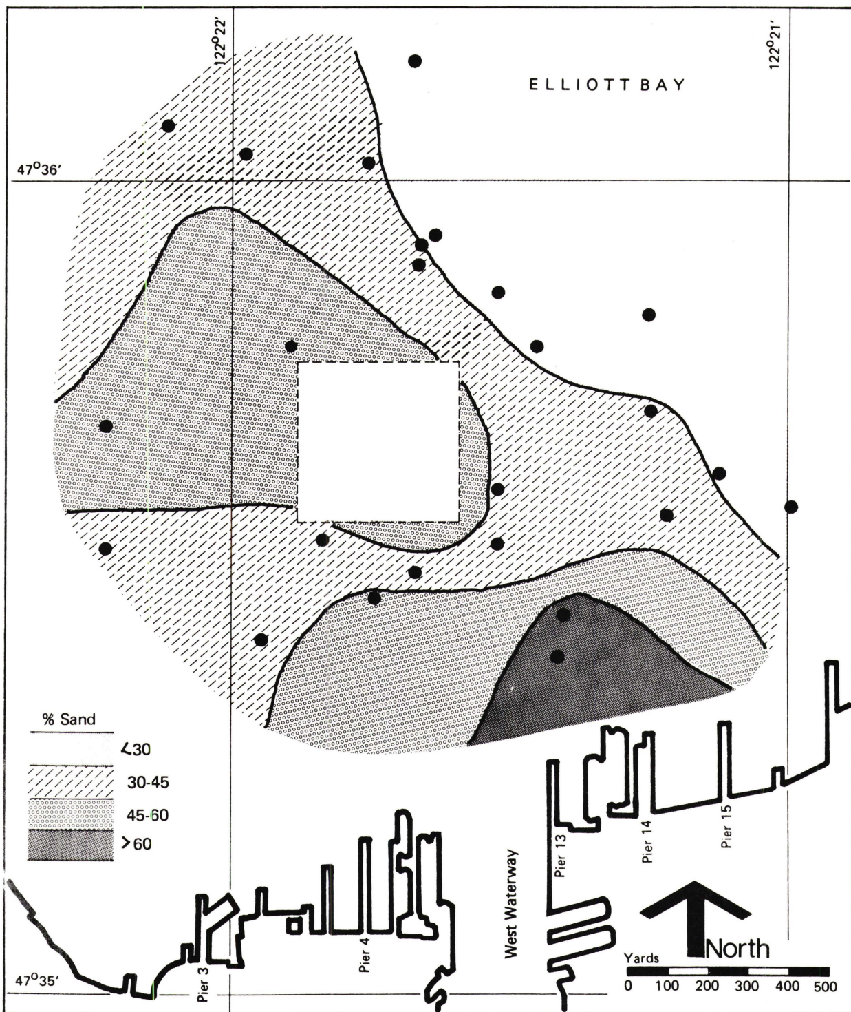
Figure 36. Distribution of Percent Sand for Stations Outside the Grid Area. Station means for Cruises 2, 3, and 4 are plotted
