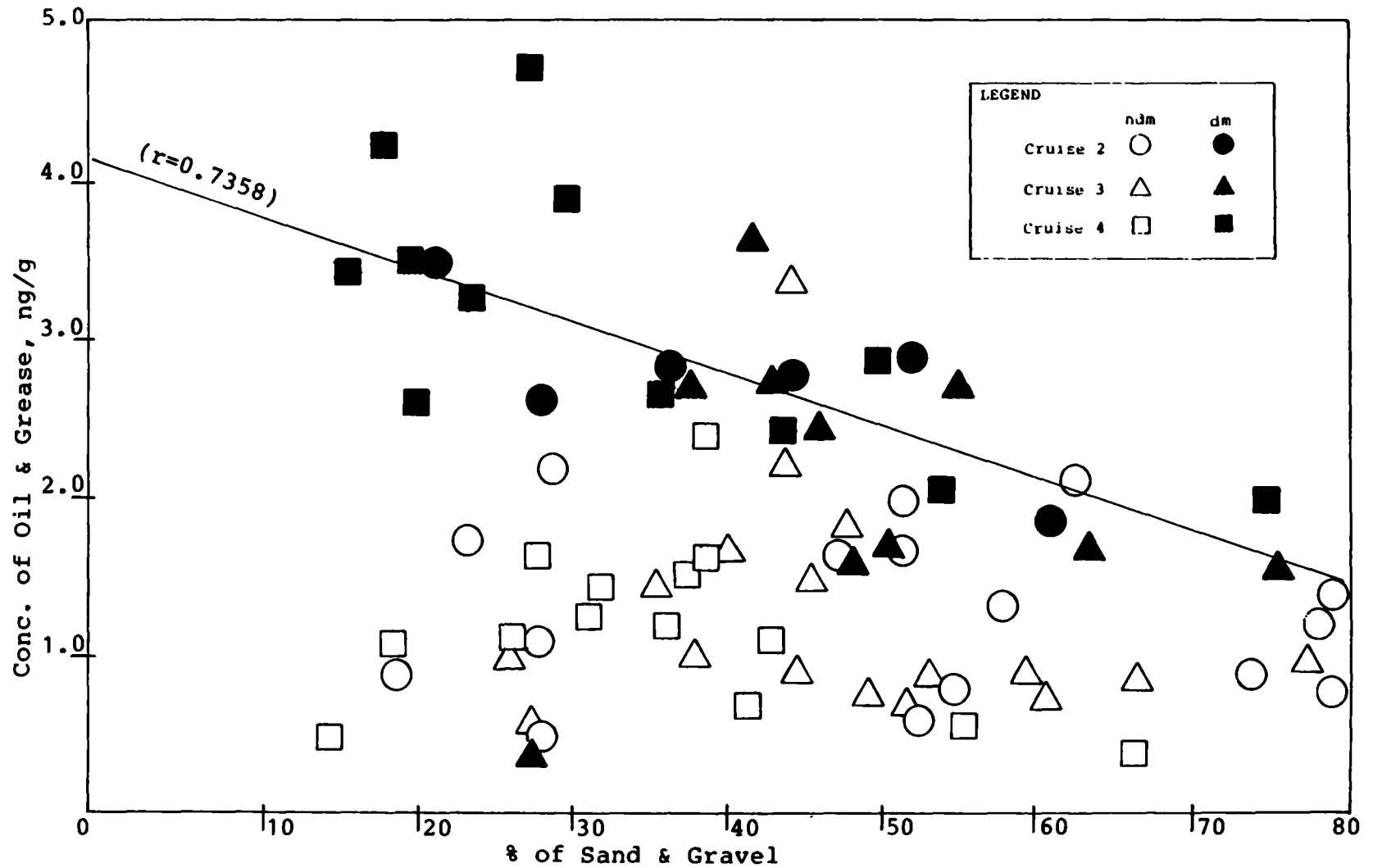
Figure 65. Plots of the Concentrations of O&G Versus the Grain Size of the Sediments. Sediment texture is expressed as the percent of sand and gravel ( \%_{<4\phi} ). The solid line depicts the linear regression correlation for the dredged material
