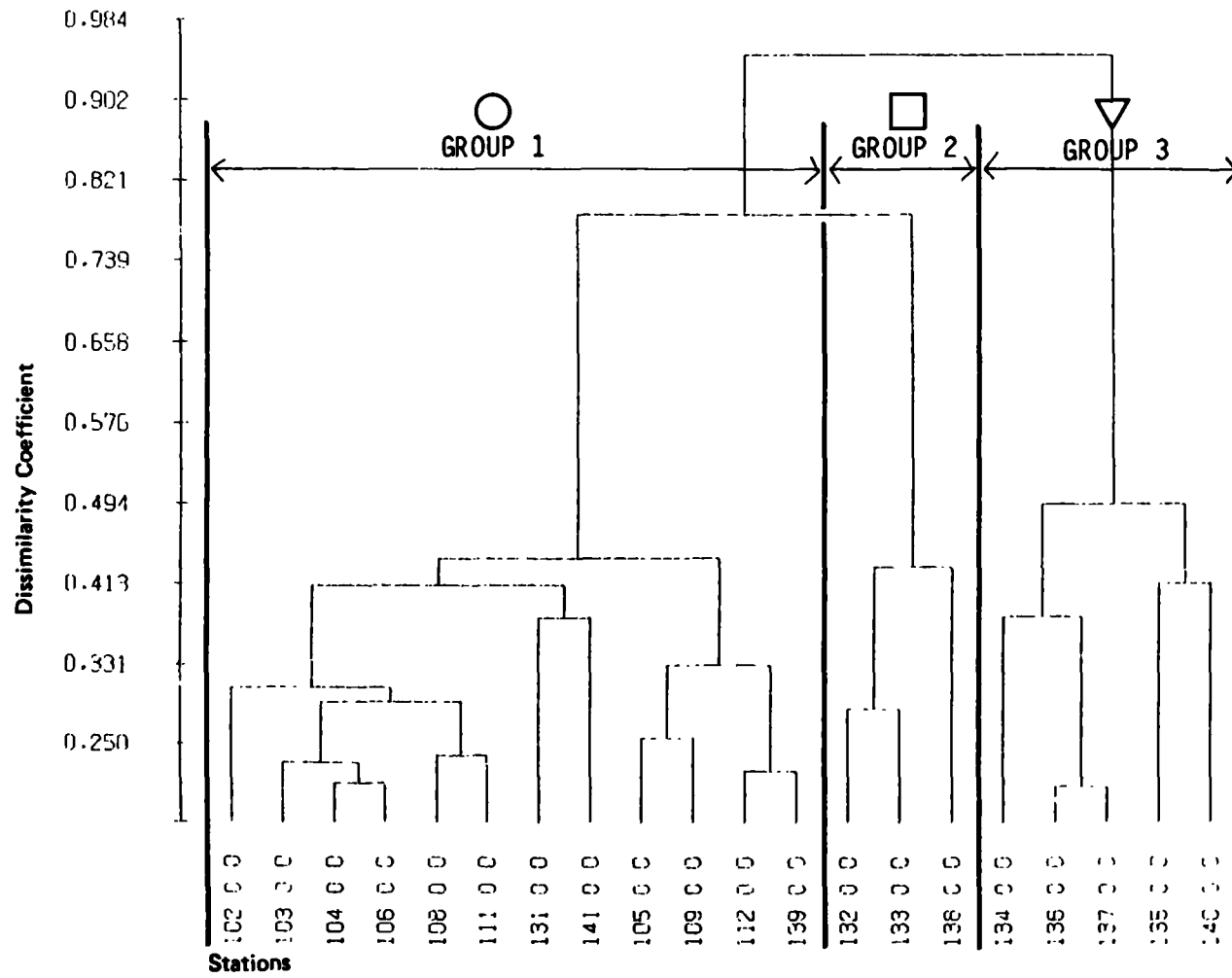
Figure 44c. Cluster Analysis Dendrogram for Station Medians of May 1979 Macrofauna Abundance, Code C2MC
