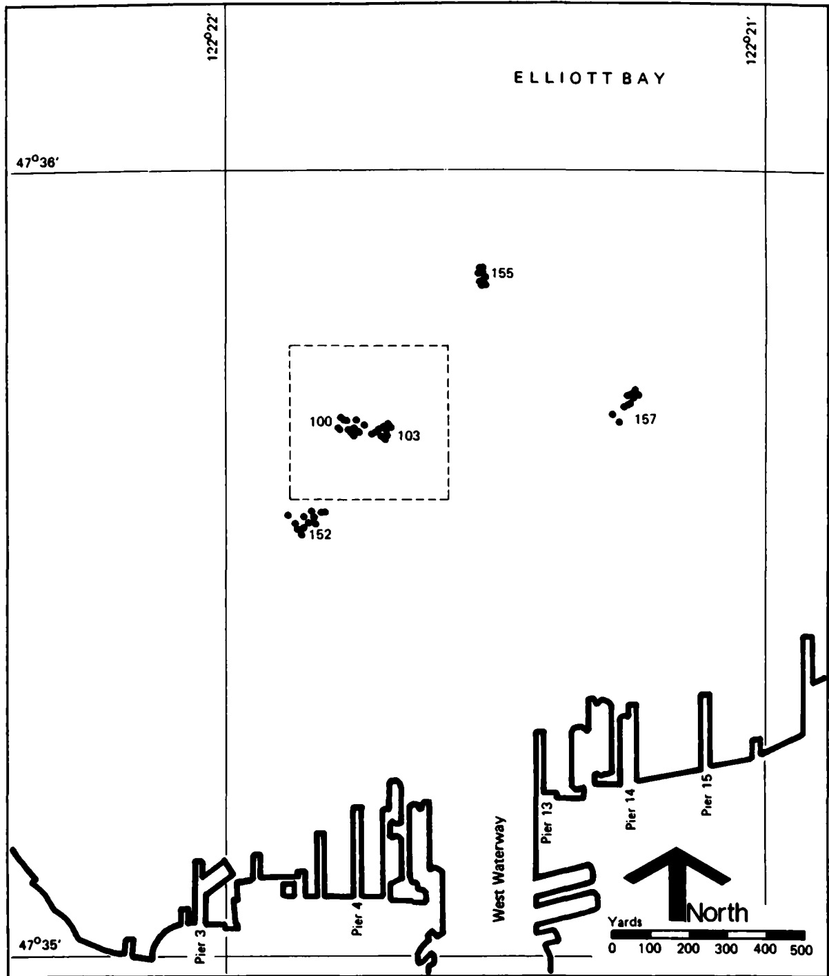
Figure 19. Station Locations (May 1980 Cruise), Grab Samples for PCB Content of Biota
