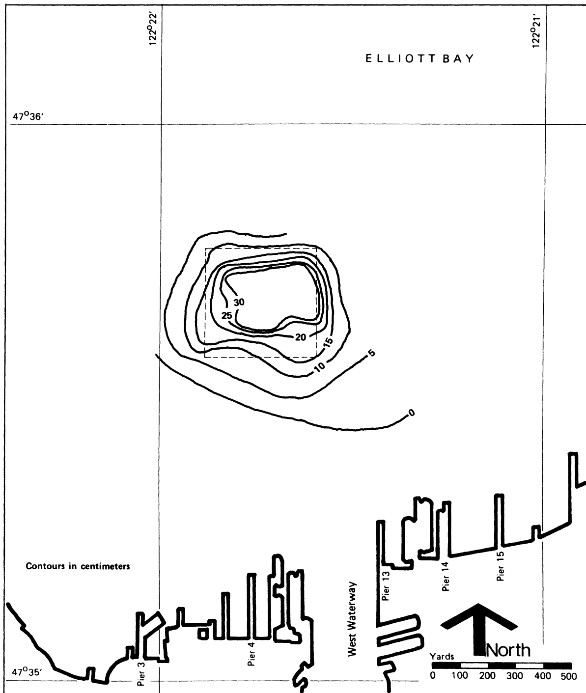
Figure 37. Contour Plot of the Depth of the MS Subsurface Horizon
