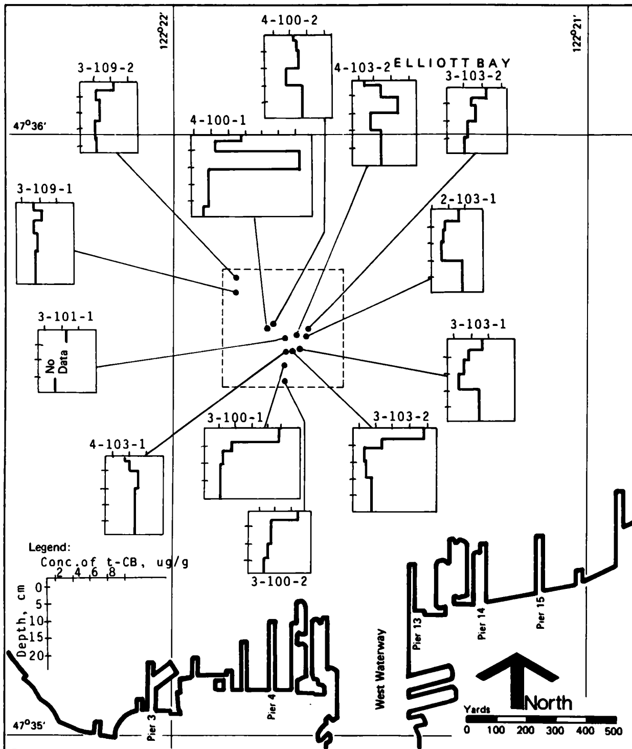
Figure 59. Depth Profiles of the t-CB Concentrations in the Dredged Material Cores. The core profiles are named as cruise-station-replicate number, and are keyed to the actual station locations
