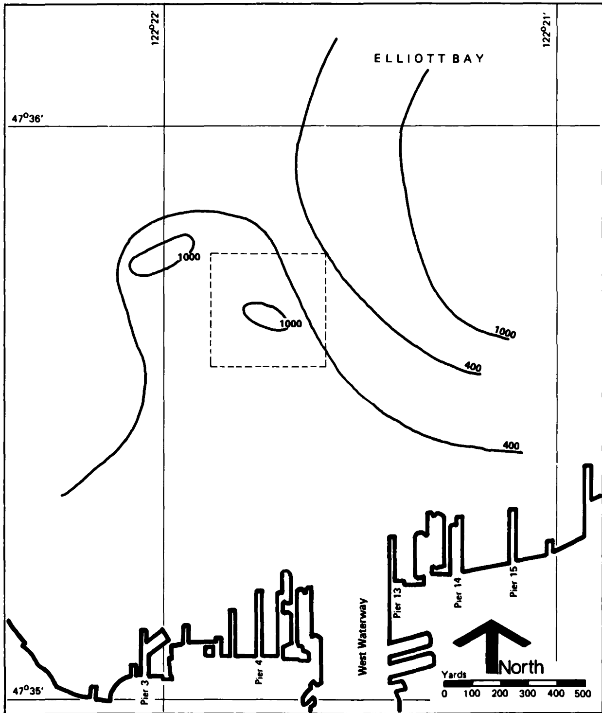
Figure 58. Contours of the Approximate Concentrations of t-CB in Background Sediments at the Disposal Site together with Surface Sediments at Non-Dredged Material Sites, Cruises 1, 2, 3, and 4. Concentrations are in units of nanograms
