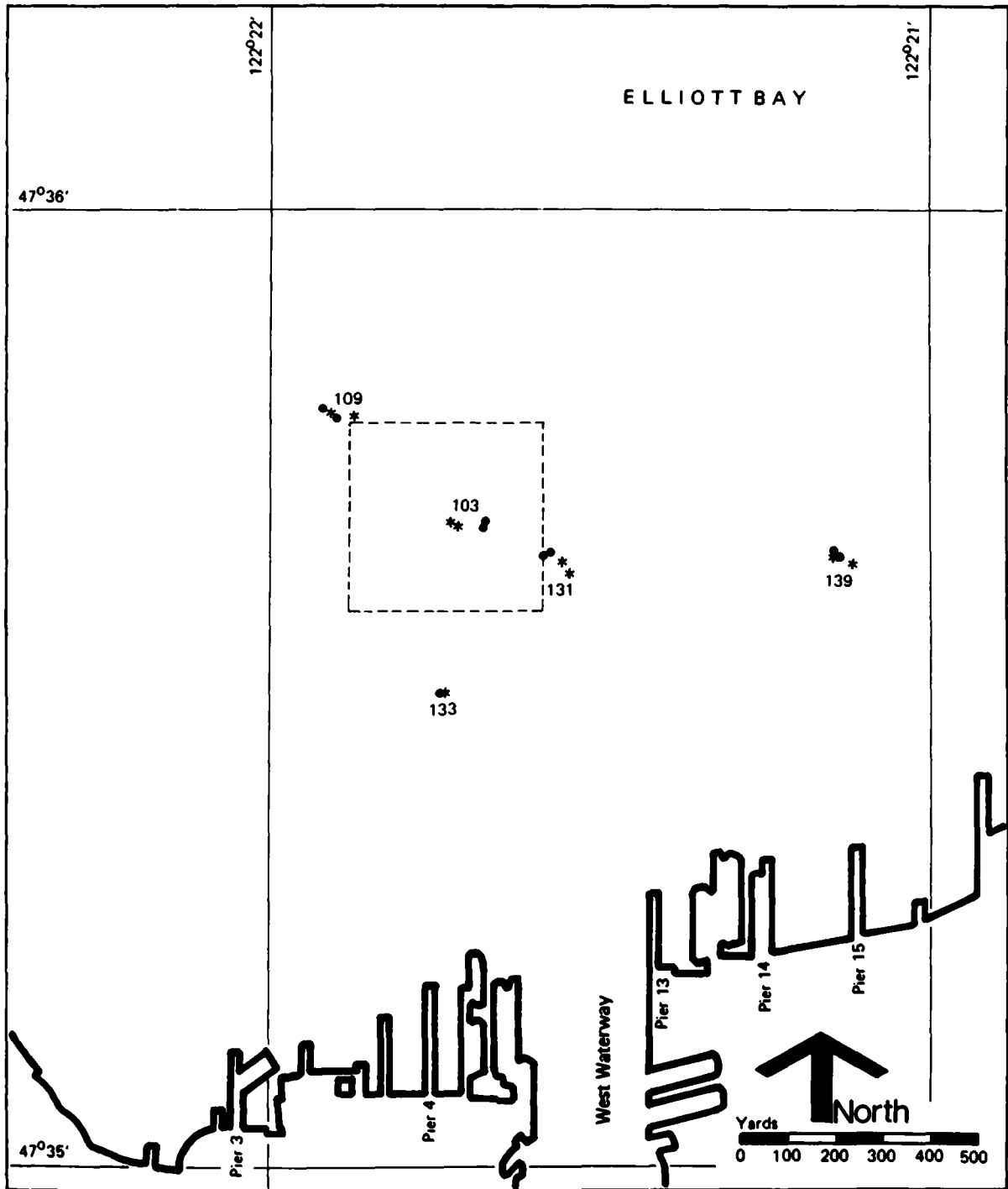
Figure 8. Station Locations (May 1979 Cruise), Samples for PCB Content of Sediments • and Interstitial Water *
