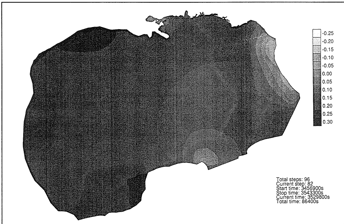
Figure 12. Surface elevation contours for the Gulf of Mexico shown using XMVIS
