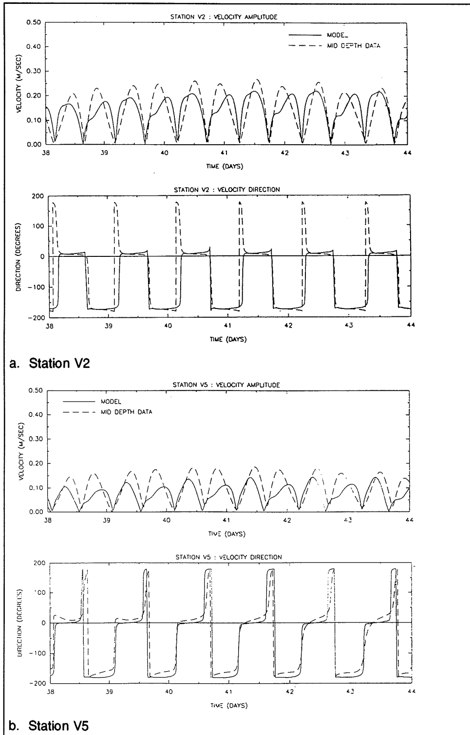
Figure 11. Comparisons of time histories of computed velocities and time histories of synthesized velocities from harmonically decomposed measured constituent data (using K_1 , O_1 , M_2 and N_2 ) at representative current stations within the Mississippi Sound (Sheet 1 of 3)
