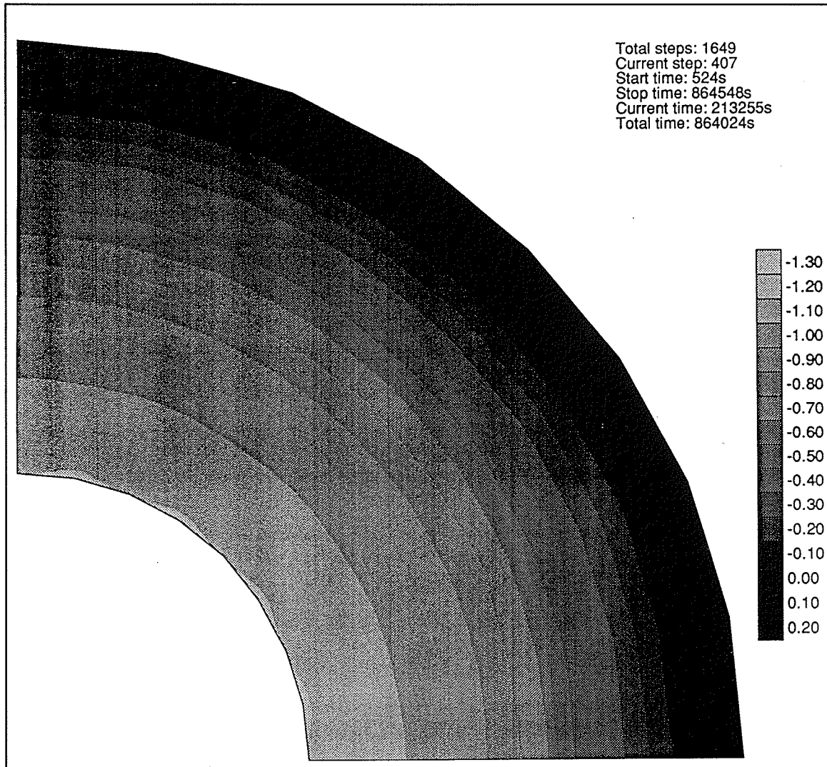
Figure 6. Surface elevation contours for the quarter annular case shown using XMVIS
