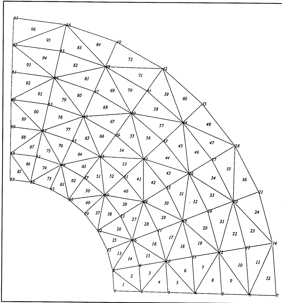
Figure 2. Finite element discretization of the quarter annular test problem showing node and element numbers
