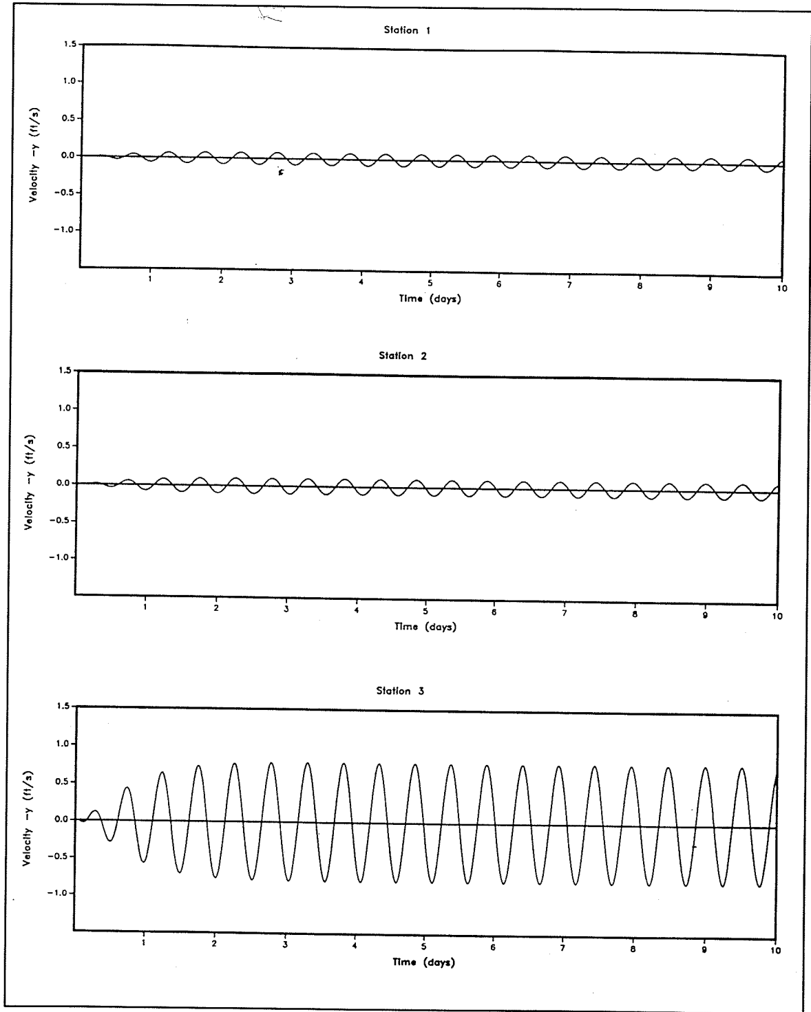
Figure 5. Time histories of the computed y component velocities at the three velocity recording stations
