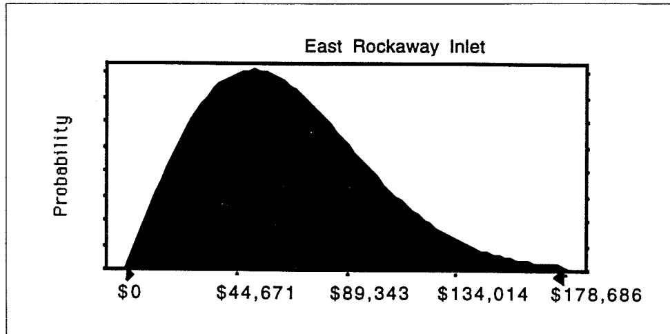
Figure 6. Example of Weibull distribution of O&M benefits for the East Rockaway Inlet project
