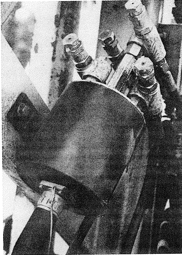
Figure 2. Close-up of pressure transducers showing DPR transducer housing for sensing drilling fluid pressure, pressure to hydraulic drive motor, downthrust and holdback pressures
