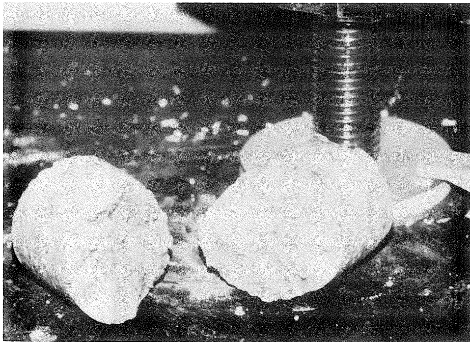
Figure 18. Typical diametrical point load sample after failure
