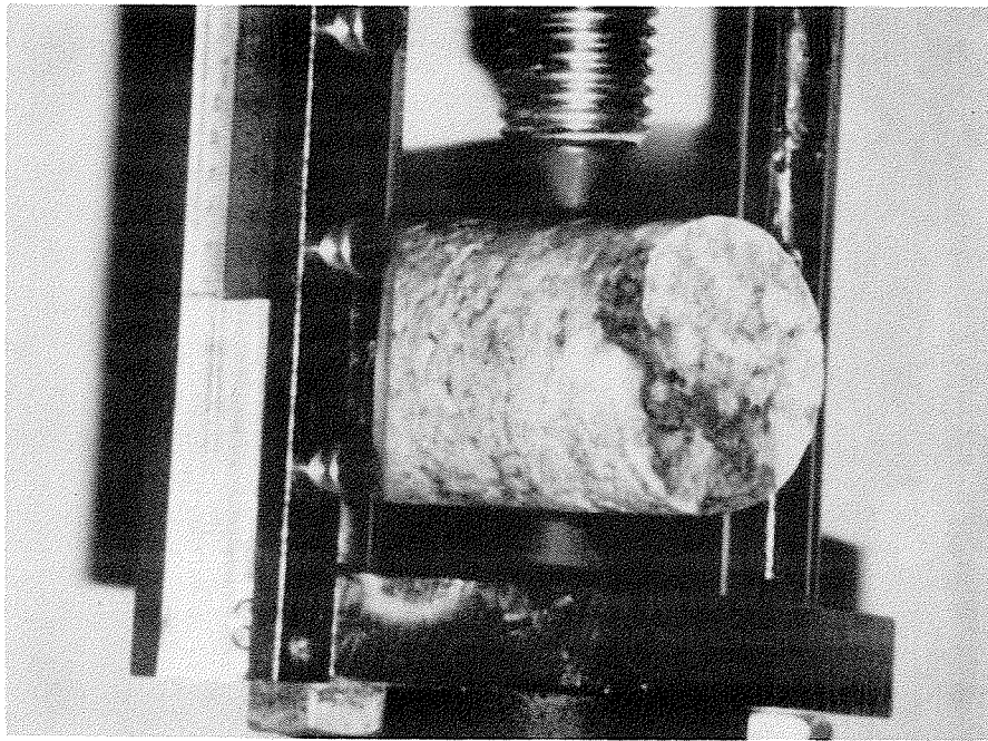
Figure 17. Diametrical point load sample under test (ends were sawn but could be irregular)
