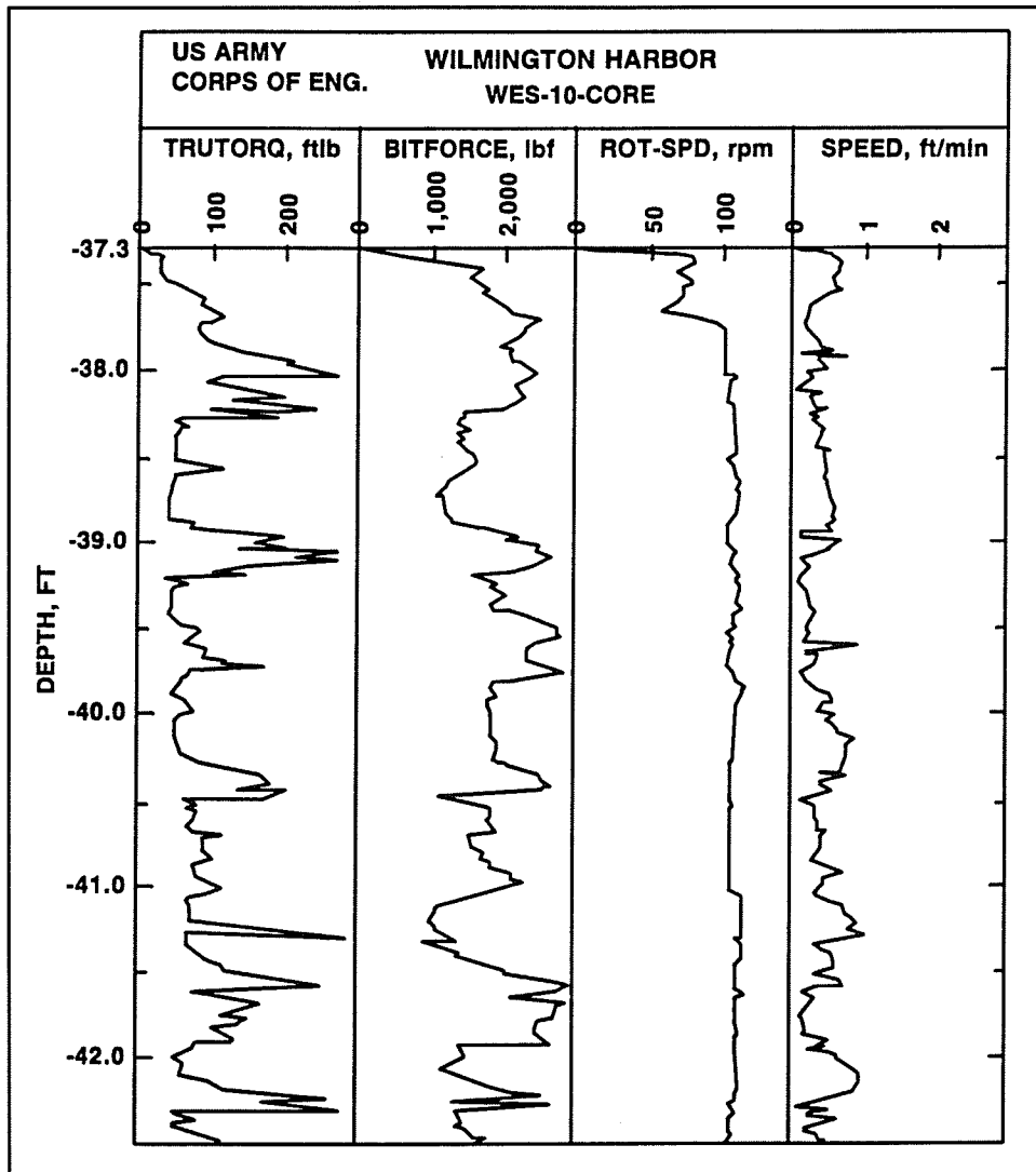
Figure 6. Calculated drill rig mechanical parameters from the raw data shown in Figure 5
