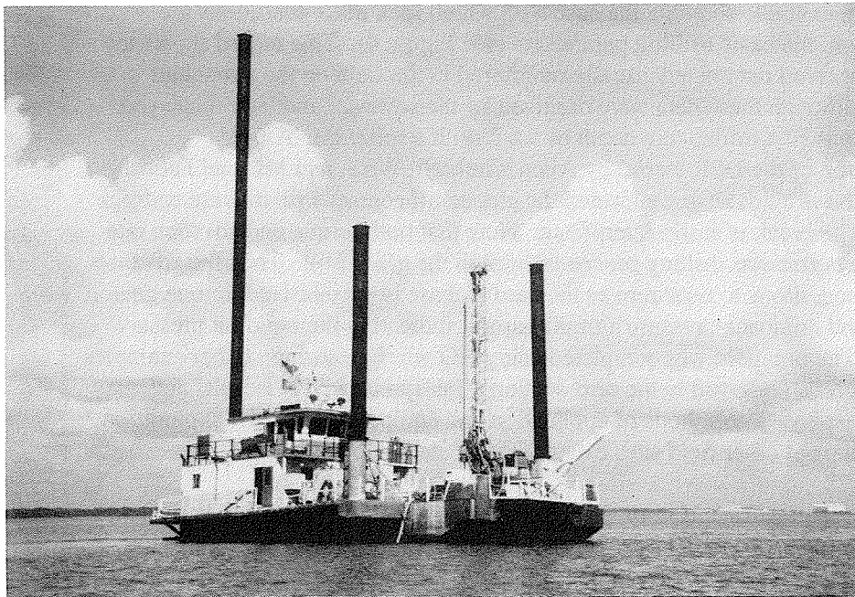
Figure 3. DPR exploration using the jack-up barge, Explorer, at Kings Bay, Georgia. Similar floating plant was used at New York Harbor
