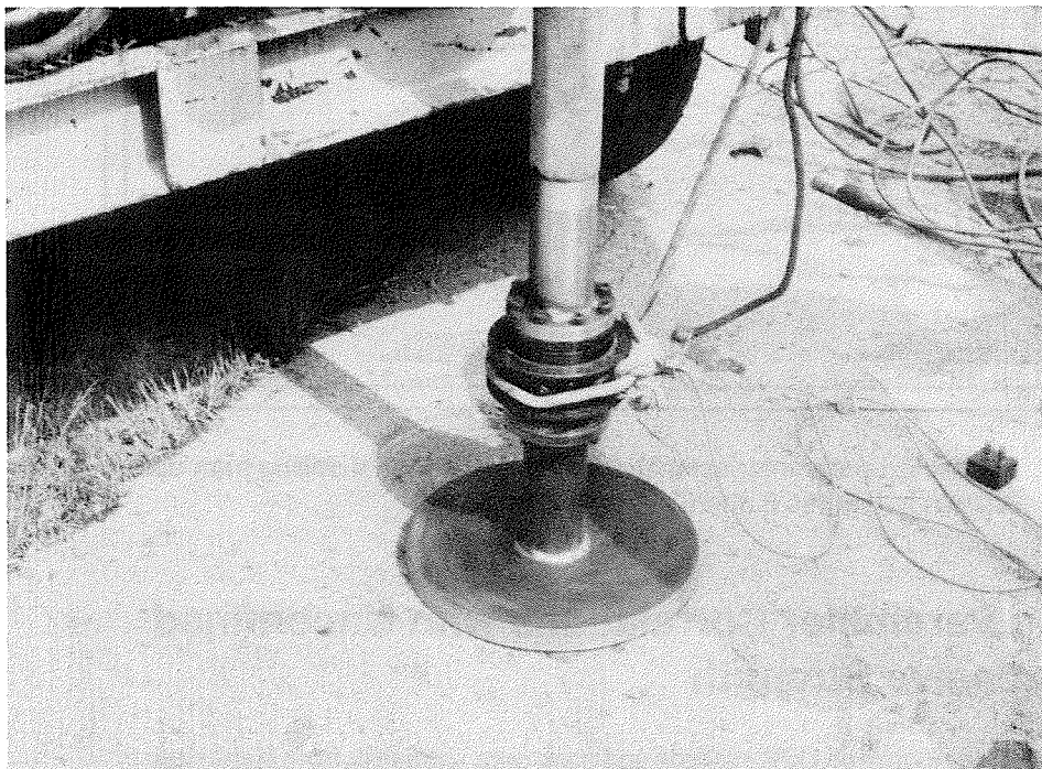
Figure 9. Close-up of torque cell and reaction disk
