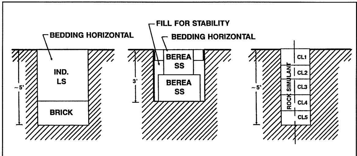
Figure 11. Rock and rock simulant setup for DPR laboratory drilling tests
