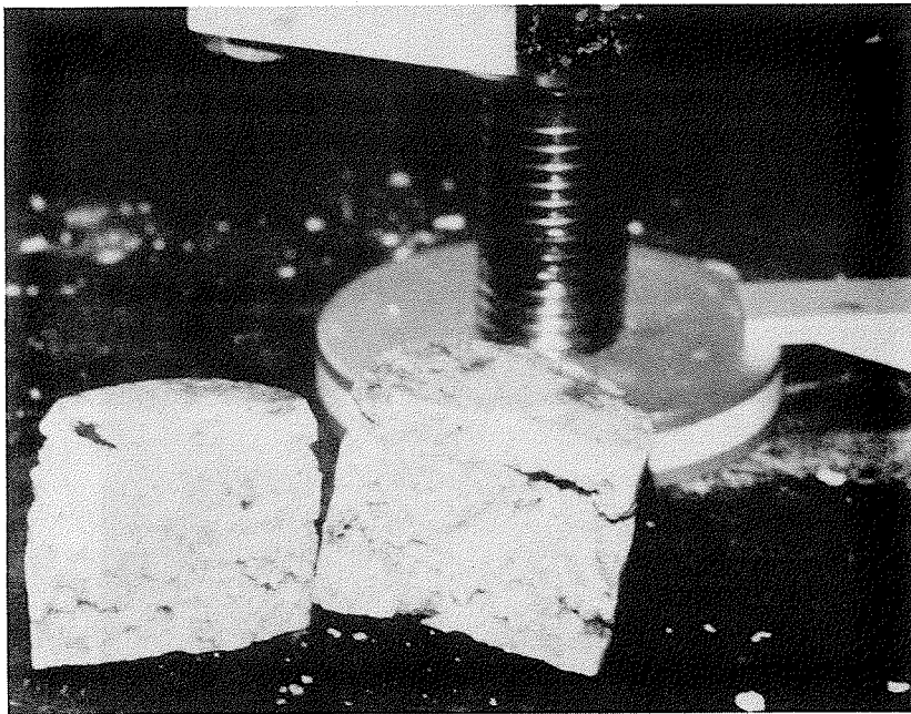
Figure 16. Typical axial point load sample after failure
