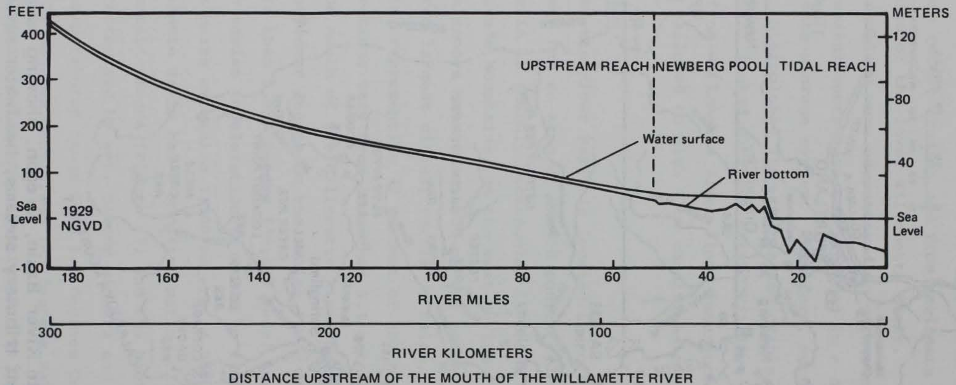
Figure 12. Water surface and bottom elevations of the Willamette River, Oregon, during the mid-July 1973 low-flow period (adapted from Rickert and others, 1977)
