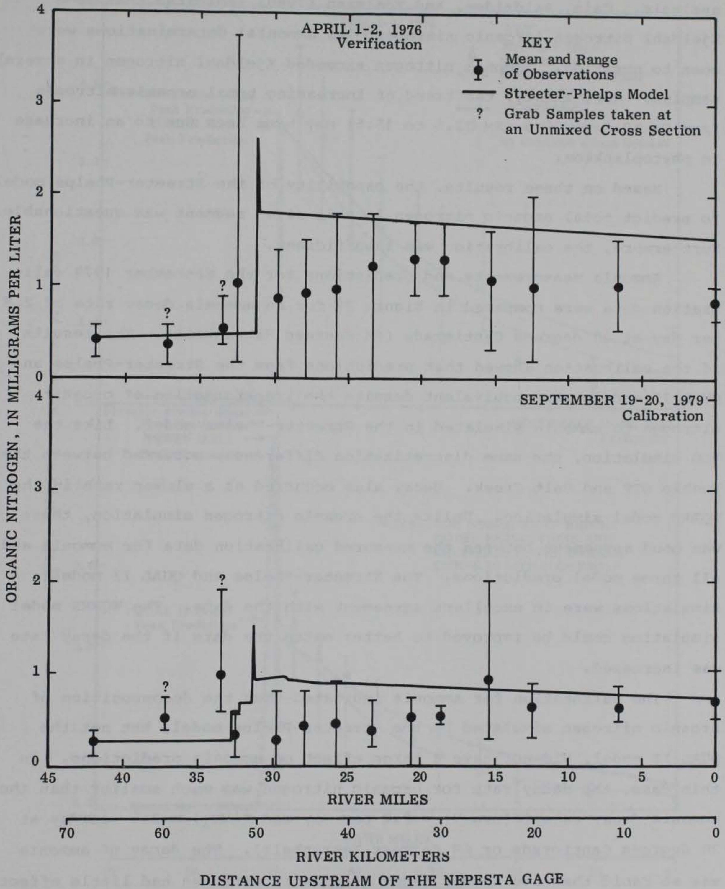
Figure 36. Observed and predicted organic nitrogen, Arkansas River
