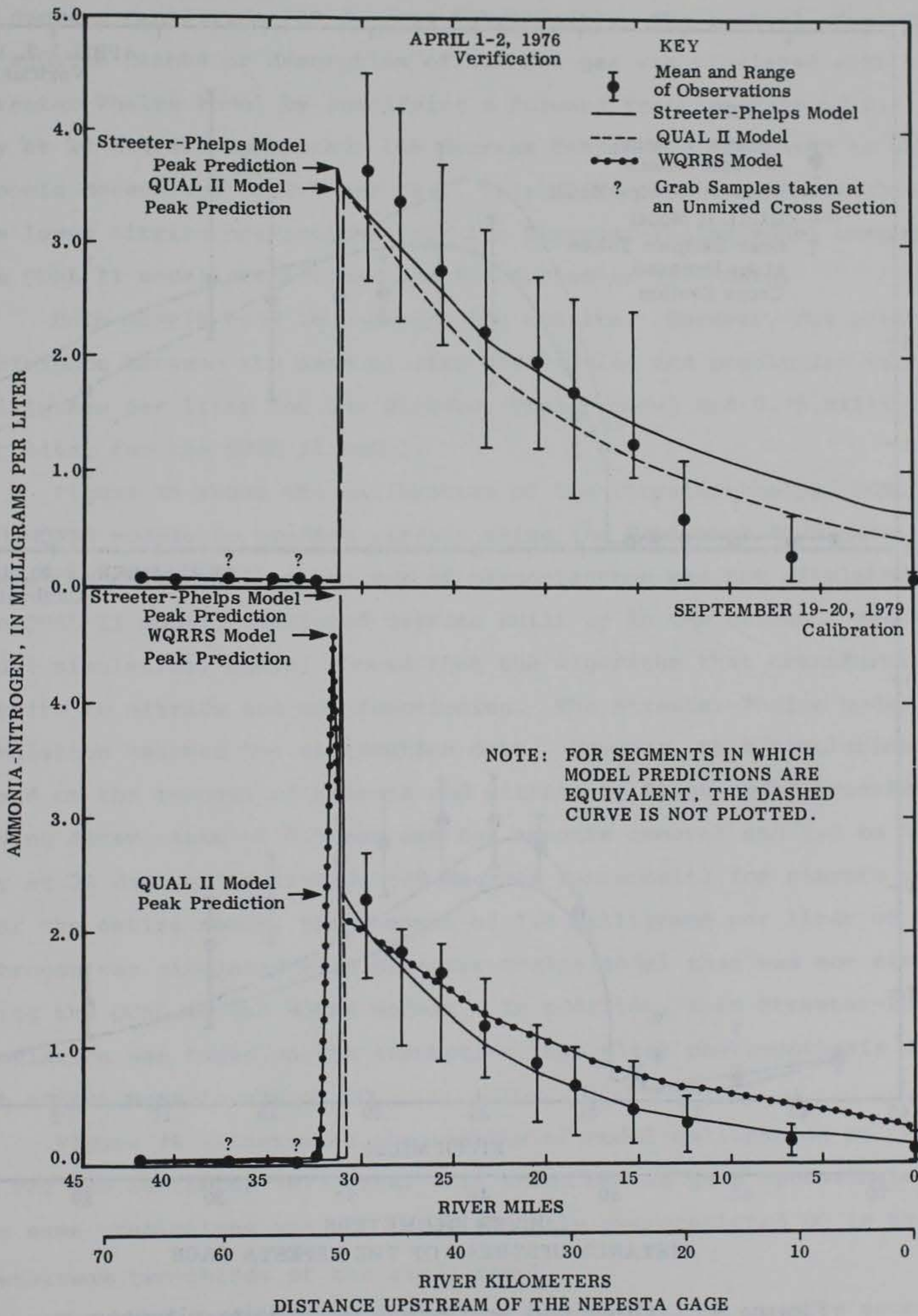
Figure 37. Observed and predicted ammonia-nitrogen, Arkansas River
