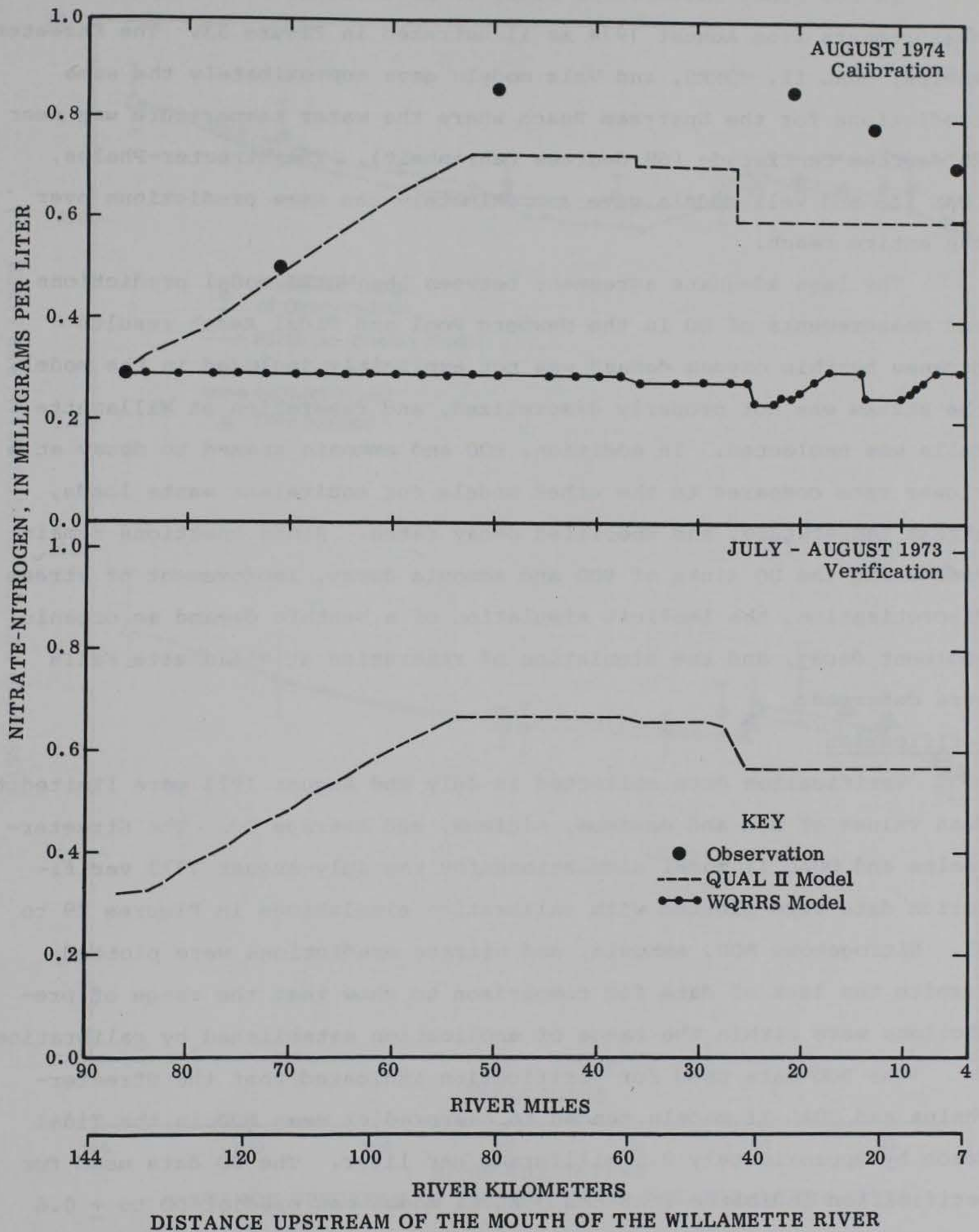
Figure 32. Observed and predicted nitrate-nitrogen, Willamette River
