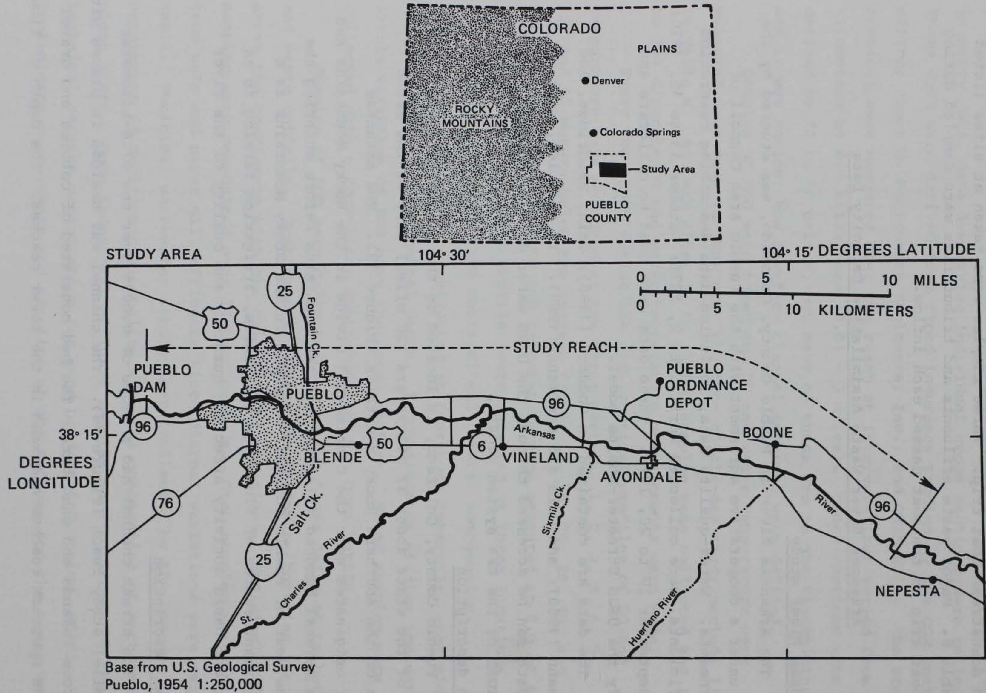
Figure 13. Arkansas River and significant tributaries between Pueblo Dam and Nepesta, Colorado (adapted from Goddard, 1980)
