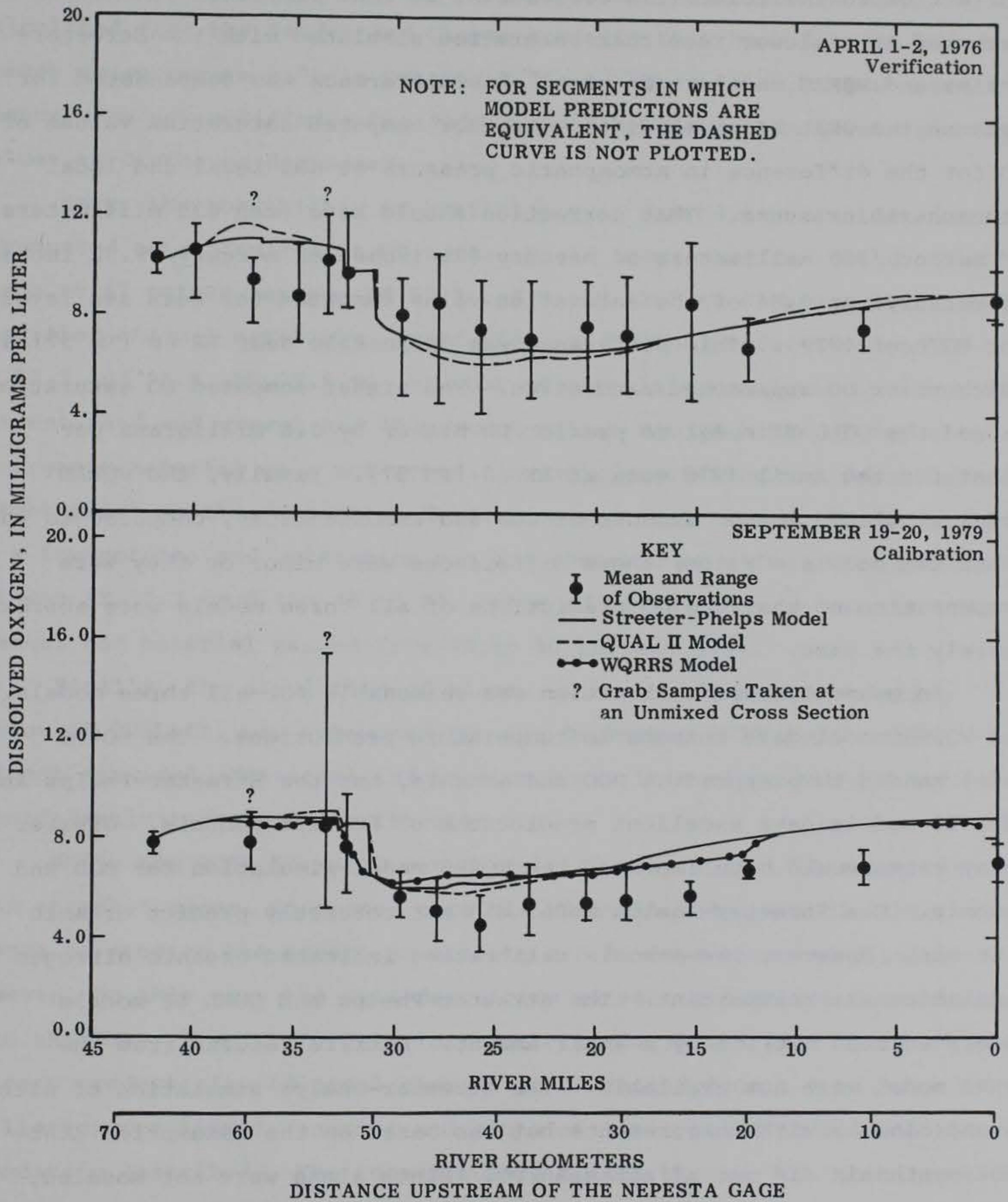
Figure 40. Observed and predicted dissolved oxygen, Arkansas River
