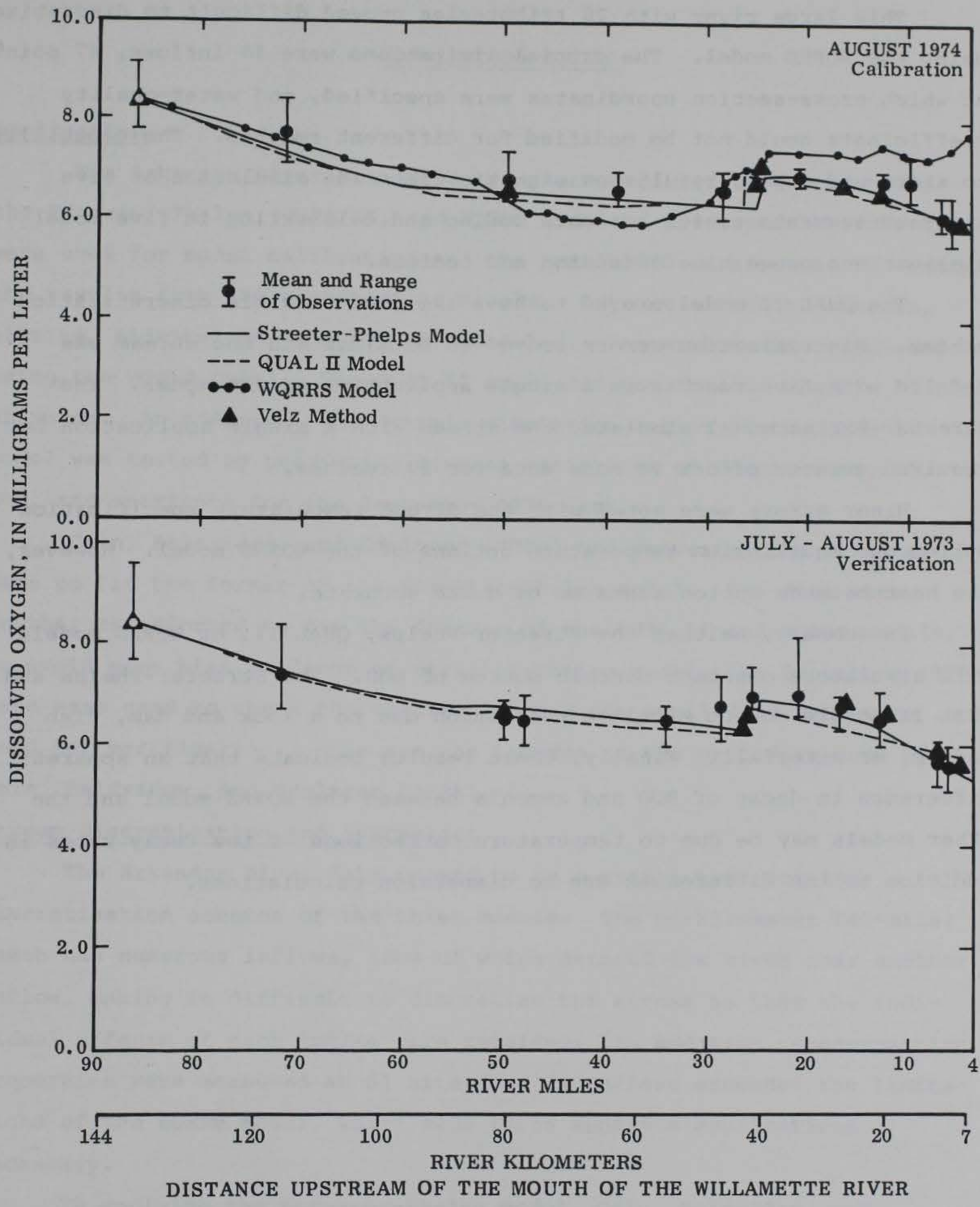
Figure 33. Observed and predicted dissolved oxygen, Willamette River
