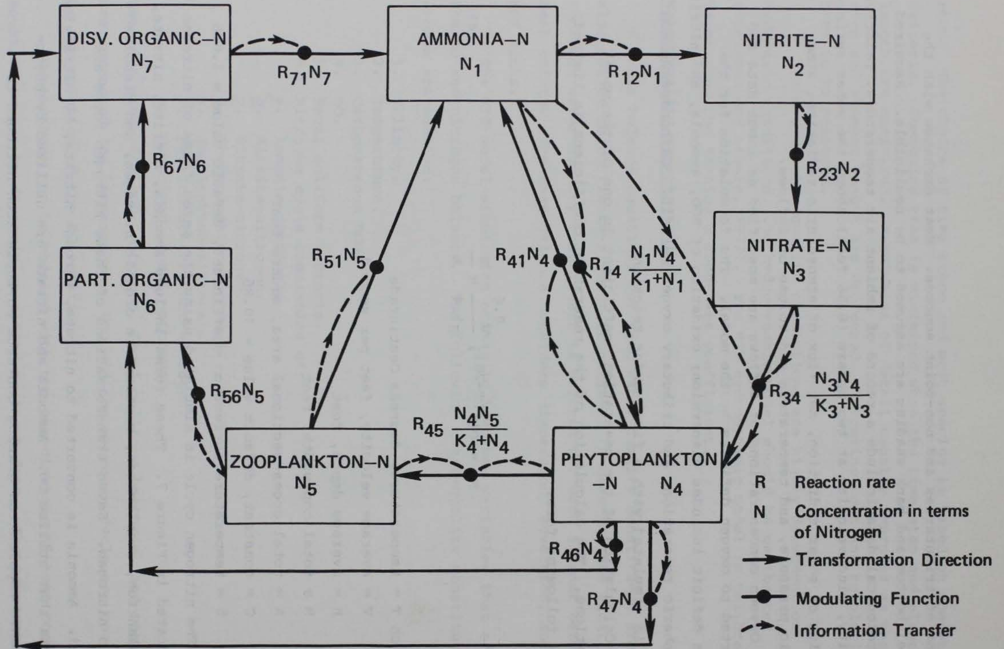
Figure 7. Nitrogen cycle modeled by the MIT model (adapted from Harleman and others, 1977)
