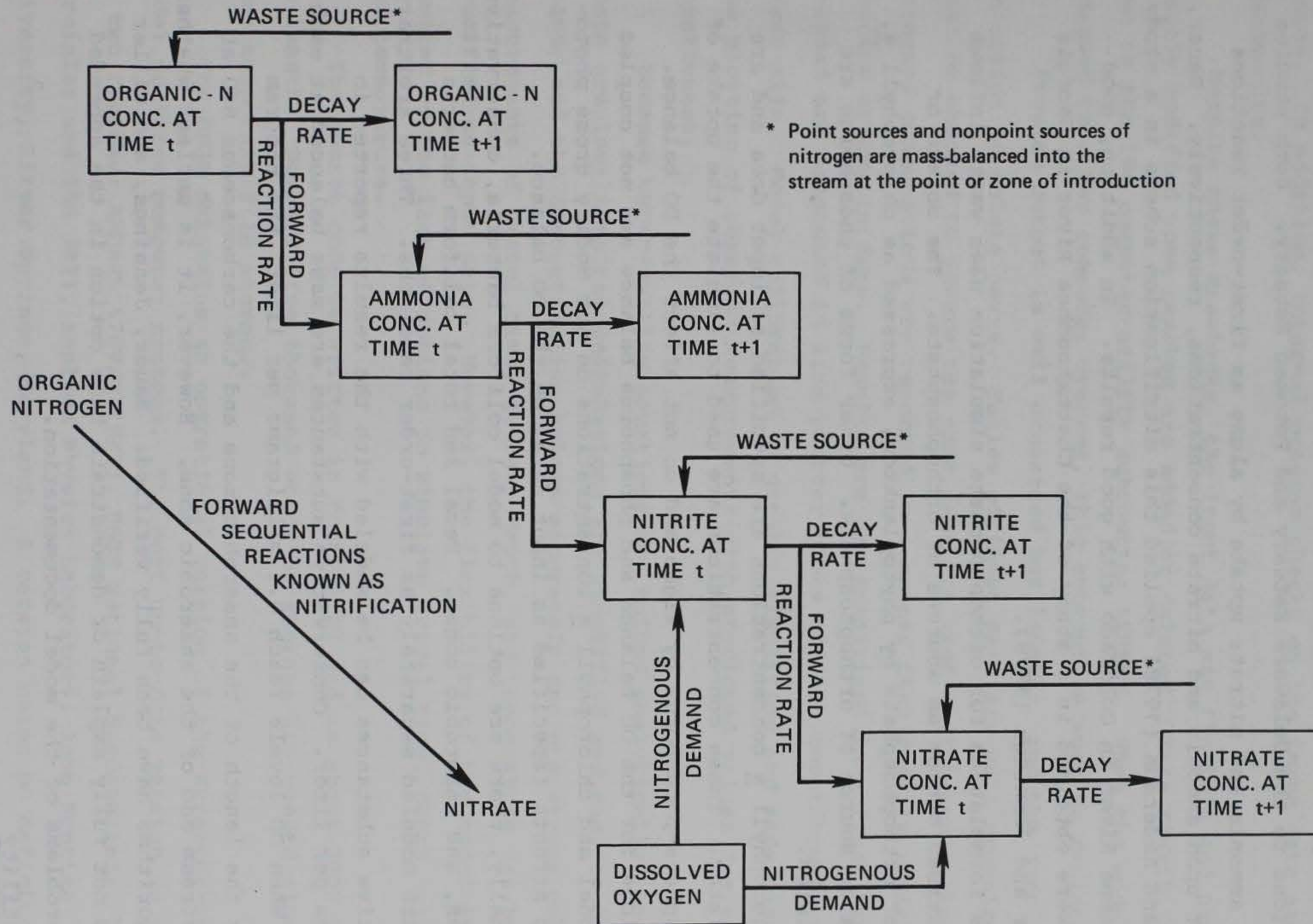
Figure 2. Nitrification cycle used by the Streeter-Phelps model (adapted from Bauer, Jennings, and Miller, 1979)
