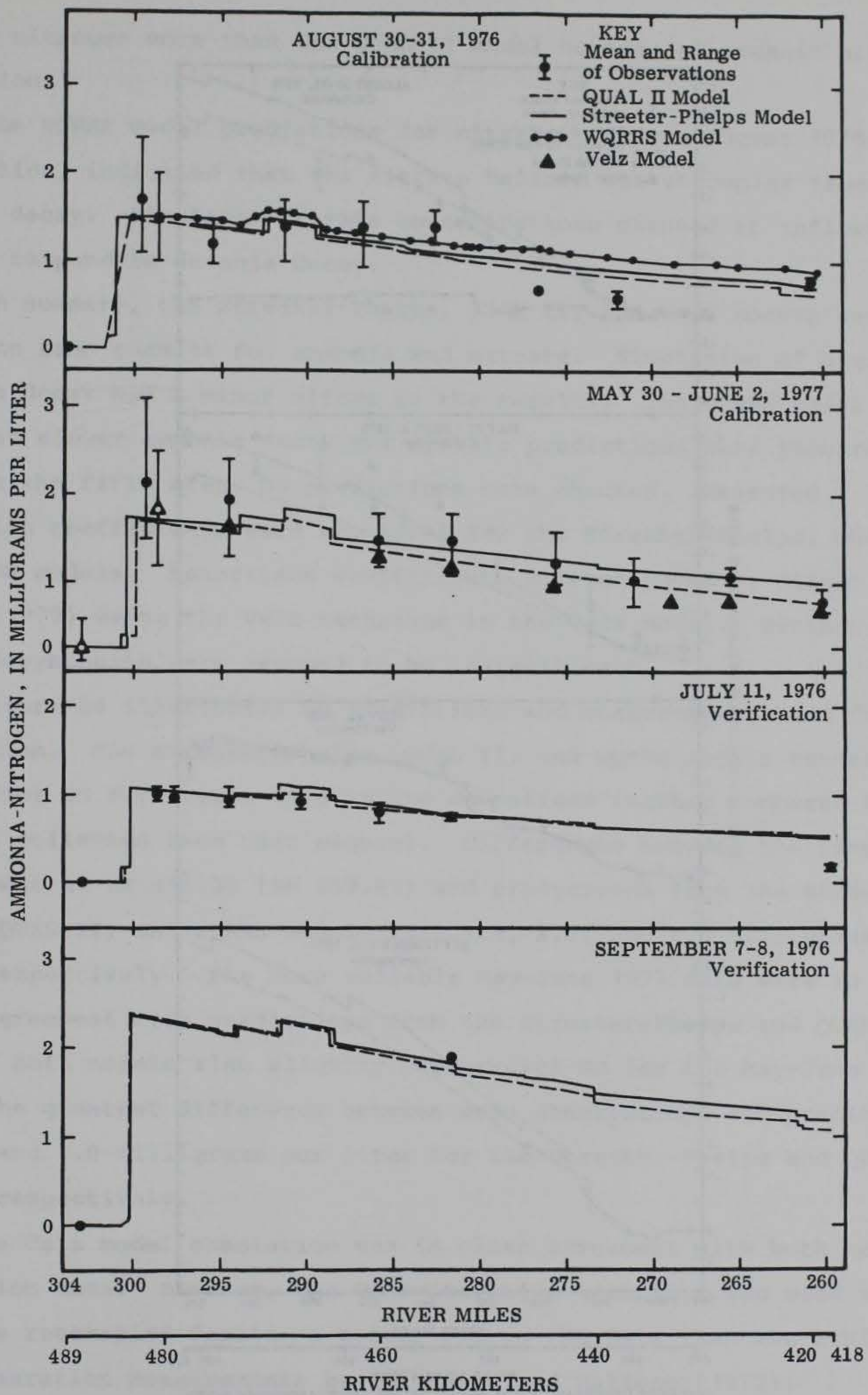
Figure 22. Observed and predicted ammonia-nitrogen, Chattahoochee River
