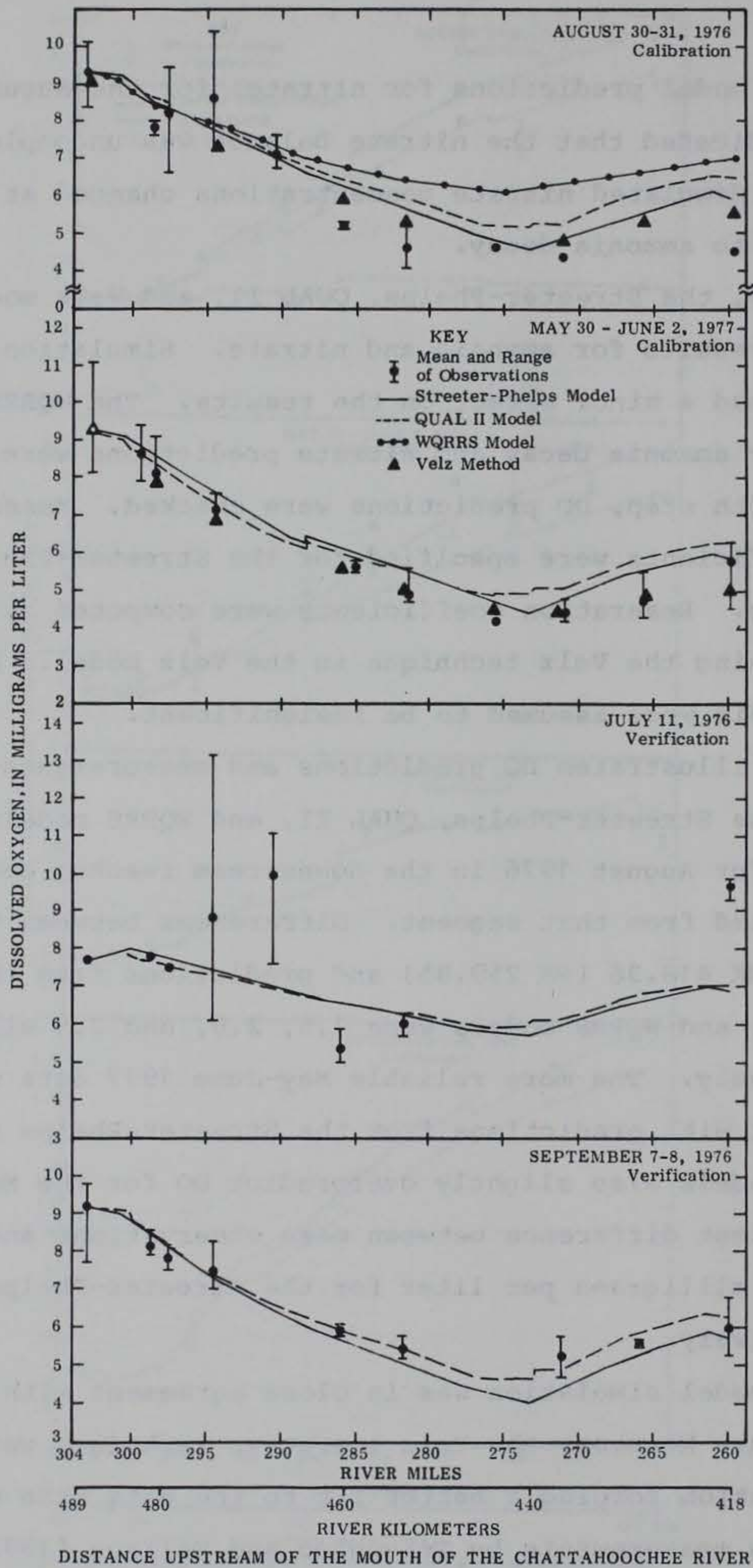
Figure 24. Observed and predicted dissolved oxygen, Chattahoochee River
