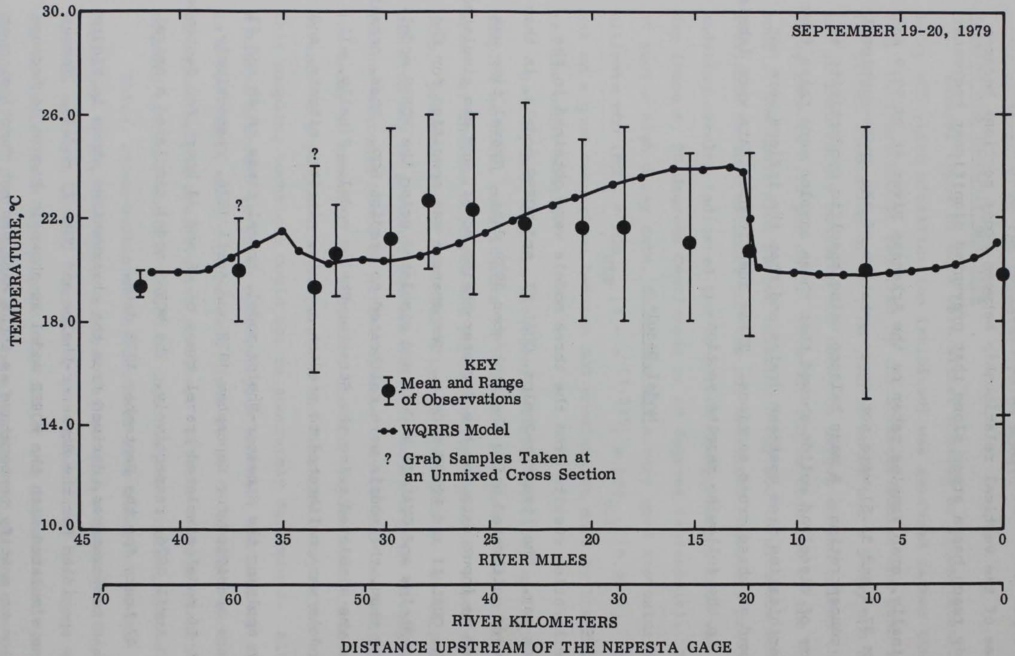
Figure 34. Water temperatures predicted by the WQRRS model compared to observed temperatures for the Arkansas River
