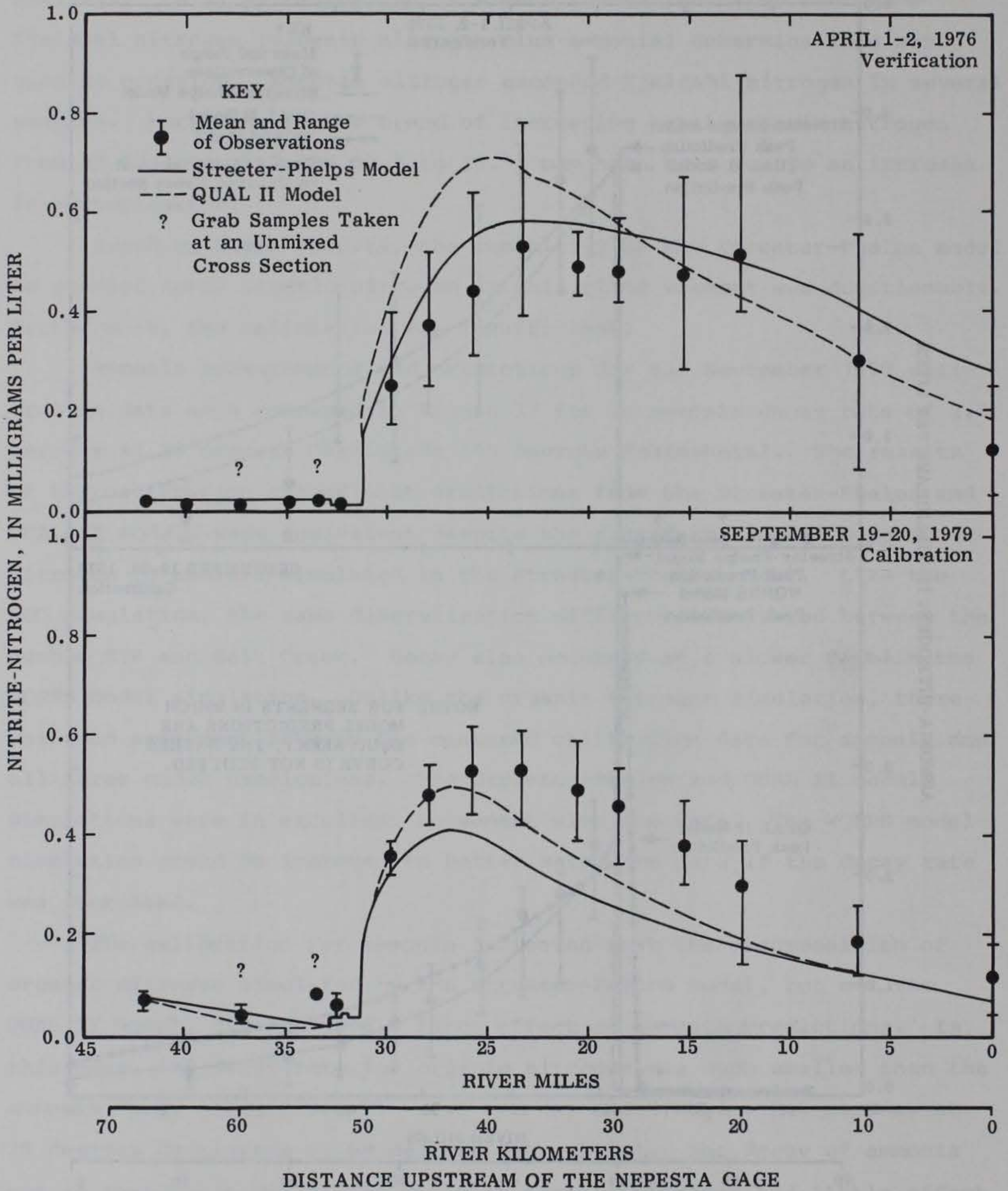
Figure 38. Observed and predicted nitrite-nitrogen, Arkansas River
