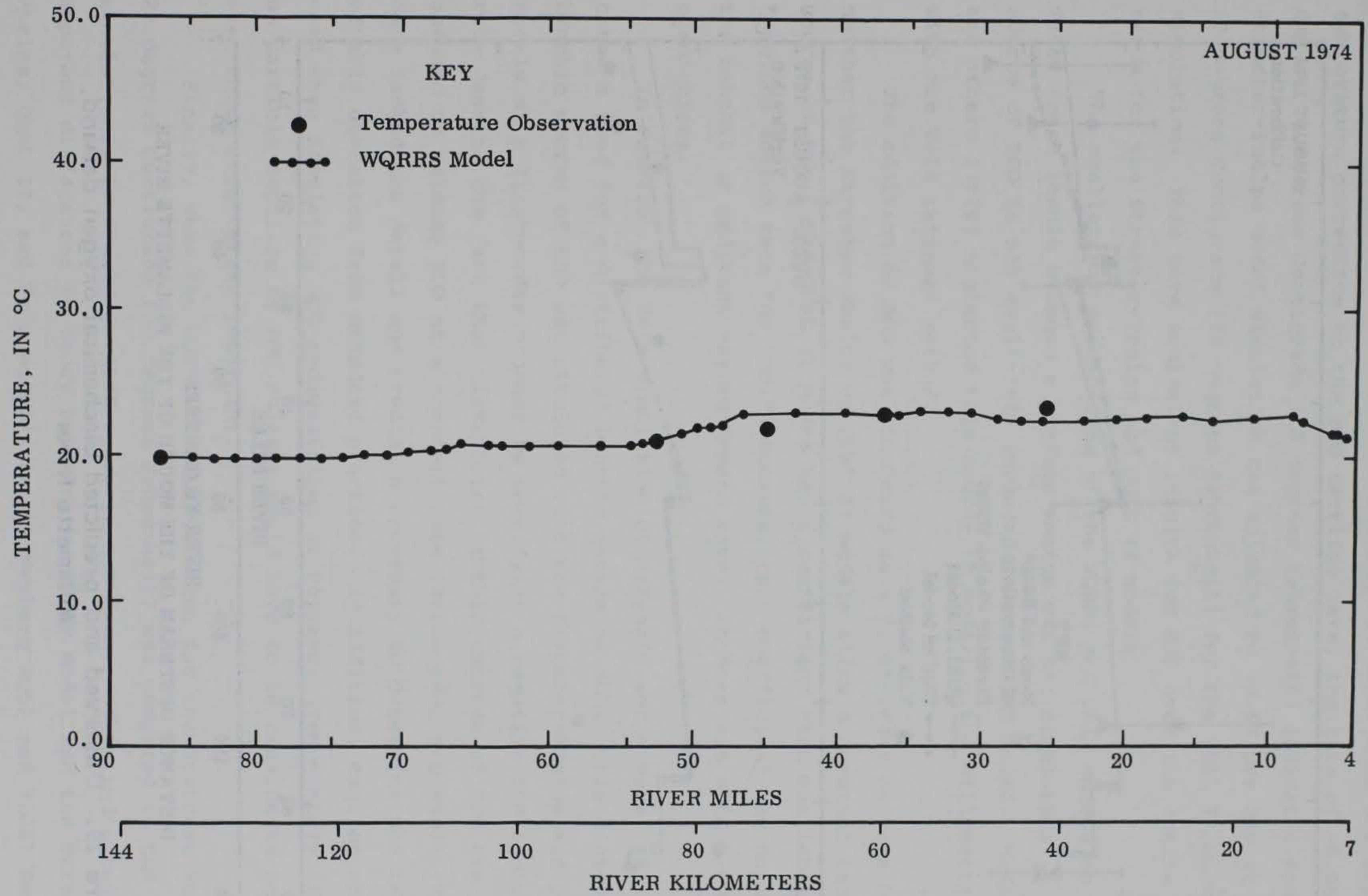
DISTANCE UPSTREAM OF THE MOUTH OF THE WILLAMETTE RIVER Figure 28. Observed water temperatures compared to WQRRS model predictions, Willamette River
