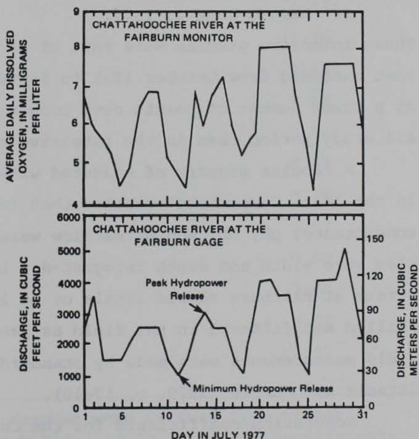
Figure 10. Dissolved-oxygen concentrations and mean daily discharge during 1977
