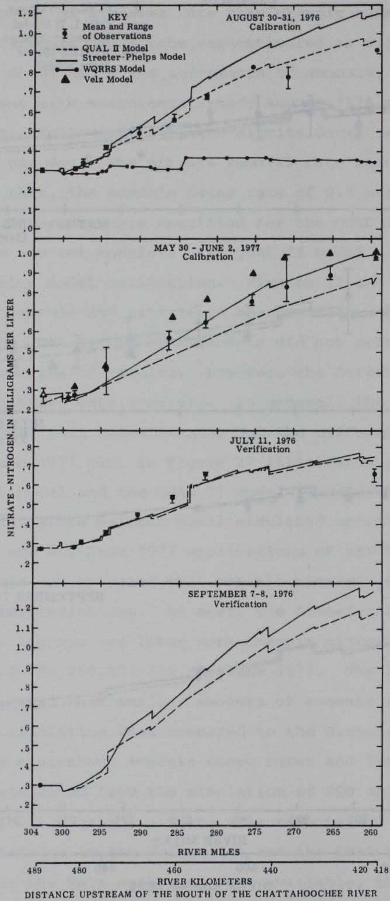
Figure 23. Observed and predicted nitrate-nitrogen, Chattahoochee River
