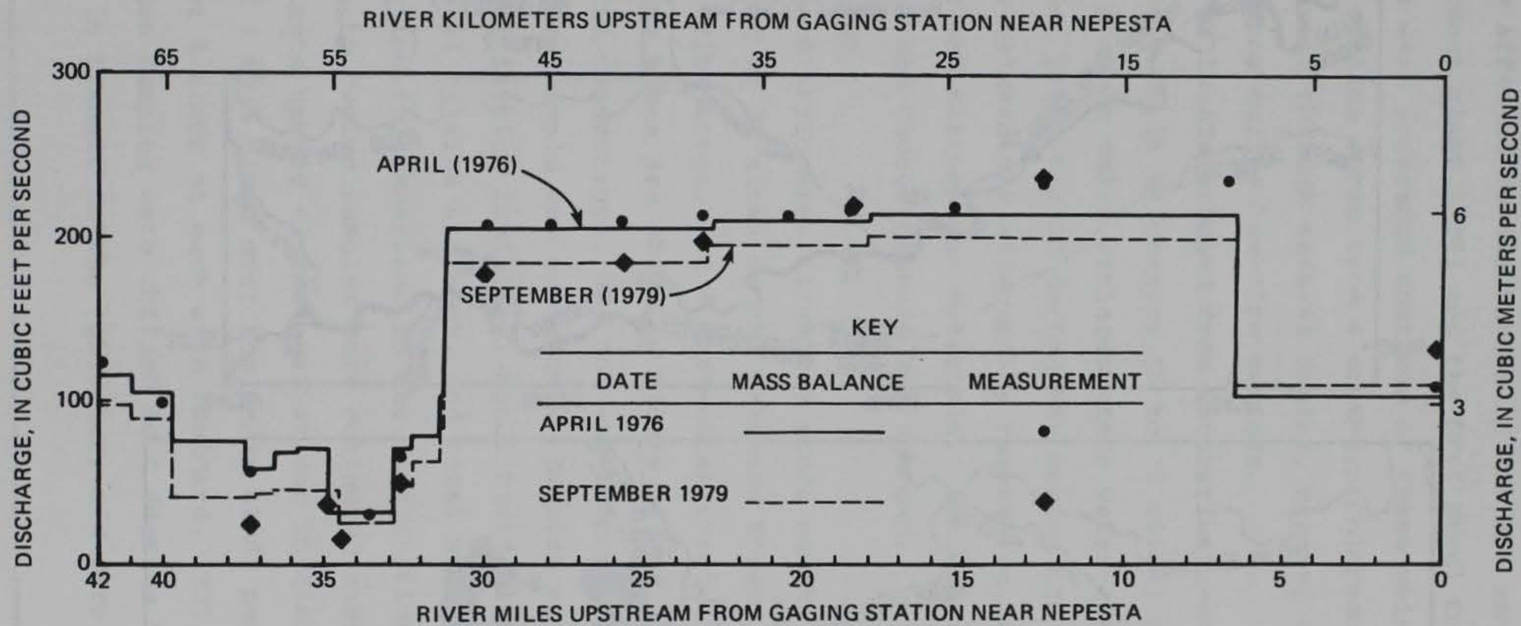
Figure 15. Discharge profiles and discharge measurements for the Arkansas River in Colorado, April 1976 and September 1979 (1 ft 3 /s = 0.028 m 3 /s and 1 mile = 1.6 km)
