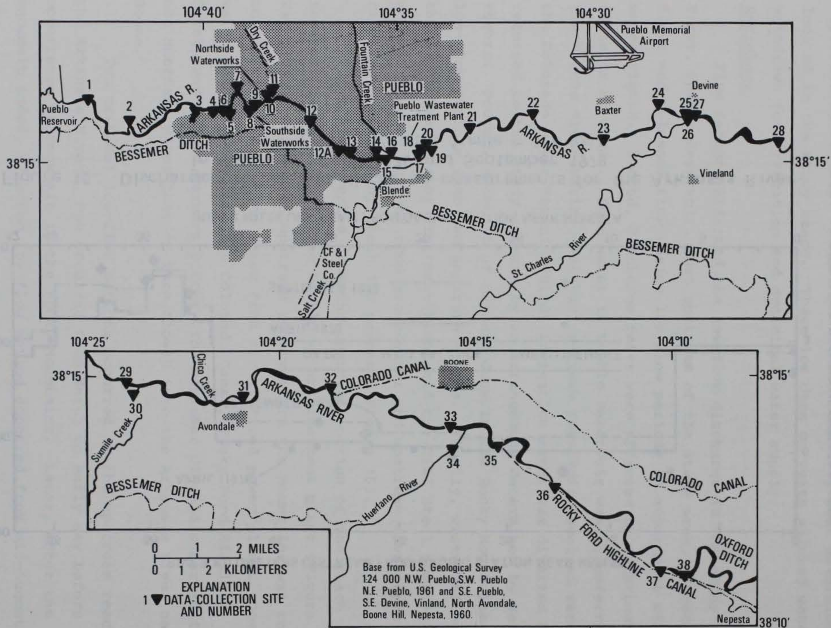
Figure 16. Location of sample sites on the Arkansas River between Pueblo and Nepesta, Colorado; and sample sites on tributaries and point sources (adapted from Goddard, 1980)
