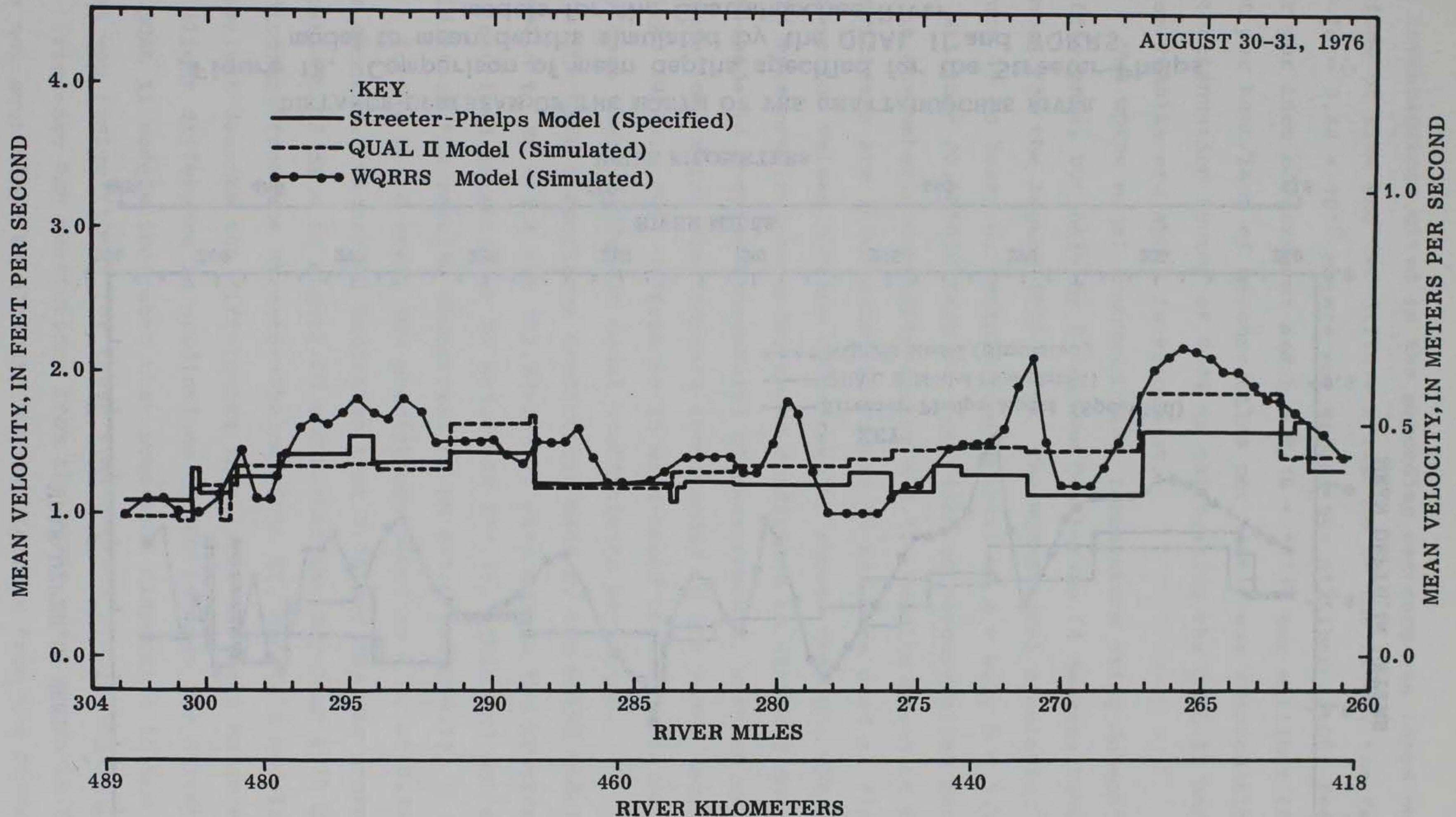
Figure 17. Comparison of mean velocities specified for the Streeter-Phelps model to mean velocities simulated by the QUAL II and WQRRS models for the Chattahoochee River
