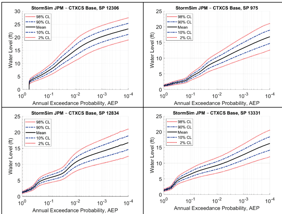
Figure F-23. Hazard curves for select cross-shore hazard locations in Gilchrist area of Bolivar Peninsula for Beach-Dune SLCO alternative.
