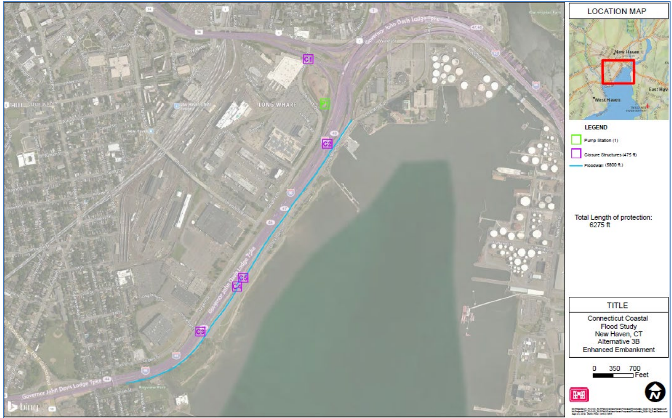
Figure 6 The Recommended Plan, Alternative 3B. The location of the flood wall is shown in blue, closure structures in purple and the 900 CFS pump station is highlighted in green.
