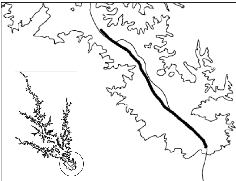
Figure 5. Longitudinal transect (bold line) along the thalweg (thin line) in the downstream reach of Richard B. Russell Lake. Locations based on GPS navigational information
