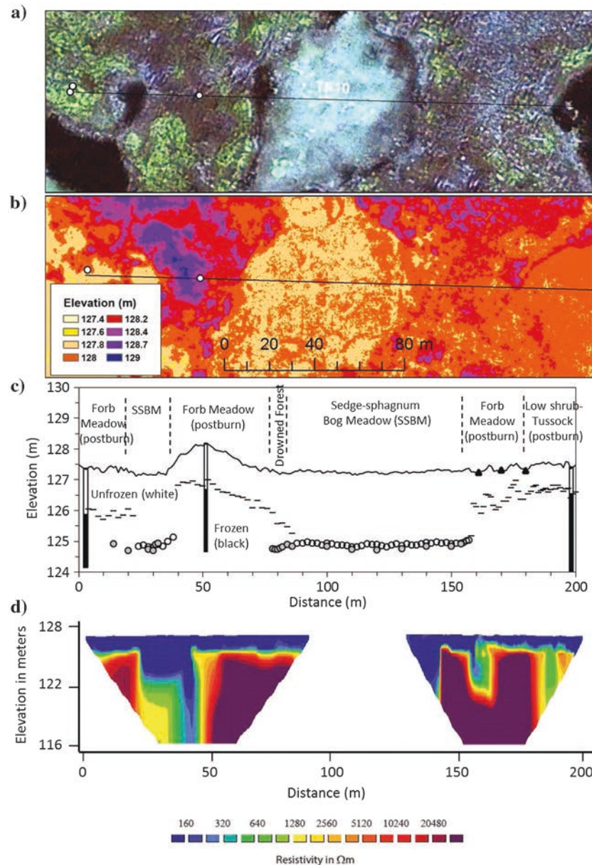
Figure 6. (a) An aerial image of the 2010 fire scar. (b) Airborne LiDAR imagery, shaded by elevation, for the same region presented in the upper panel. The bold line indicates the location and length of the transect at the site, whereas circles denote locations where SIPRE cores were collected. (c) A detailed cross section of the vegetation, ground elevation, SIPRE core depths, seasonal thaw depths, and elevations of unfrozen material across the transect. Black line, ground surface; black triangle, water surface; dashes, thaw-depth elevation in 2012; open circles, unfrozen elevation in 2012; and gray circles, unfrozen elevation in 2013. (d) ERT survey results across the transect.
