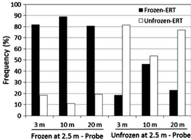
Figure 8. Correlation between permafrost status determined by thaw probing and by ERT across the 1930, 1988, 2001, and 2010 fire scar transects. The frequencies are grouped for locations where soil was frozen or unfrozen at 2.5 m by probing, with frequencies of frozen and unfrozen ground at 3-, 10-, and 20-m depths as determined by ERT (unfrozen when \Omega m < 600 and frozen when \Omega m > 600 ).
