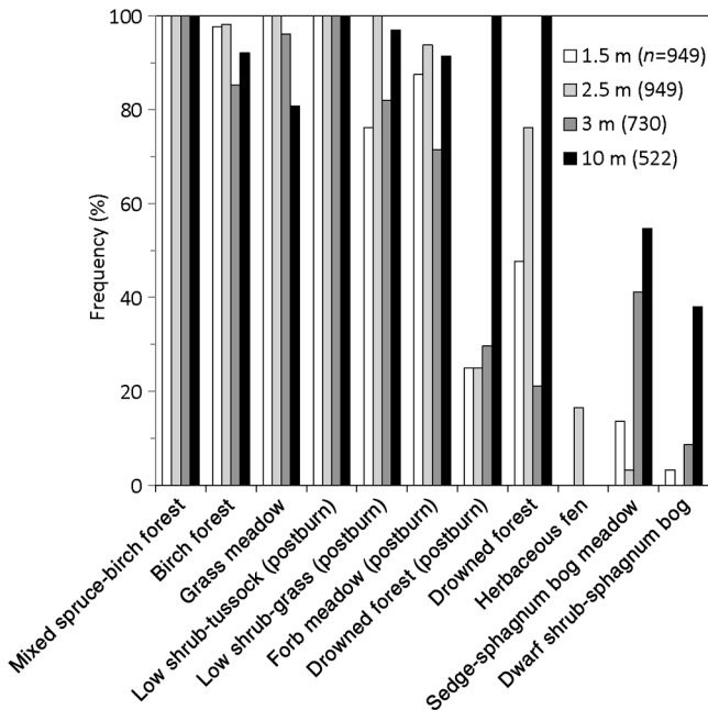
Figure 9. A histogram of the percent frequency of permafrost, by depth, across the 11 ecotypes present at the fire scars.
