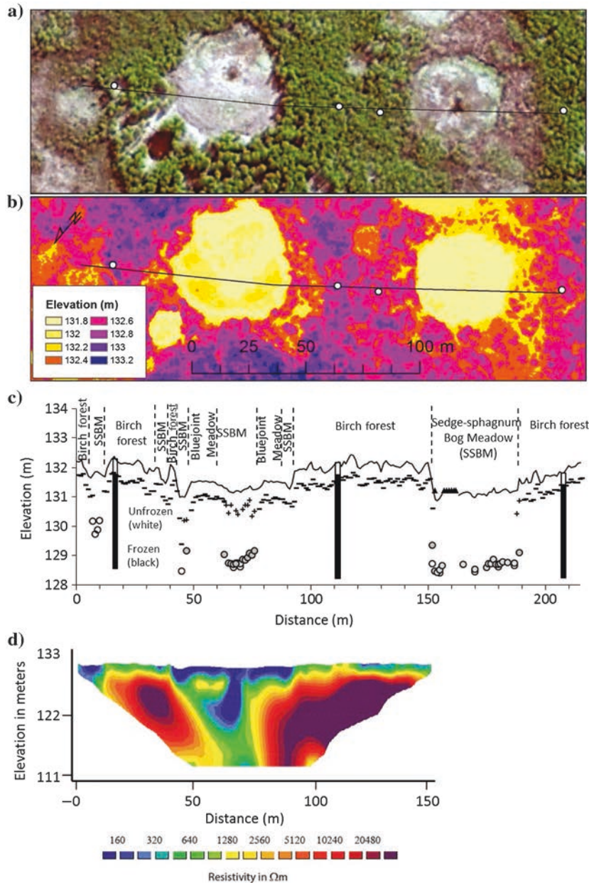
Figure 4. (a) An aerial image of the 1988 fire scar. (b) Airborne LiDAR imagery, shaded by elevation, for the same region presented in (a). The bold line indicates the location and length of the transect at the site, whereas circles denote locations where SIPRE cores were collected. (c) A detailed cross section of the vegetation, ground elevation, SIPRE core depths, seasonal thaw depths, and elevations of unfrozen material across the transect. Black line, ground surface; black triangle, water surface; dashes, thaw-depth elevation in 2012; crosses, seasonal frost elevation in 2012; open circles, unfrozen elevation in 2012; and gray circles, unfrozen elevation in 2013. (d) ERT survey results across the transect.
