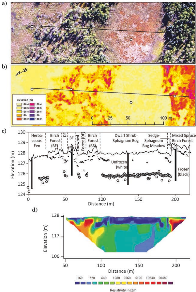
Figure 2. (a) An aerial image of the 1930 fire scar. (b) Airborne LiDAR imagery, shaded by elevation, for the same region presented in the upper panel. The bold line indicates the location and length of the transect at the site, whereas circles denote locations where SIPRE cores were collected. (c) A detailed cross section of the vegetation, ground elevation, SIPRE core depths, seasonal thaw depths, and elevations of unfrozen material across the transect. Black line, ground surface; dashes, thaw-depth elevation in 2012; crosses, seasonal frost elevation in 2012; open circles, unfrozen elevation in 2012; and gray circles, unfrozen elevation in 2014. (d) ERT survey results across the transect.
