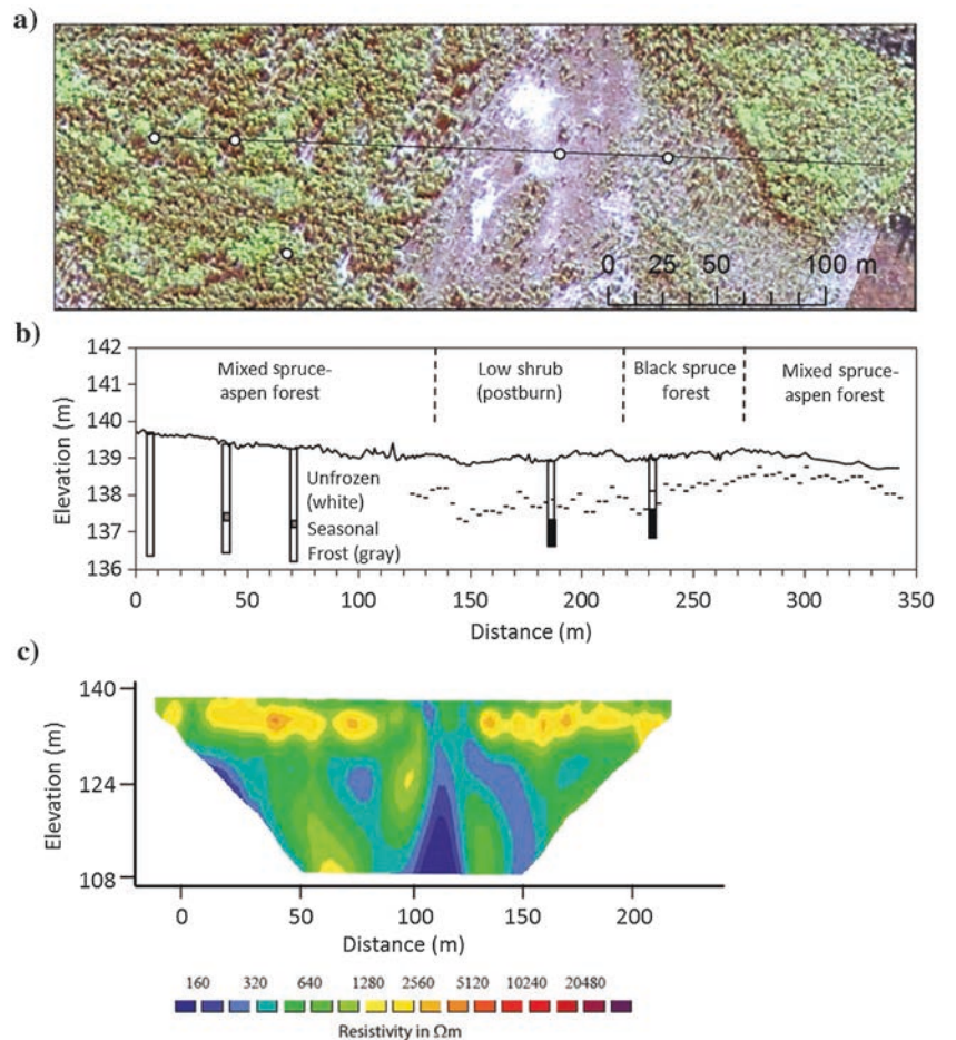
Figure 3. (a) An aerial image of the 1975 fire scar. The bold line indicates the location and length of the transect at the site, whereas circles denote locations where SIPRE cores were collected. (b) A detailed cross section of the vegetation, ground elevation, SIPRE core depths, seasonal thaw depths, and elevations of unfrozen material across the transect. Black line, ground surface and dashes, thaw-depth elevation in 2012. (c) ERT survey results across the transect.
