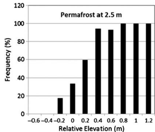
Figure 10. The relationship between the percentage of permafrost extent and the relative elevation.
