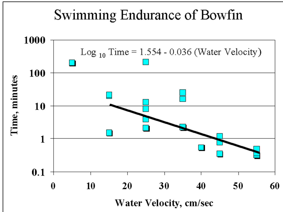
Figure 7. Bowfin swimming performance model
