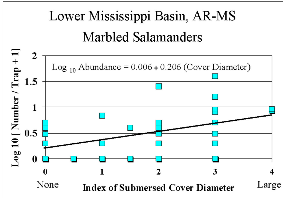
Figure 5. Marbled salamander habitat model
