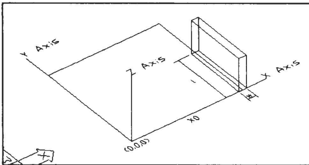
Figure 3. Wall local coordinate system.
