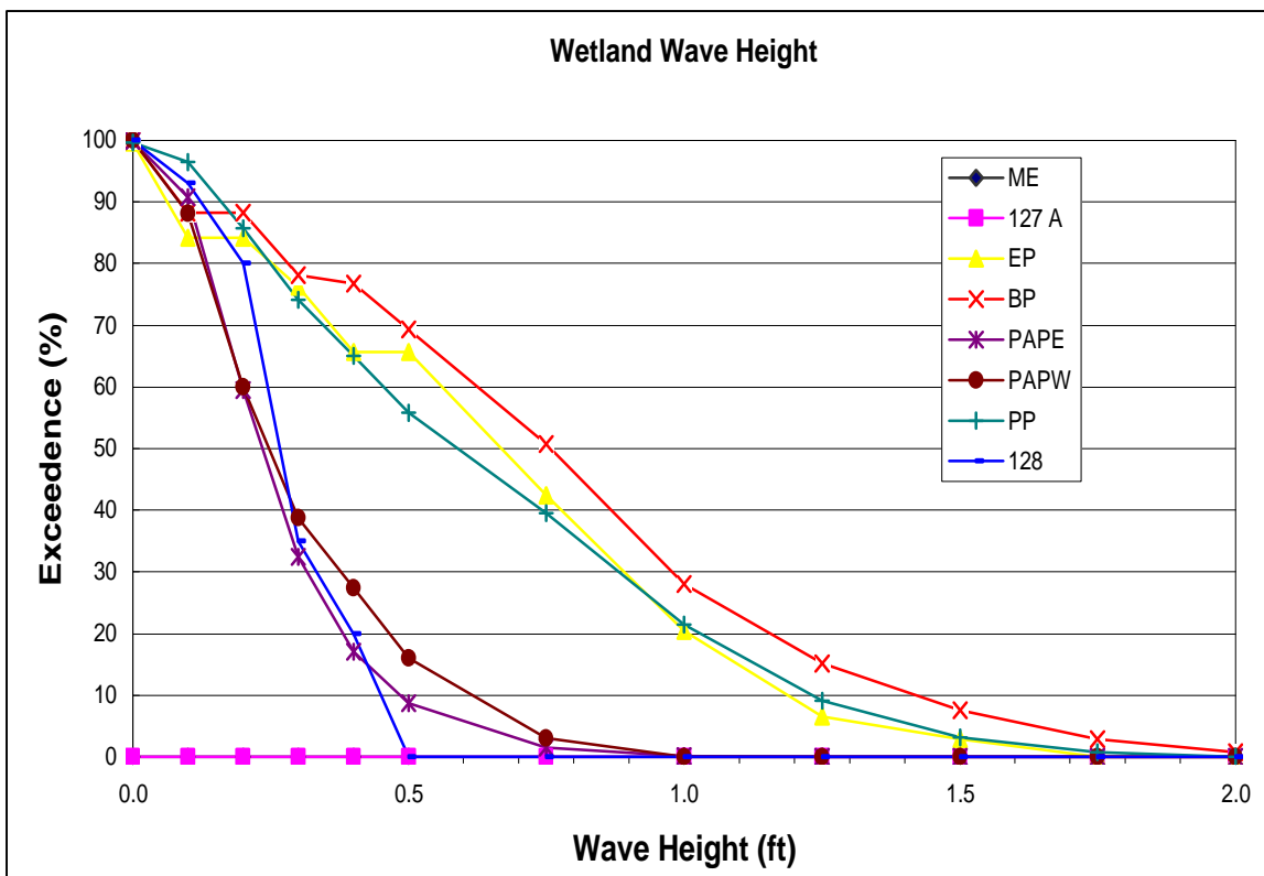
Figure 5. Exceedence curves for wetland wave height (to convert wave heights to meters, multiply by 0.3048)
