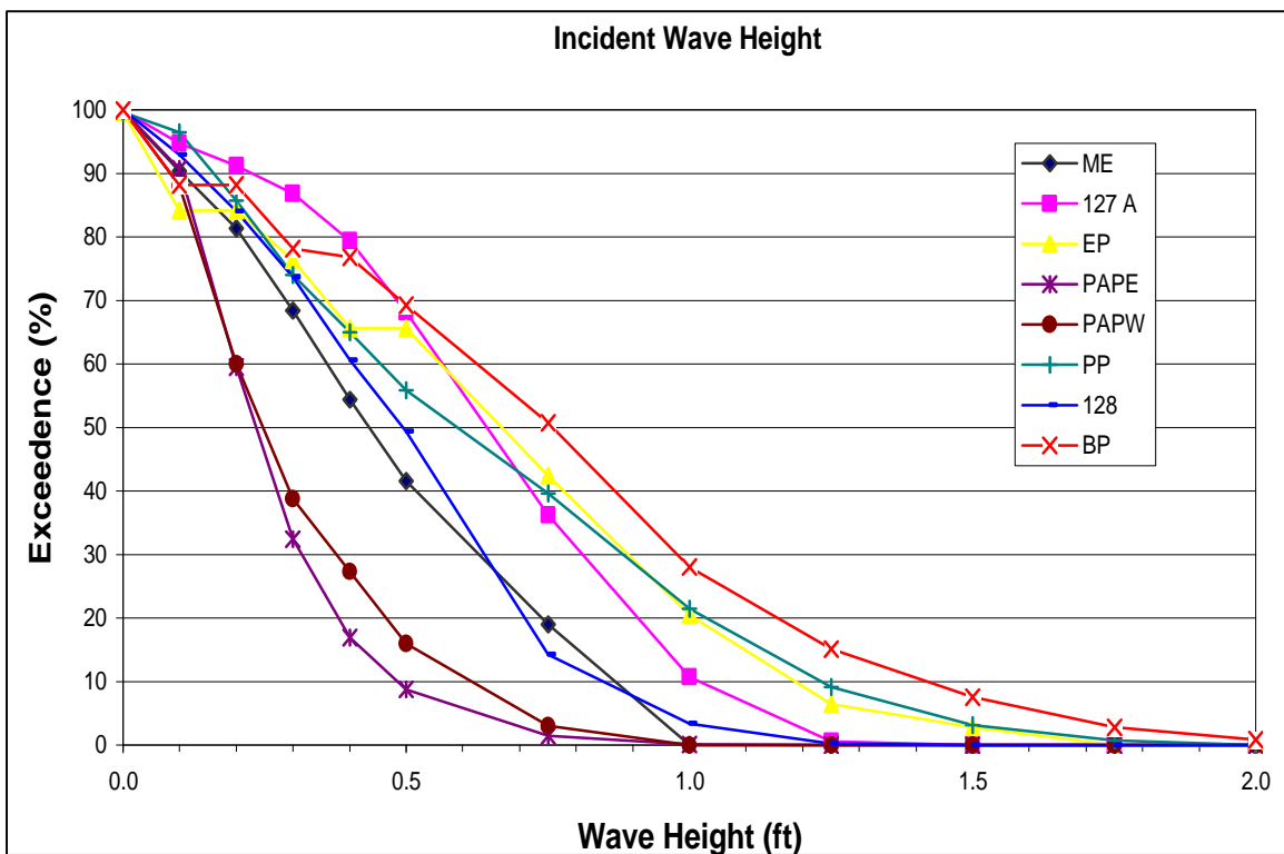
Figure 4. Exceedence curves for incident wave height (to convert wave heights to meters, multiply by 0.3048)
