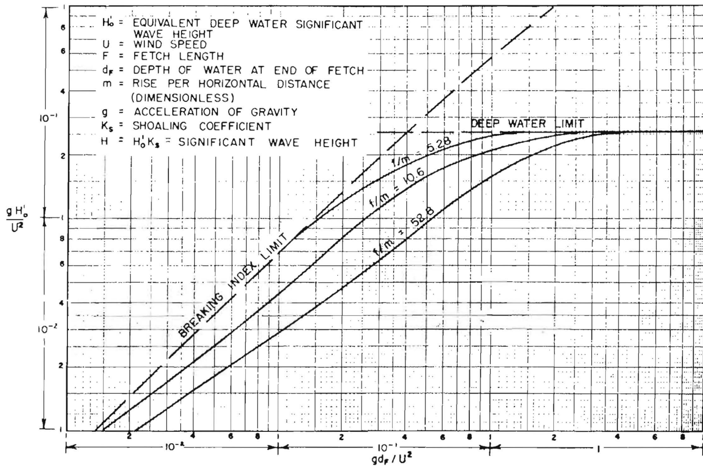
STEADY STATE GENERATION OF WIND WAVES OVER A BOTTOM OF CONSTANT SLOPE, m , FOR VARIOUS FRICTION FACTORS, f NOTE: FOR UNLIMITED FETCH AND UNLIMITED WIND DURATION
