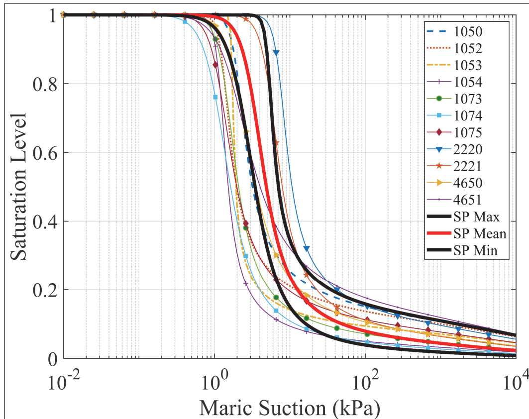
Figure 38. UNSODA coarse-grained data set fitted with Fredlund and Xing model.
