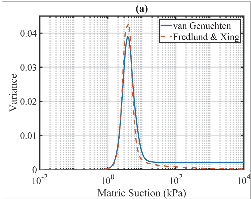
Figure 29. Variance across preparation energies for samples prepared at 18 percent saturation level.
