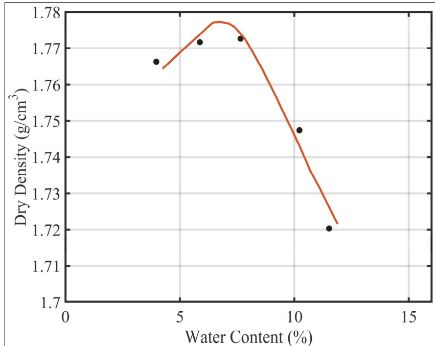
Figure 6. Compaction curve for fine sand, per ASTM D1557 (2012).
