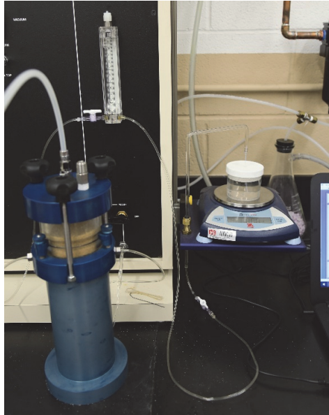
Figure 12. Assembled TRIM chamber and sample saturating.
