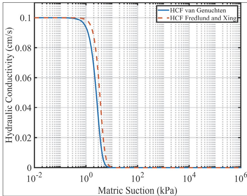
Figure 5. HCF using van Genuchten and Fredlund and Xing models, coarse-grained soil with a saturated hydraulic conductivity of 0.1 cm/s.
