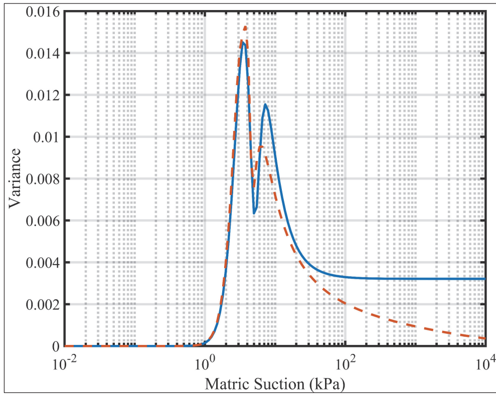
Figure 30. Variance across preparation energies for samples prepared at 24 percent saturation level.
