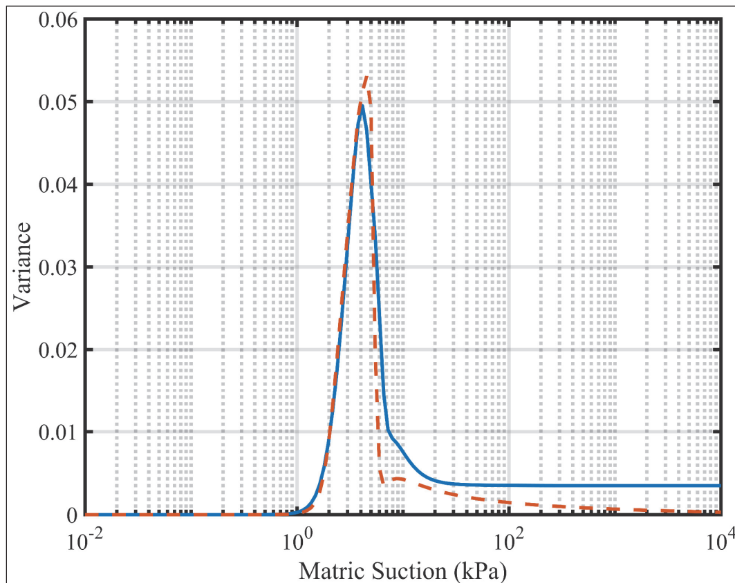
Figure 31. Variance across preparation energies for samples prepared at 30 percent saturation level.
