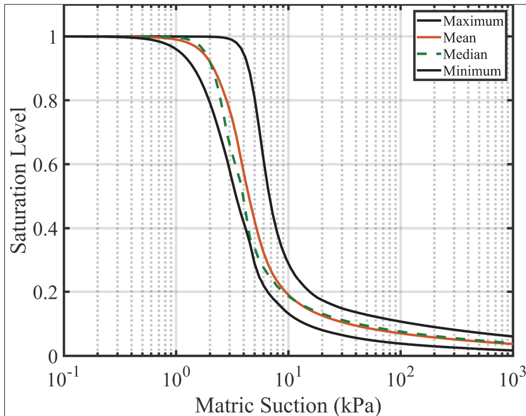
Figure 18. Maximum, minimum, mean, and median SWCC data for samples prepared at a saturation of 18 percent, Fredlund and Xing model.
