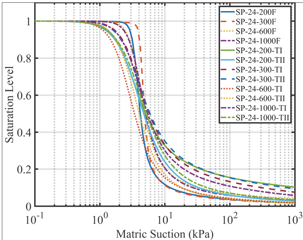
Figure 20. Sand samples prepared at 24 percent saturation fitted with the Fredlund and Xing model.
