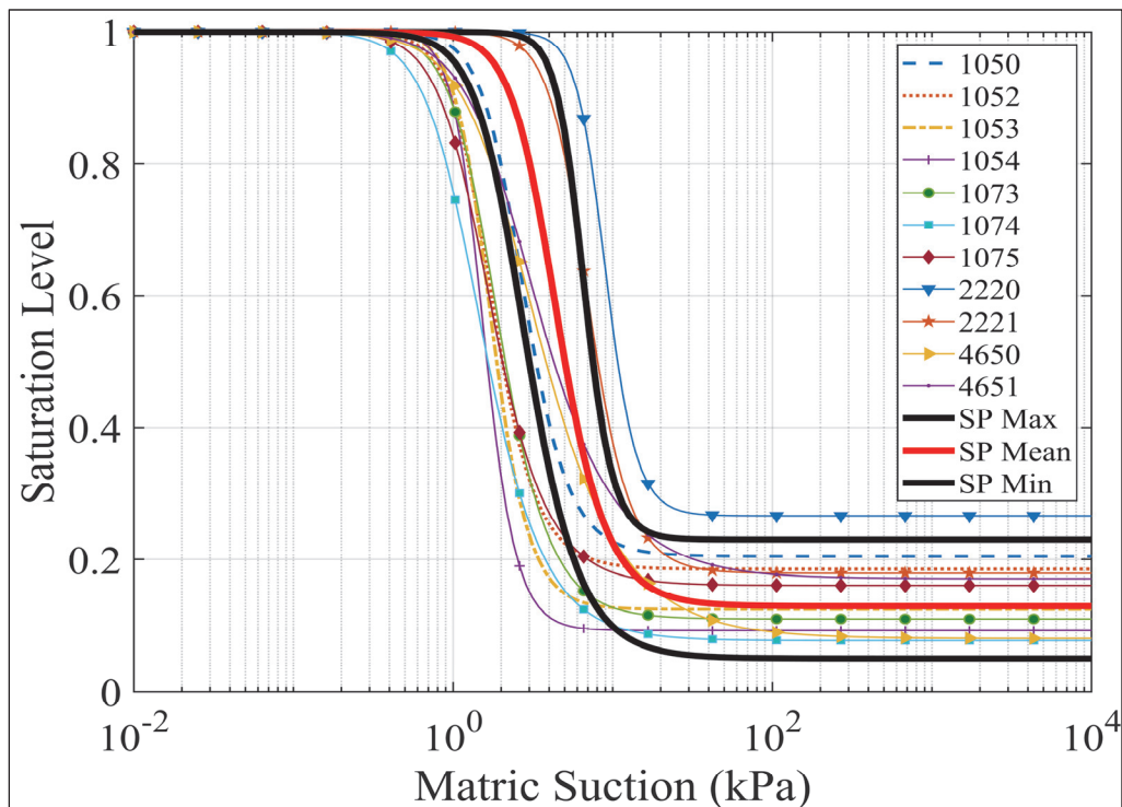
Figure 37. UNSODA coarse-grained data set fitted with van Genuchten model.
