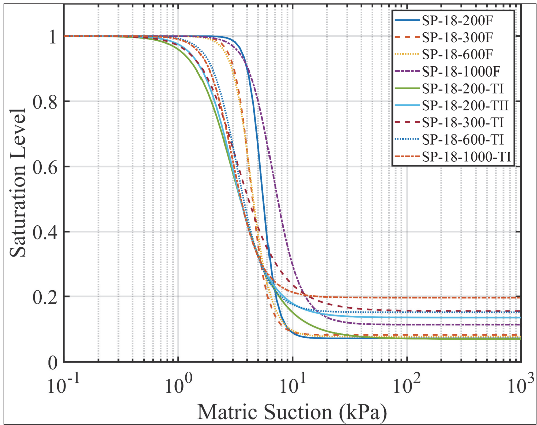
Figure 15. Sand samples prepared at 18 percent saturation fitted with the van Genuchten model.
