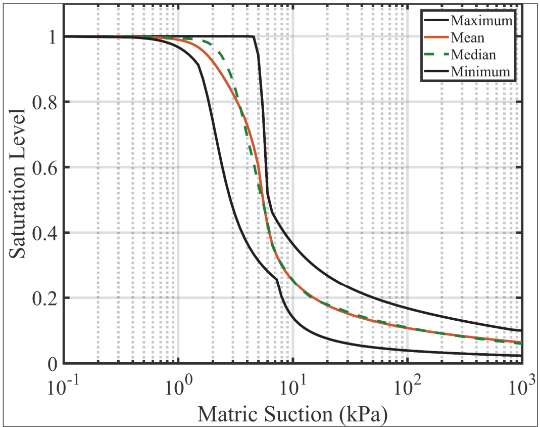
Figure 27. Maximum, minimum, mean, and median SWCC data for samples prepared at a saturation of 30 percent, Fredlund and Xing model.
