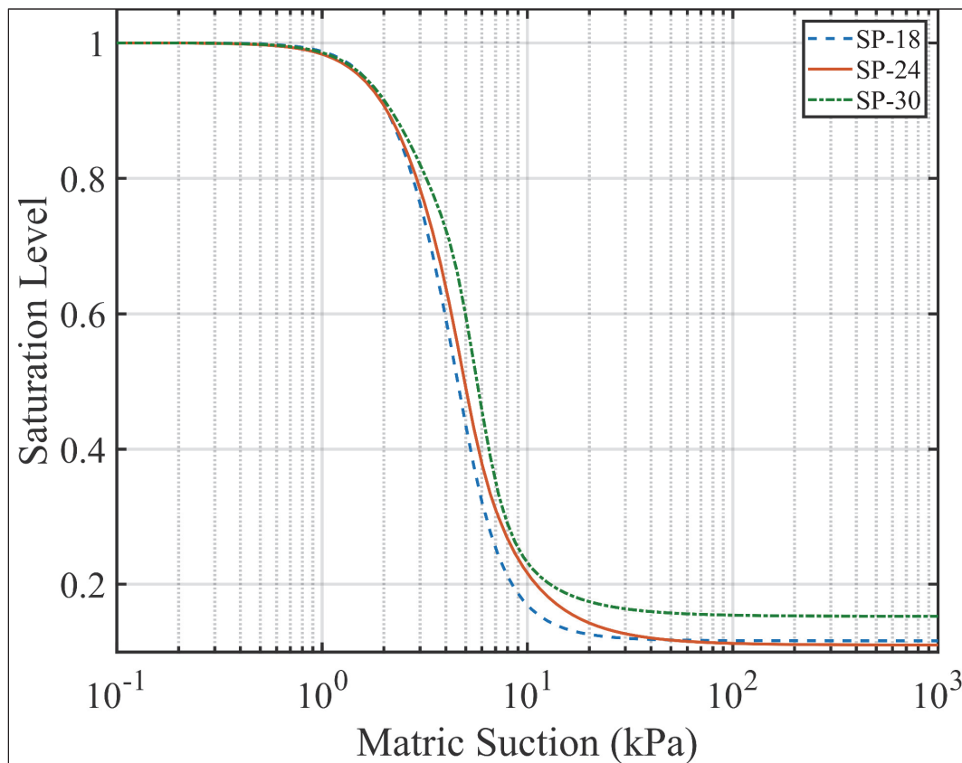
Figure 28. Mean SWCC's for 18, 24 and 30 percent saturation levels.
