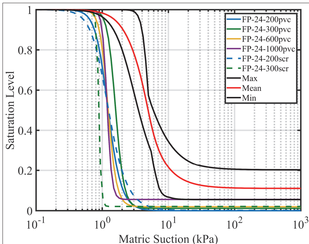
Figure 23. Results of FPM compared to Fredlund and TRIM device mean, maximum, and minimum data.
