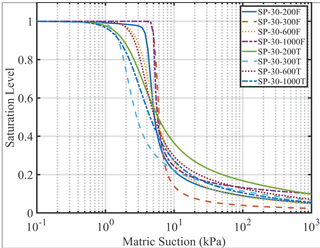
Figure 25. Sand samples prepared at 24 percent saturation fitted with the Fredlund and Xing model.
