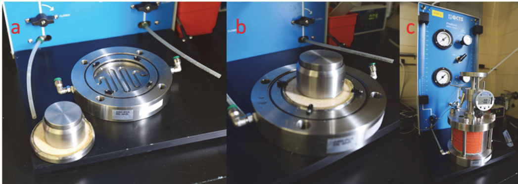
Figure 9. Sample following saturation loaded into Fredlund device.
