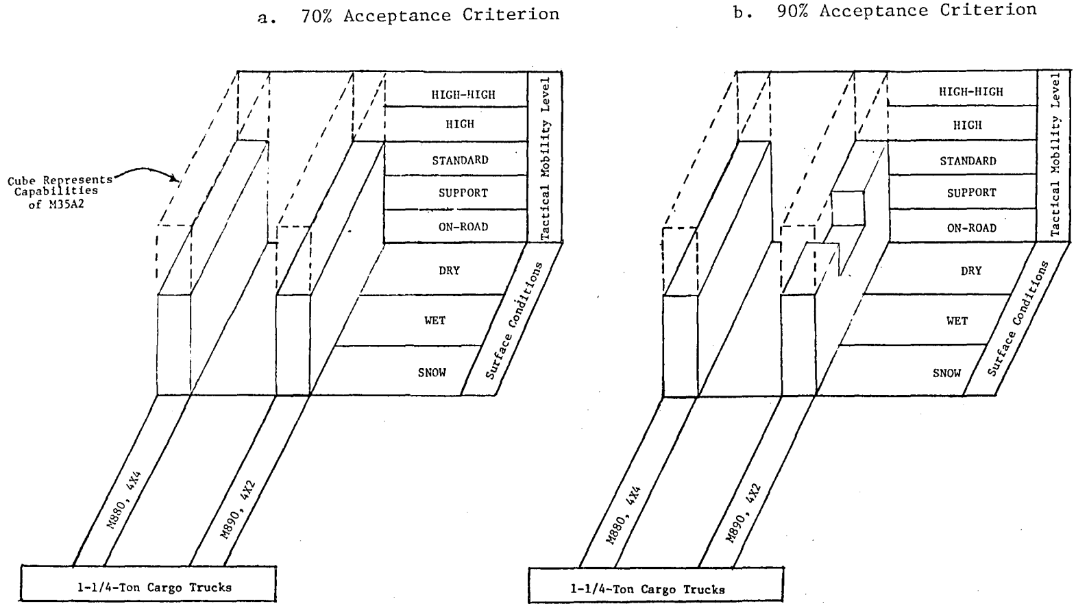
Figure 5. Tactical mobility levels based on two levels of acceptance criteria for study vehicles having 1-1/4-ton payload in HIMO West Germany study area
