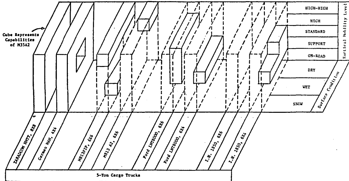
Figure 7. Tactical mobility levels based on two levels of acceptance criteria for study vehicles having 5-ton payload in HIMO West Germany study area
