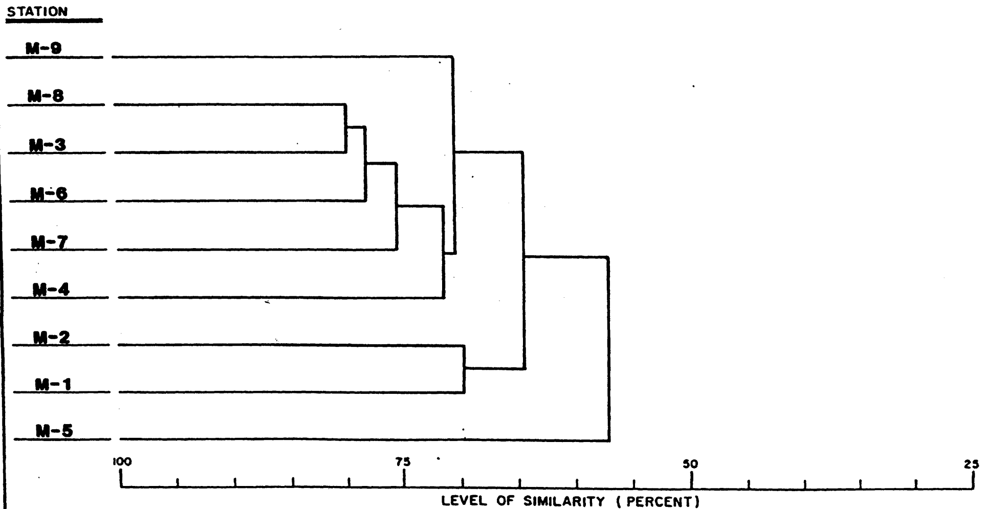
FIGURE A-5 CLUSTER DENDROGRAM SHOWING STATION ASSOCIATIONS BASED ON BENTHIC MACROINVERTEBRATE SIMILARITY AS DETERMINED USING THE BRAY-CURTIS INDEX
