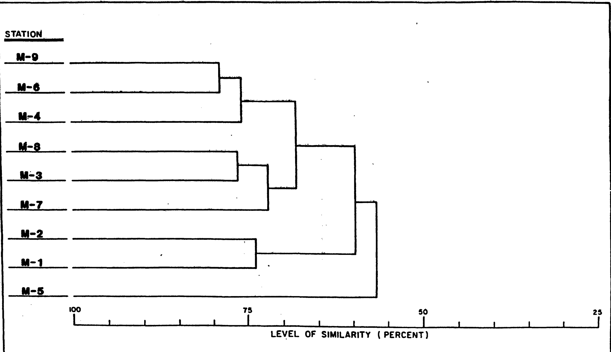
FIGURE A-6 CLUSTER DENDROGRAM SHOWING STATION ASSOCIATIONS BASED ON BENTHIC MACROINVERTEBRATE SIMILARITY AS DETERMINED BY SIMPLE MATCHING (PRESENCE/ABSENCE) Ocean Dredged Material Disposal Site Miami, Florida
