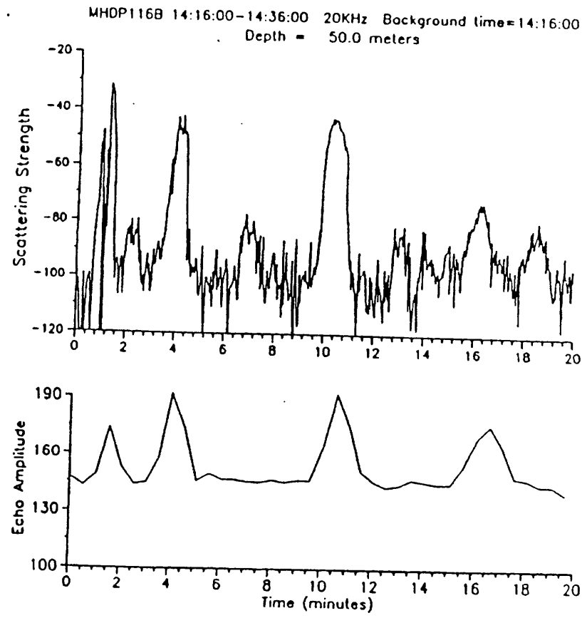
Fig. 12. Comparison between acoustic scattering strength from ACP and echo amplitude from ADCP at 30 m and 50 m. Top: from ACP; bottom: from ADCP.
