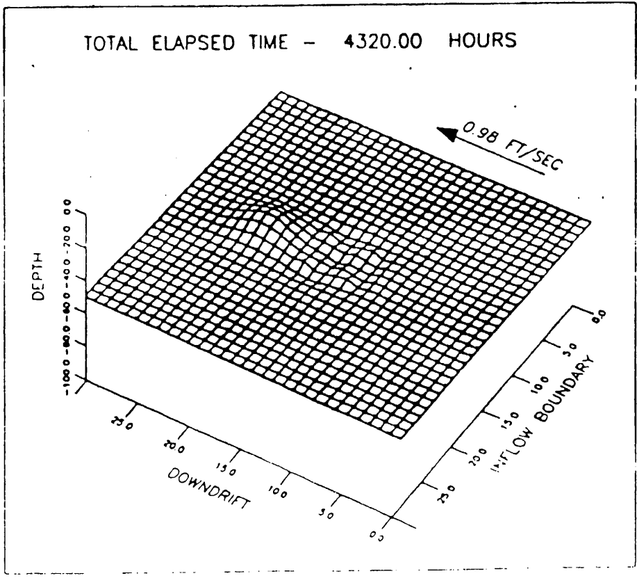
Figure 3.8. Fort Pierce mound configuration at 6 months
