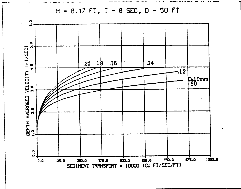
Figure 3.2. Sediment transport vs velocity - Fort Pierce disposal site
