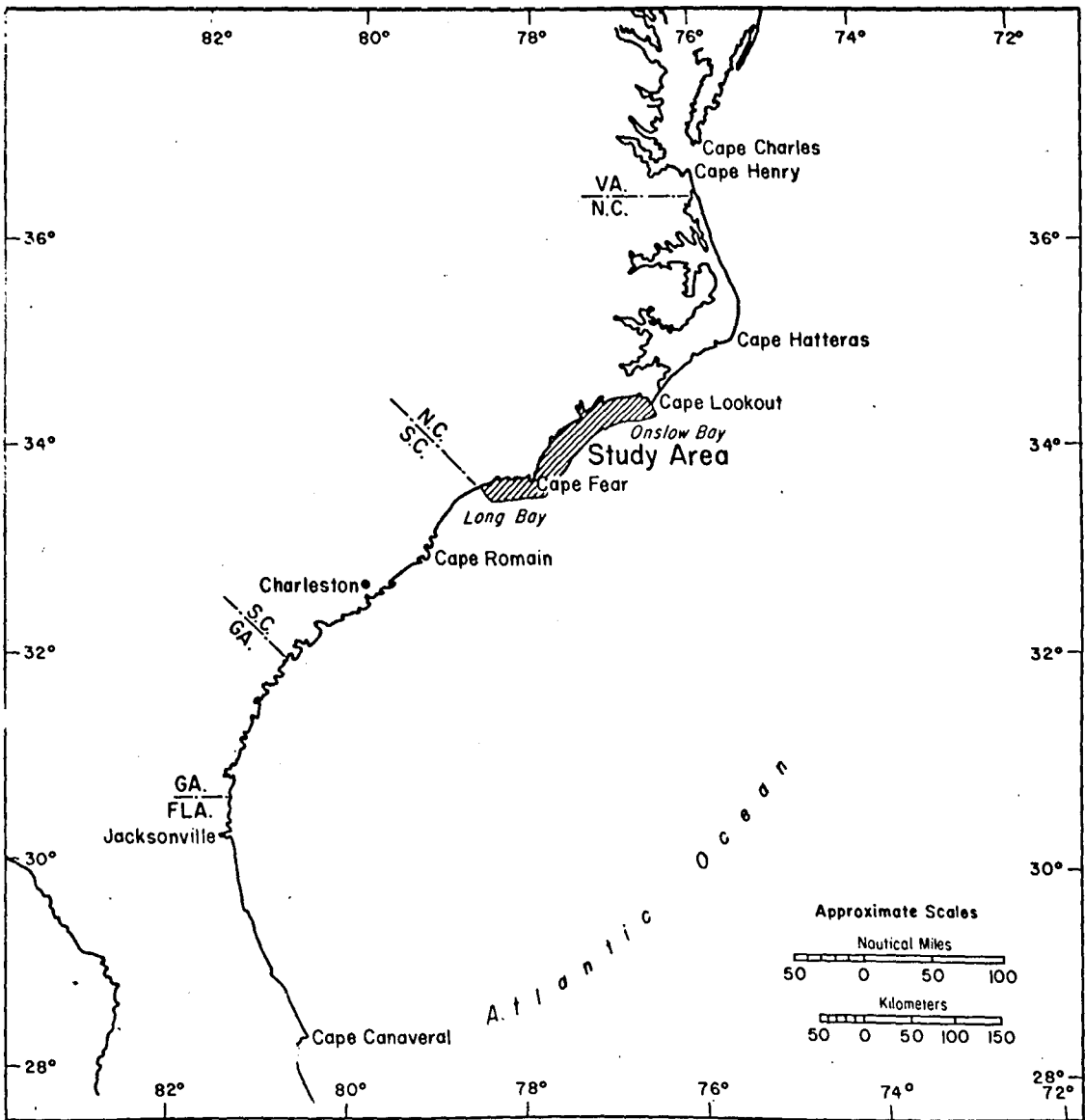
Figure 1. Location of the study region and boundaries of the ICONS survey area.
