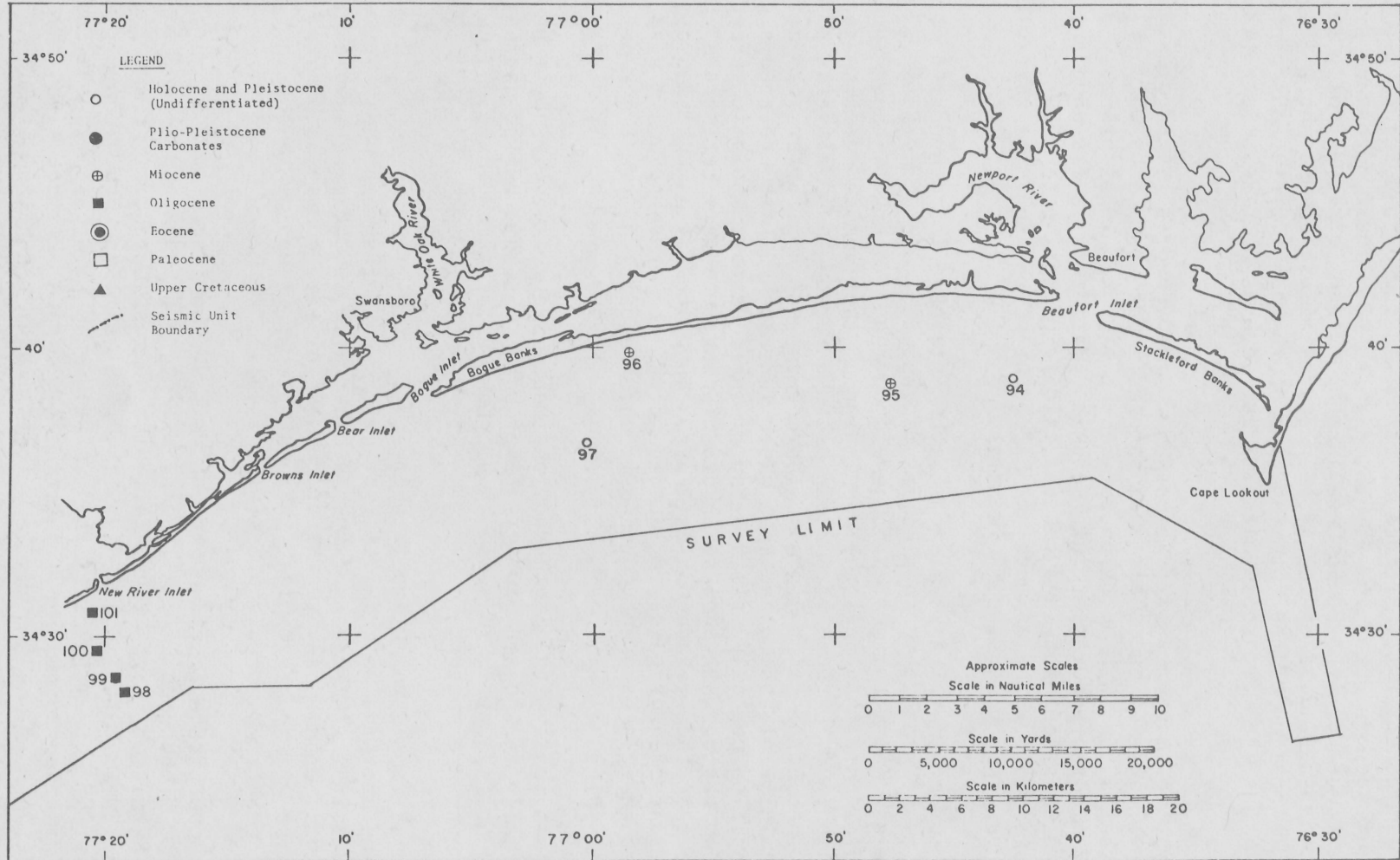
Figure 25. Probable age of sediments in the reconnaissance area.
