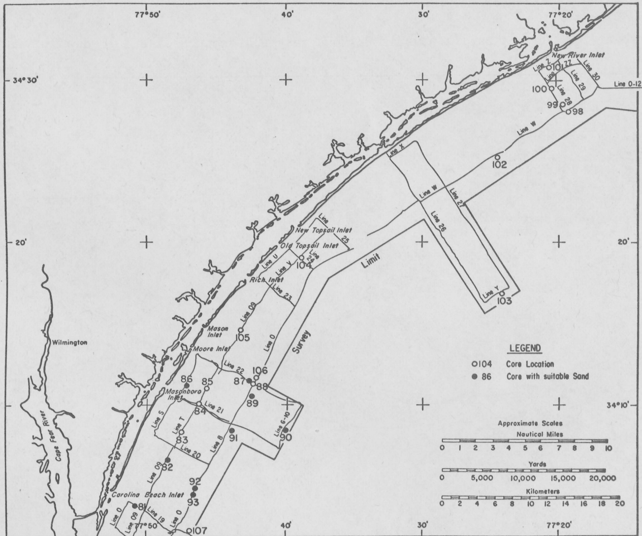
Figure 3. Map of the northeastern part of the main survey area showing seismic reflection survey lines and core sites.
