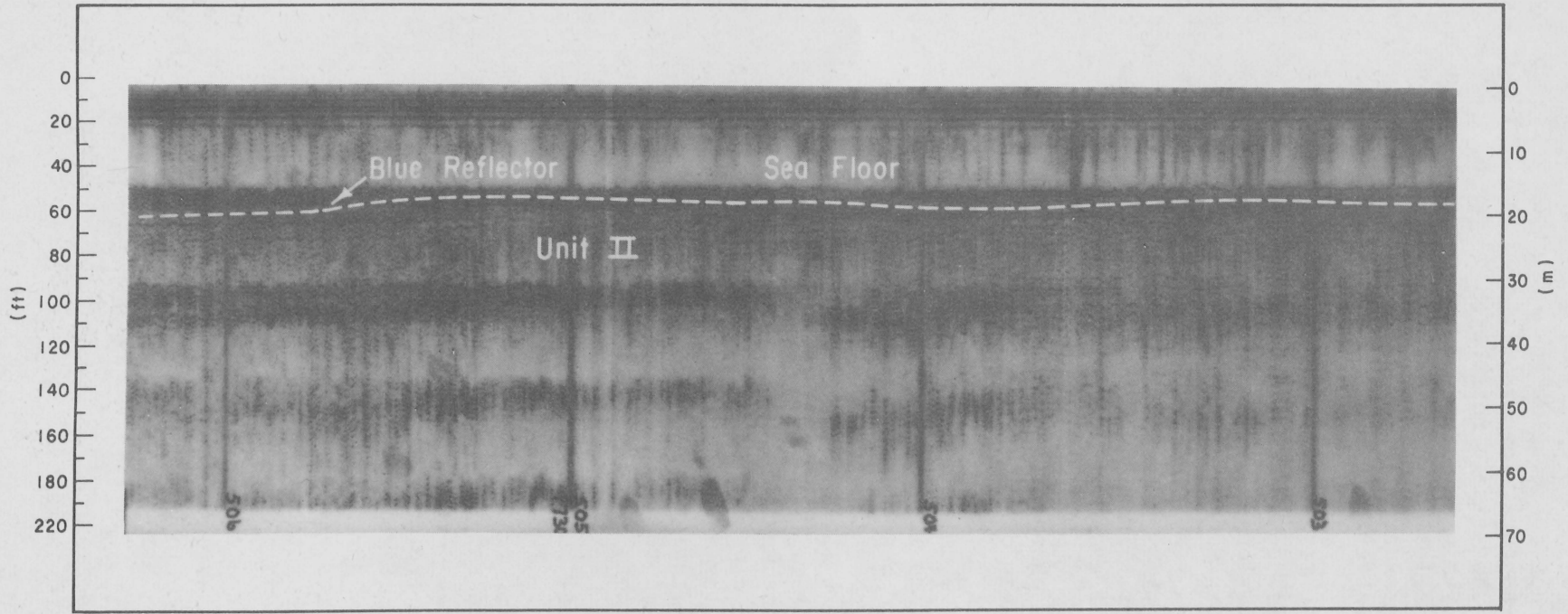
Figure 12. Seismic reflection profile showing the typical near-surface reflector and lack of internal reflectors in reflection unit II.
