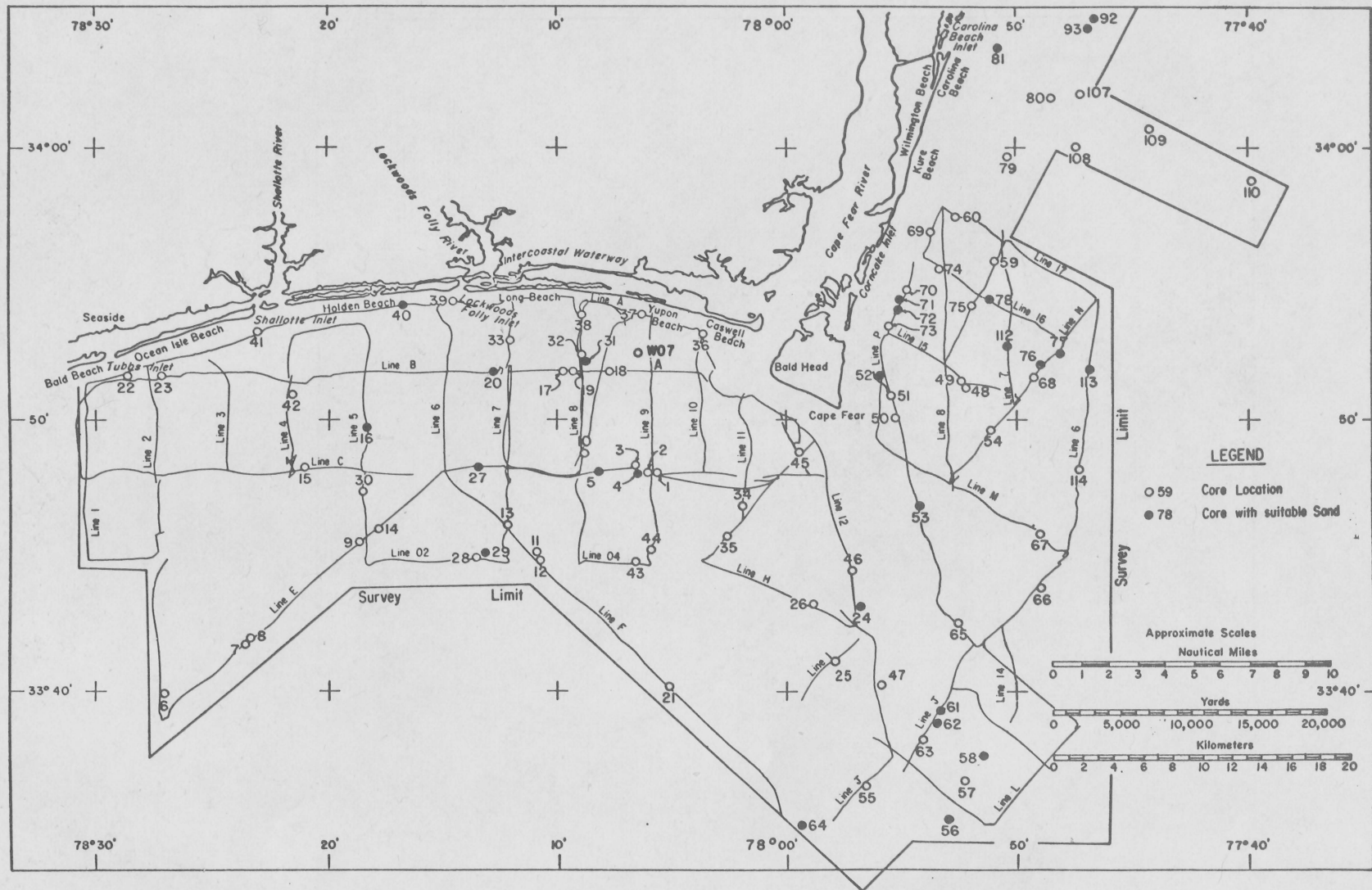
Figure 2. General map of the western part of the study area showing survey coverage.
