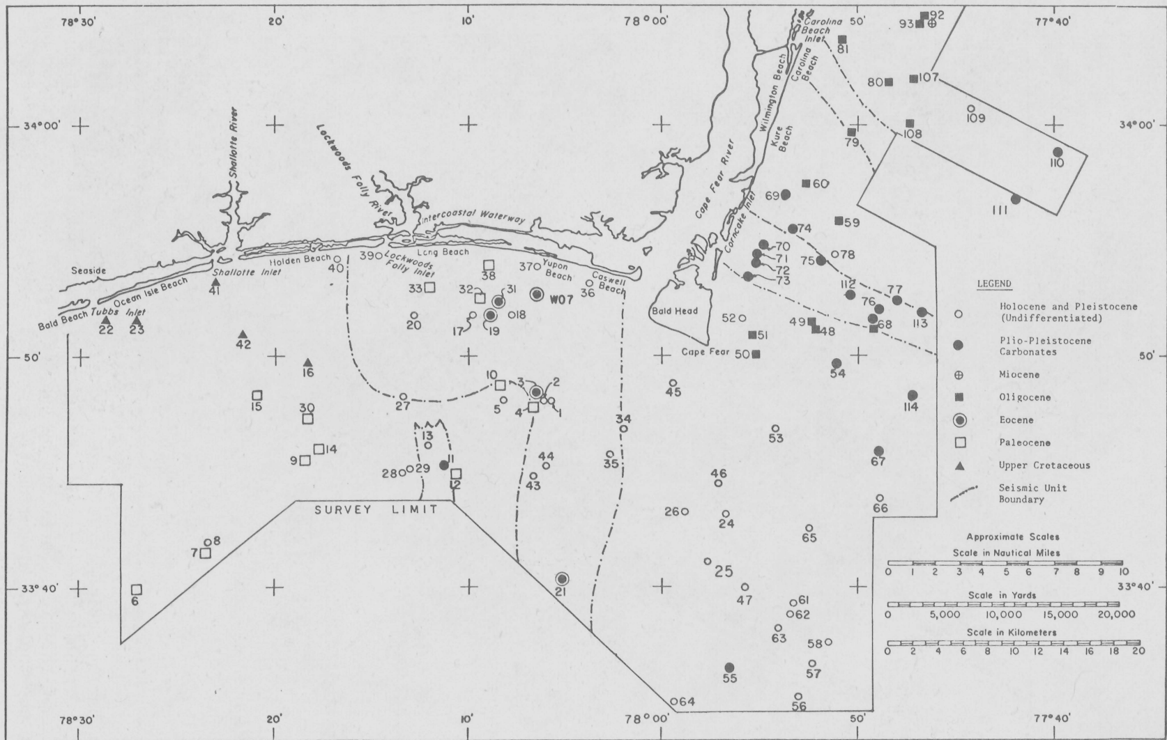
Figure 23. Probable age of sediments in the western part of the main survey area.
