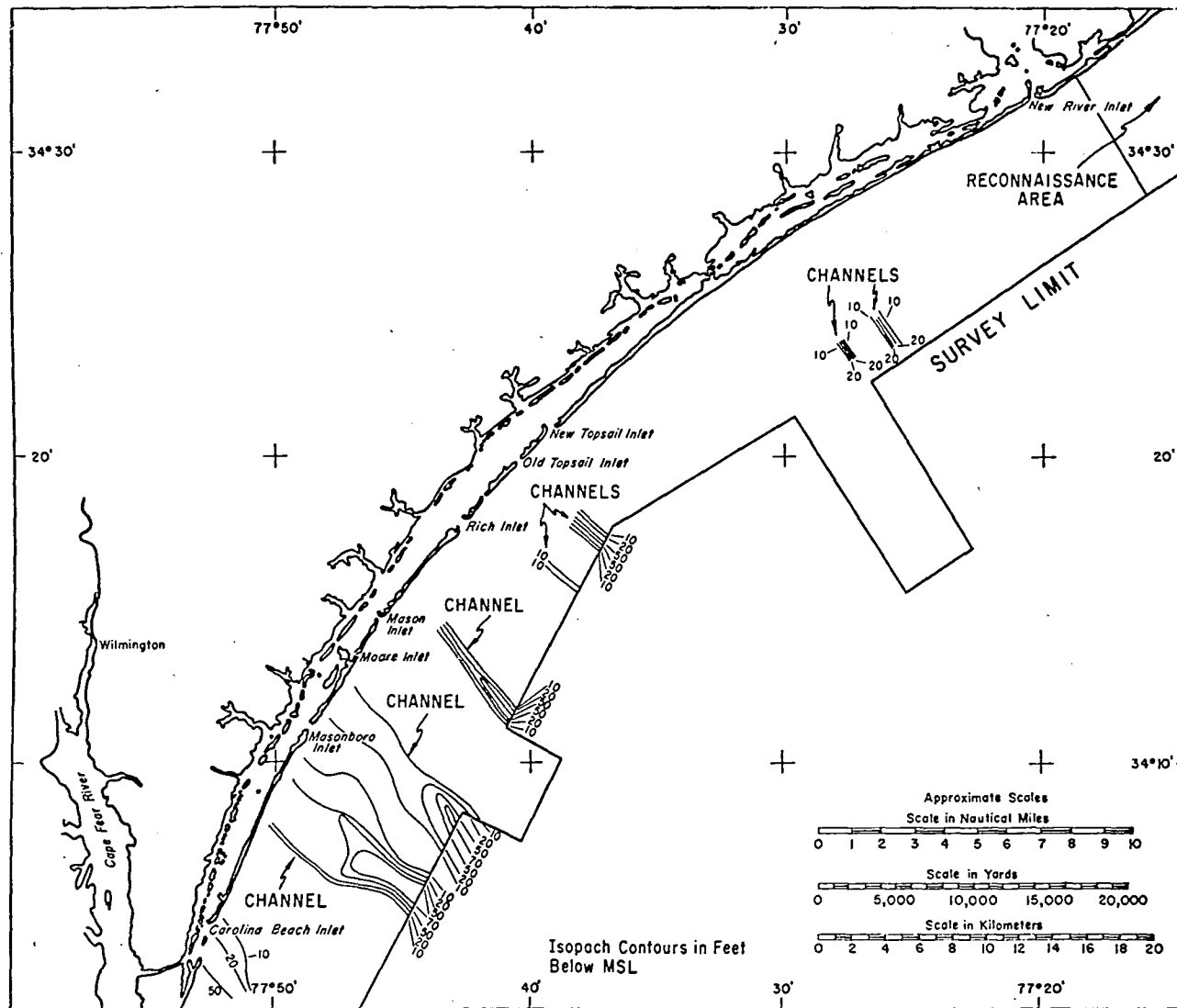
Figure 8. Isopach map showing the surfaces of reflection unit III and base of unit IV in the western part of the main survey area.
