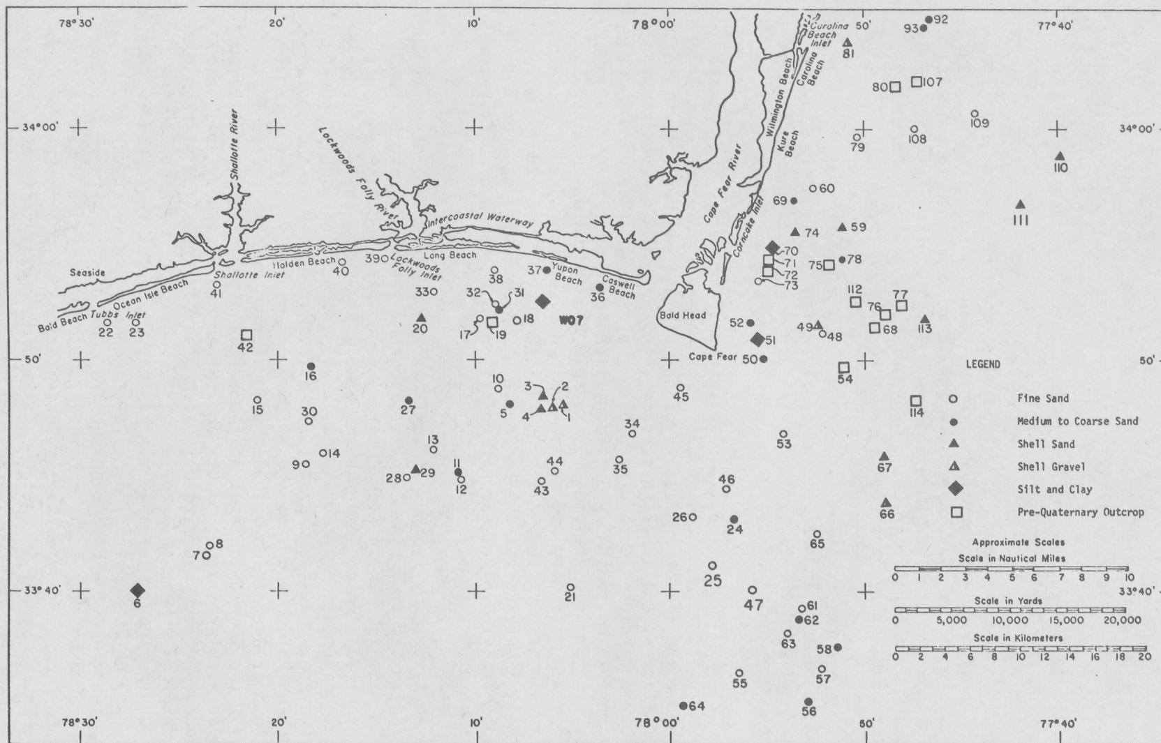
Figure 26. Map of the western part of the main survey area showing surface sediment characteristics in the numbered ICONS cores (see App. B for core descriptions).
