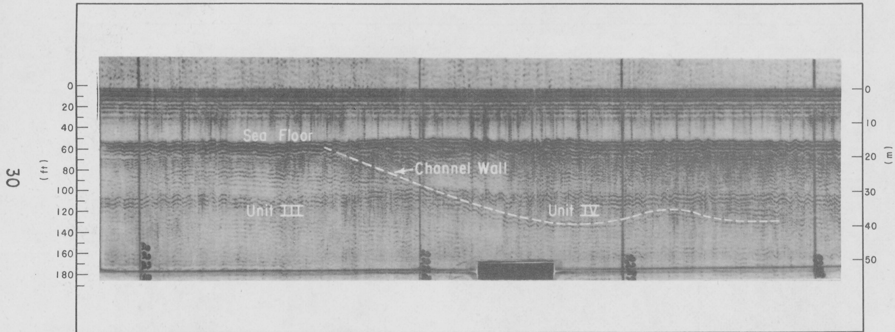
Figure 14. Seismic reflection profile showing typical internal reflection patterns in reflection unit IV.
