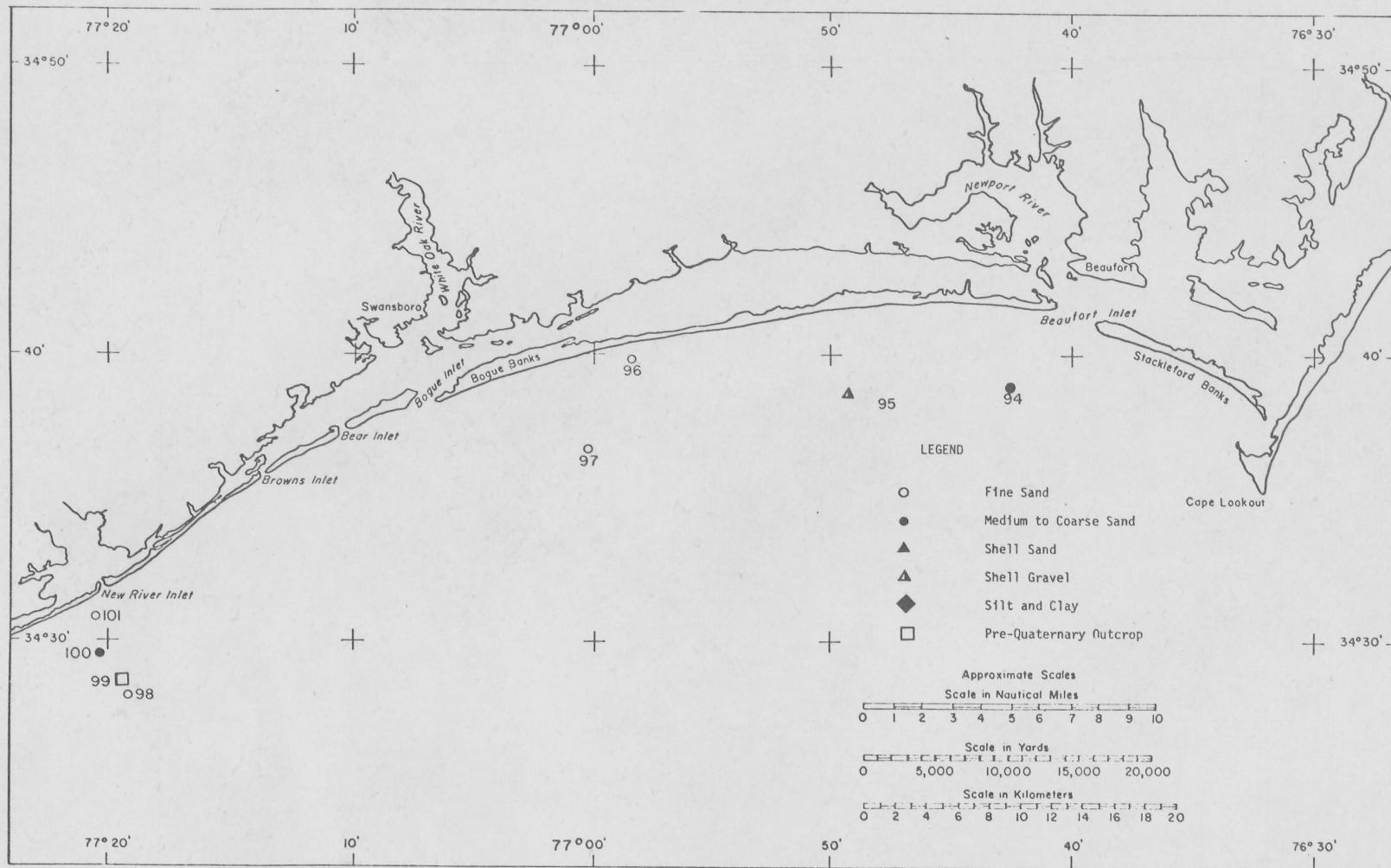
Figure 28. Map of the reconnaissance area showing surface sediment characteristics.
