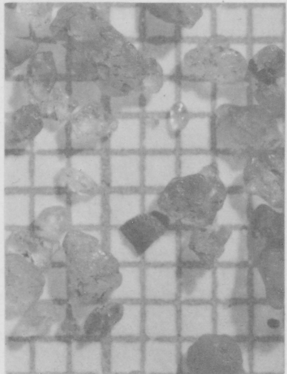
Figure 19. Typical examples of type D sediment (grid interval, 1 millimeter).
