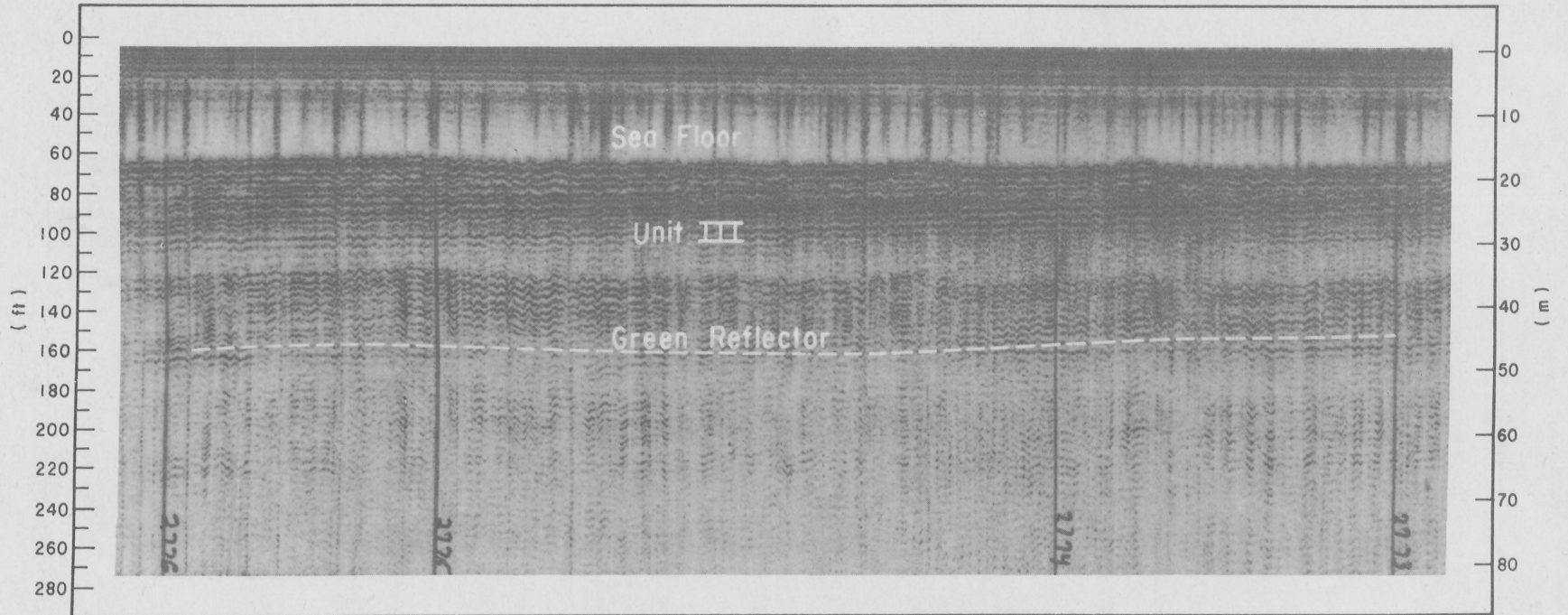
Figure 13. Seismic reflection profile showing the typical pattern of internal reflectors in reflection unit III.
