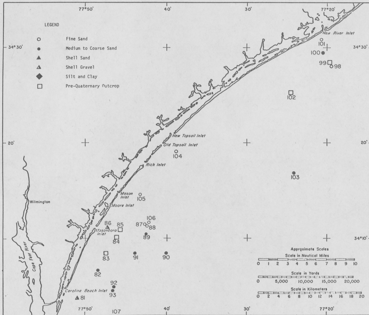
Figure 27. Map of the northeastern part of the main survey area showing surface sediment characteristics.
