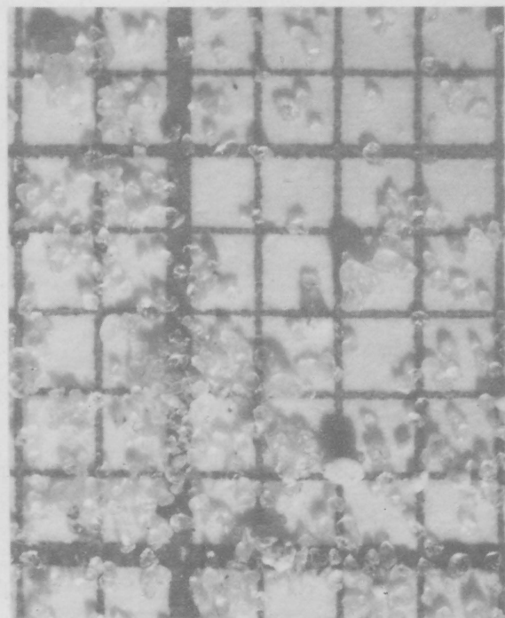
Figure 17. Photos of typical samples of type B, fine angular sand (grid interval, 1 millimeter).
