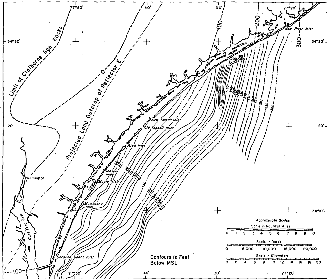
Figure 10. Contours on the surface of the green reflector in the central part of Onslow Bay.
