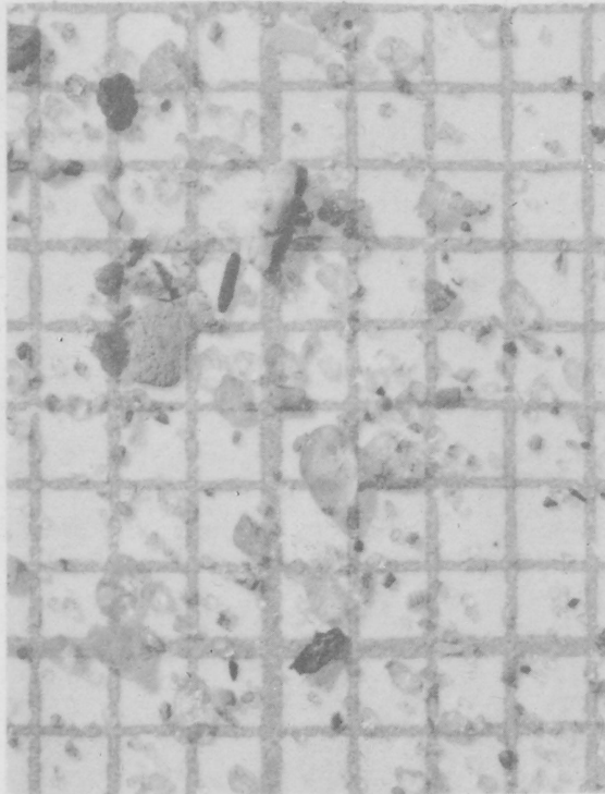
Figure 16. Photos of typical type A, shelf facies sand (grid interval, 1 millimeter).
