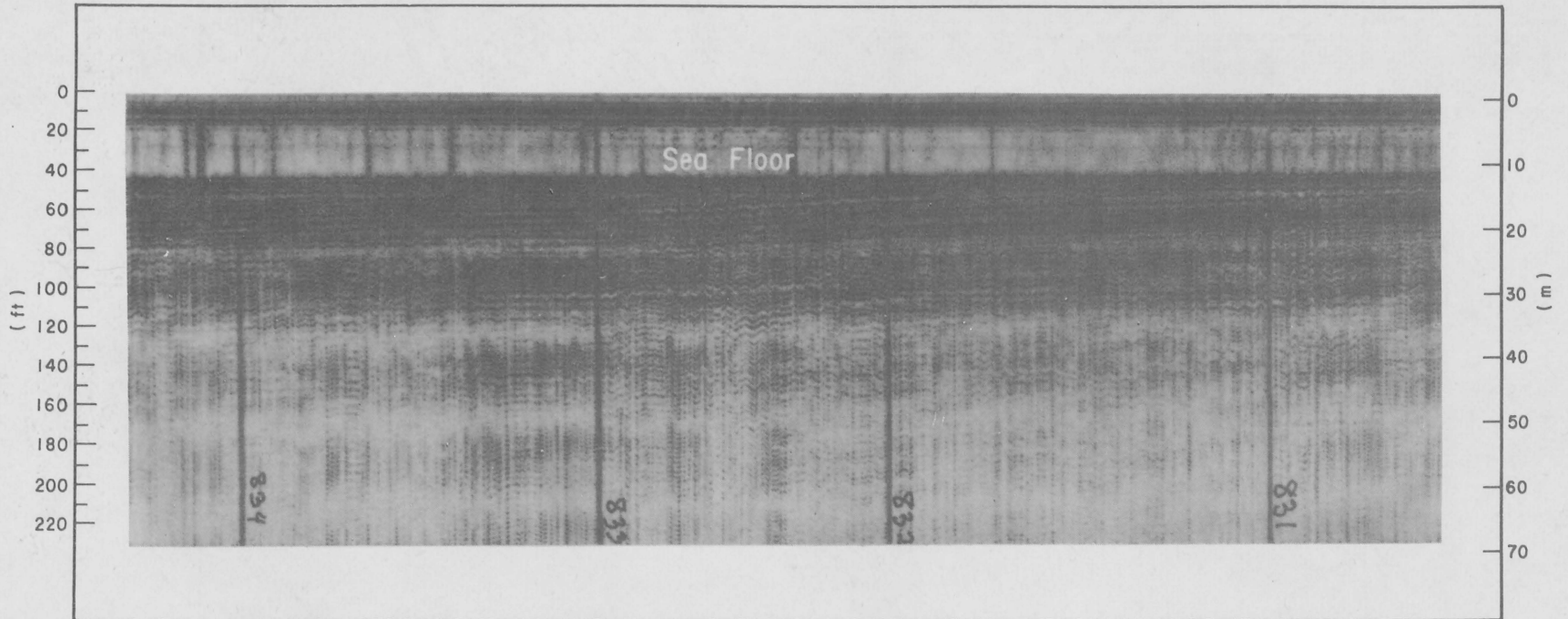
Figure 11. Seismic reflection profile showing the typical pattern of internal reflectors in reflection unit I.
