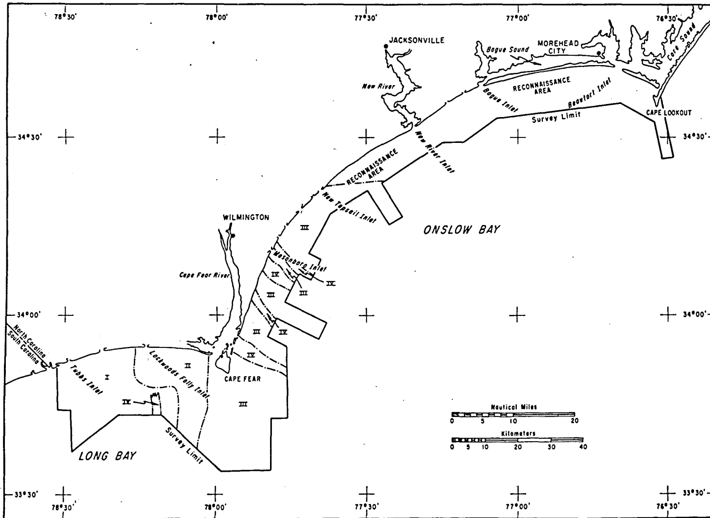
Figure 6. Map of the study area showing outcrop or shallow subcrop areas (generally less than 3 meters) of the various reflection units.
