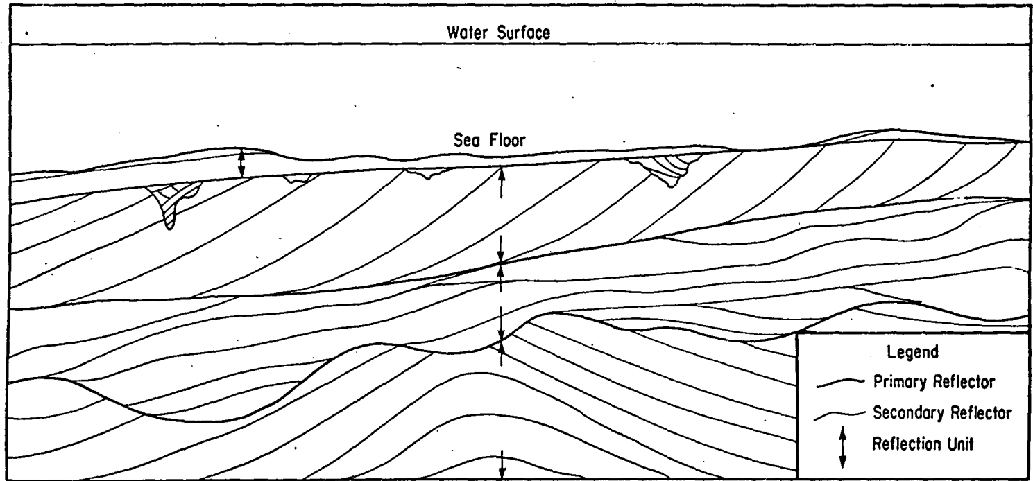
Figure 5. Idealized seismic reflection profile showing primary and secondary reflectors and a reflection unit.
