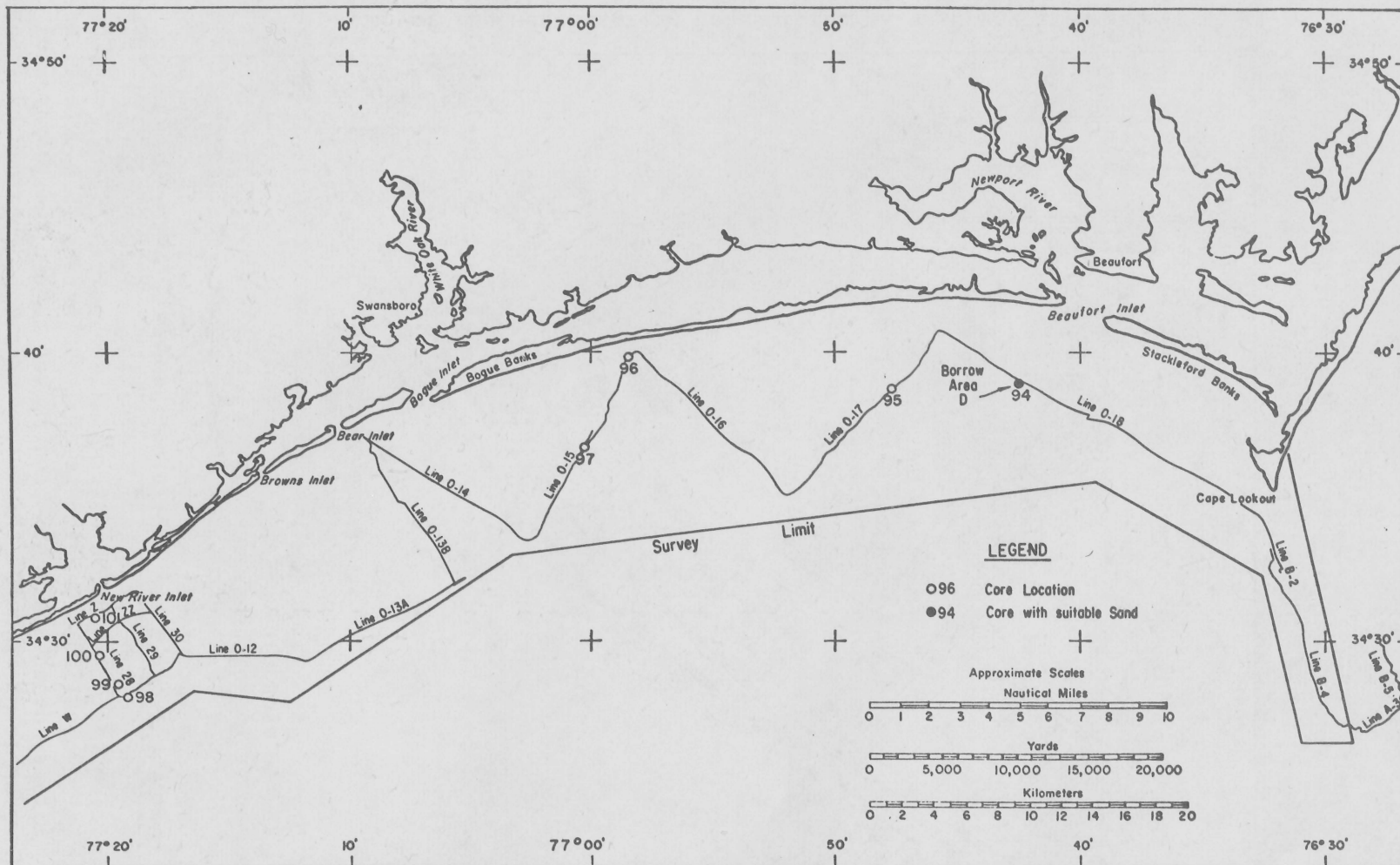
Figure 4. Map of the reconnaissance area showing seismic reflection and core coverage.
