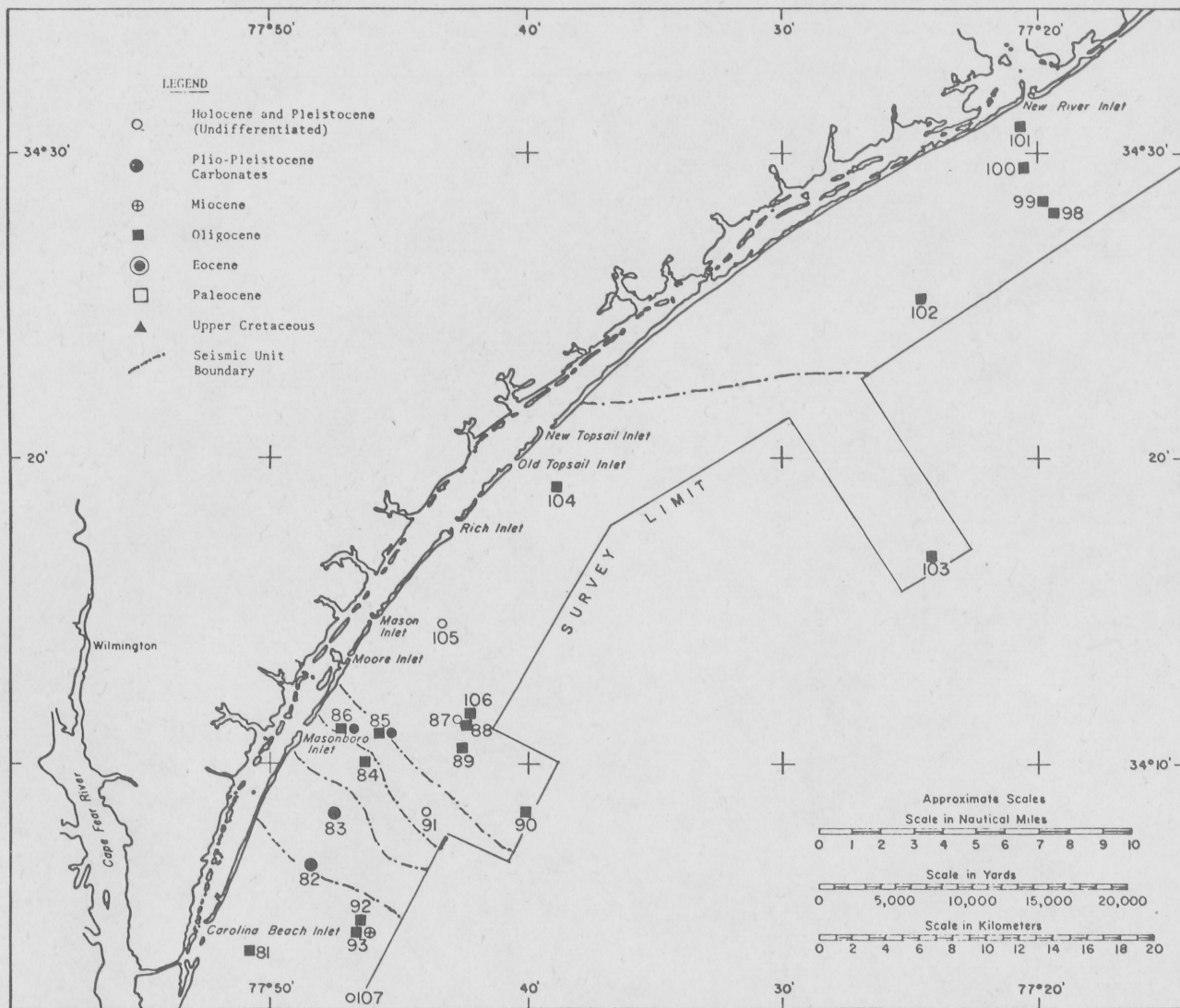
Figure 24. Probable age of sediments in the northeastern part of the main survey area.
