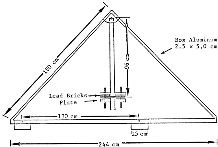
Figure 10. Calibrated creeper.
