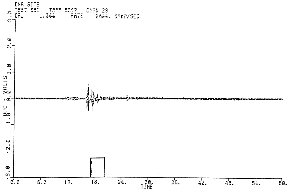
b. FPS response to a dog intrusion.
