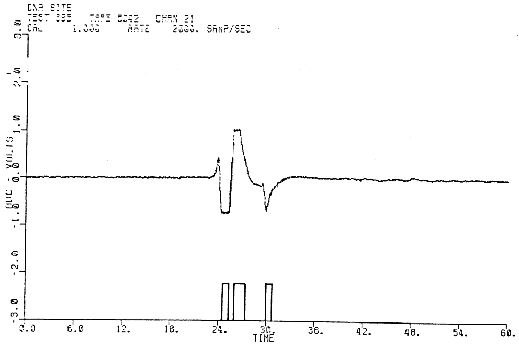
a. E-field responses to a man-run.
