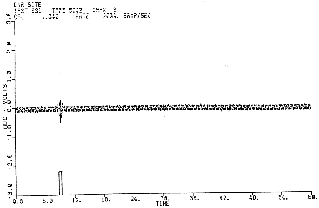
a. MAID/MILES responses to a man-run.
