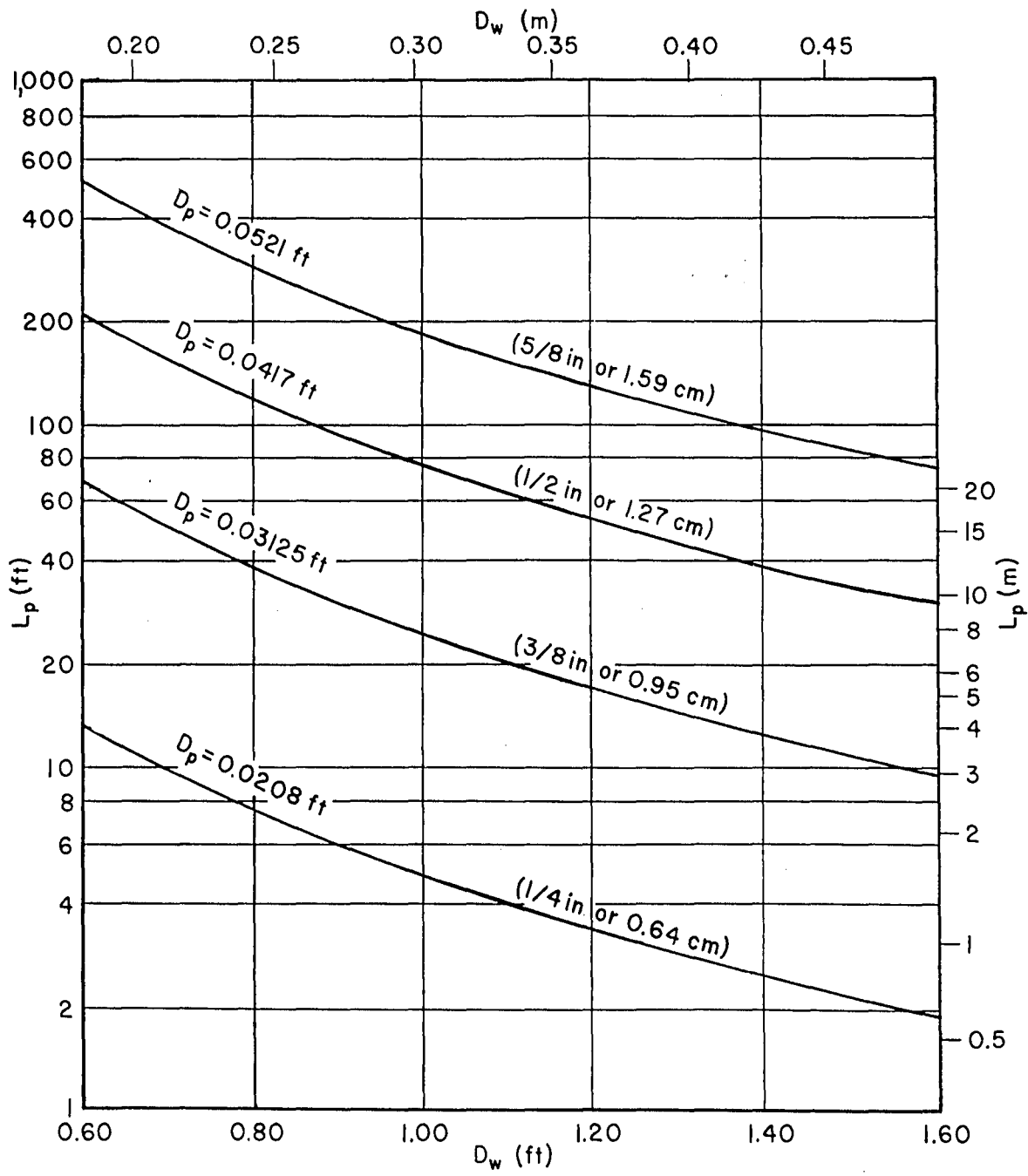
Figure 4. Theoretical linear stilling well design to obtain 90 percent of a 1-hour wave.
