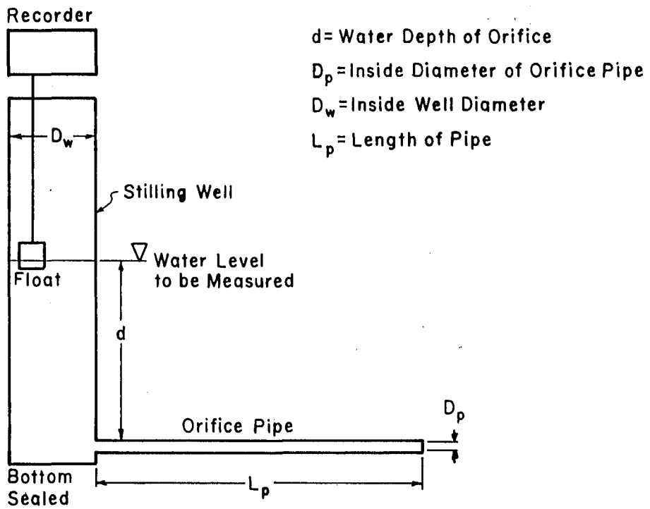
Figure 2. The linear stilling well.
