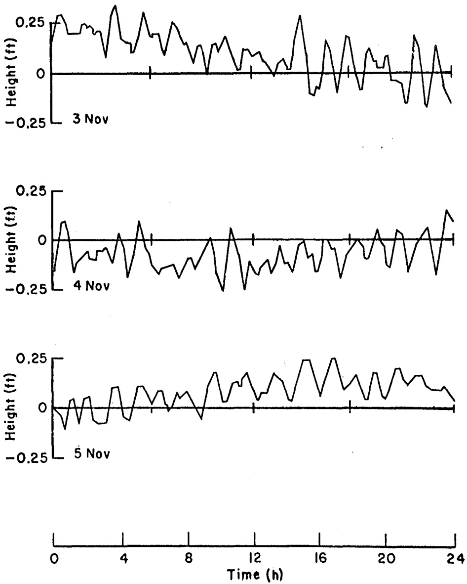
Figure 7. Pentwater water levels, November 1974.
