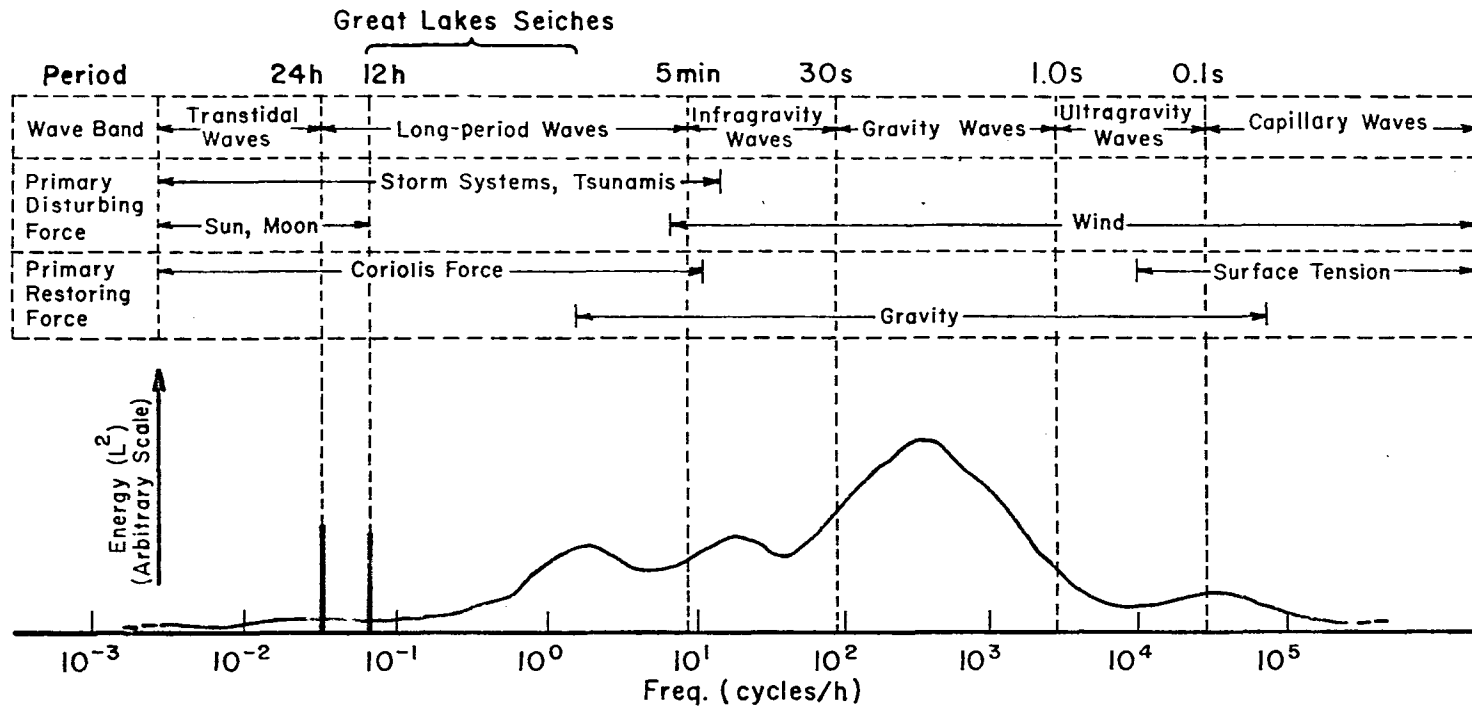
Figure 1. Approximate distribution of ocean surface wave energy illustrating the classification of surface waves by wave band, primary distributing force, and primary restoring force.
