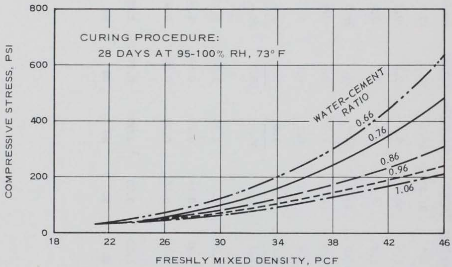
Figure 3.1 Strength versus density for a neat (no aggregate) cellular concrete (Reference 14).
