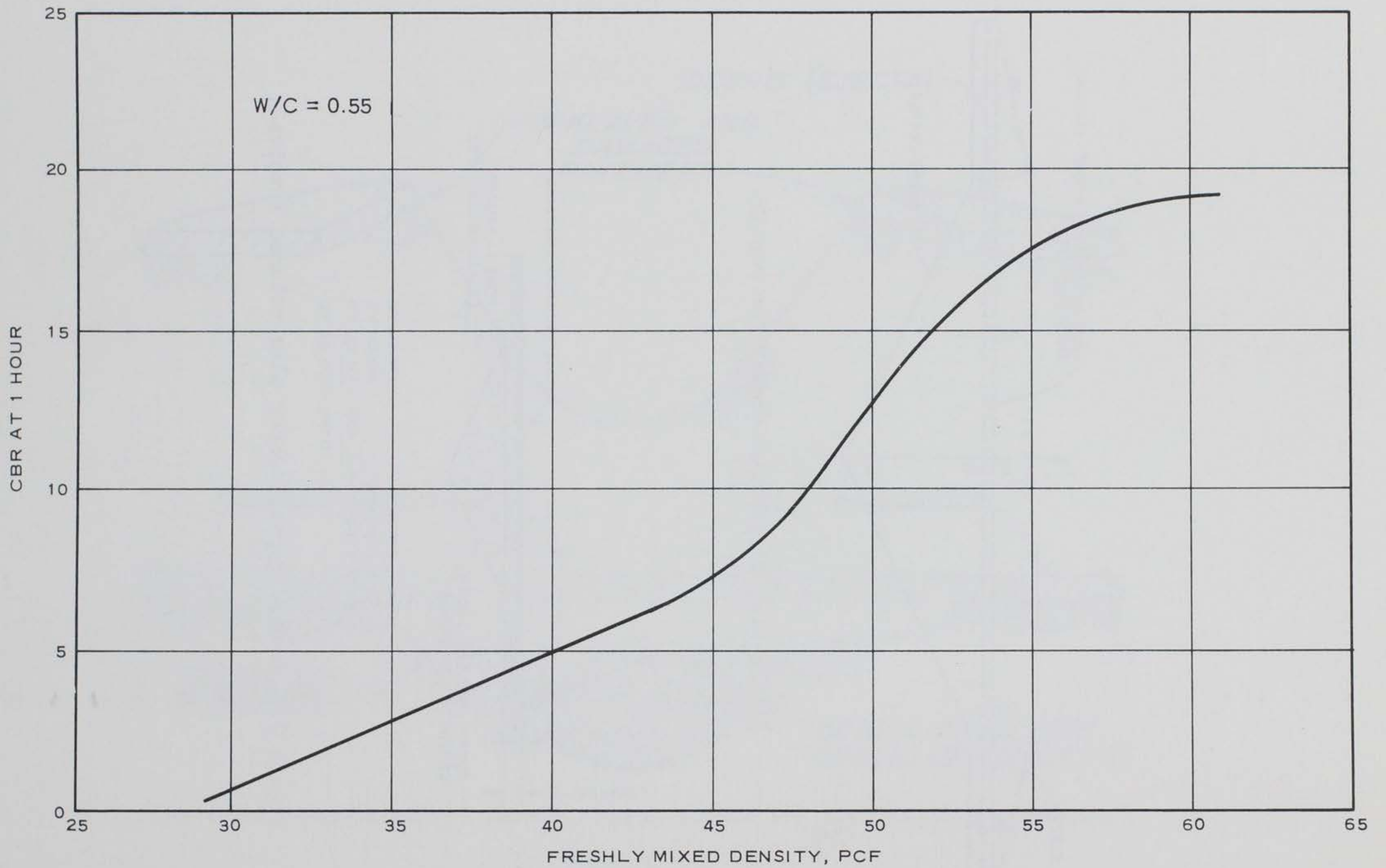
Figure 2.4 One-hour CBR value versus density for a neat cellular concrete.
