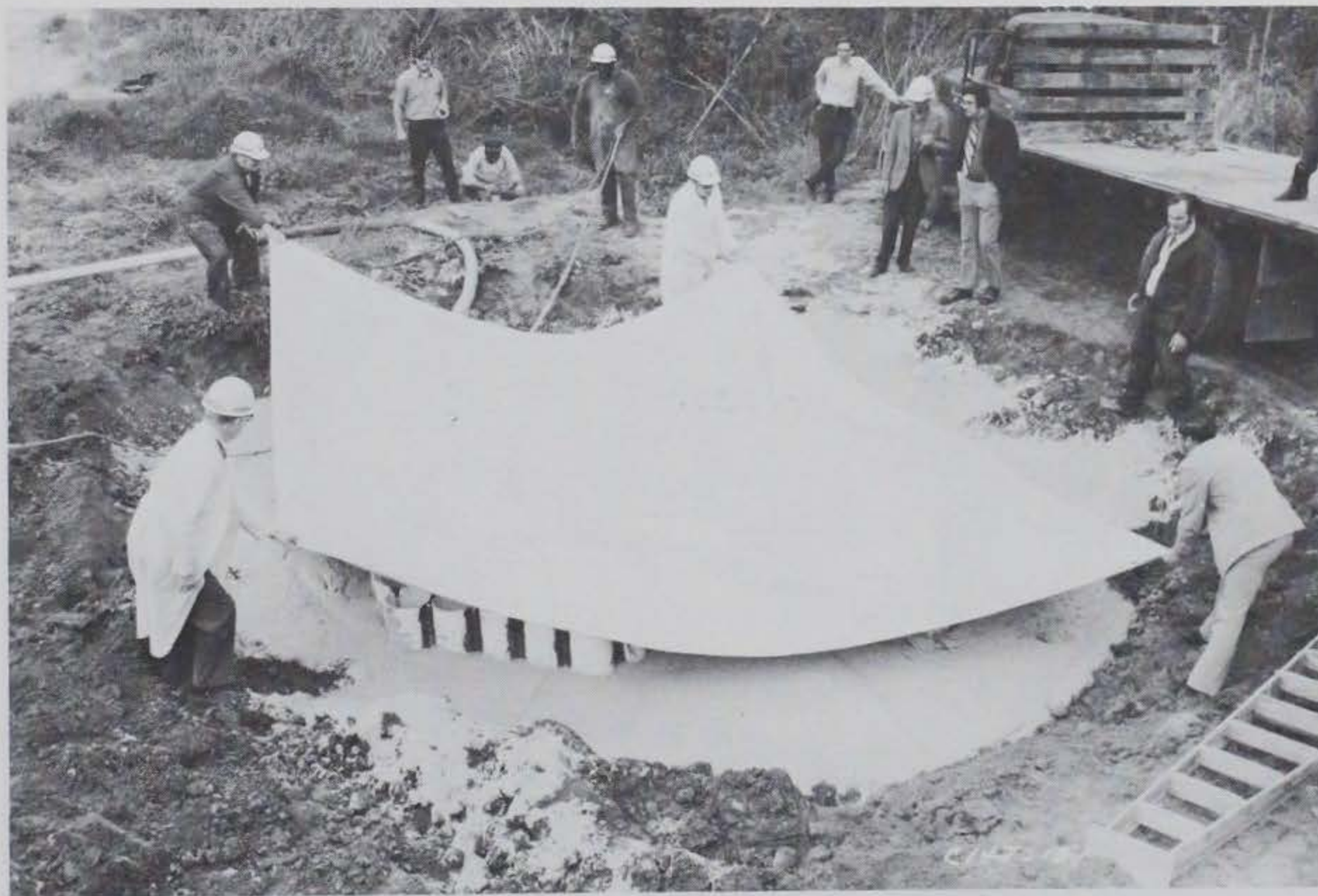
Figure 5.18 Covering the pipe openings with a nylon sheet.
