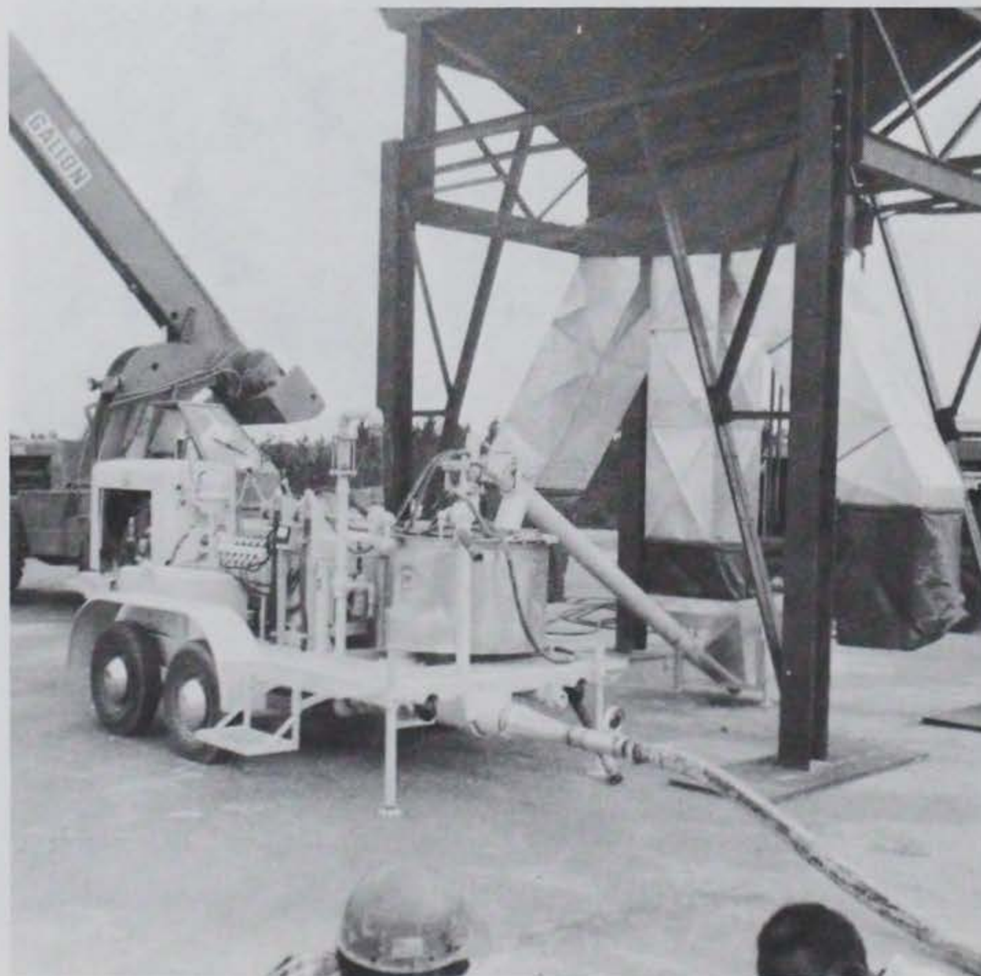
Figure 5.32 Batching and pumping equipment arrangement.
