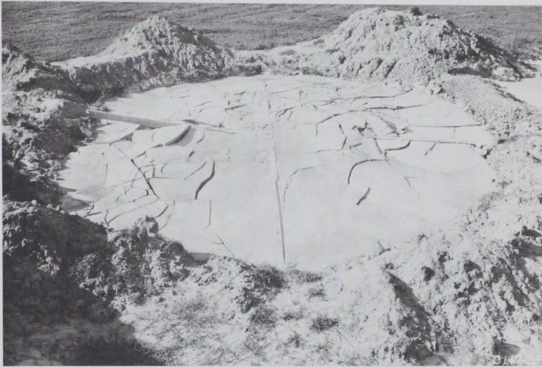
Figure 5.29 Severe drying shrinkage cracking.
