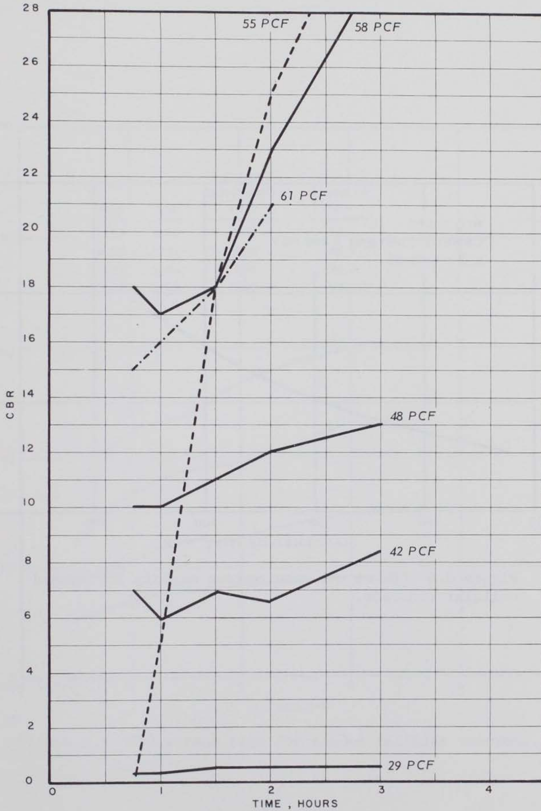
Figure 2.5 CBR value versus elapsed time for neat cellular concretes of various densities.
