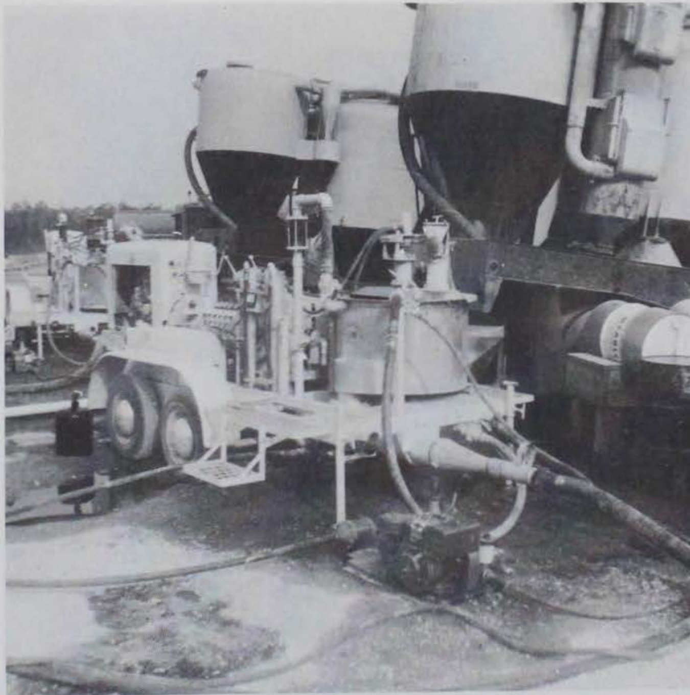
Figure 5.38 Unit 1, foam generator, and cement supply arrangement.
