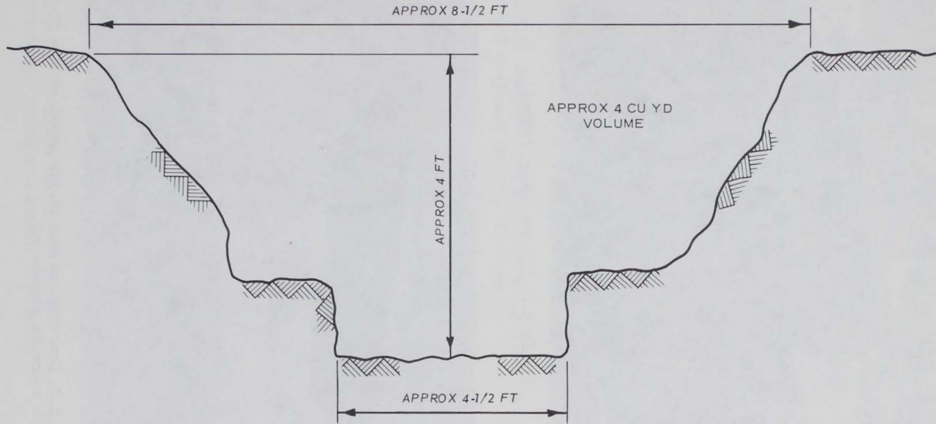
Figure 5.1 Cross section of small simulated crater.
