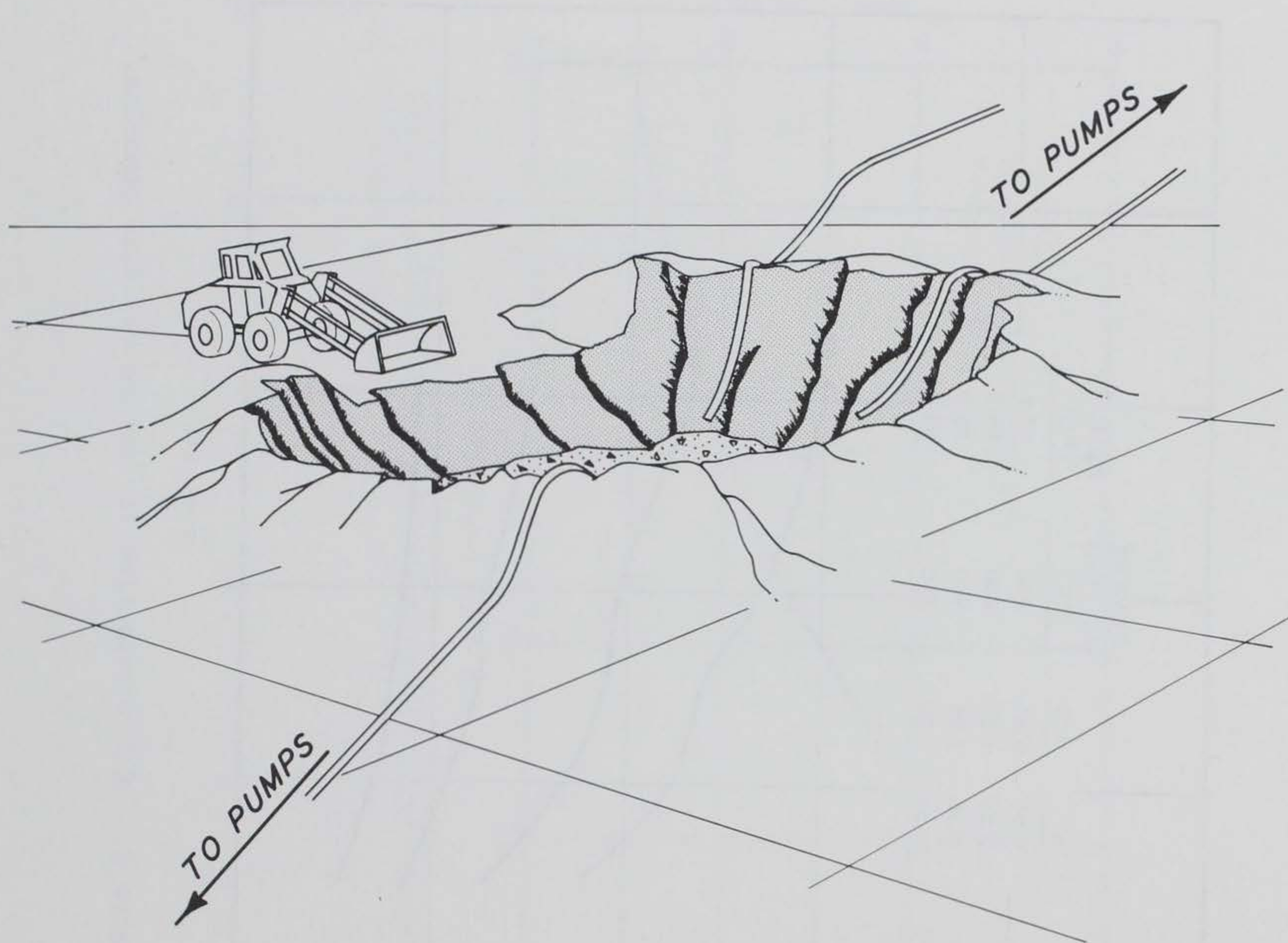
Figure 2.8 Concurrent filling of crater with debris and neat cellular concrete.
