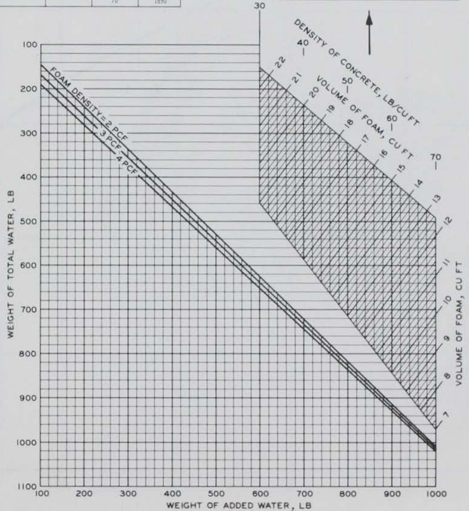
Figure 3.9 Nomograph for proportioning neat cellular concrete.
