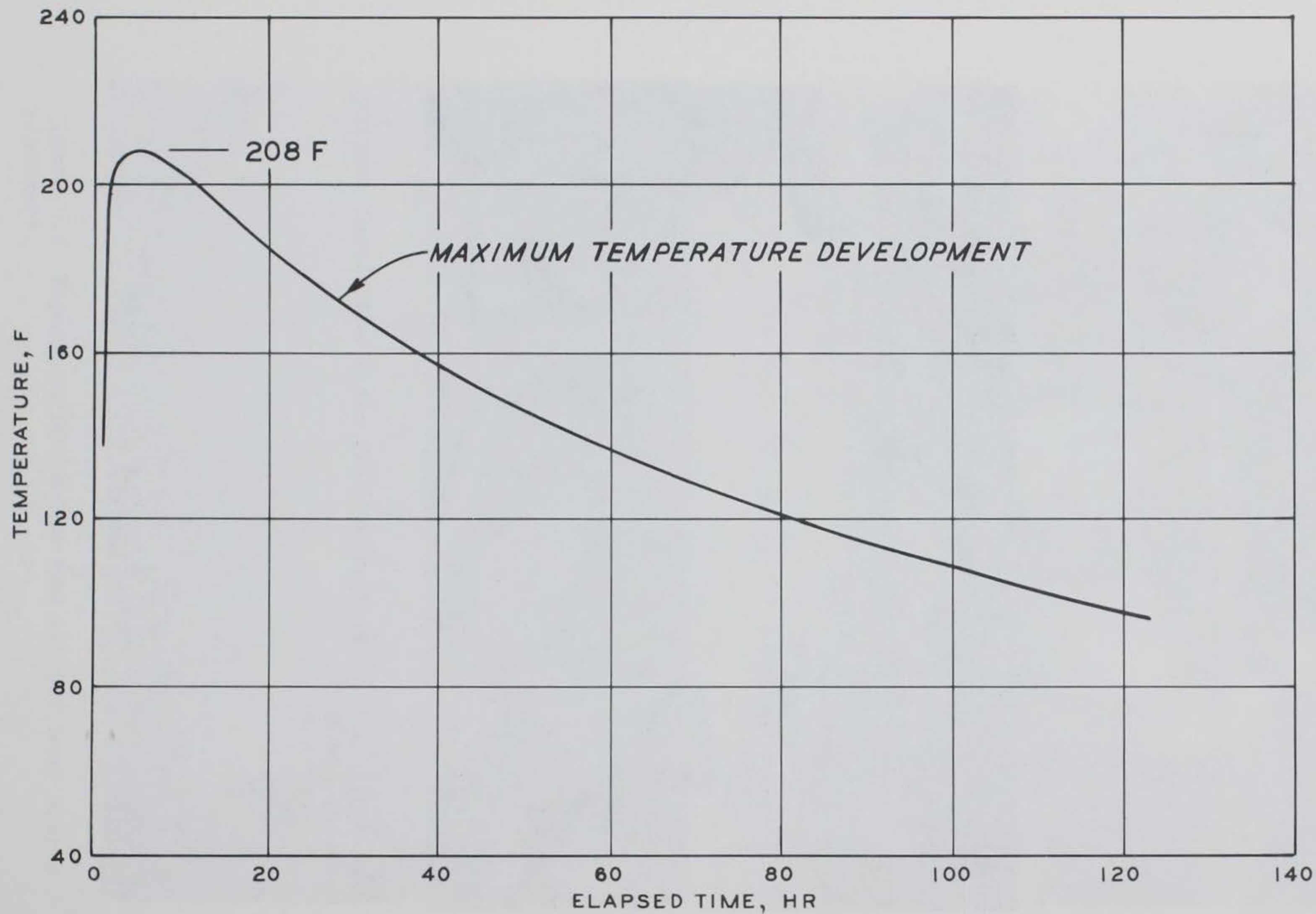
Figure 5.9 Maximum temperature development versus time after placing relation for simulated crater repair.
