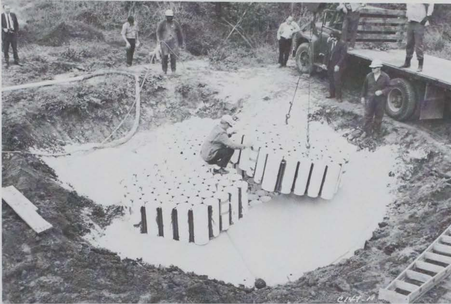
Figure 5.17 Positioning of top layer of modules.
