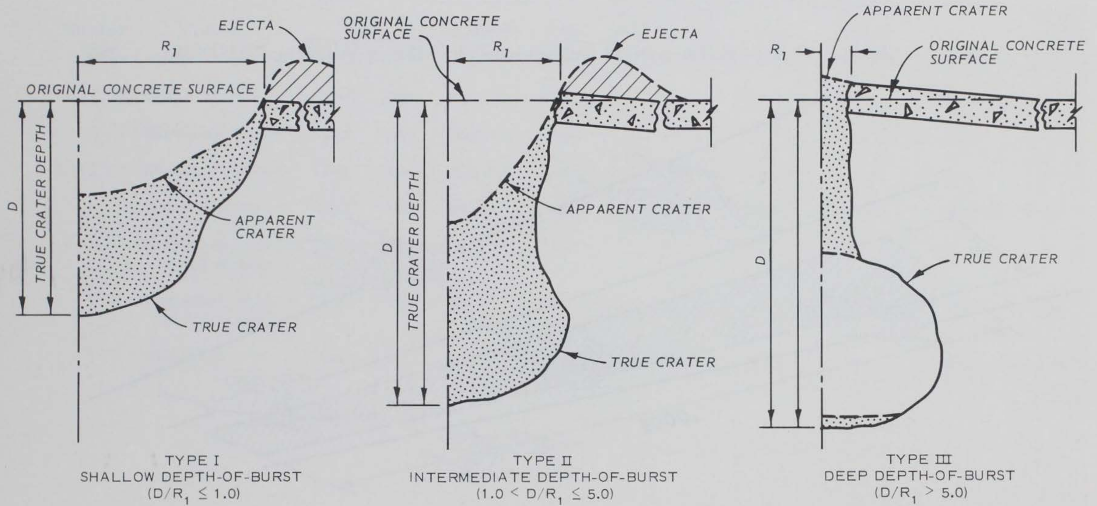
Figure 1.2 U. S. Air Force pavement crater classifications (Reference 2).
