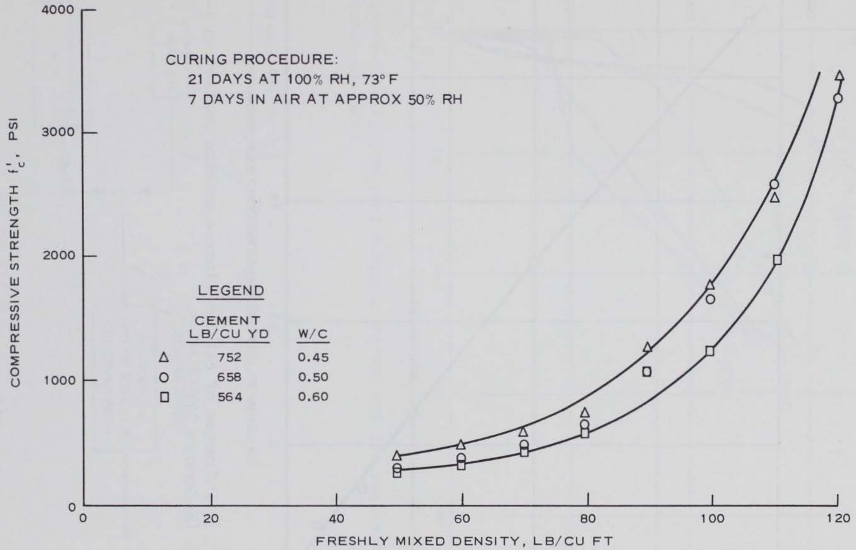
Figure 3.2 Strength versus density for sanded cellular concretes (Reference 13).
