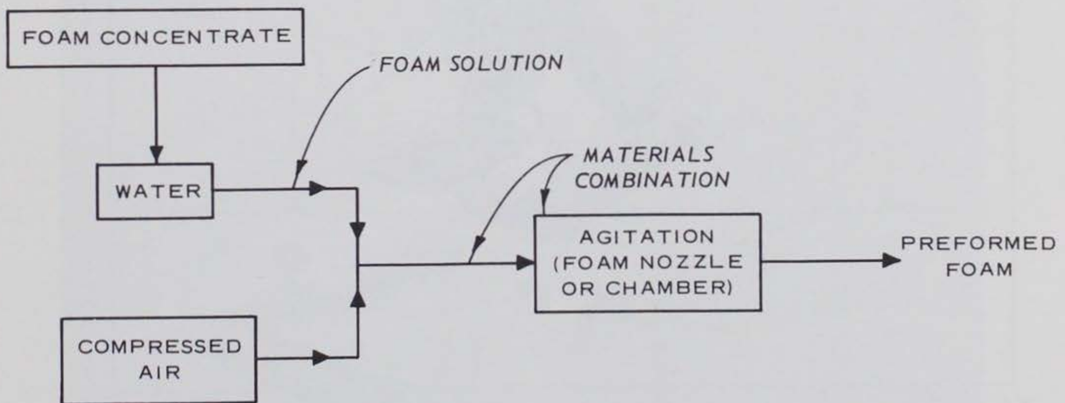
Figure 3.5 Preformed foam generation system.
