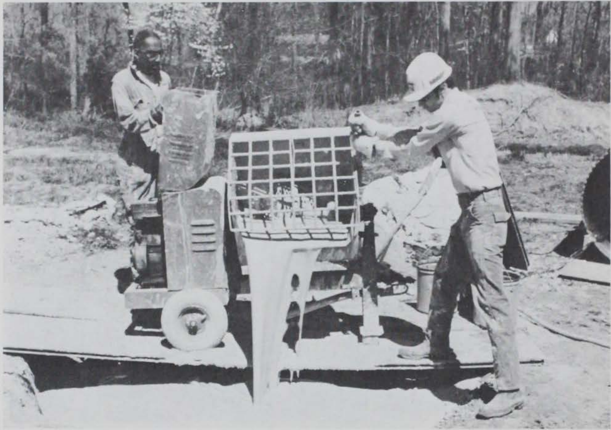
Figure 5.6 Placement of the 85-pcf cellular concrete.
