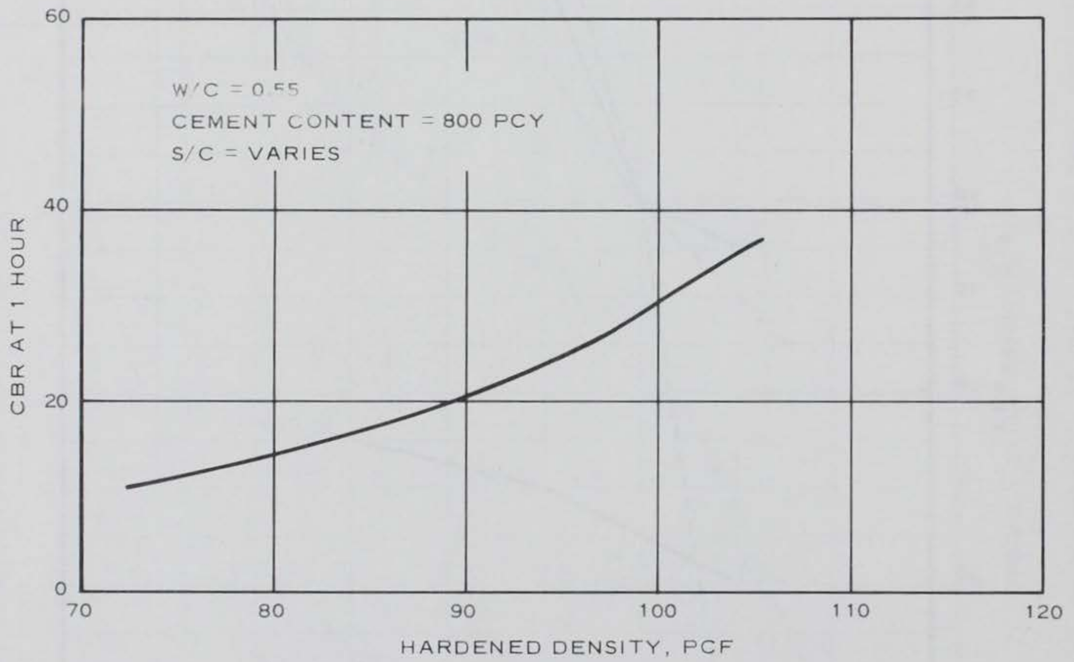
Figure 2.6 CBR at one hour versus density for sanded cellular concrete.
