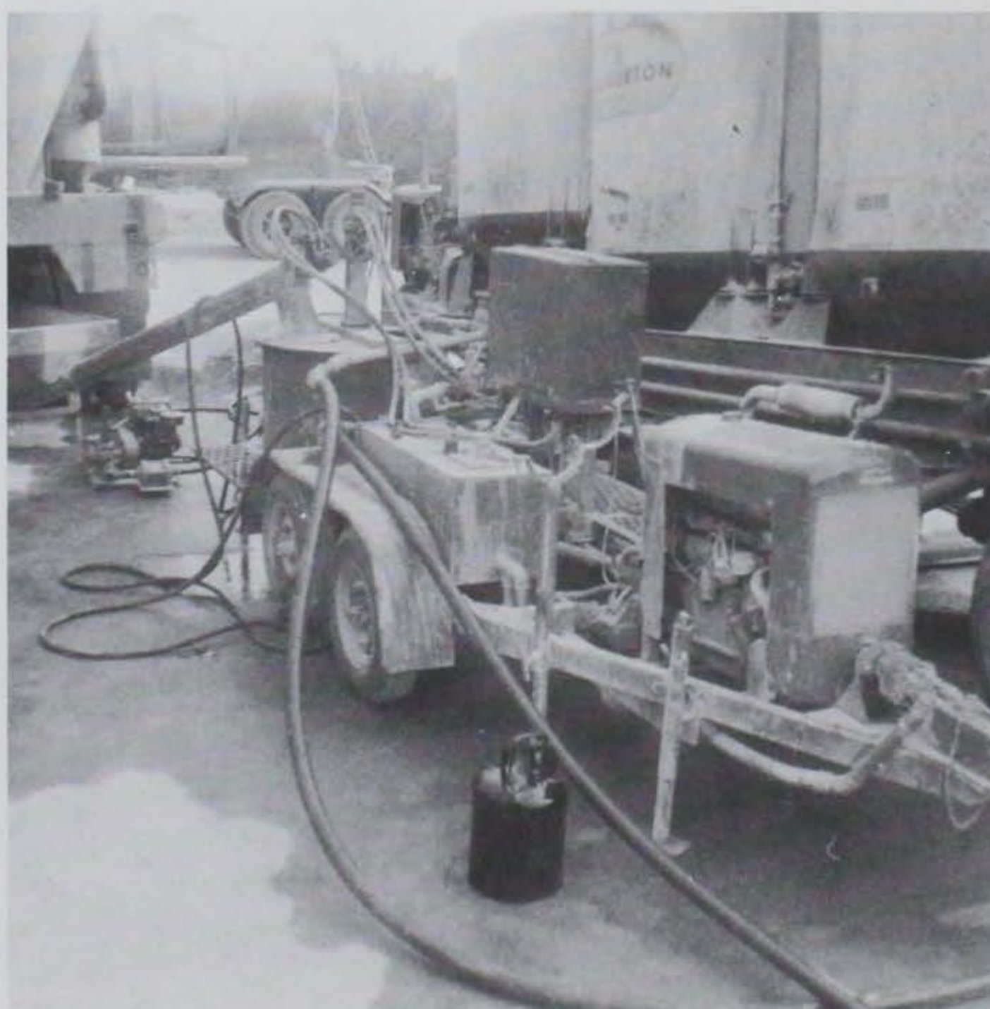
Figure 5.40 U. S. Air Force unit, foam generator, and cement supply arrangement.
