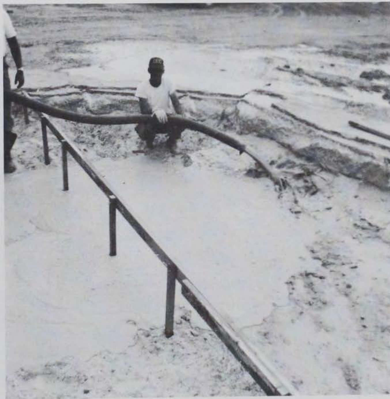
Figure 5.58 Placement of cellular concrete fill.
