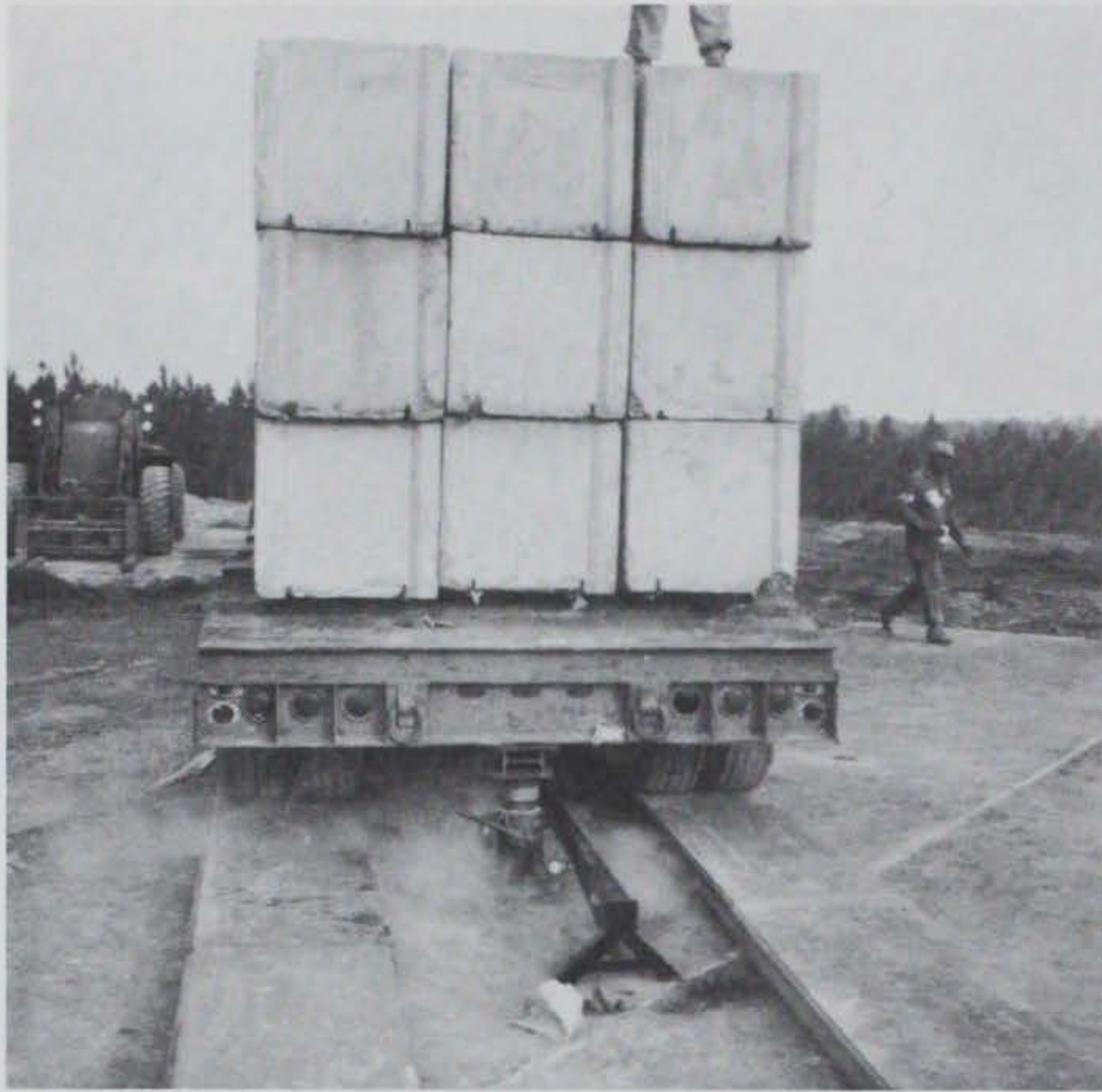
Figure 5.51 Loading of repaired crater. Note reference beam in foreground.
