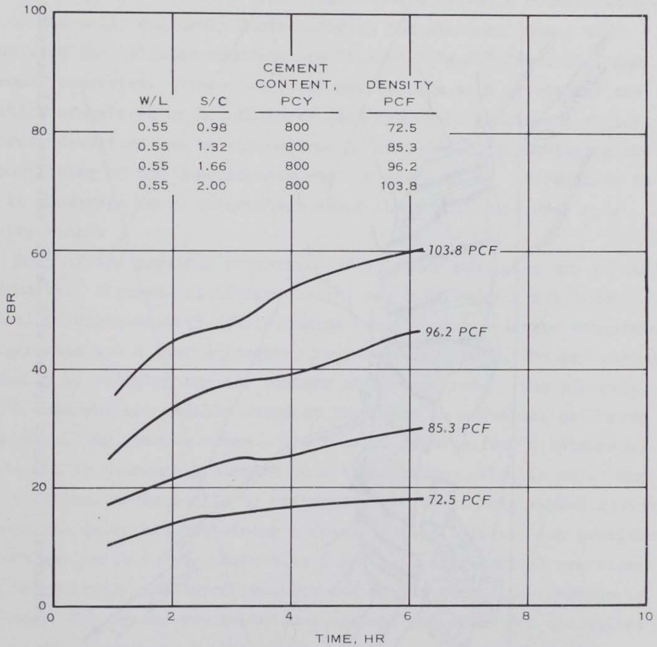
Figure 2.7 CBR versus time for sanded cellular concrete.
