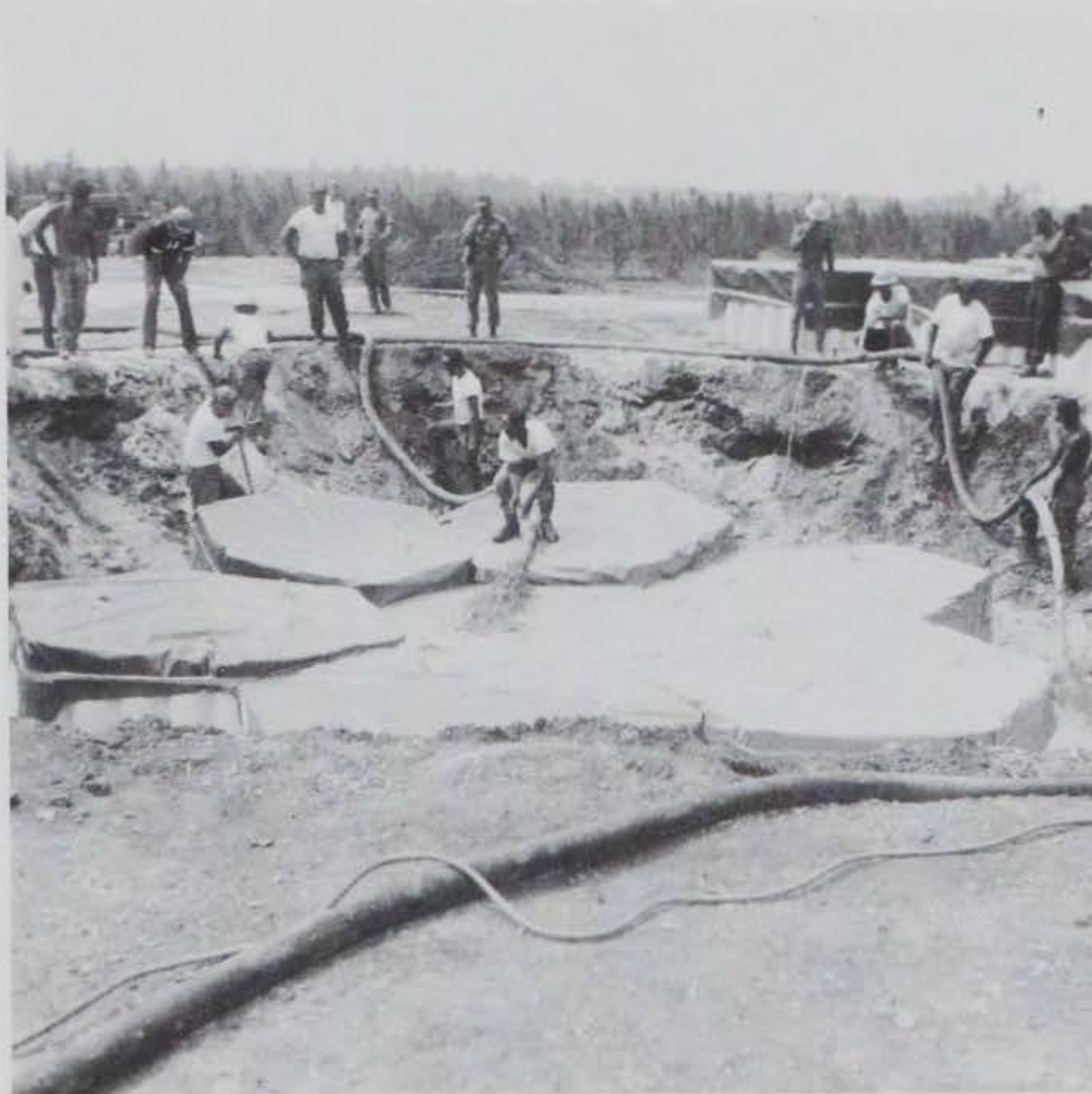
Figure 5.65 Placement of neat slurry between layers of modules.
