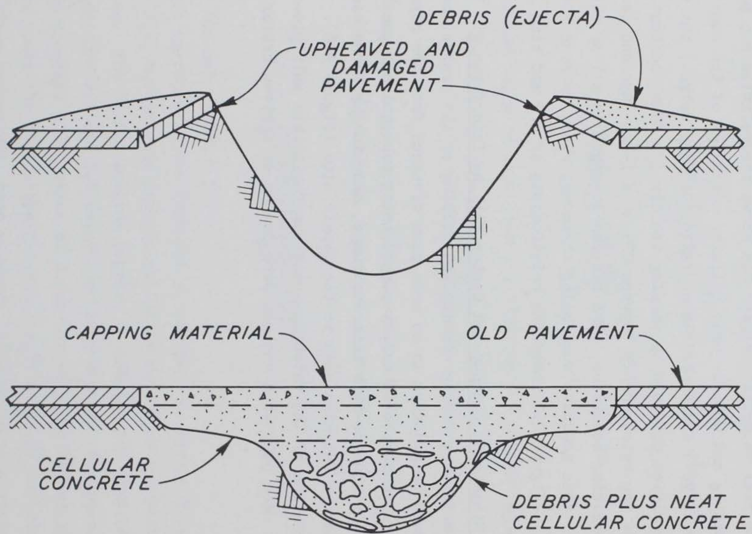
Figure 2.1 Regulated-set cement repair scheme for bomb-damaged pavements.
