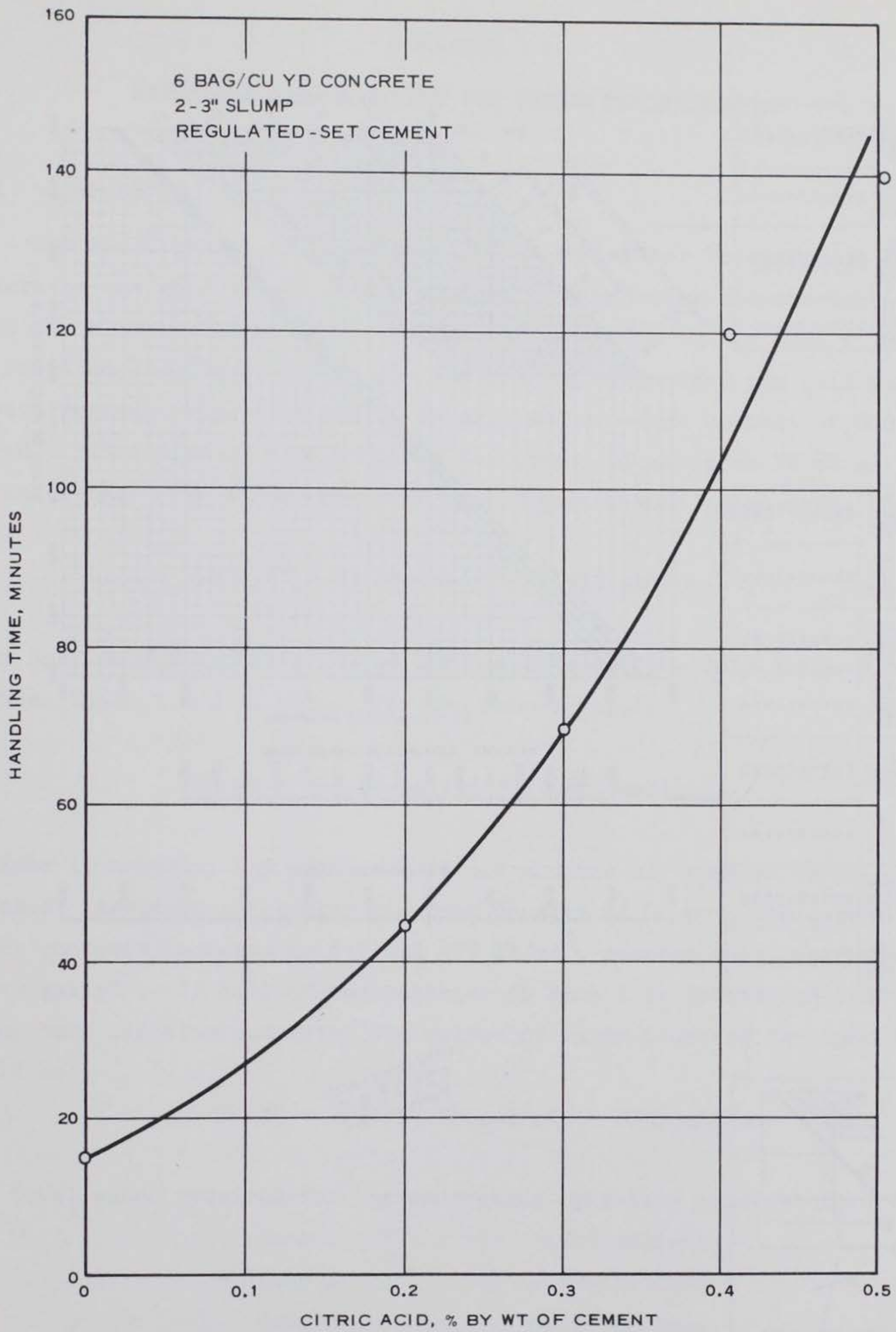
Figure 3.8 Effect of citric acid on handling time of concrete (Reference 17).
