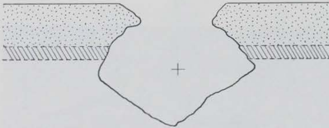
TYPE 5 - CAMOUFLET WITH SPALL CRATER
