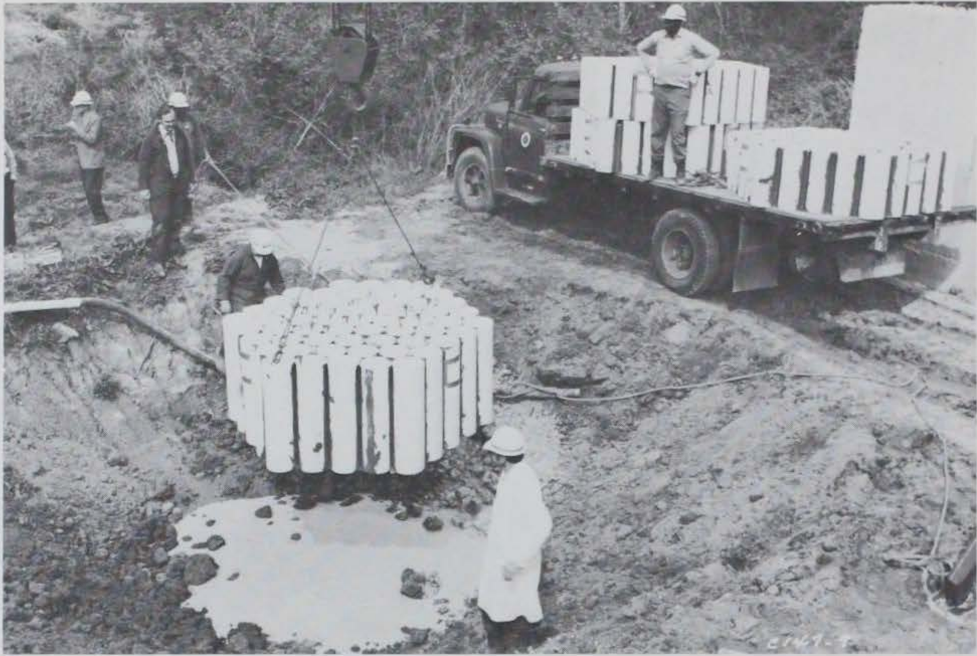
Figure 5.15 Placement of the bottom PVC pipe module.
