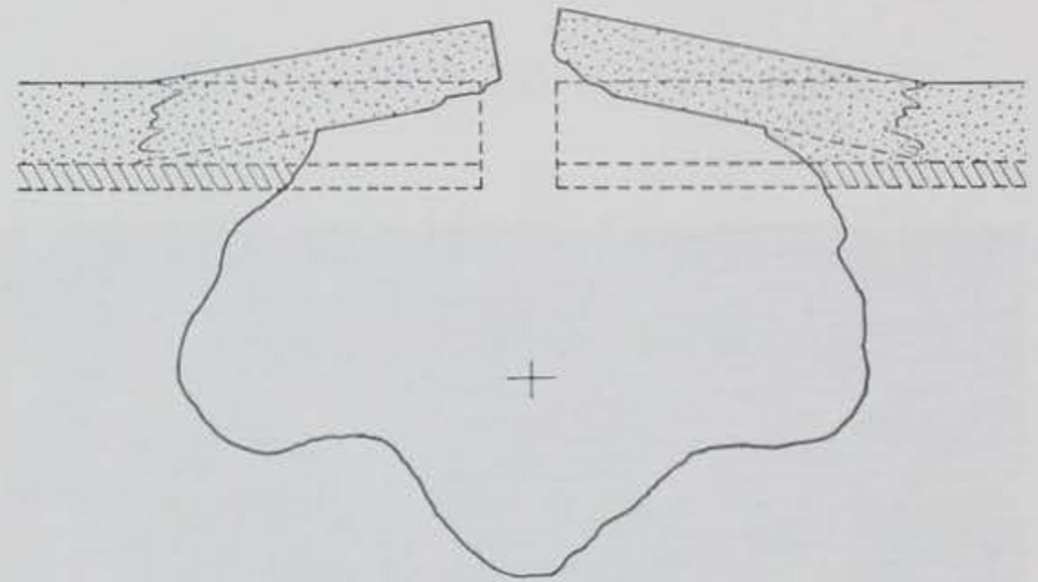
TYPE 6 - CAMOUFLET WITH HEAVE MOUND
