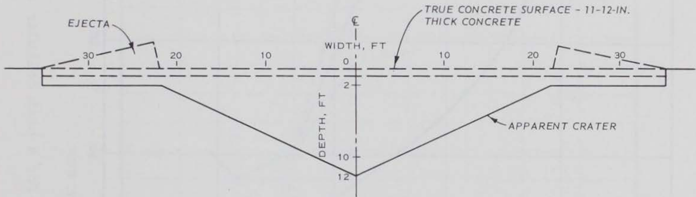
Figure 2.2 Simplified crater for repair.
