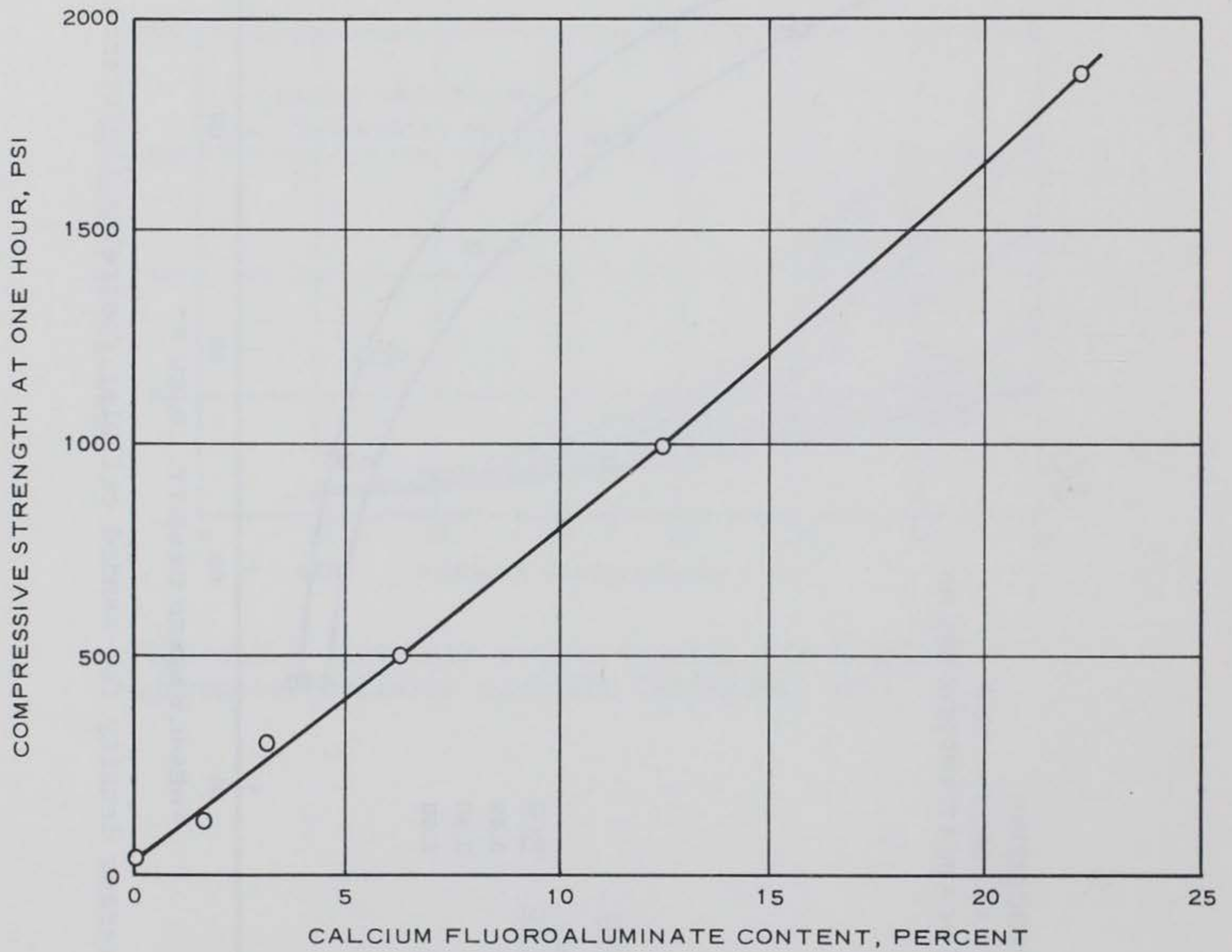
Figure 3.3 Influence of calcium fluoroaluminate content on 1-hour strength (Reference 17).
