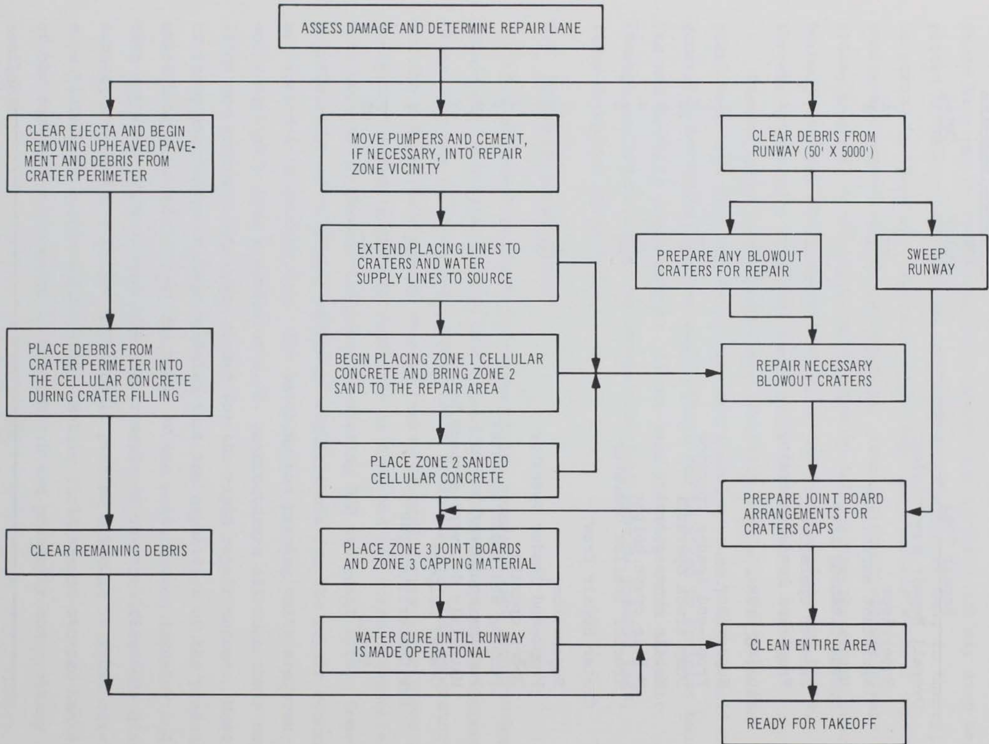
Figure 6.1 Regulated-set cement system repair flow diagram
