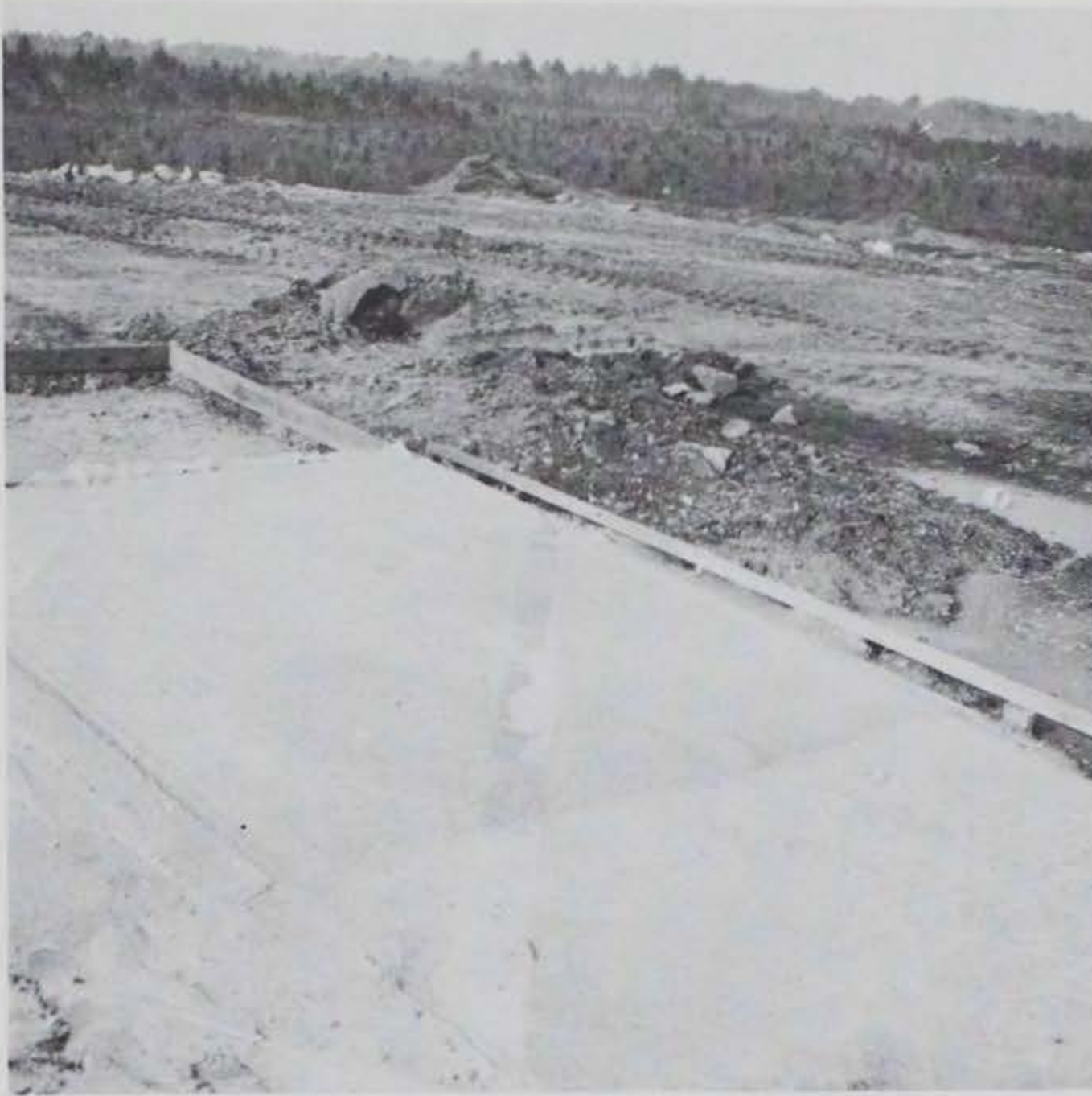
Figure 5.49 Rough screeded top surface of repair.
