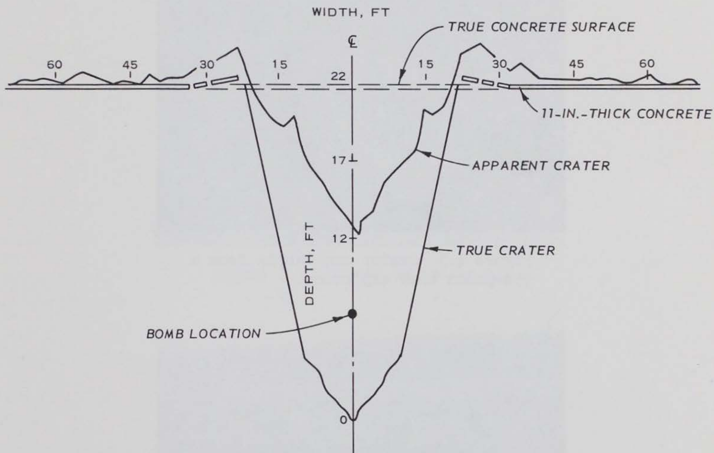
Figure 1.4 Cross section of 750-pound bomb crater, Hays, Kansas (Reference 4).
