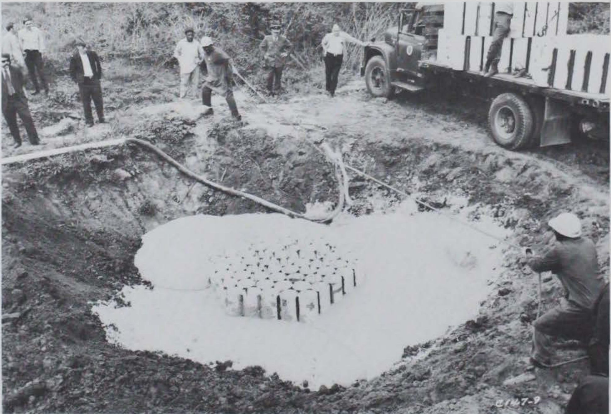
Figure 5.16 Placement of cellular concrete around bottom module.
