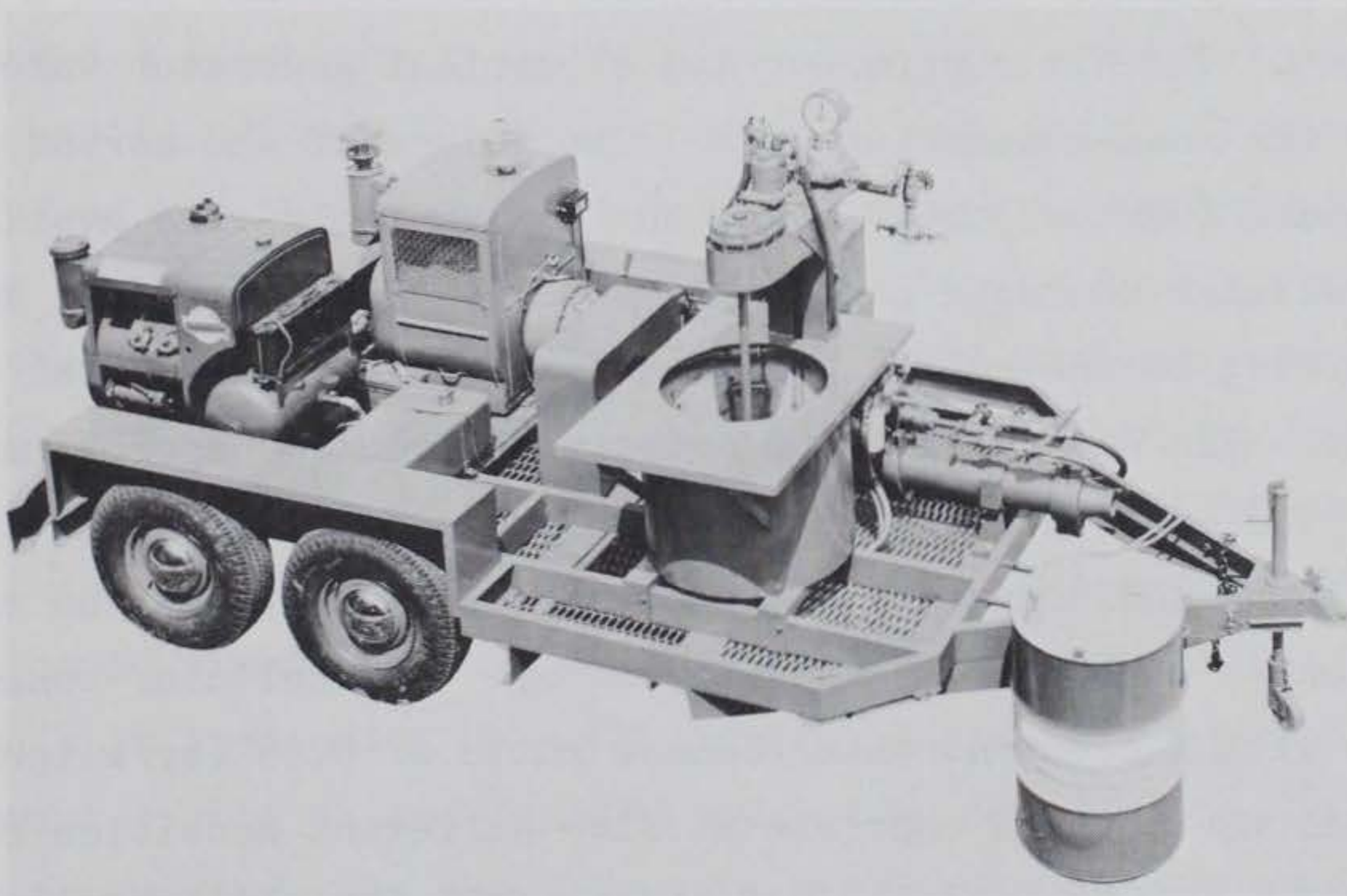
Figure 4.6 Self-contained cellular concrete production unit.
