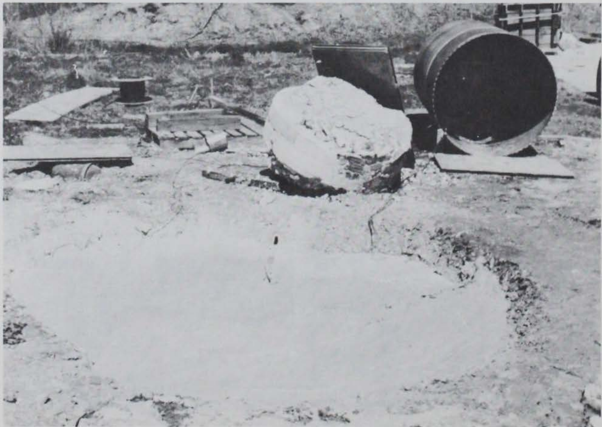
Figure 5.7 Repair surface after the 110-pcf neat slurry placement.
