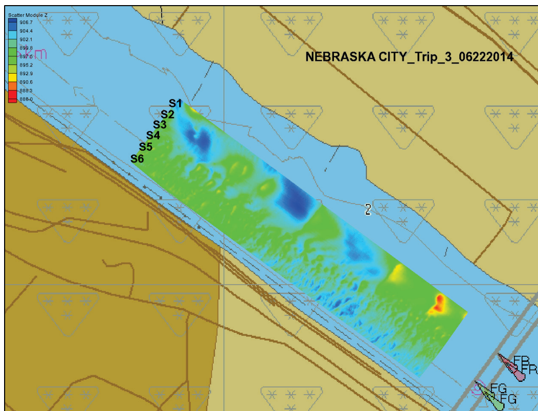
Figure 109. Bathymetry for Nebraska City, NE, showing swath locations.
