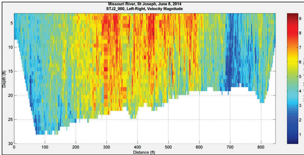
Figure 115. Velocity magnitude at St. Joseph, MO – June 8, 2014, 15:06:47.
