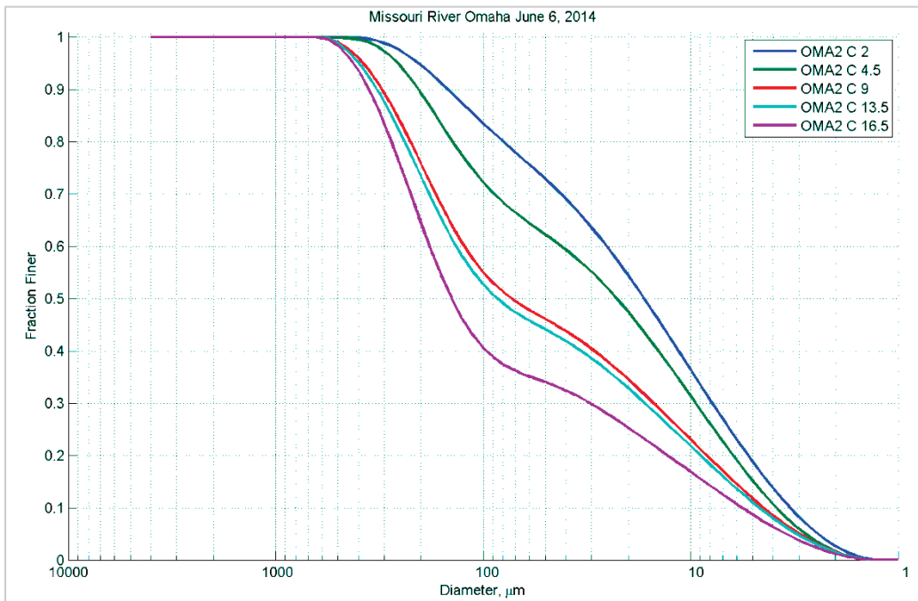
Figure 57. Particle size distribution at different depths (feet) in Station C – June 6, 2014.
