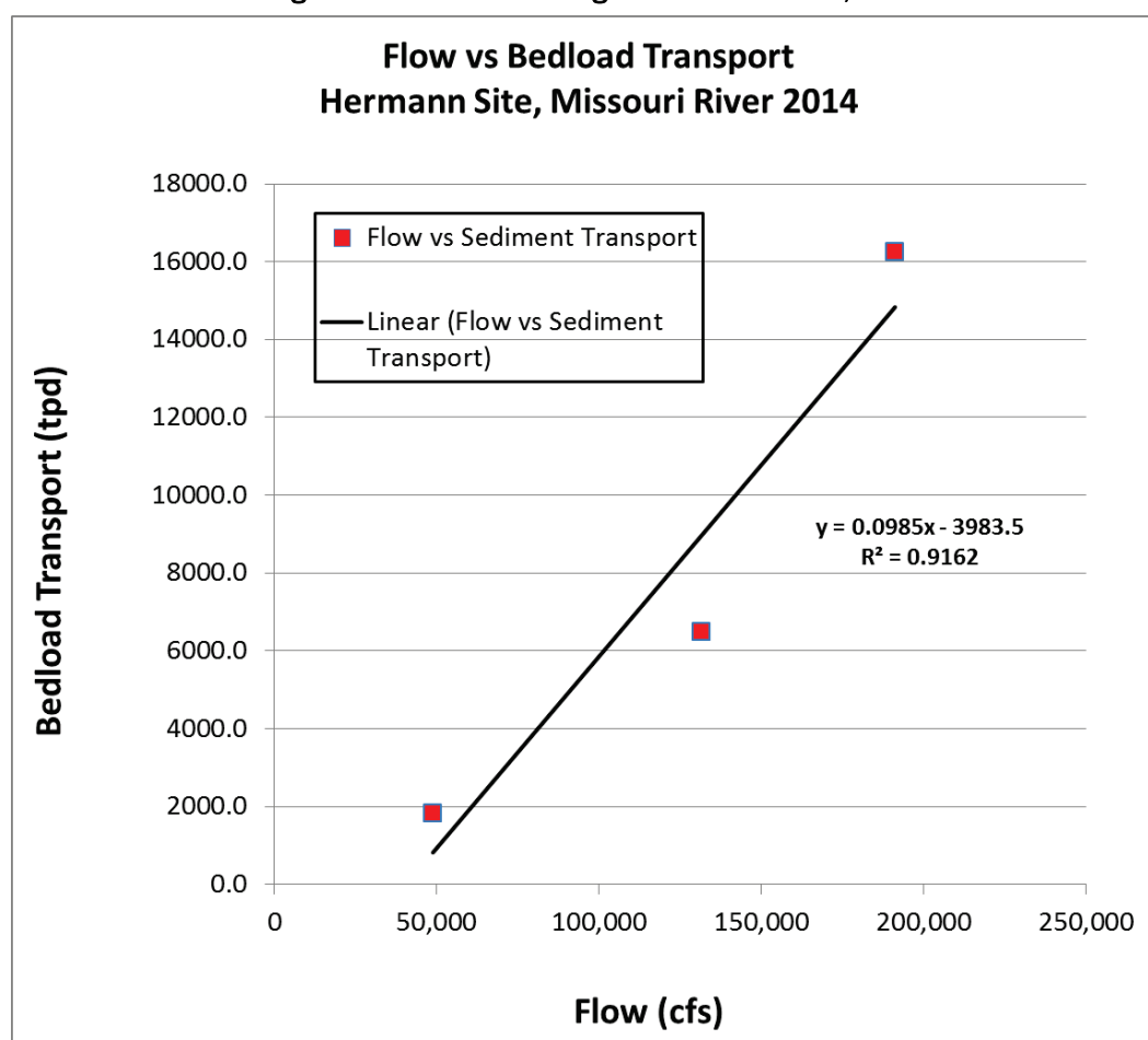
Figure 256. Bed-load rating curve for Hermann, MO.
