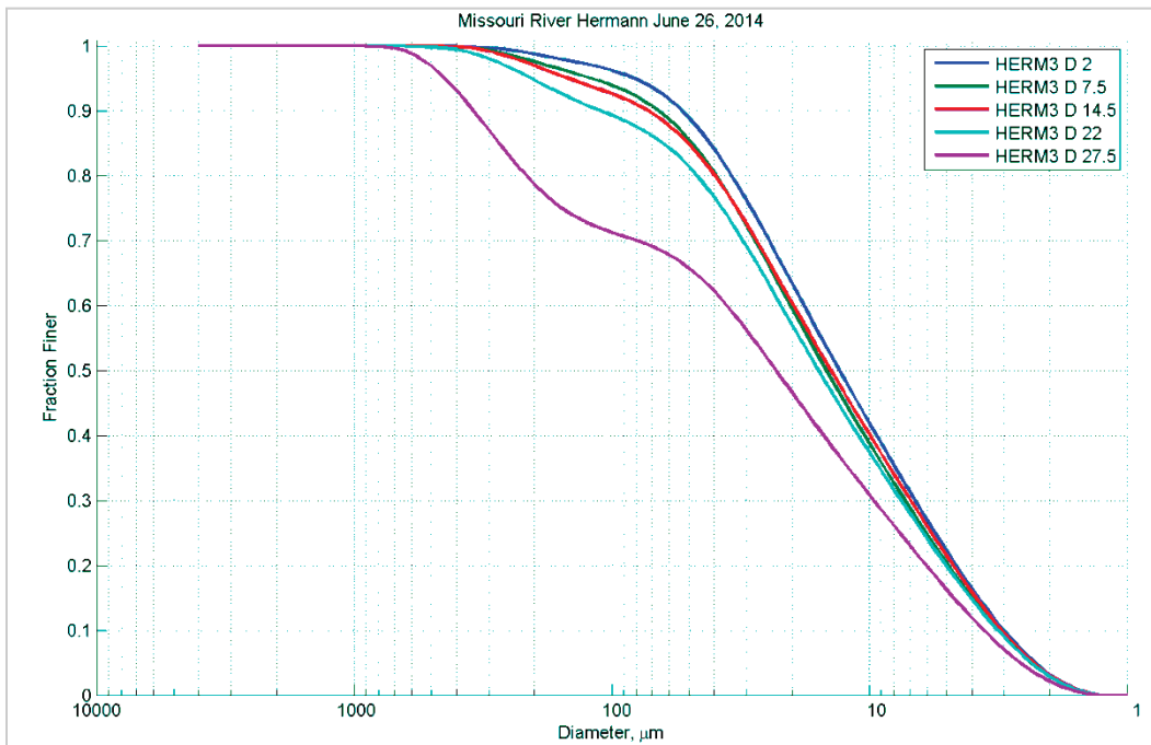
Figure 248. Particle size distribution at different depths (feet) in Station D – June 26, 2014.
