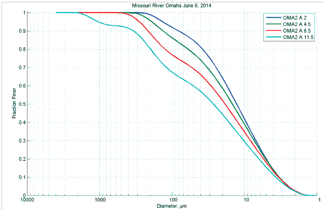
Figure 55. Particle size distribution at different depths (feet) in Station A – June 6, 2014.
