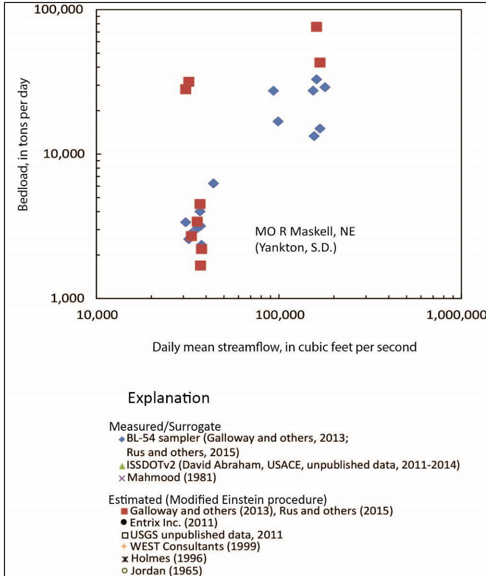
Figure 261. USGS bed-load data - Maskell, NE.
