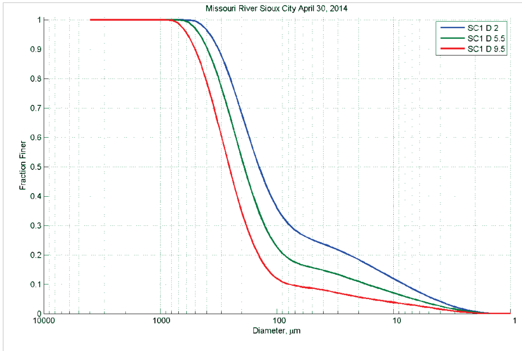
Figure 16. Particle size distribution at different depths (feet) in Station D – April 30, 2014.
