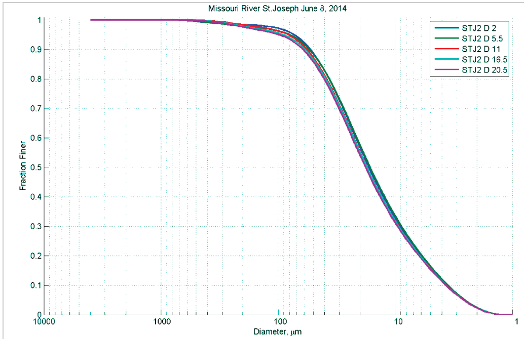
Figure 132. Particle size distribution at different depths (feet) in Station D – June 8, 2014.
