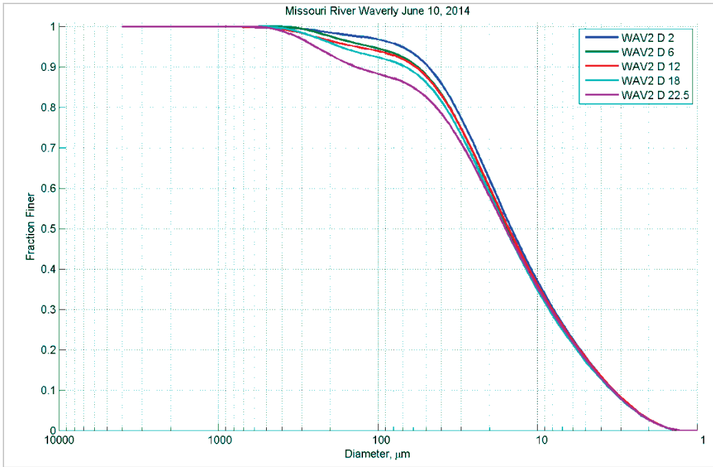
Figure 206. Particle size distribution at different depths (feet) in Station D – June 10, 2014.
