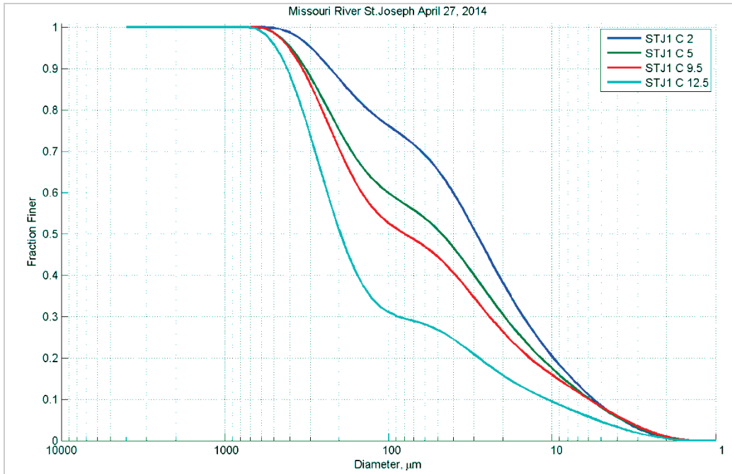
Figure 126. Particle size distribution at different depths (feet) in Station C - April 27, 2014.
