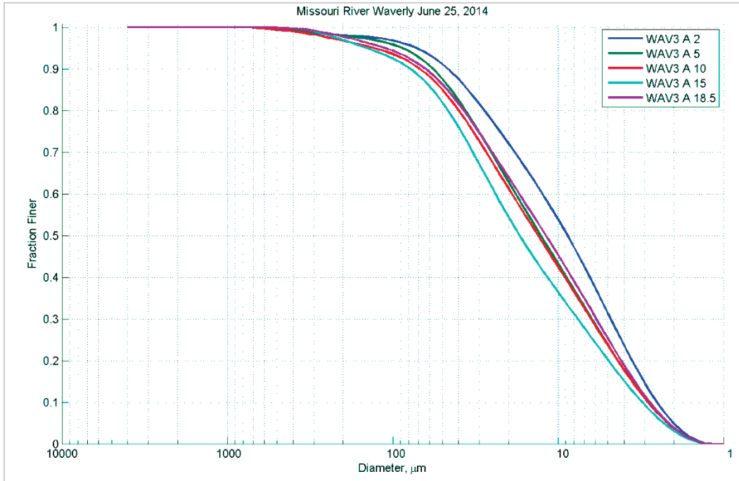
Figure 208. Particle size distribution at different depths (feet) in Station A – June 25, 2014.
