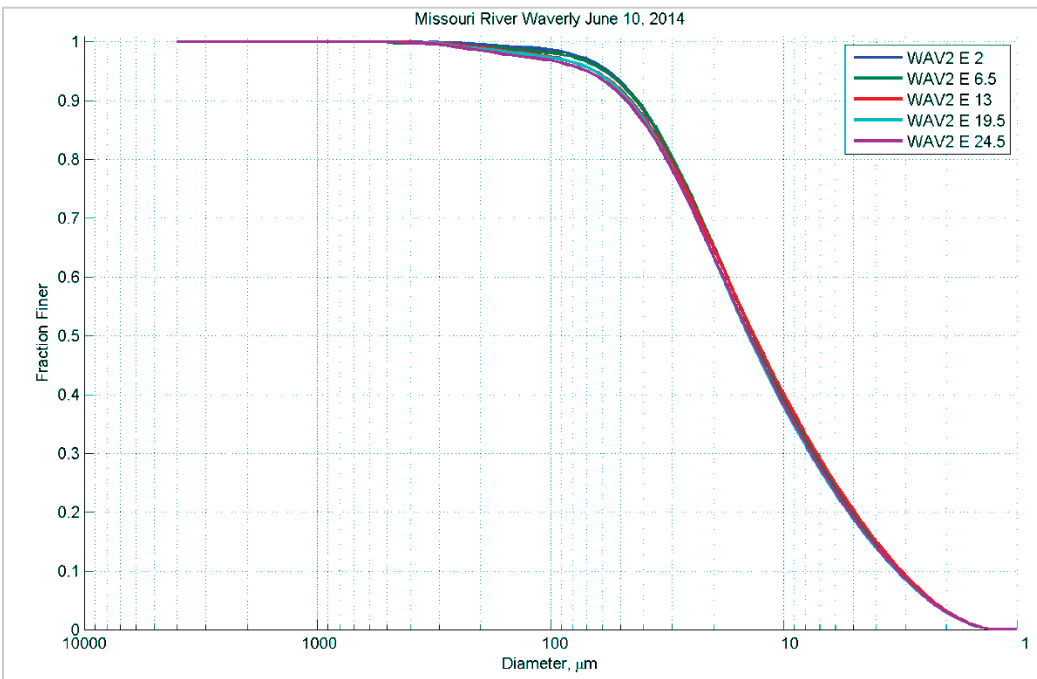
Figure 207. Particle size distribution at different depths (feet) in Station E – June 10, 2014.
