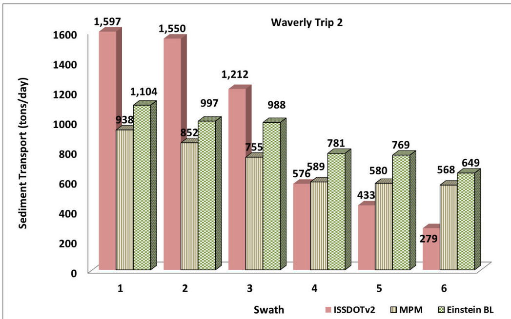
Figure 222. Bed-load transport at Waverly, MO – June 10, 2014: ISSDOTv2 values compared to transport function computed values.
