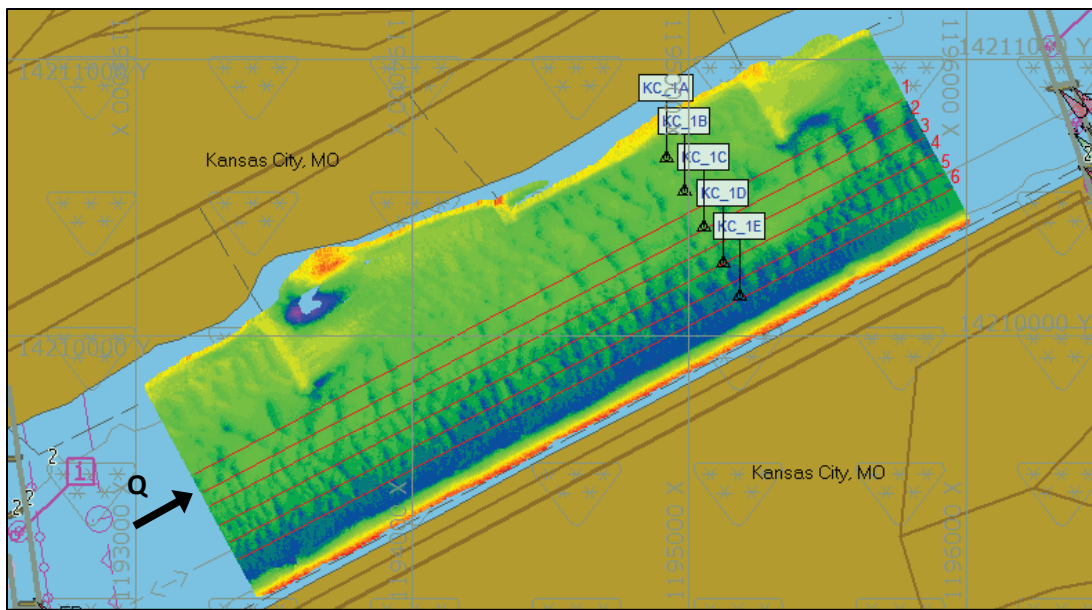
Figure 155. Multi-beam survey extent at Kansas City, MO – April 26, 2014.
