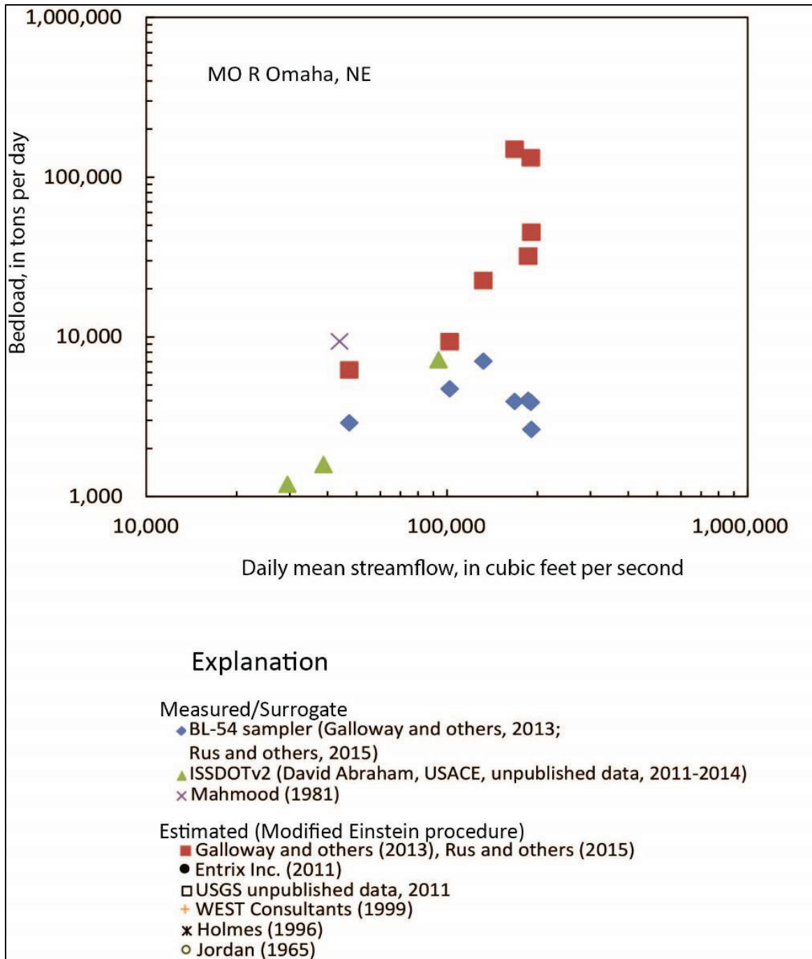
Figure 263. USGS bed-load data - Omaha, NE.
