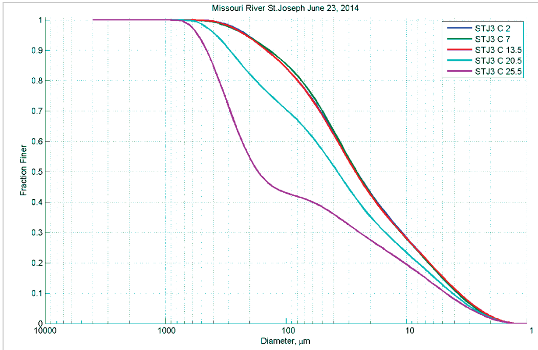
Figure 136. Particle size distribution at different depths (feet) in Station C – June 24, 2014.
