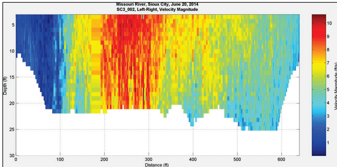
Figure 5. Velocity magnitude at Sioux City, IA – June 20, 2014, 16:11:59.
