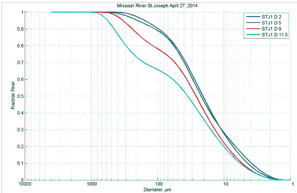
Figure 127. Particle size distribution at different depths (feet) in Station D - April 27, 2014.
