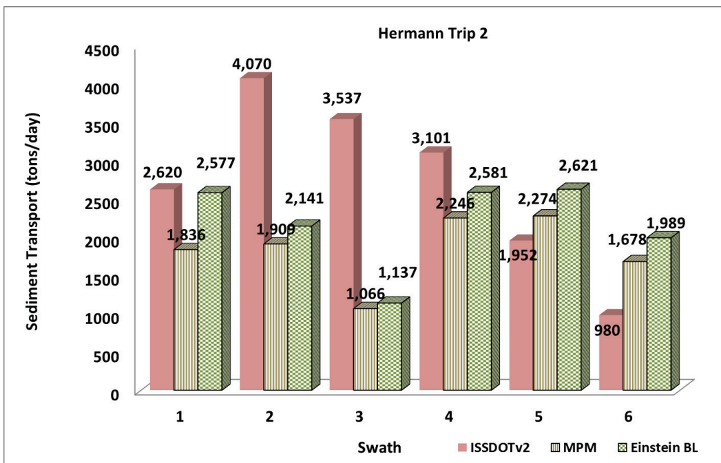
Figure 259. Bed-load transport at Hermann, MO– June 11, 2014: ISSDOTv2 values compared to transport function computed values.
