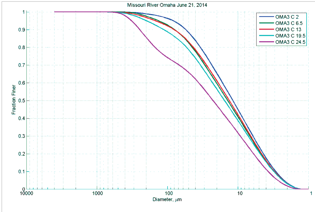
Figure 62. Particle size distribution at different depths (feet) in Station C – June 21, 2014.
