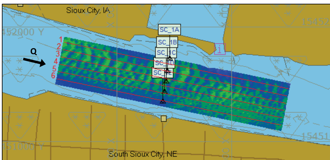
Figure 8. Multi-beam survey extent at Sioux City, IA – June 5 and June 20, 2014.
