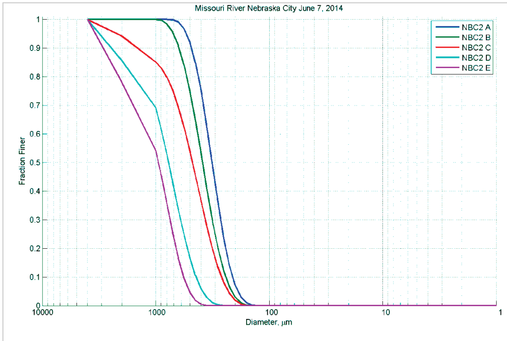
Figure 85. Bed material grain size distribution for Nebraska City, NE – June 7, 2014.
