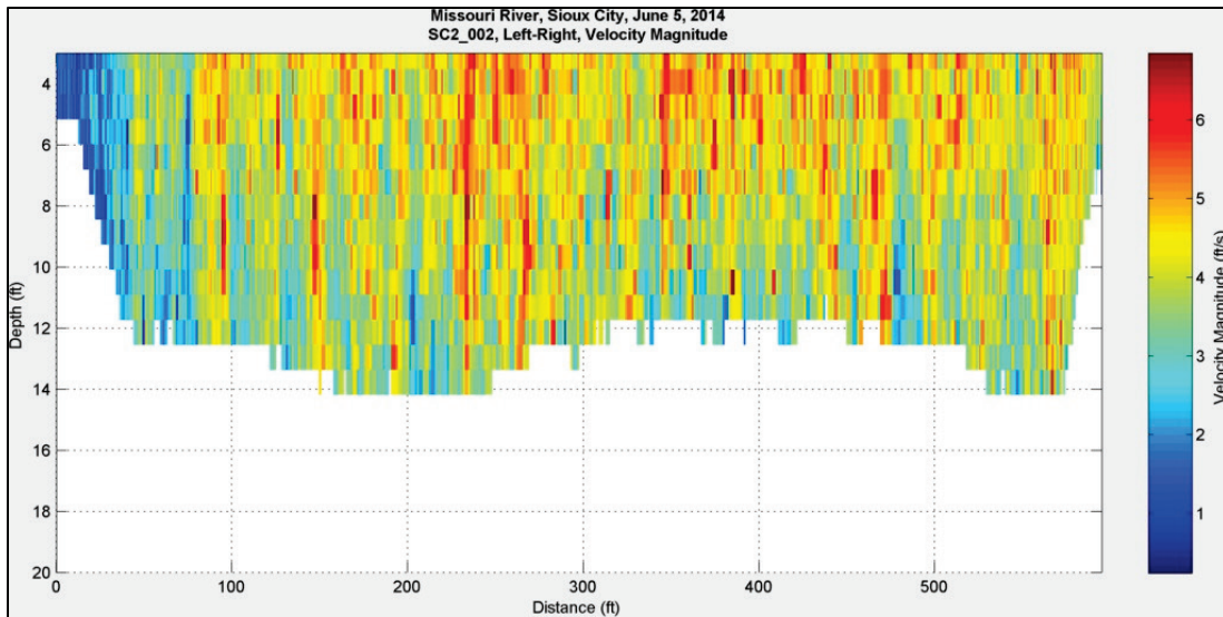
Figure 4. Velocity magnitude at Sioux City, IA – June 5, 2014, 15:51:45.
