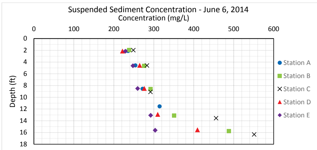
Figure 66. Suspended sediment concentration at Omaha, NE – June 6, 2014.
