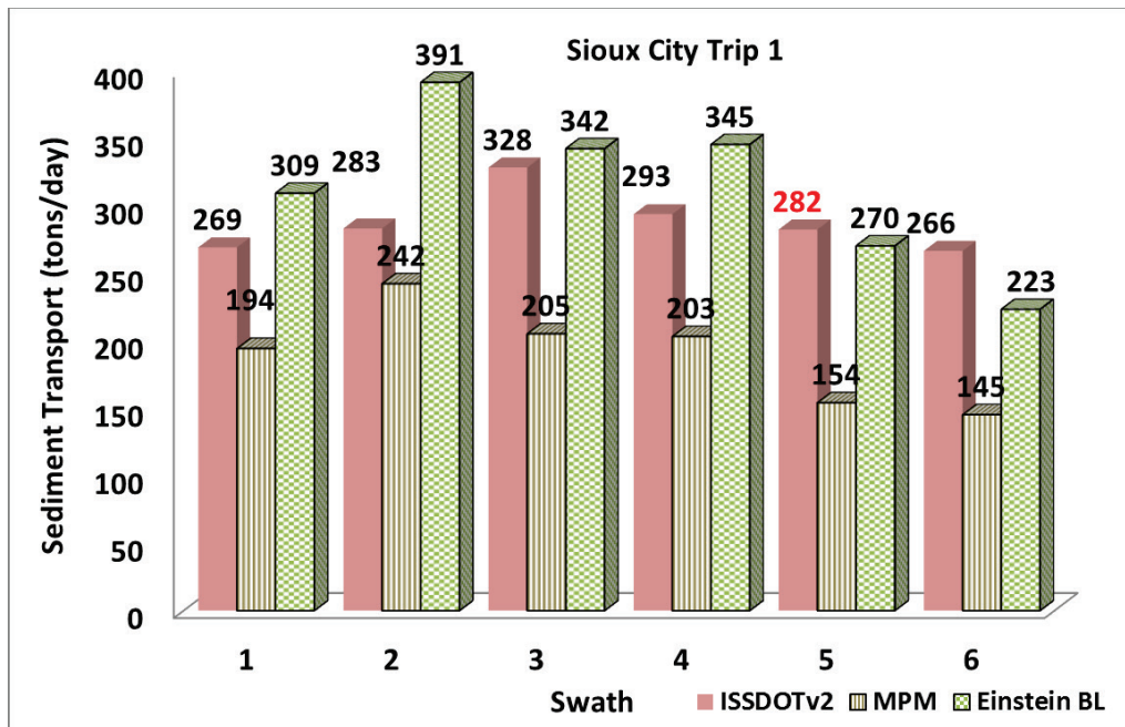
Figure 36. Bed-load transport at Sioux City, IA – April 30, 2014: ISSDOTv2 values compared to transport function computed values, where red indicates an interpolated value.
