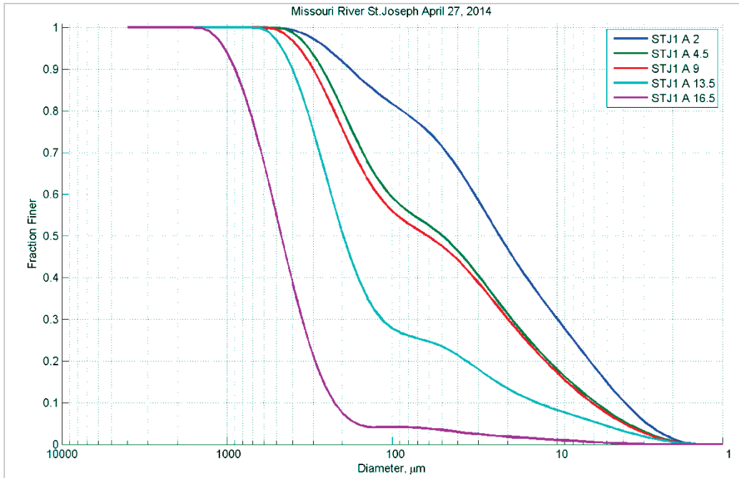
Figure 124. Particle size distribution at different depths (feet) in Station A - April 27, 2014.
