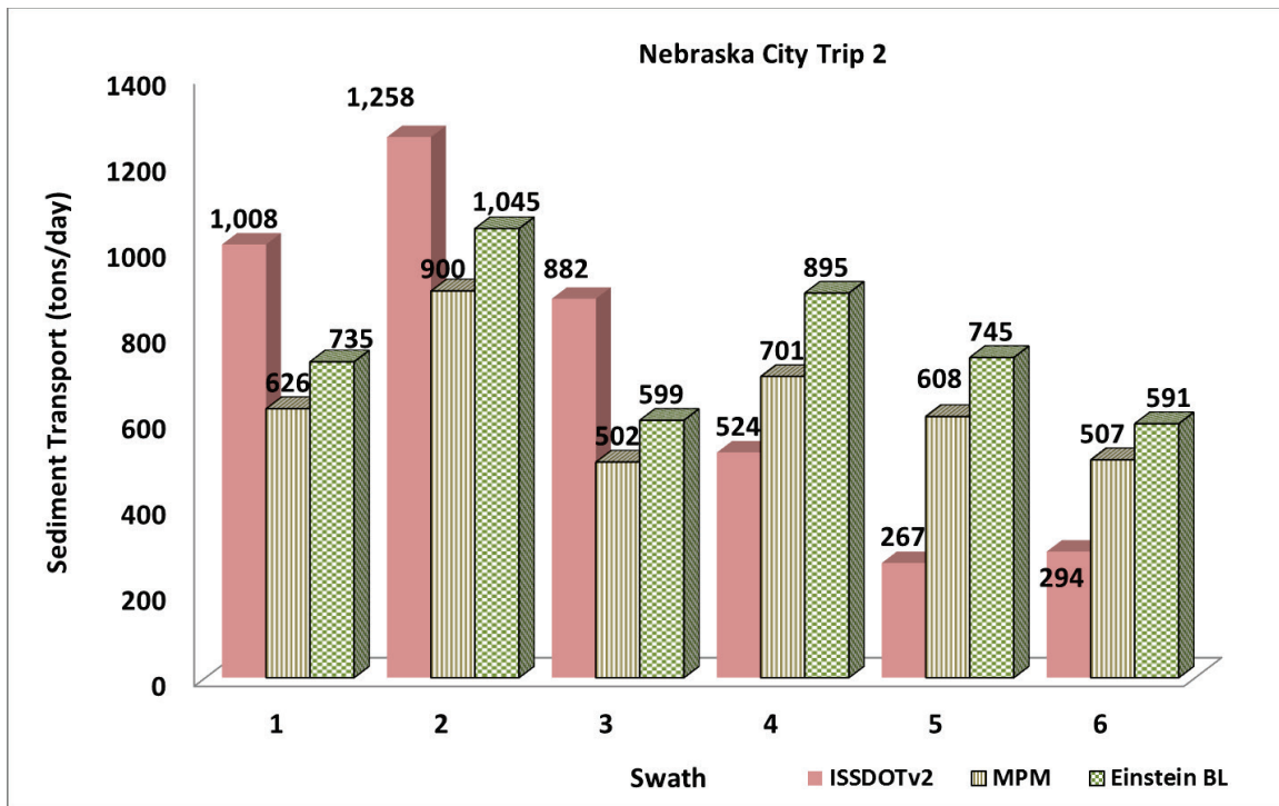
Figure 111. Bed-load transport at Nebraska City, NE- June 7, 2014: ISSDOTv2 values compared to transport function computed values.
