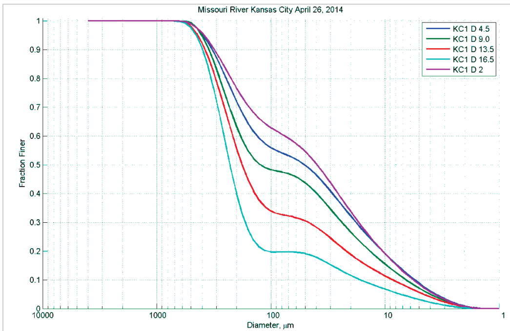
Figure 164. Particle size distribution at different depths (feet) in Station D - April 26, 2014.
