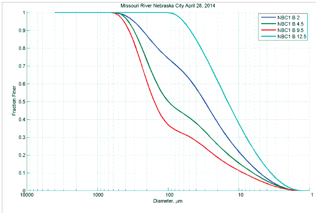
Figure 88. Particle size distribution at different depths (feet) in Station B - April 28, 2014.
