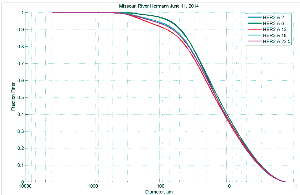
Figure 240. Particle size distribution at different depths (feet) in Station A - June 11, 2014.
