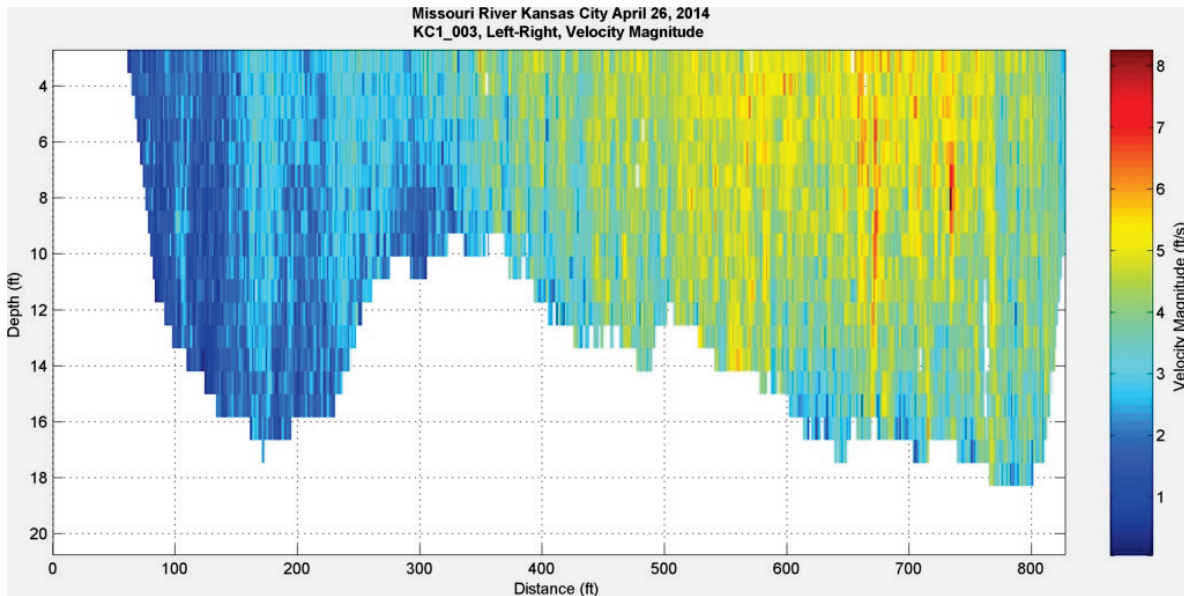
Figure 151. Velocity magnitude at Kansas City, MO – April 26, 2014, 17:19:53.
