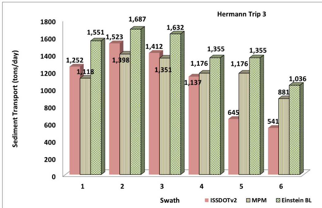
Figure 260. Bed-load transport at Hermann, MO – June 26, 2014: ISSDOTv2 values compared to transport function computed values.
