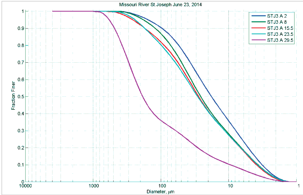
Figure 134. Particle size distribution at different depths (feet) in Station A – June 24, 2014.
