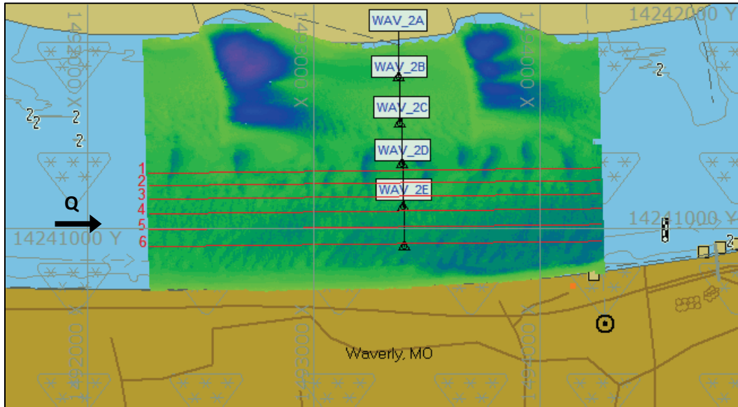
Figure 192. Multi-beam survey extent at Waverly, MO – April 25, 2014.
