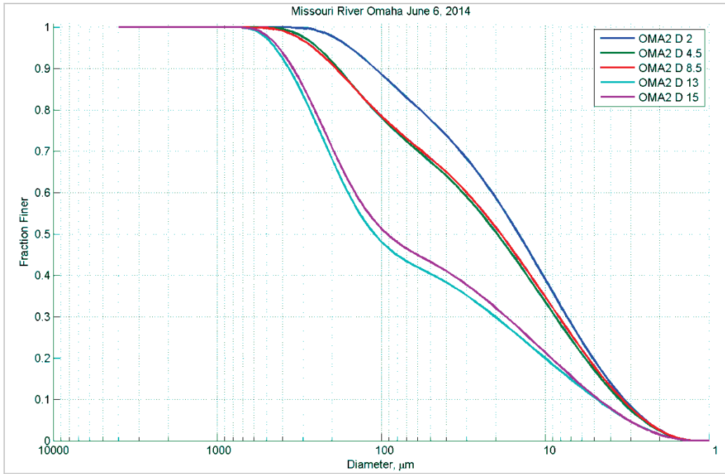
Figure 58. Particle size distribution at different depths (feet) in Station D – June 6, 2014.
