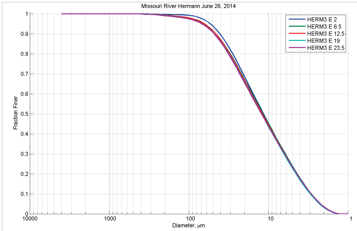
Figure 249. Particle size distribution at different depths (feet) in Station E – June 26, 2014.
