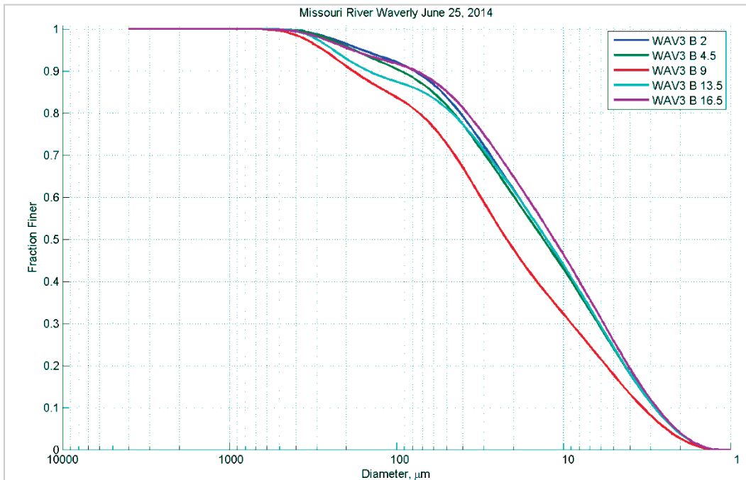
Figure 209. Particle size distribution at different depths (feet) in Station B – June 25, 2014.
