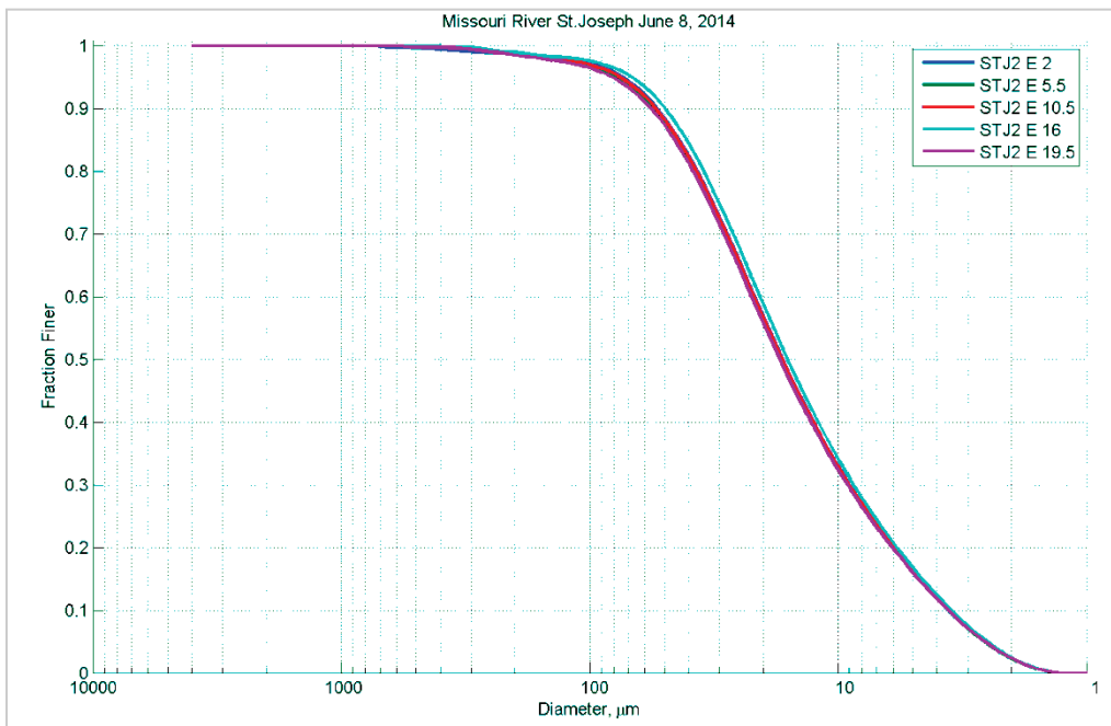
Figure 133. Particle size distribution at different depths (feet) in Station E – June 8, 2014.
