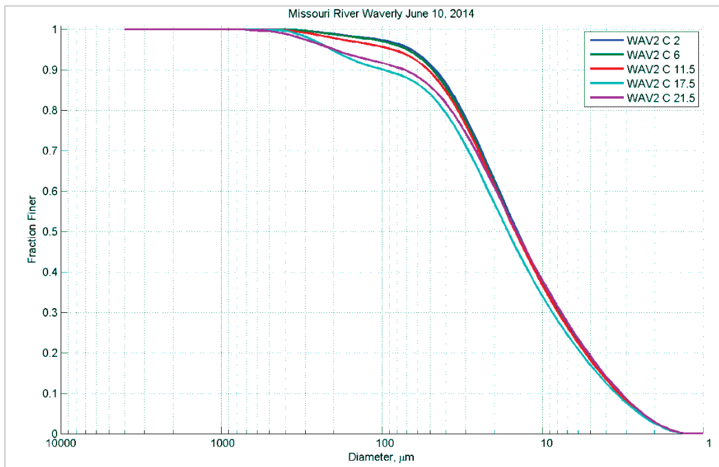
Figure 205. Particle size distribution at different depths (feet) in Station C – June 10, 2014.
