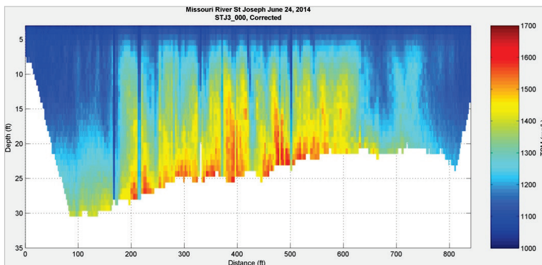
Figure 144. Suspended sediment concentration profile at St. Joseph, MO – June 24, 2014.
