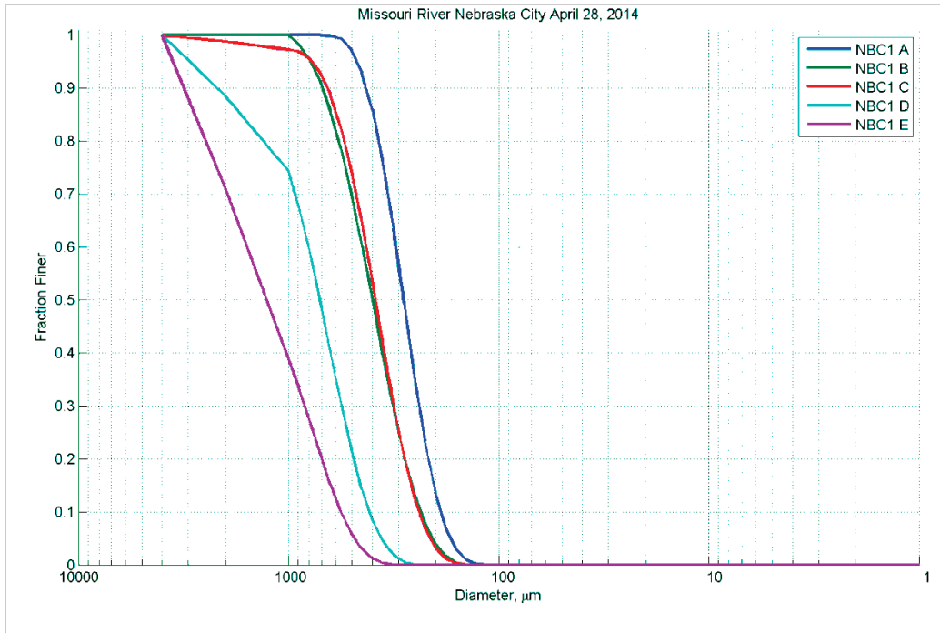
Figure 84. Bed material grain size distribution for Nebraska City, NE – April 28, 2014.
