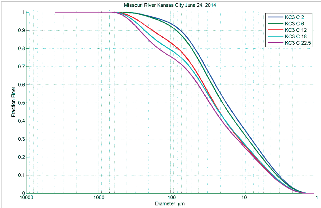
Figure 173. Particle size distribution at different depths (feet) in Station C – June 24, 2014.
