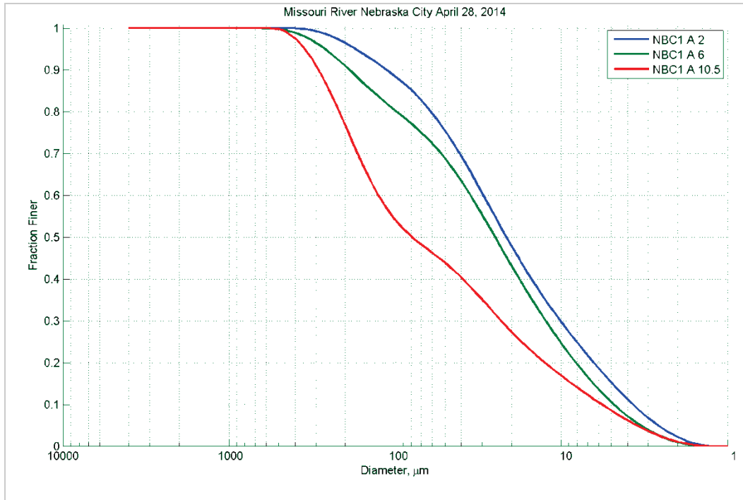
Figure 87. Particle size distribution at different depths (feet) in Station A - April 28, 2014.
