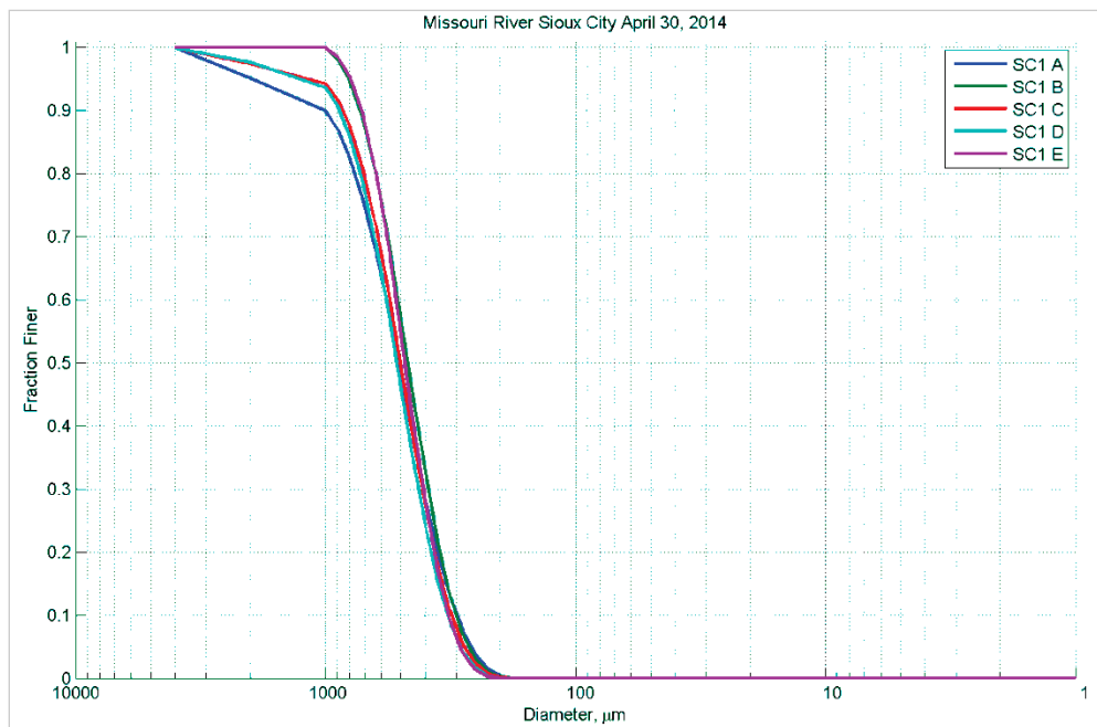
Figure 10. Bed material grain size distribution for Sioux City, IA – April 30, 2014.
