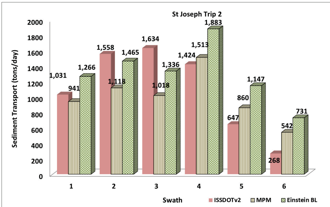
Figure 148. Bed-load transport at St. Joseph, MO – June 8, 2014: ISSDOTv2 values compared to transport function computed values.
