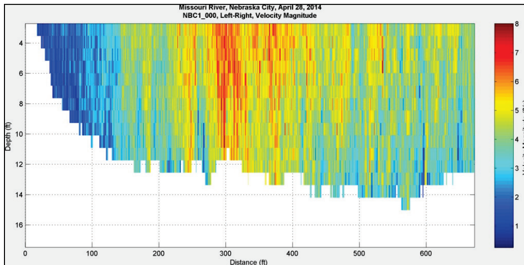
Figure 77. Velocity Magnitude at Nebraska City, NE – April 28, 2014. 15:41:04.
