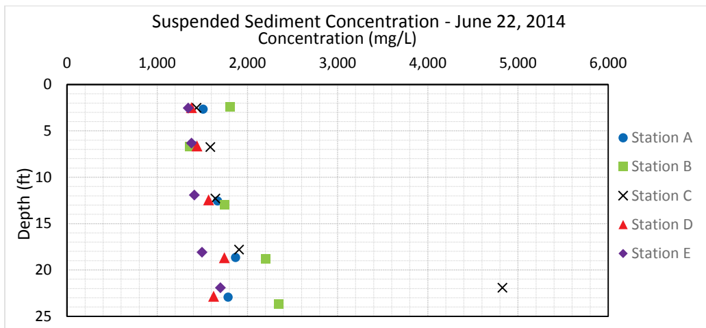
Figure 104. Suspended sediment concentration at Nebraska City, NE – June 22, 2014.
