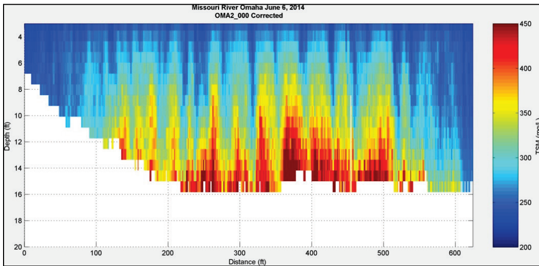
Figure 69. Suspended sediment concentration Profile at Omaha, NE - June 6, 2014.
