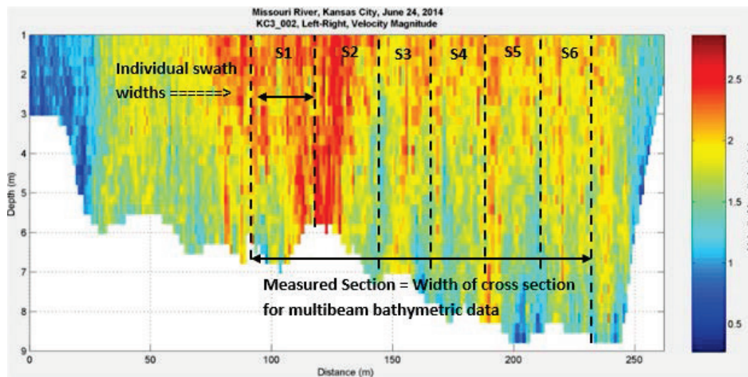
Figure 268. Cross section of measured velocities, Kansas City, trip 3.
