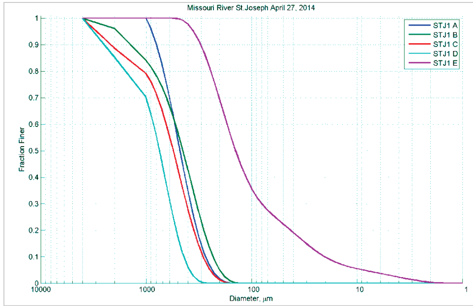
Figure 121. Bed material grain size distribution for St. Joseph, MO – April 27, 2014.
