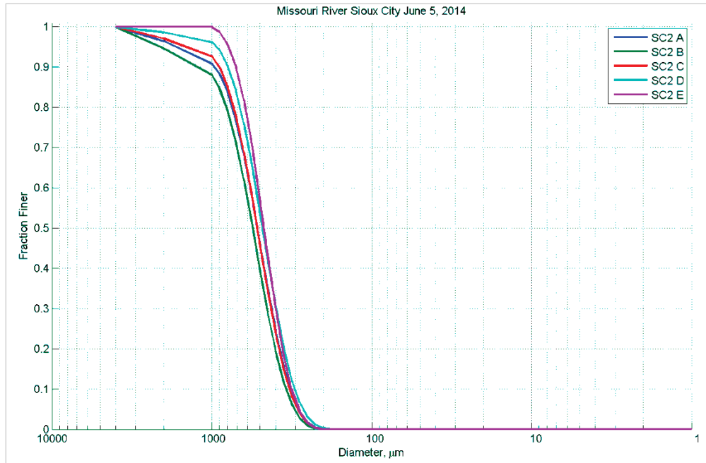
Figure 11. Bed material grain size distribution for Sioux City, IA – June 5, 2014.
