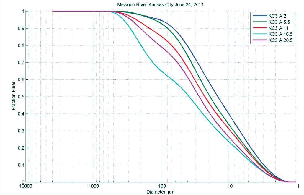
Figure 171. Particle size distribution at different depths (feet) in Station A – June 24, 2014.
