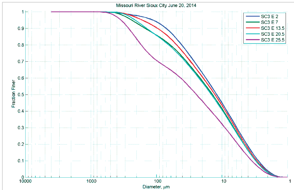
Figure 27. Particle size distribution at different depths (feet) in Station E – June 20, 2014.
