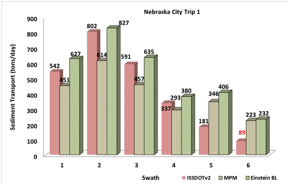
Figure 110. Bed-load transport at Nebraska City, NE- April 28, 2014: ISSDOTv2 values compared to transport function computed values, where red indicates an interpolated value.
