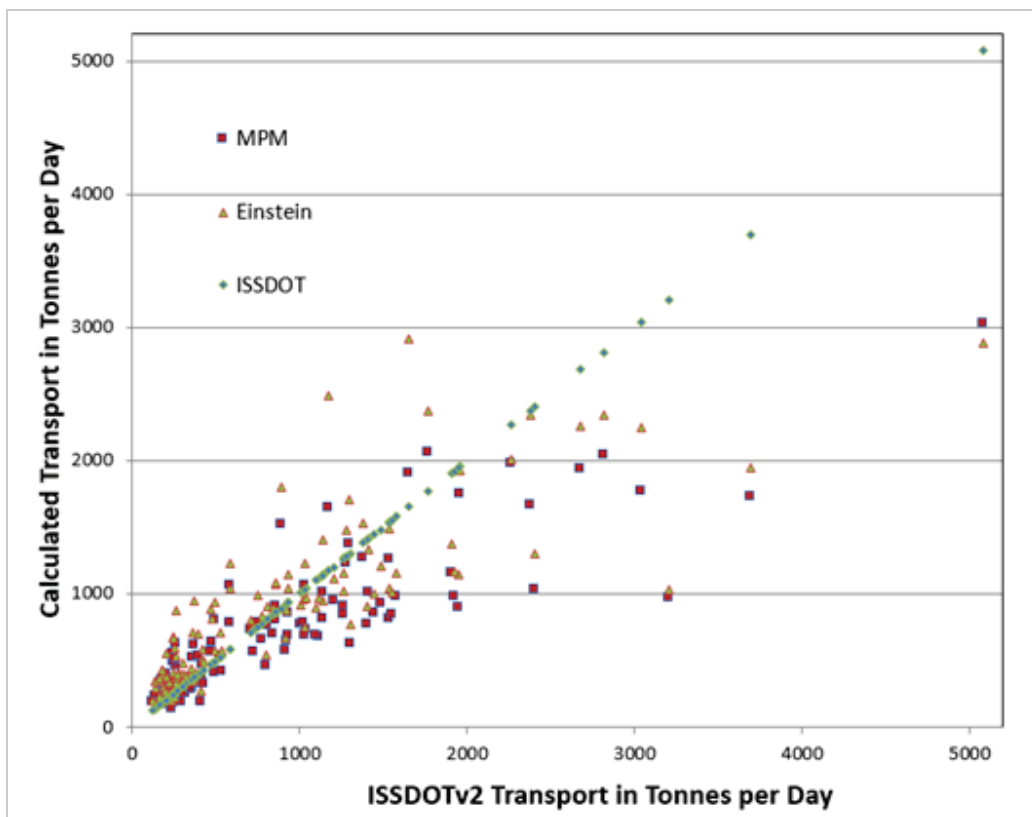
Figure 270. MPM and Einstein transport rates compared to ISSDOTv2 measurements at the sub-cross-section scale.
