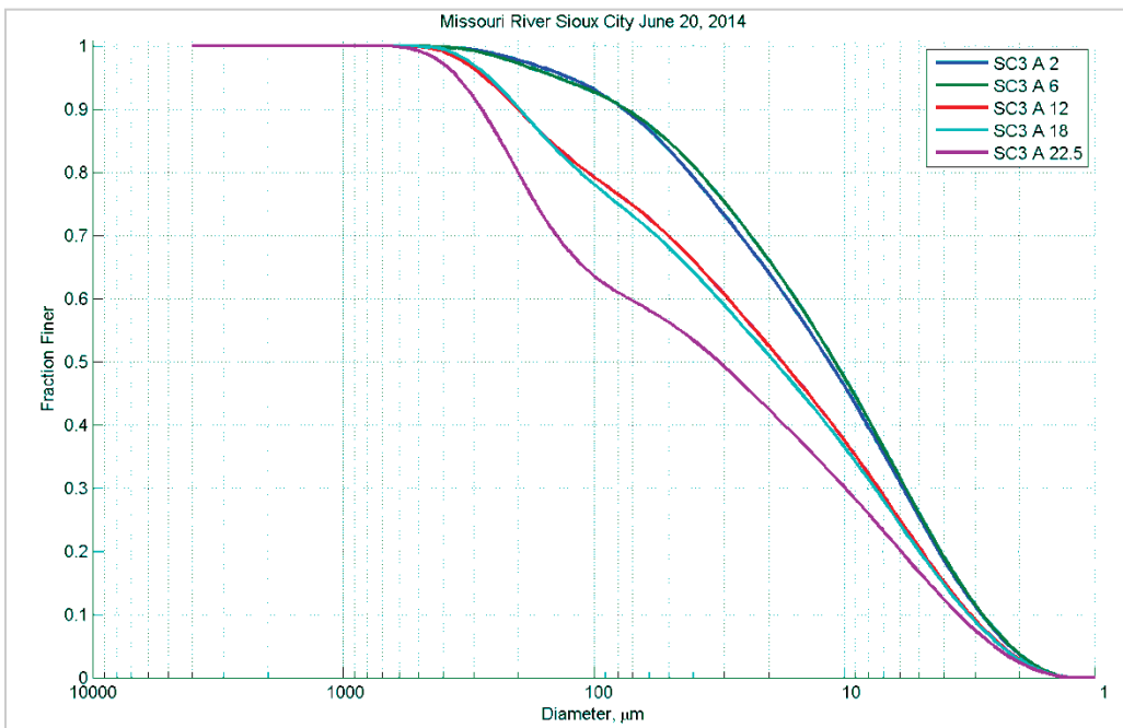
Figure 23. Particle size distribution at different depths (feet) in Station A – June 20, 2014.
