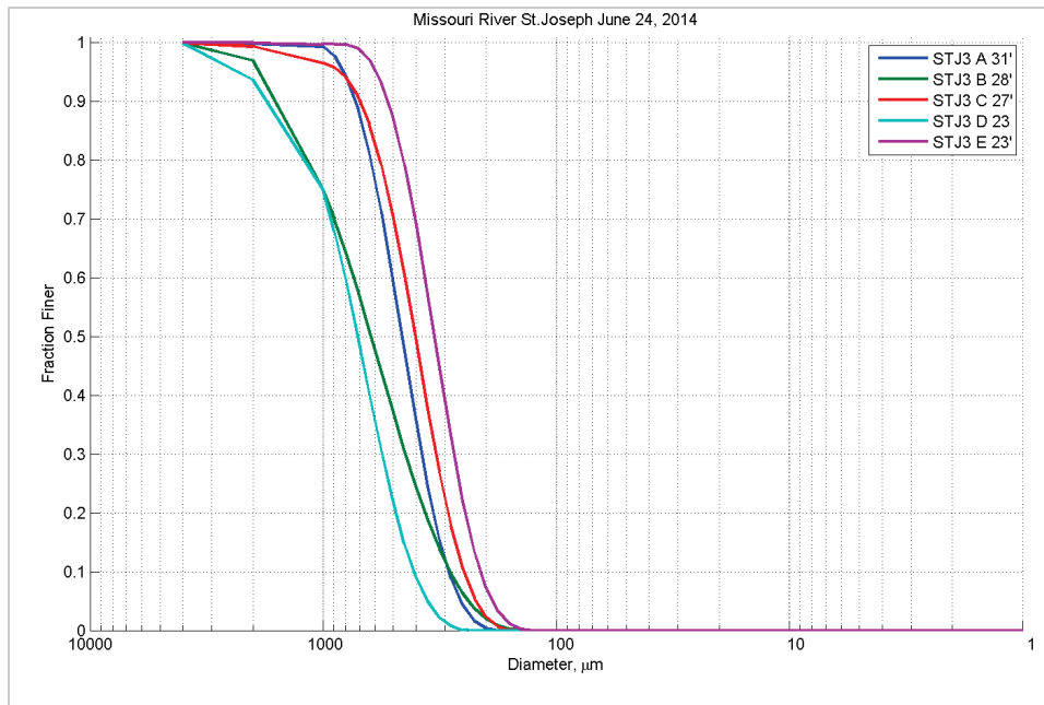
Figure 123. Bed material grain size distribution for St. Joseph, MO – June 24, 2014.
