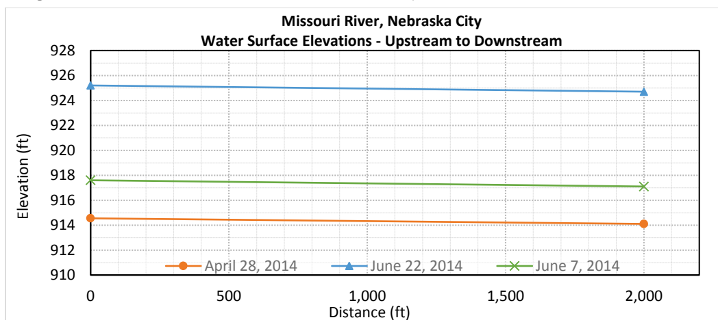
Figure 80. Water surface elevation at Nebraska City, NE – From upstream to downstream.
