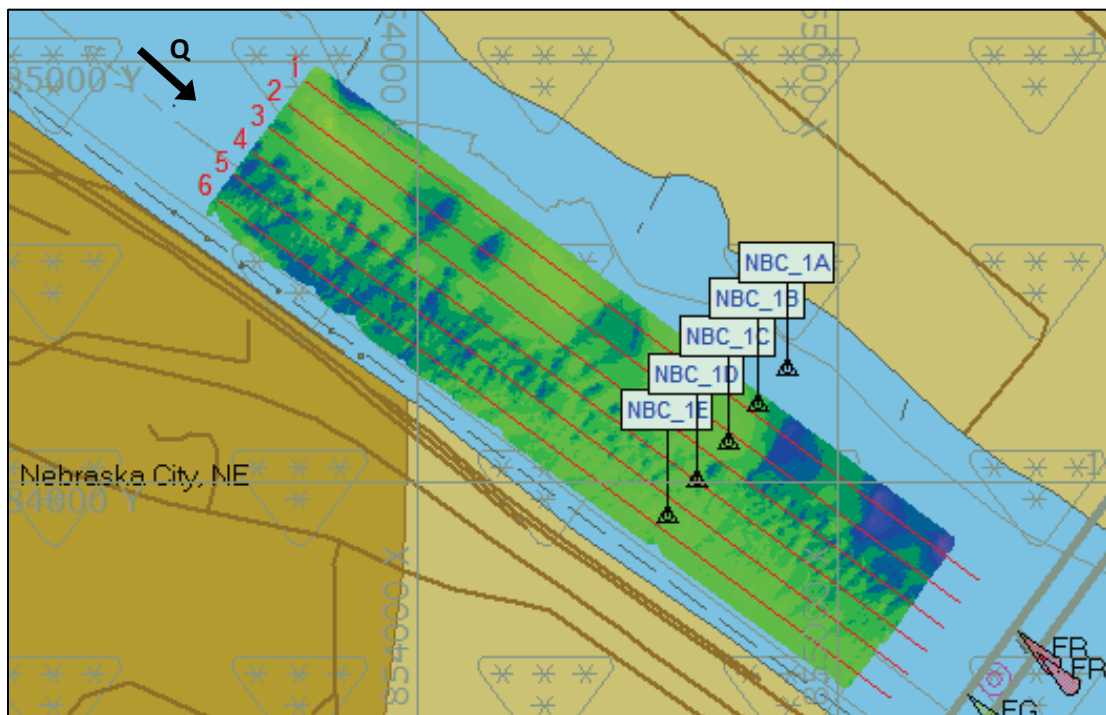
Figure 82. Multi-beam survey extent at Nebraska City, NE - June 7 and June 22, 2014.
