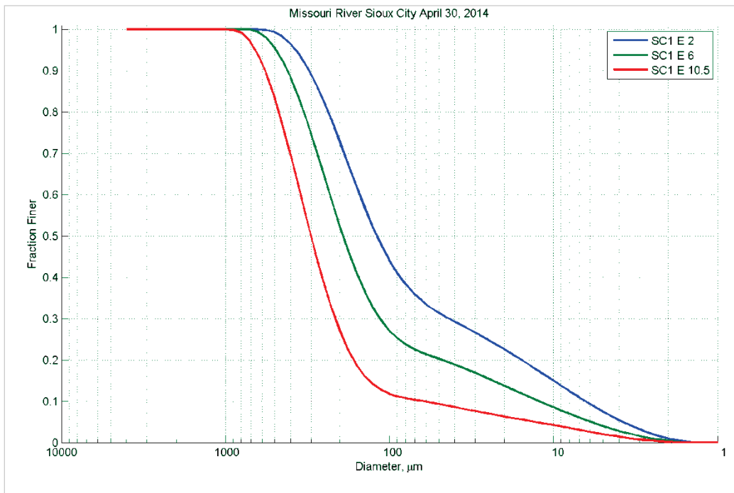
Figure 17. Particle size distribution at different depths (feet) in Station E – April 30, 2014.
