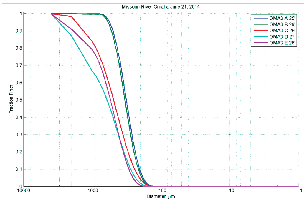
Figure 49. Bed material grain size distribution for Omaha, NE – June 21, 2014.
