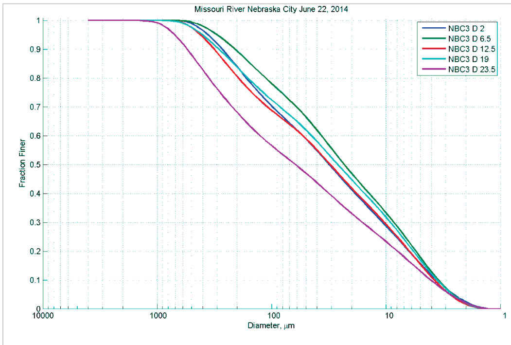
Figure 100. Particle size distribution at different depths (feet) in Station D – June 22, 2014.
