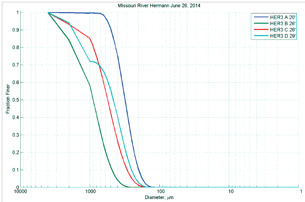
Figure 234. Bed material grain size distribution for Hermann, MO – June 26, 2014.
