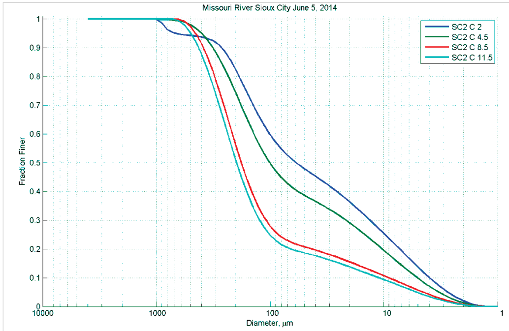
Figure 20. Particle size distribution at different depths (feet) in Station C – June 5, 2014.
