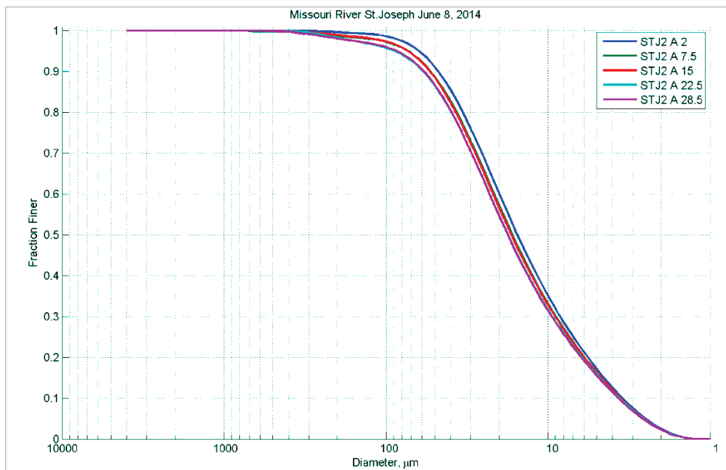
Figure 129. Particle size distribution at different depths (feet) in Station A - June 8, 2014.
