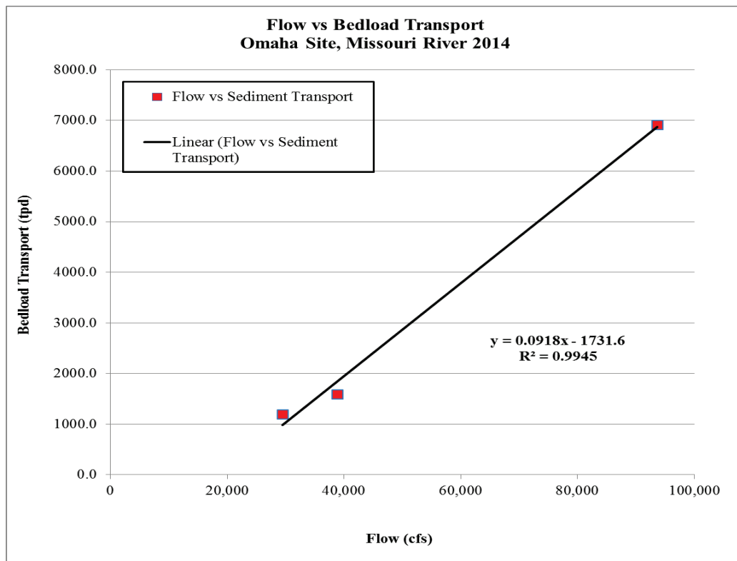
Figure 71. Bed-load rating curve Omaha, NE.
