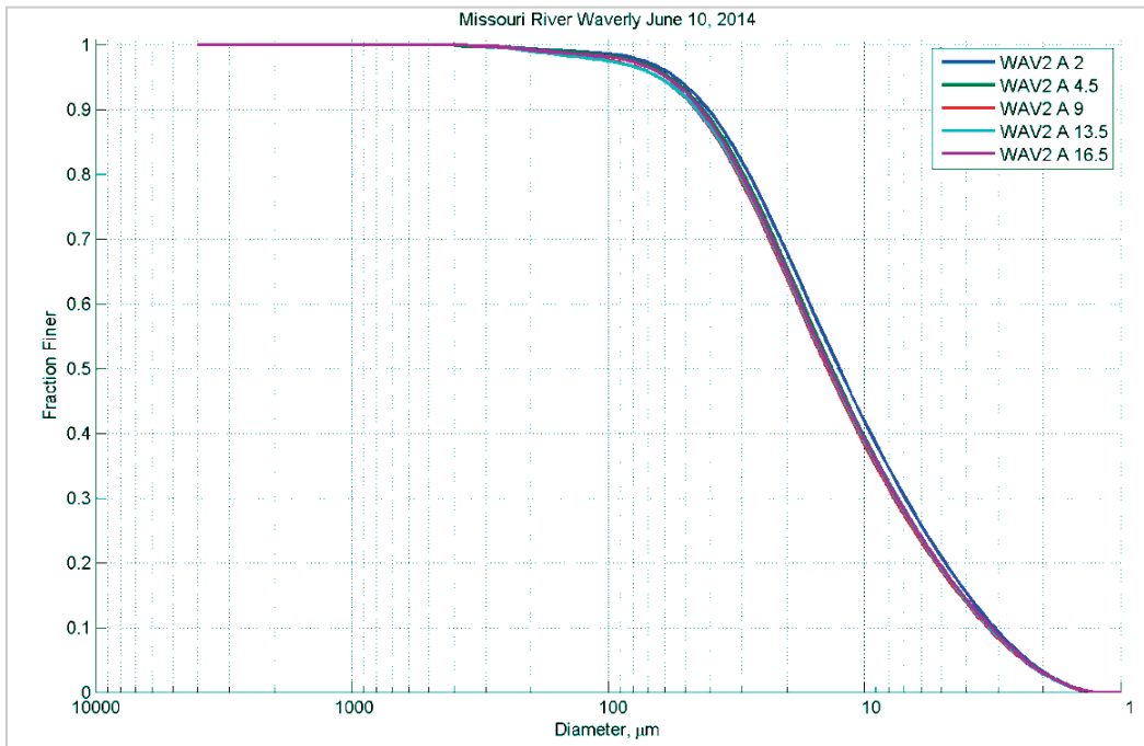
Figure 203. Particle size distribution at different depths (feet) in Station A - June 10, 2014.
