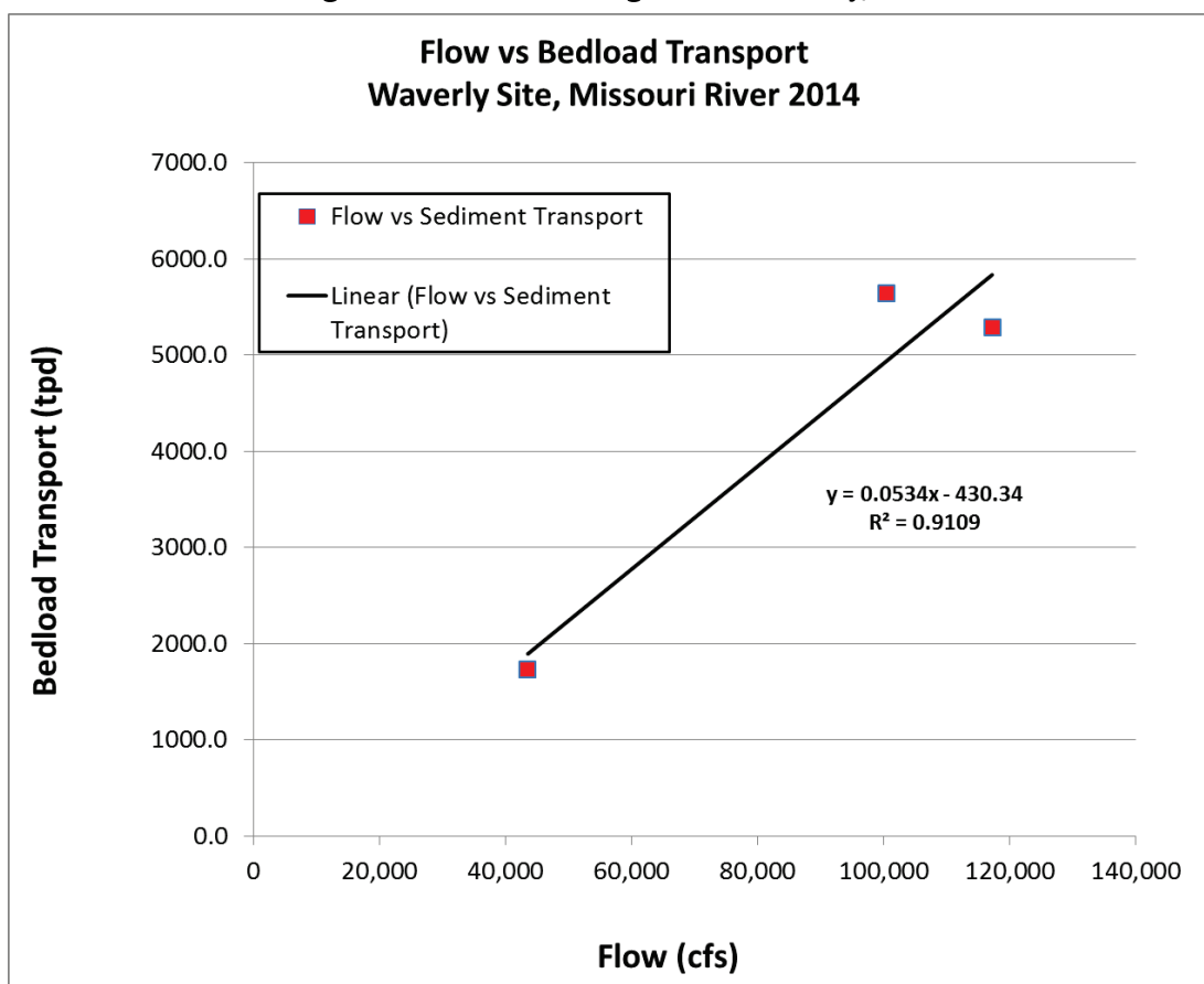
Figure 219. Bed-load rating curve for Waverly, MO.
