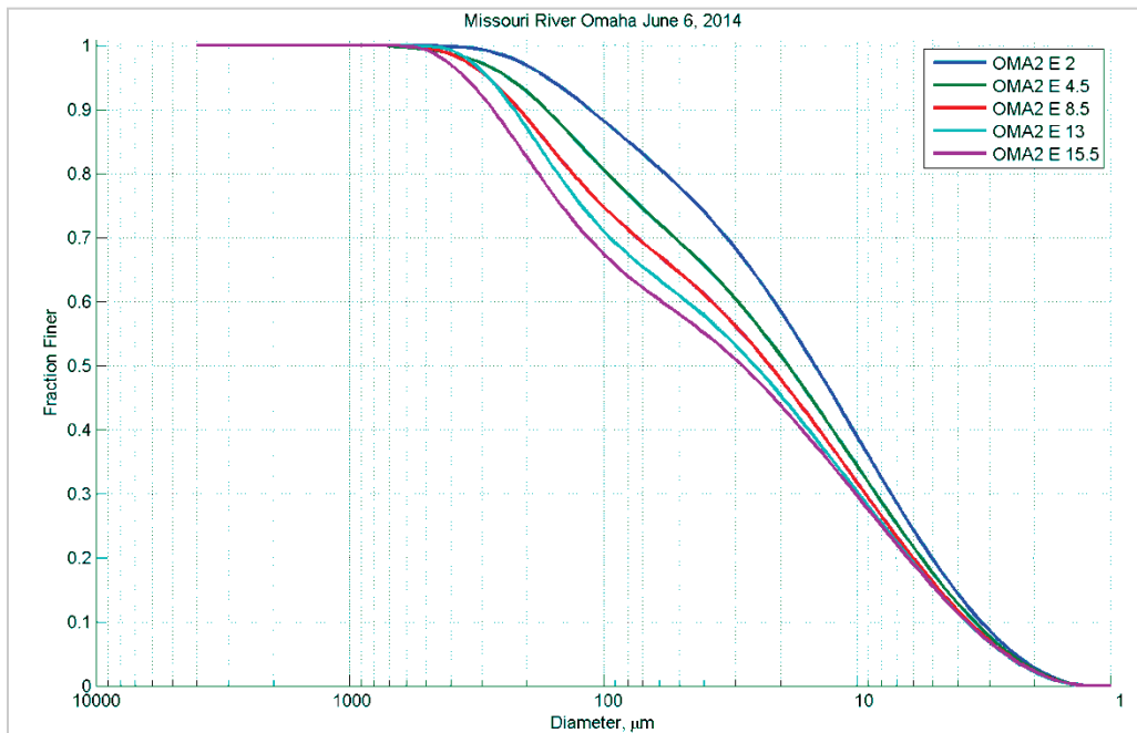
Figure 59. Particle size distribution at different depths (feet) in Station E – June 6, 2014.
