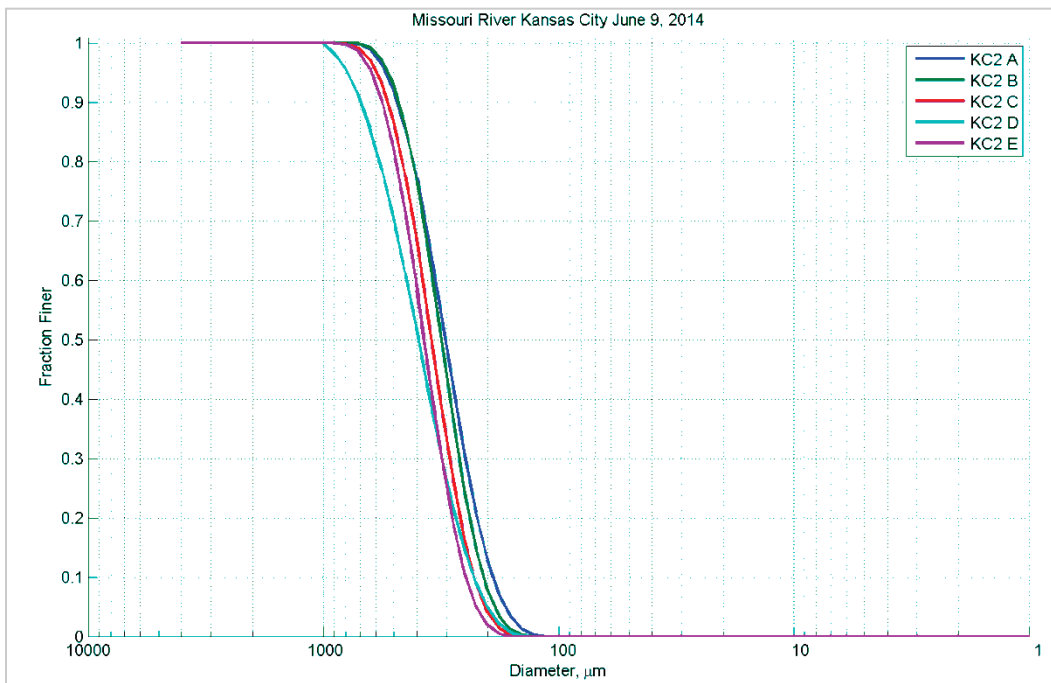
Figure 159. Bed material grain size distribution for Kansas City, MO – June 9, 2014.
