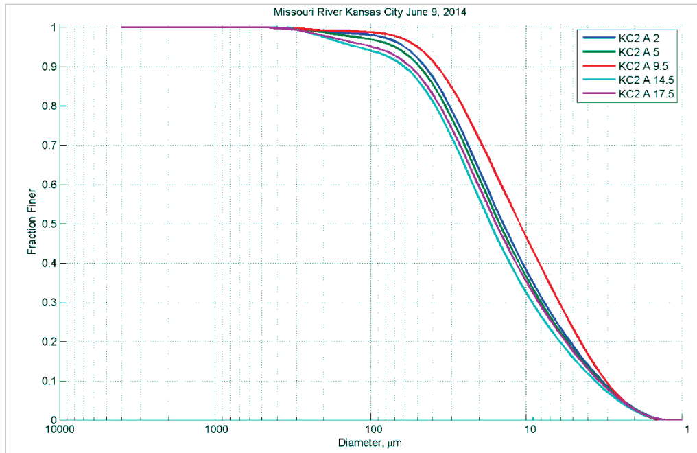
Figure 166. Particle size distribution at different depths (feet) in Station A - June 9, 2014.
