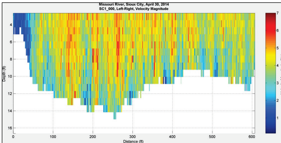
Figure 3. Velocity magnitude at Sioux City, IA – April 30, 2014, 15:15:00.
