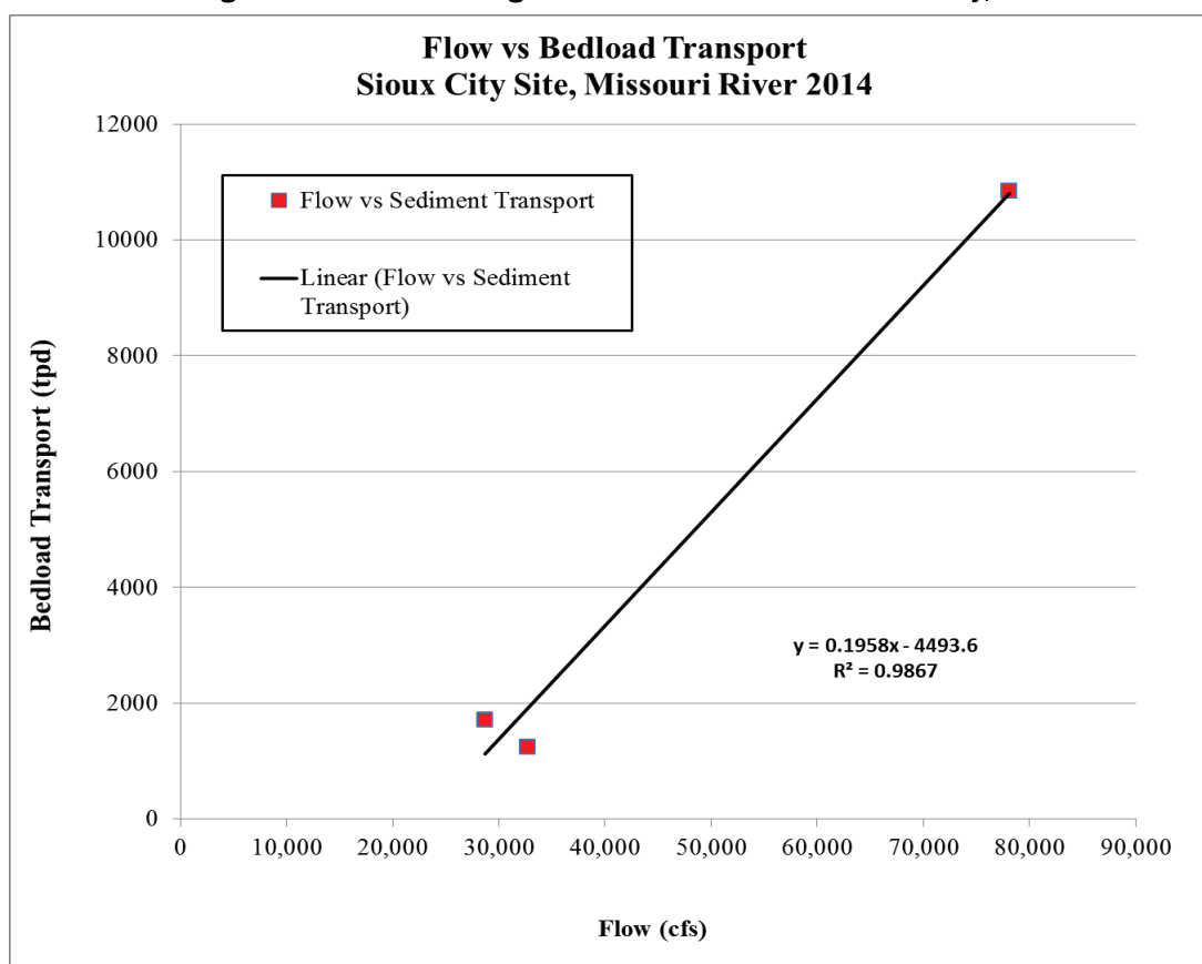
Figure 34. Bed-load rating curve for Missouri River at Sioux City, IA.
