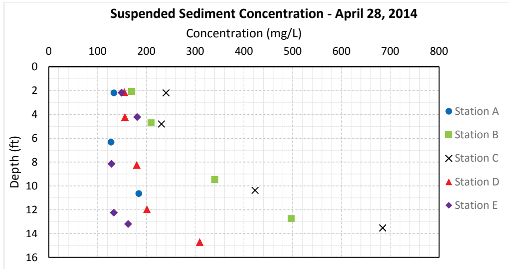
Figure 102. Suspended sediment concentration at Nebraska City, NE – April 28, 2014.
