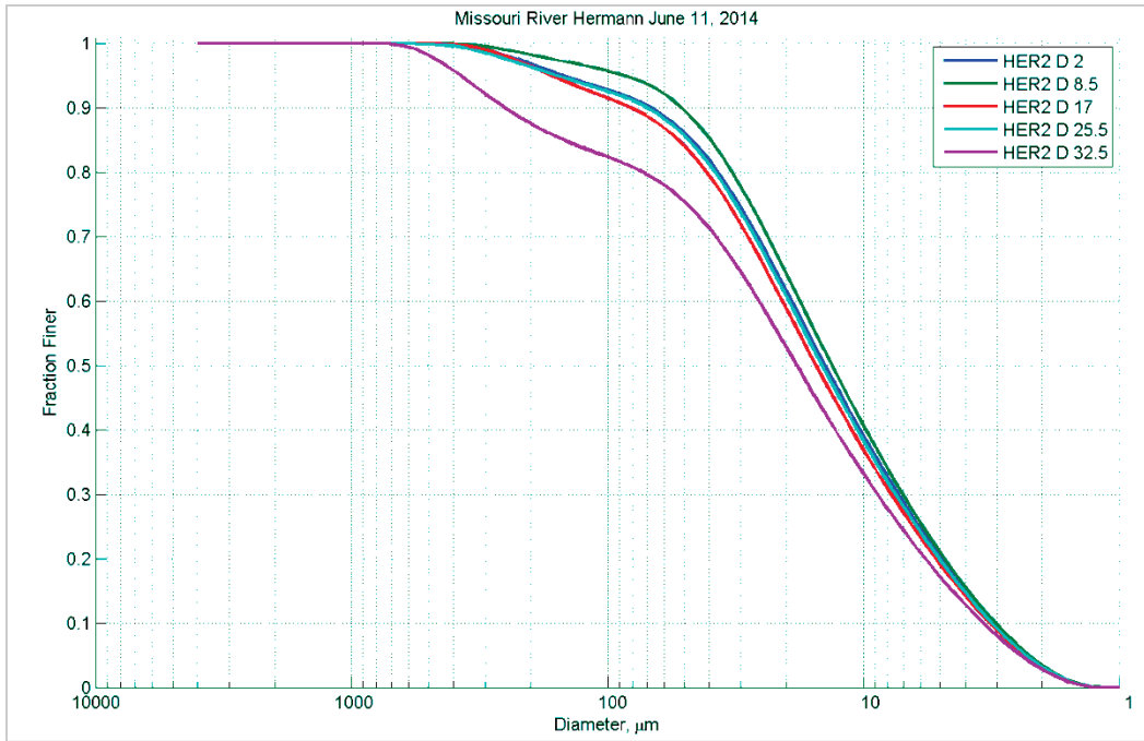
Figure 243. Particle size distribution at different depths (feet) in Station D – June 11, 2014.
