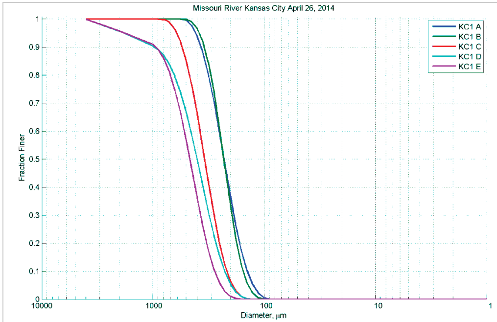
Figure 158. Bed material grain size distribution for Kansas City, MO – April 26, 2014.
