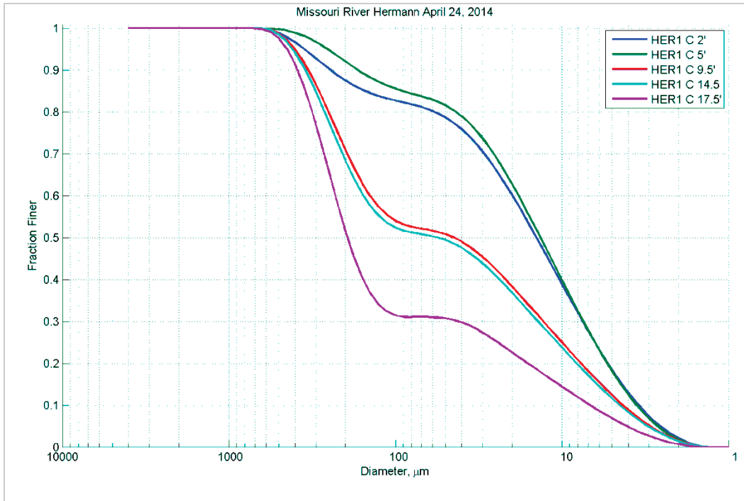
Figure 237. Particle size distribution at different depths (feet) in Station C - April 24, 2014.
