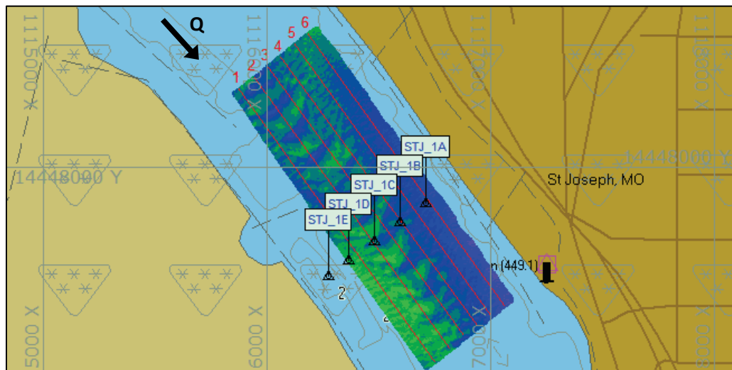
Figure 119. Multi-beam survey extent at St. Joseph, MO – June 8 and June 24, 2014.
