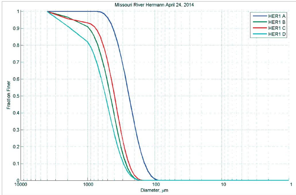
Figure 232. Bed material grain size distribution for Hermann, MO – April 24, 2014.
