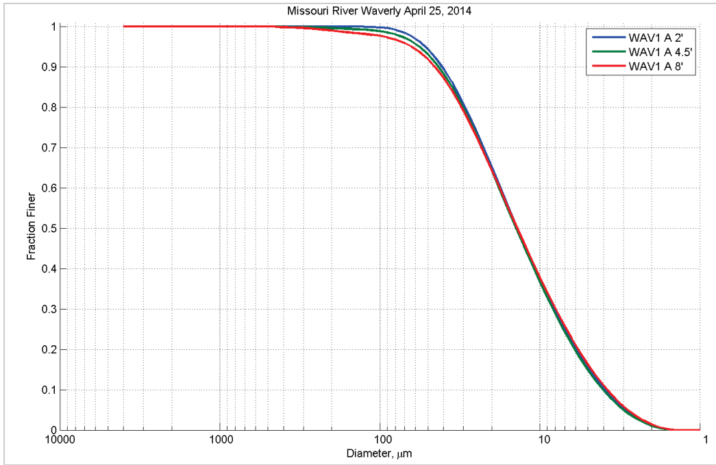
Figure 198. Particle Size Distribution at Station A - April 25, 2014.
