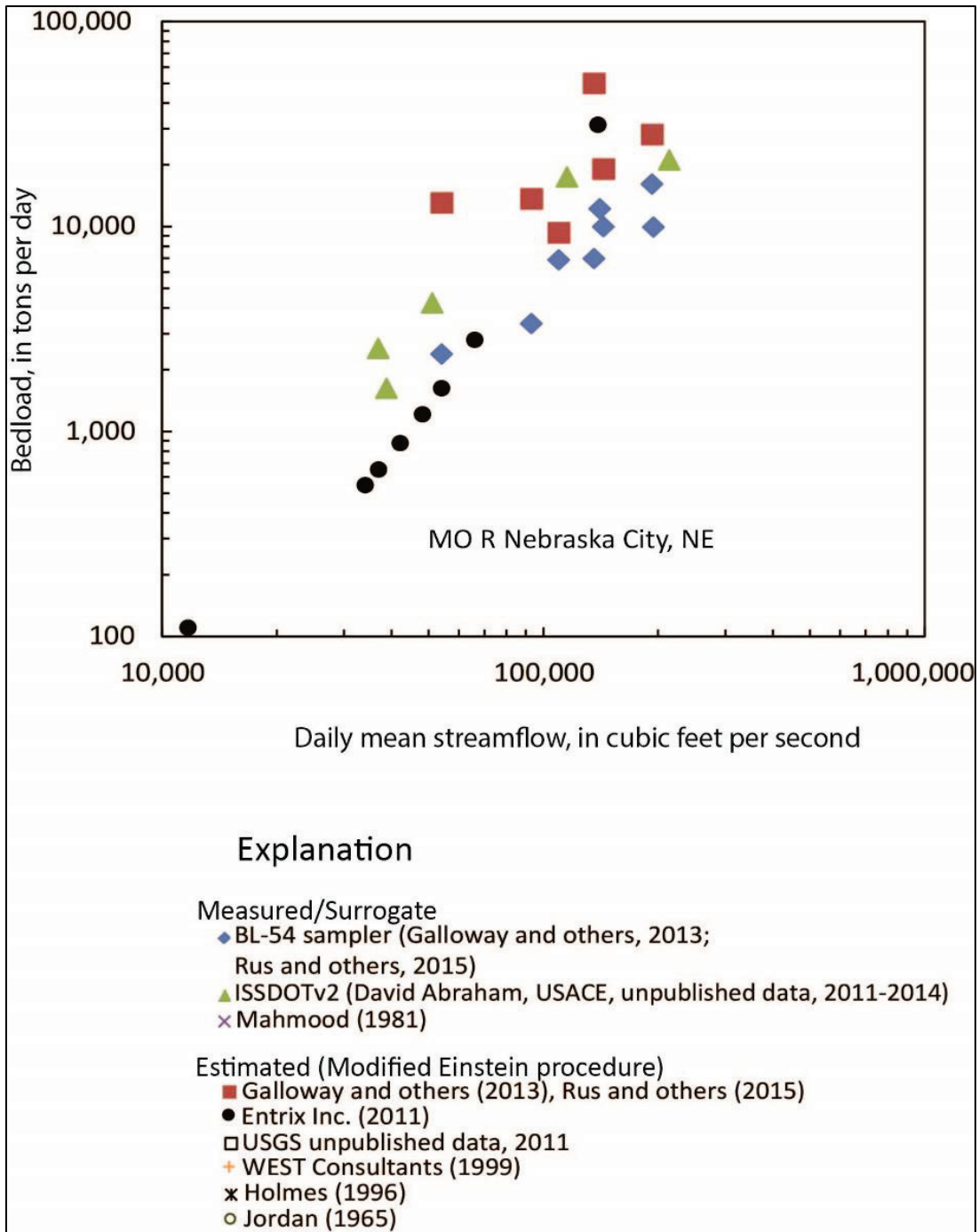
Figure 264. USGS bed-load data - Nebraska City, NE.
