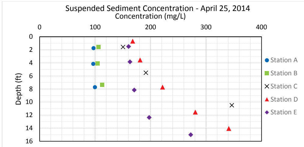
Figure 213. Suspended sediment concentration at Waverly, MO – April 25, 2014.
