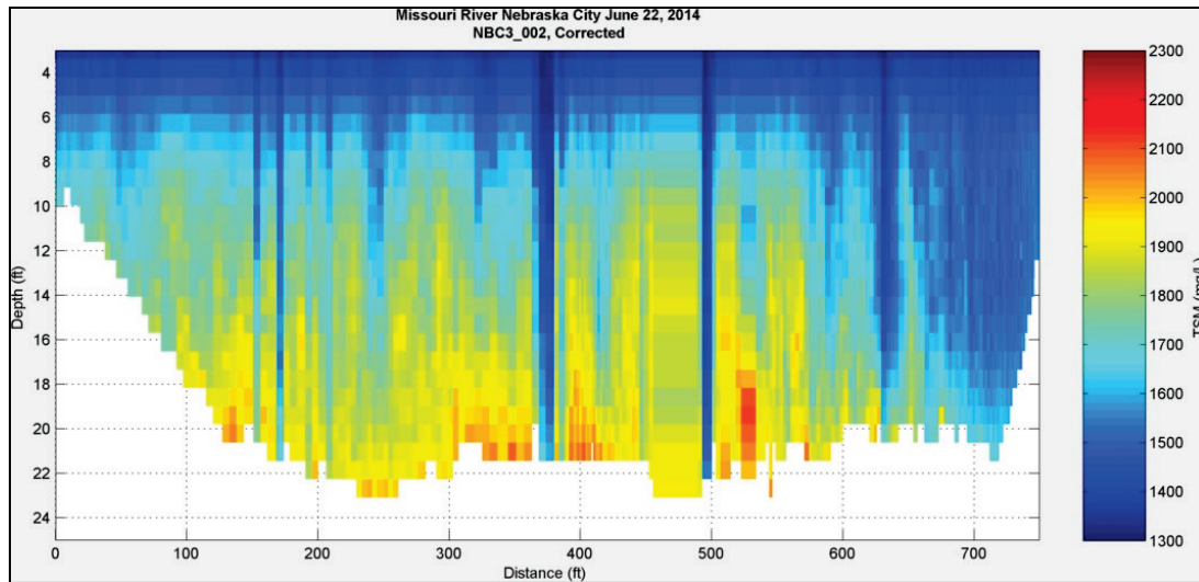
Figure 107. Suspended sediment concentration profile at Nebraska City, NE – June 22, 2014.
