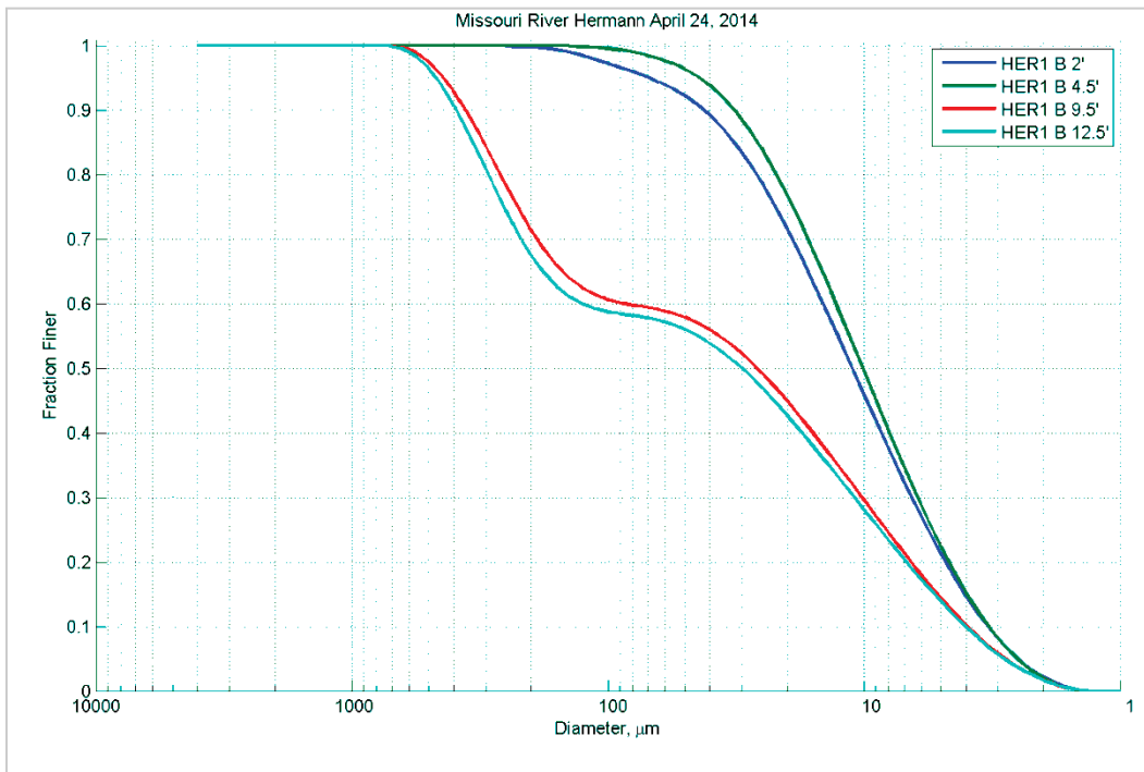
Figure 236. Particle size distribution at different depths (feet) in Station B - April 24, 2014.
