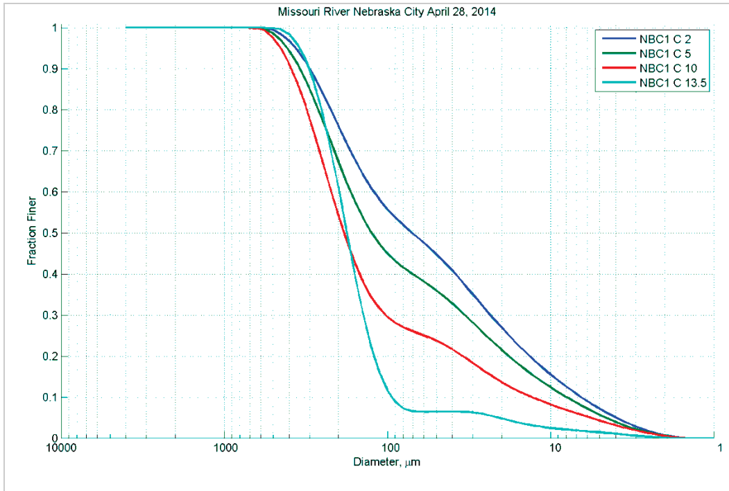
Figure 89. Particle size distribution at different depths (feet) in Station C - April 28, 2014.
