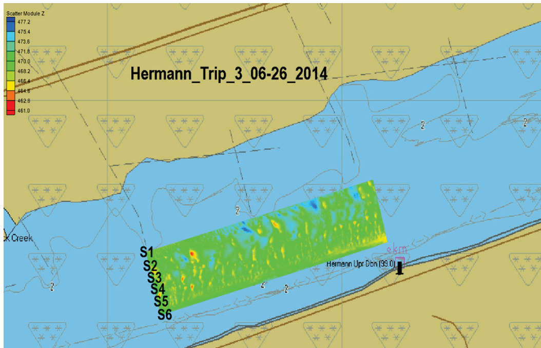
Figure 257. Bathymetry for Missouri River at Hermann, MO, showing swath locations.
