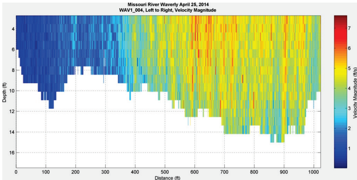
Figure 188. Velocity magnitude at Waverly, MO – April 25, 2014, 17:31:13.
