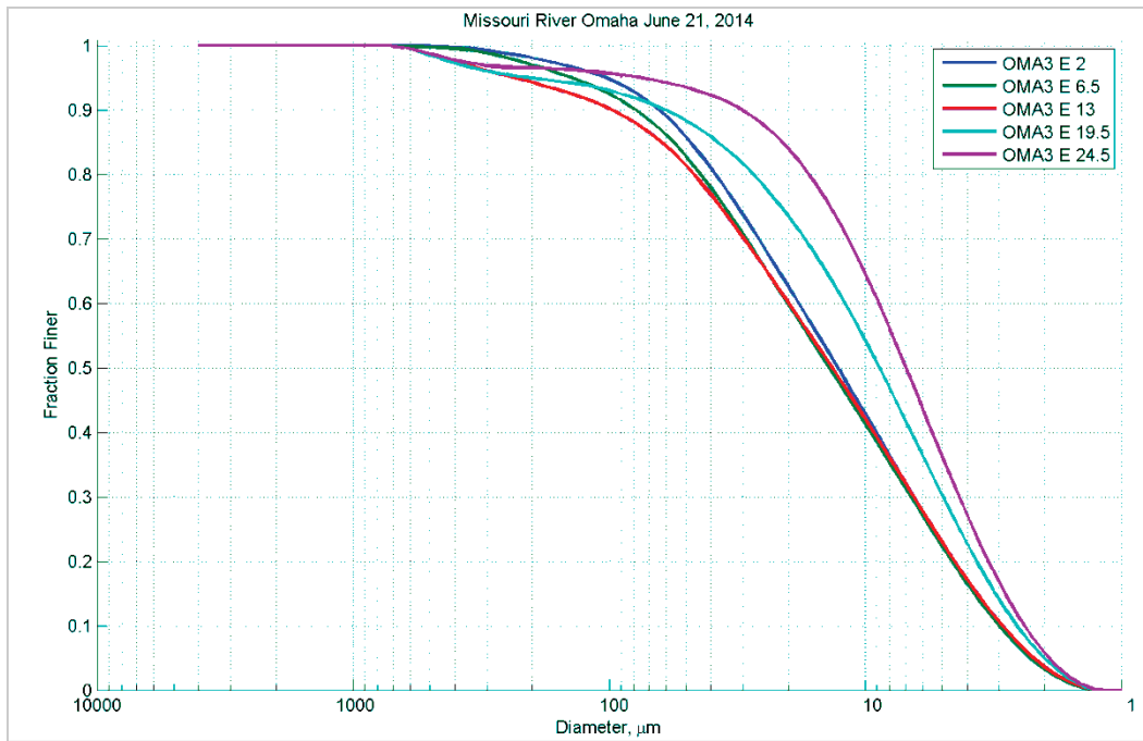
Figure 64. Particle size distribution at different depths (feet) in Station E – June 21, 2014.
