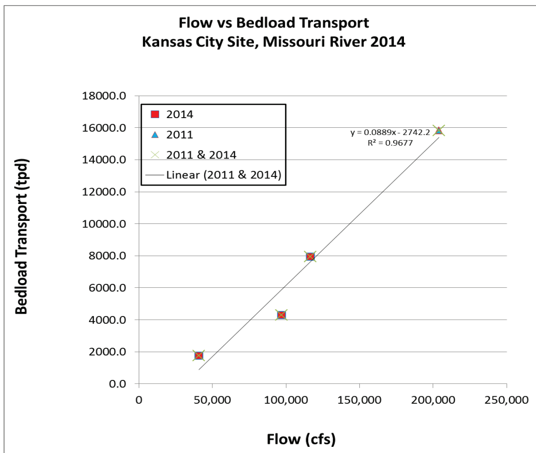
Figure 182. Bed-load rating curve for Kansas City, MO.
