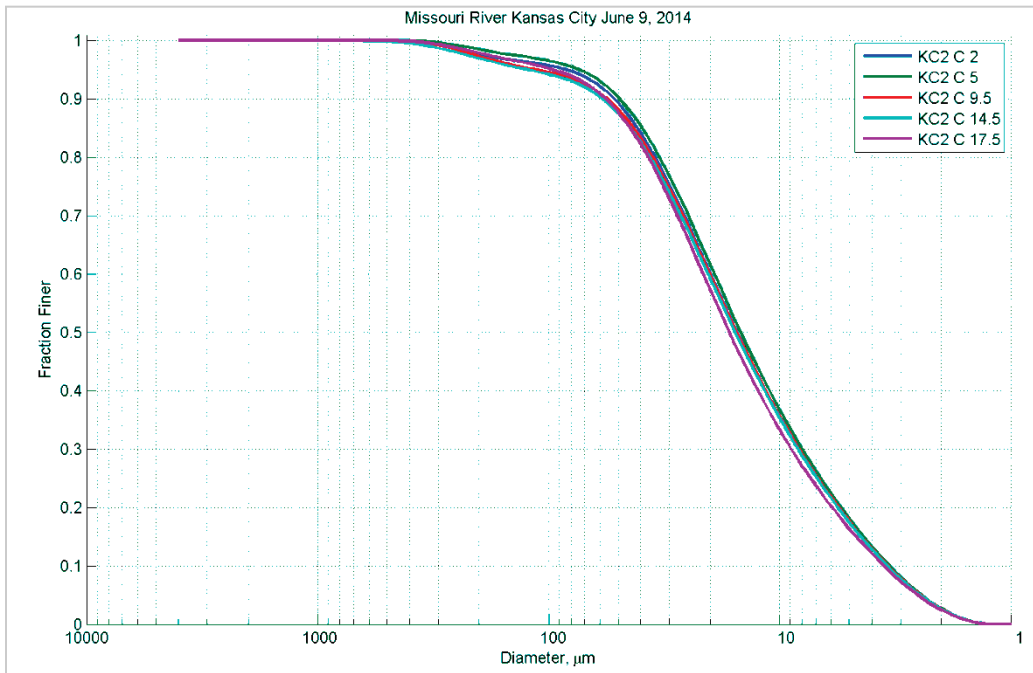
Figure 168. Particle size distribution at different depths (feet) in Station C – June 9, 2014.
