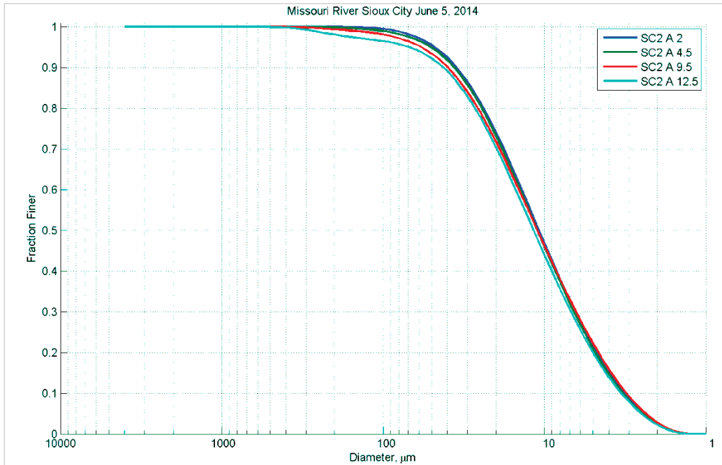
Figure 18. Particle size distribution at different depths (feet) in Station A – June 5, 2014.
