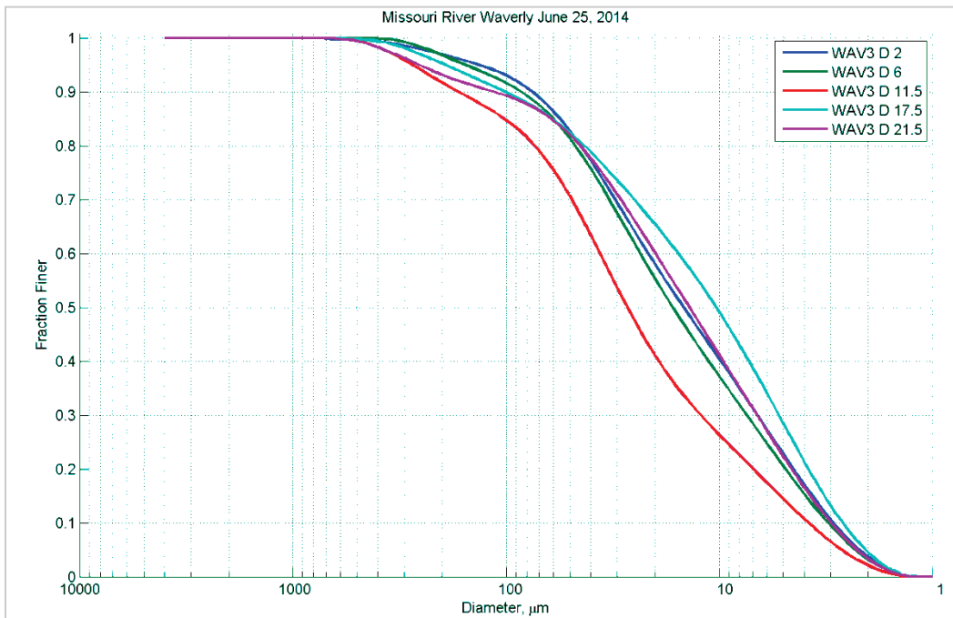
Figure 211. Particle size distribution at different depths (feet) in Station D – June 25, 2014.
