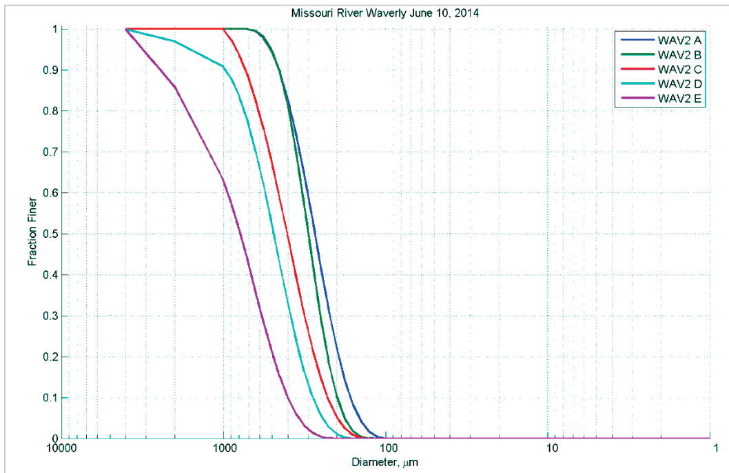
Figure 196. Bed material grain size distribution for Waverly, MO – June 10, 2014.
