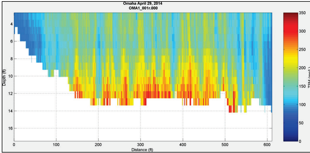
Figure 68. Suspended sediment concentration Profile at Omaha, NE - April 29, 2014.
