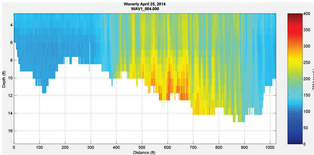
Figure 216. Suspended sediment concentration profile at Waverly, MO – April 25, 2014.
