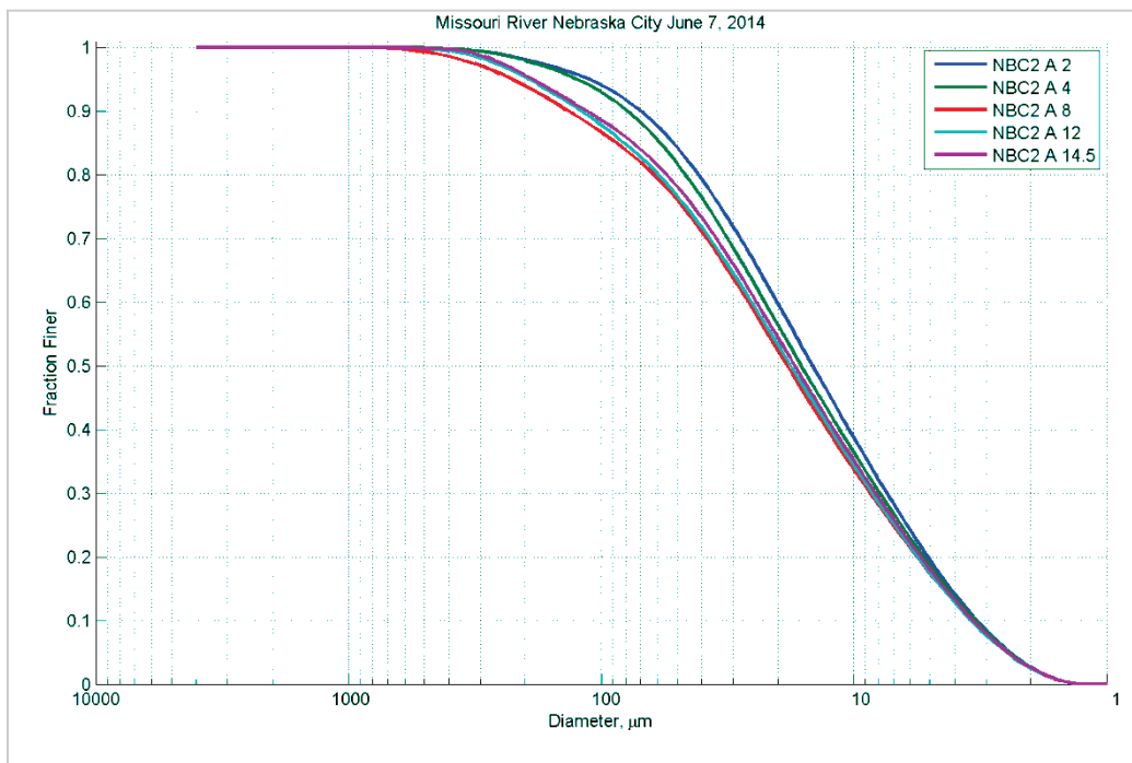
Figure 92. Particle size distribution at different depths (feet) in Station A – June 7, 2014.
