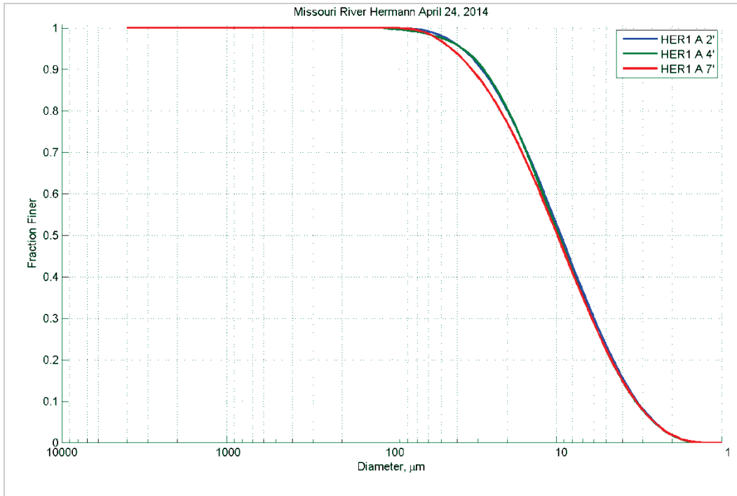
Figure 235. Particle size distribution at different depths (feet) in Station A - April 24, 2014.
