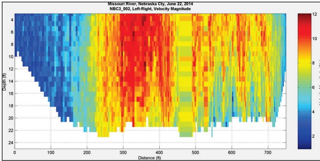
Figure 79. Velocity magnitude at Nebraska City, NE – June 22, 2014, 17:46:13.
