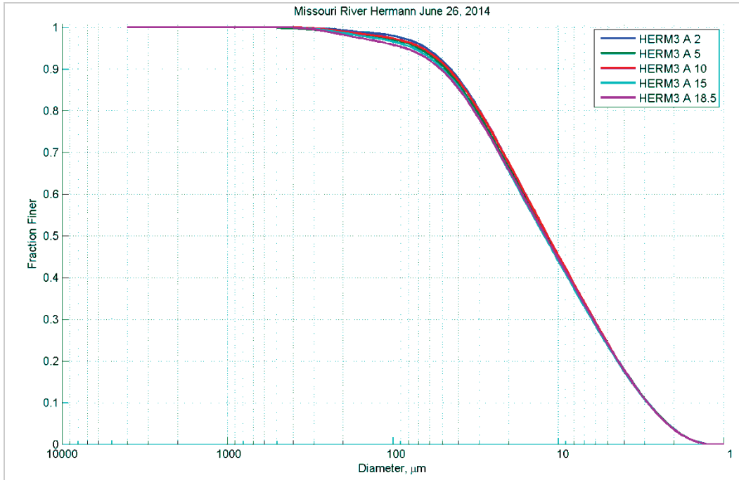
Figure 245. Particle size distribution at different depths (feet) in Station A – June 26, 2014.
