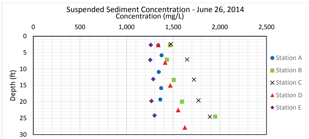
Figure 252. Suspended sediment concentration at Hermann, MO – June 26, 2014.
