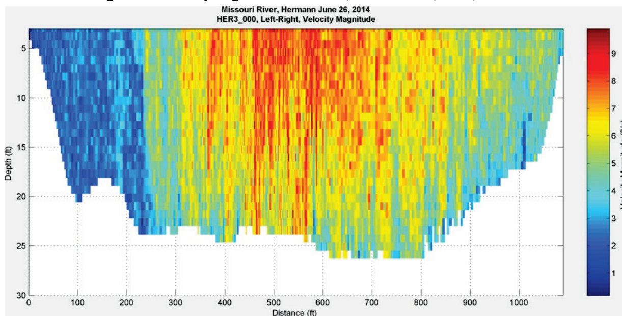
Figure 227. Velocity magnitude at Hermann, MO – June 26, 2014, 16:40:20.
