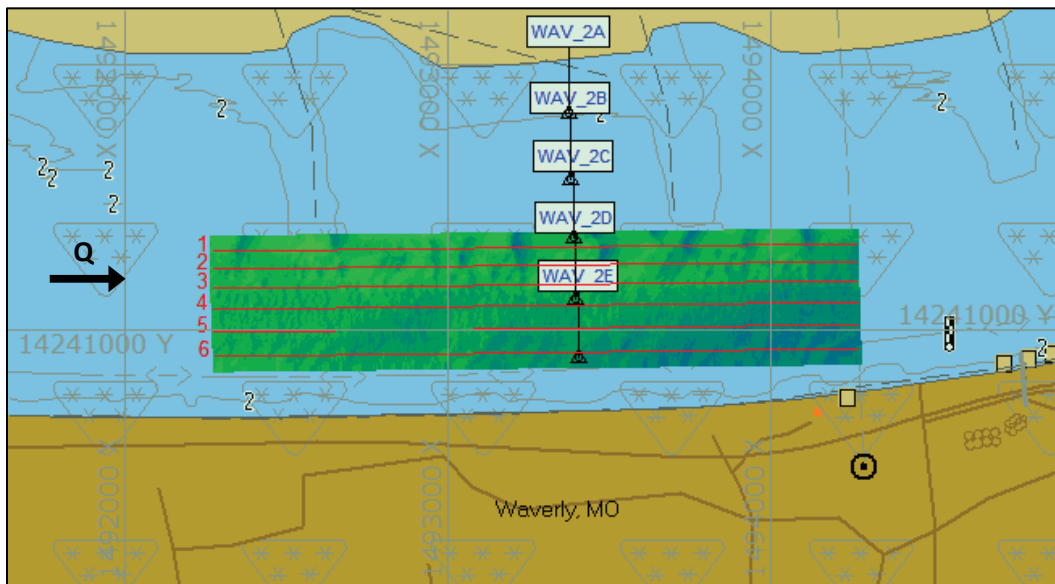
Figure 193. Multi-beam survey extent at Waverly, MO – June 10 and June 25, 2014.
