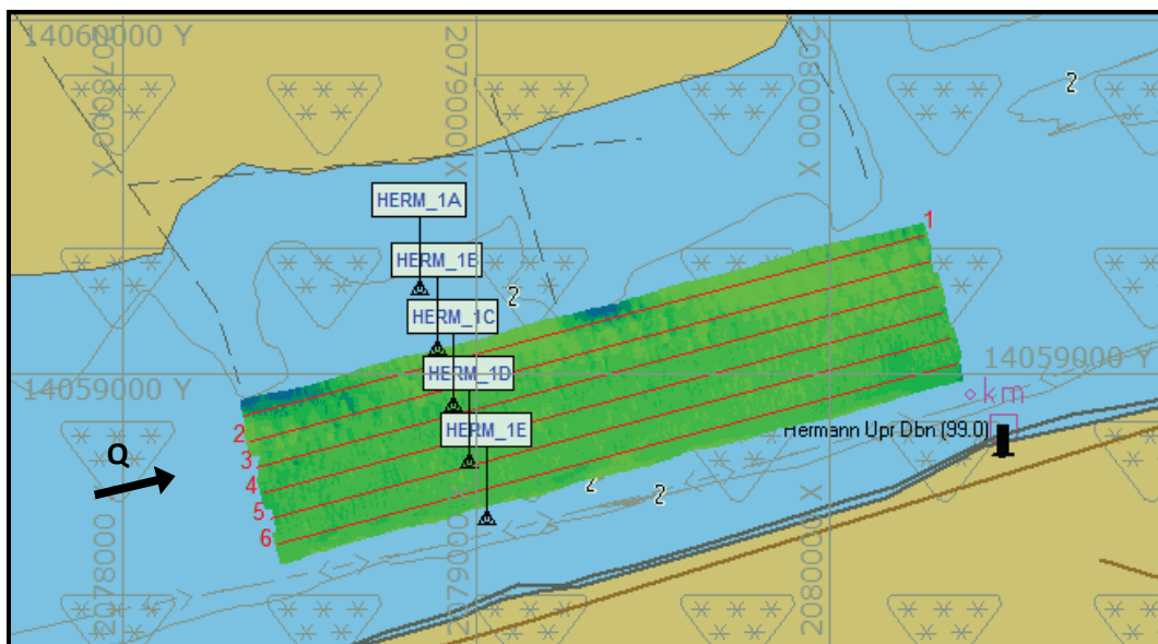
Figure 230. Multi-beam survey extent at Waverly, MO – June 11 and June 26, 2014.
