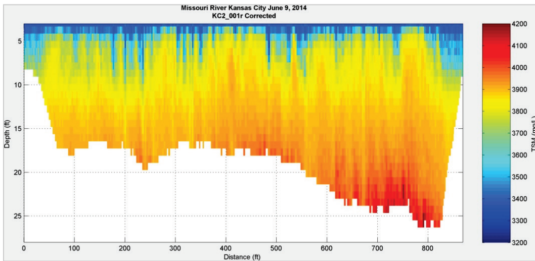
Figure 180. Suspended sediment concentration profile at Kansas City, MO – June 9, 2014.
