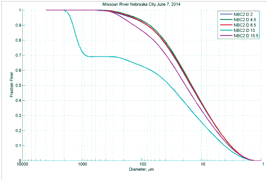
Figure 95. Particle size distribution at different depths (feet) in Station D – June 7, 2014.
