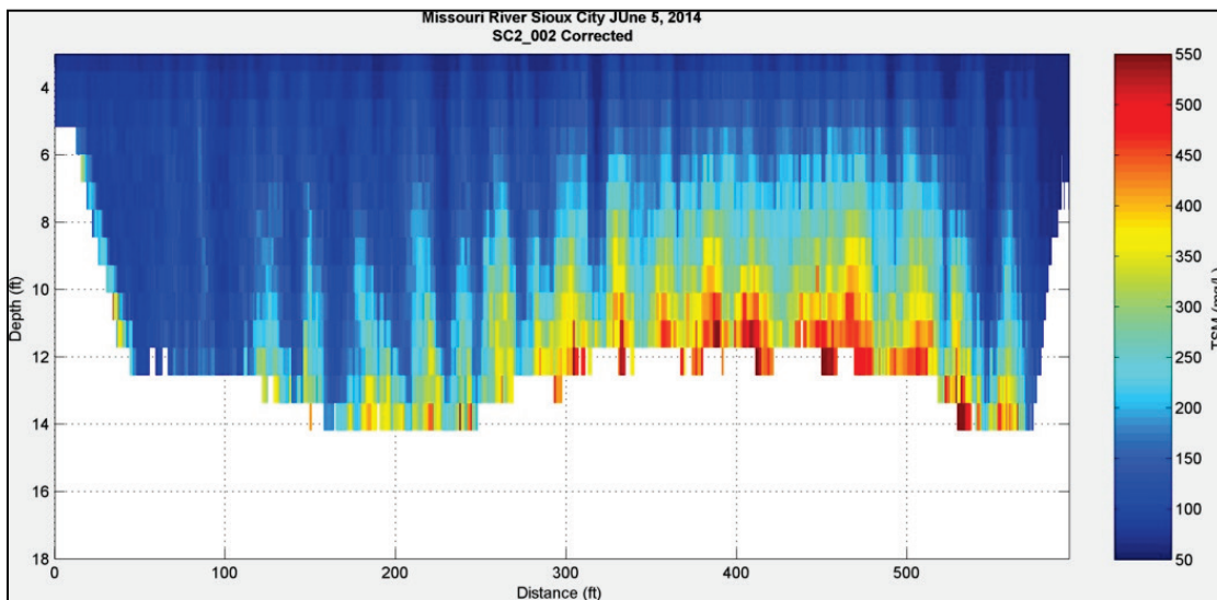
Figure 32. Suspended sediment concentration profile at Sioux City, IA – June 5, 2014.
