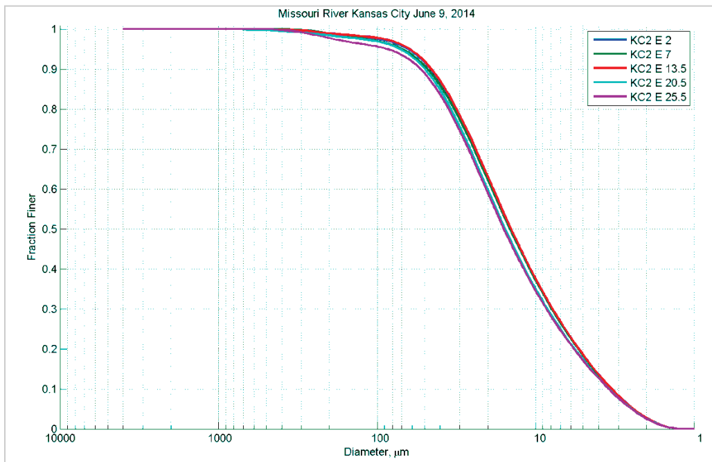
Figure 170. Particle size distribution at different depths (feet) in Station E – June 9, 2014.
