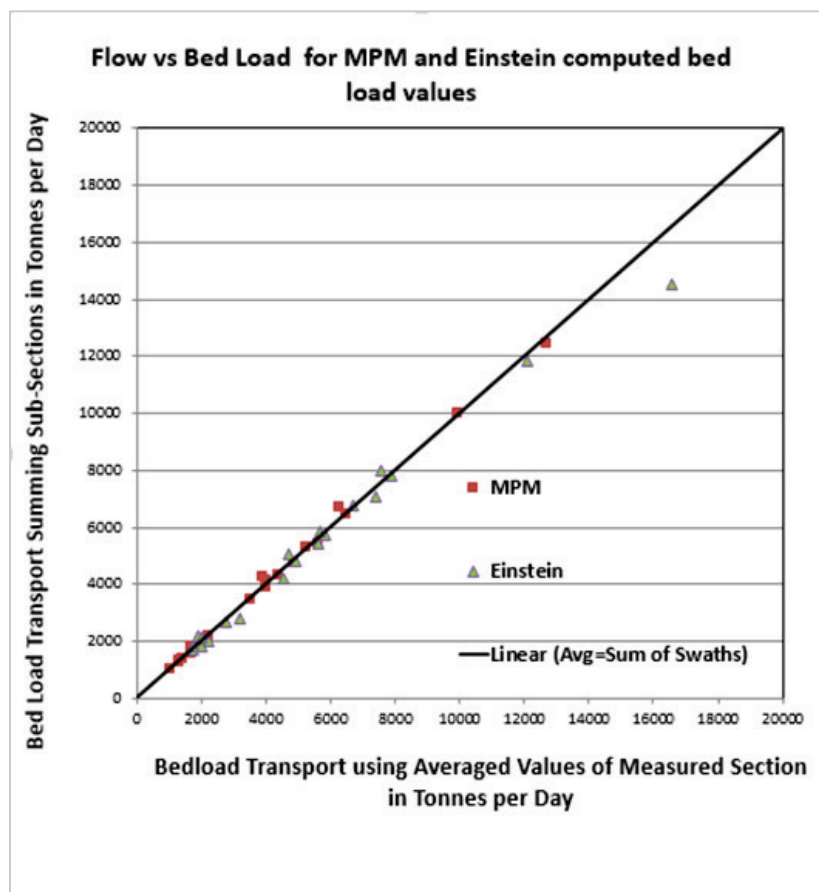
Figure 271. Measured section values of bed load compared to sub-cross-section sums.
