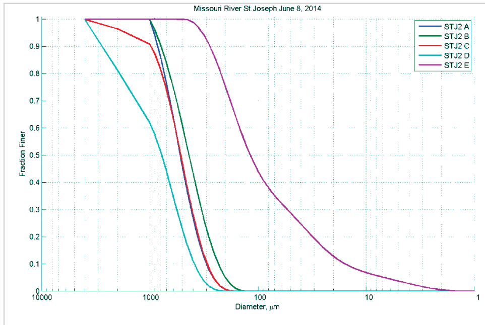
Figure 122. Bed material grain size distribution for St. Joseph, MO – June 8, 2014.
