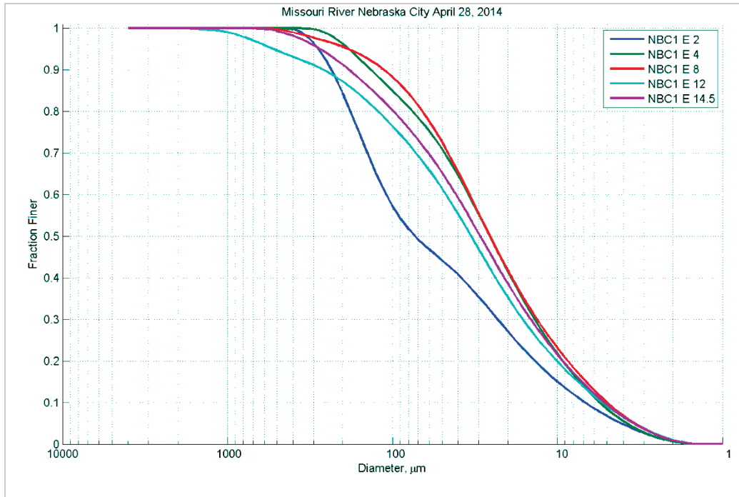
Figure 91. Particle size distribution at different depths (feet) in Station E - April 28, 2014.
