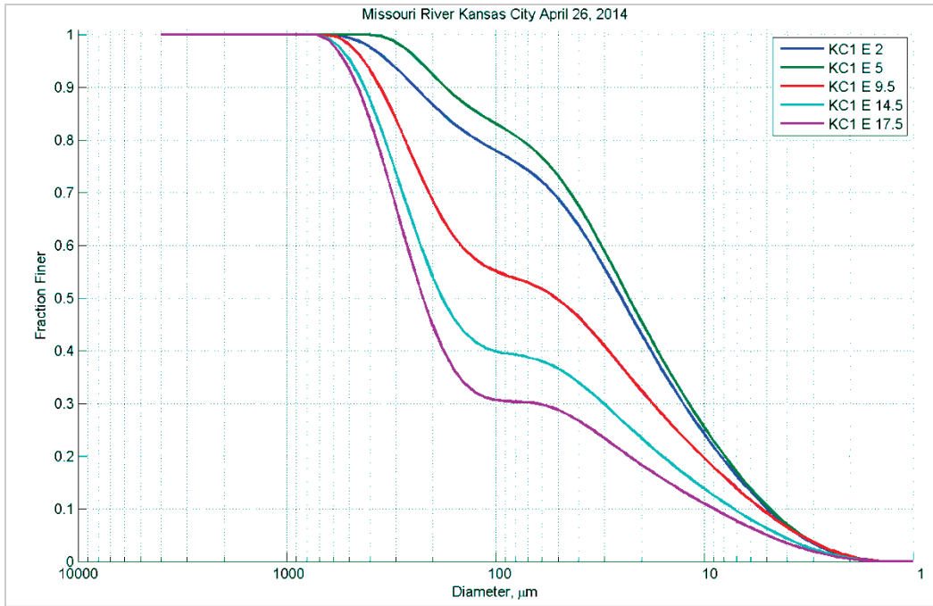
Figure 165. Particle size distribution at different depths (feet) in Station E - April 26, 2014.
