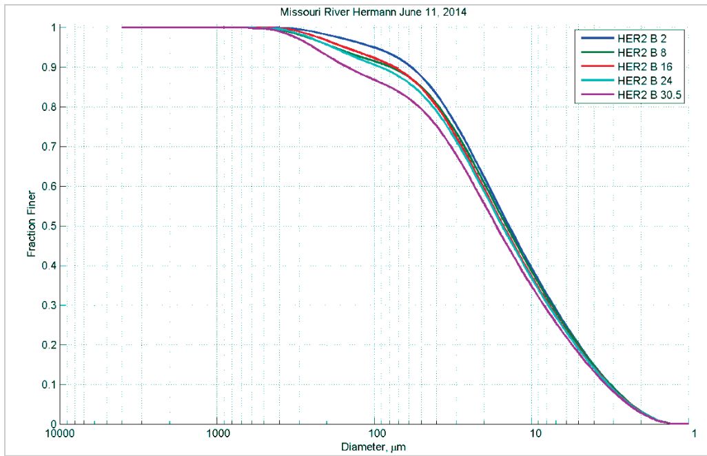
Figure 241. Particle size distribution at different depths (feet) in Station B – June 11, 2014.
