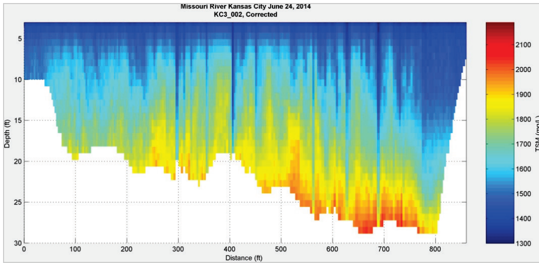
Figure 181. Suspended sediment concentration profile at Kansas City, MO – June 24, 2014.
