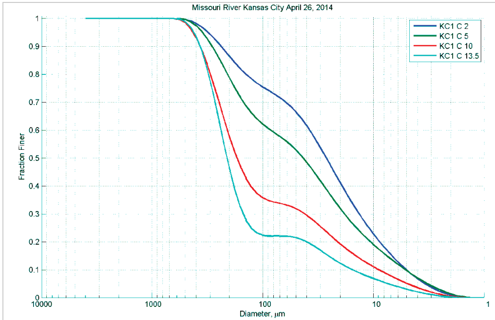
Figure 163. Particle size distribution at different depths (feet) in Station C - April 26, 2014.
