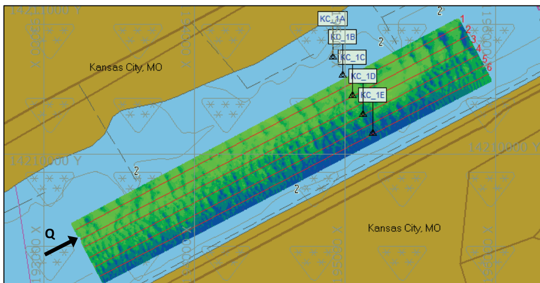
Figure 156. Multi-beam survey extent at Kansas City, MO – June 9 and June 24, 2014.
