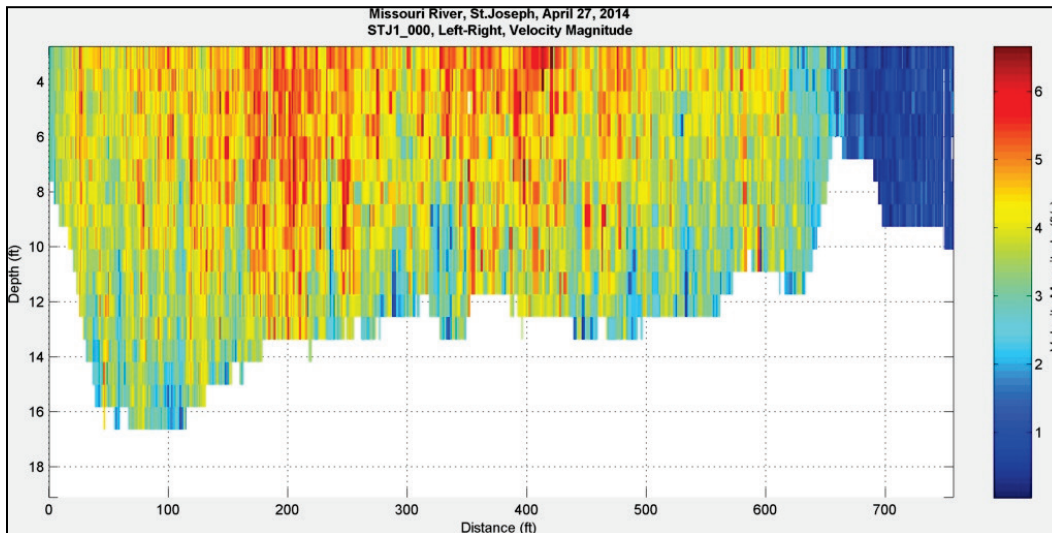
Figure 114. Velocity magnitude at St. Joseph, MO – April 27, 2014, 14:20:08.
