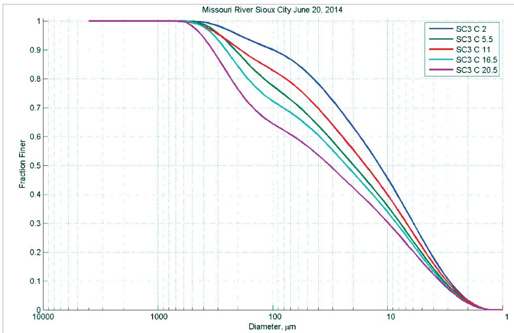
Figure 25. Particle size distribution at different depths (feet) in Station C – June 20, 2014.
