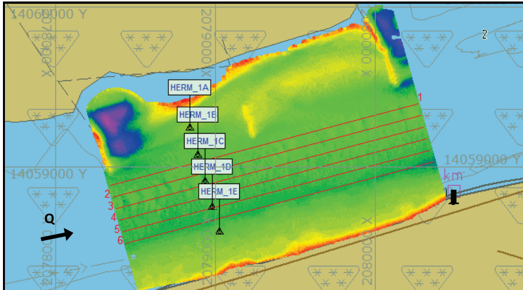
Figure 229. Multi-beam survey extent at Hermann, MO – April 24, 2014.
