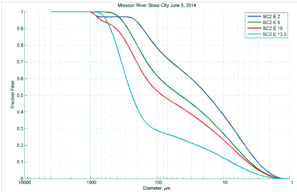
Figure 22. Particle size distribution at different depths (feet) in Station E – June 5, 2014.
