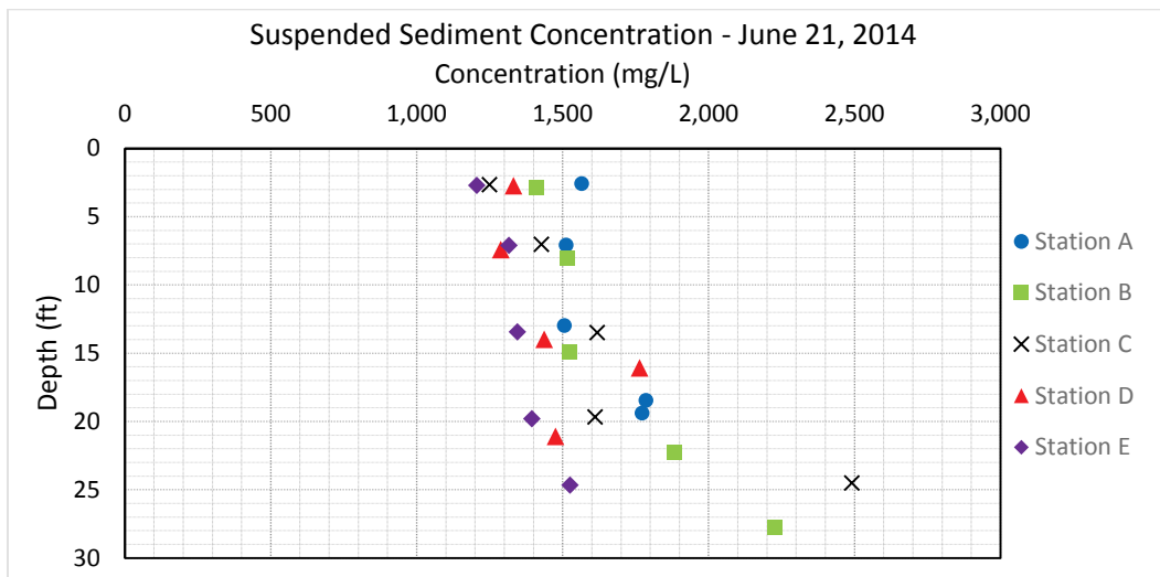
Figure 67. Suspended sediment concentration at Omaha, NE – June 21, 2014.
