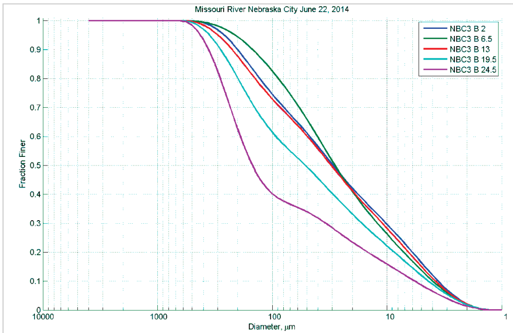
Figure 98. Particle size distribution at different depths (feet) in Station B – June 22, 2014.
