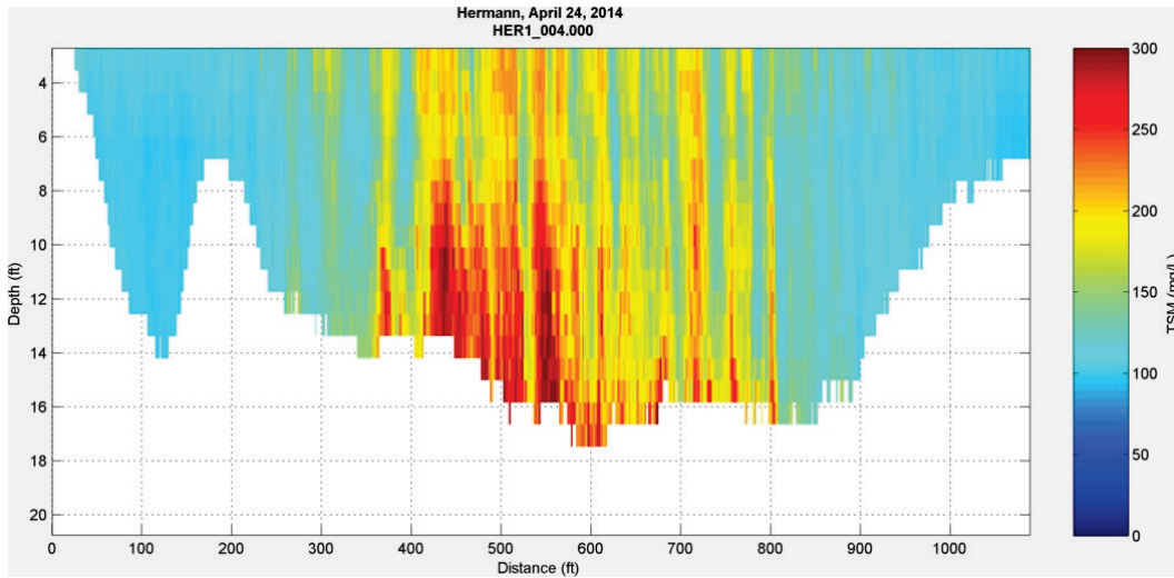
Figure 253. Suspended sediment concentration profile at Hermann, MO – April 24, 2014.
