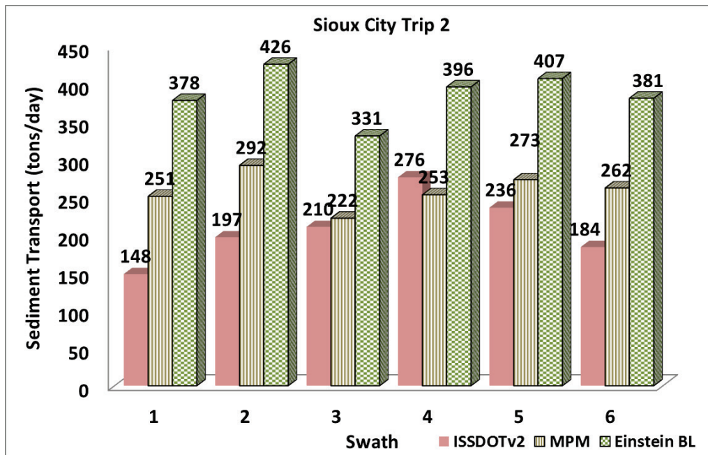
Figure 37. Bed-load transport at Sioux City, IA – June 5, 2014: ISSDOTv2 values compared to transport function computed values.
