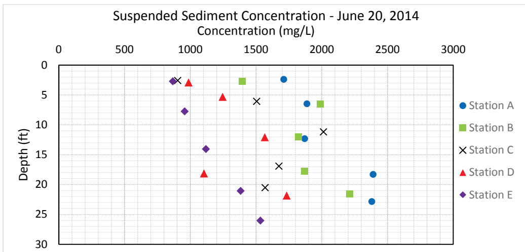
Figure 30. Suspended sediment concentration at Sioux City, IA – June 20, 2014.
