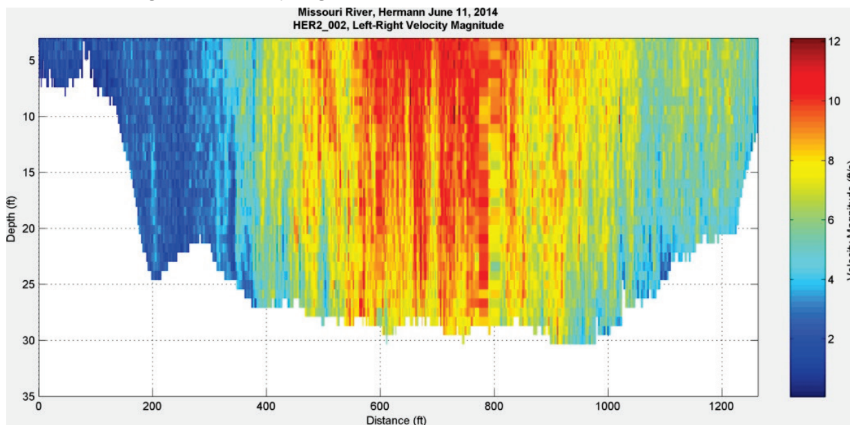
Figure 226. Velocity magnitude at Hermann, MO – June 11, 2014, 16:38:54.
