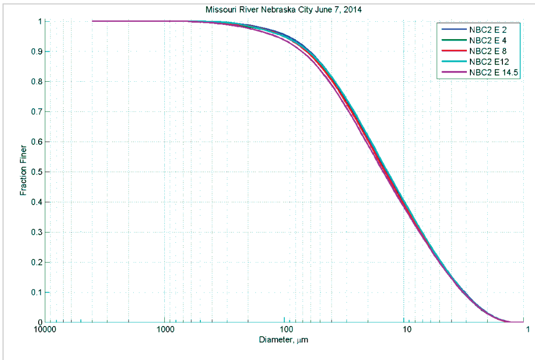
Figure 96. Particle size distribution at different depths (feet) in Station E – June 7, 2014.
