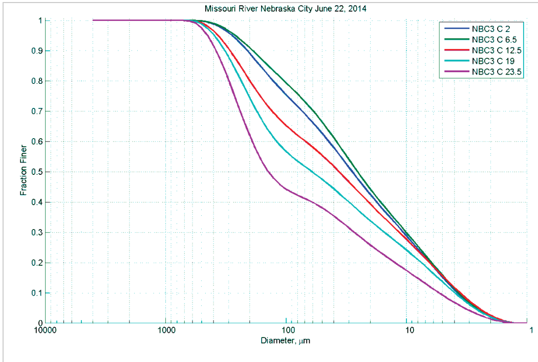
Figure 99. Particle size distribution at different depths (feet) in Station C – June 22, 2014.
