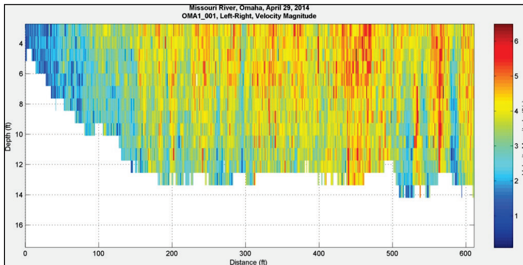
Figure 40. Velocity magnitude at Omaha, NE – April 29, 2014, 14:45:51.
