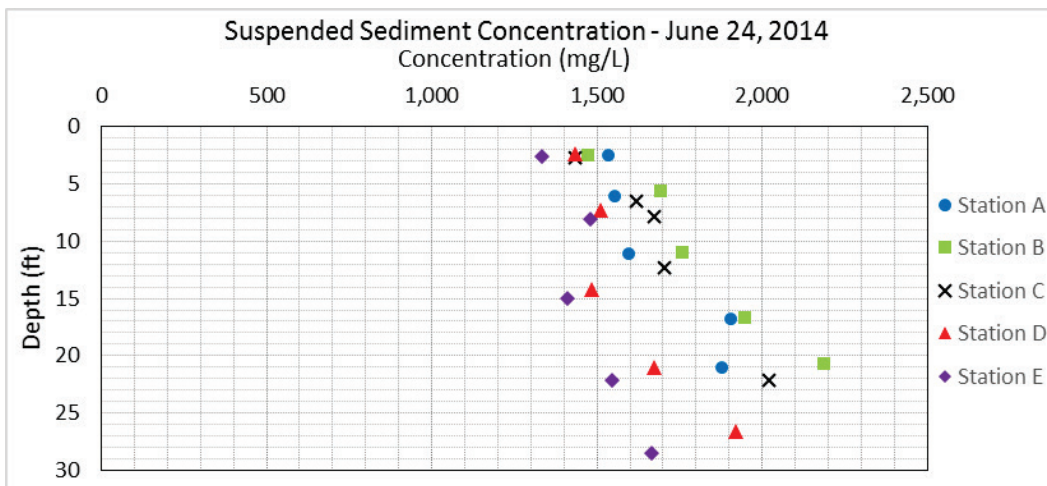
Figure 178. Suspended sediment concentration at Kansas City, MO – June 24, 2014.
