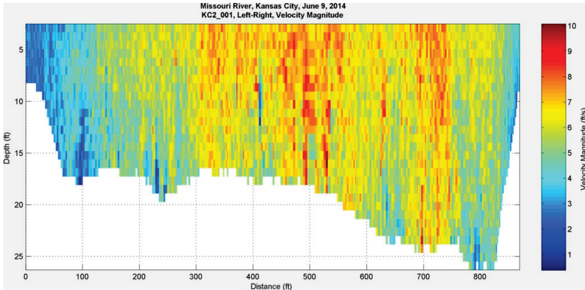
Figure 152. Velocity magnitude at Kansas City, MO – June 9, 2014, 17:21:41.
