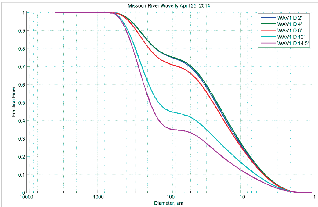
Figure 201. Particle size distribution at different depths (feet) in Station D - April 25, 2014.
