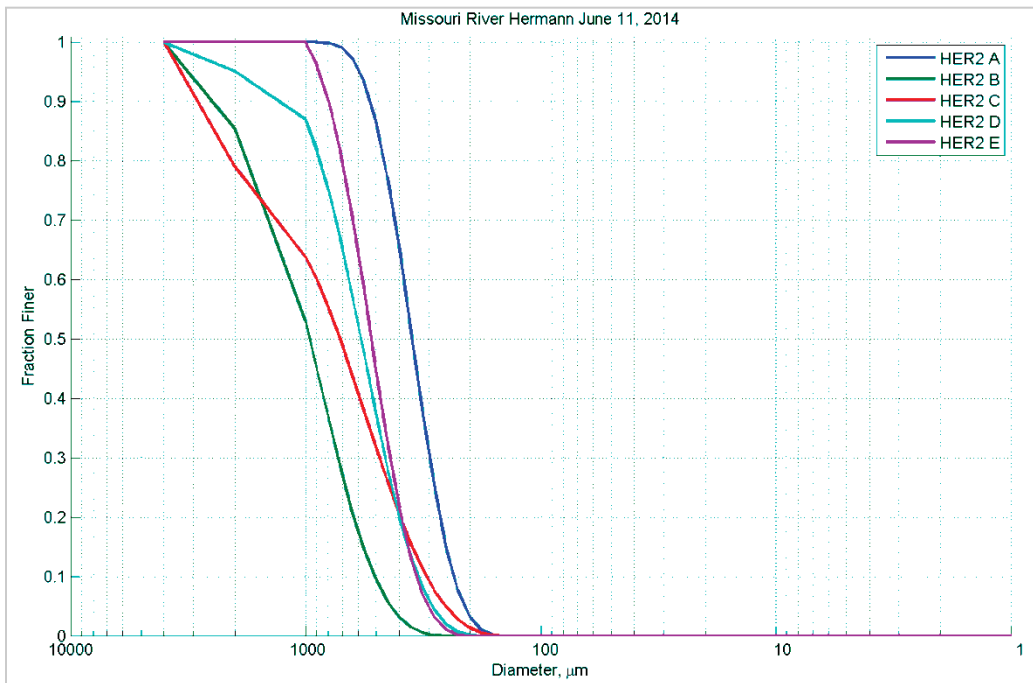
Figure 233. Bed material grain size distribution for Hermann, MO – June 11, 2014.
