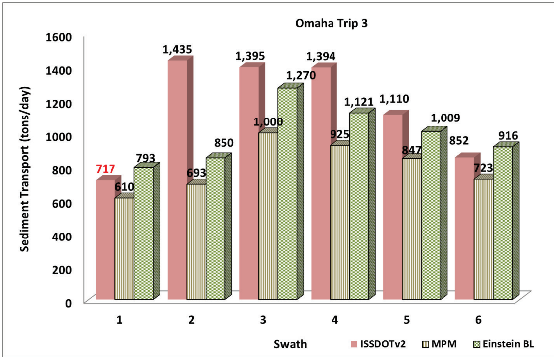
Figure 75. Bed-load transport at Omaha, NE– June 21, 2014: ISSDOTv2 values compared to transport function computed values, where red indicates an interpolated value.
