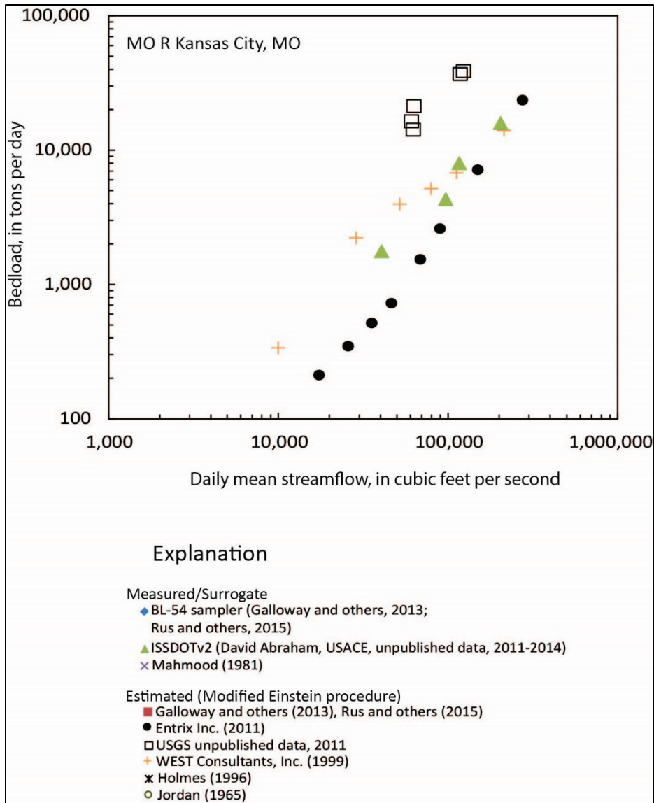
Figure 266. USGS bed-load data – Kansas City, MO.
