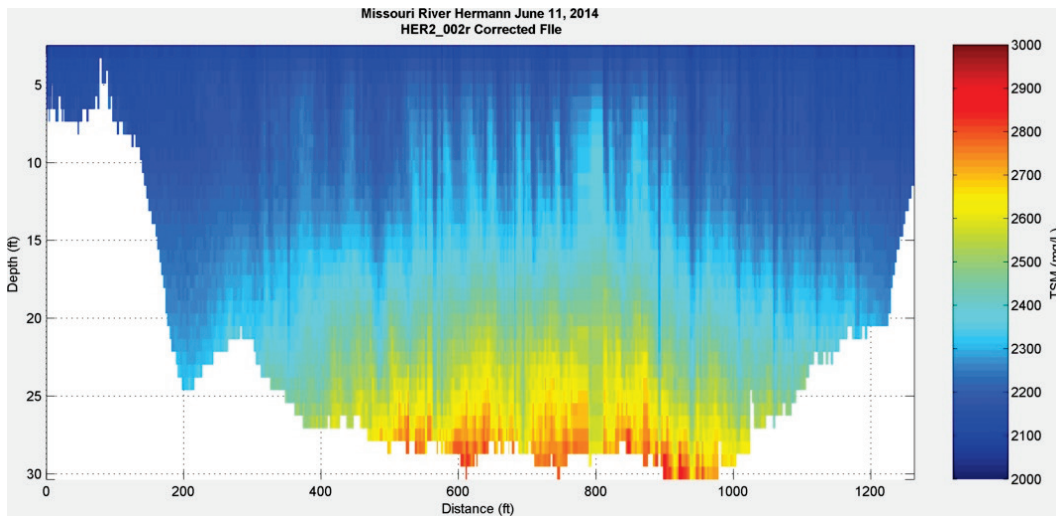
Figure 254. Suspended sediment concentration profile at Hermann, MO – June 11, 2014.
