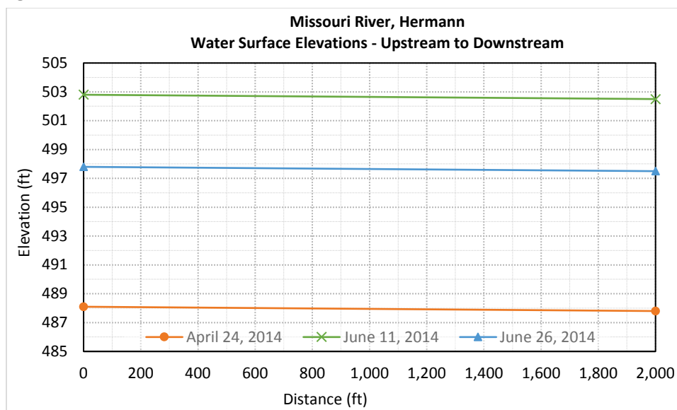
Figure 228. Water surface elevation at Hermann, MO – from upstream to downstream.
