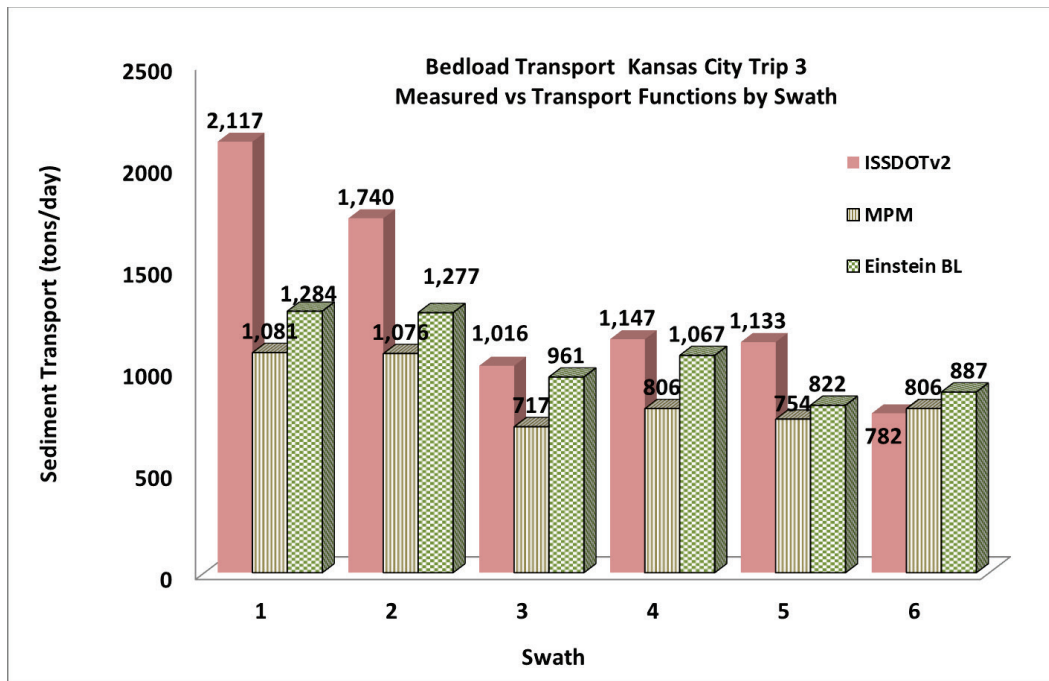
Figure 186. Bed-load transport at Kansas City, MO – June 26, 2014: ISSDOTv2 values compared to transport function computed values.
