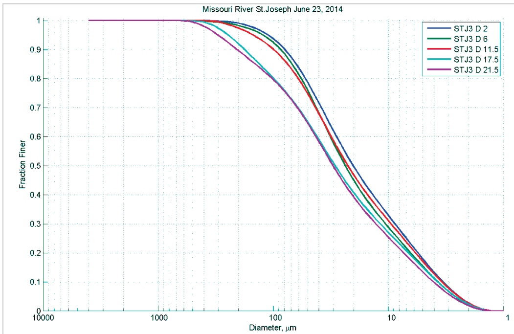
Figure 137. Particle size distribution at different depths (feet) in Station D – June 24, 2014.
