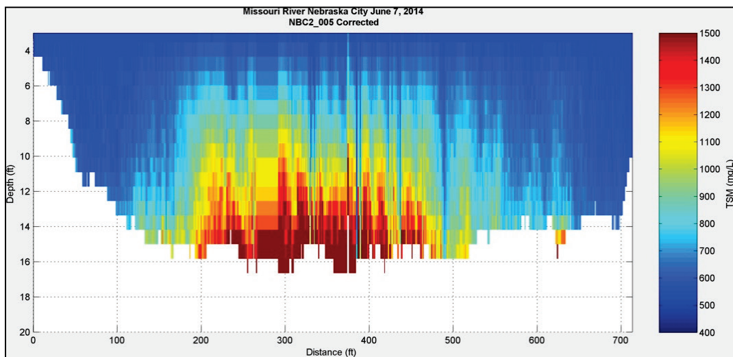
Figure 106. Suspended sediment concentration profile at Nebraska City, NE - June 7, 2014.
