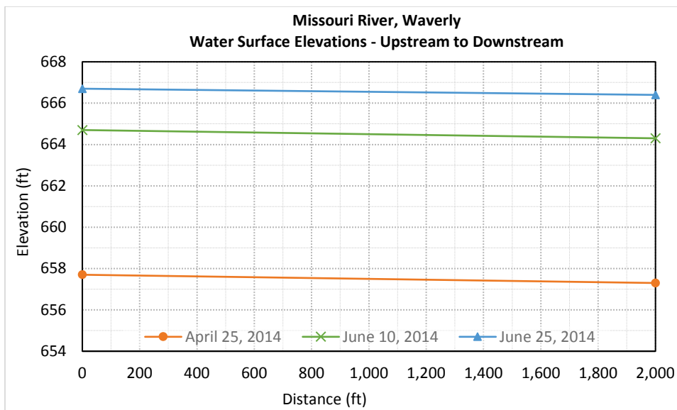
Figure 191. Water surface elevation at Waverly, MO – from upstream to downstream.
