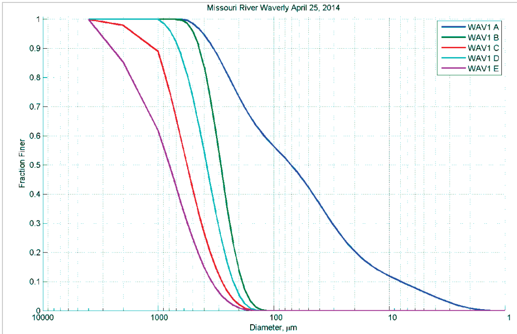
Figure 195. Bed material grain size distribution for Waverly, MO – April 25, 2014.
