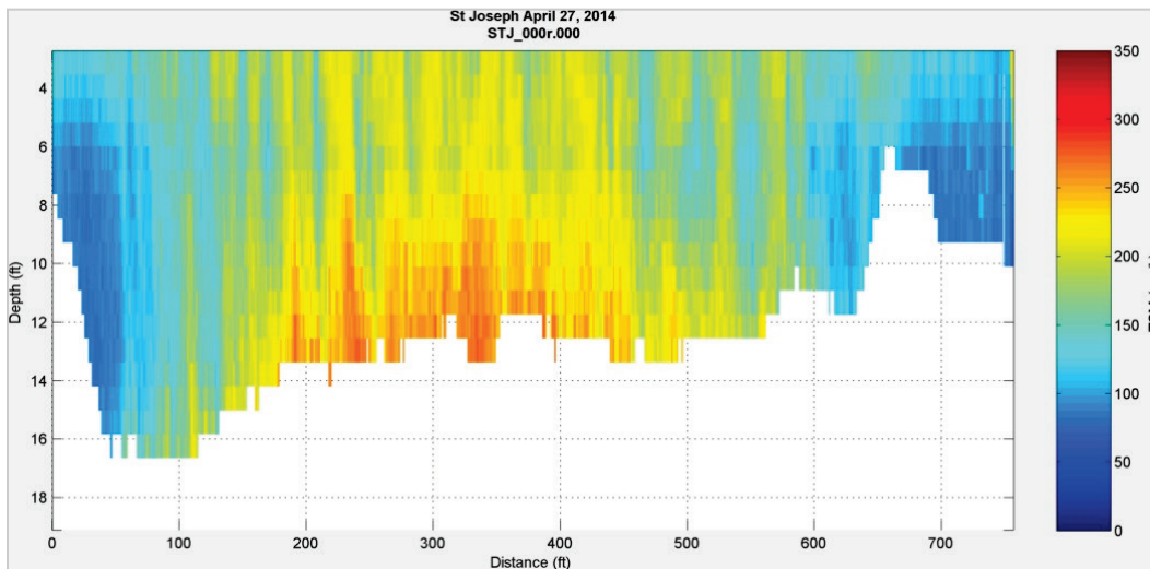
Figure 142. Suspended sediment concentration profile at St. Joseph, MO - April 27, 2014.
