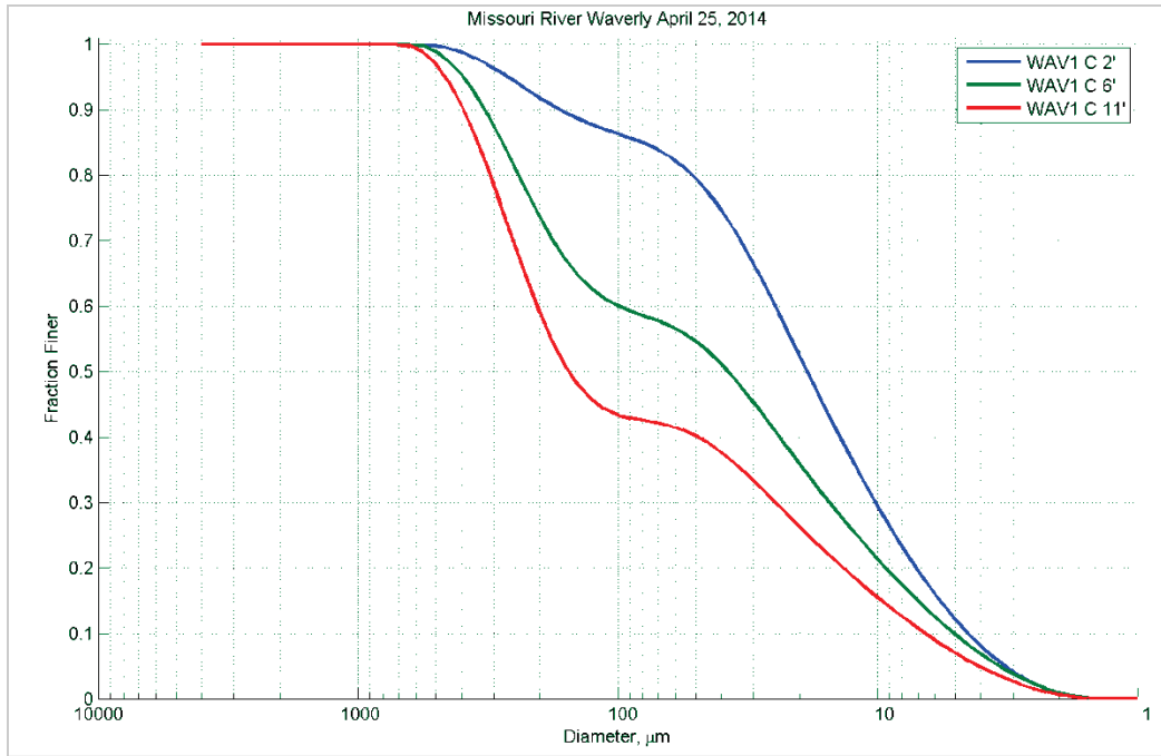
Figure 200. Particle size distribution at different depths (feet) in Station C - April 25, 2014.
