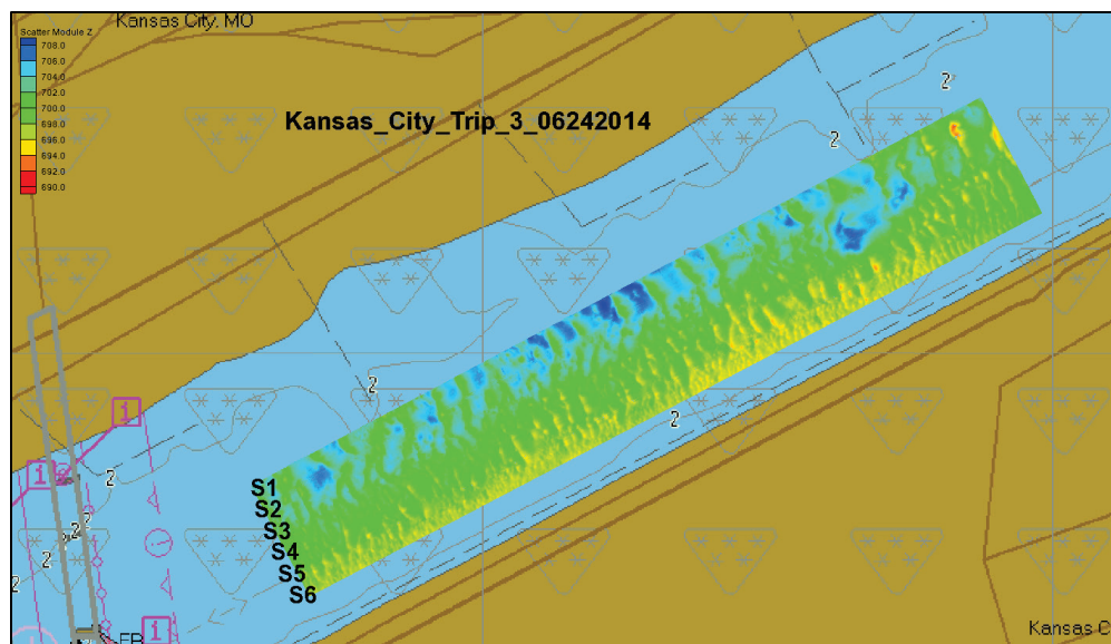
Figure 183. Bathymetry for Kansas City showing swath locations.
