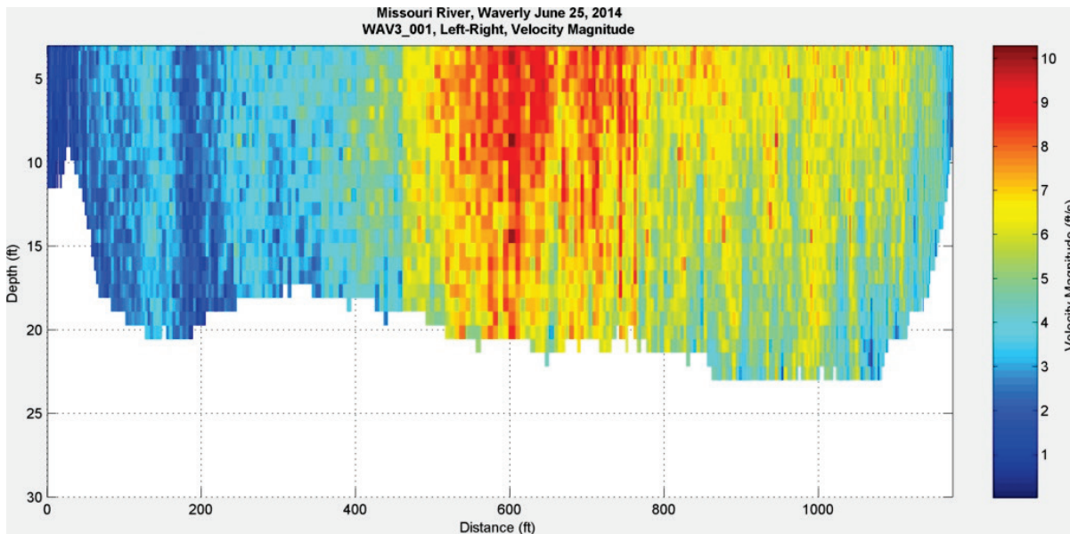
Figure 190. Velocity magnitude at Waverly, MO – June 25, 2014, 16:26:28.
