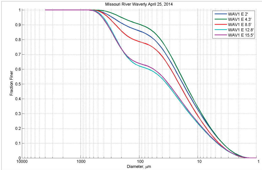
Figure 202. Particle size distribution at different depths (feet) in Station E - April 25, 2014.
