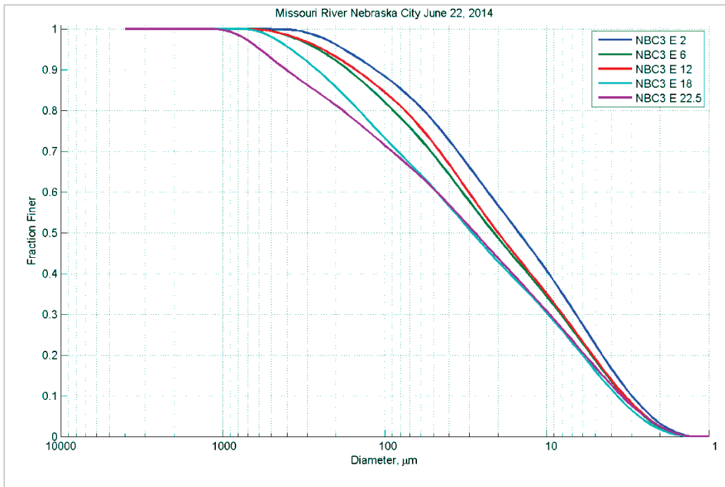
Figure 101. Particle size distribution at different depths (feet) in Station E – June 22, 2014.
