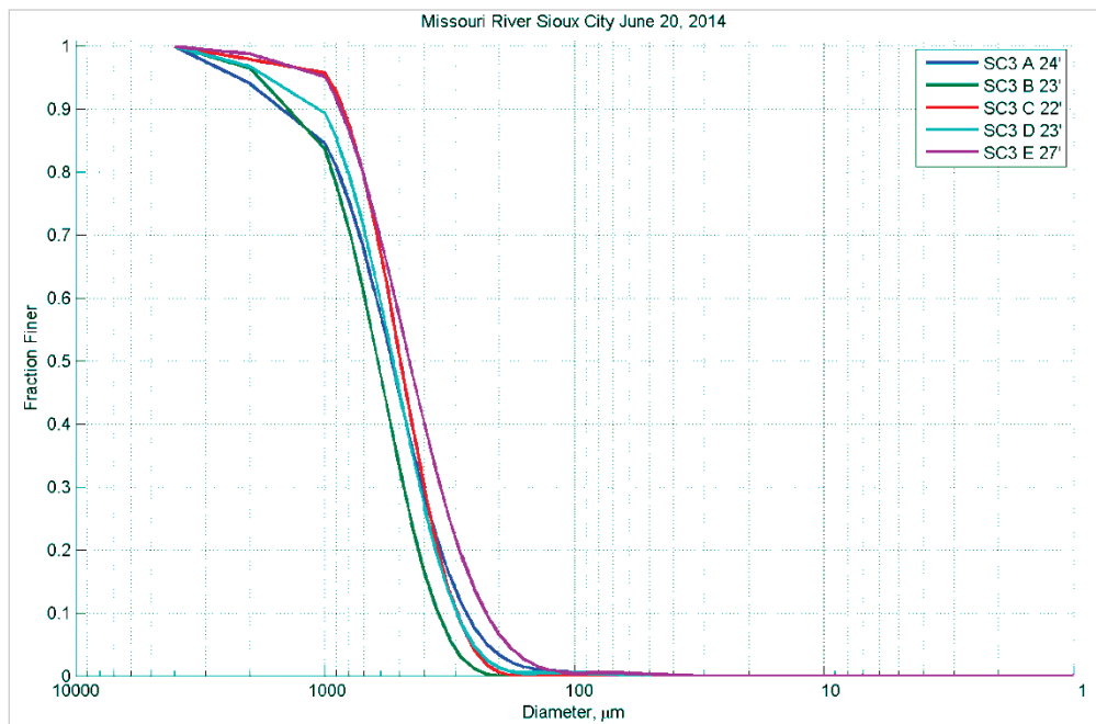
Figure 12. Bed material grain size distribution for Sioux City, IA – June 20, 2014.
