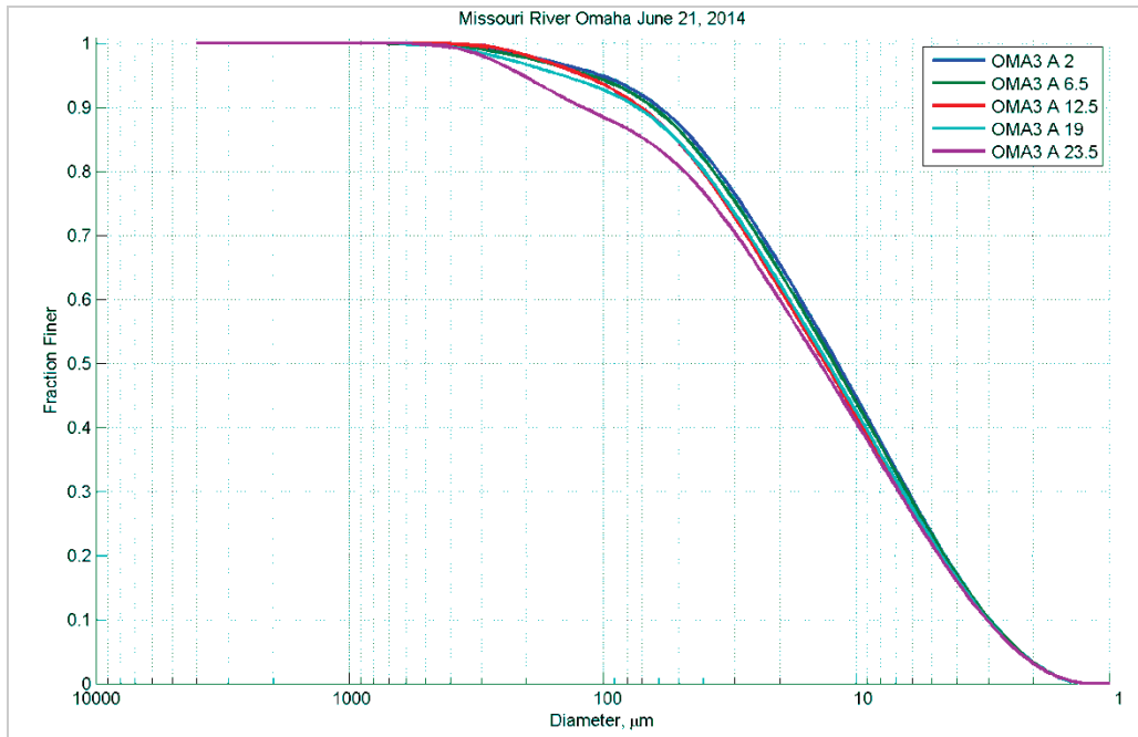
Figure 60. Particle size distribution at different depths (feet) in Station A – June 21, 2014.
