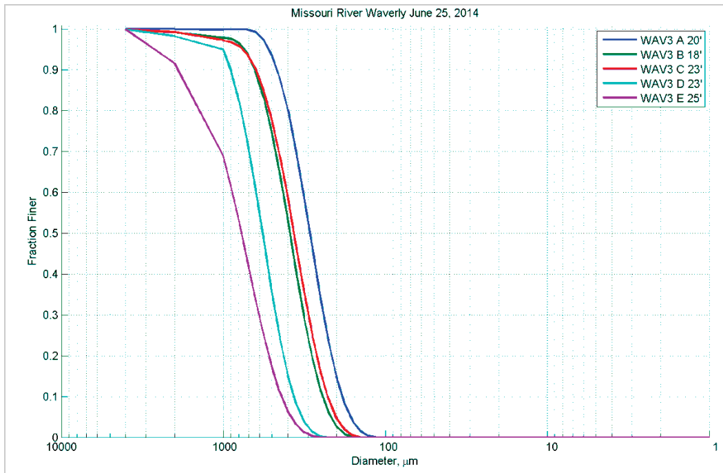
Figure 197. Bed material grain size distribution for Waverly, MO – June 25, 2014.
