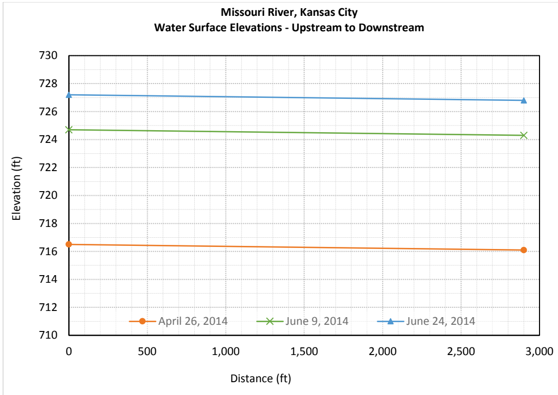
Figure 154. Water surface elevation at Kansas City, MO – from upstream to downstream.
