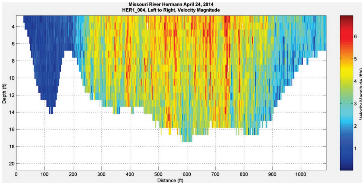
Figure 225. Velocity magnitude at Hermann, MO – April 24, 2014, 16:48:52.
