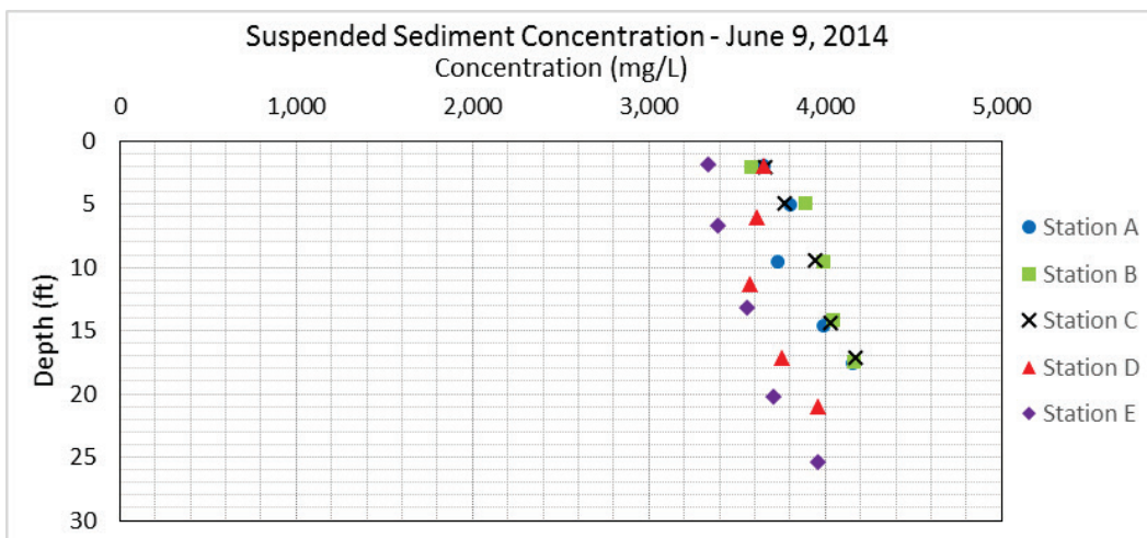
Figure 177. Suspended sediment concentration at Kansas City, MO – June 9, 2014.
