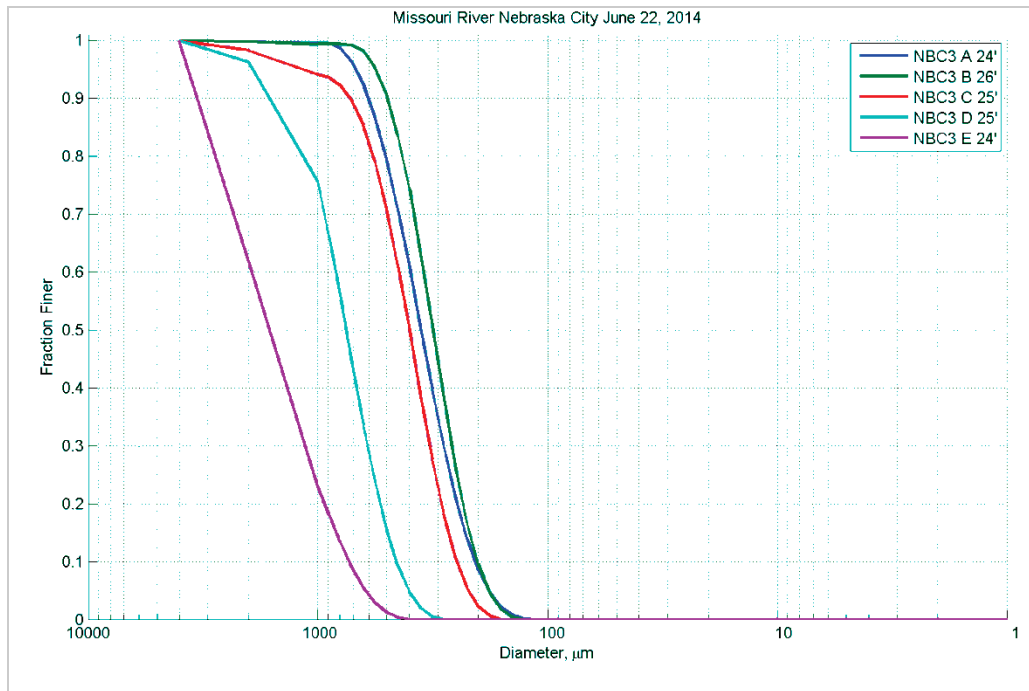
Figure 86. Bed material grain size distribution for Nebraska City, NE – June 22, 2014.
