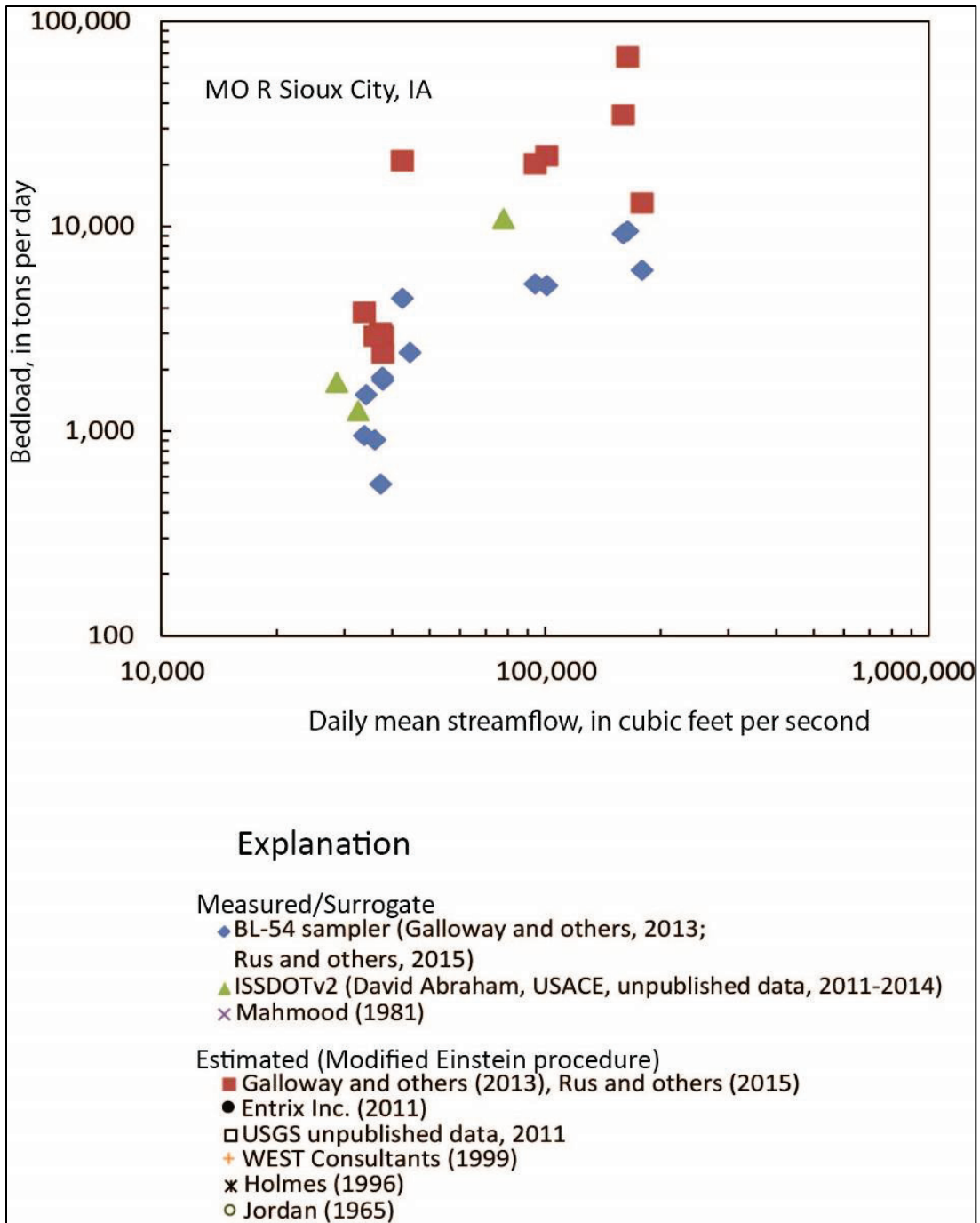
Figure 262. USGS bed-load data - Sioux City, IA.
