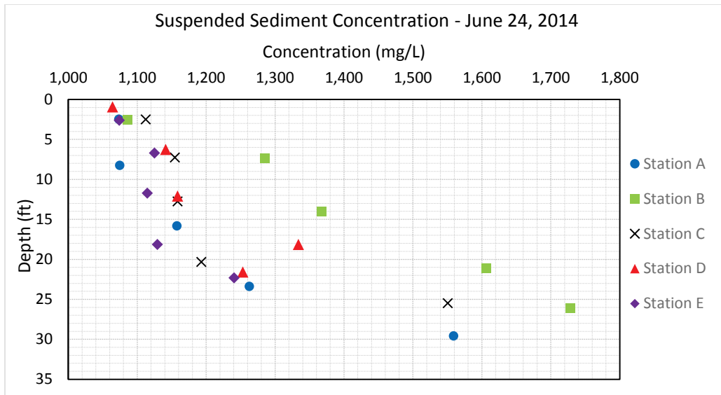
Figure 141. Suspended sediment concentration at St. Joseph, MO – June 24, 2014.
