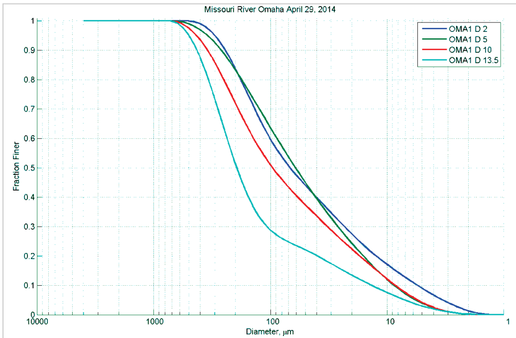
Figure 53. Particle size distribution at different depths (feet) in Station D – April 29, 2014.
