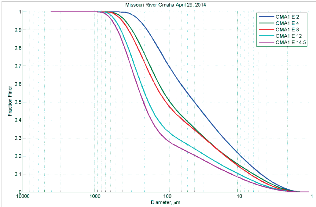
Figure 54. Particle size distribution at different depths (feet) in Station E – April 29, 2014.
