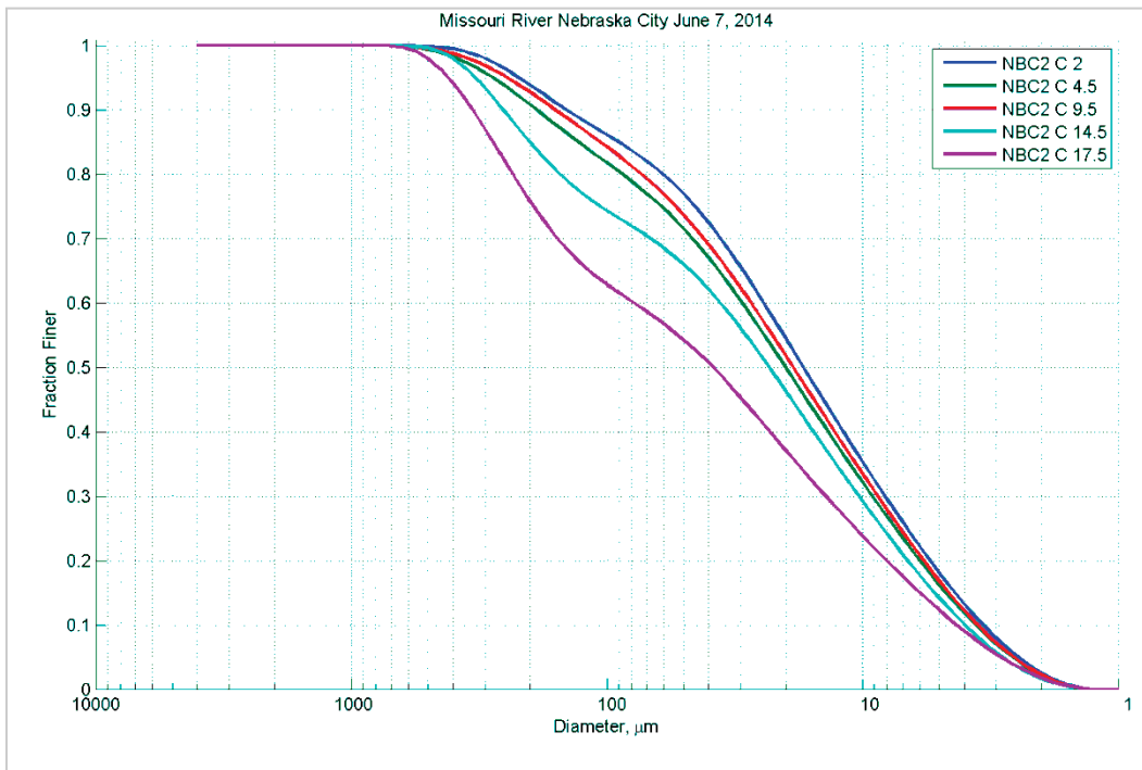
Figure 94. Particle size distribution at different depths (feet) in Station C – June 7, 2014.
