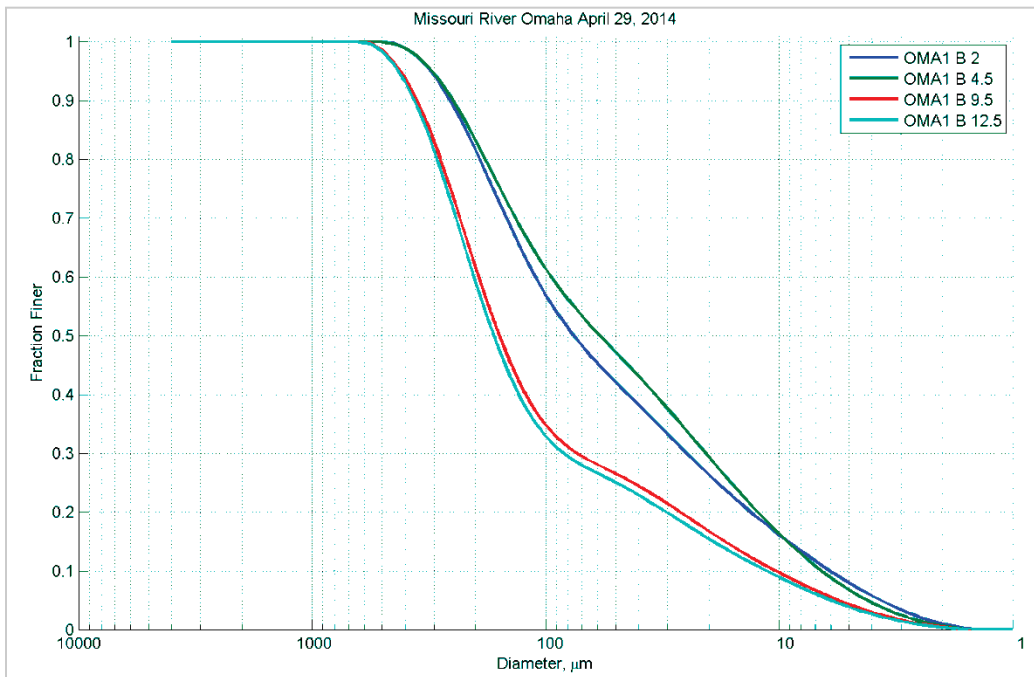
Figure 51. Particle size distribution at different depths (feet) in Station B – April 29, 2014.
