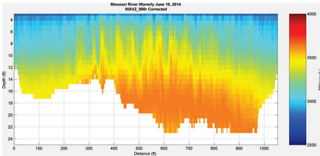
Figure 217. Suspended sediment concentration profile at Waverly, MO – June 10, 2014.
