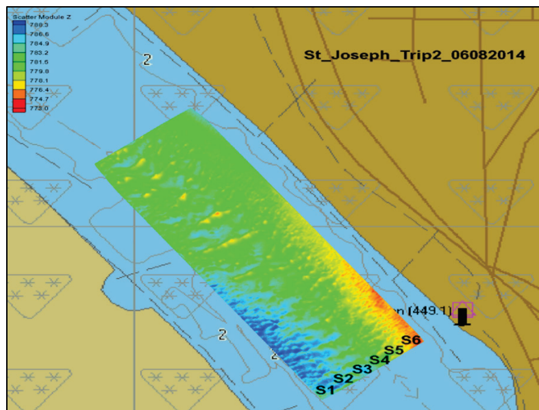
Figure 146. Bathymetry for Missouri River at St. Joseph showing swath locations.
