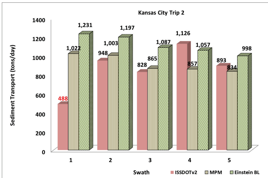
Figure 185. Bed-load transport at Kansas City, MO – June 9, 2014: ISSDOTv2 values compared to transport function computed values, where red indicates an interpolated value.
