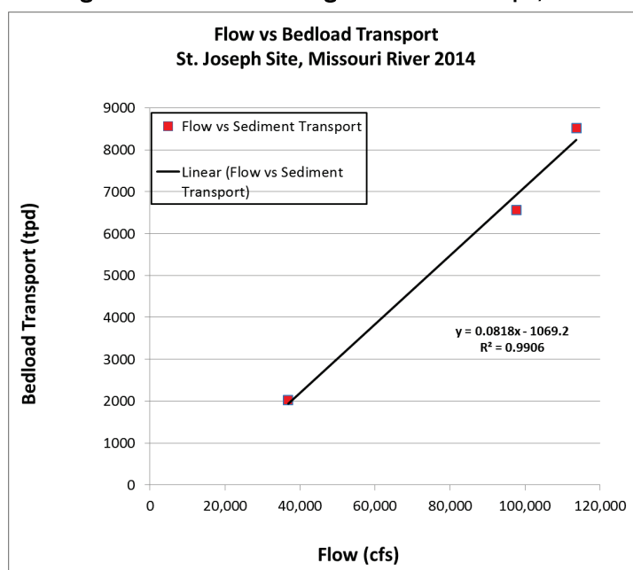
Figure 145. Bed-load rating curve for St. Joseph, MO.
