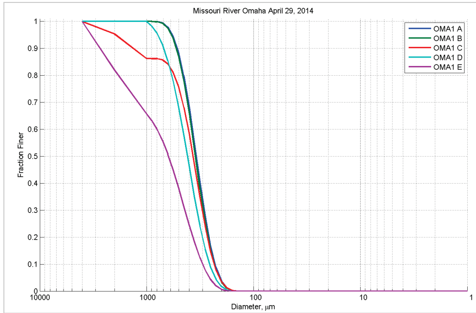
Figure 47. Bed material grain size distribution for Omaha, NE – April 29, 2014.
