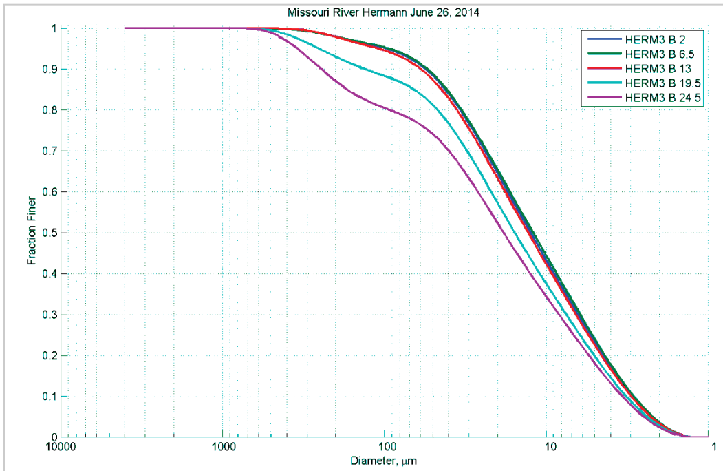
Figure 246. Particle size distribution at different depths (feet) in Station B – June 26, 2014.
