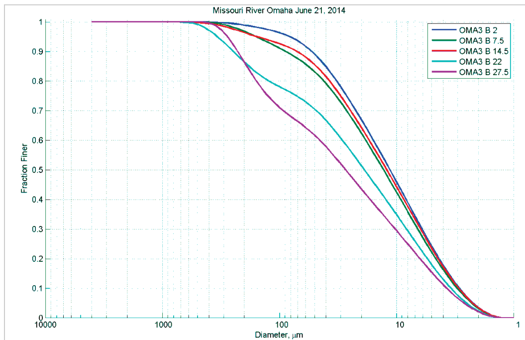
Figure 61. Particle size distribution at different depths (feet) in Station B – June 21, 2014.
