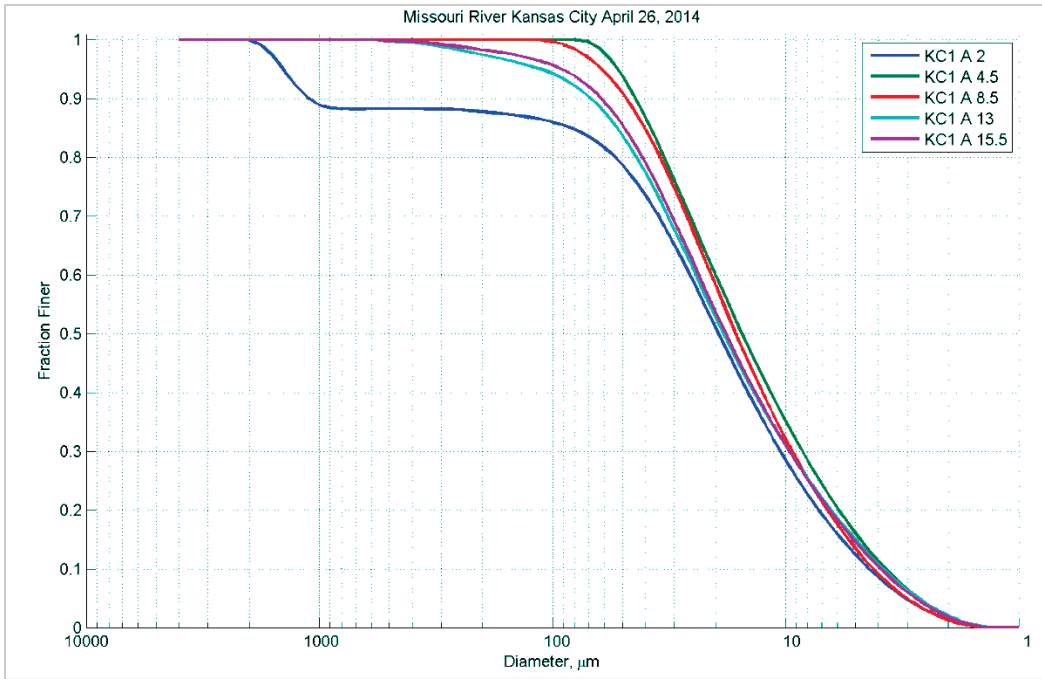
Figure 161. Particle size distribution at different depths (feet) in Station A - April 26, 2014.
