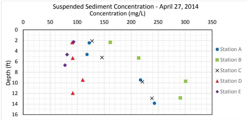
Figure 139. Suspended sediment concentration at St. Joseph, MO – April 27, 2014.
