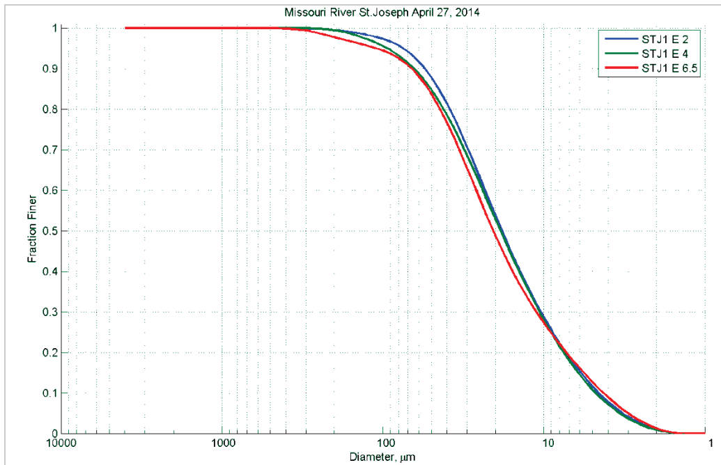
Figure 128. Particle size distribution at different depths (feet) in Station E - April 27, 2014.
