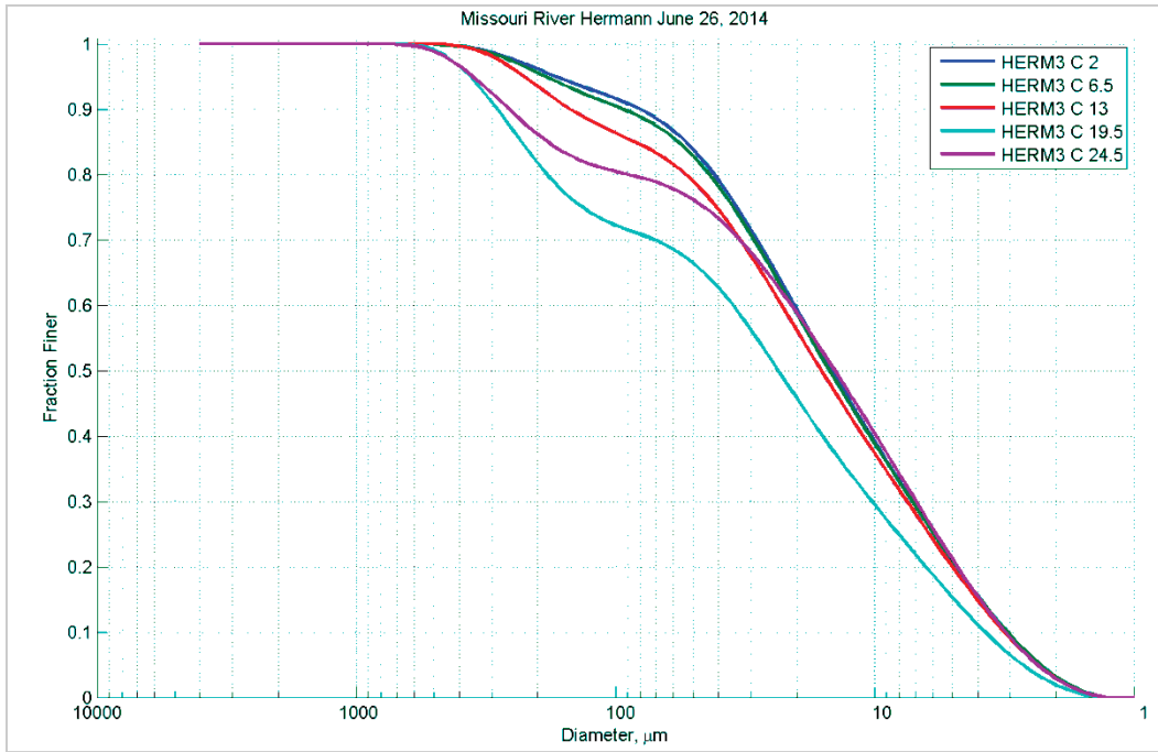
Figure 247. Particle size distribution at different depths (feet) in Station C – June 26, 2014.
