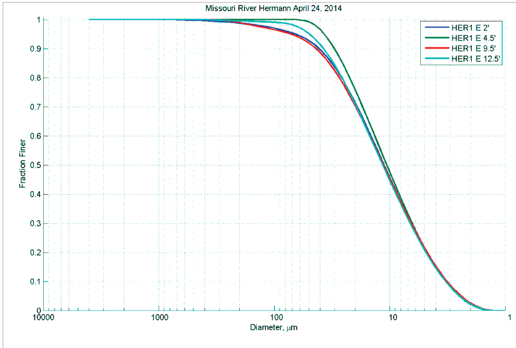
Figure 239. Particle size distribution at different depths (feet) in Station E - April 24, 2014.
