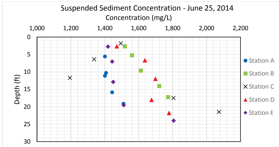
Figure 215. Suspended sediment concentration at Waverly, MO – June 25, 2014.
