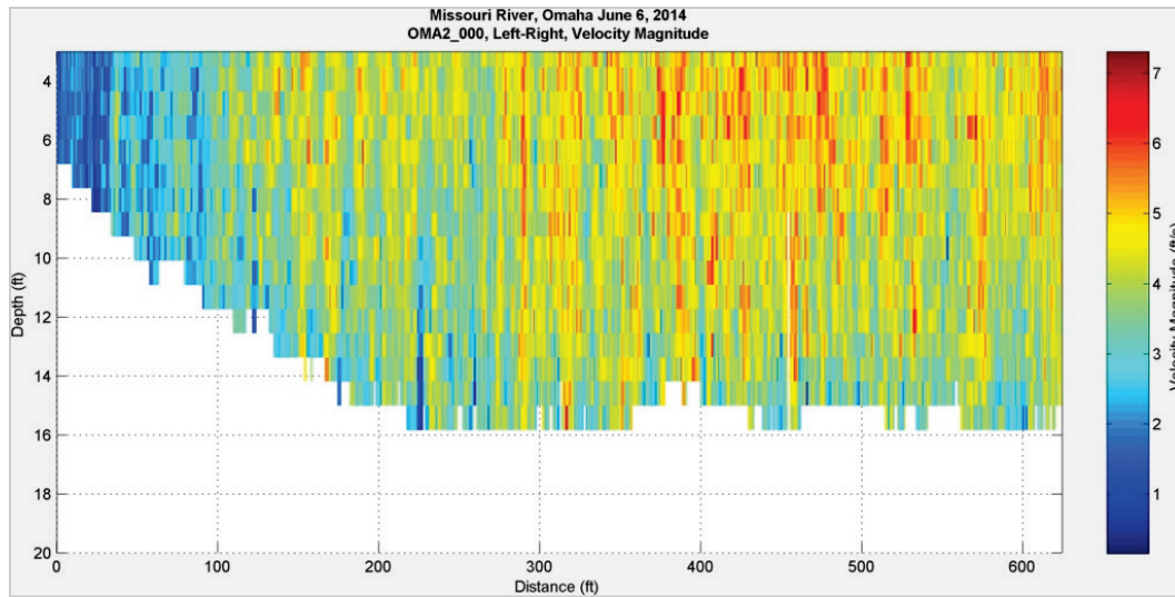
Figure 41. Velocity magnitude at Omaha, NE – June 6, 2014, 14:41:44.
