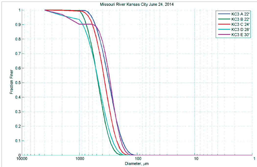
Figure 160. Bed material grain size distribution for Kansas City, MO – June 24, 2014.
