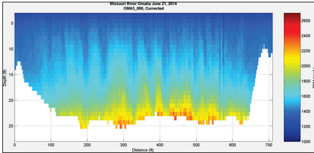
Figure 70. Suspended sediment concentration Profile at Omaha, NE – June 21, 2014.
