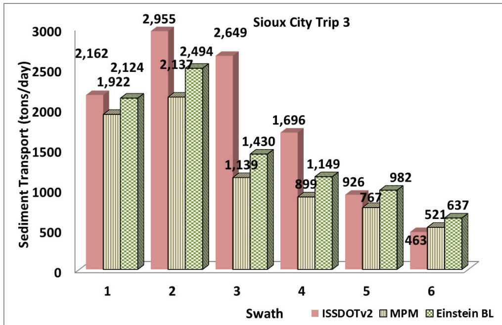
Figure 38. Bed-load transport at Sioux City, IA – June 20, 2014: ISSDOTv2 values compared to transport function computed values.
