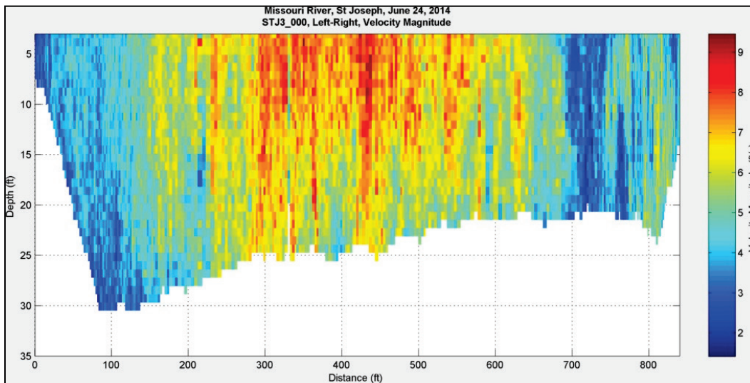
Figure 116. Velocity magnitude at St. Joseph, MO – June 24, 2014, 13:32:30.
