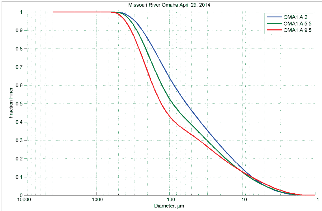
Figure 50. Particle size distribution at different depths (feet) in Station A – April 29, 2014.
