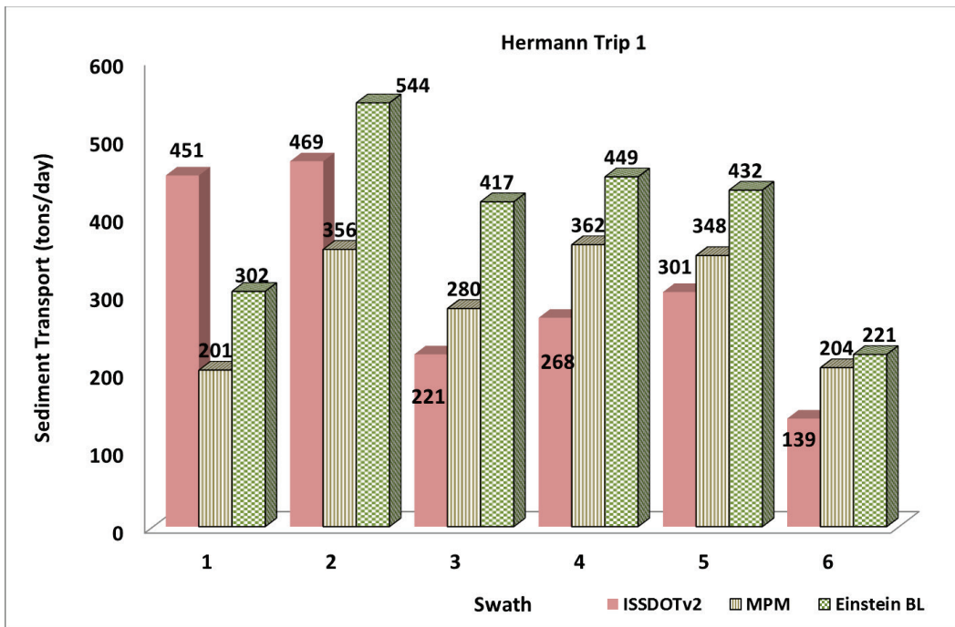
Figure 258. Bed-load transport at Hermann, MO – April 24, 2014: ISSDOTv2 values compared to transport function computed values.
