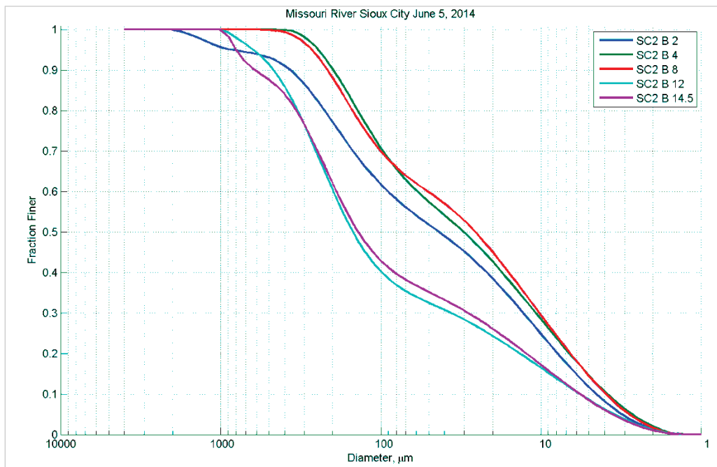
Figure 19. Particle size distribution at different depths (feet) in Station B – June 5, 2014.
