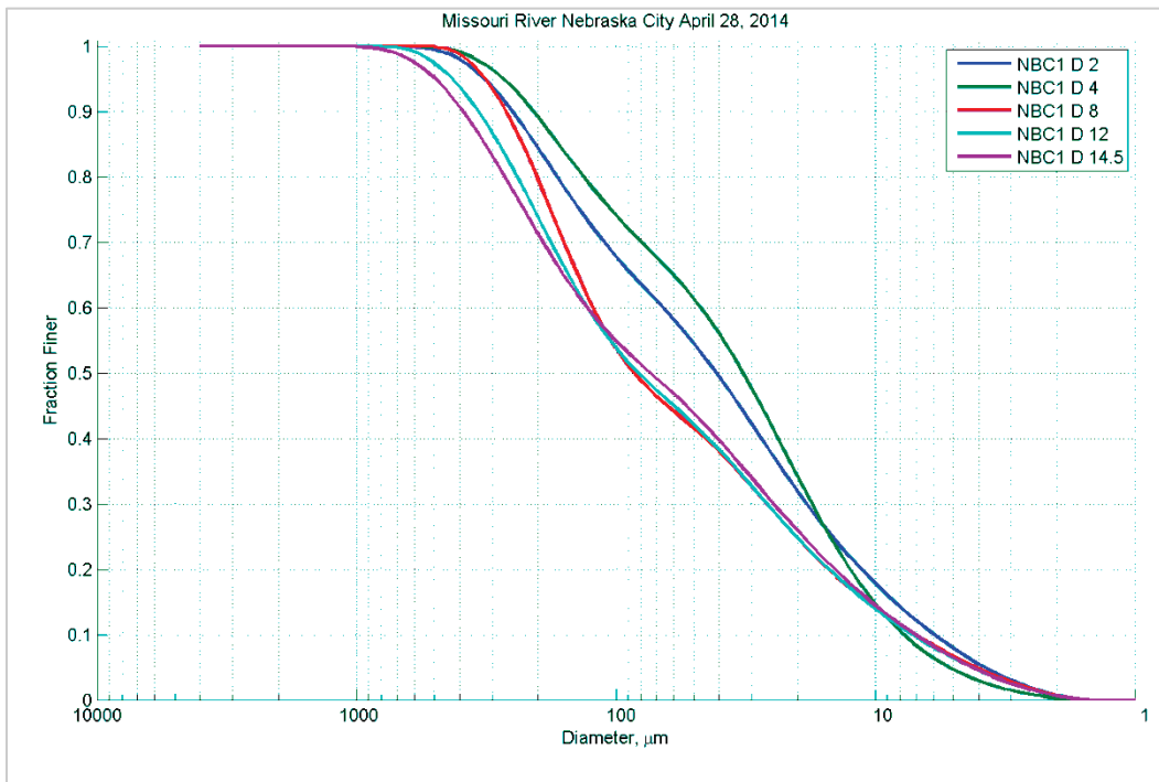
Figure 90. Particle size distribution at different depths (feet) in Station D - April 28, 2014.
