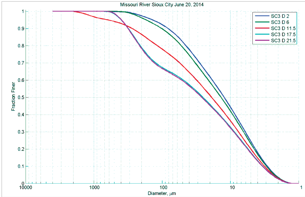
Figure 26. Particle size distribution at different depths (feet) in Station D – June 20, 2014.
