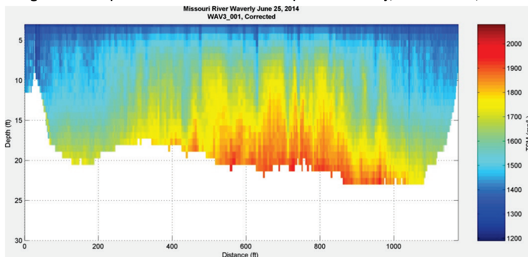
Figure 218. Suspended sediment concentration profile at Waverly, MO – June 25, 2014.
