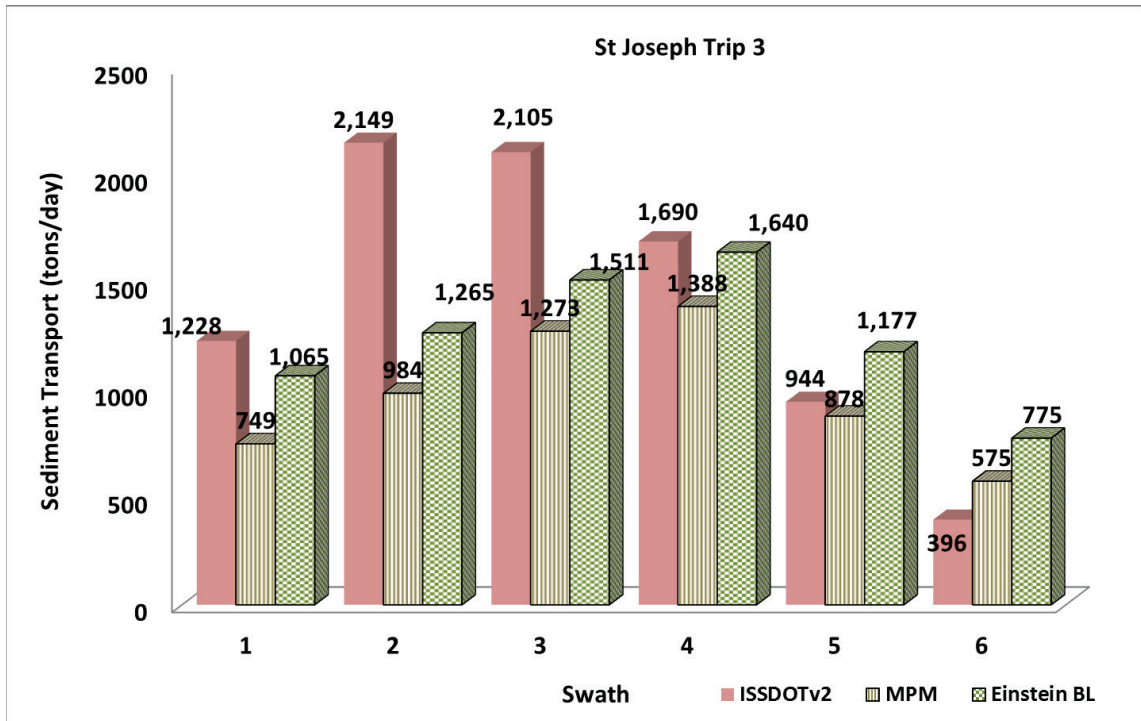
Figure 149. Bed-load transport at St. Joseph, MO – June 24, 2014: ISSDOTv2 values compared to transport function computed values.
