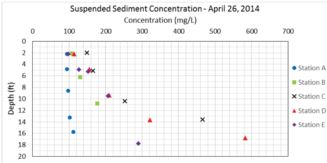
Figure 176. Suspended sediment concentration at Kansas City, MO – April 26, 2014.
