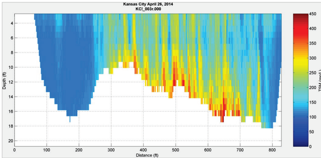
Figure 179. Suspended sediment concentration profile at Kansas City, MO – April 26, 2014.
