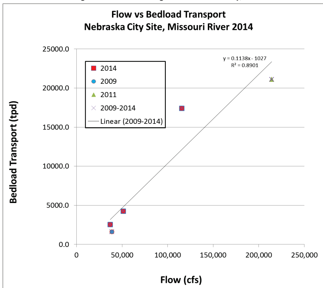
Figure 108. Bed-load rating curve for Nebraska City, NE.
