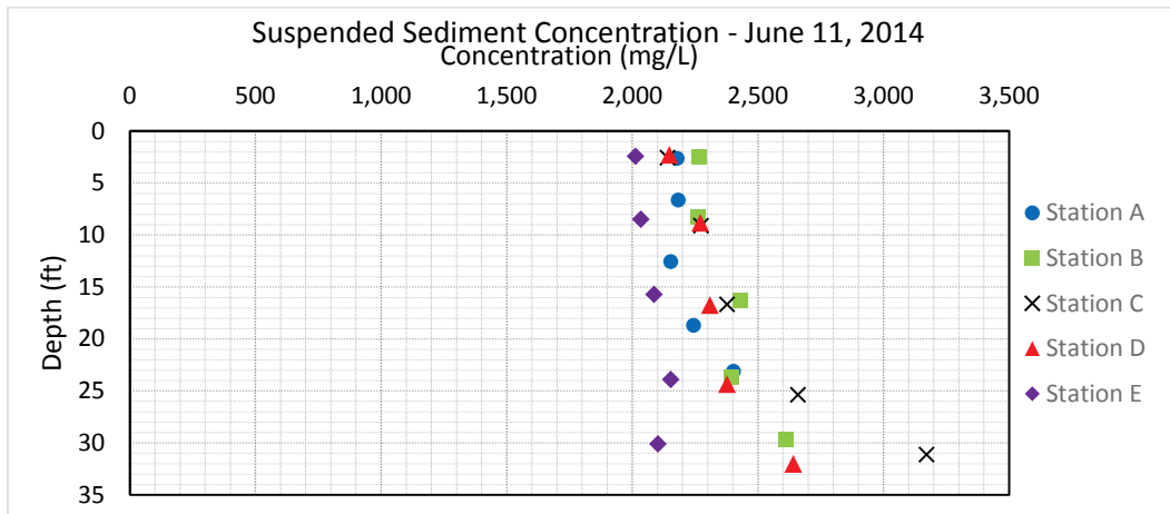
Figure 251. Suspended sediment concentration at Hermann, MO – June 11, 2014.
