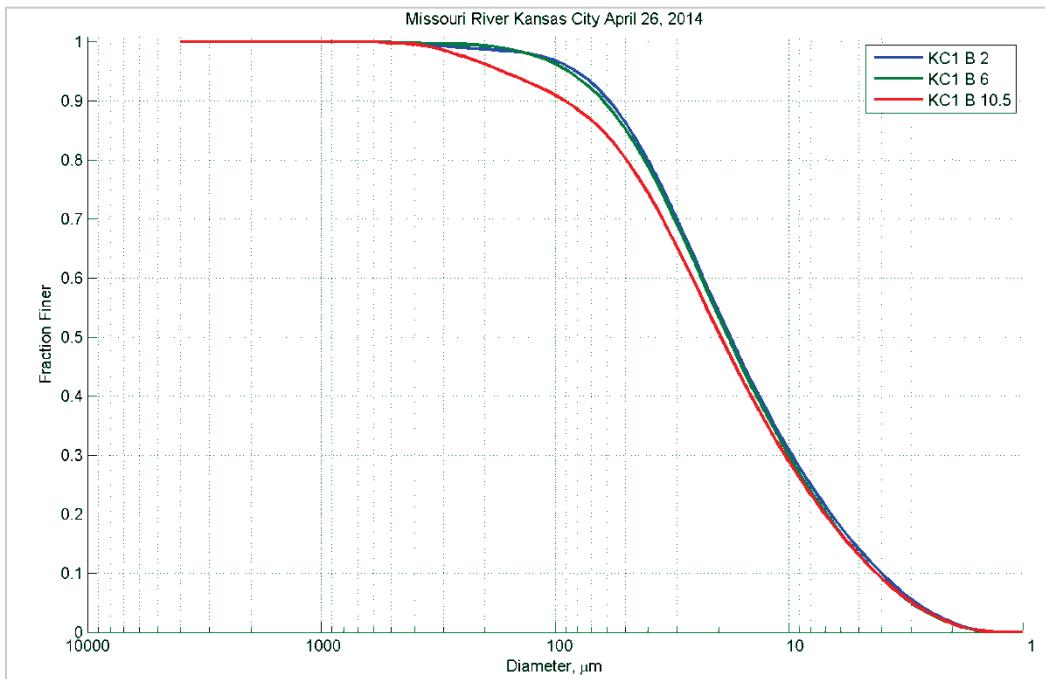
Figure 162. Particle size distribution at different depths (feet) in Station B - April 26, 2014.
