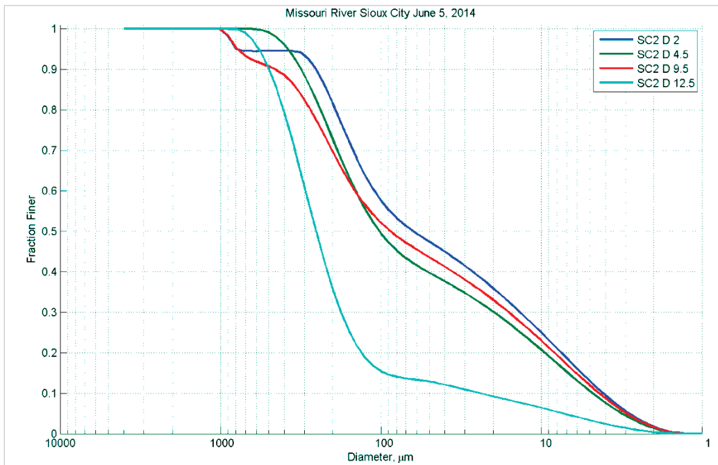
Figure 21. Particle size distribution at different depths (feet) in Station D – June 5, 2014.
