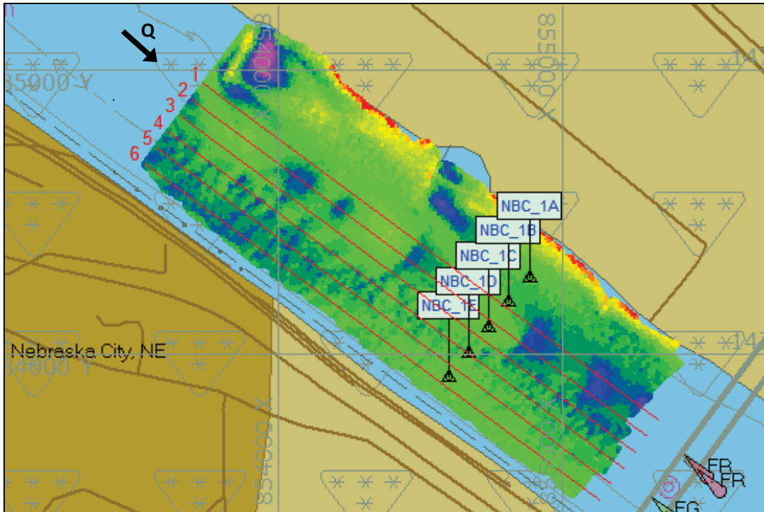
Figure 81. Multi-beam survey extent at Nebraska City, NE - April 28, 2014.
