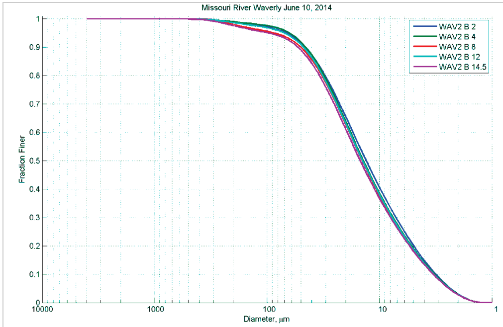
Figure 204. Particle size distribution at different depths (feet) in Station B – June 10, 2014.
