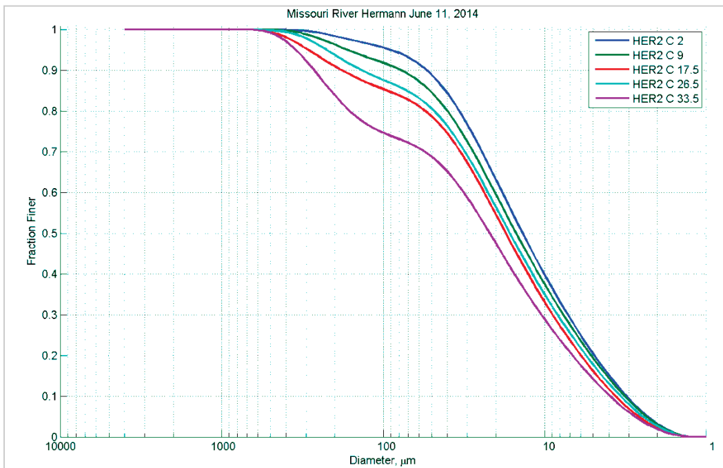
Figure 242. Particle size distribution at different depths (feet) in Station C – June 11, 2014.
