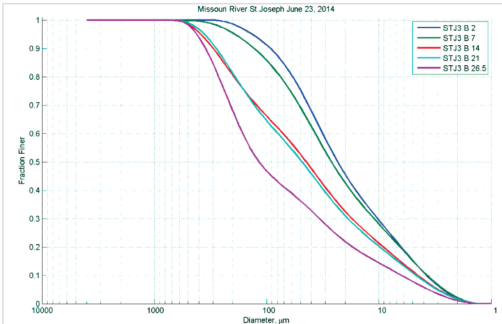
Figure 135. Particle size distribution at different depths (feet) in Station B – June 24, 2014.
