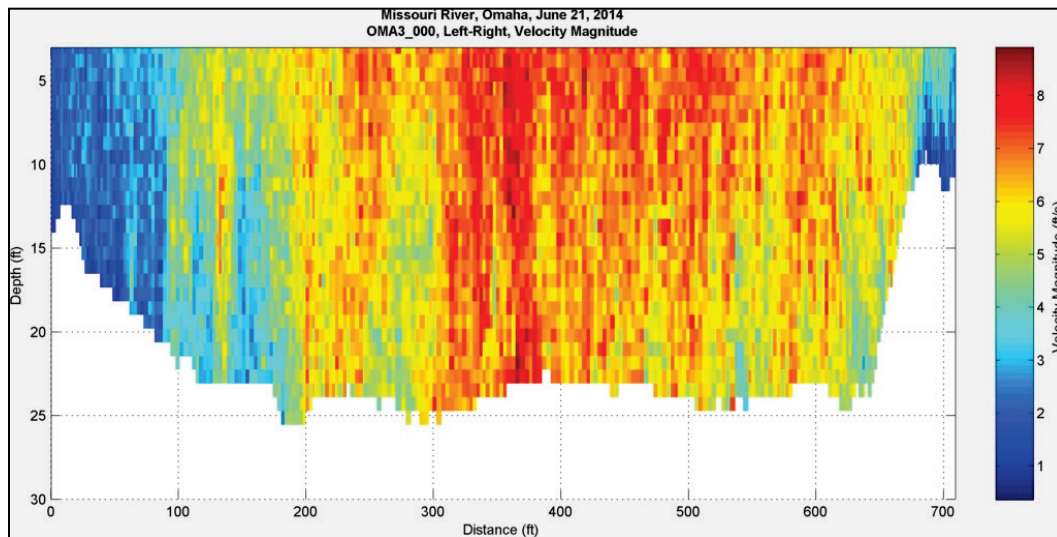
Figure 42. Velocity magnitude at Omaha, NE – June 21, 2014, 14:48:48.
