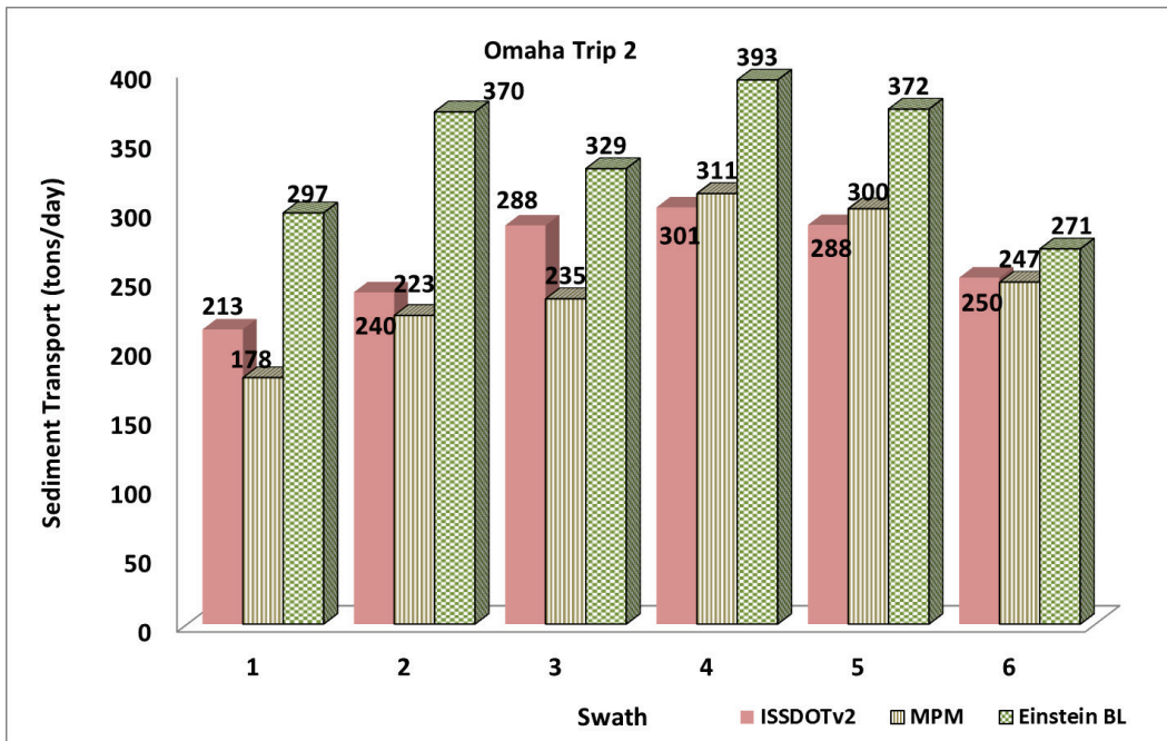
Figure 74. Bed-load transport at Omaha, NE – June 6, 2014: ISSDOTv2 values compared to transport function computed values.
