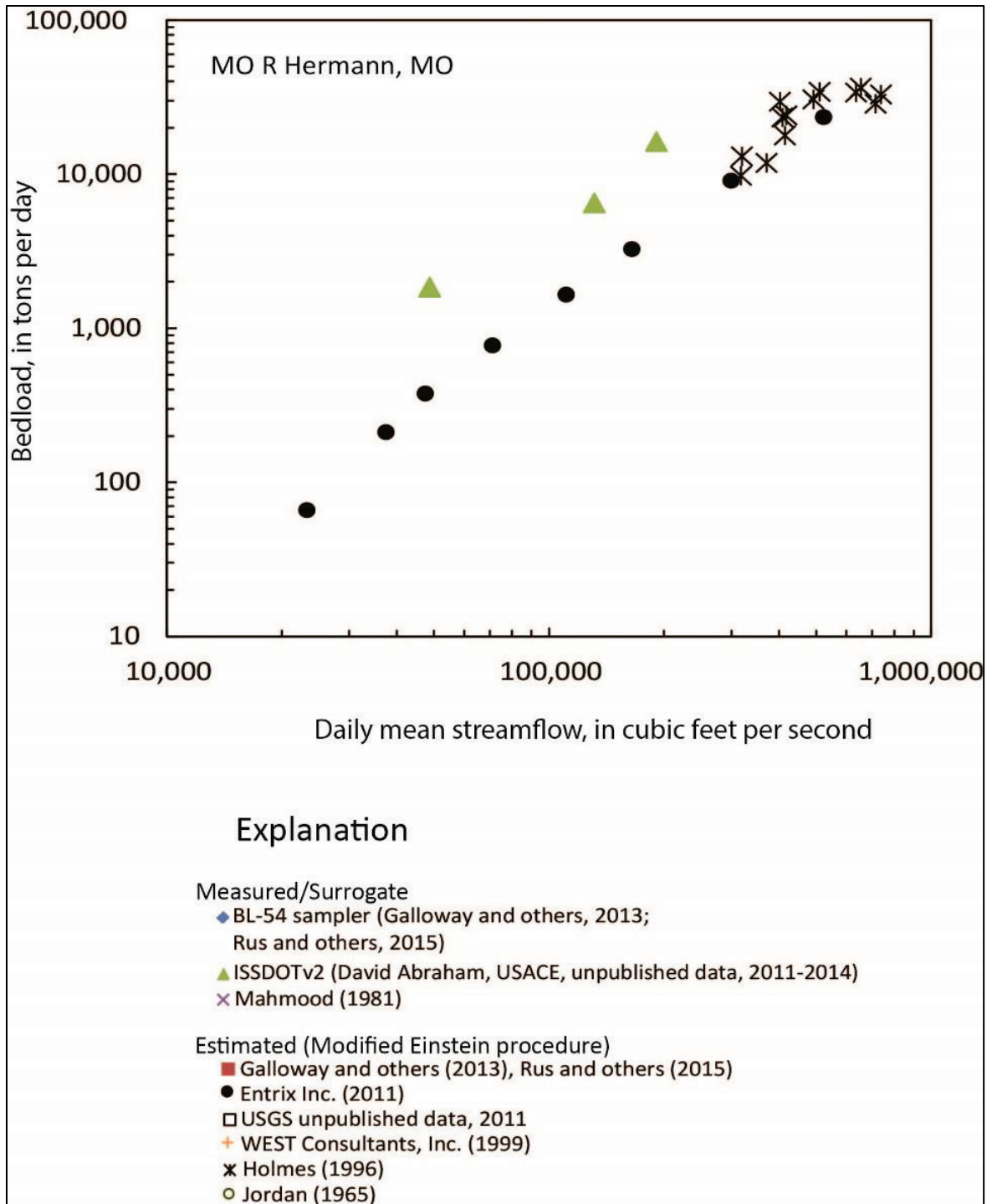
Figure 267. USGS bed-load data – Hermann, MO.
