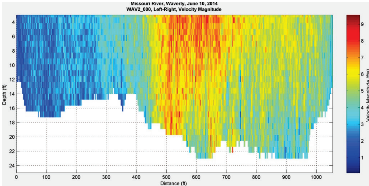
Figure 189. Velocity magnitude at Waverly, MO – June 10, 2014, 16:44:16.
