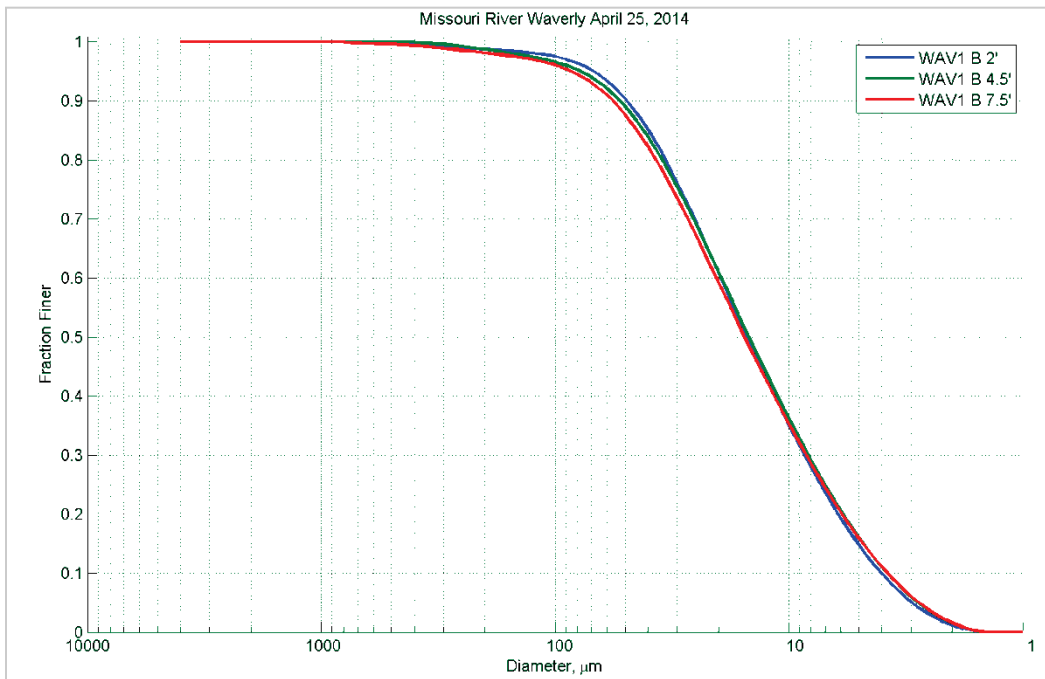
Figure 199. Particle size distribution at different depths (feet) in Station B - April 25, 2014.
