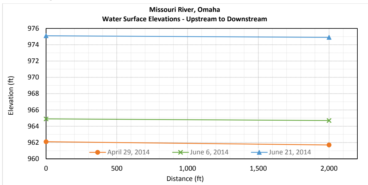
Figure 43. Water surface elevation at Omaha, NE – from upstream to downstream.
