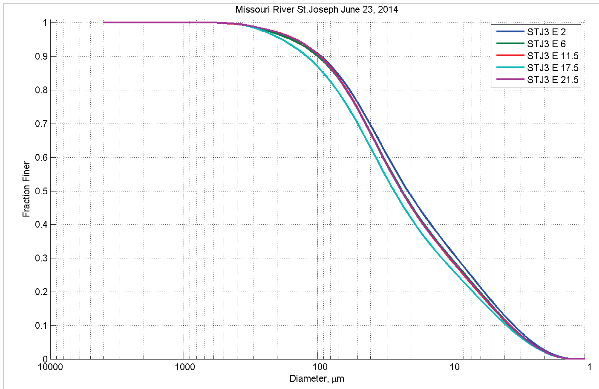
Figure 138. Particle size distribution at different depths (feet) in Station E – June 24, 2014.
