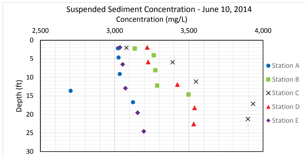
Figure 214. Suspended Sediment concentration at Waverly, MO – June 10, 2014.
