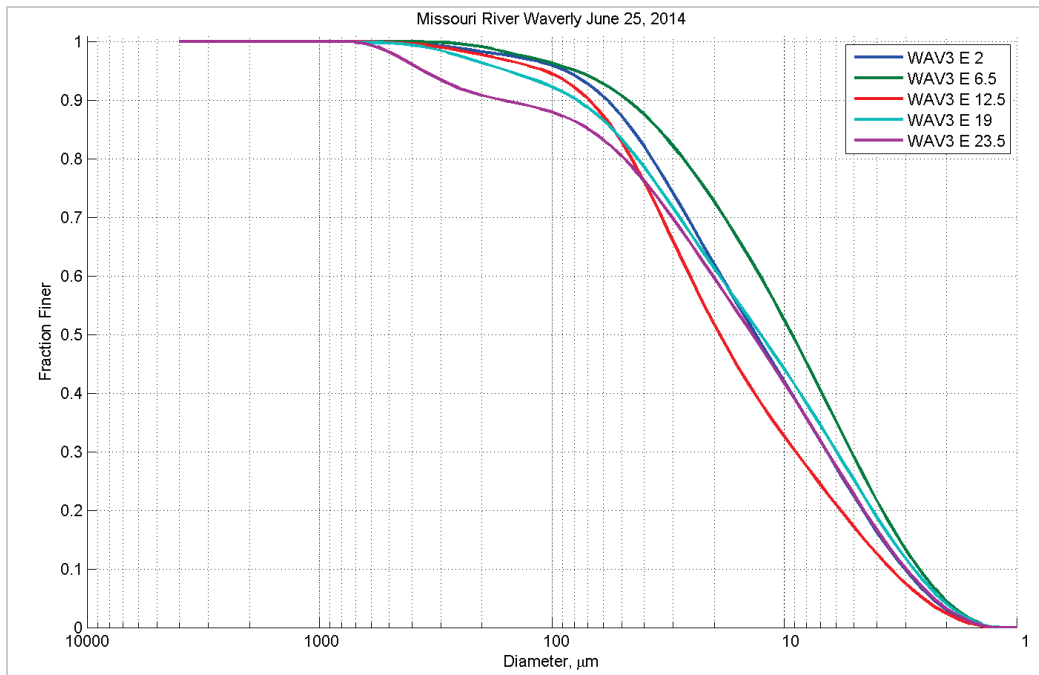
Figure 212. Particle size distribution at different depths (feet) in Station E – June 25, 2014.
