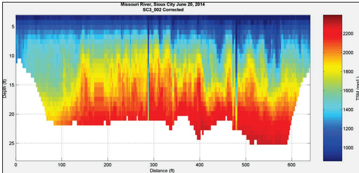
Figure 33. Suspended sediment concentration profile at Sioux City, IA – June 20, 2014.
