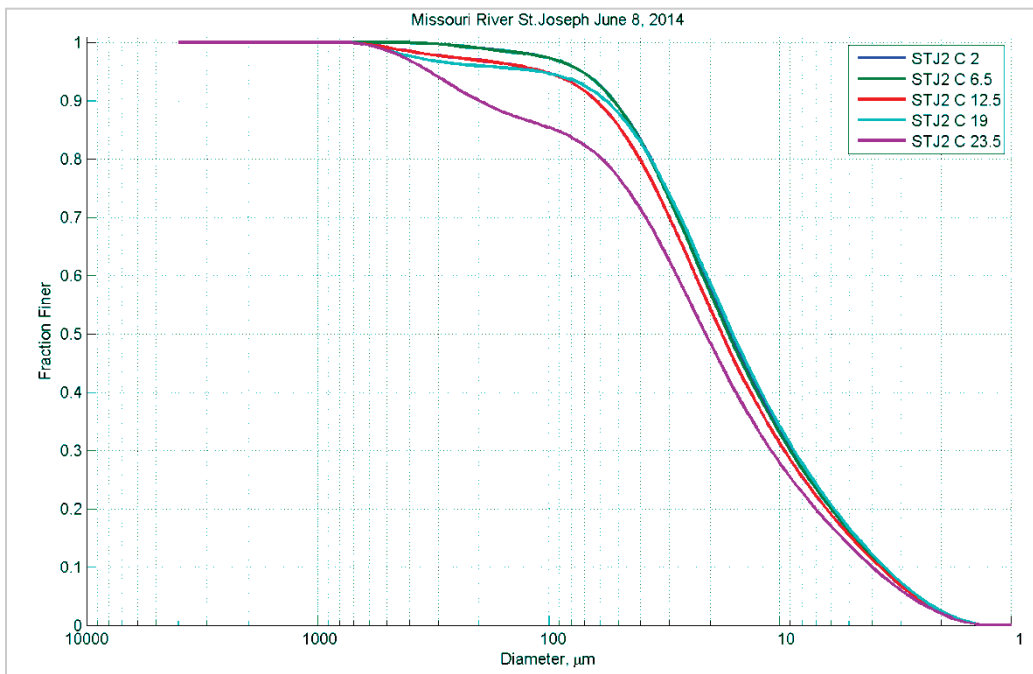
Figure 131. Particle size distribution at different depths (feet) in Station C – June 8, 2014.
