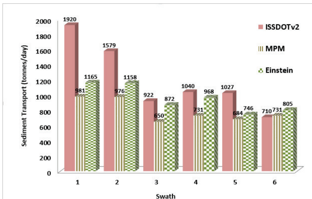
Figure 269. Measured and computed values of bed load transport. Site is Kansas City, trip 3.
