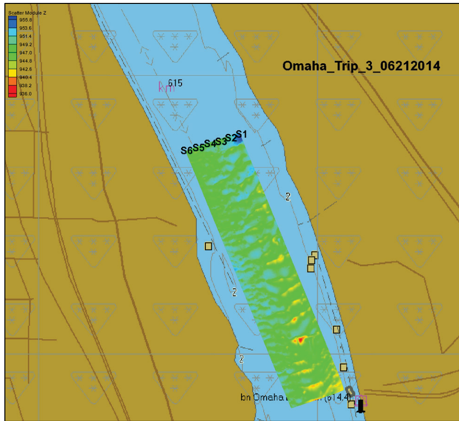
Figure 72. Bathymetry for Missouri River at Omaha showing swath locations.
