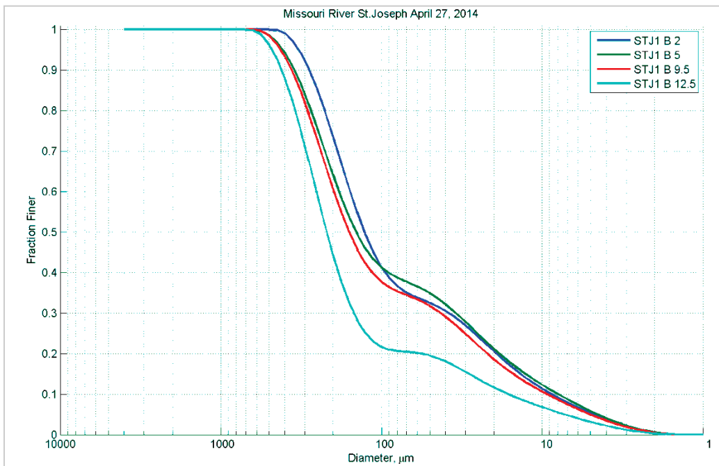
Figure 125. Particle size distribution at different depths (feet) in Station B - April 27, 2014.
