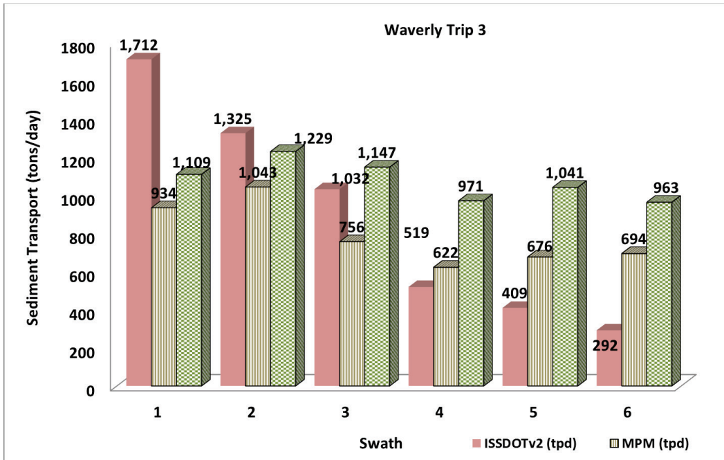
Figure 223. Bed-load transport at Waverly, MO – June 25, 2014: ISSDOTv2 values compared to transport function computed values.
