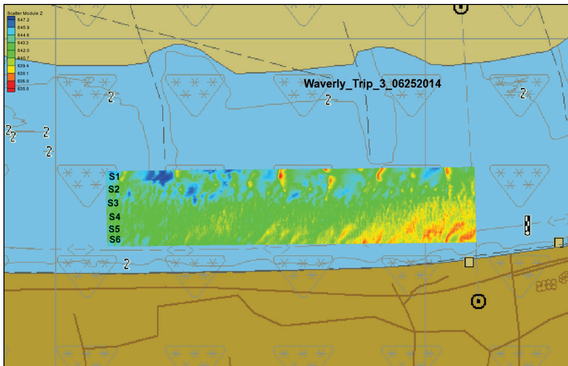
Figure 220. Bathymetry for Missouri River at Waverly, MO, showing swath locations.
