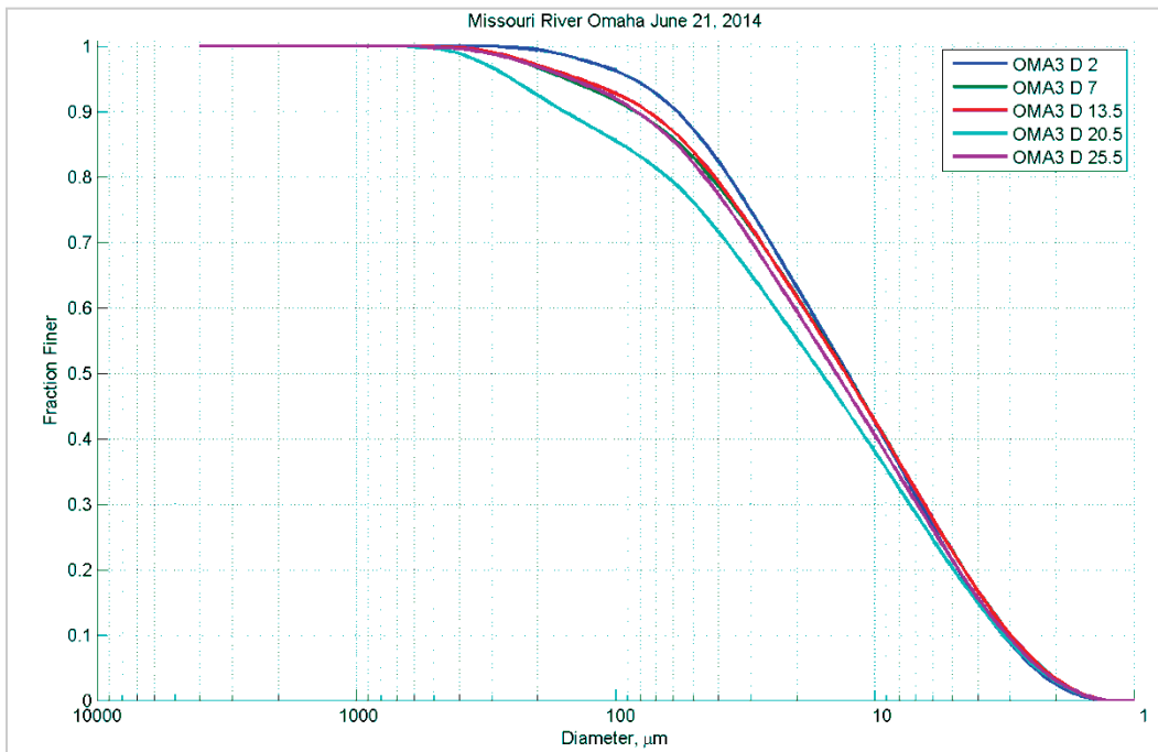
Figure 63. Particle size distribution at different depths (feet) in Station D – June 21, 2014.
