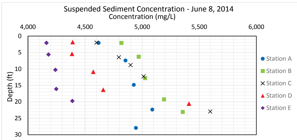
Figure 140. Suspended sediment concentration at St. Joseph, MO– June 8, 2014.
