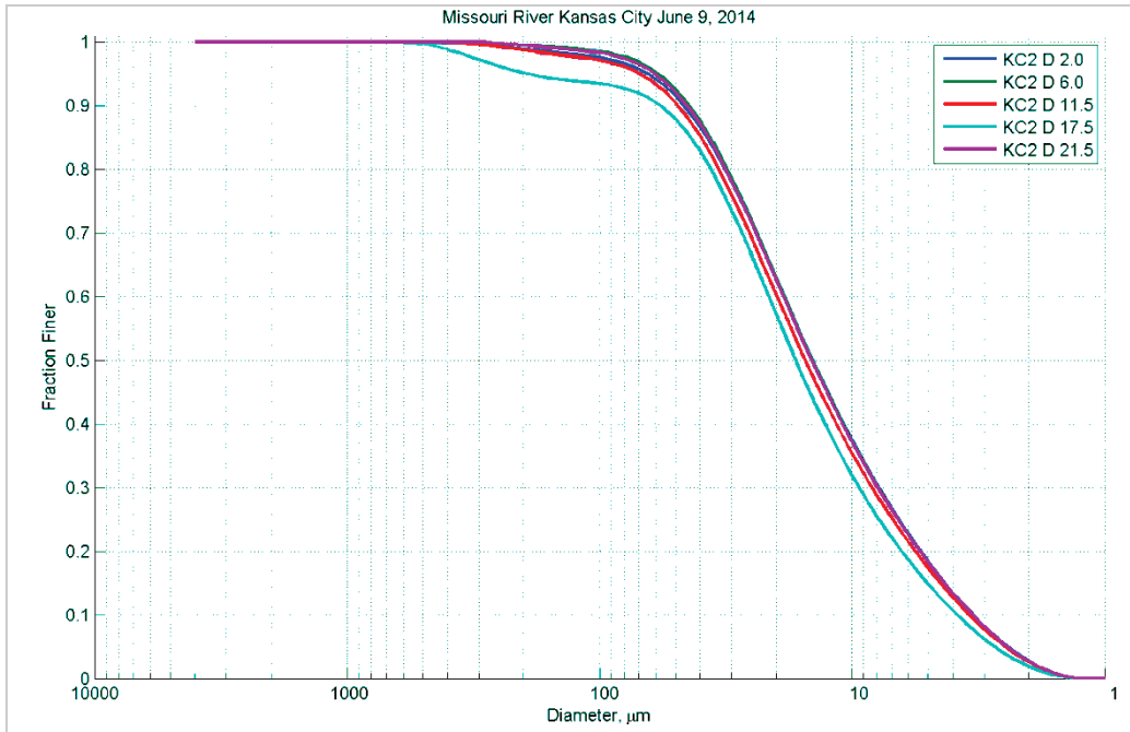
Figure 169. Particle size distribution at different depths (feet) in Station D – June 9, 2014.
