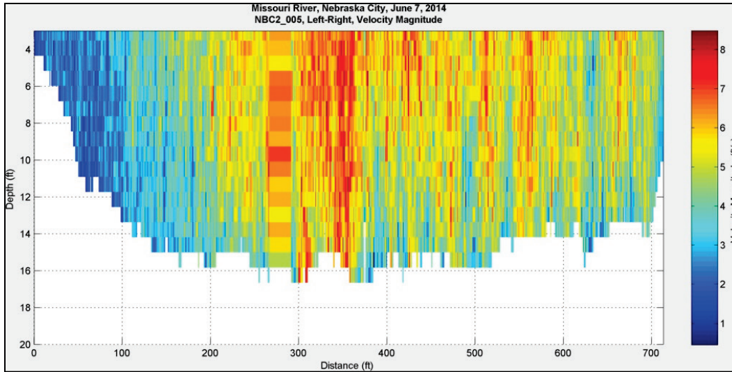
Figure 78. Velocity magnitude at Nebraska City, NE – June 7, 2014, 19:39:14.
