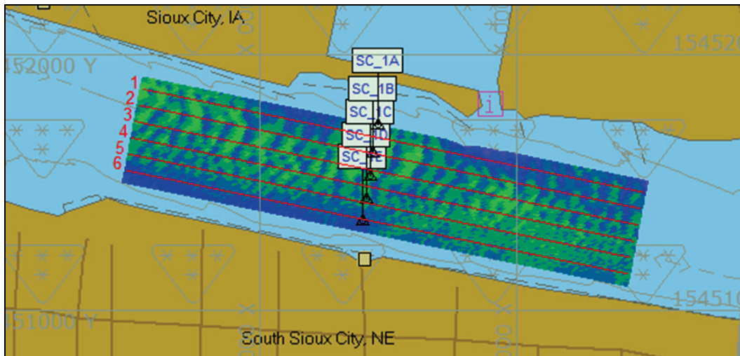
Figure 35. Bathymetry for Missouri River at Sioux City, showing swath locations.
