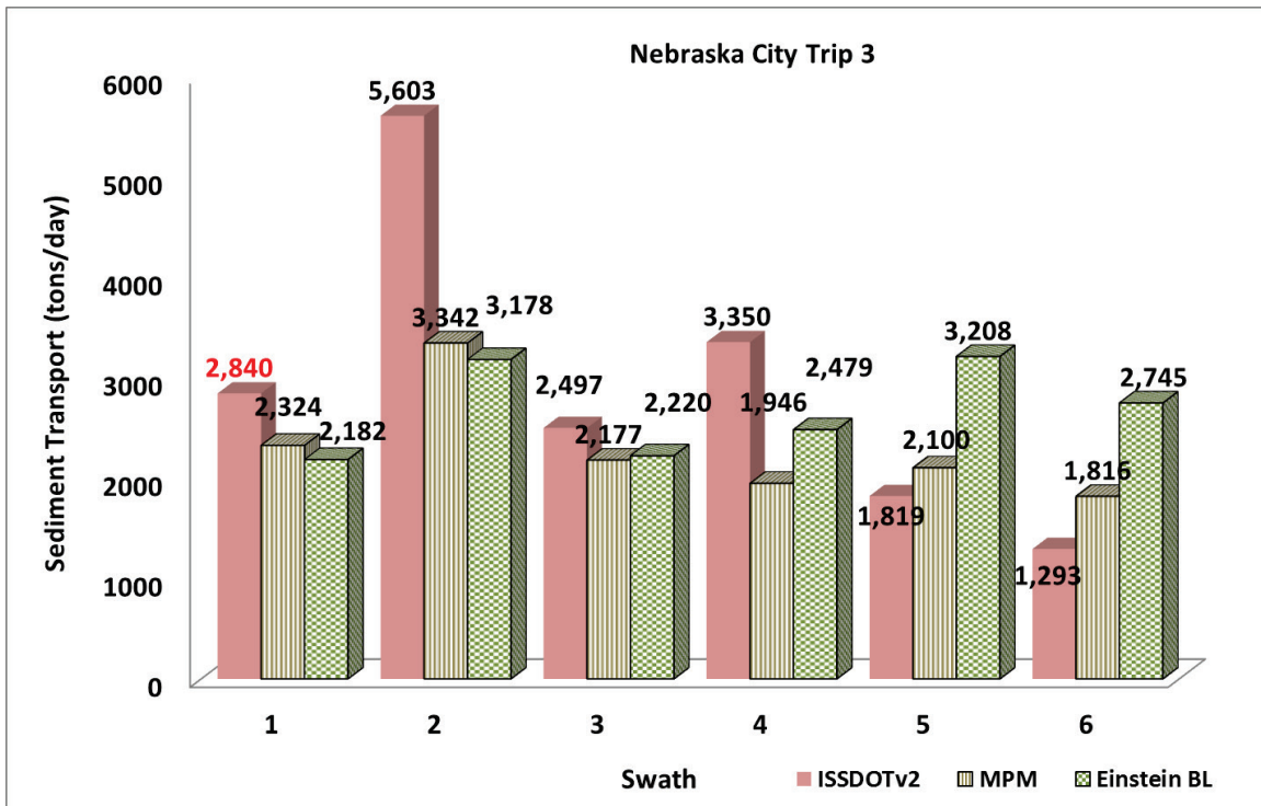
Figure 112. Bed-load transport at Nebraska City, NE- June 22, 2014: ISSDOTv2 values compared to transport function computed values, where red indicates an interpolated value.
