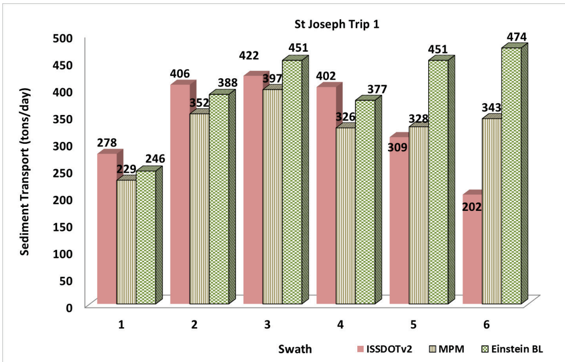
Figure 147. Bed-load transport at St. Joseph, MO – April 27, 2014: ISSDOTv2 values compared to transport function computed values.
