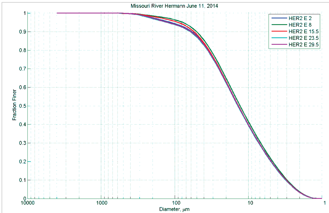
Figure 244. Particle size distribution at different depths (feet) in Station E – June 11, 2014.
