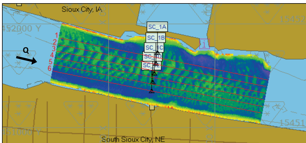
Figure 7. Multi-beam survey extent at Sioux City, IA – April 30, 2014.
