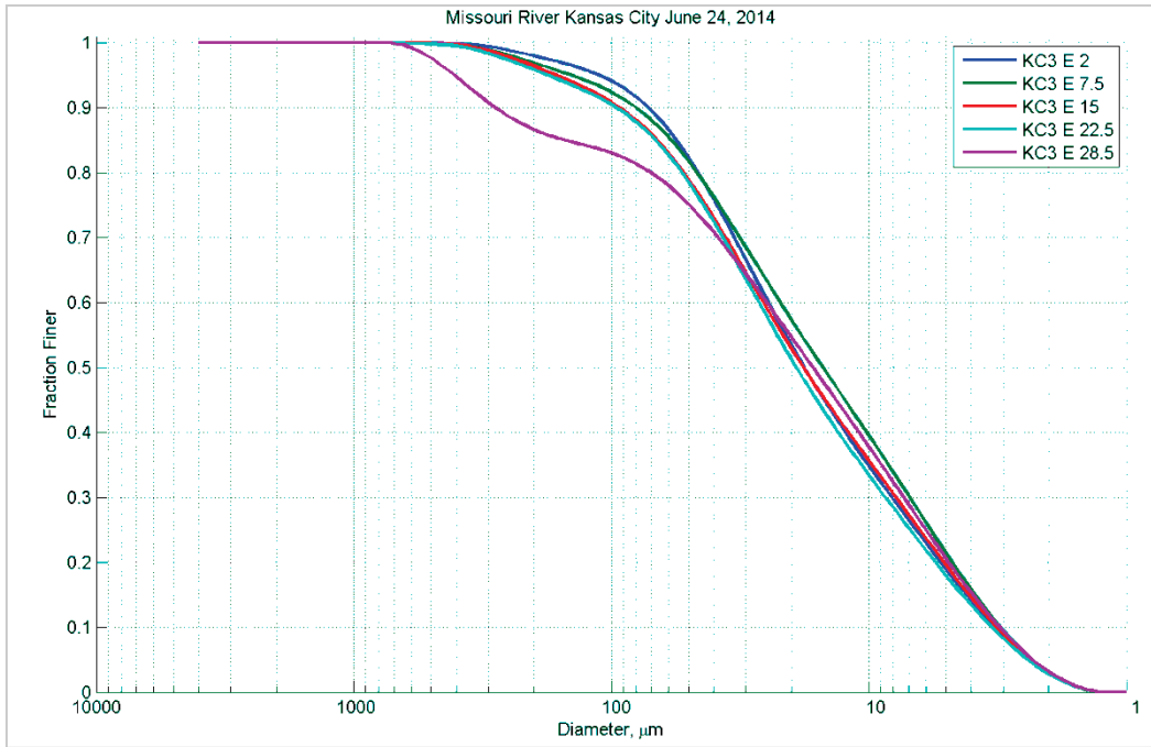
Figure 175. Particle size distribution at different depths (feet) in Station E – June 24, 2014.
