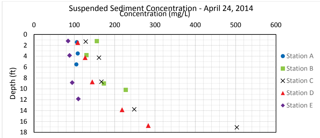
Figure 250. Suspended sediment concentration at Hermann, MO – April 24, 2014.
