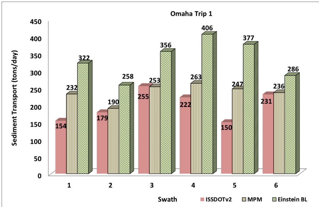
Figure 73. Bed-load transport at Omaha, NE – April 29, 2014: ISSDOTv2 values compared to transport function computed values.
