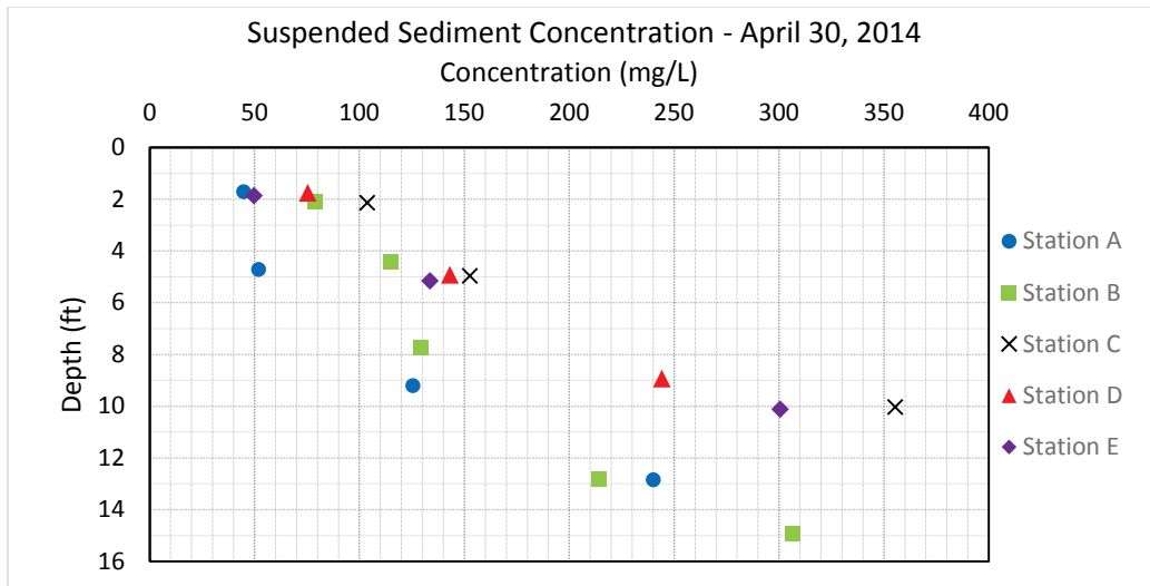
Figure 28. Suspended sediment concentration at Sioux City, IA – April 30, 2014.
