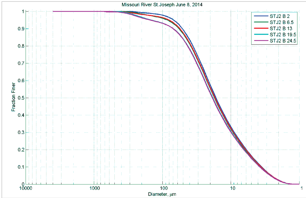
Figure 130. Particle size distribution at different depths (feet) in Station B – June 8, 2014.
