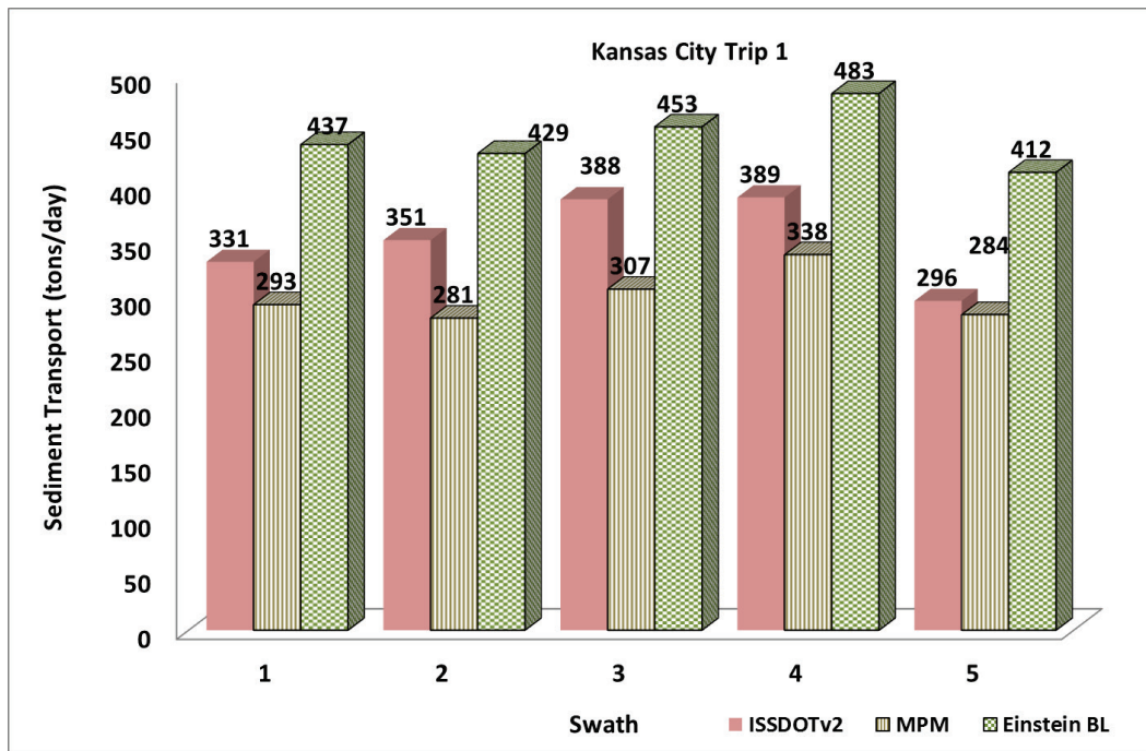
Figure 184. Bed-load transport at Kansas City, MO – April 26, 2014: ISSDOTv2 values compared to transport function computed values.
