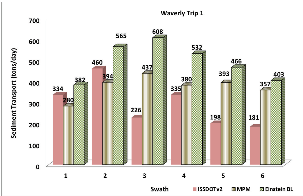
Figure 221. Bed-load transport at Waverly, MO – April 25, 2014: ISSDOTv2 values compared to transport function computed values.
