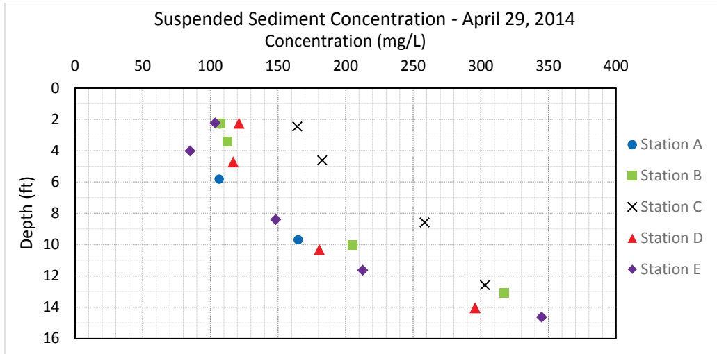
Figure 65. Suspended sediment concentration at Omaha, NE – April 29, 2014.
