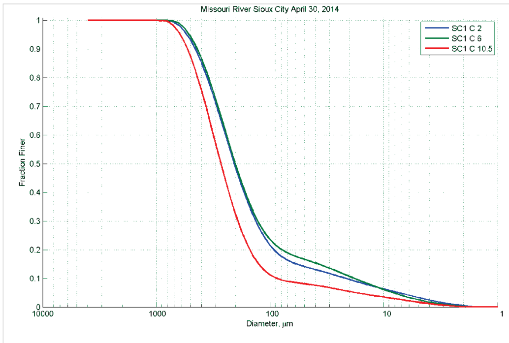
Figure 15. Particle size distribution at different depths (feet) in Station C – April 30, 2014.
