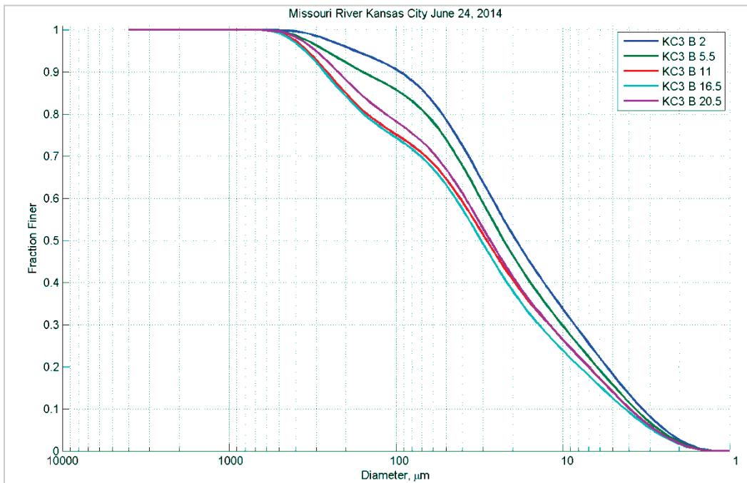
Figure 172. Particle size distribution at different depths (feet) in Station B – June 24, 2014.
