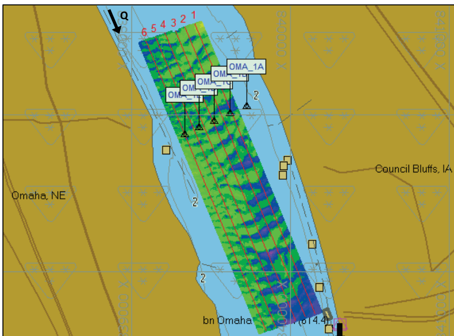
Figure 45. Multi-beam survey extent at Omaha, NE – June 6 and June 21, 2014.
