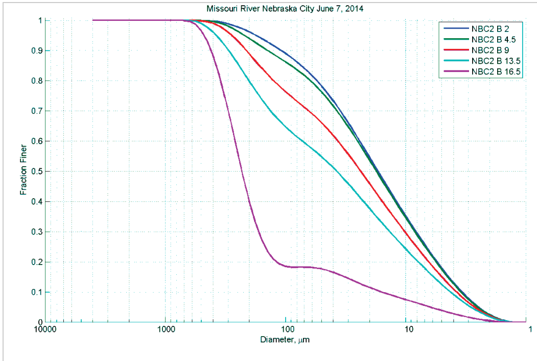
Figure 93. Particle size distribution at different depths (feet) in Station B – June 7, 2014.
