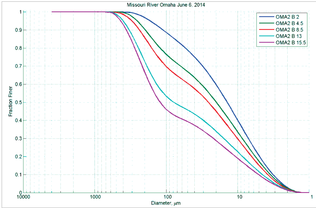
Figure 56. Particle size distribution at different depths (feet) in Station B – June 6, 2014.
