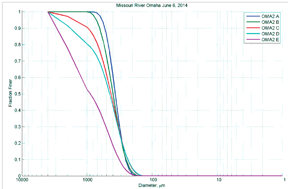
Figure 48. Bed material grain size distribution for Omaha, NE – June 6, 2014.
