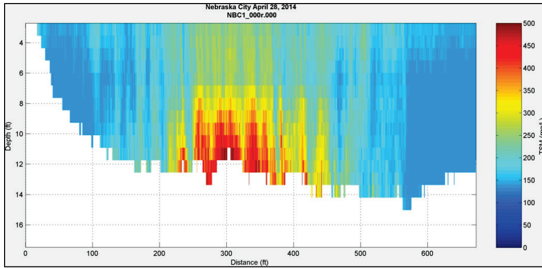
Figure 105. Suspended sediment concentration profile at Nebraska City, NE - April 28, 2014.
