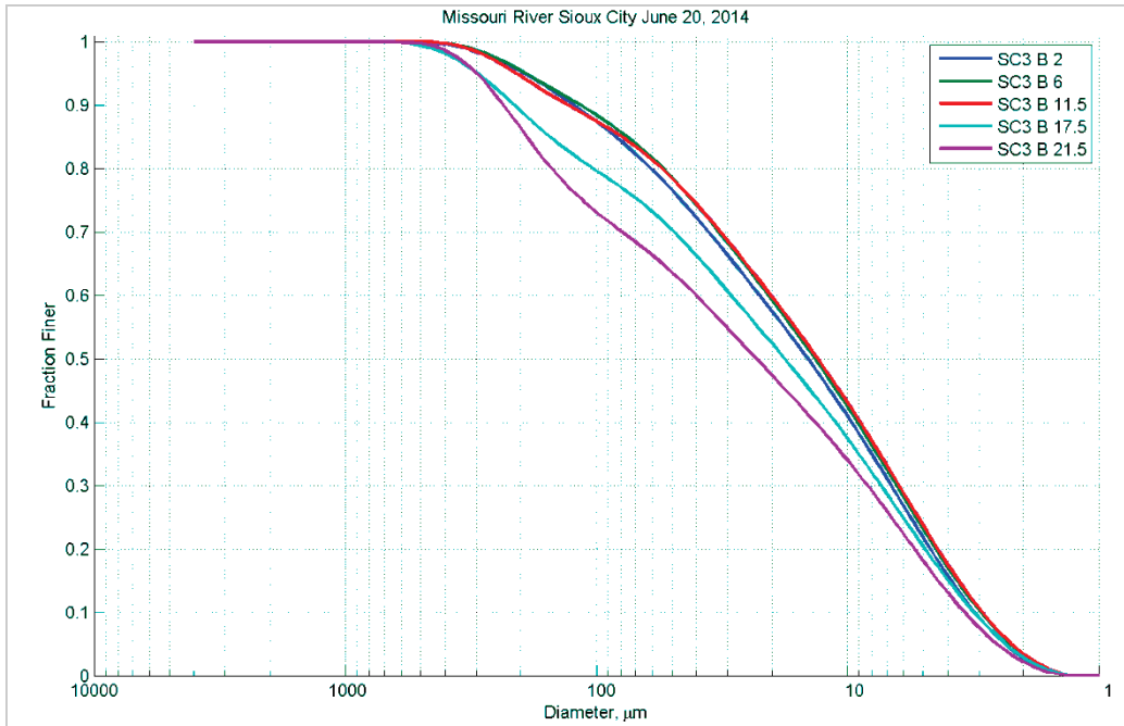
Figure 24. Particle size distribution at different depths (feet) in Station B – June 20, 2014.
