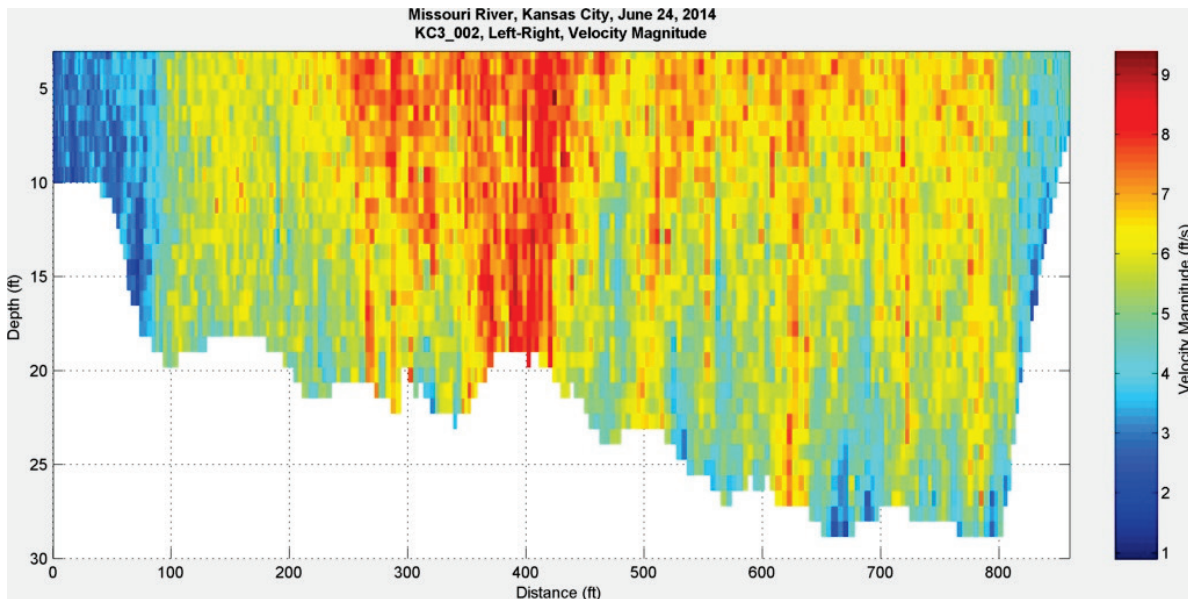
Figure 153. Velocity magnitude at Kansas City, MO – June 24, 2014, 18:38:11.
