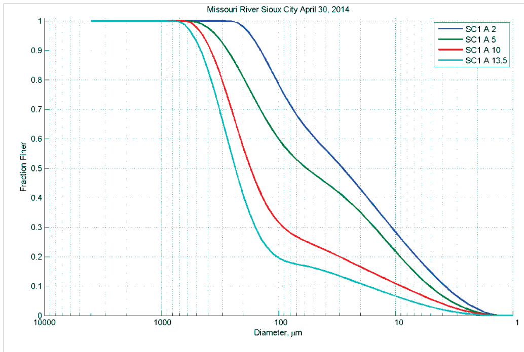
Figure 13. Particle size distribution at different depths (feet) in Station A – April 30, 2014.
