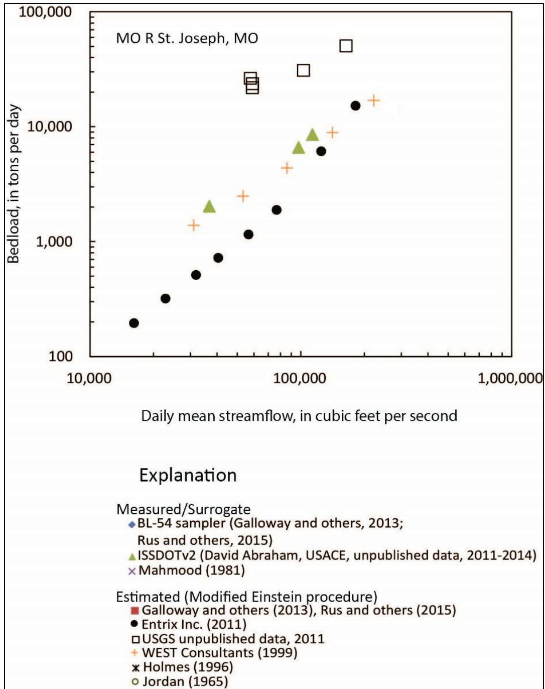
Figure 265. USGS bed-load data - St. Joseph, MO.
