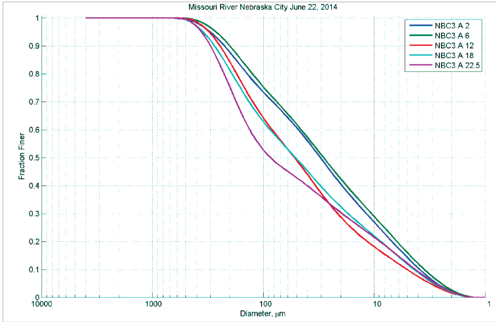
Figure 97. Particle size distribution at different depths (feet) in Station A – June 22, 2014.
