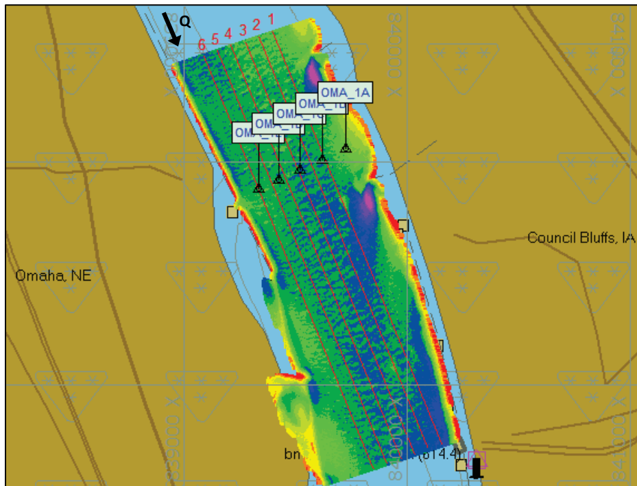
Figure 44. Multi-beam survey extent at Omaha, NE – April 29, 2014.
