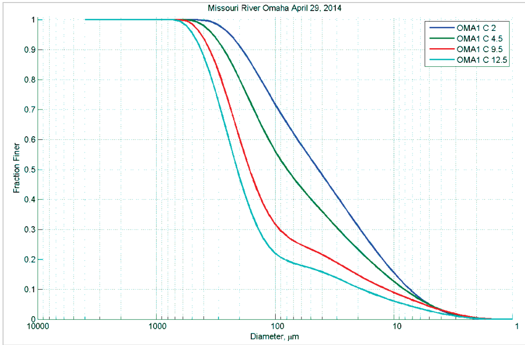
Figure 52. Particle size distribution at different depths (feet) in Station C – April 29, 2014.
