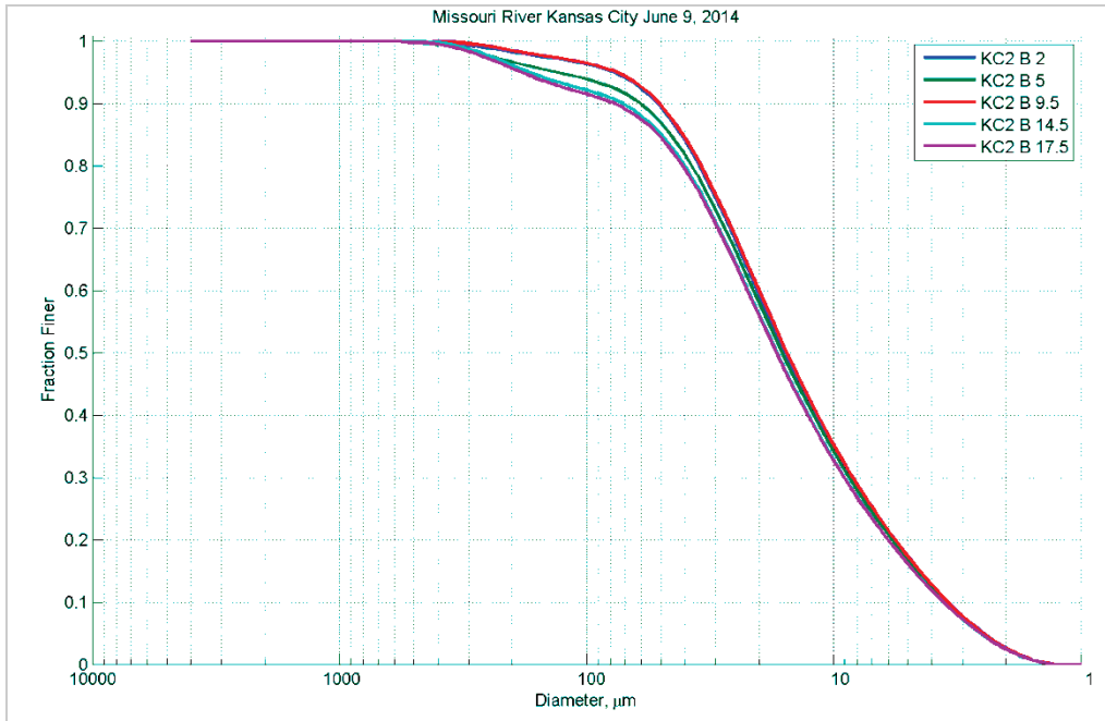
Figure 167. Particle size distribution at different depths (feet) in Station B – June 9, 2014.
