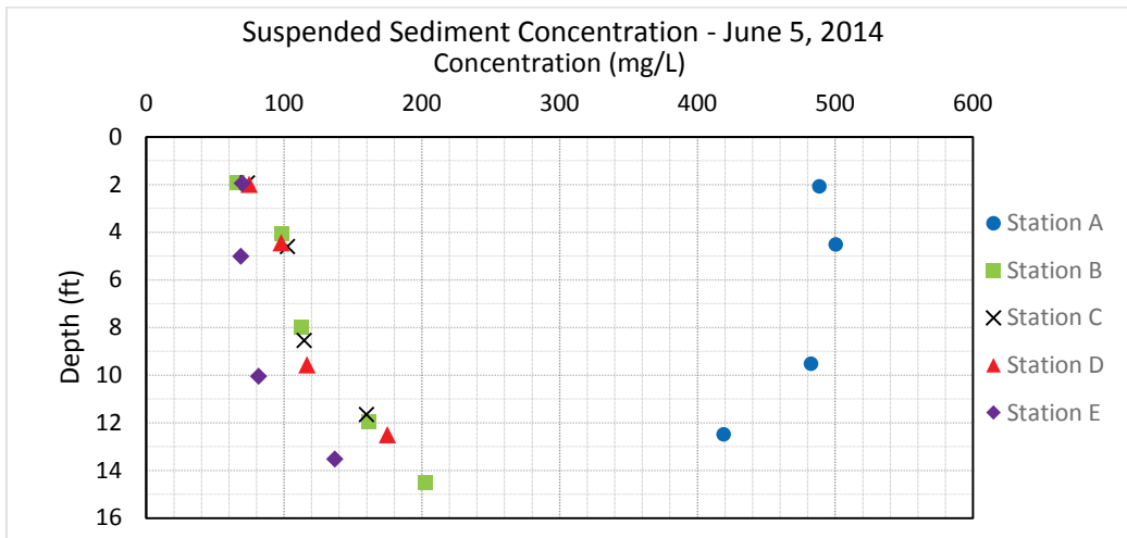
Figure 29. Suspended sediment concentration at Sioux City, IA – June 5, 2014.
