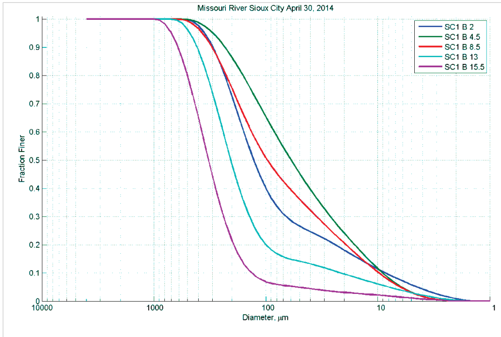
Figure 14. Particle size distribution at different depths (feet) in Station B – April 30, 2014.
