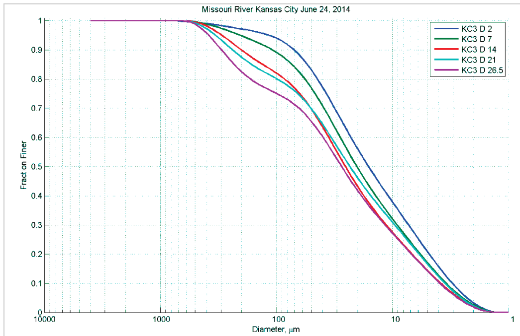
Figure 174. Particle size distribution at different depths (feet) in Station D – June 24, 2014.
