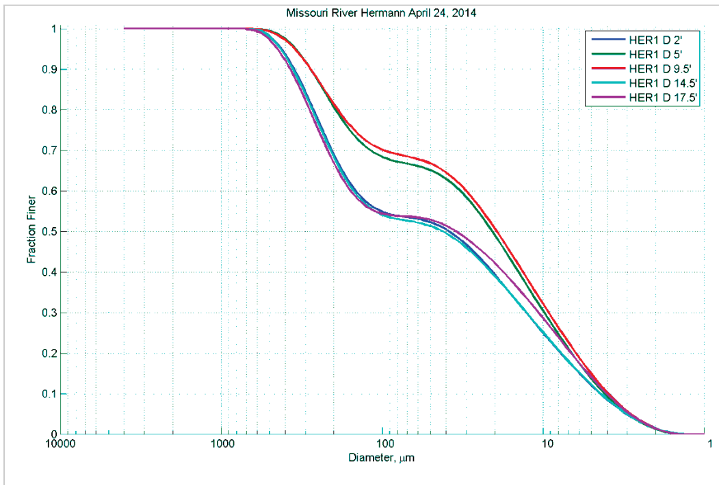
Figure 238. Particle size distribution at different depths (feet) in Station D - April 24, 2014.
