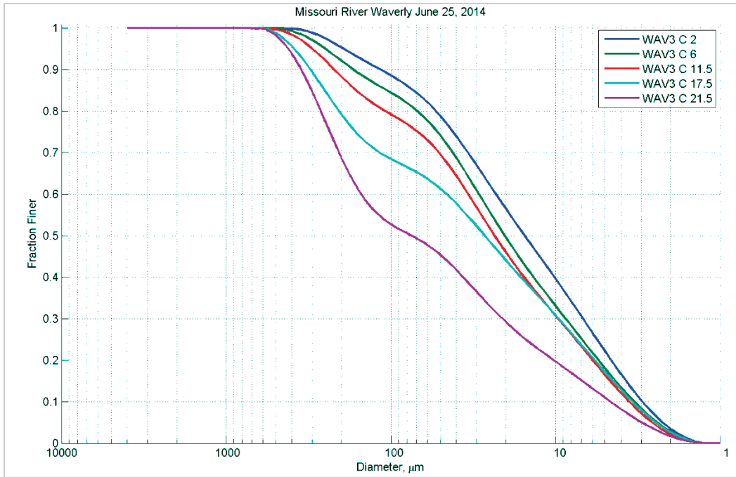
Figure 210. Particle size distribution at different depths (feet) in Station C – June 25, 2014.
