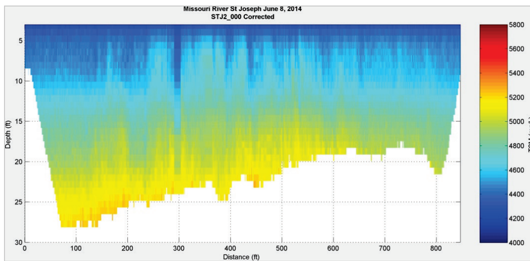
Figure 143. Suspended sediment concentration profile at St. Joseph, MO – June 8, 2014.
