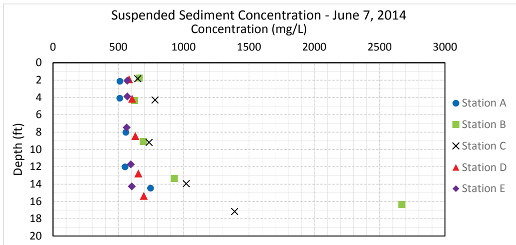
Figure 103. Suspended sediment Concentration at Nebraska City, NE – June 7, 2014.
