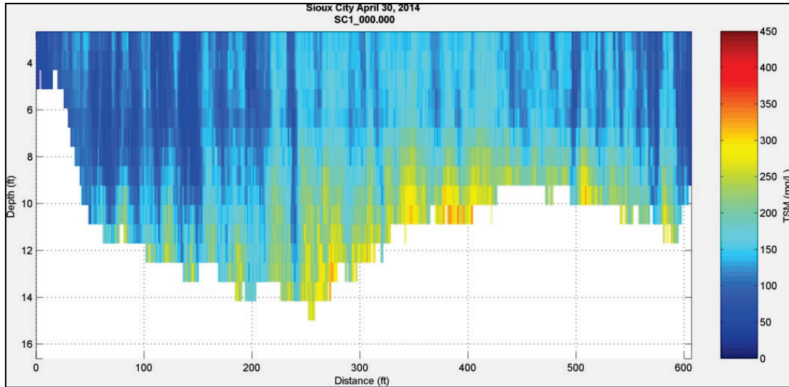
Figure 31. Suspended sediment concentration profile at Sioux City, IA – April 30, 2014.
