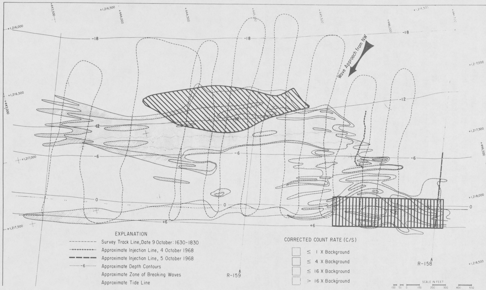
Figure 25. Comparison of tagged sand dispersal patterns. The base map is the RIST survey of 9 October 1968 with gold as the sand label. The rectangular area in lower right, drawn to same scale as the base and positioned environmentally, represents the study by Ingle (1966) on Trancas Beach, near Los Angeles. The crudely fish shaped area in the upper center, drawn to the same scale as the base and positioned environmentally, represents tagged sand dispersal pattern reported in the study of Courtois and Monaco (1969); elapsed time of the study approximately 30 days
