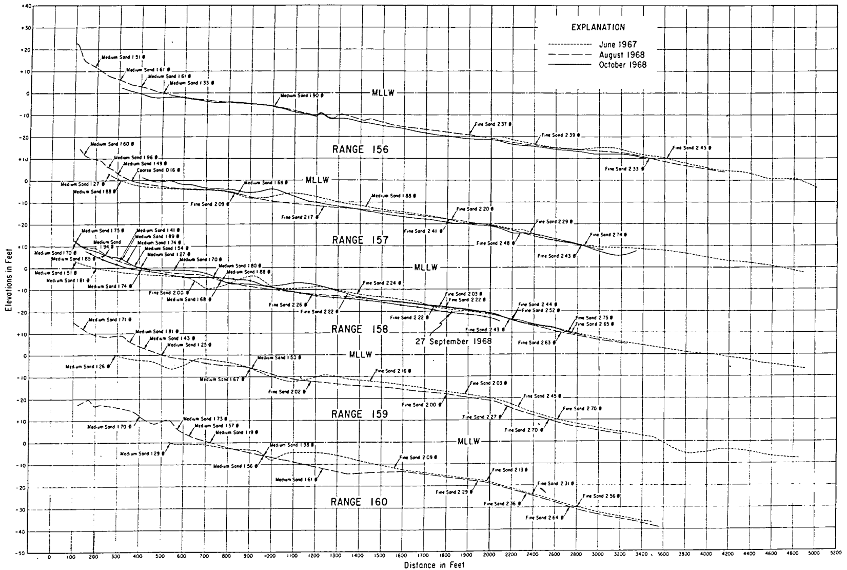
Figure 9. Profiles normal to the shore. Horizontal distances are from off-set hubs, not the main turning points. Sand characteristics are phi mean; samples collected at time of profiling.
