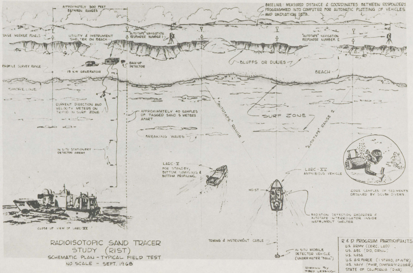
Figure 10. Schematic illustration of RIST tracing operations.
