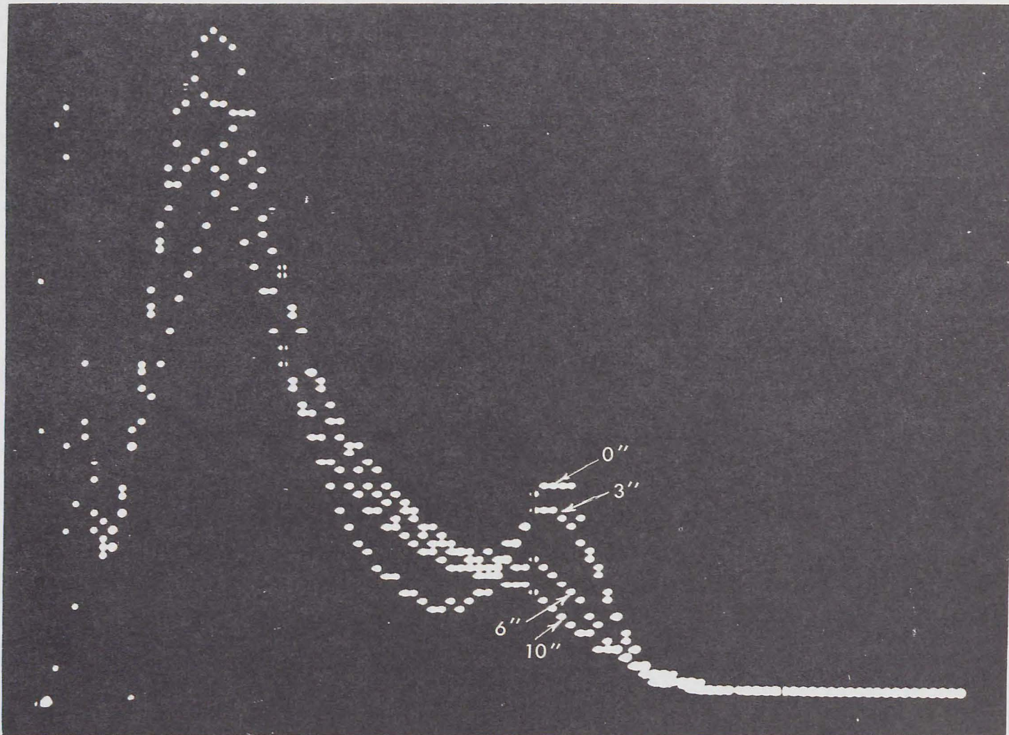
Figure 24. Changes in radioactive gold 198-199 spectrum resulting from burial by non-radioactive (dead) sand. Numbers indicate overburden thickness.
