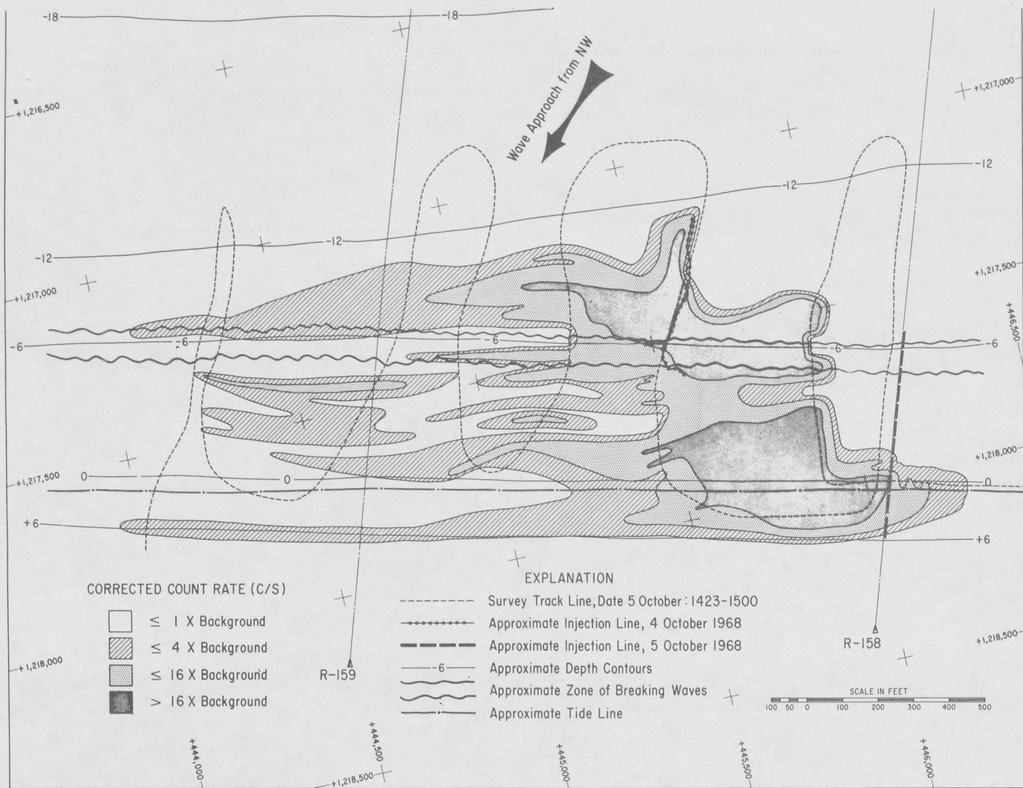
Figure 20. Dispersal pattern of gold-tagged sand observed approximately 1 hour after the pattern depicted in Figure 19.
