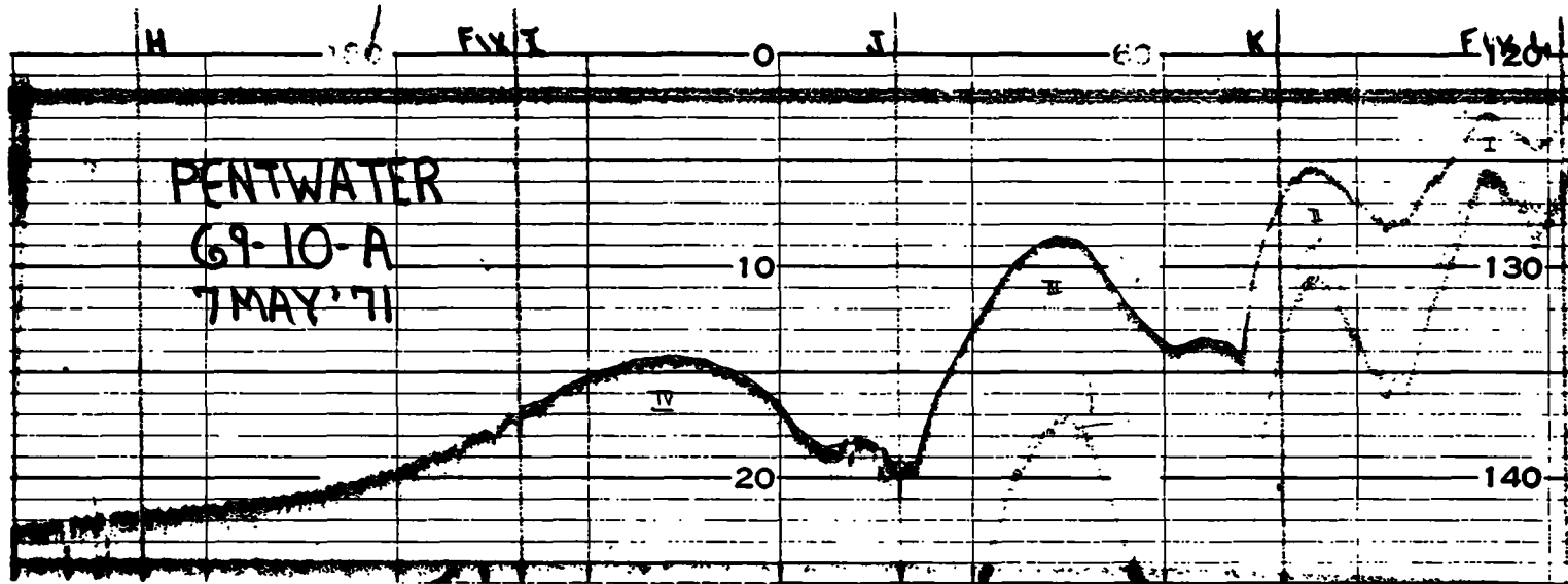
Figure 14. Bathogram with field notations. Note that limited wave distortion is on a scale completely distinct from undulations of the bottom caused by the presence of longshore bars.
