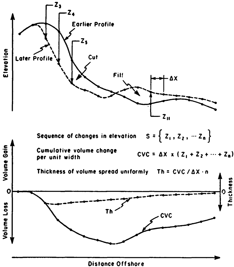
Figure 12. Schematic diagram of volume change calculations.
