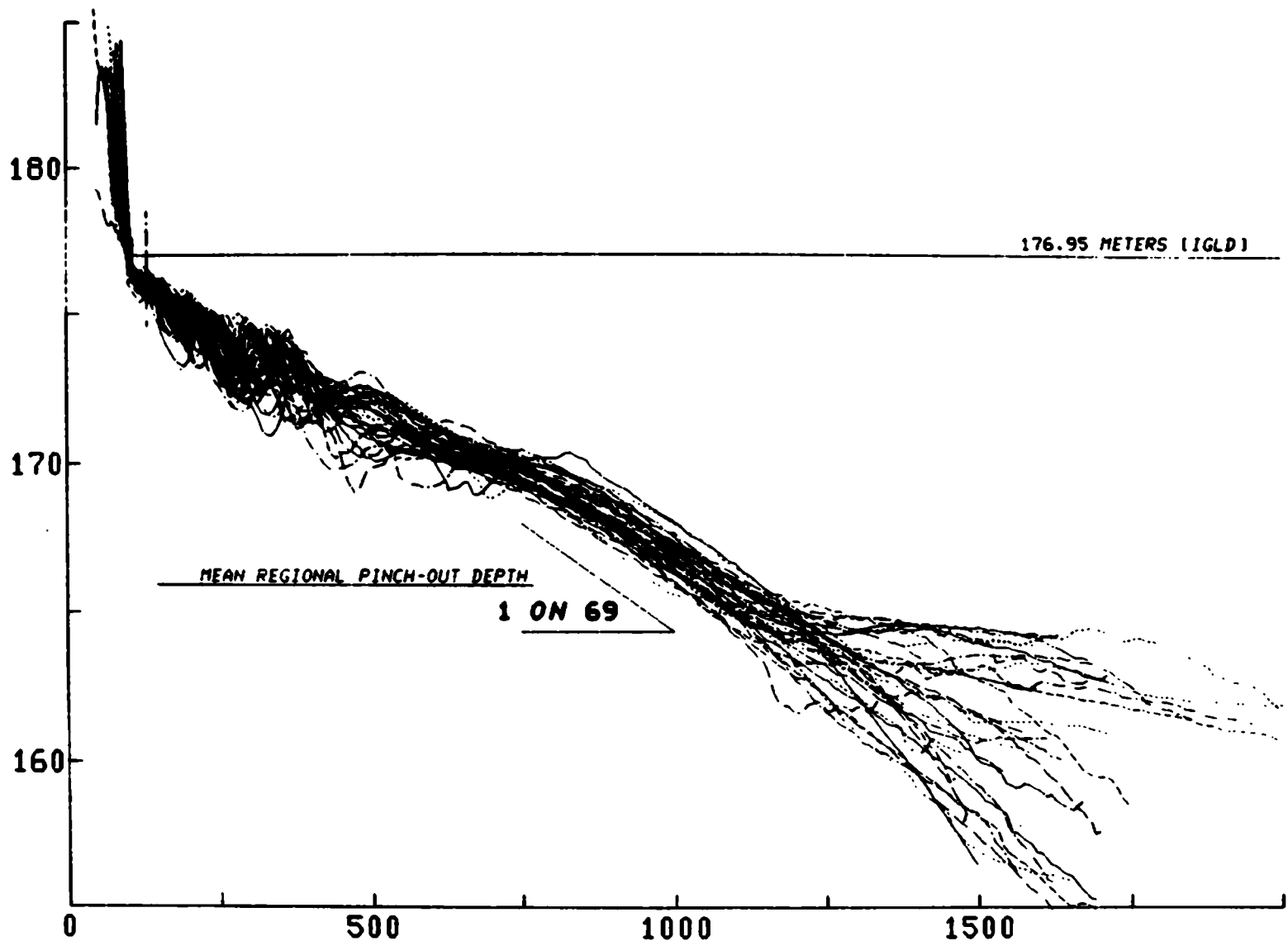
Figure 25. A composite of all profiles as surveyed in 1975. The divergence in profile shapes within the barred zone and again farther offshore contrasts with a constancy in slope across an area from about 750 to 1,100 meters from the shore reference line. The presence and the angle of slope of this area fit the concept of a trailing edge left behind as the profile retreated, in response to not just the recent rise in lake level, but to a persistent submergence of this shore over thousands of years as the outlet to the north rose faster than the remainder of the Lake Michigan basin.
