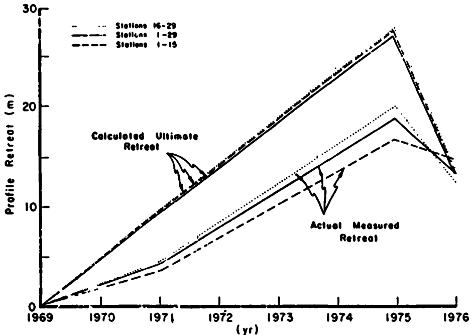
Figure 20. Calculated versus measured retreat. The predicted ultimate retreat, in response to post-1969 changes in mean lake level, exceeded the observed retreat by more than 100 percent in 1971 and about 50 percent in 1975, presumably because the active profile had not had time to completely readjust to the higher water levels. Almost perfect agreement had developed by the time of the last survey, 3 years after the lake levels peaked.
