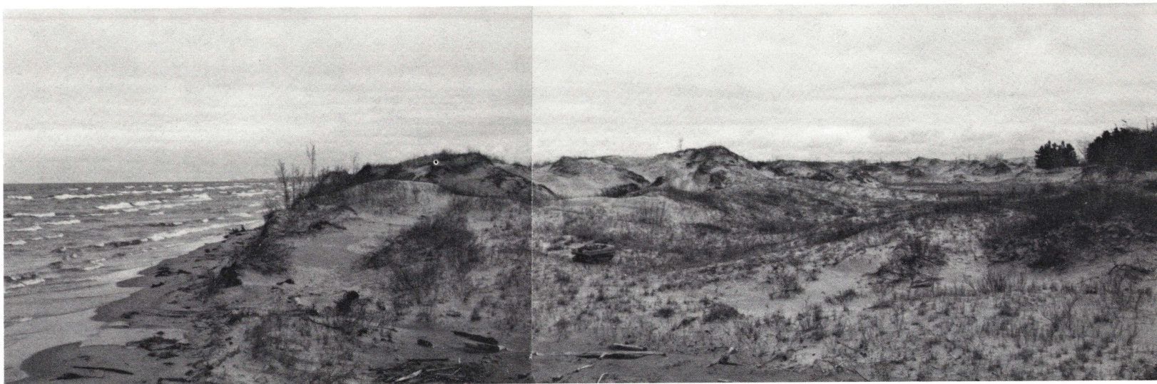
Figure 18. Shoreline scarps along Silver Lake dunes, looking northward over station 16, May 1973. Abrupt escarpments, narrow beaches, and eroding dunes characterized conditions in the early seventies. Note four-seater, all-terrain vehicle in center for scale.
