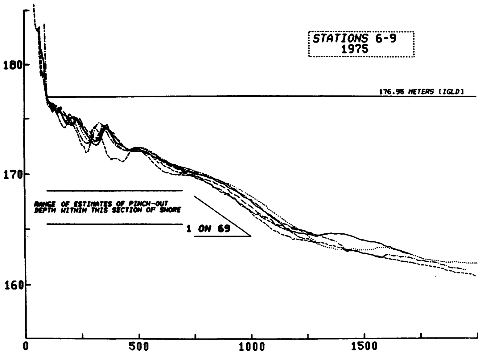
Figure 24. Adjacent profiles from various subregions within the study area. The slope of each profile can be compared with a constant reference slope of 1 on 69, which is based on the regional angle of effective profile adjustment ( \tan^{-1} x/z ) between 1969 and 1975. The maximum and minimum estimates of the pinch-out depth within each subregion are shown. Similarity among bottom slopes is evident over a wide area near the pinch-out depth.--Continued
